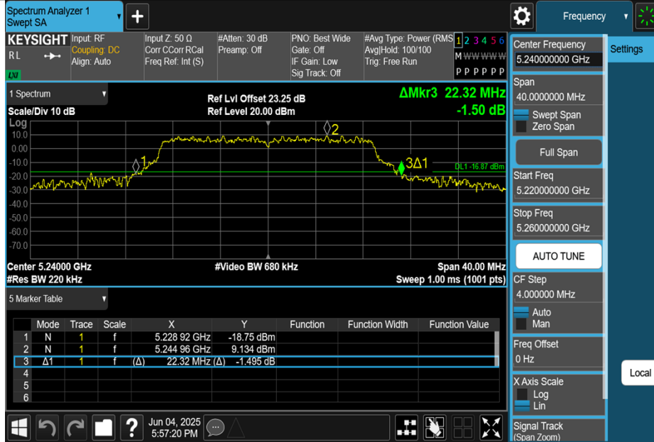
11N20MIMO-Ant2-5240
