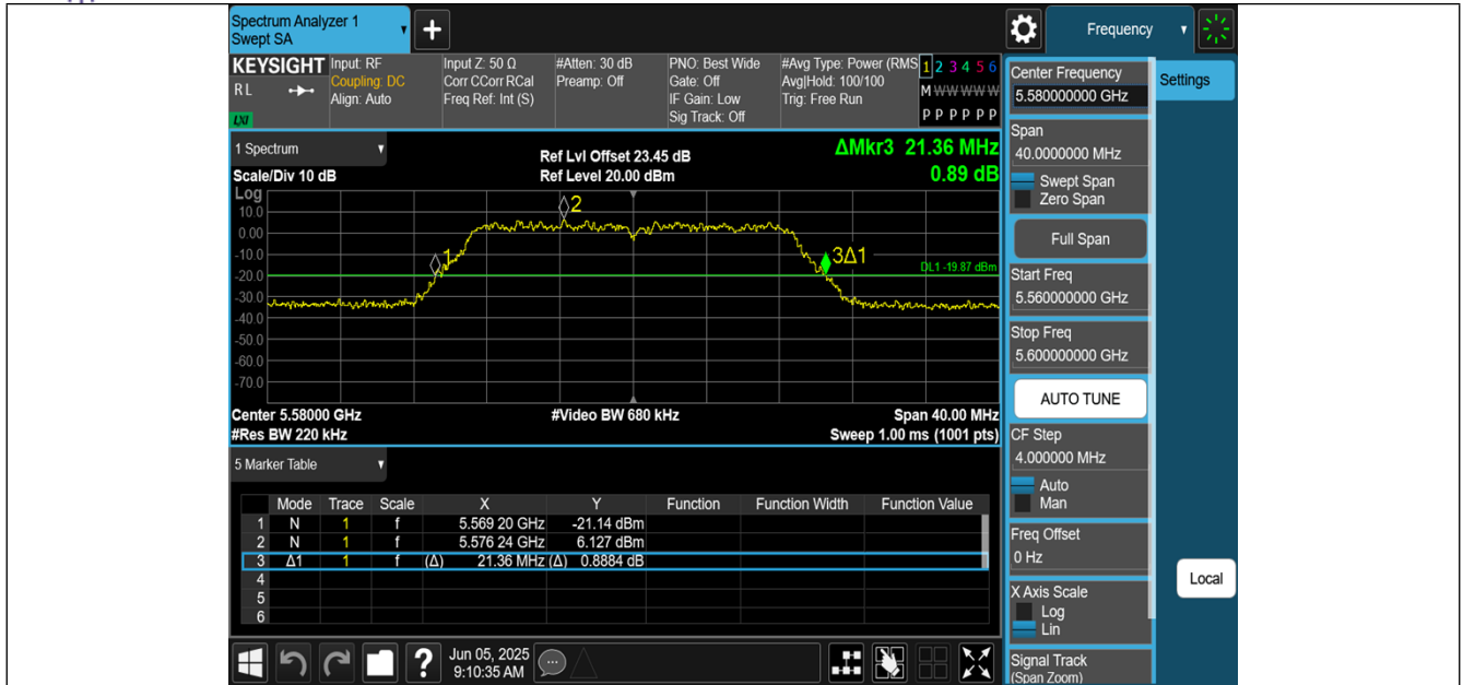
11N20MIMO-Ant0-5580
