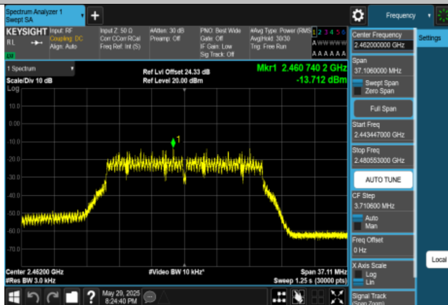
11N20MIMO-Ant3-2462-PASS
