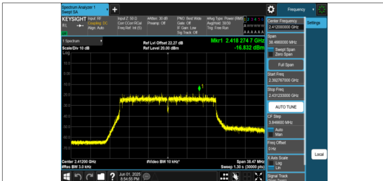
11BE20MIMO-Ant2-2412-PASS
