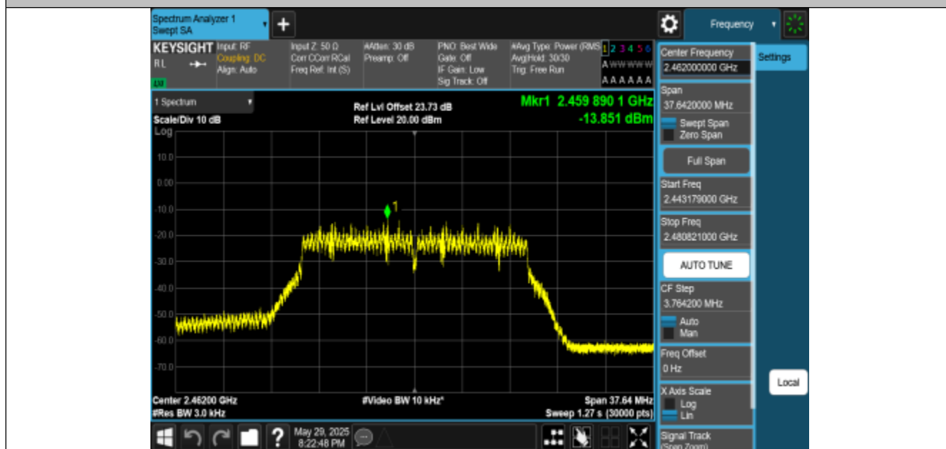
11N20MIMO-Ant1-2462-PASS
