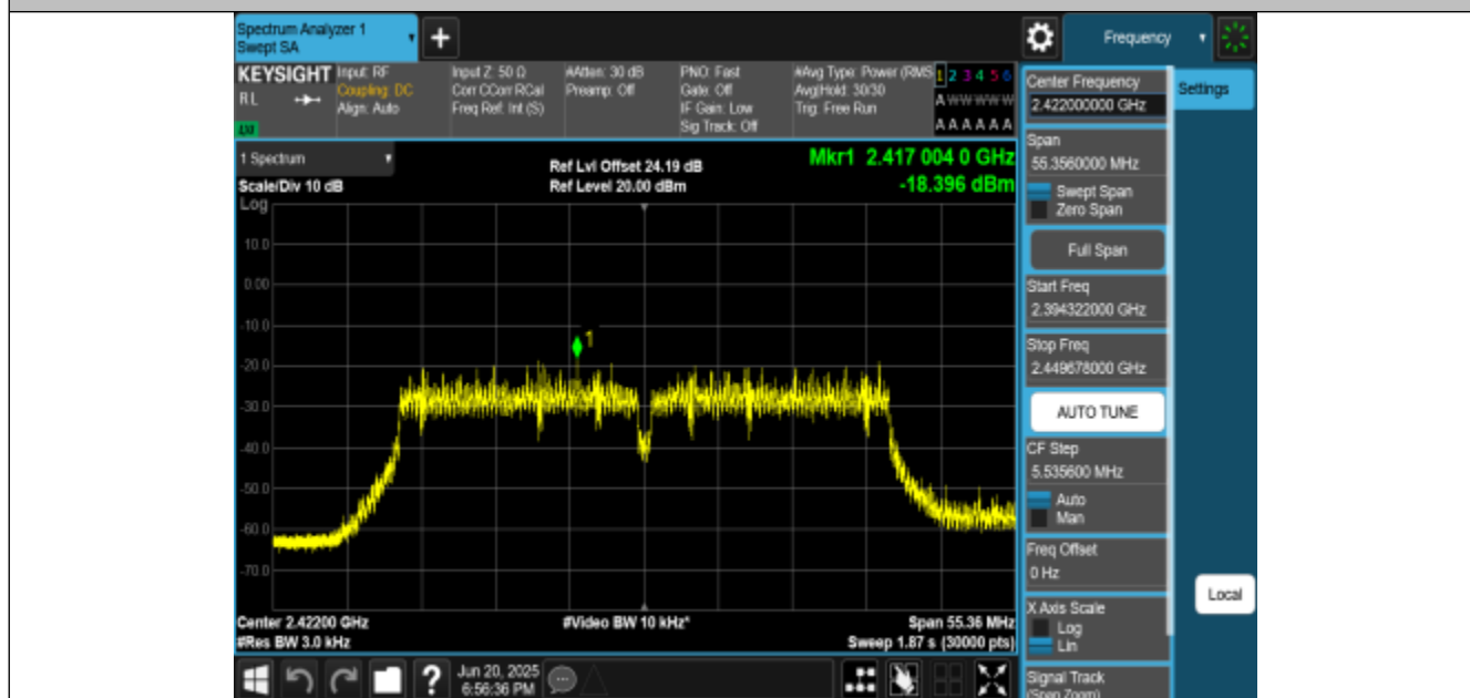
11N40MIMO-Ant1-2422-PASS
