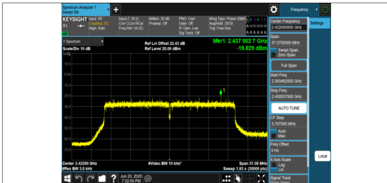
11BE40MIMO-Ant2-2422-PASS
