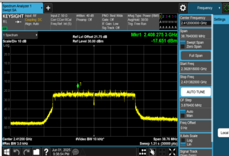
11AX20MIMO-Ant1-2412-PASS
