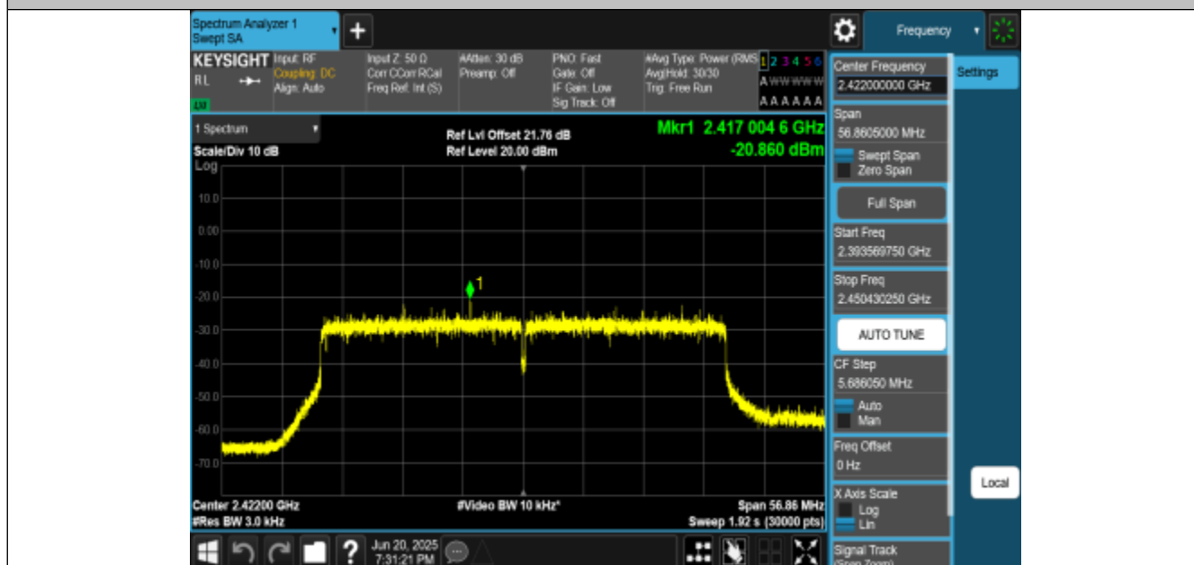
11BE40MIMO-Ant1-2422-PASS
