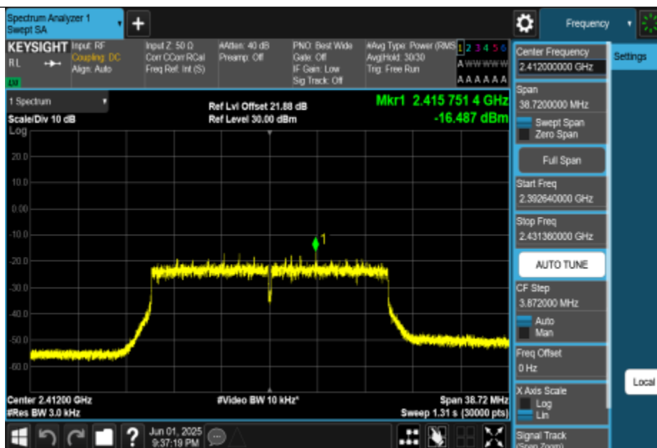
11AX20MIMO-Ant0-2412-PASS
