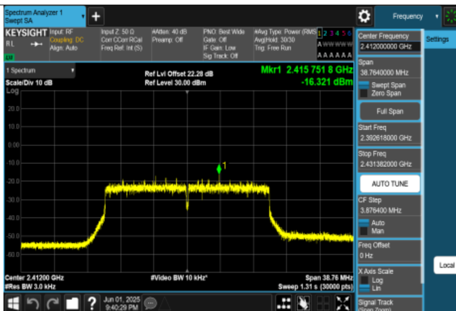
11AX20MIMO-Ant2-2412-PASS
