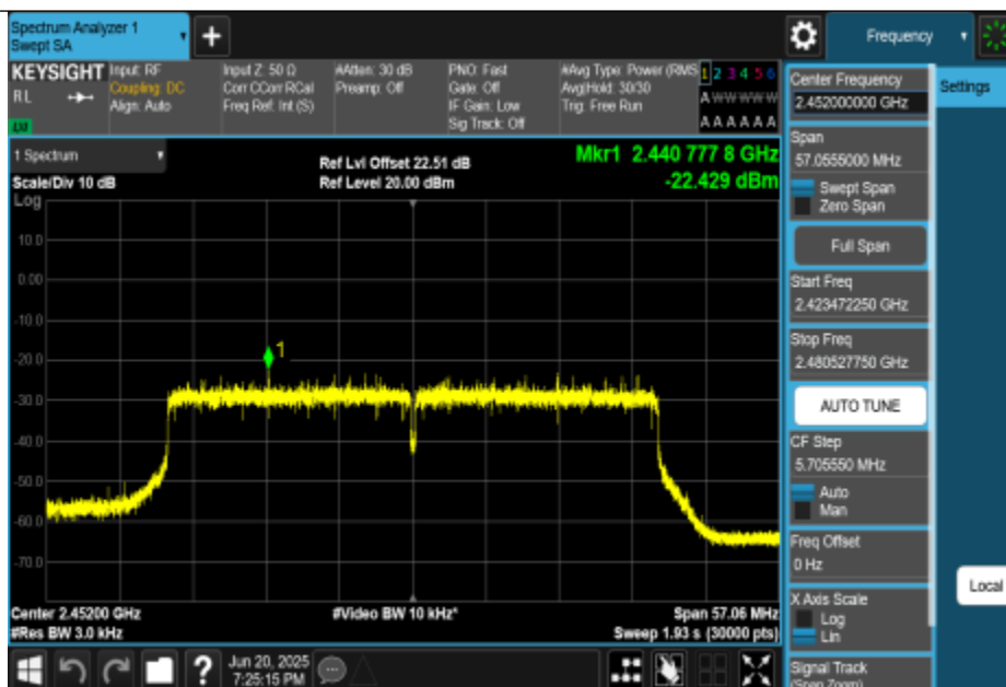
11AX40MIMO-Ant3-2452-PASS
