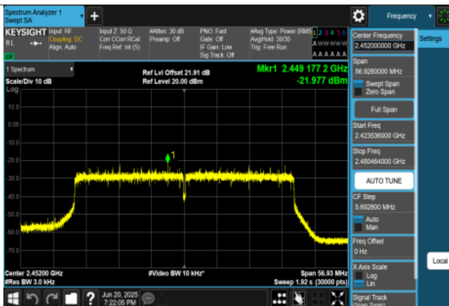
11AX40MIMO-Ant1-2452-PASS
