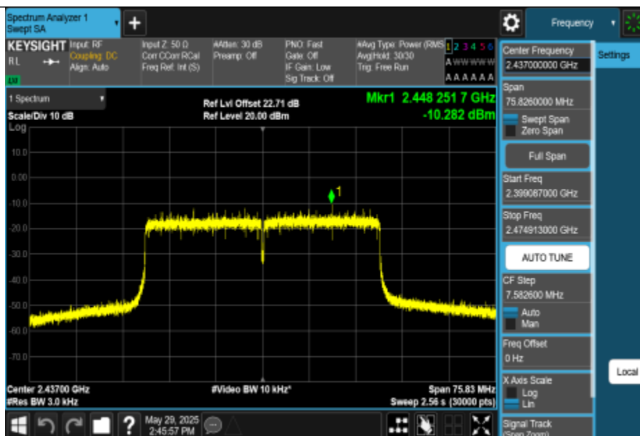
11AX40MIMO-Ant2-2437-PASS
