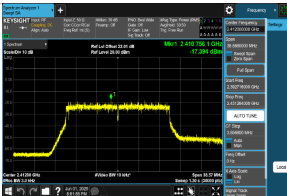
11BE20MIMO-Ant0-2412-PASS
