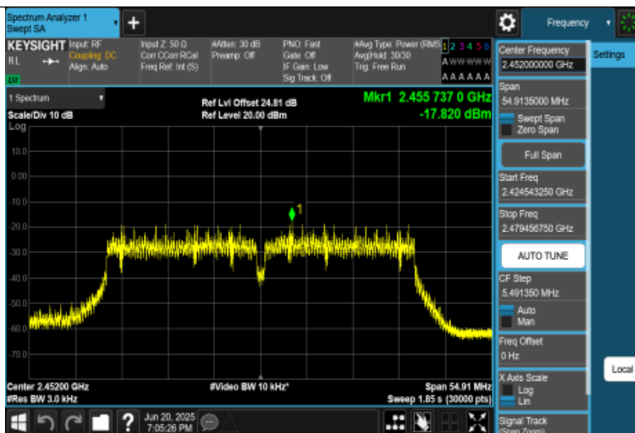
11N40MIMO-Ant2-2452-PASS
