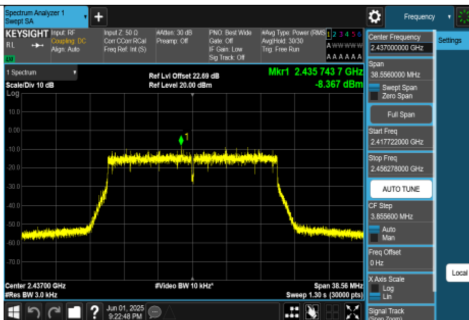
11BE20MIMO-Ant2-2437-PASS
