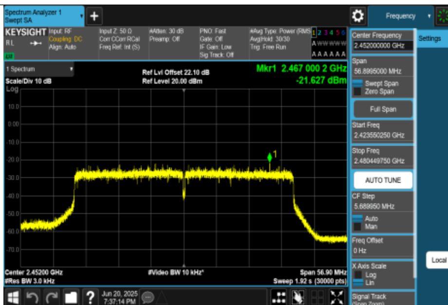
11BE40MIMO-Ant0-2452-PASS
