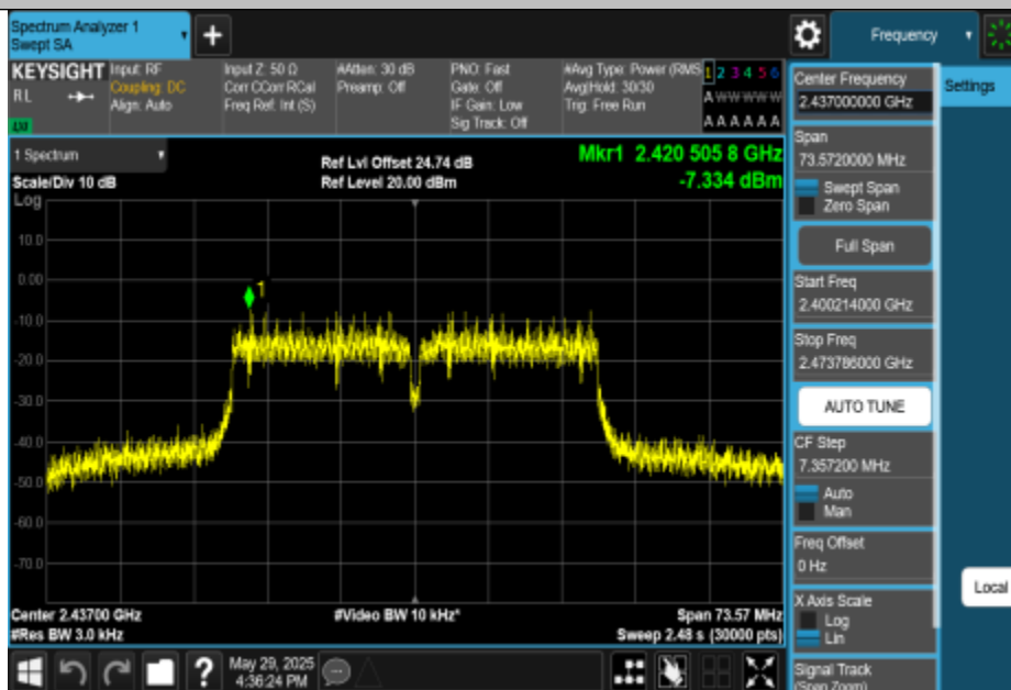
11N40MIMO-Ant3-2437-PASS
