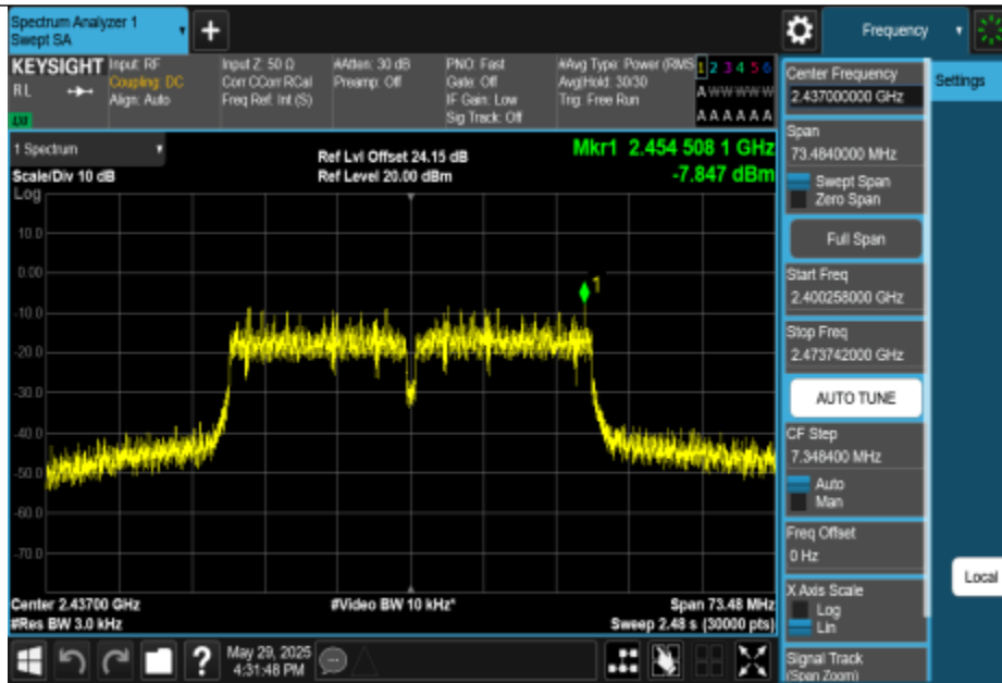
11N40MIMO-Ant0-2437-PASS
