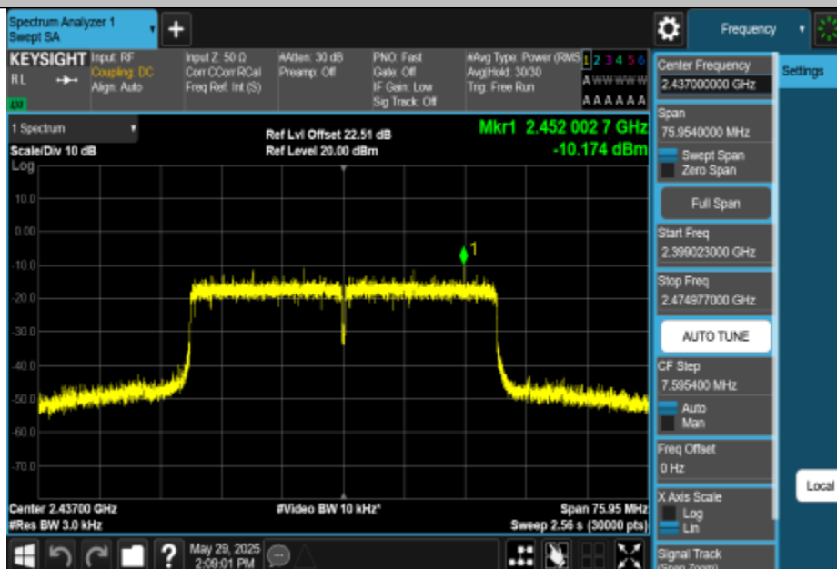
11BE40MIMO-Ant3-2437-PASS
