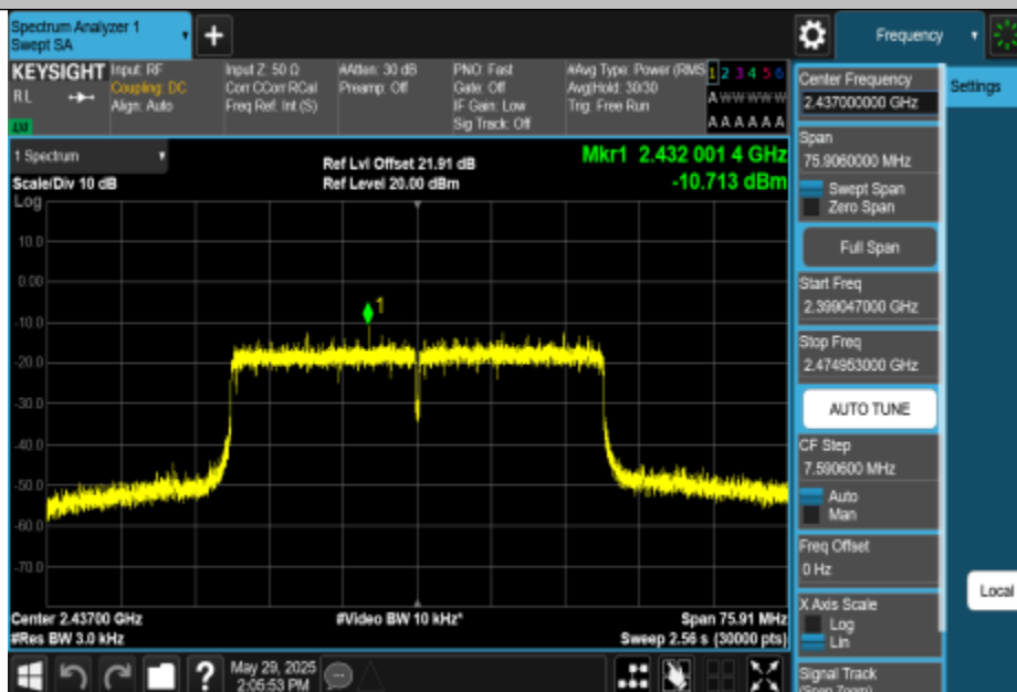
11BE40MIMO-Ant1-2437-PASS
