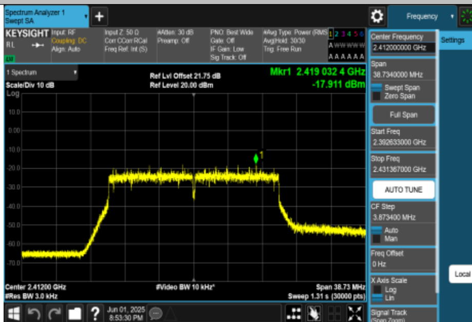
11BE20MIMO-Ant1-2412-PASS
