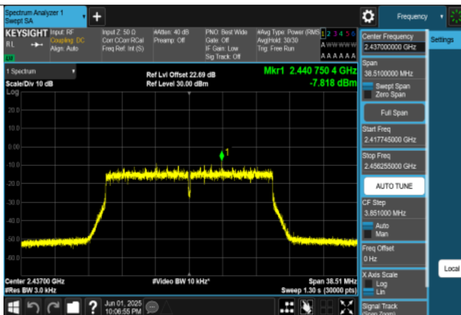
11AX20MIMO-Ant2-2437-PASS
