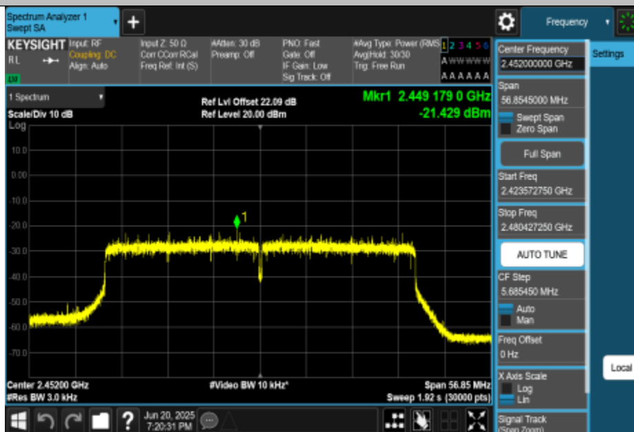
11AX40MIMO-Ant0-2452-PASS
