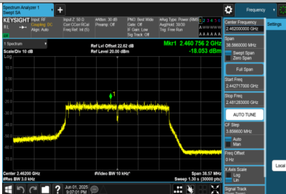
11BE20MIMO-Ant3-2462-PASS
