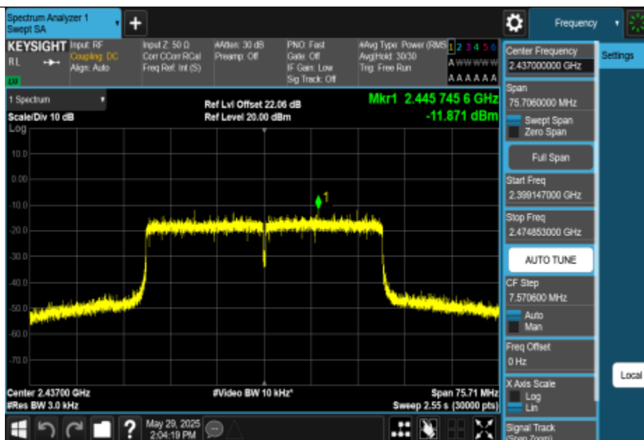
11BE40MIMO-Ant0-2437-PASS
