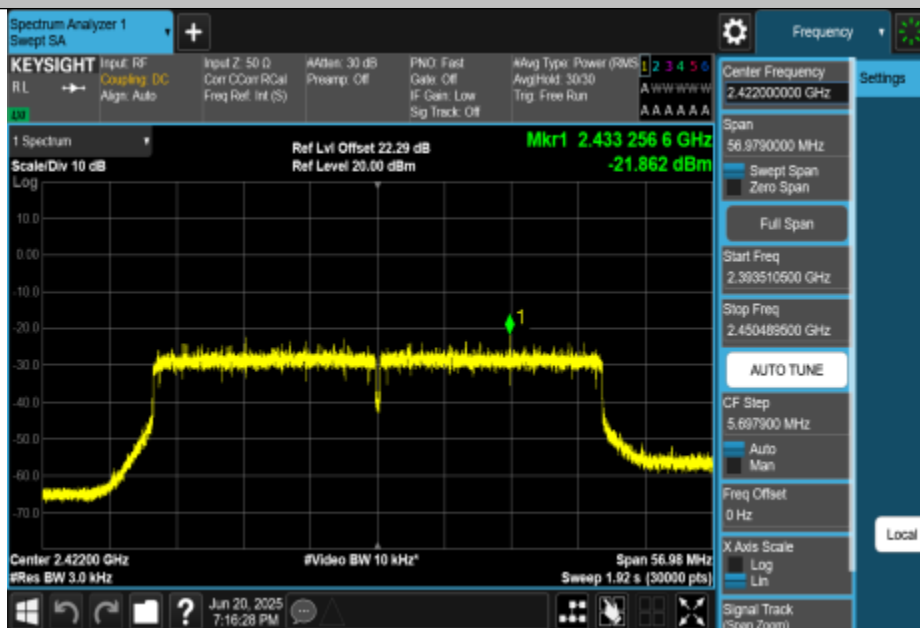
11AX40MIMO-Ant2-2422-PASS
