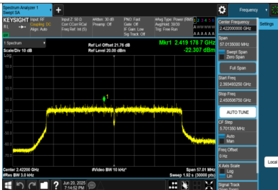
11AX40MIMO-Ant1-2422-PASS
