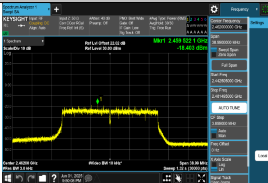
11AX20MIMO-Ant1-2462-PASS
