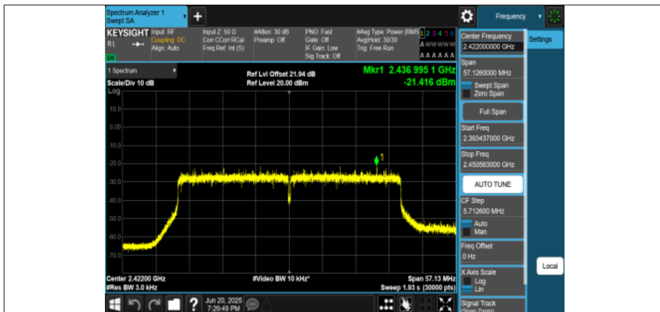
11BE40MIMO-Ant0-2422-PASS
