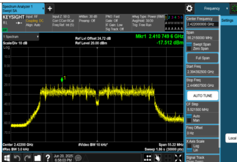
11N40MIMO-Ant2-2422-PASS
