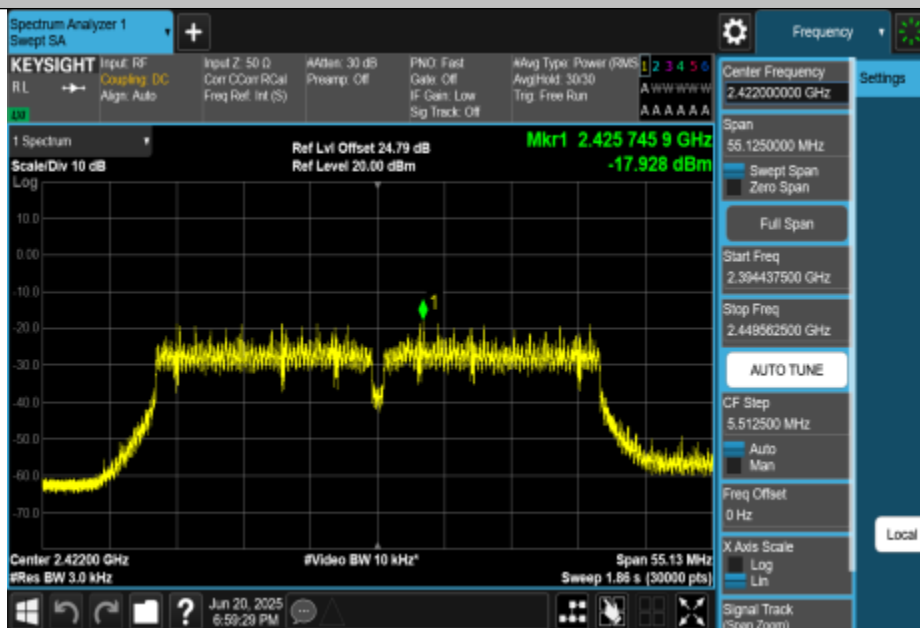
11N40MIMO-Ant3-2422-PASS
