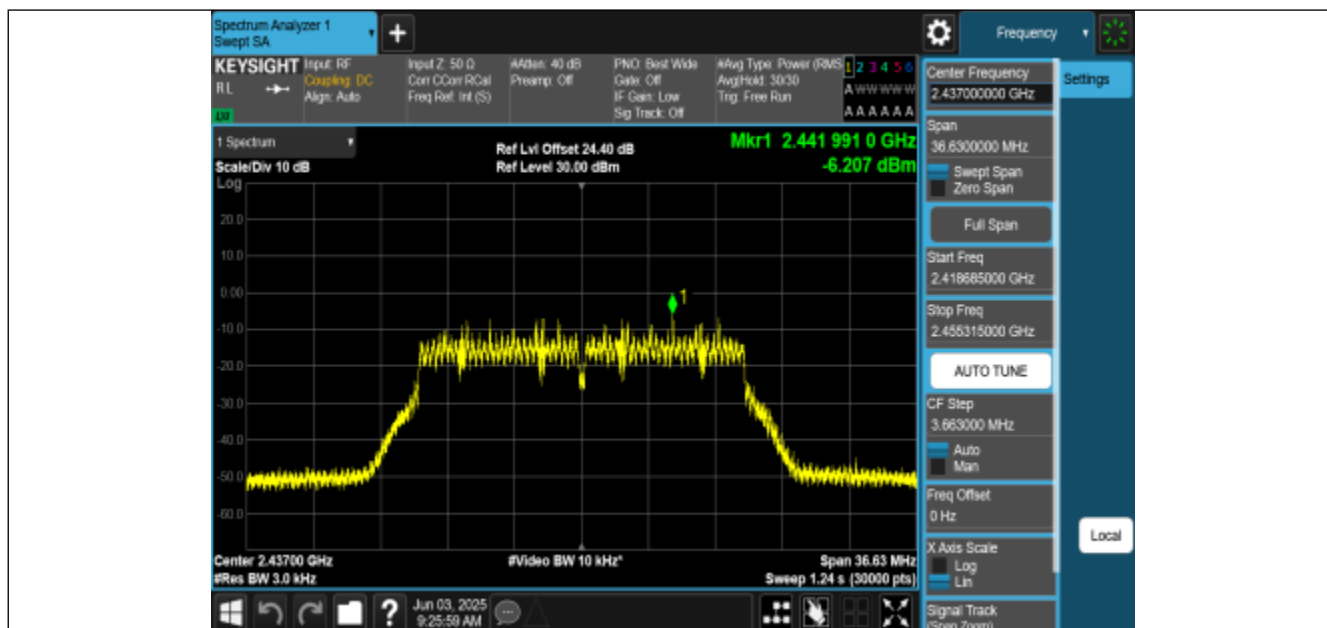
11N20MIMO-Ant2-2437-PASS
