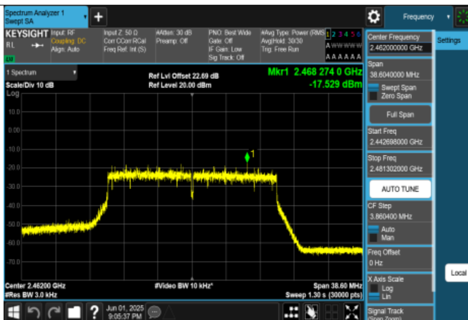
11BE20MIMO-Ant2-2462-PASS
