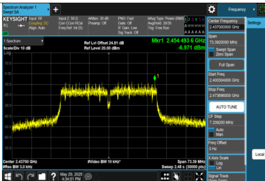
11N40MIMO-Ant2-2437-PASS
