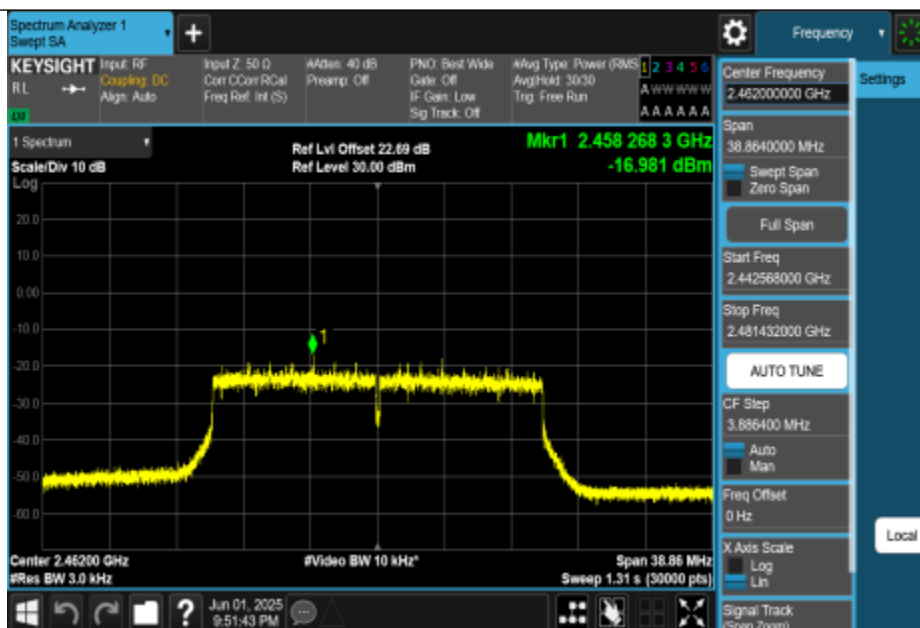
11AX20MIMO-Ant2-2462-PASS
