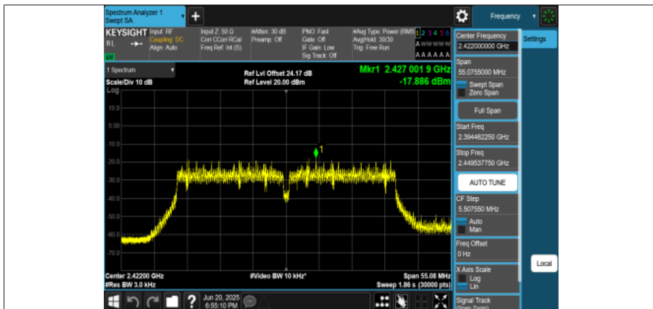
11N40MIMO-Ant0-2422-PASS
