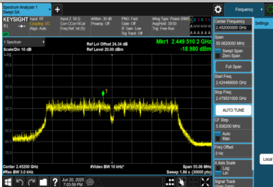
11N40MIMO-Ant1-2452-PASS
