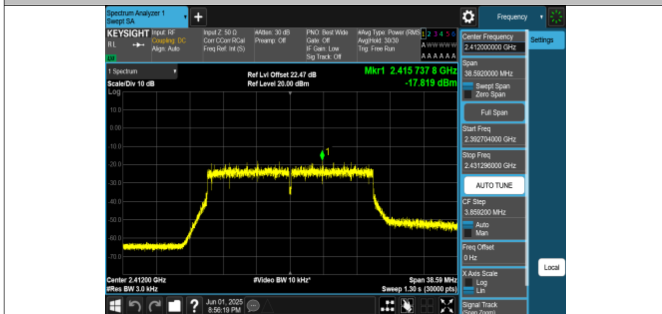
11BE20MIMO-Ant3-2412-PASS
