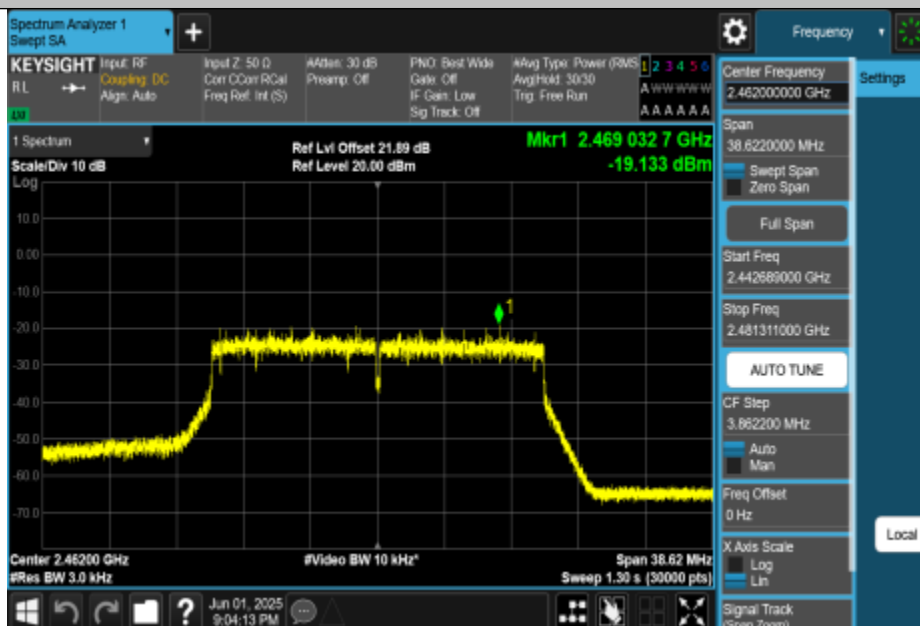
11BE20MIMO-Ant1-2462-PASS
