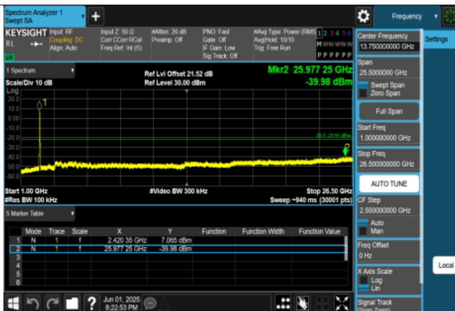
11BE40MIMO-Ant0-2437-1000~26500-PASS
