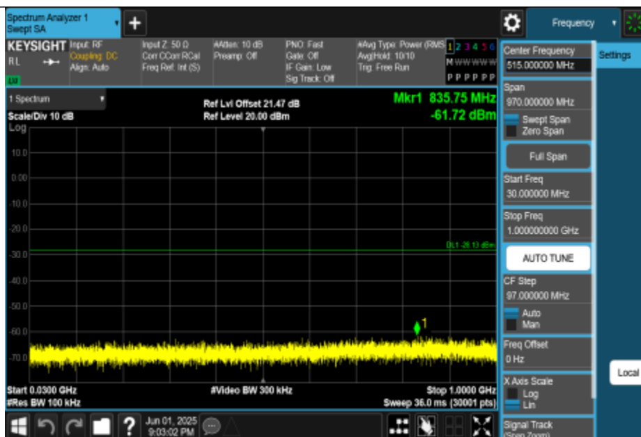
11BE20MIMO-Ant0-2462-30~1000-PASS
