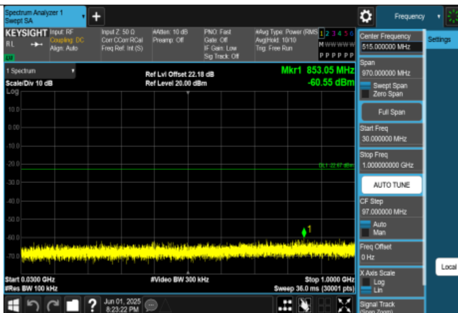
11BE40MIMO-Ant2-2437-30~1000-PASS
