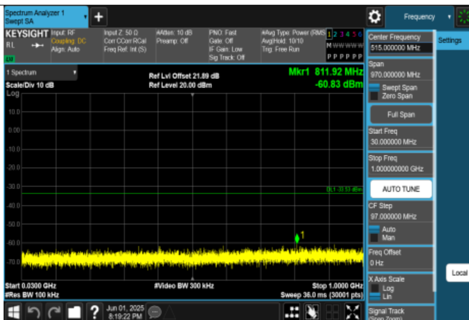
11BE40MIMO-Ant2-2422-30~1000-PASS
