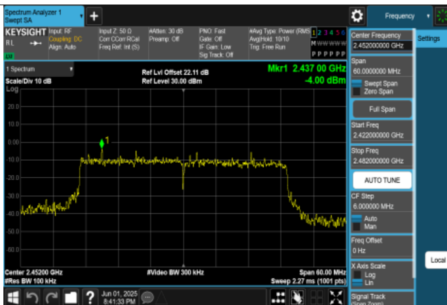
11BE40MIMO-Ant3-2452-0~Reference-PASS
