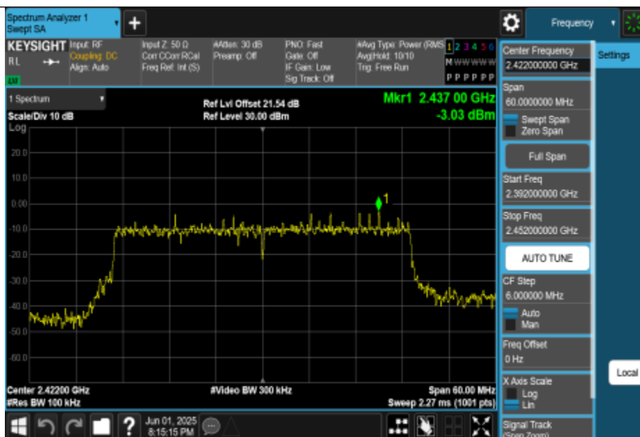
11BE40MIMO-Ant0-2422-0~Reference-PASS
