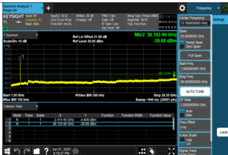
11BE40MIMO-Ant2-2422-1000~26500-PASS
