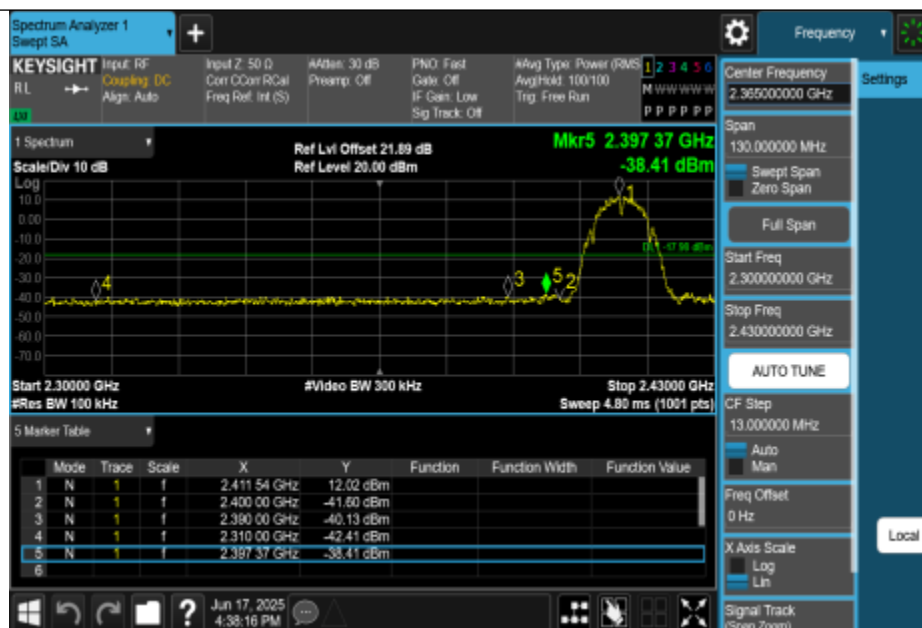
11B-CDD-Ant2-2412-PASS
