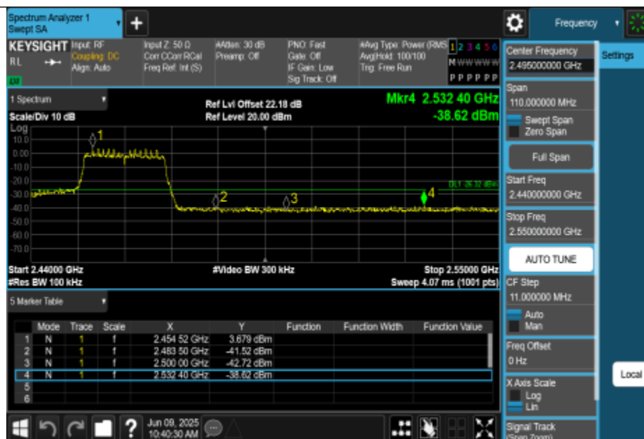
11AX20MIMO-Ant2-2462-PASS
