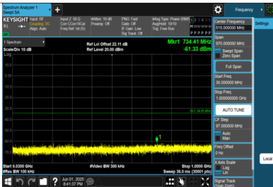
11BE40MIMO-Ant3-2452-30~1000-PASS
