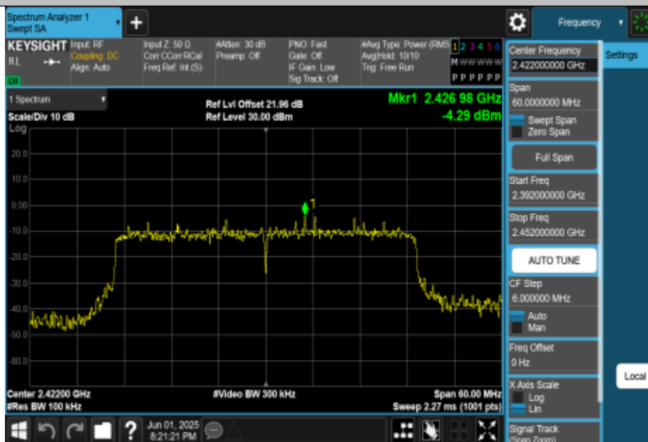
11BE40MIMO-Ant3-2422-0~Reference-PASS
