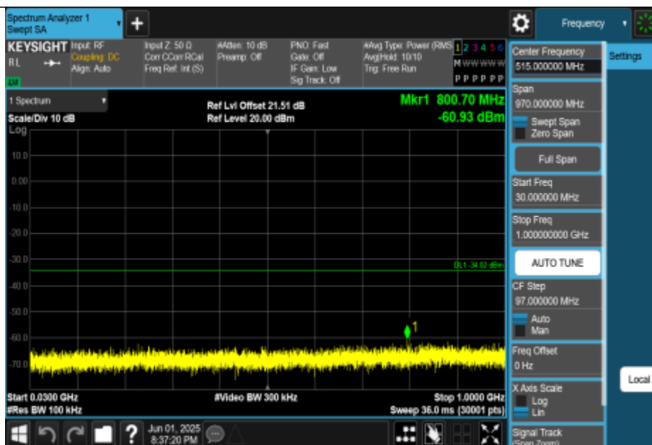
11BE40MIMO-Ant1-2452-30~1000-PASS
