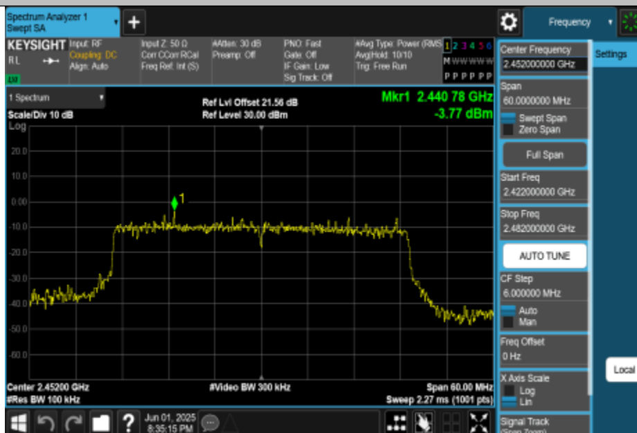
11BE40MIMO-Ant0-2452-0~Reference-PASS
