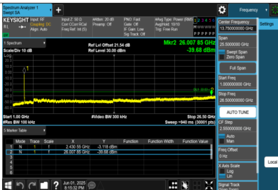
11BE40MIMO-Ant0-2422-1000~26500-PASS
