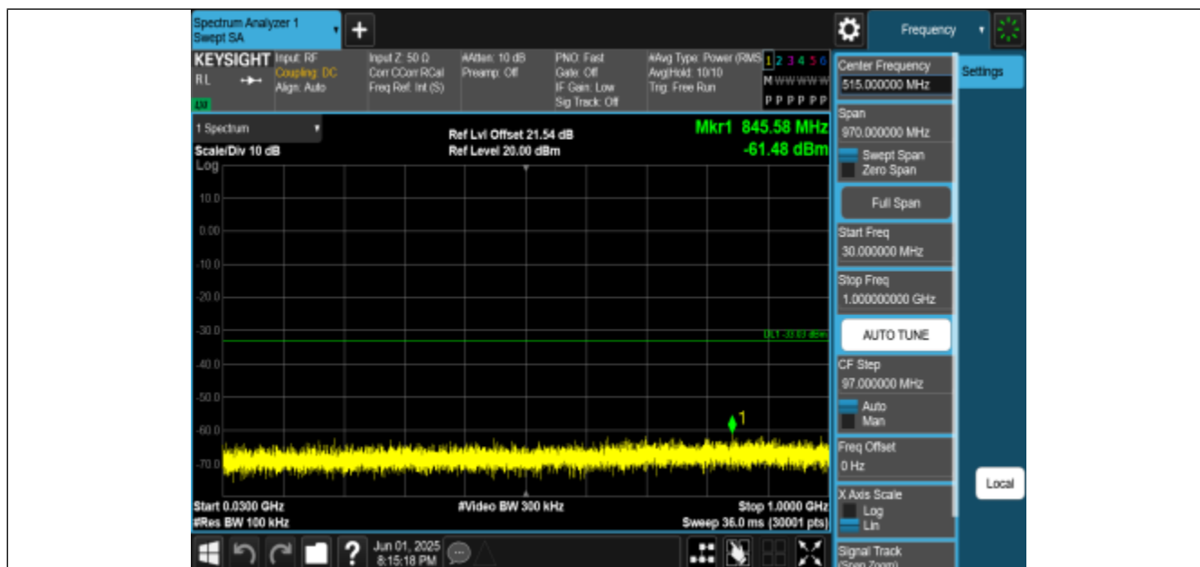
11BE40MIMO-Ant0-2422-30~1000-PASS
