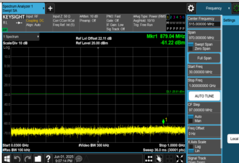
11BE20MIMO-Ant3-2462-30~1000-PASS
