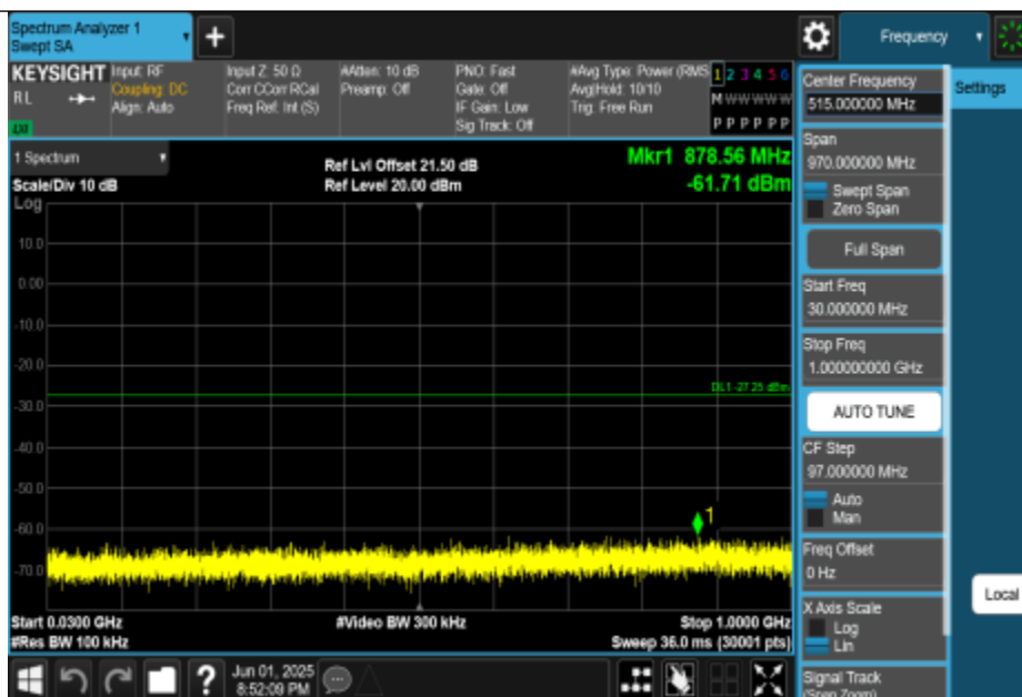
11BE20MIMO-Ant0-2412-30~1000-PASS
