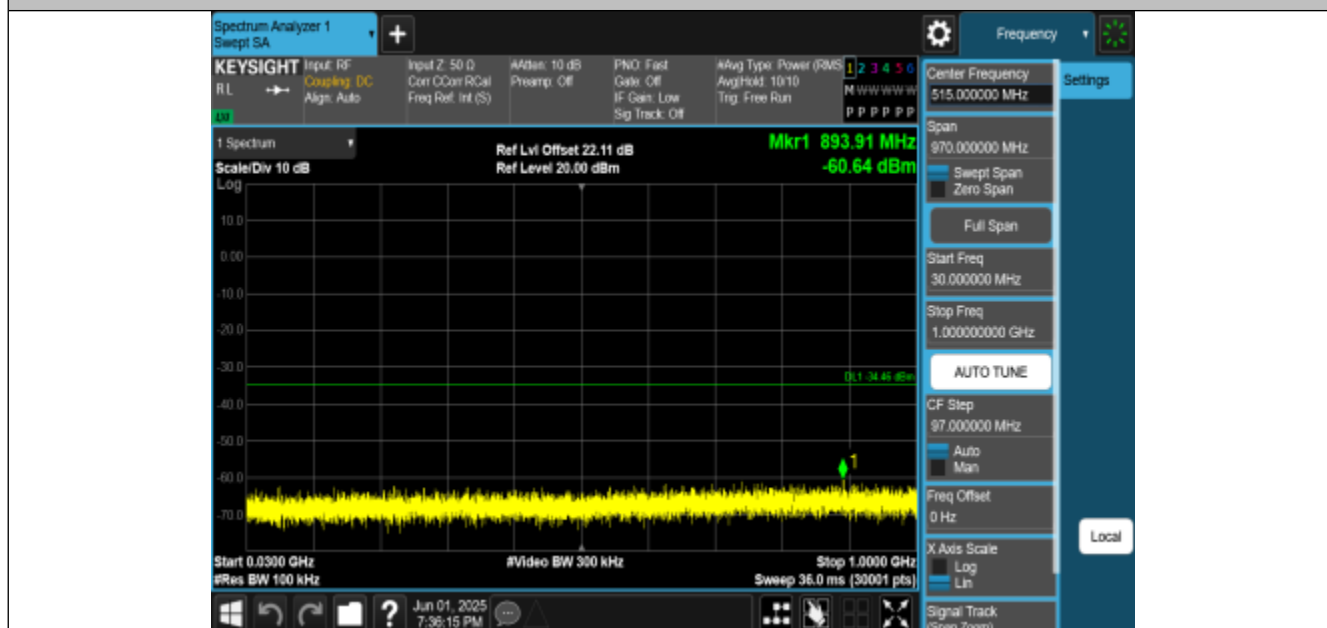
11AX40MIMO-Ant3-2452-30~1000-PASS
