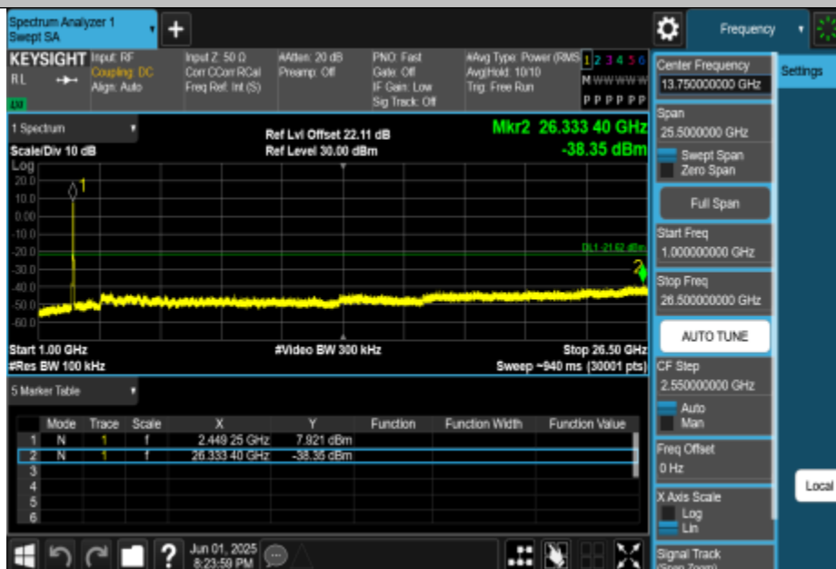
11BE40MIMO-Ant3-2437-1000~26500-PASS
