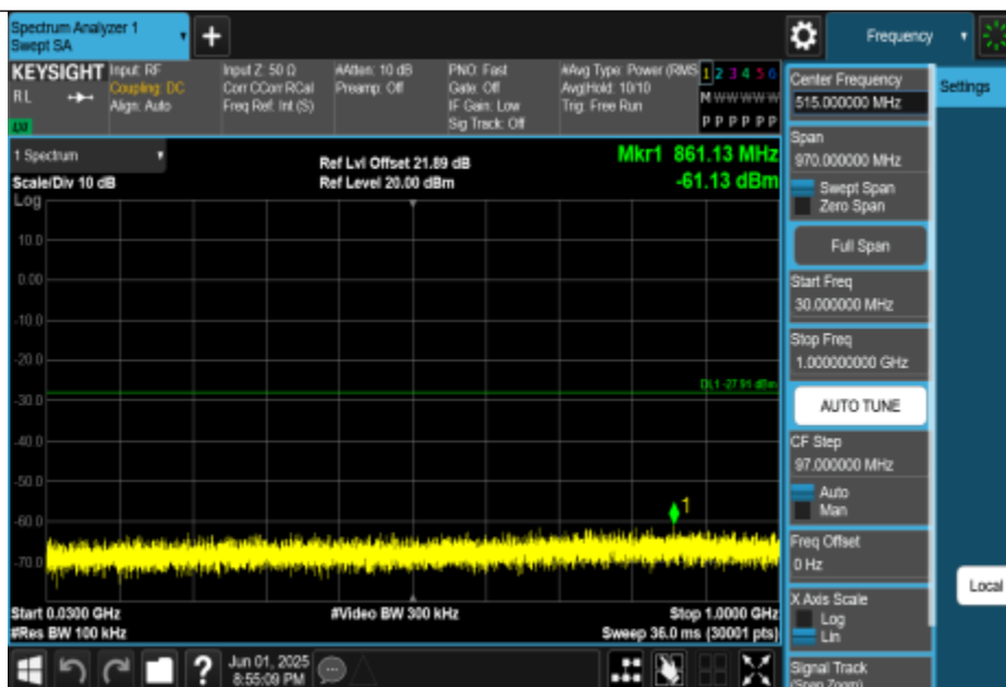
11BE20MIMO-Ant2-2412-30~1000-PASS
