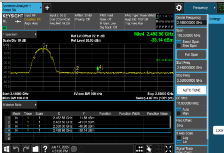
11B-CDD-Ant3-2462-PASS
