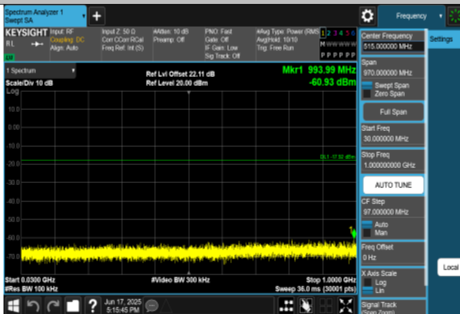
11N20MIMO-Ant3-2437-30~1000-PASS
