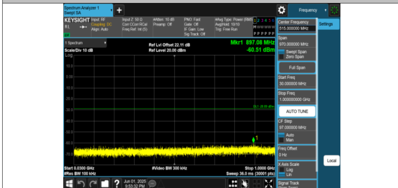
11AX20MIMO-Ant3-2462-30~1000-PASS
