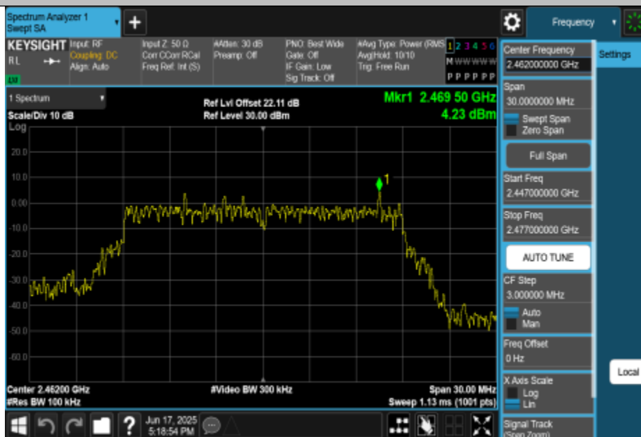
11N20MIMO-Ant3-2462-0~Reference-PASS
