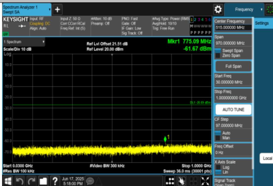
11N20MIMO-Ant1-2462-30~1000-PASS
