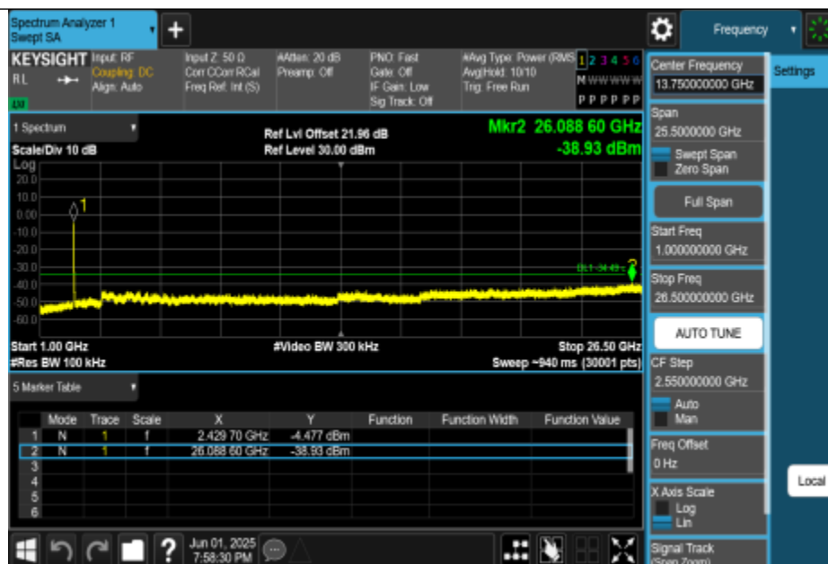
11AX40MIMO-Ant3-2422-1000~26500-PASS
