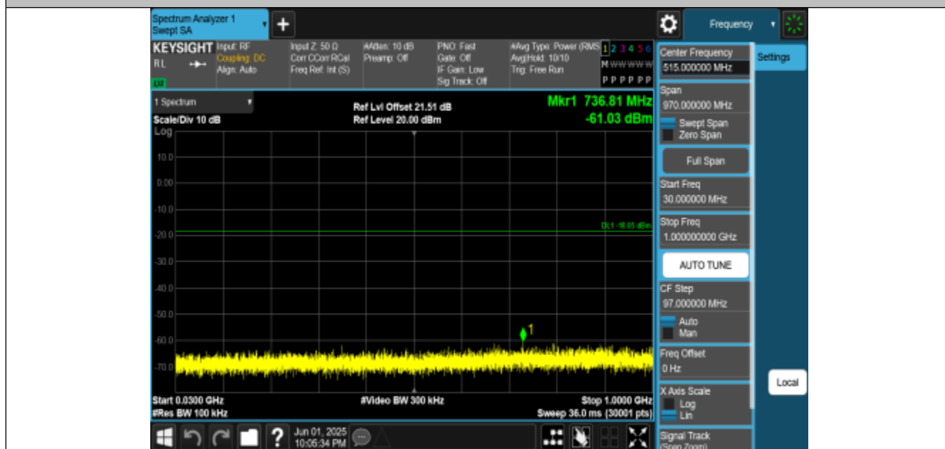
11AX20MIMO-Ant1-2437-30~1000-PASS
