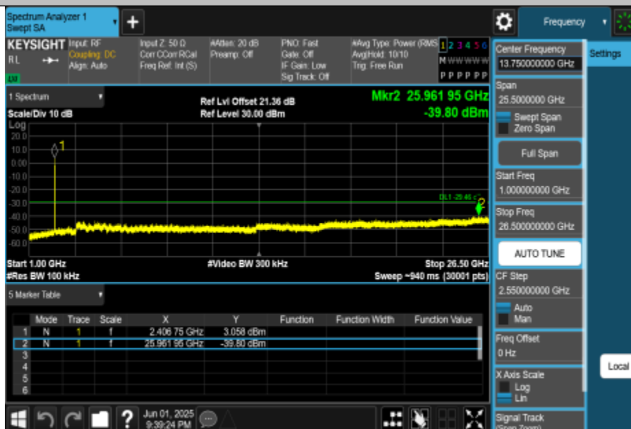
11AX20MIMO-Ant1-2412-1000~26500-PASS
