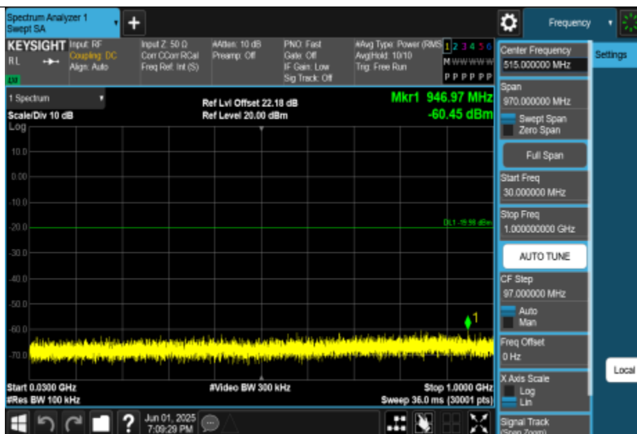
11N40MIMO-Ant2-2437-30~1000-PASS
