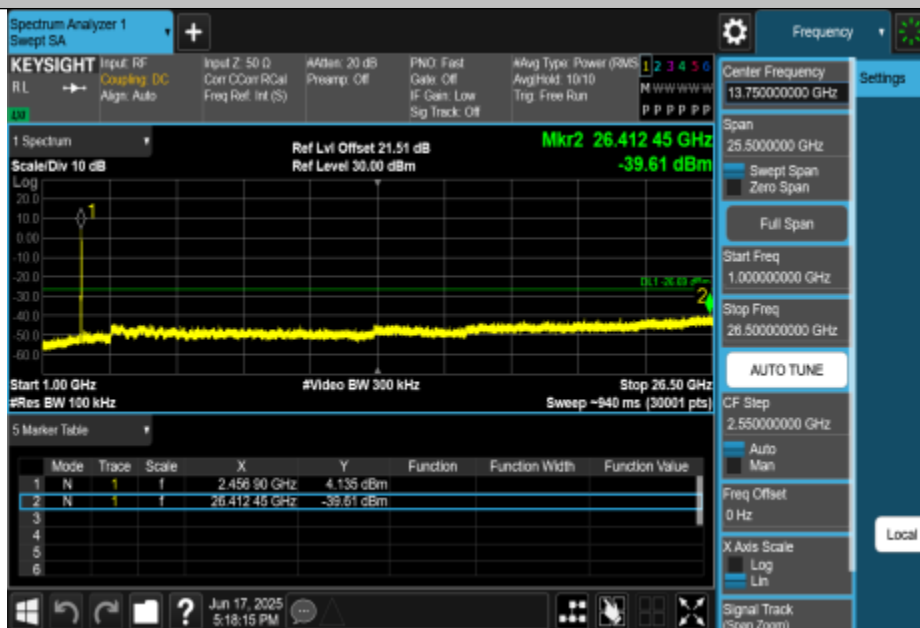
11N20MIMO-Ant1-2462-1000~26500-PASS
