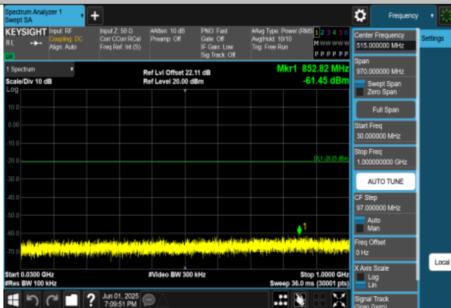
11N40MIMO-Ant3-2437-30~1000-PASS
