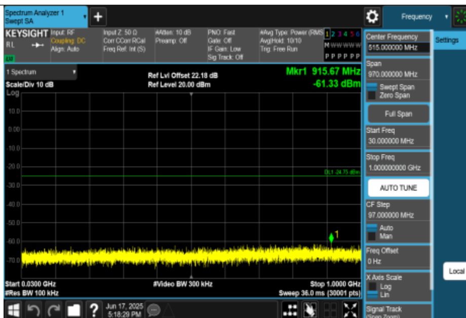
11N20MIMO-Ant2-2462-30~1000-PASS
