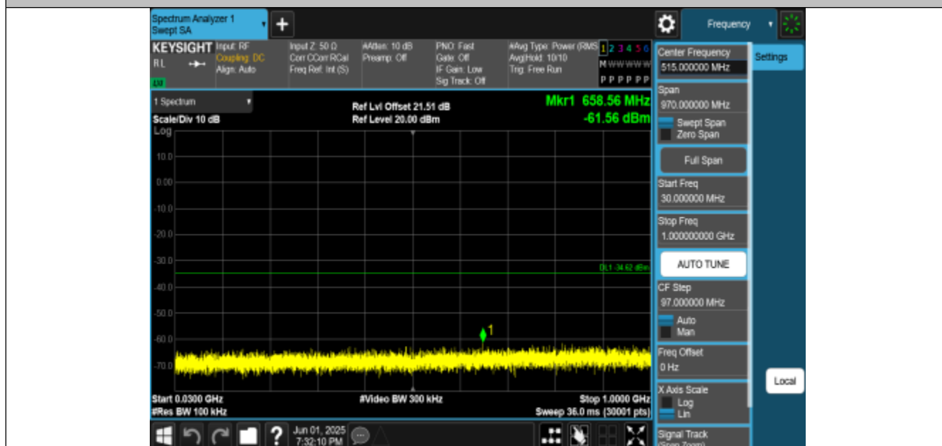
11AX40MIMO-Ant1-2452-30~1000-PASS
