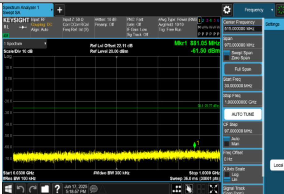
11N20MIMO-Ant3-2462-30~1000-PASS
