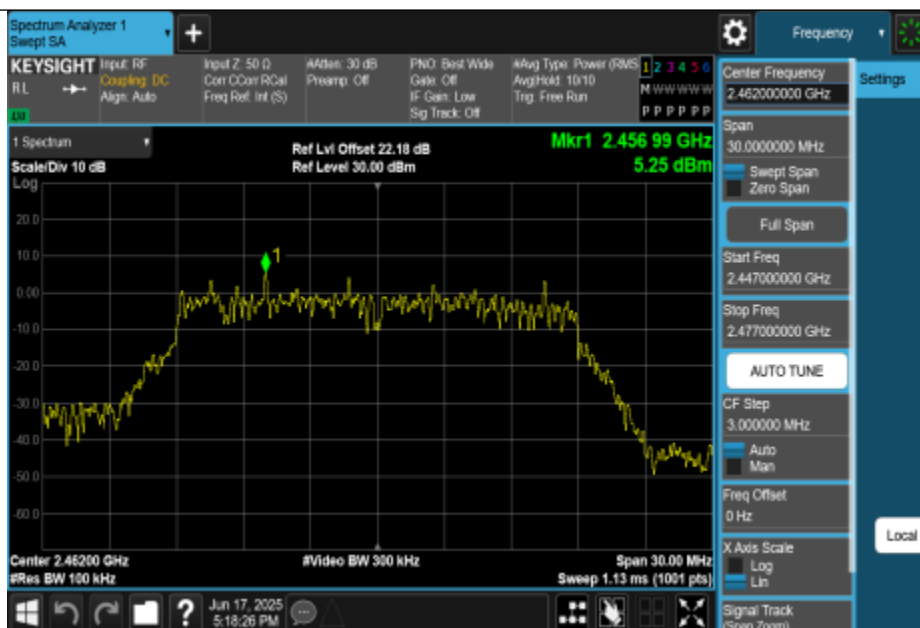
11N20MIMO-Ant2-2462-0~Reference-PASS
