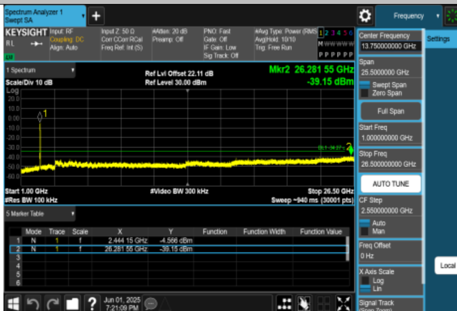
11N40MIMO-Ant3-2452-1000~26500-PASS
