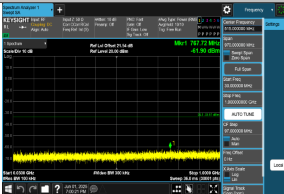
11N40MIMO-Ant0-2422-30~1000-PASS
