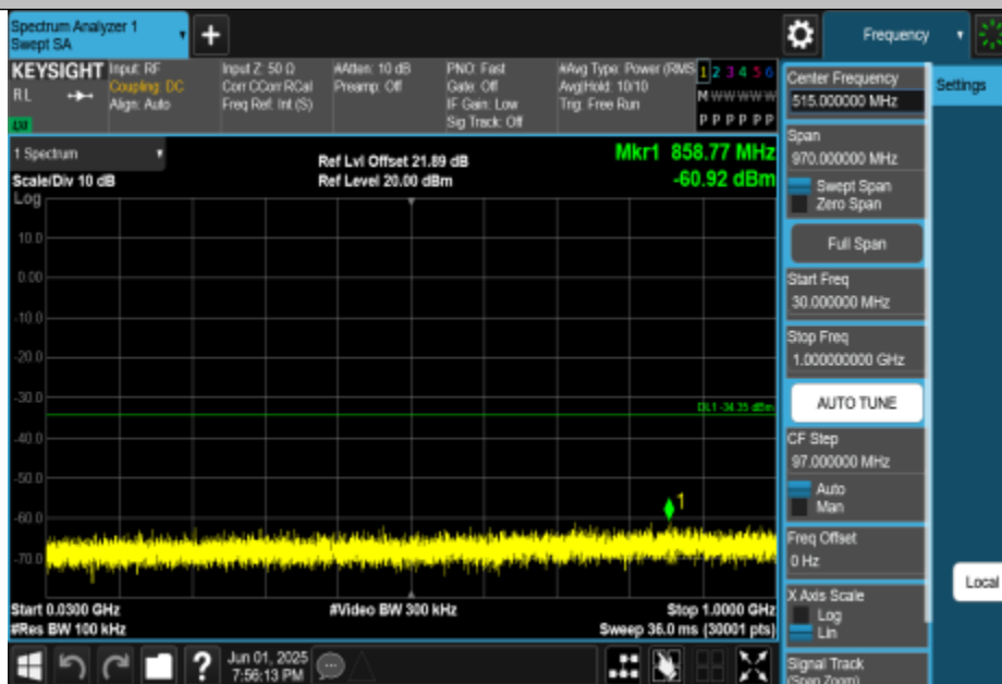
11AX40MIMO-Ant2-2422-30~1000-PASS
