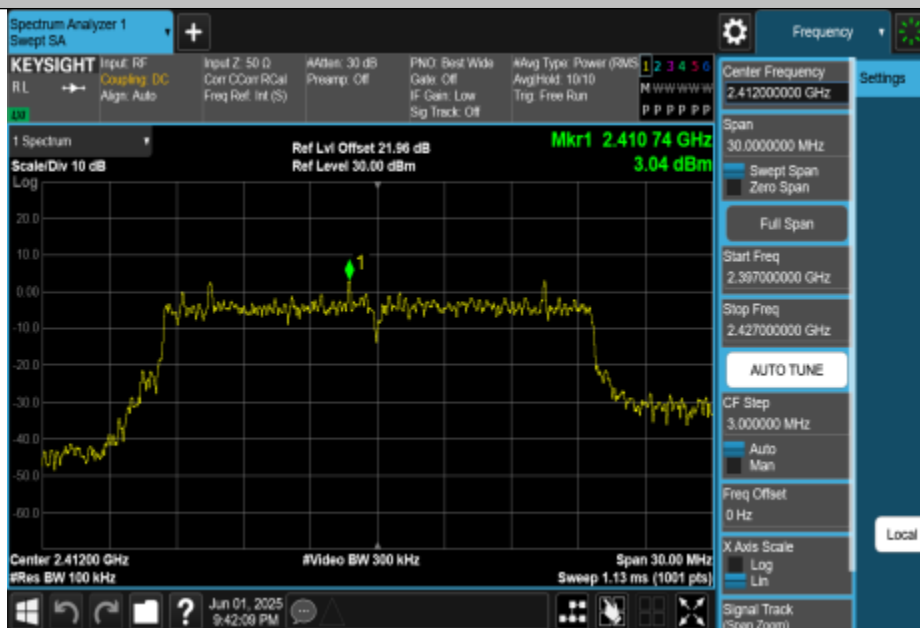
11AX20MIMO-Ant3-2412-0~Reference-PASS
