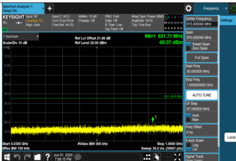
11AX40MIMO-Ant3-2422-30~1000-PASS
