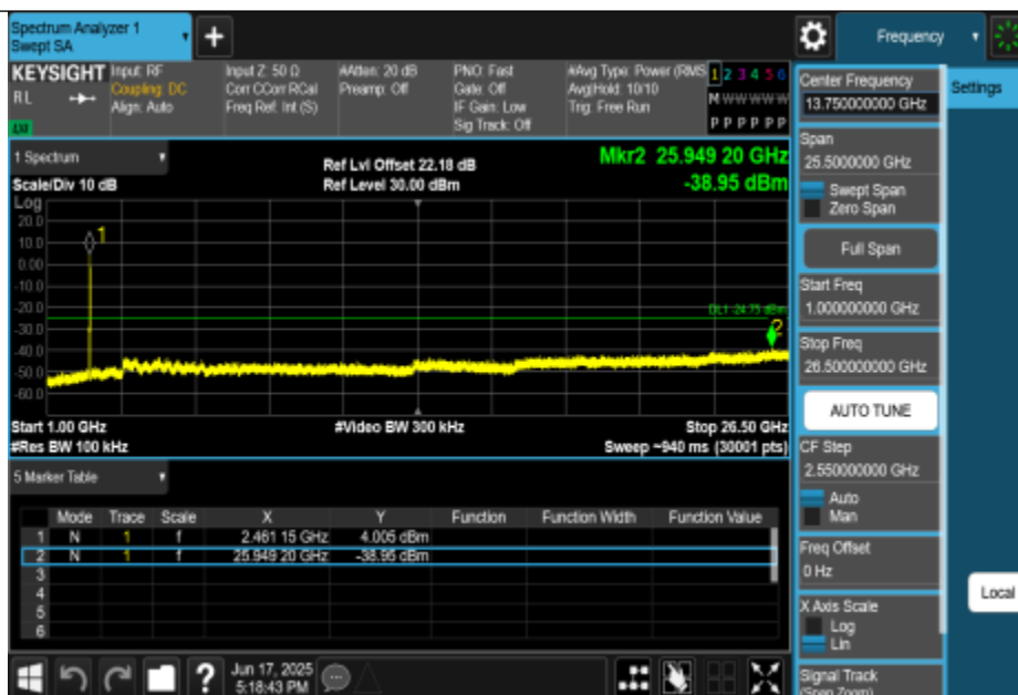
11N20MIMO-Ant2-2462-1000~26500-PASS
