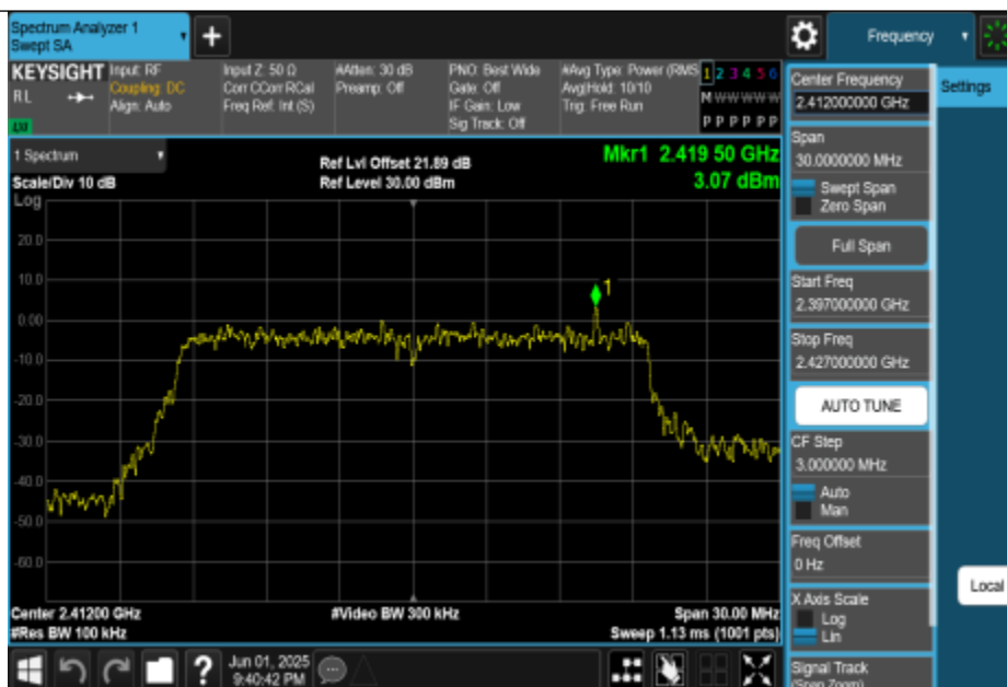
11AX20MIMO-Ant2-2412-0~Reference-PASS
