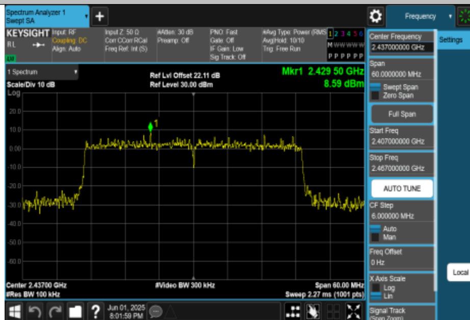
11AX40MIMO-Ant3-2437-0~Reference-PASS
