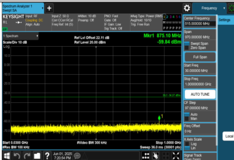
11N40MIMO-Ant3-2452-30~1000-PASS
