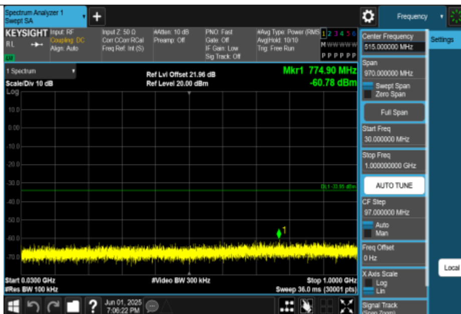
11N40MIMO-Ant3-2422-30~1000-PASS
