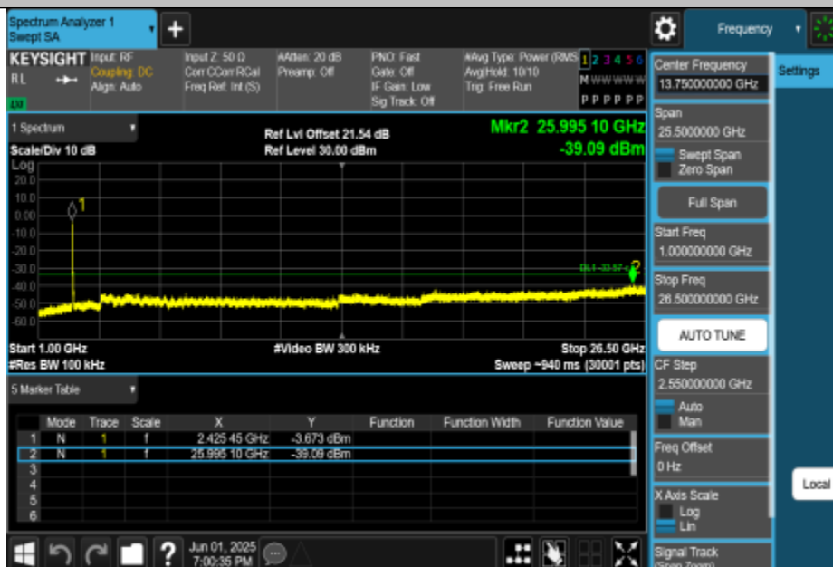
11N40MIMO-Ant0-2422-1000~26500-PASS
