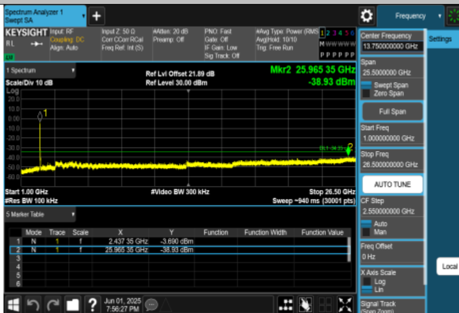
11AX40MIMO-Ant2-2422-1000~26500-PASS
