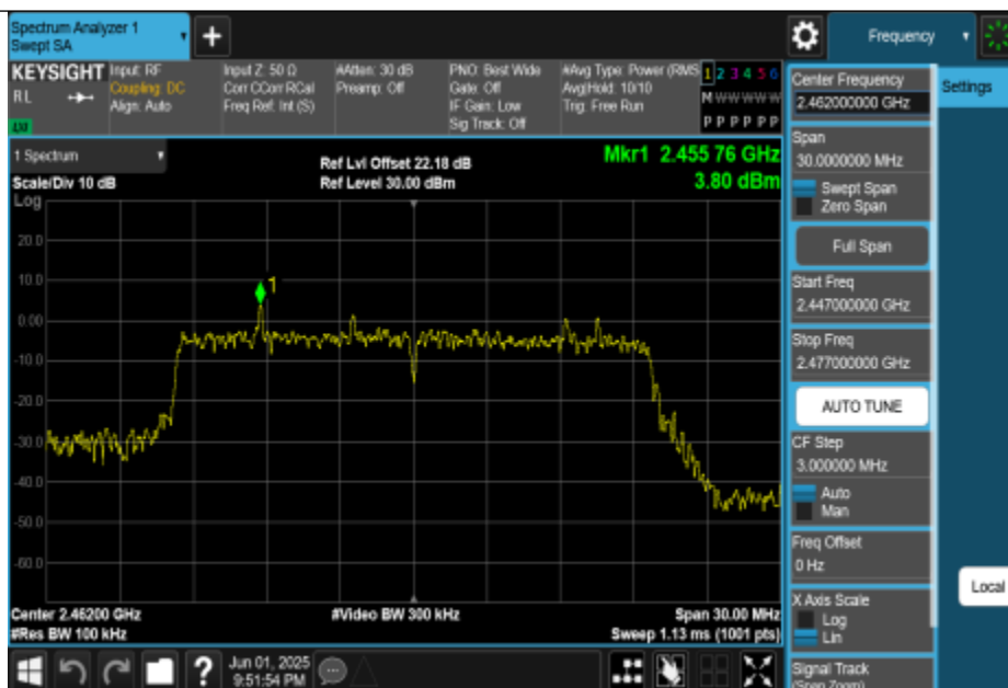
11AX20MIMO-Ant2-2462-0~Reference-PASS
