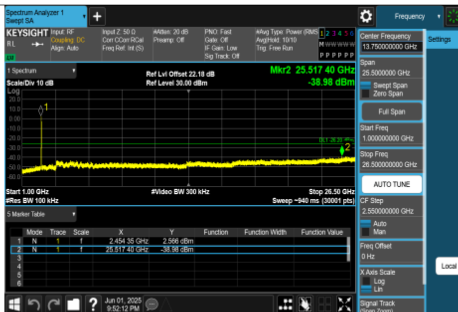
11AX20MIMO-Ant2-2462-1000~26500-PASS
