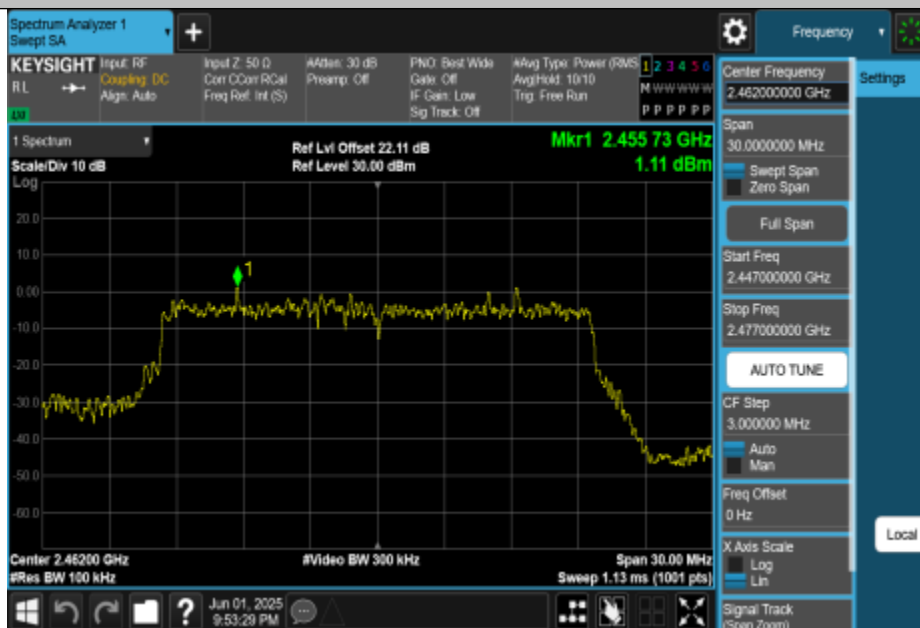
11AX20MIMO-Ant3-2462-0~Reference-PASS
