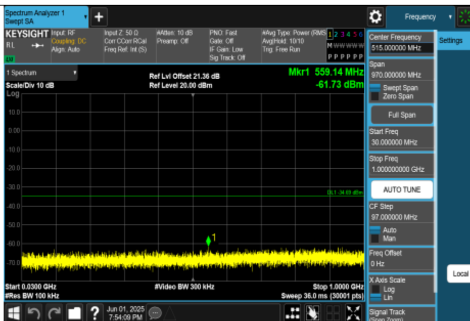
11AX40MIMO-Ant1-2422-30~1000-PASS
