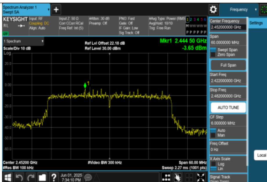
11AX40MIMO-Ant2-2452-0~Reference-PASS
