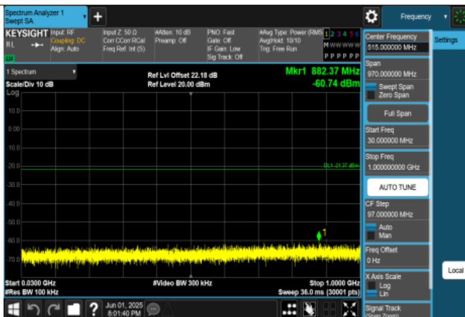
11AX40MIMO-Ant2-2437-30~1000-PASS
