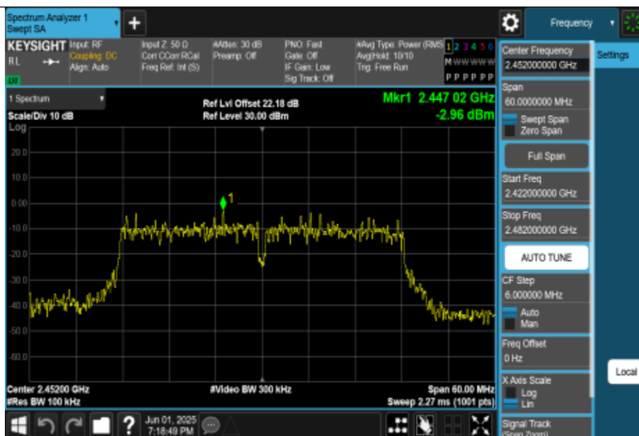
11N40MIMO-Ant2-2452-0~Reference-PASS
