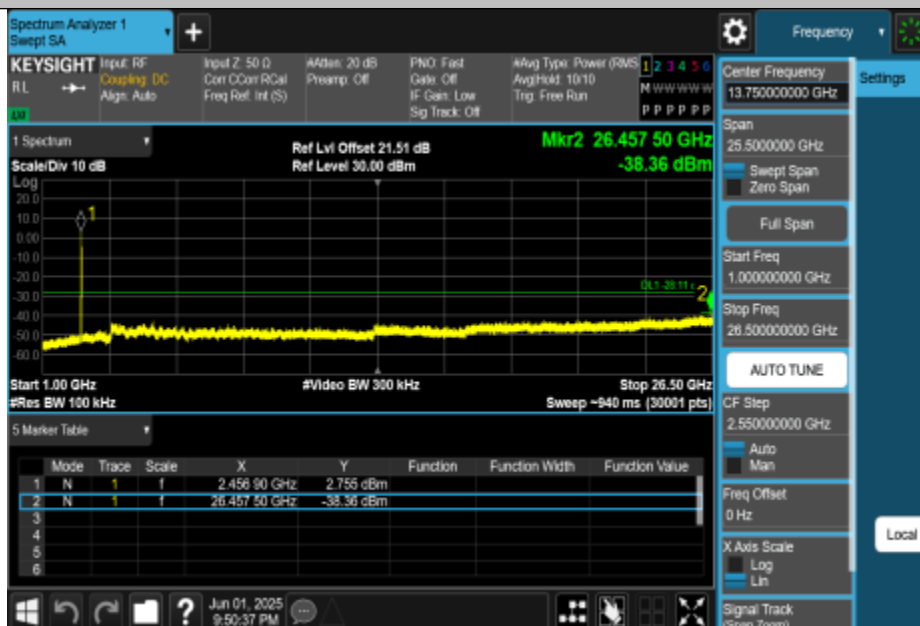
11AX20MIMO-Ant1-2462-1000~26500-PASS
