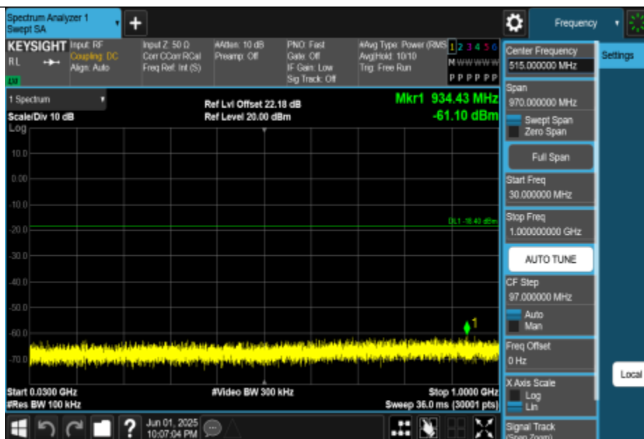
11AX20MIMO-Ant2-2437-30~1000-PASS
