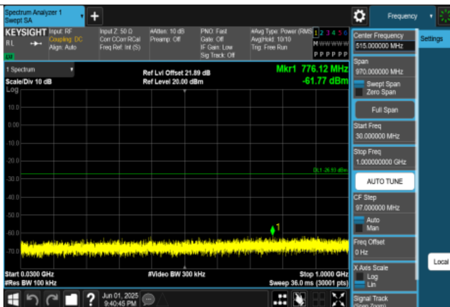
11AX20MIMO-Ant2-2412-30~1000-PASS
