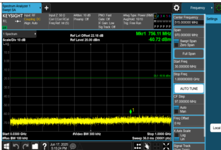
11N20MIMO-Ant2-2437-30~1000-PASS
