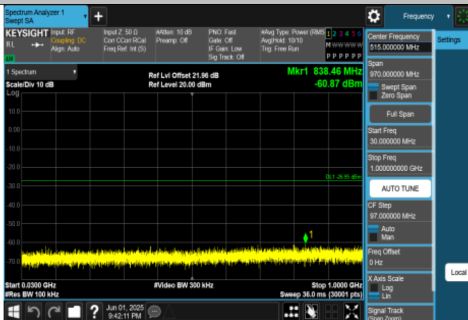
11AX20MIMO-Ant3-2412-30~1000-PASS
