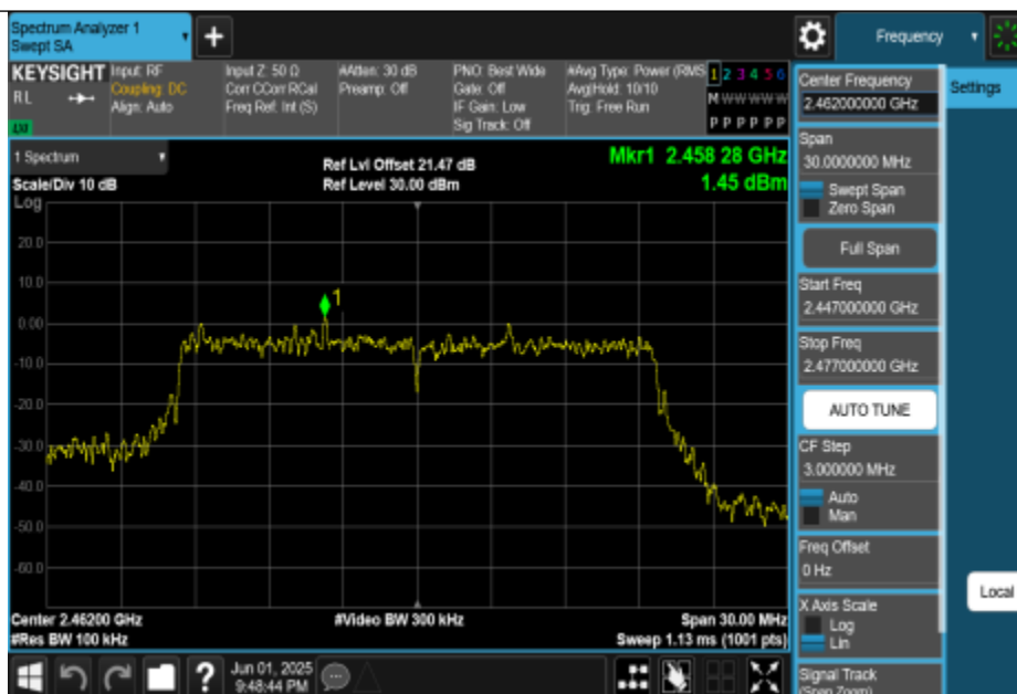
11AX20MIMO-Ant0-2462-0~Reference-PASS
