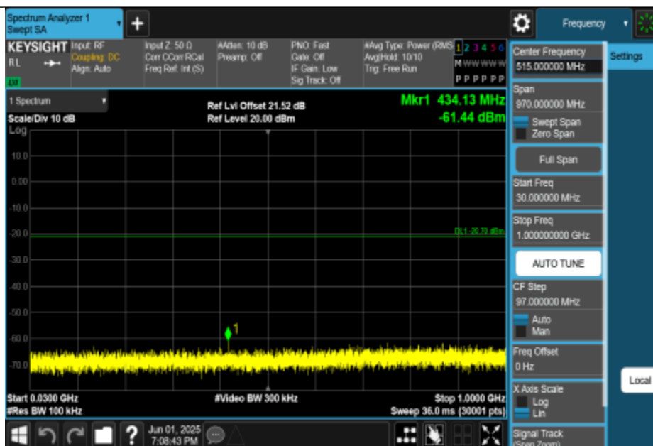
11N40MIMO-Ant0-2437-30~1000-PASS
