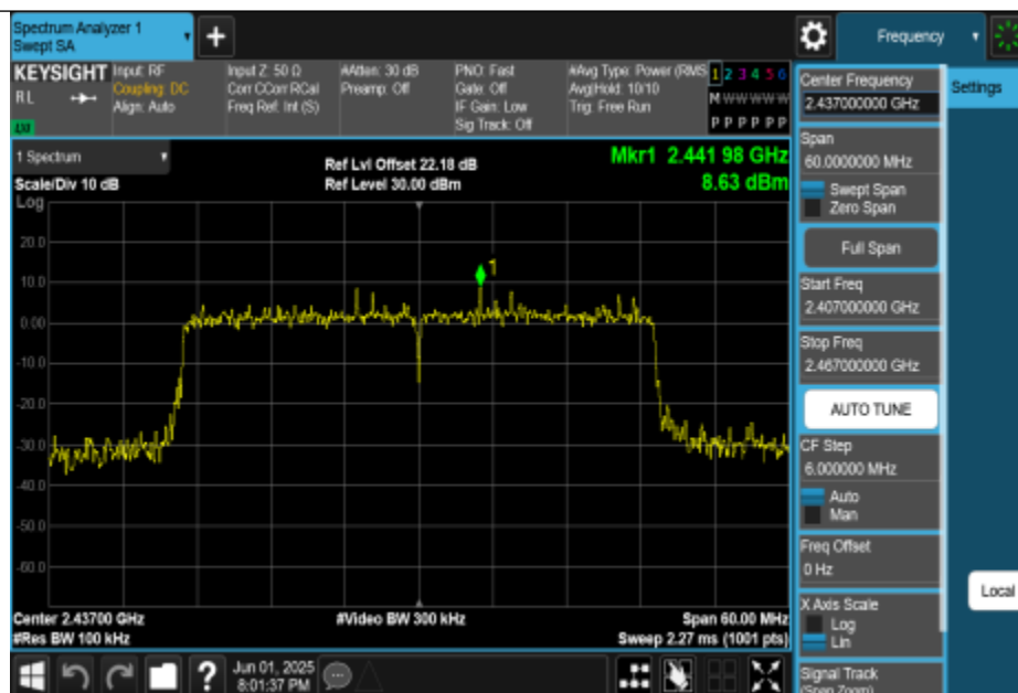
11AX40MIMO-Ant2-2437-0~Reference-PASS
