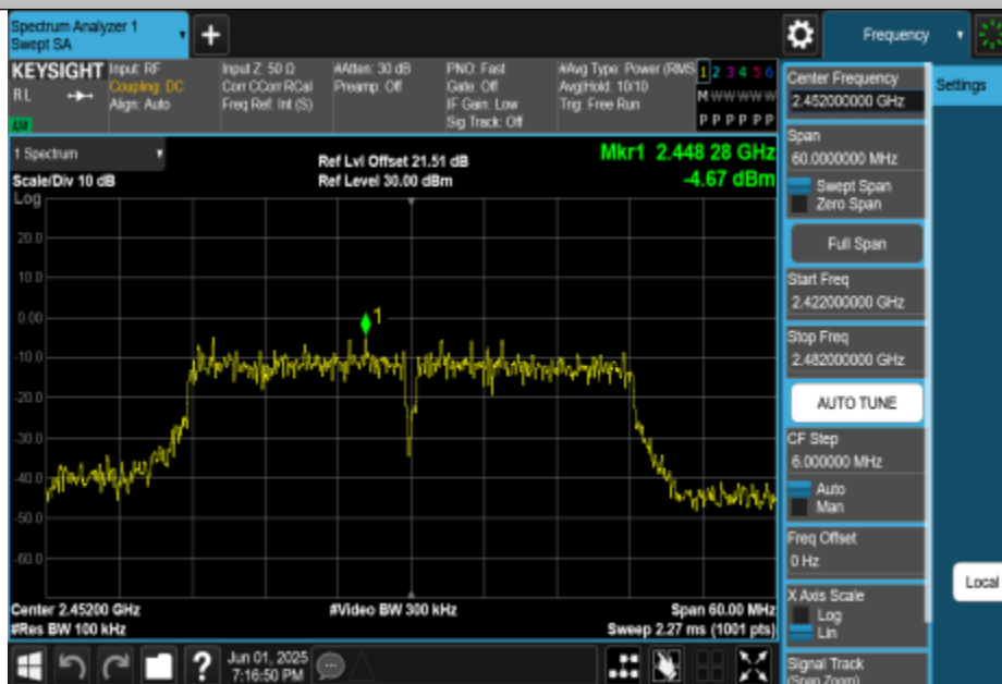
11N40MIMO-Ant1-2452-0~Reference-PASS
