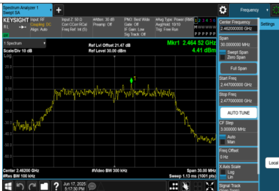
11N20MIMO-Ant0-2462-0~Reference-PASS
