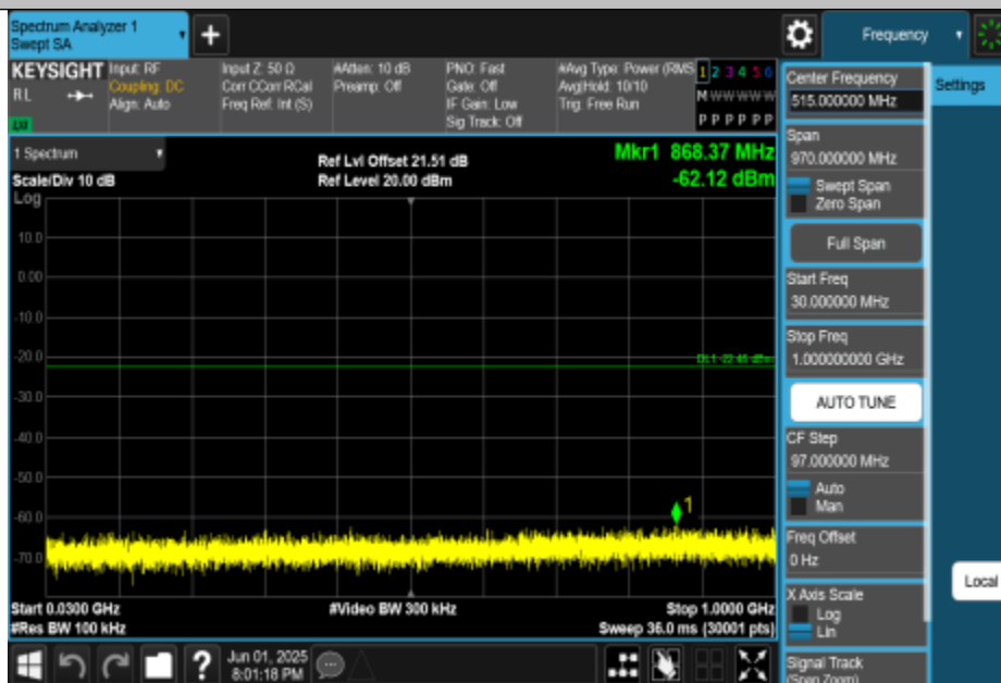
11AX40MIMO-Ant1-2437-30~1000-PASS
