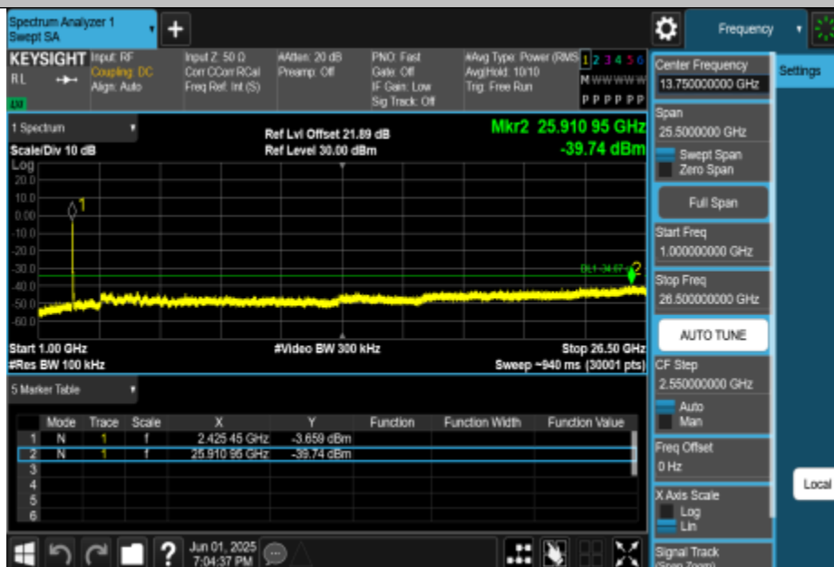
11N40MIMO-Ant2-2422-1000~26500-PASS
