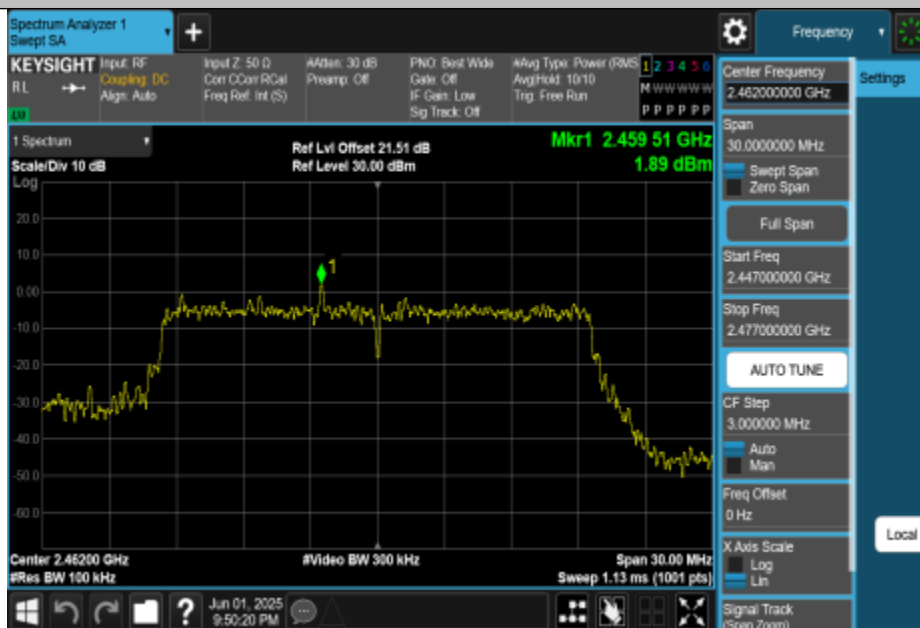
11AX20MIMO-Ant1-2462-0~Reference-PASS
