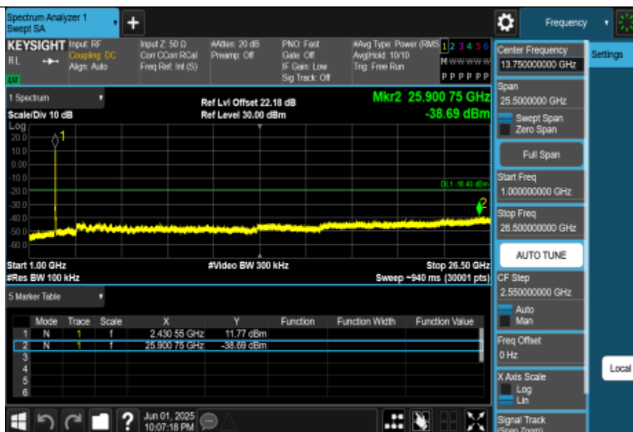
11AX20MIMO-Ant2-2437-1000~26500-PASS
