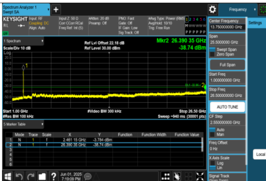
11N40MIMO-Ant2-2452-1000~26500-PASS
