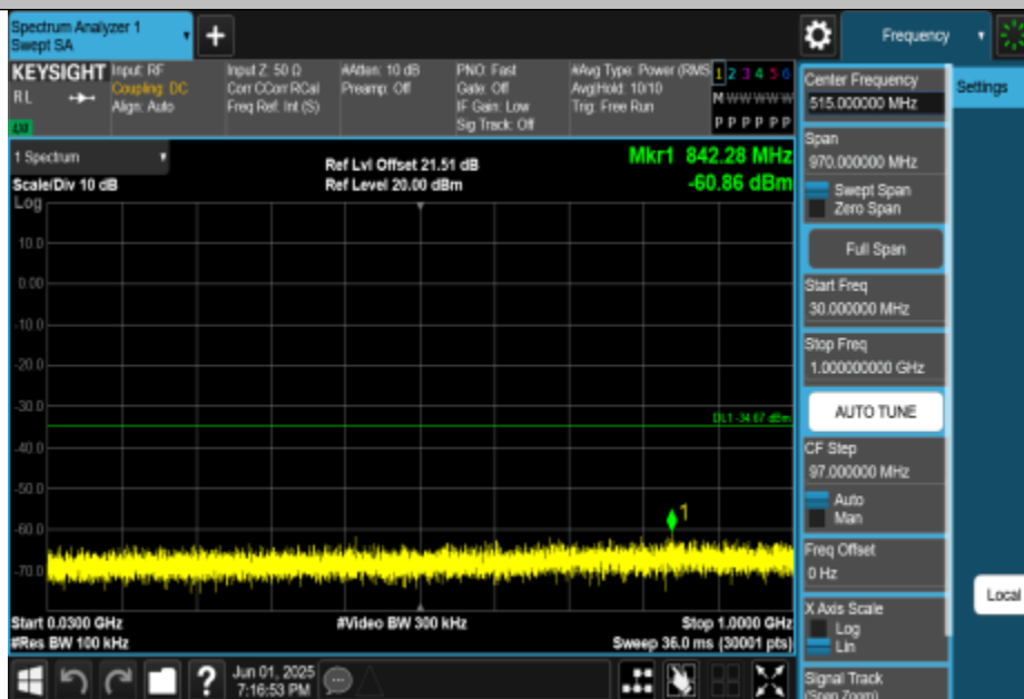
11N40MIMO-Ant1-2452-30~1000-PASS
