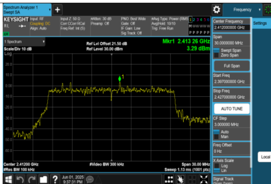
11AX20MIMO-Ant0-2412-0~Reference-PASS
