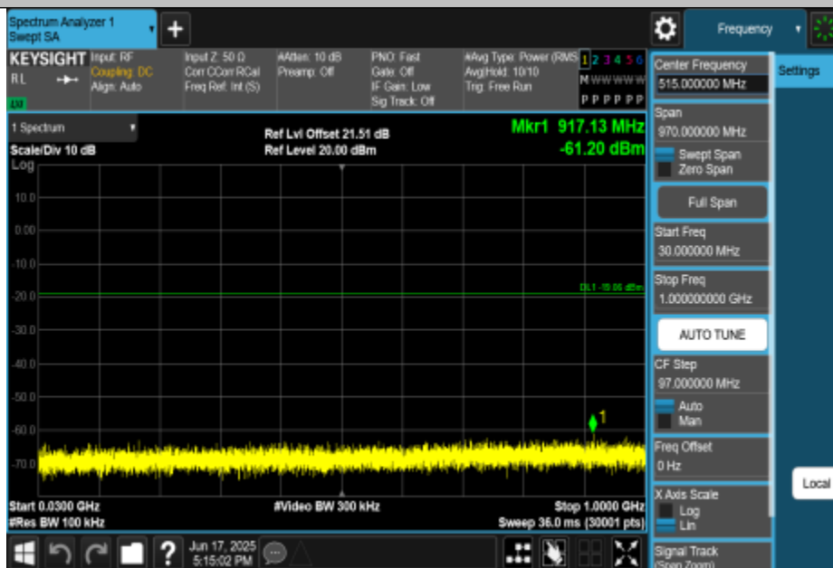
11N20MIMO-Ant1-2437-30~1000-PASS
