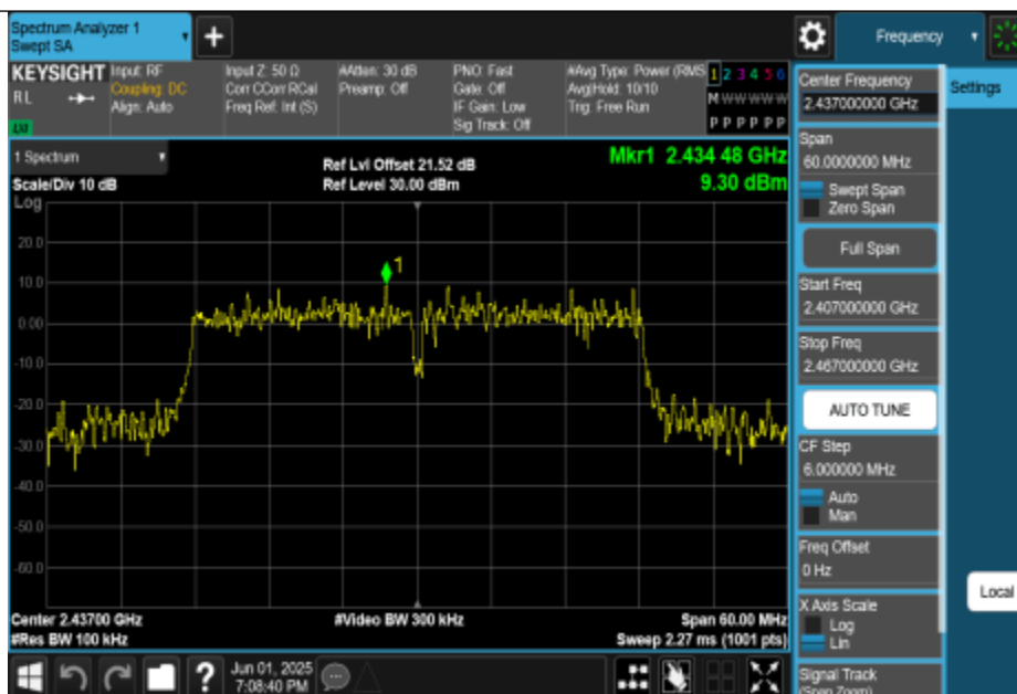
11N40MIMO-Ant0-2437-0~Reference-PASS
