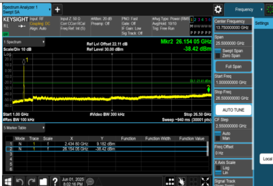
11AX40MIMO-Ant3-2437-1000~26500-PASS
