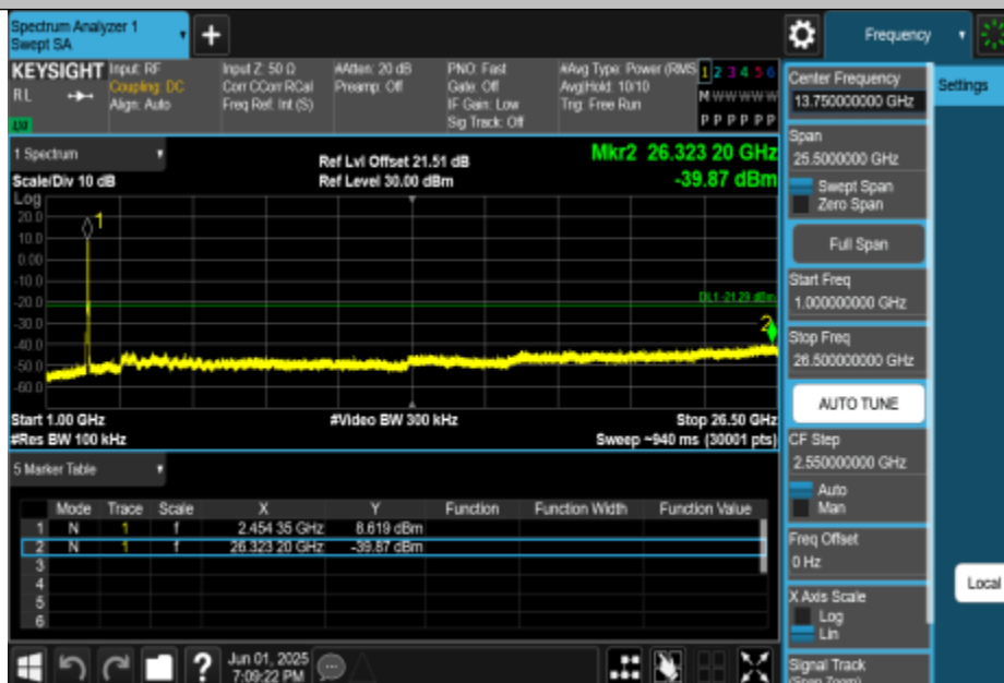
11N40MIMO-Ant1-2437-1000~26500-PASS
