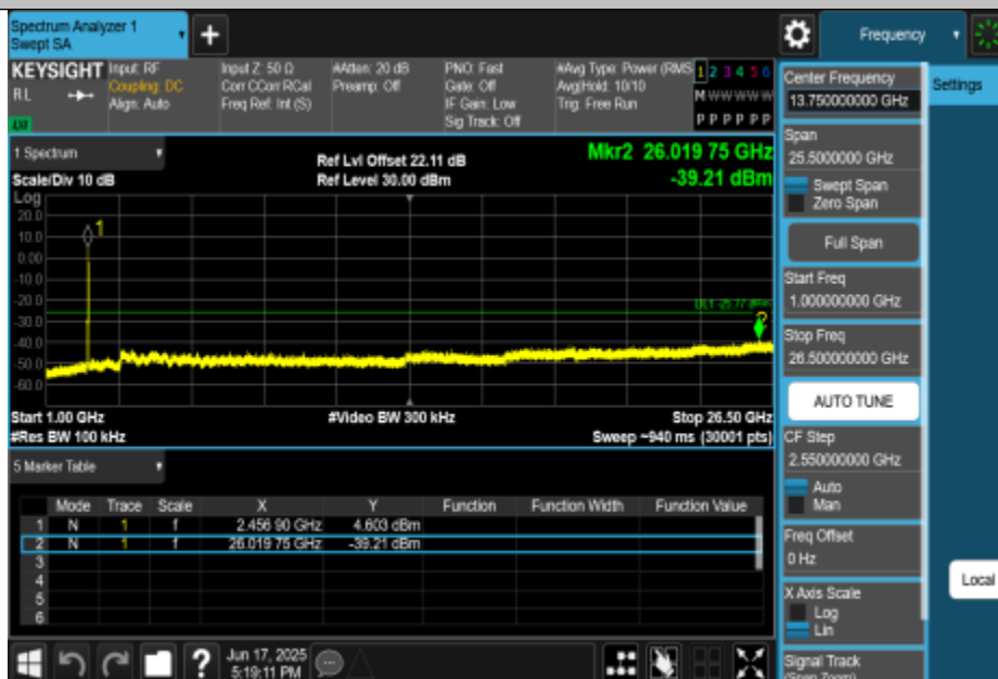
11N20MIMO-Ant3-2462-1000~26500-PASS
