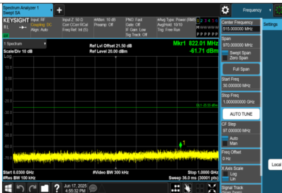
11G-CDD-Ant0-2412-30~1000-PASS
