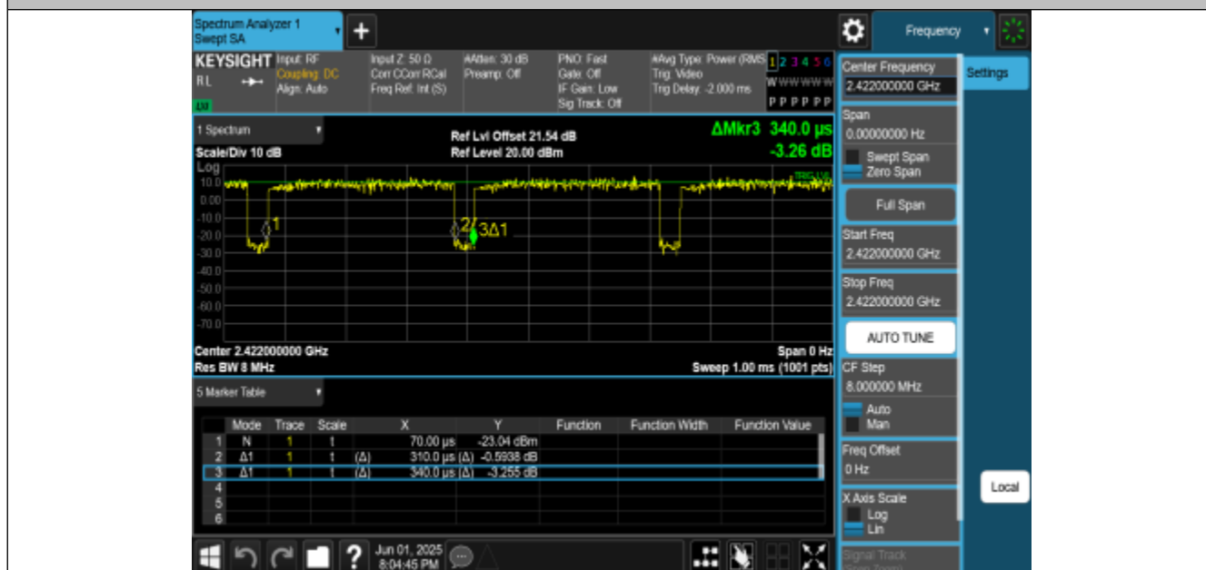
NTNV-11BE40MIMO-Ant0-2422
