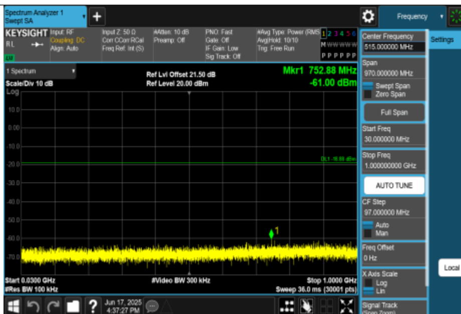
11B-CDD-Ant0-2412-30~1000-PASS
