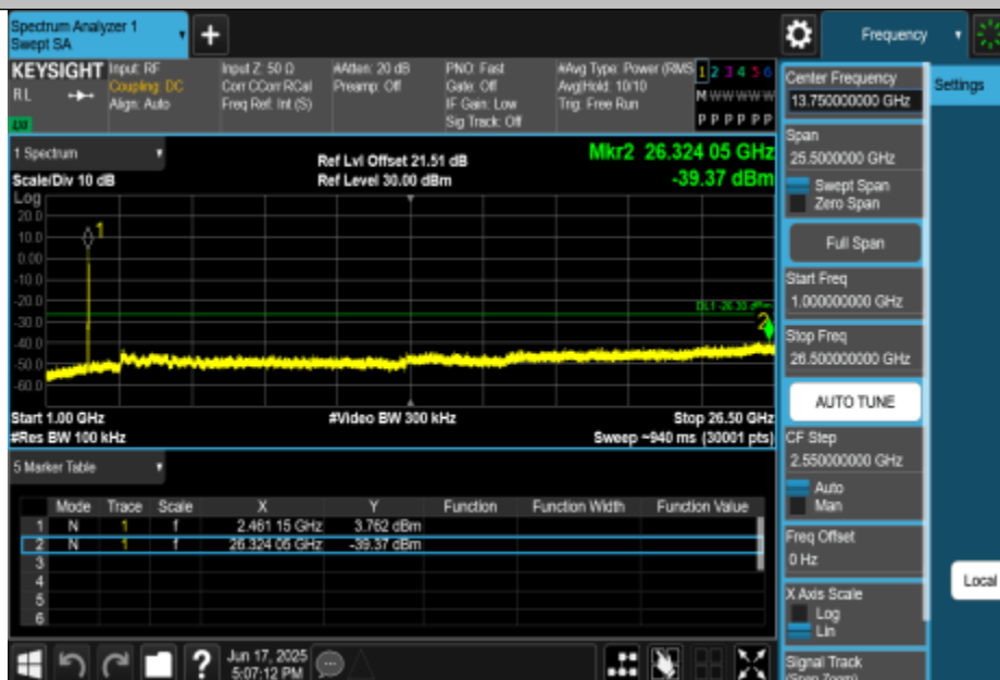
11G-CDD-Ant1-2462-1000~26500-PASS
