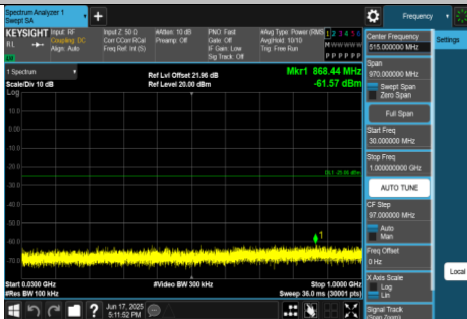
11N20MIMO-Ant3-2412-30~1000-PASS
