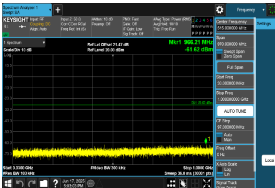
11G-CDD-Ant0-2462-30~1000-PASS
