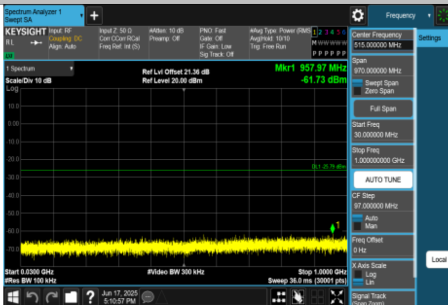
11N20MIMO-Ant1-2412-30~1000-PASS
