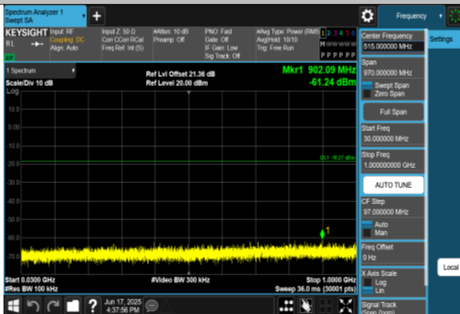
11B-CDD-Ant1-2412-30~1000-PASS
