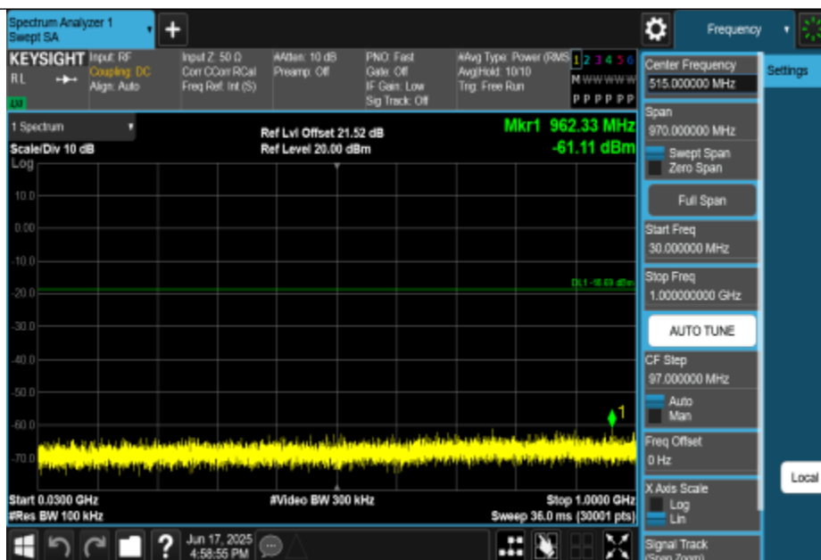
11G-CDD-Ant0-2437-30~1000-PASS
