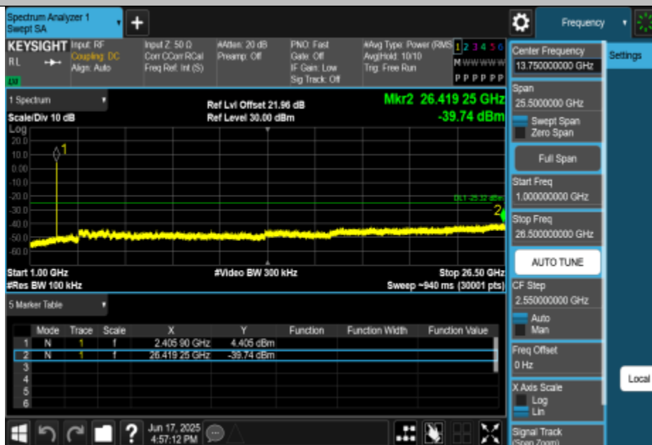
11G-CDD-Ant3-2412-1000~26500-PASS
