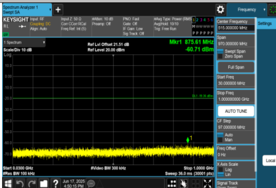
11B-CDD-Ant1-2462-30~1000-PASS
