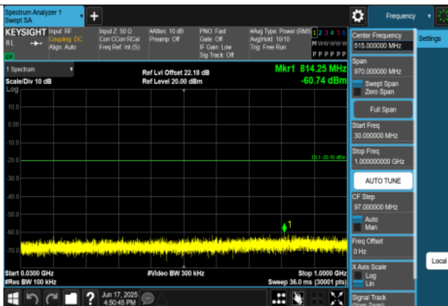
11B-CDD-Ant2-2462-30~1000-PASS
