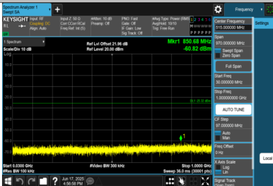
11G-CDD-Ant3-2412-30~1000-PASS
