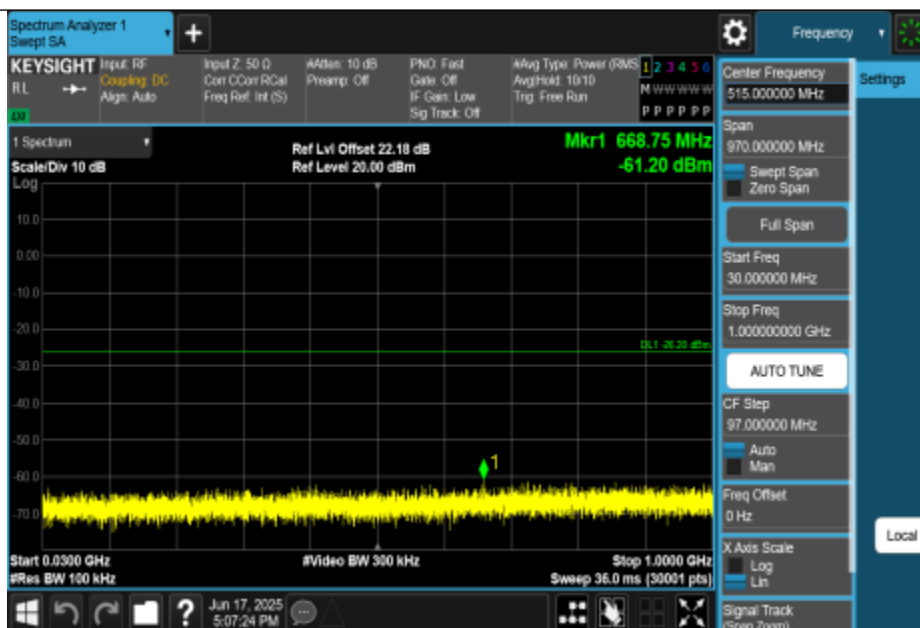
11G-CDD-Ant2-2462-30~1000-PASS
