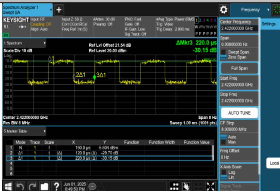
NTNV-11N40MIMO-Ant0-2422
