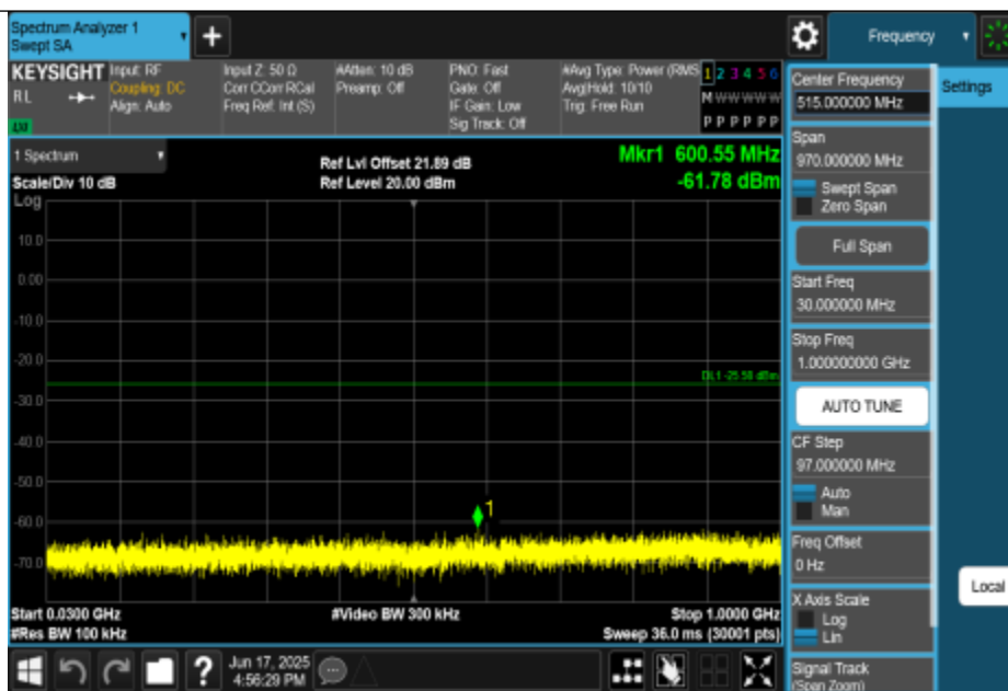
11G-CDD-Ant2-2412-30~1000-PASS
