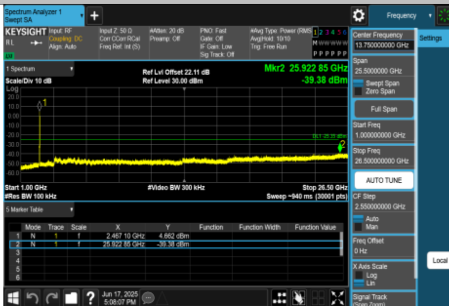
11G-CDD-Ant3-2462-1000~26500-PASS
