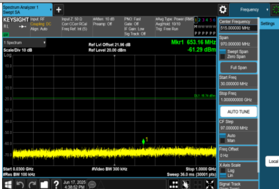
11B-CDD-Ant3-2412-30~1000-PASS
