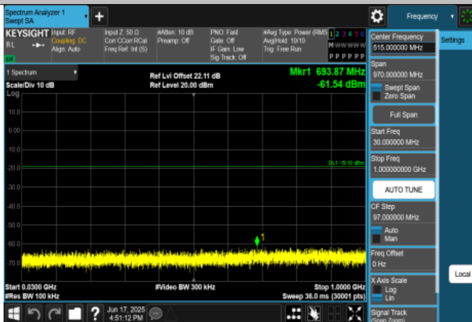
11B-CDD-Ant3-2462-30~1000-PASS
