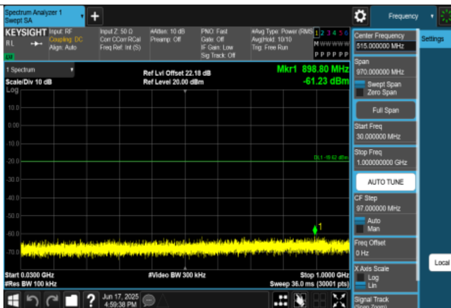
11G-CDD-Ant2-2437-30~1000-PASS
