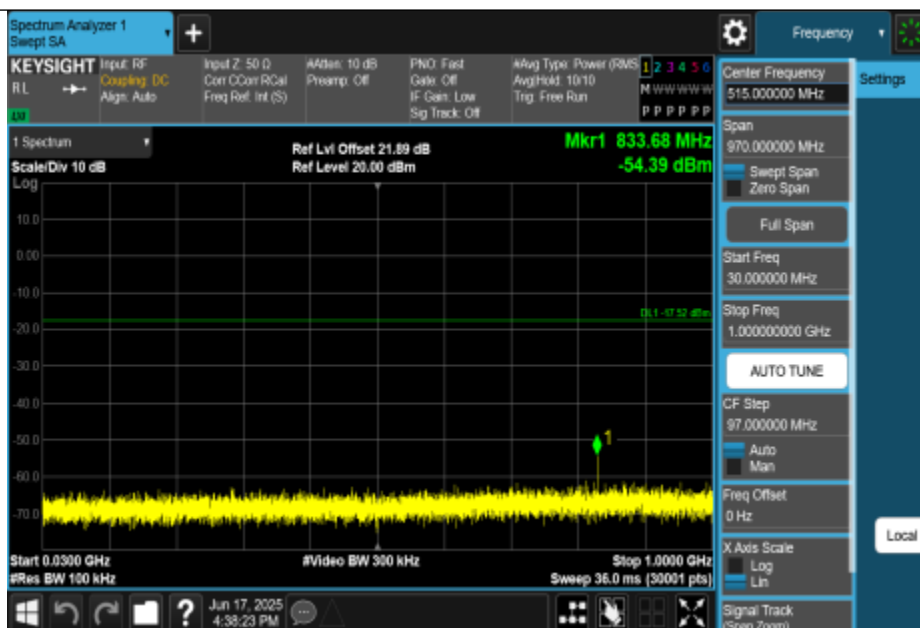
11B-CDD-Ant2-2412-30~1000-PASS
