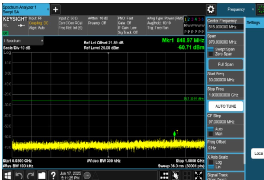
11N20MIMO-Ant2-2412-30~1000-PASS
