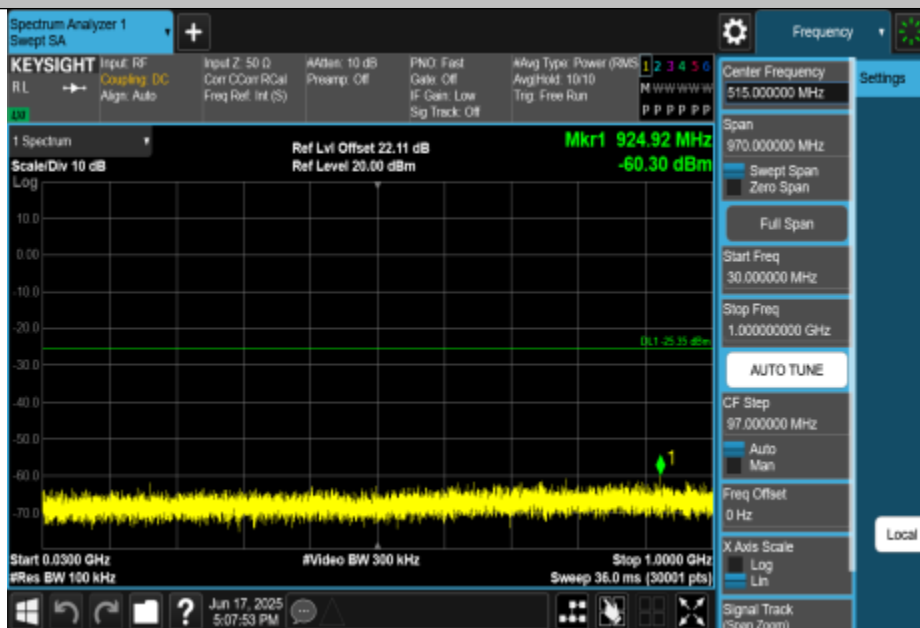
11G-CDD-Ant3-2462-30~1000-PASS
