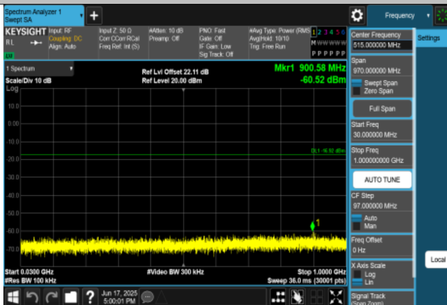
11G-CDD-Ant3-2437-30~1000-PASS
