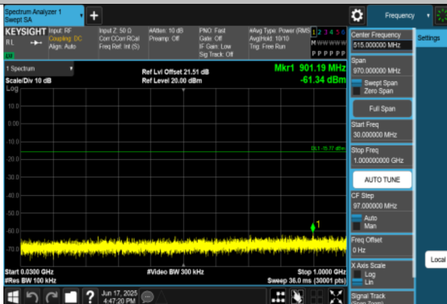
11B-CDD-Ant1-2437-30~1000-PASS
