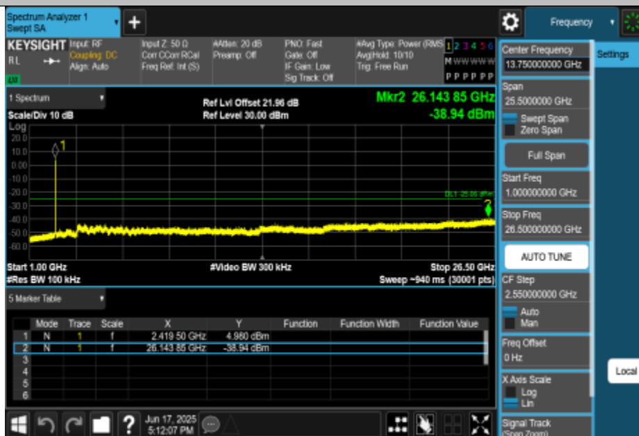
11N20MIMO-Ant3-2412-1000~26500-PASS
