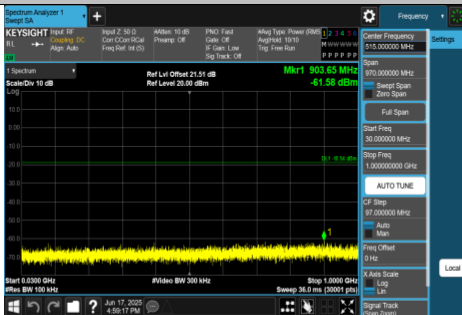
11G-CDD-Ant1-2437-30~1000-PASS
