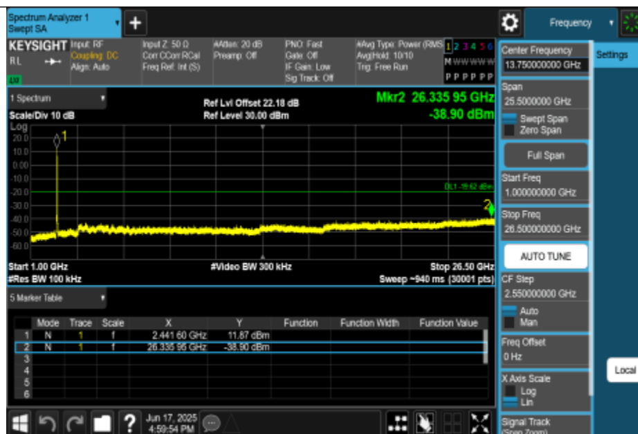
11G-CDD-Ant2-2437-1000~26500-PASS
