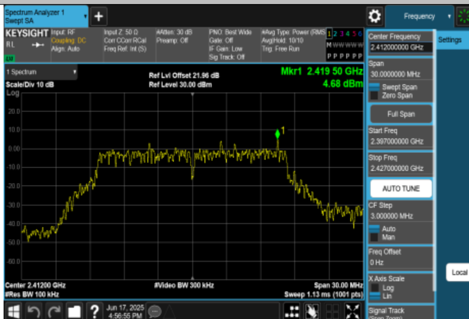
11G-CDD-Ant3-2412-0~Reference-PASS
