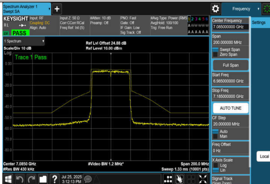
NTNV-11BE40MIMO-Ant3-7085-PASS
