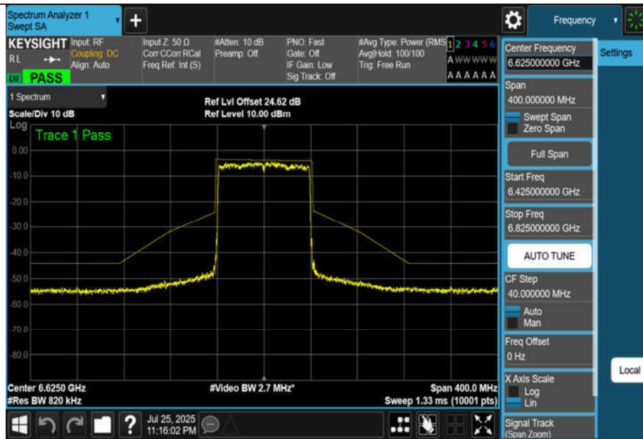
NTNV-11BE80MIMO-Ant1-6625-PASS
