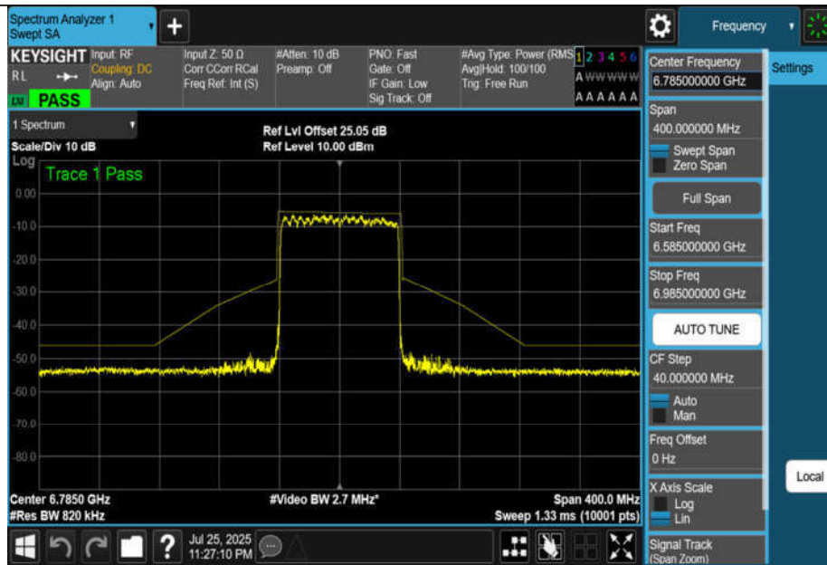
NTNV-11BE80MIMO-Ant3-6785-PASS
