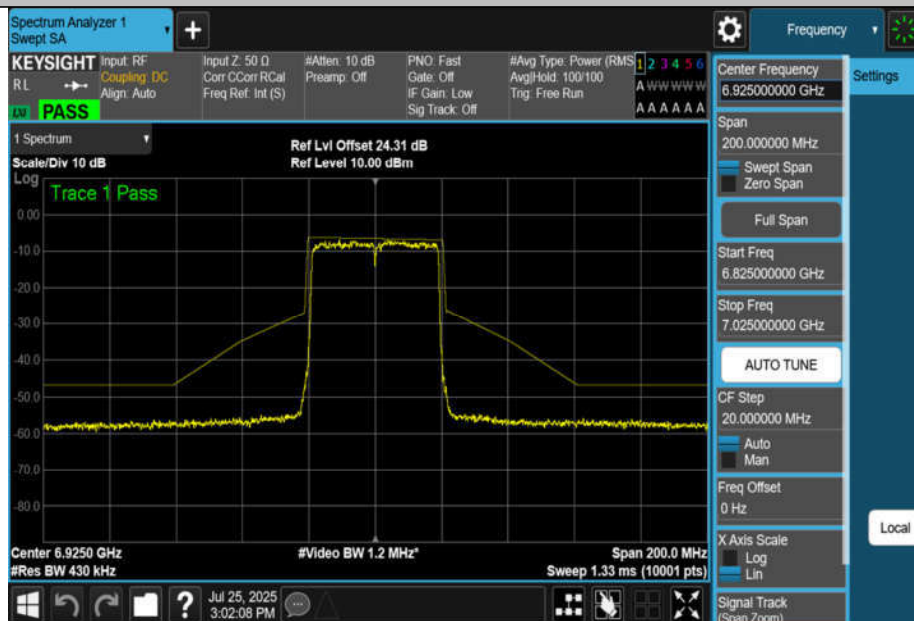
NTNV-11BE40MIMO-Ant2-6925-PASS
