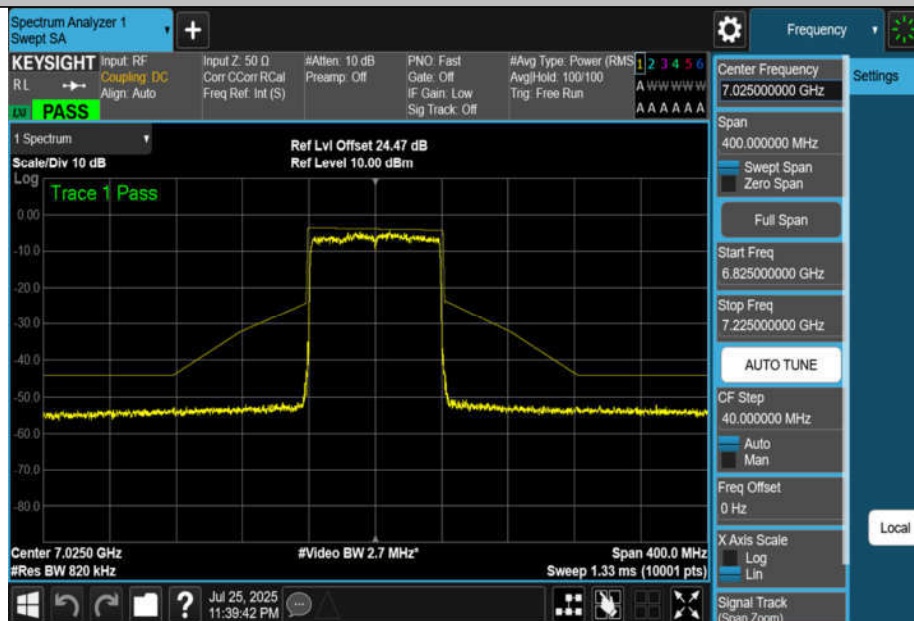
NTNV-11BE80MIMO-Ant2-7025-PASS
