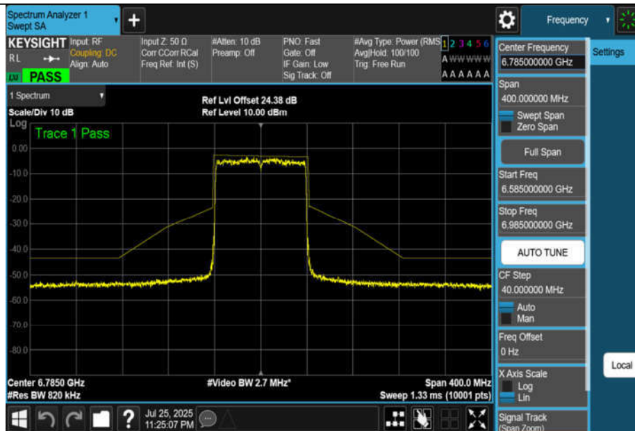
NTNV-11BE80MIMO-Ant1-6785-PASS
