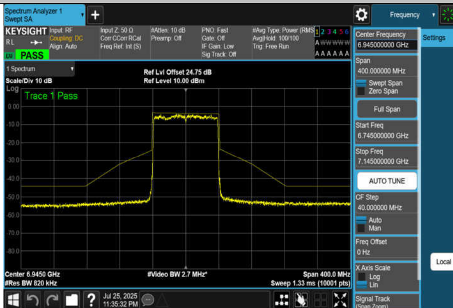
NTNV-11BE80MIMO-Ant2-6945-PASS
