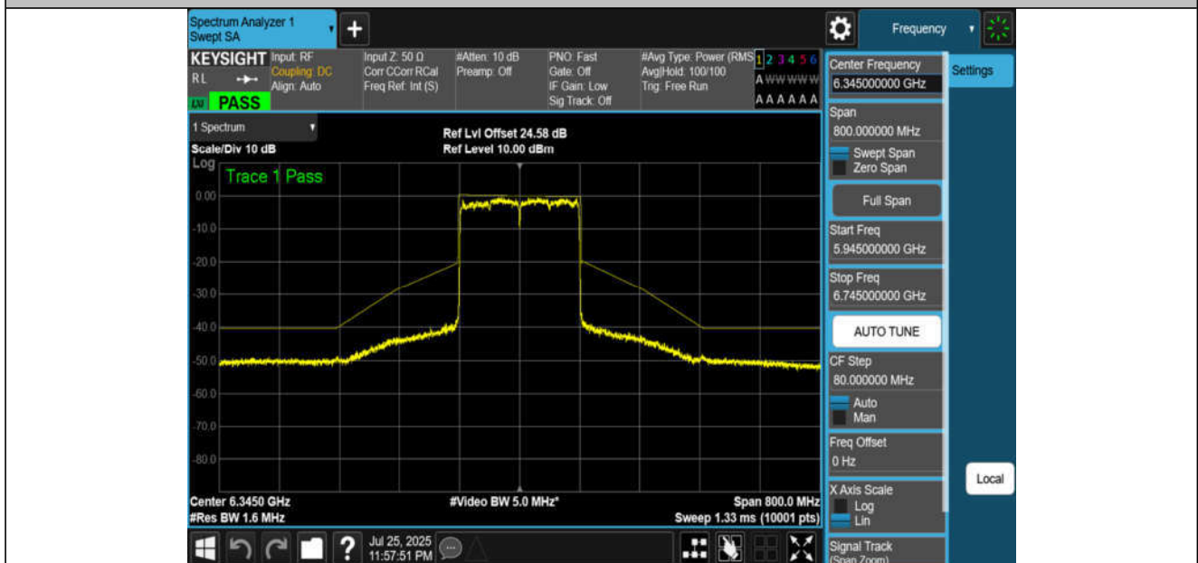
NTNV-11BE160MIMO-Ant4-6345-PASS
