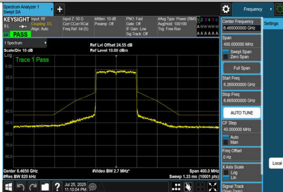
NTNV-11BE80MIMO-Ant4-6465-PASS
