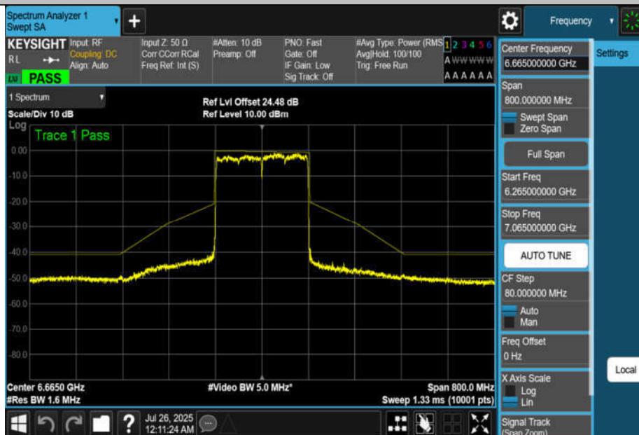
NTNV-11BE160MIMO-Ant4-6665-PASS
