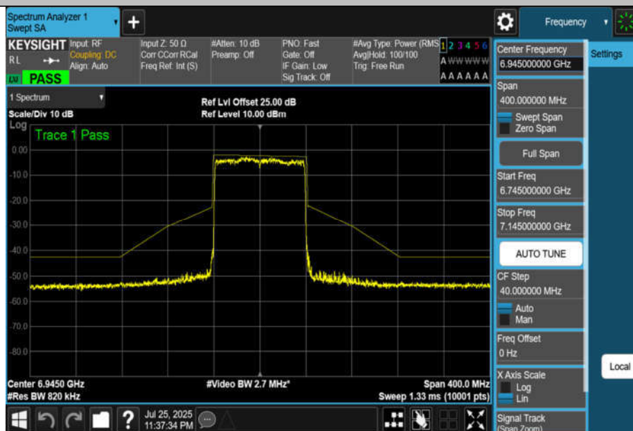
NTNV-11BE80MIMO-Ant4-6945-PASS
