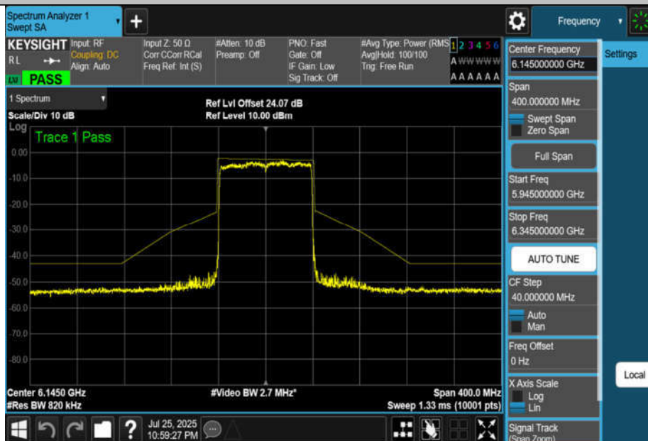
NTNV-11BE80MIMO-Ant4-6145-PASS
