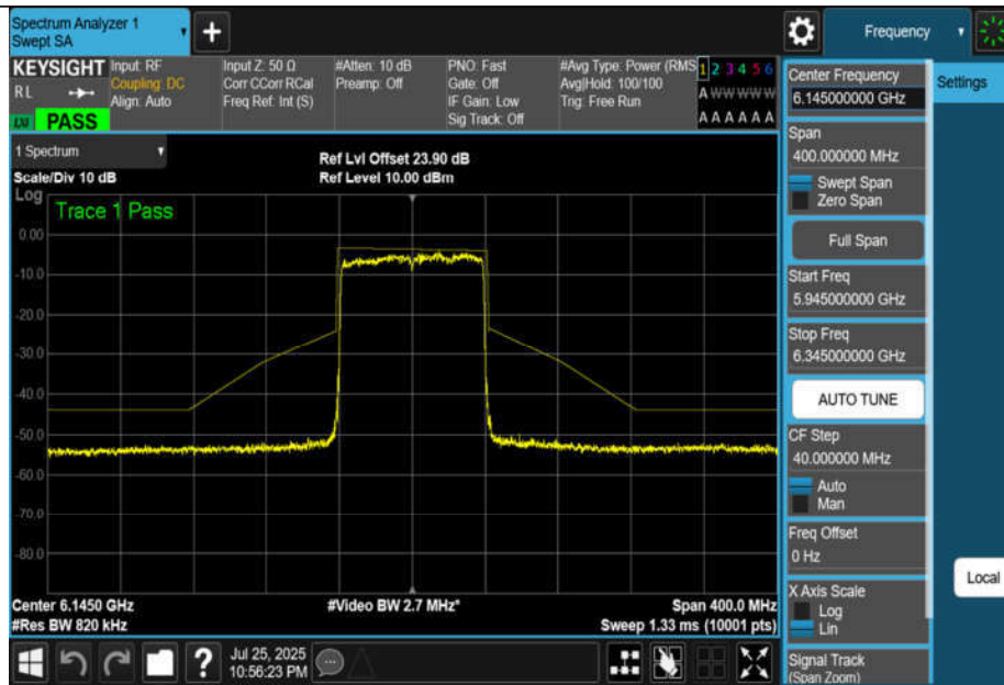
NTNV-11BE80MIMO-Ant1-6145-PASS
