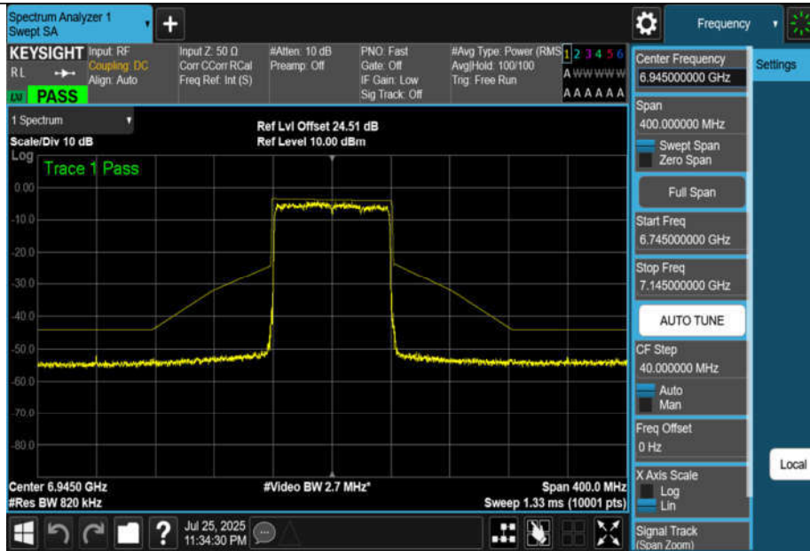
NTNV-11BE80MIMO-Ant1-6945-PASS
