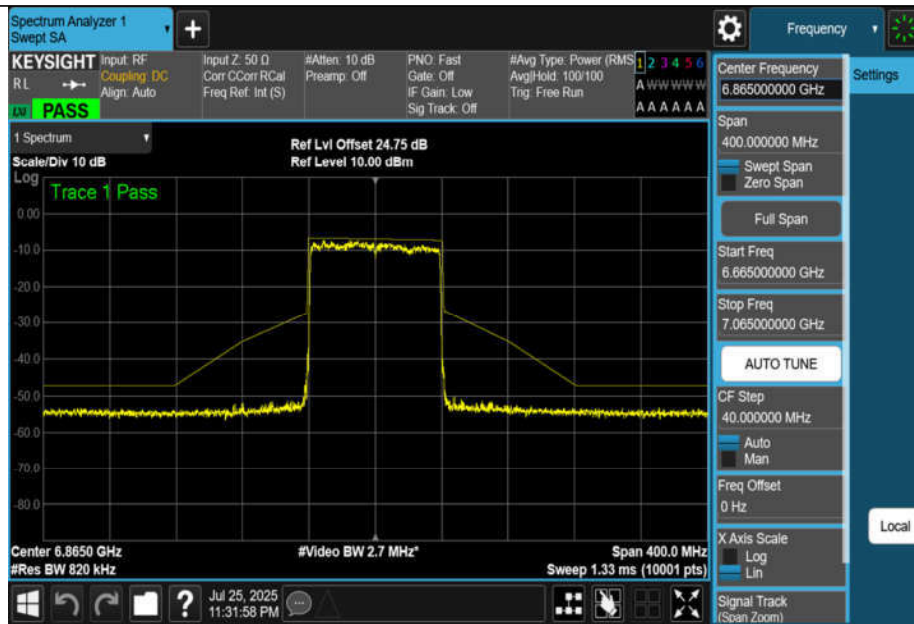
NTNV-11BE80MIMO-Ant3-6865-PASS
