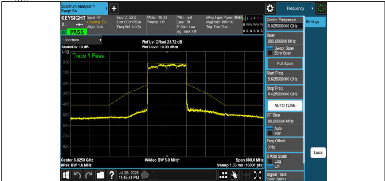
NTNV-11BE160MIMO-Ant3-6025-PASS
