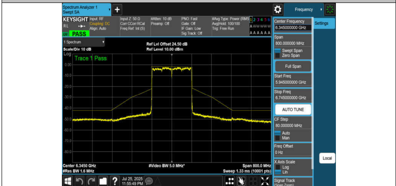
NTNV-11BE160MIMO-Ant2-6345-PASS
