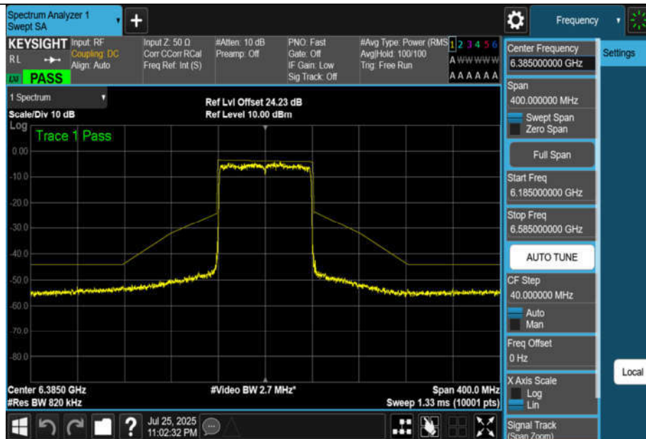
NTNV-11BE80MIMO-Ant1-6385-PASS
