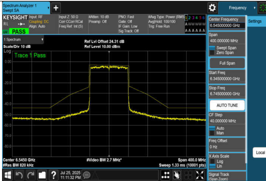
NTNV-11BE80MIMO-Ant1-6545-PASS
