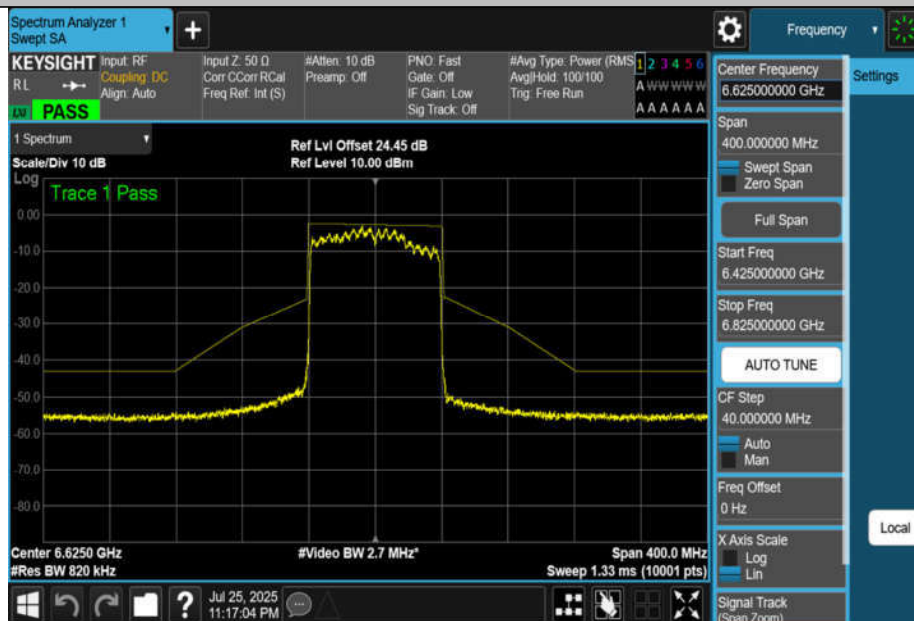
NTNV-11BE80MIMO-Ant2-6625-PASS
