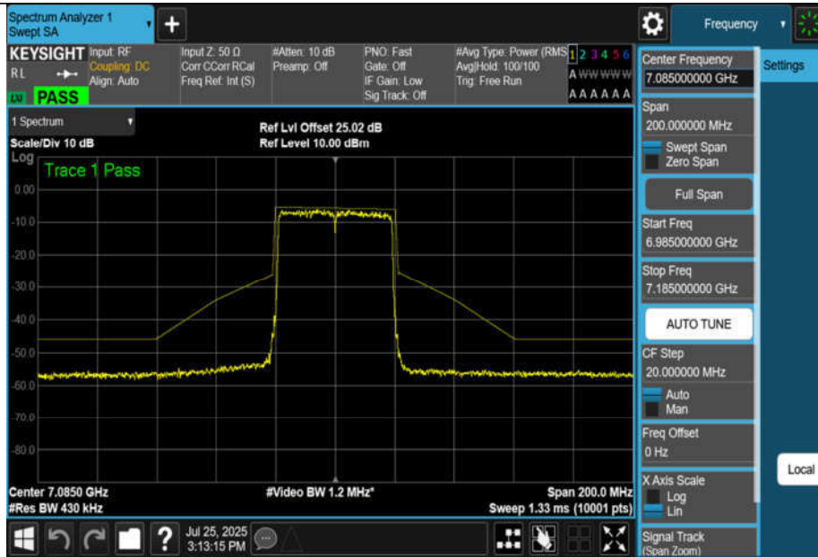
NTNV-11BE40MIMO-Ant4-7085-PASS
