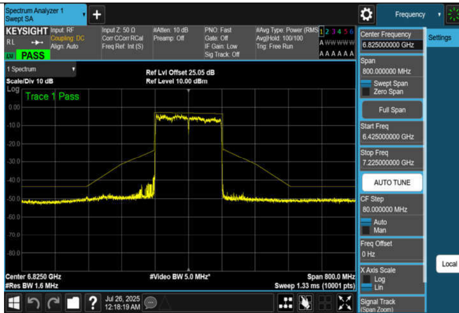
NTNV-11BE160MIMO-Ant3-6825-PASS
