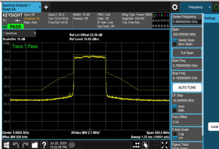
NTNV-11BE80MIMO-Ant2-5985-PASS
