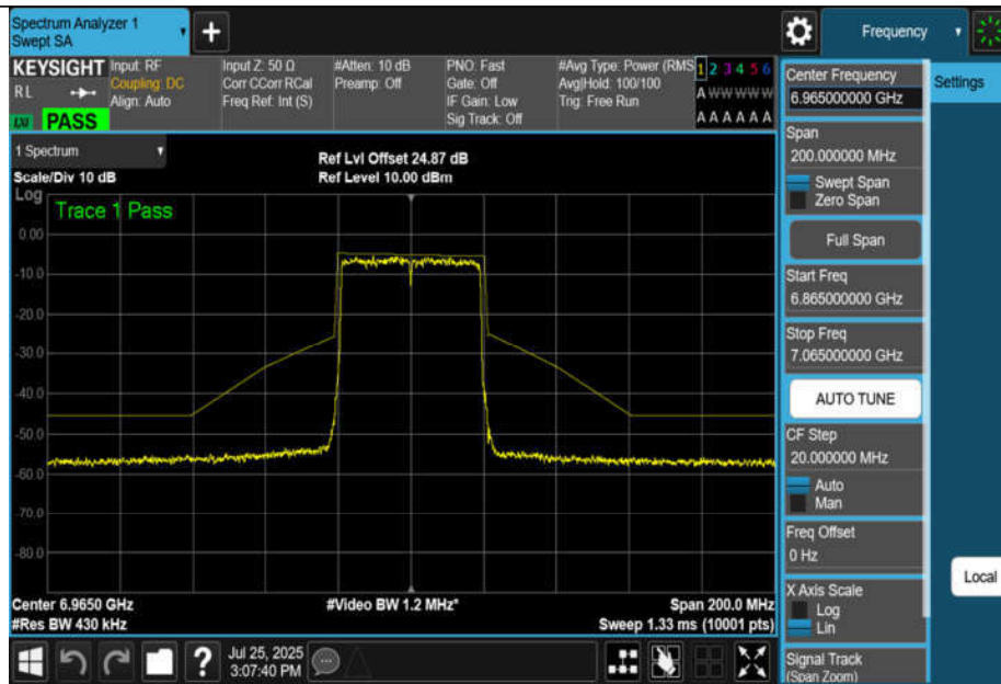
NTNV-11BE40MIMO-Ant3-6965-PASS
