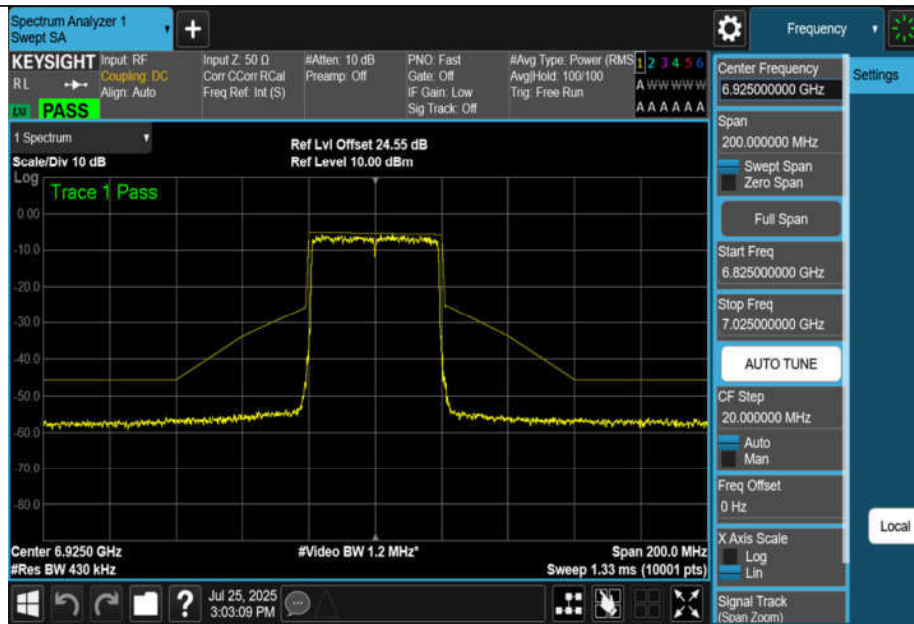
NTNV-11BE40MIMO-Ant3-6925-PASS
