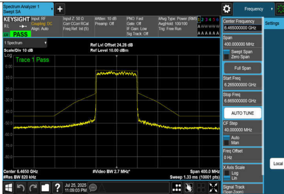
NTNV-11BE80MIMO-Ant3-6465-PASS
