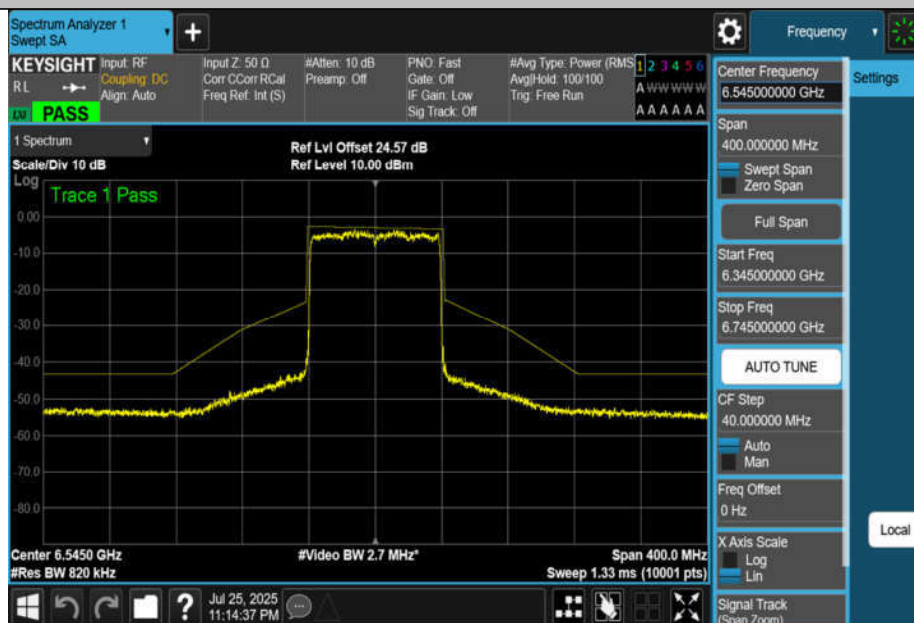
NTNV-11BE80MIMO-Ant4-6545-PASS
