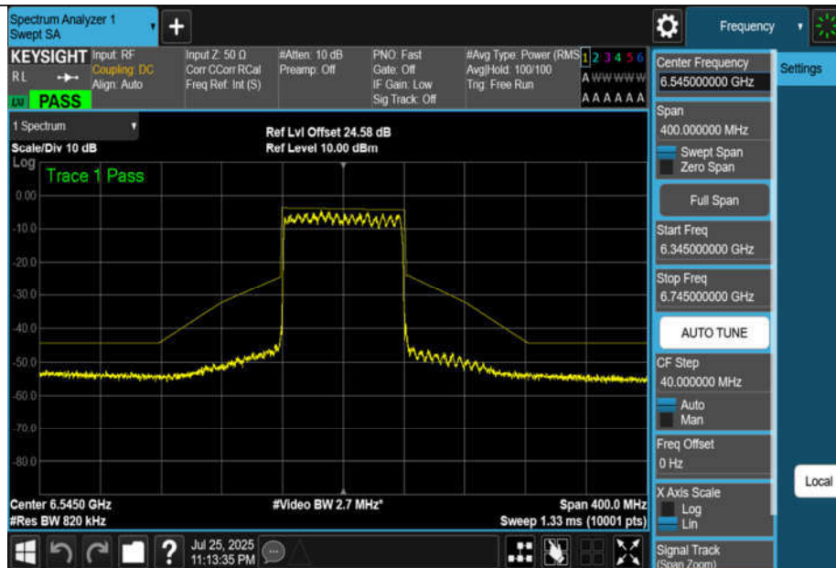
NTNV-11BE80MIMO-Ant3-6545-PASS
