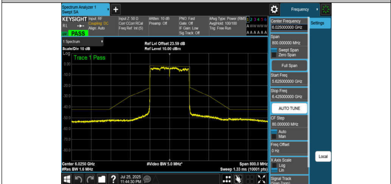
NTNV-11BE160MIMO-Ant2-6025-PASS
