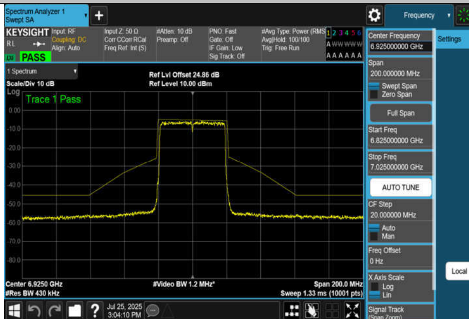
NTNV-11BE40MIMO-Ant4-6925-PASS
