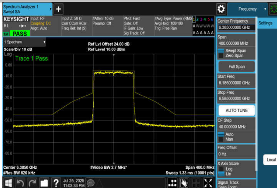
NTNV-11BE80MIMO-Ant2-6385-PASS
