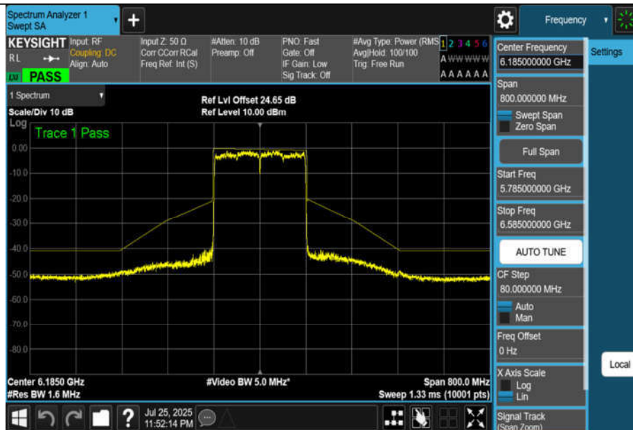
NTNV-11BE160MIMO-Ant3-6185-PASS
