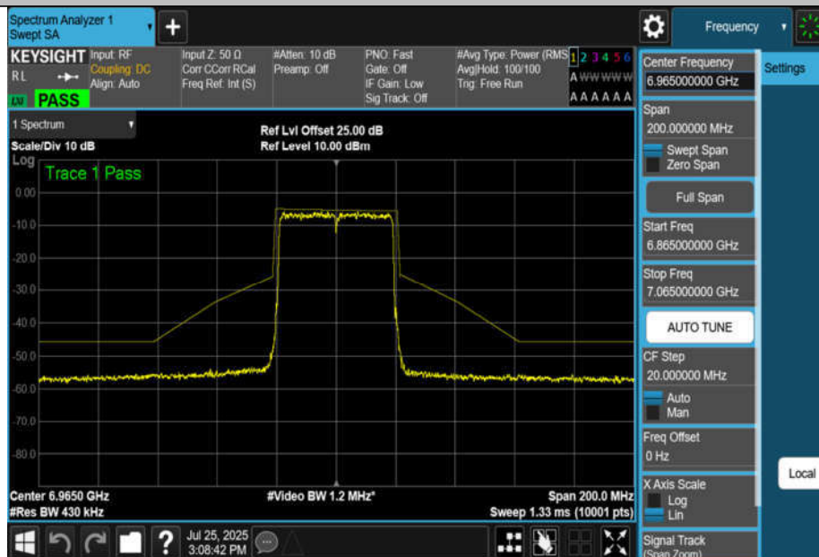
NTNV-11BE40MIMO-Ant4-6965-PASS
