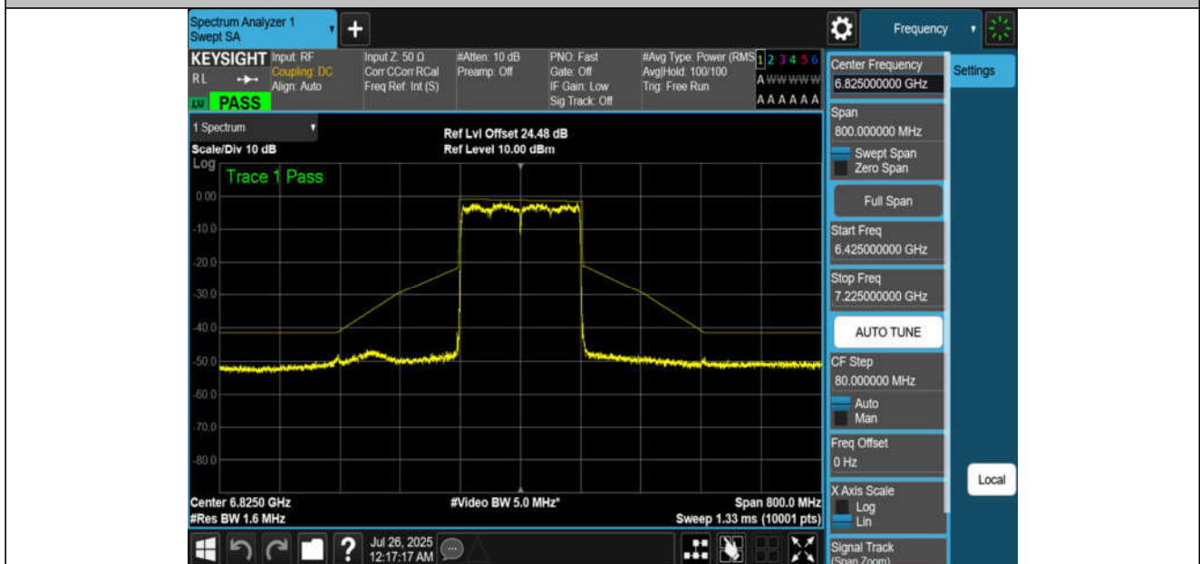
NTNV-11BE160MIMO-Ant2-6825-PASS
