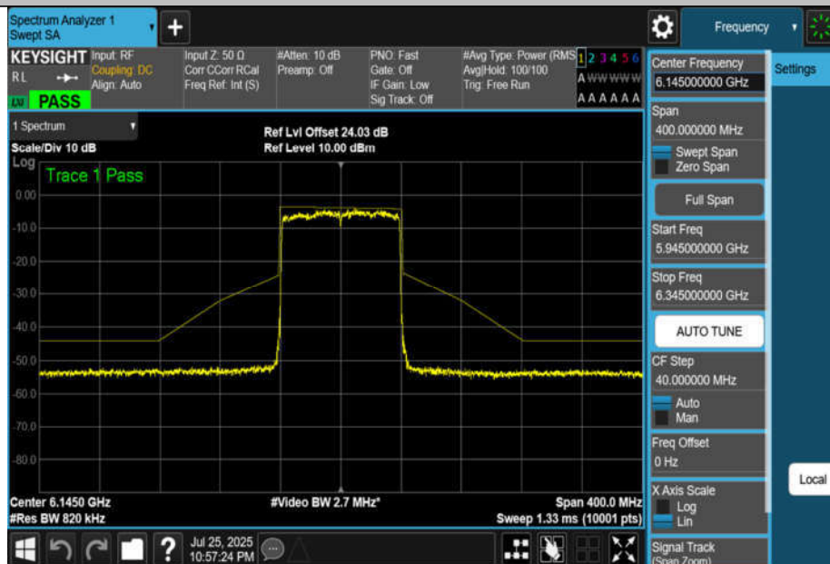
NTNV-11BE80MIMO-Ant2-6145-PASS
