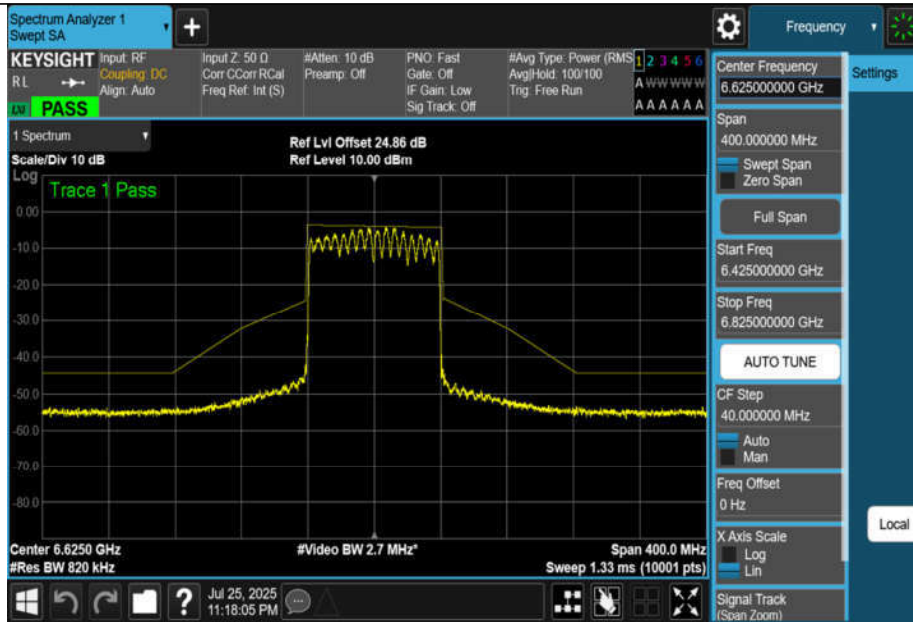
NTNV-11BE80MIMO-Ant3-6625-PASS
