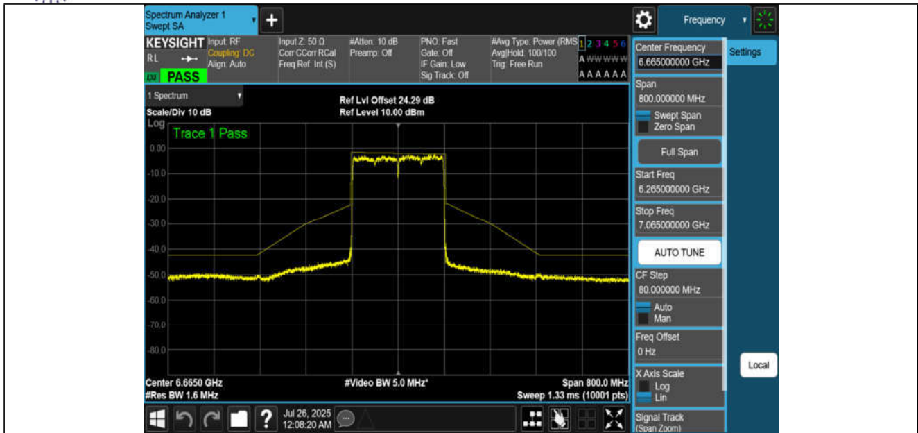
NTNV-11BE160MIMO-Ant1-6665-PASS
