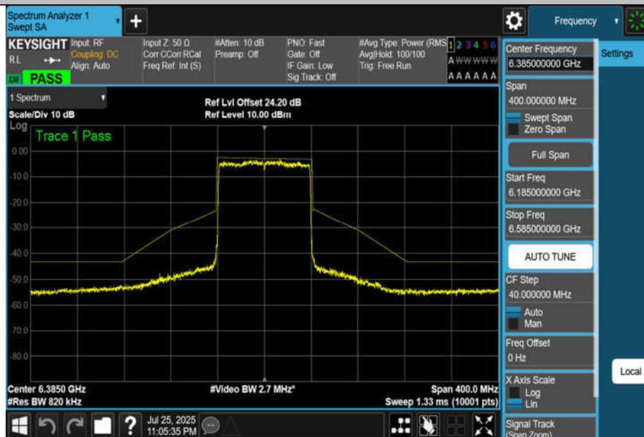
NTNV-11BE80MIMO-Ant4-6385-PASS
