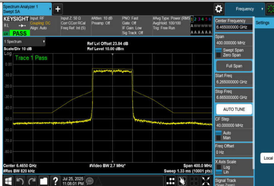
NTNV-11BE80MIMO-Ant2-6465-PASS
