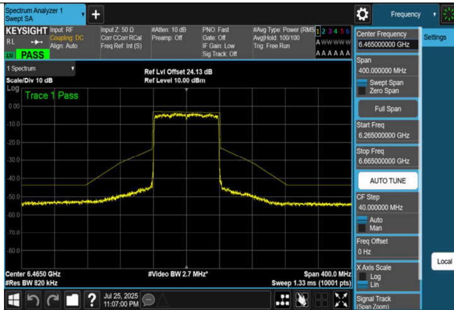
NTNV-11BE80MIMO-Ant1-6465-PASS
