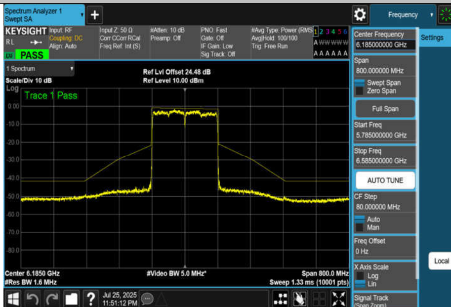
NTNV-11BE160MIMO-Ant2-6185-PASS
