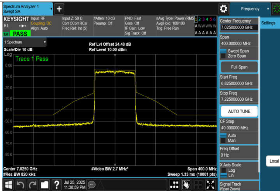
NTNV-11BE80MIMO-Ant1-7025-PASS
