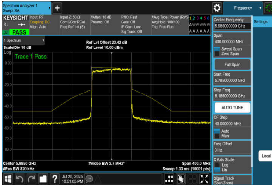
NTNV-11BE80MIMO-Ant1-5985-PASS
