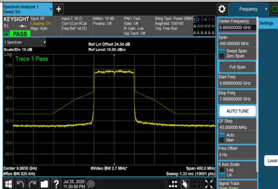
NTNV-11BE80MIMO-Ant2-6865-PASS
