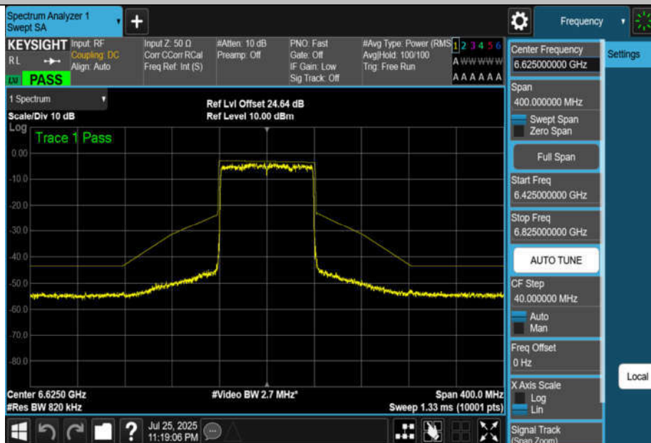
NTNV-11BE80MIMO-Ant4-6625-PASS
