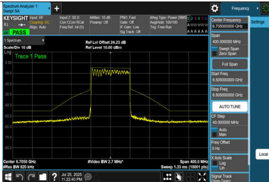
NTNV-11BE80MIMO-Ant3-6705-PASS
