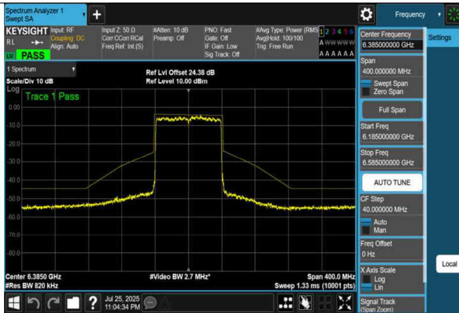
NTNV-11BE80MIMO-Ant3-6385-PASS
