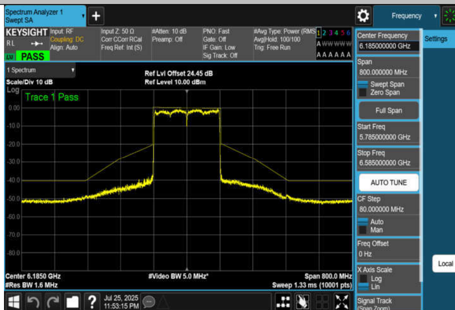
NTNV-11BE160MIMO-Ant4-6185-PASS
