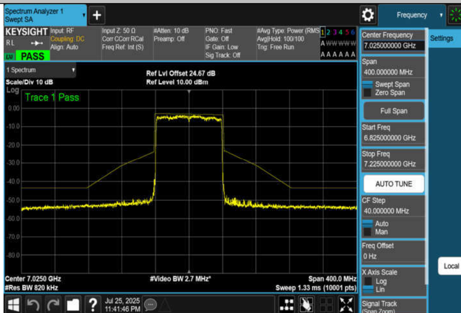
NTNV-11BE80MIMO-Ant4-7025-PASS
