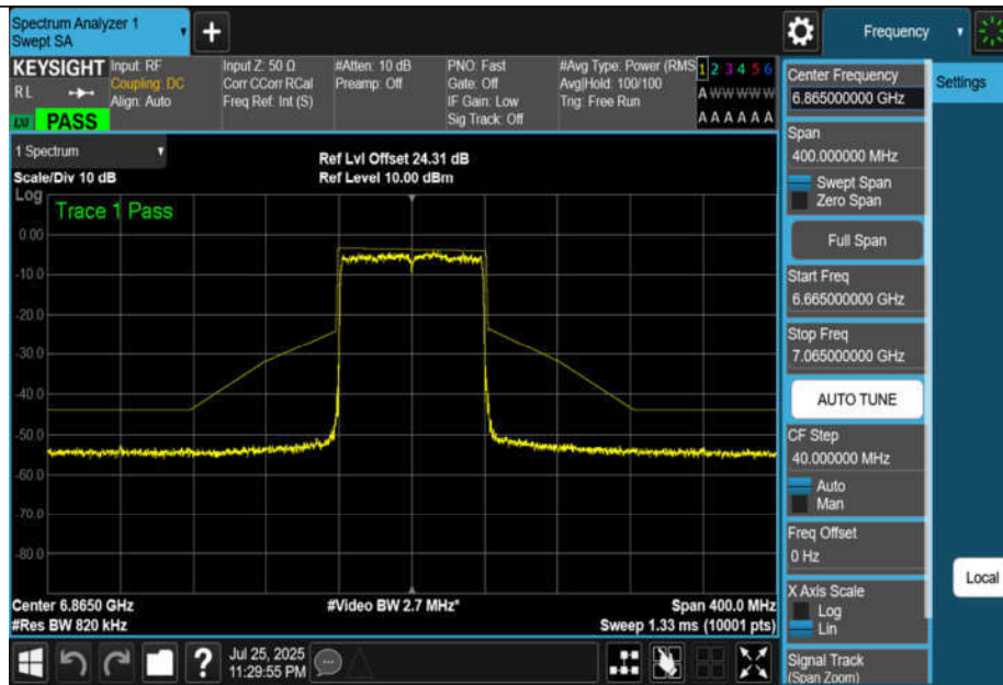
NTNV-11BE80MIMO-Ant1-6865-PASS
