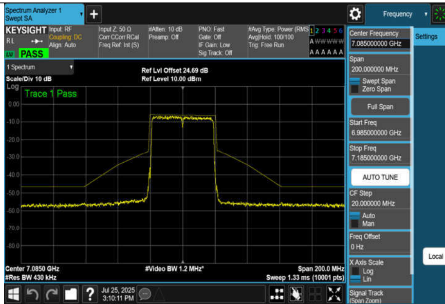
NTNV-11BE40MIMO-Ant1-7085-PASS
