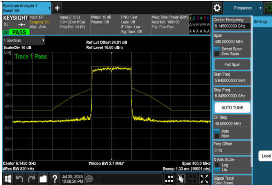
NTNV-11BE80MIMO-Ant3-6145-PASS
