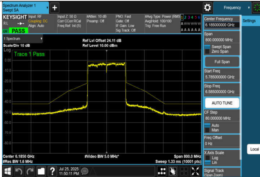
NTNV-11BE160MIMO-Ant1-6185-PASS
