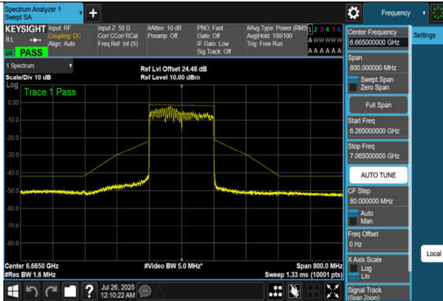
NTNV-11BE160MIMO-Ant3-6665-PASS
