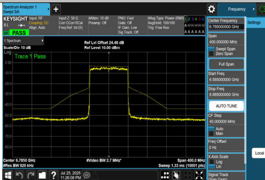
NTNV-11BE80MIMO-Ant2-6785-PASS
