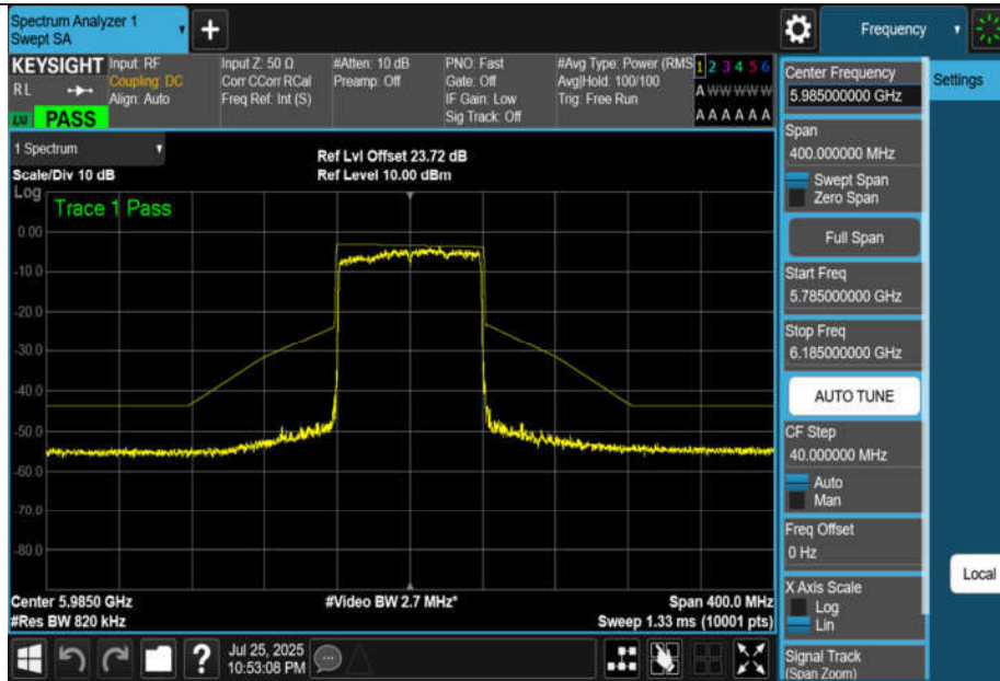
NTNV-11BE80MIMO-Ant3-5985-PASS
