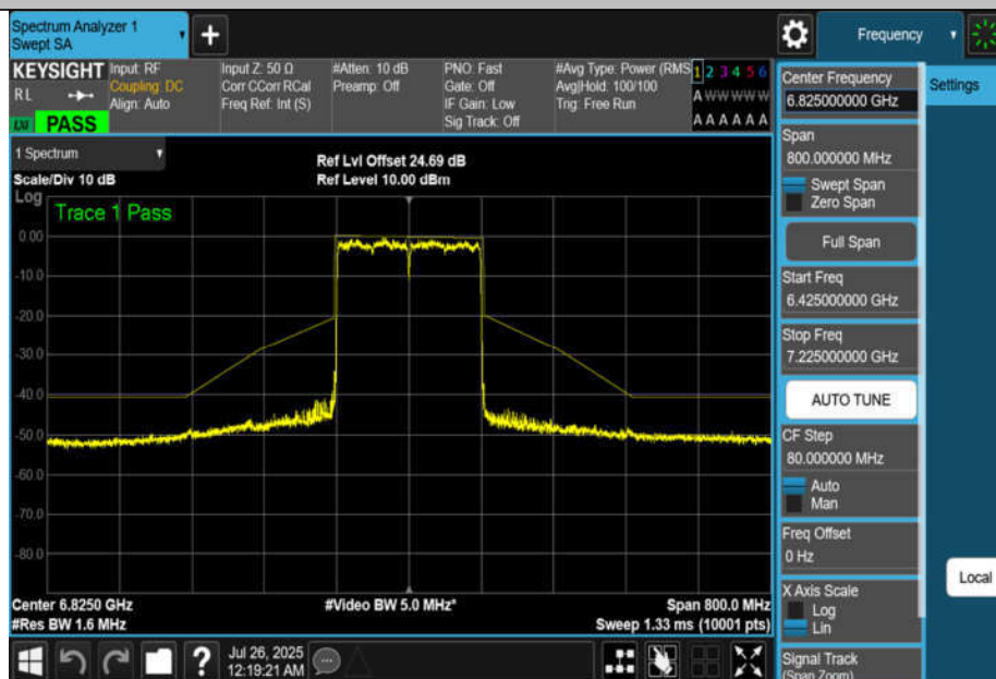
NTNV-11BE160MIMO-Ant4-6825-PASS
