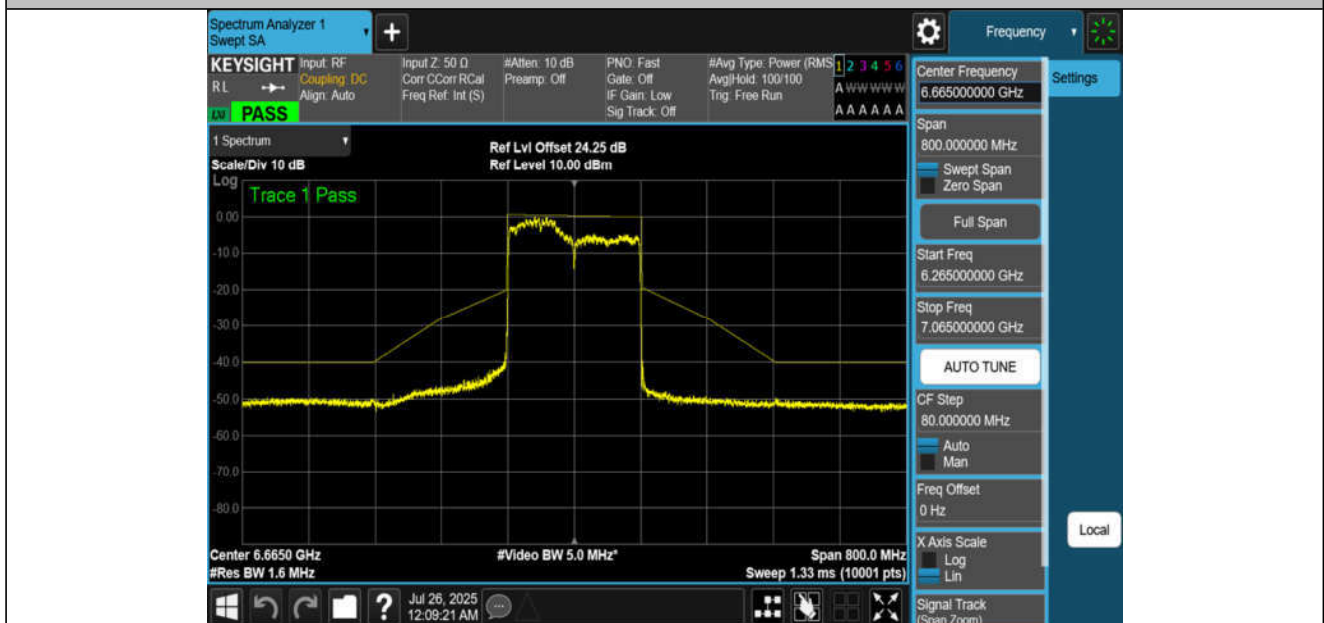
NTNV-11BE160MIMO-Ant2-6665-PASS
