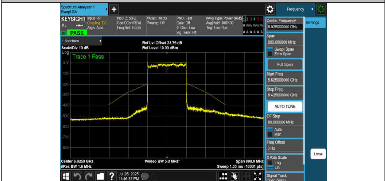
NTNV-11BE160MIMO-Ant4-6025-PASS
