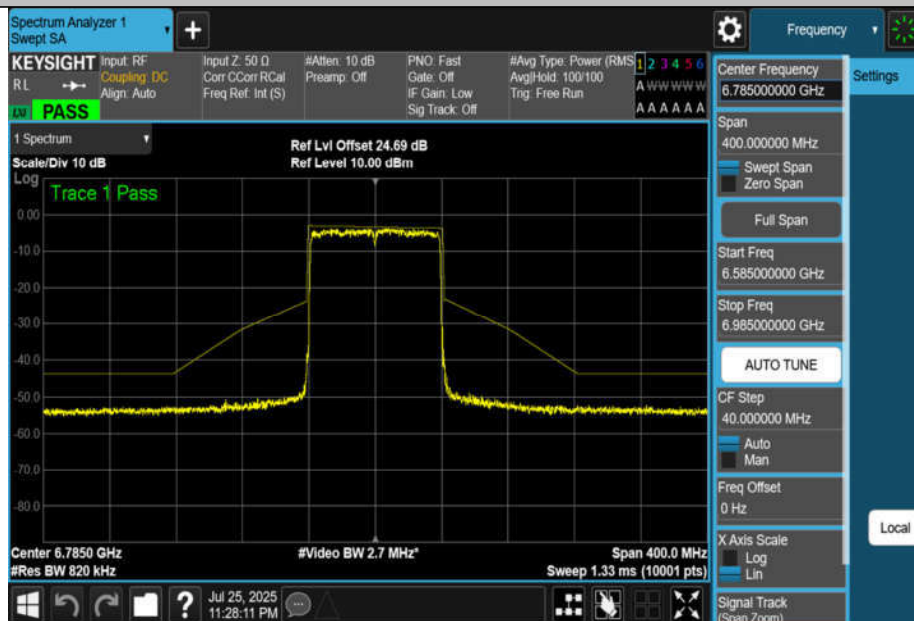
NTNV-11BE80MIMO-Ant4-6785-PASS
