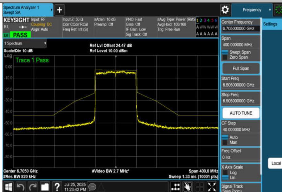
NTNV-11BE80MIMO-Ant4-6705-PASS
