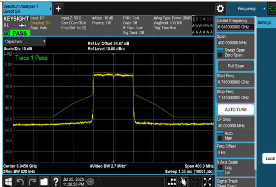
NTNV-11BE80MIMO-Ant3-6945-PASS
