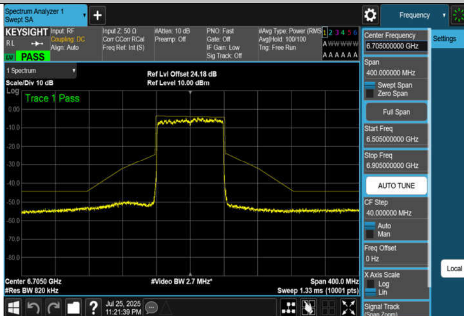
NTNV-11BE80MIMO-Ant2-6705-PASS
