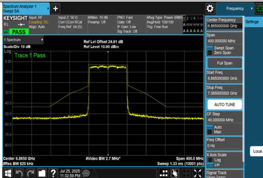
NTNV-11BE80MIMO-Ant4-6865-PASS
