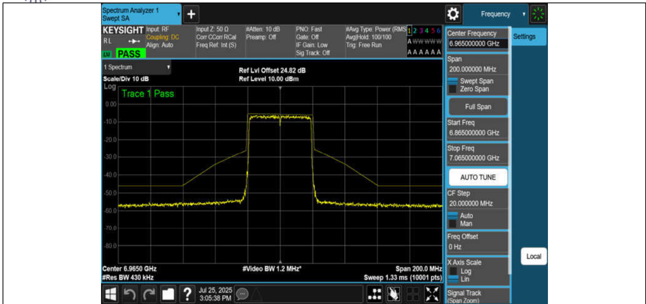
NTNV-11BE40MIMO-Ant1-6965-PASS
