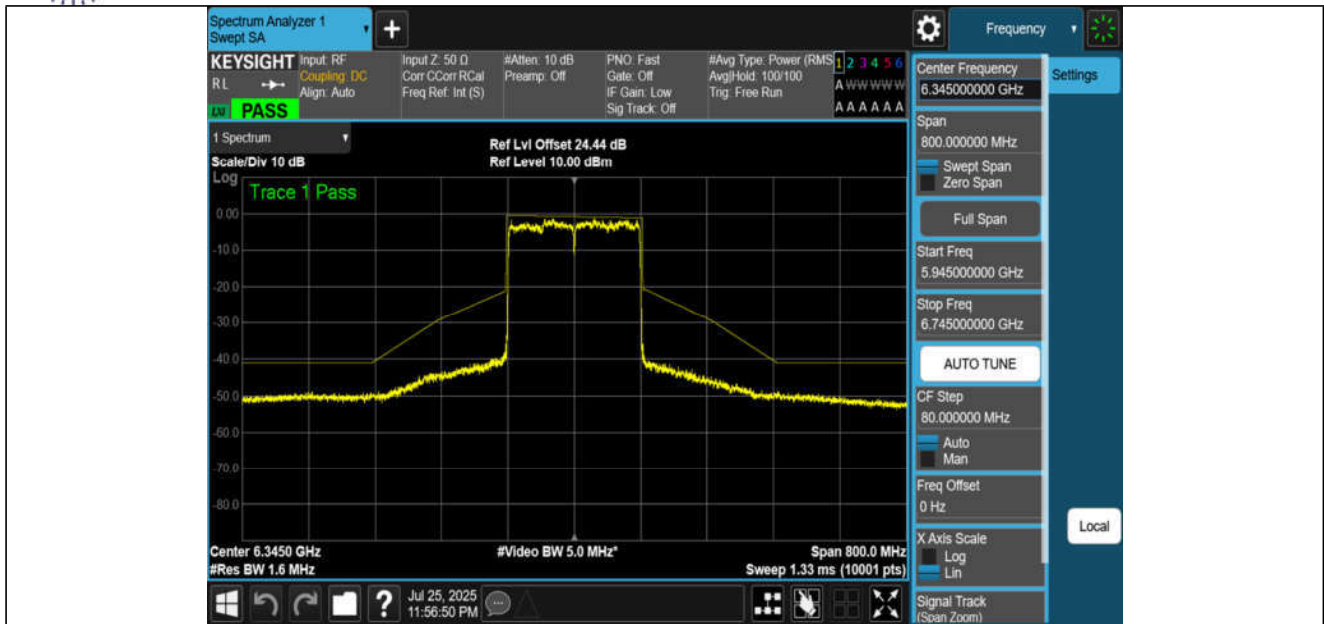
NTNV-11BE160MIMO-Ant3-6345-PASS
