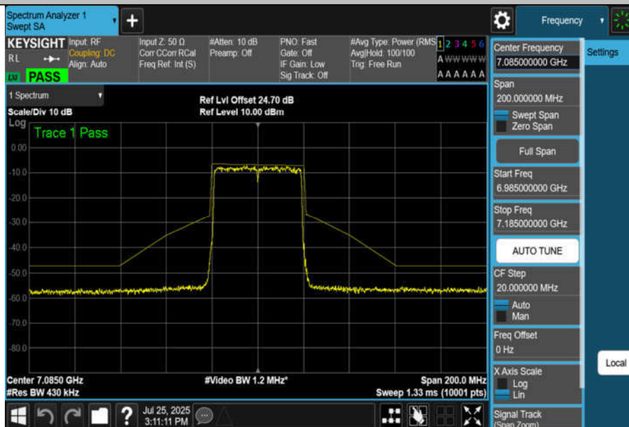
NTNV-11BE40MIMO-Ant2-7085-PASS
