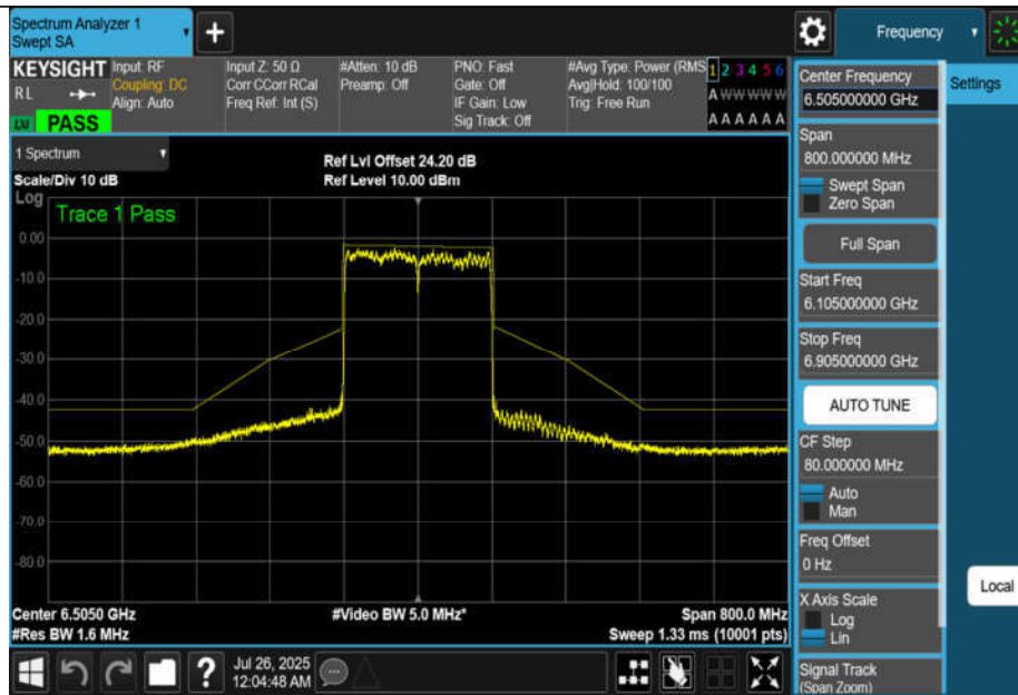
NTNV-11BE160MIMO-Ant3-6505-PASS
