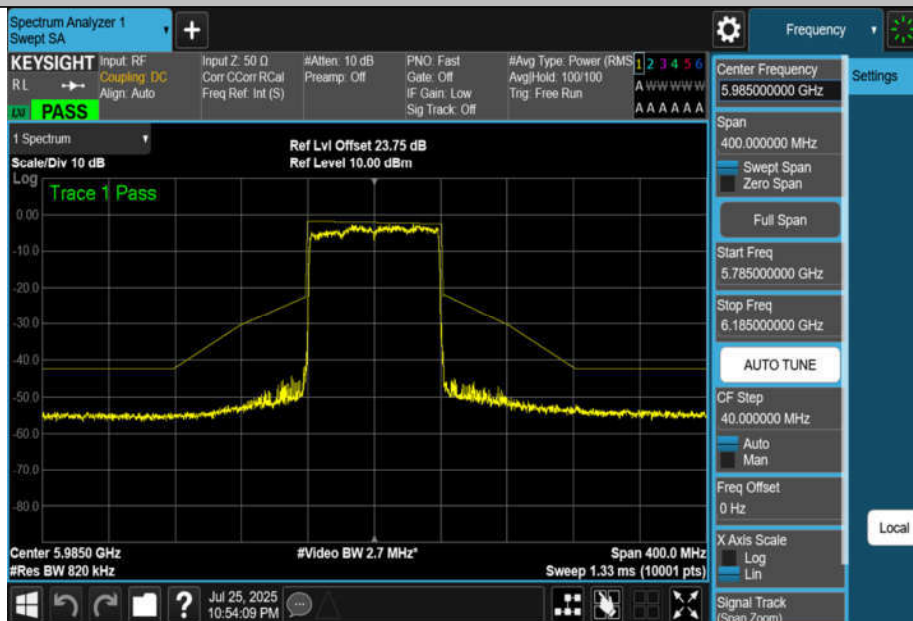
NTNV-11BE80MIMO-Ant4-5985-PASS
