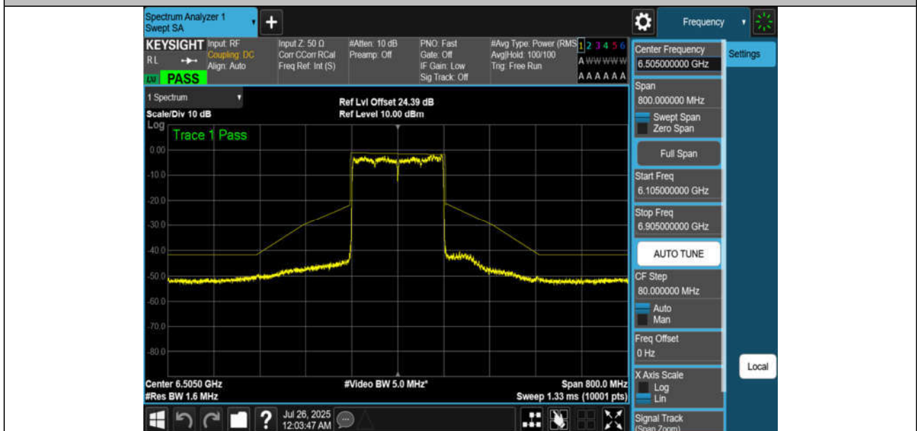
NTNV-11BE160MIMO-Ant2-6505-PASS
