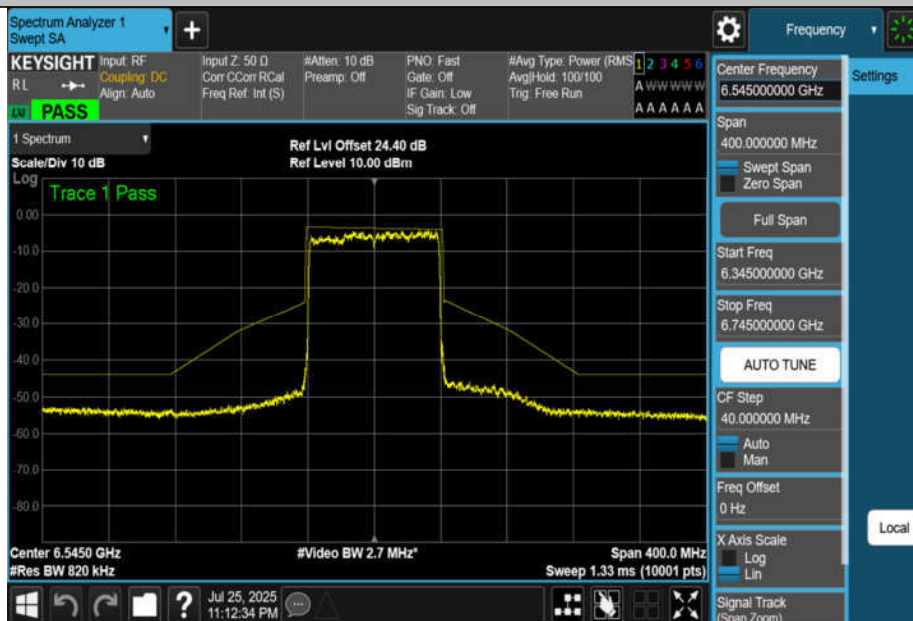
NTNV-11BE80MIMO-Ant2-6545-PASS
