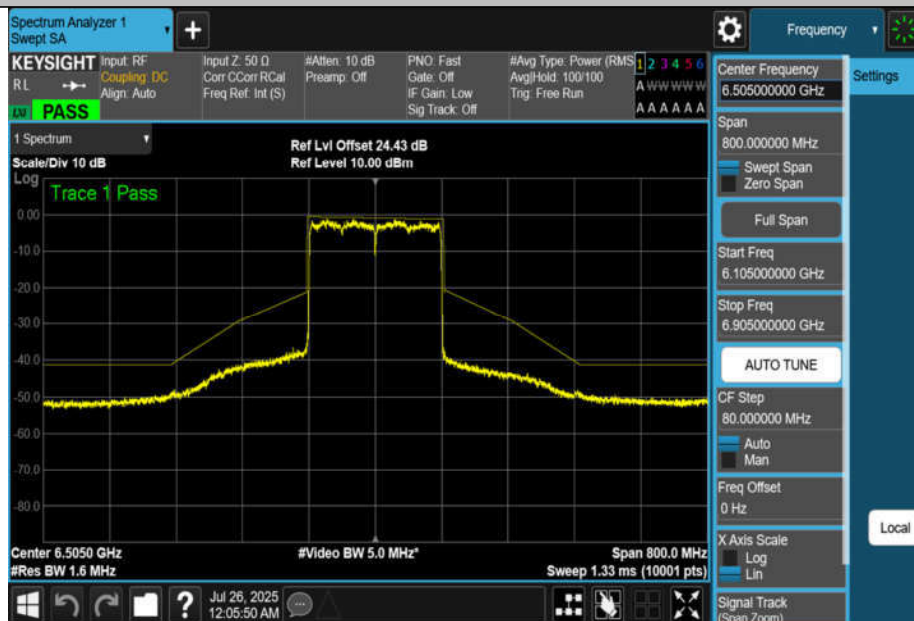
NTNV-11BE160MIMO-Ant4-6505-PASS
