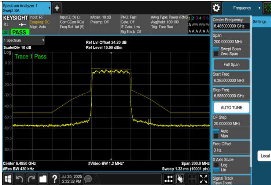
NTNV-11BE40MIMO-Ant3-6485-PASS
