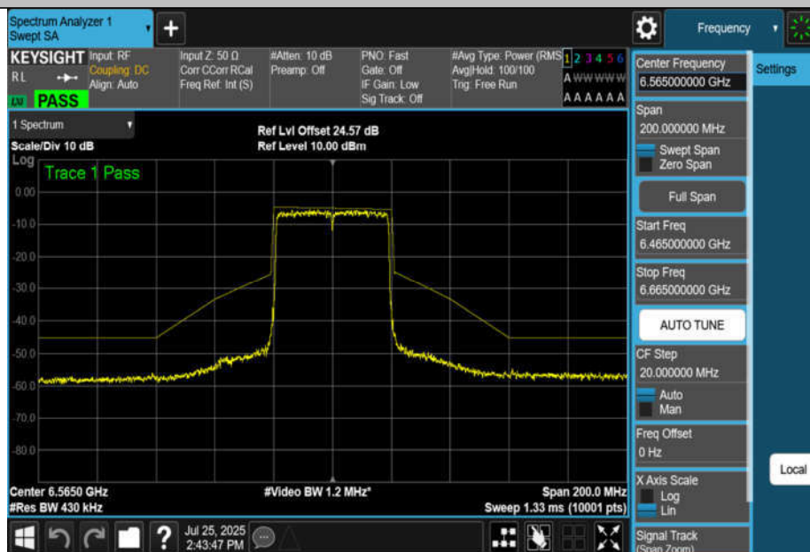
NTNV-11BE40MIMO-Ant4-6565-PASS
