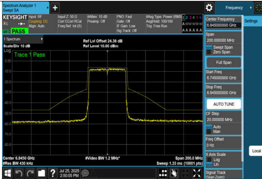
NTNV-11BE40MIMO-Ant1-6845-PASS
