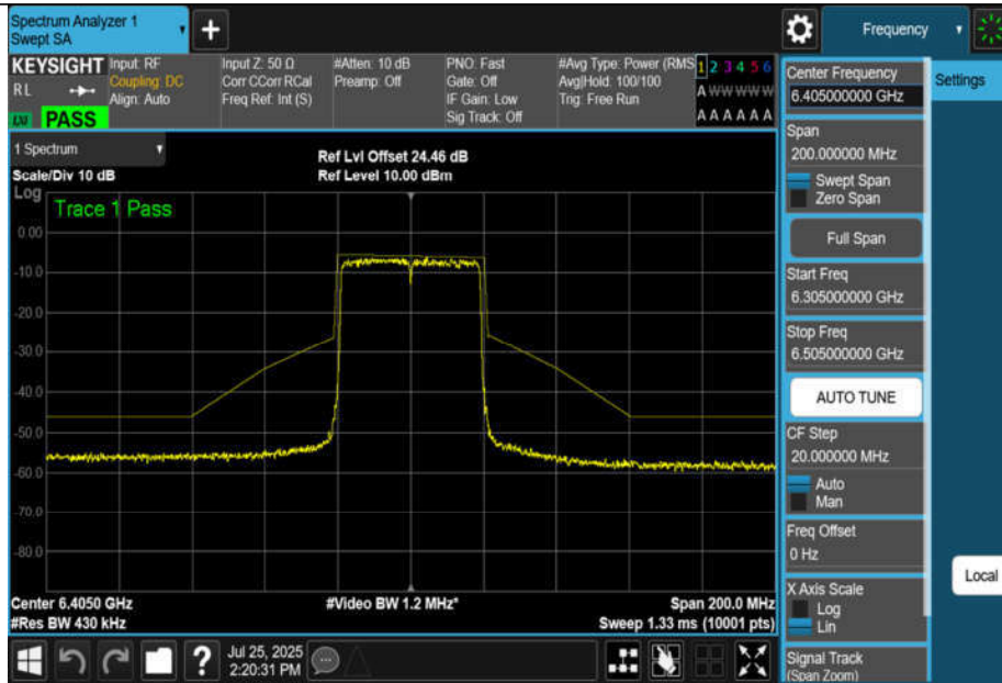
NTNV-11BE40MIMO-Ant1-6405-PASS
