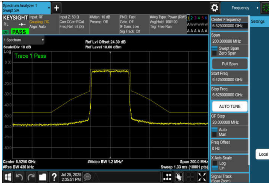
NTNV-11BE40MIMO-Ant1-6525-PASS
