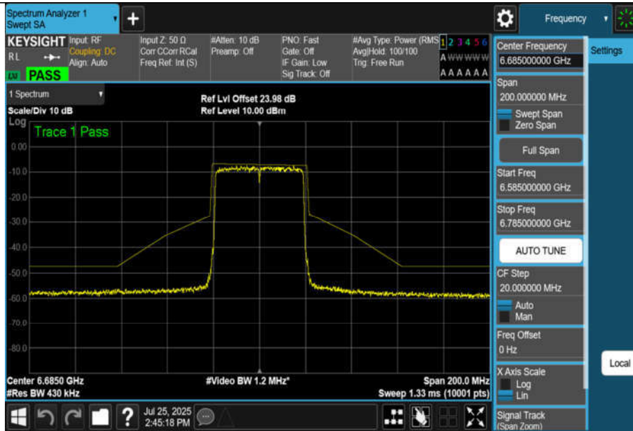
NTNV-11BE40MIMO-Ant1-6685-PASS
