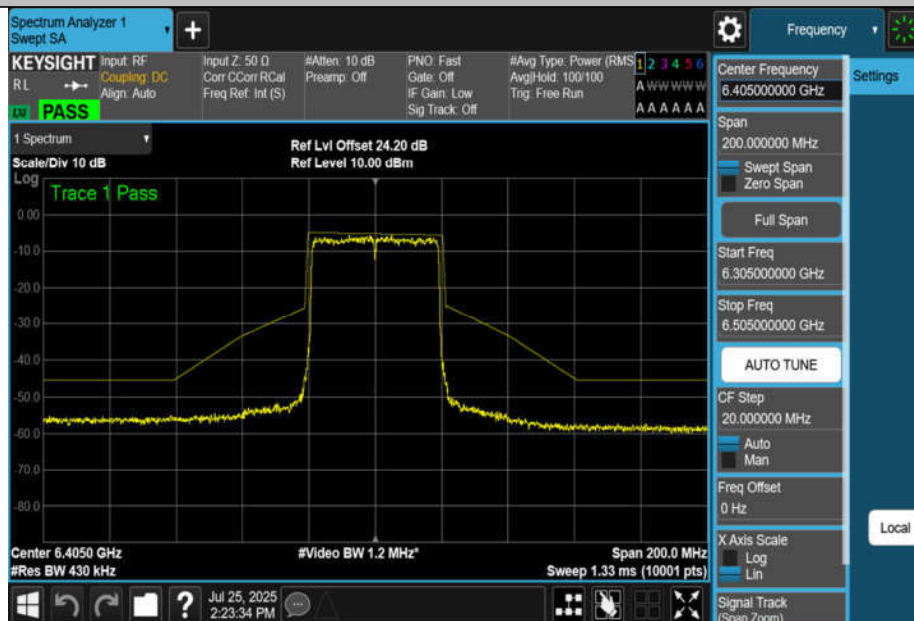
NTNV-11BE40MIMO-Ant4-6405-PASS
