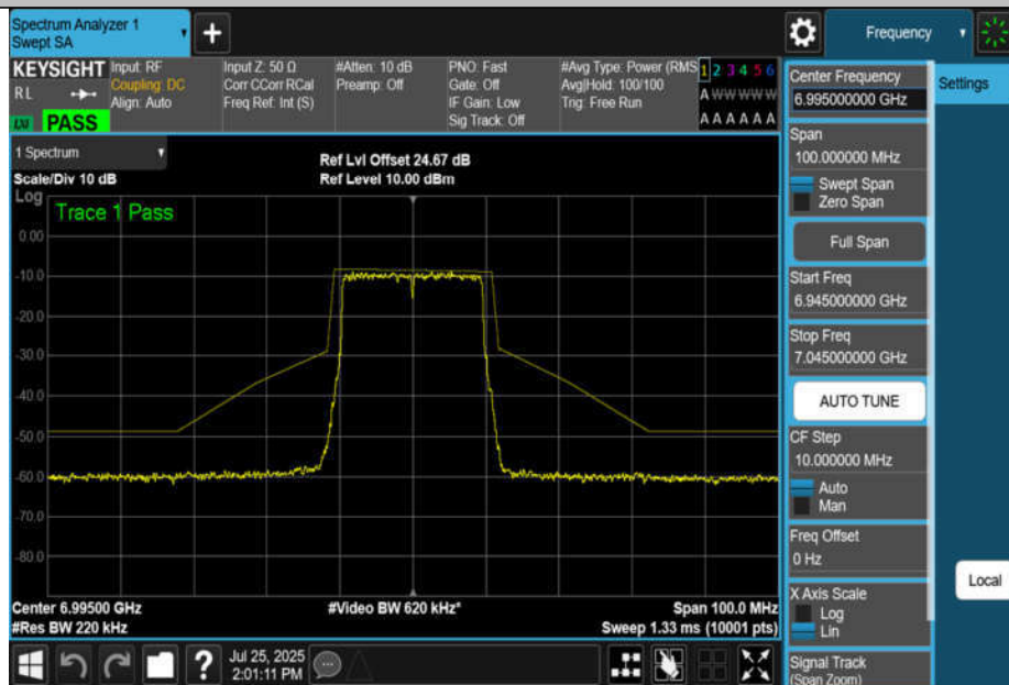
NTNV-11BE20MIMO-Ant4-6995-PASS
