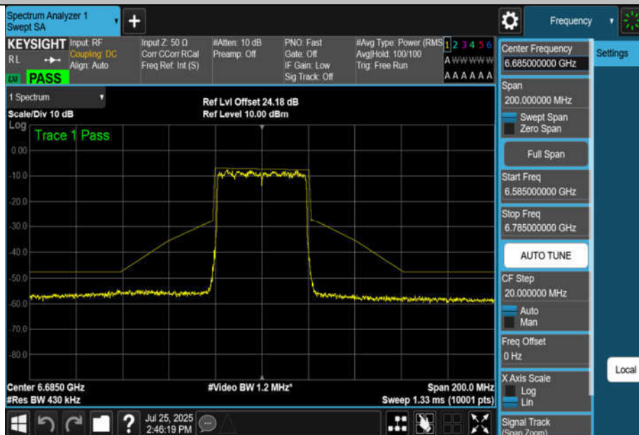
NTNV-11BE40MIMO-Ant2-6685-PASS
