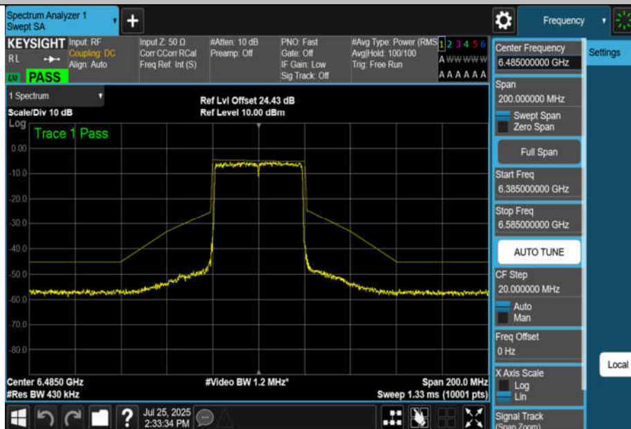
NTNV-11BE40MIMO-Ant4-6485-PASS
