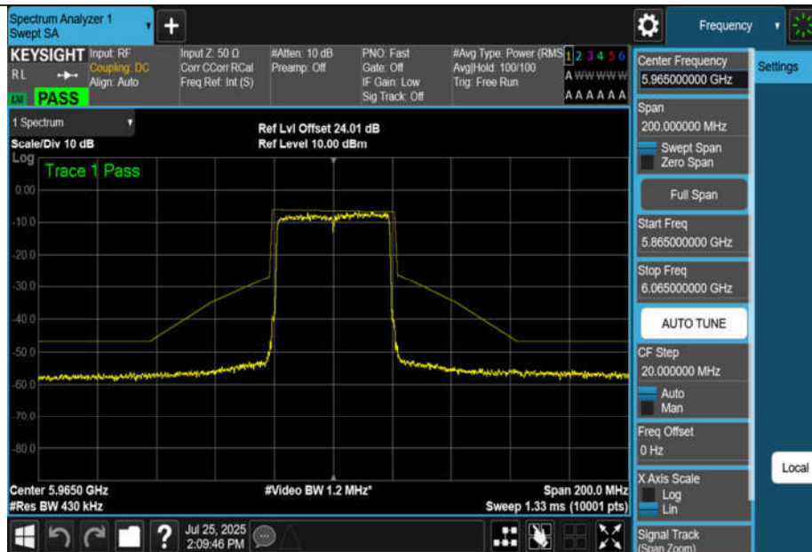
NTNV-11BE40MIMO-Ant1-5965-PASS
