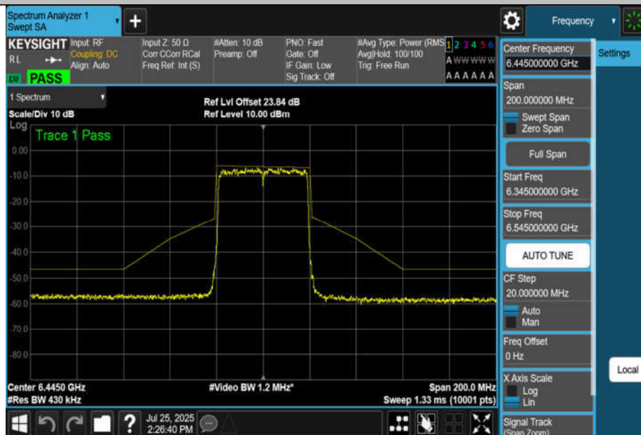
NTNV-11BE40MIMO-Ant2-6445-PASS
