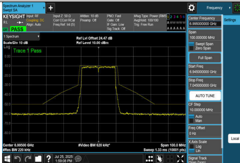
NTNV-11BE20MIMO-Ant2-6995-PASS
