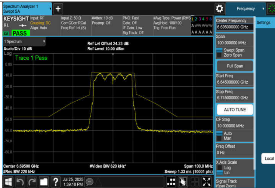
NTNV-11BE20MIMO-Ant3-6695-PASS
