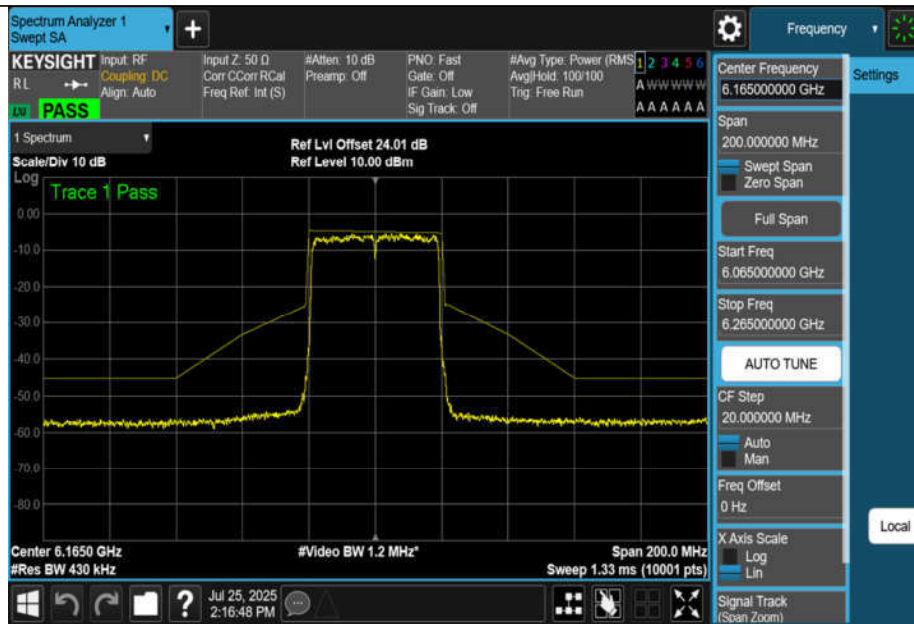
NTNV-11BE40MIMO-Ant3-6165-PASS
