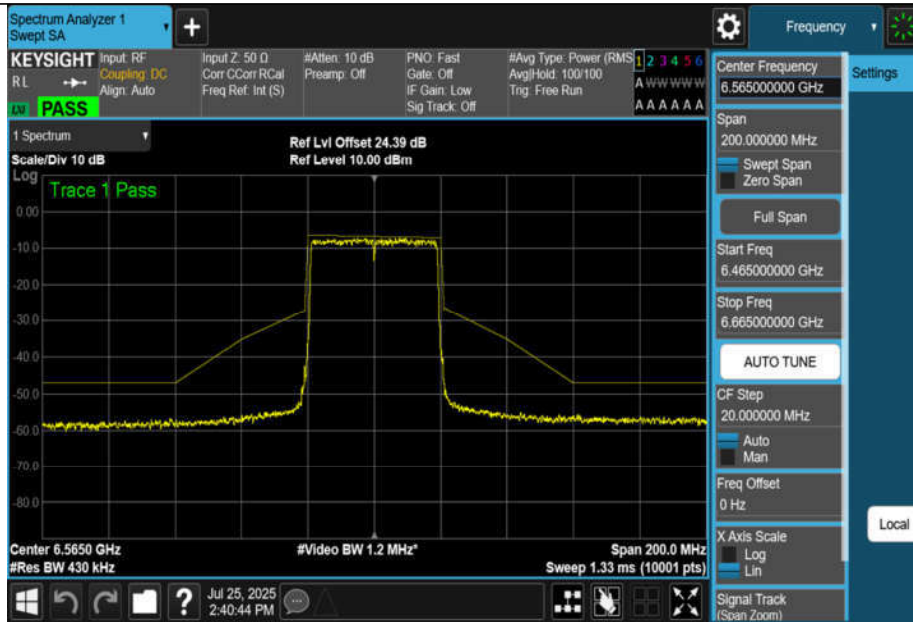
NTNV-11BE40MIMO-Ant1-6565-PASS
