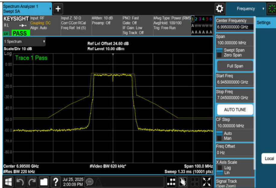
NTNV-11BE20MIMO-Ant3-6995-PASS
