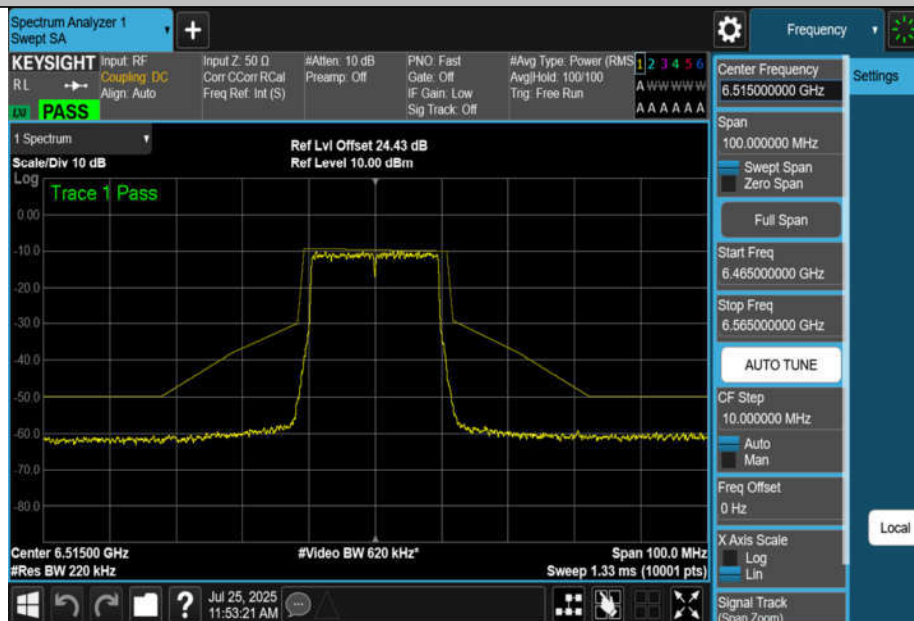
NTNV-11BE20MIMO-Ant4-6515-PASS
