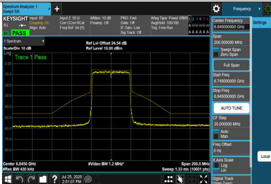
NTNV-11BE40MIMO-Ant2-6845-PASS
