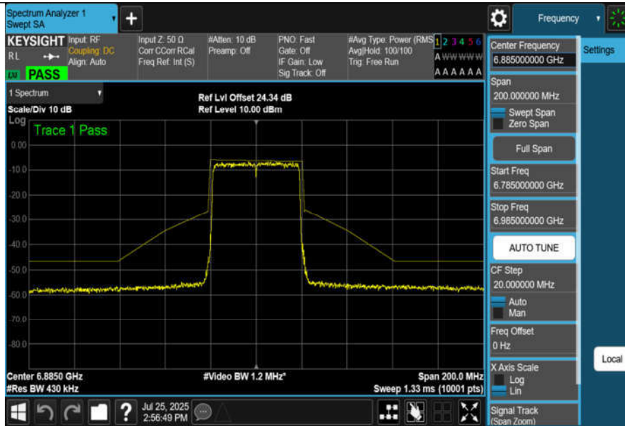
NTNV-11BE40MIMO-Ant1-6885-PASS
