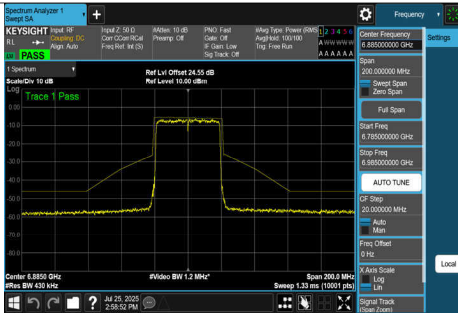
NTNV-11BE40MIMO-Ant3-6885-PASS
