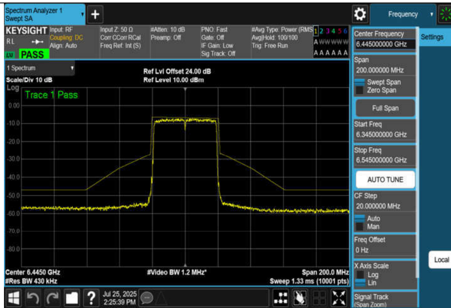
NTNV-11BE40MIMO-Ant1-6445-PASS
