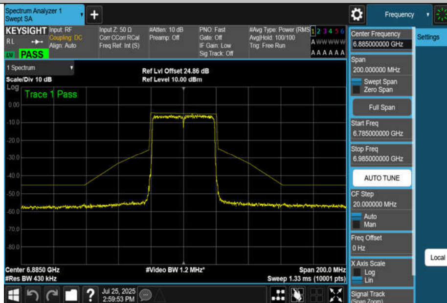
NTNV-11BE40MIMO-Ant4-6885-PASS
