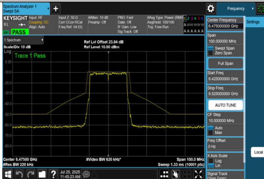
NTNV-11BE20MIMO-Ant2-6475-PASS
