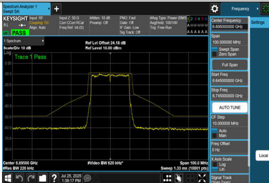
NTNV-11BE20MIMO-Ant2-6695-PASS
