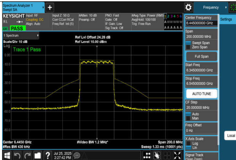
NTNV-11BE40MIMO-Ant3-6445-PASS
