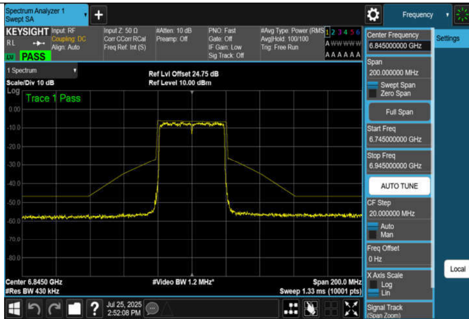
NTNV-11BE40MIMO-Ant3-6845-PASS
