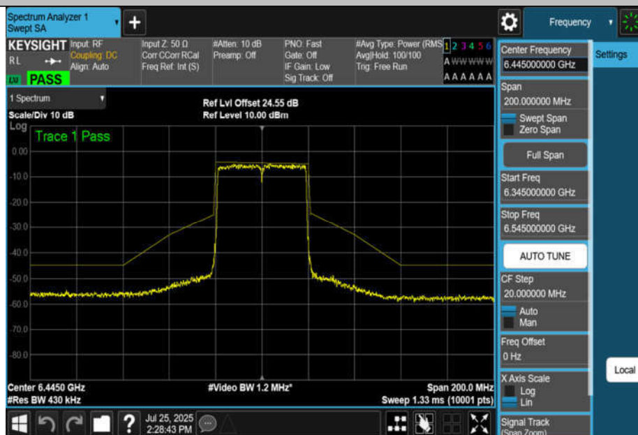
NTNV-11BE40MIMO-Ant4-6445-PASS
