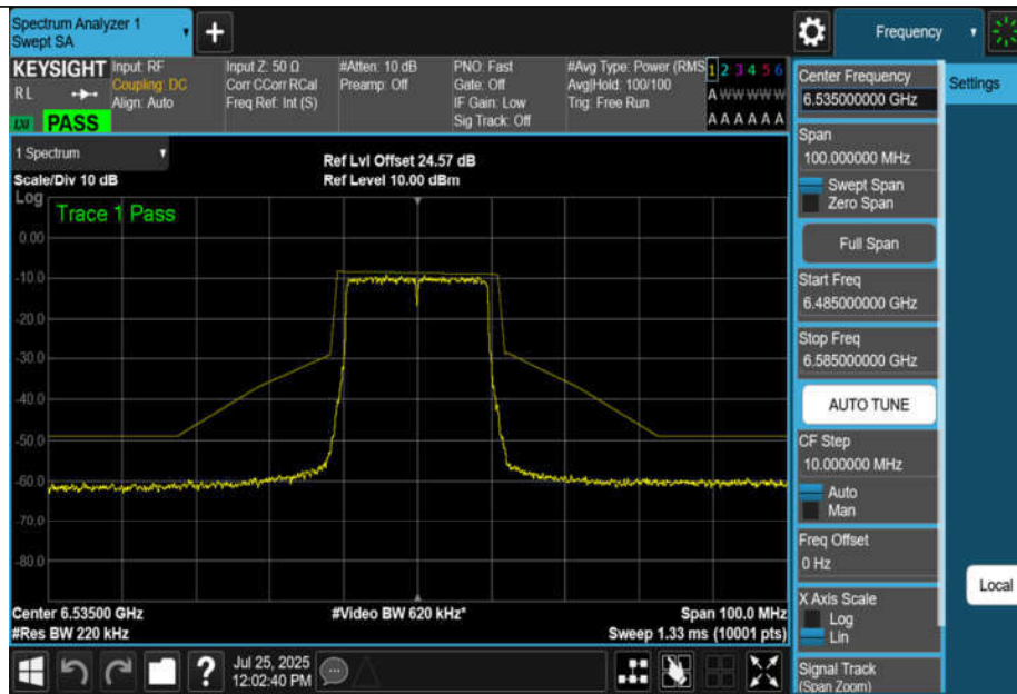
NTNV-11BE20MIMO-Ant4-6535-PASS
