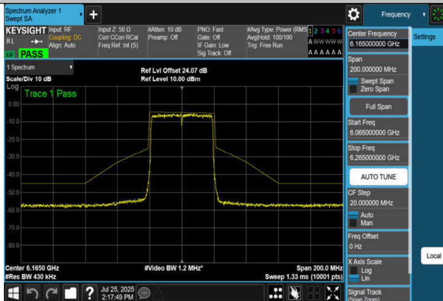
NTNV-11BE40MIMO-Ant4-6165-PASS
