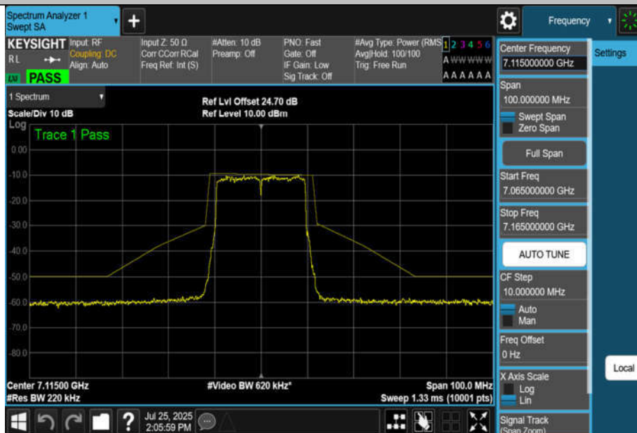
NTNV-11BE20MIMO-Ant2-7115-PASS
