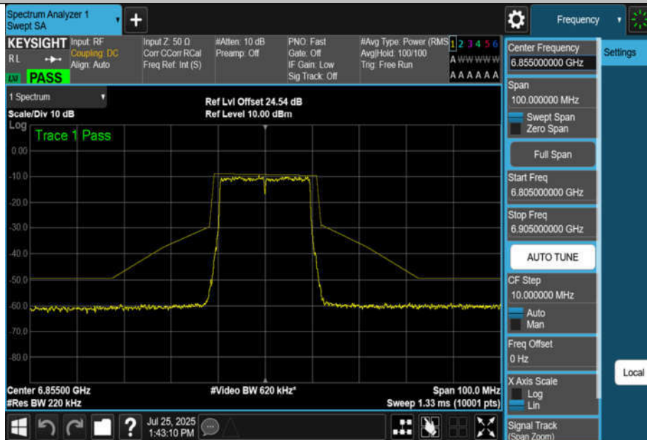
NTNV-11BE20MIMO-Ant2-6855-PASS
