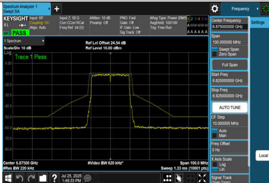
NTNV-11BE20MIMO-Ant2-6875-PASS
