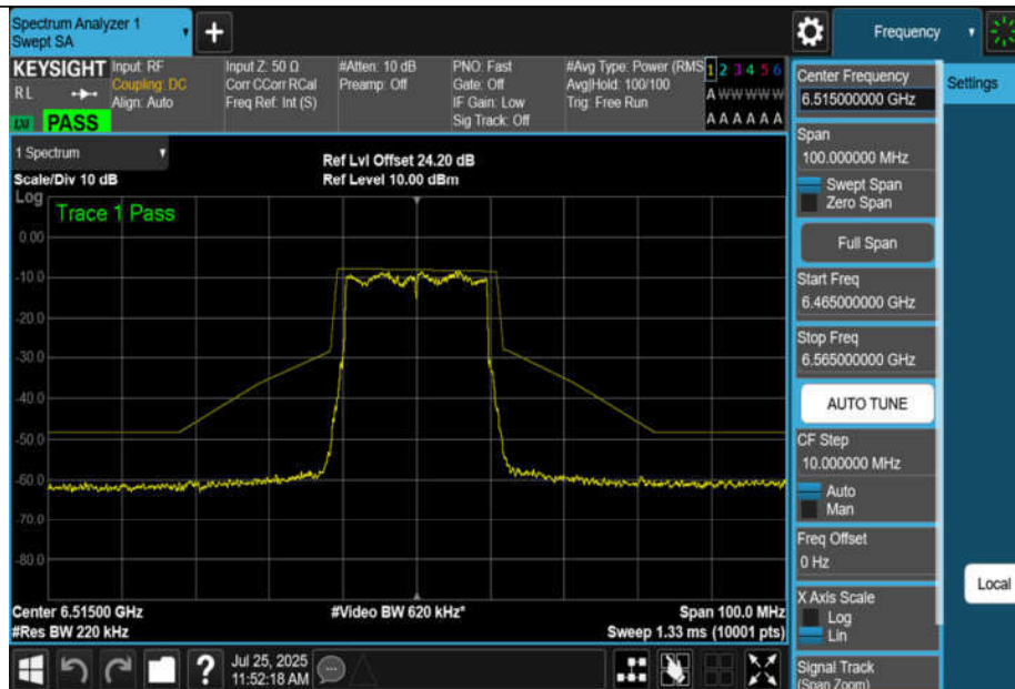
NTNV-11BE20MIMO-Ant3-6515-PASS
