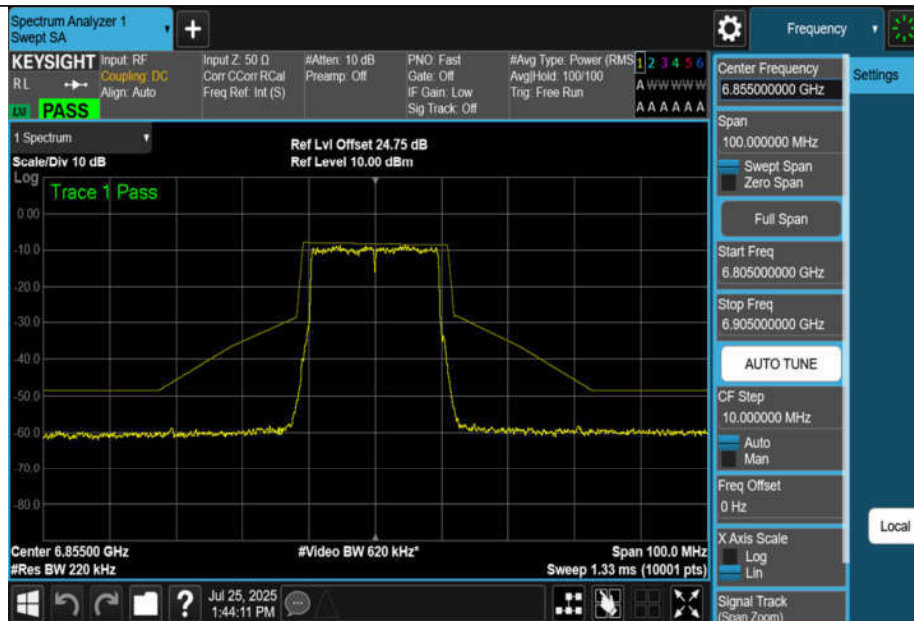
NTNV-11BE20MIMO-Ant3-6855-PASS
