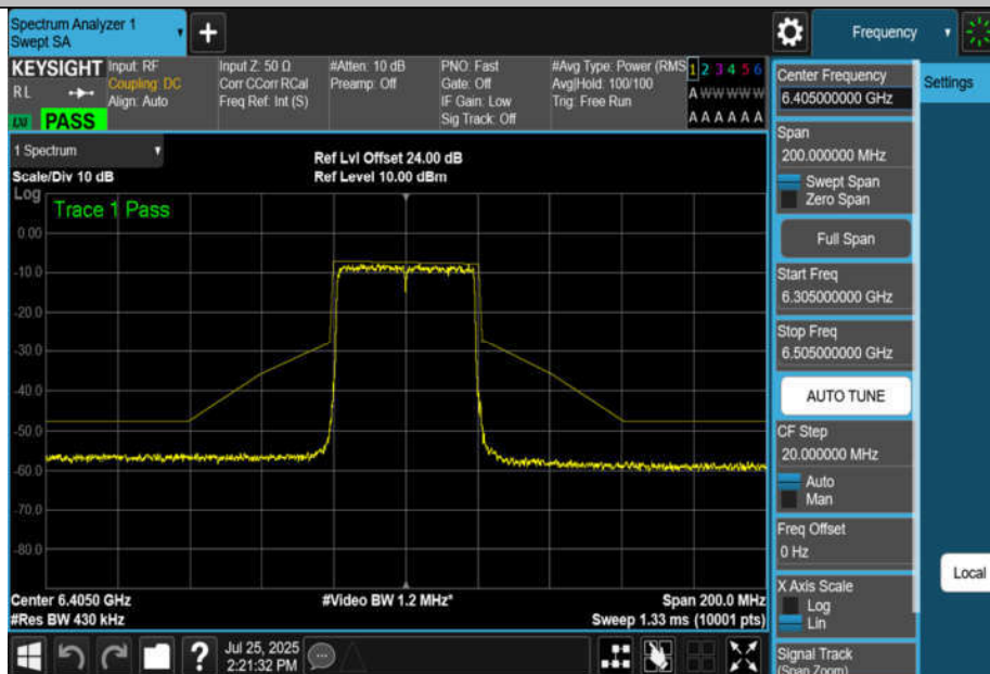
NTNV-11BE40MIMO-Ant2-6405-PASS
