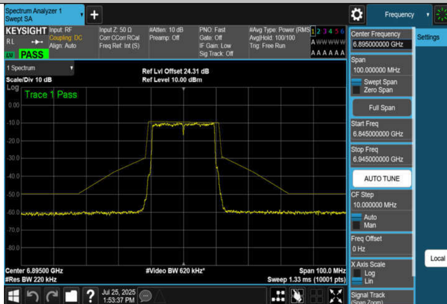
NTNV-11BE20MIMO-Ant2-6895-PASS
