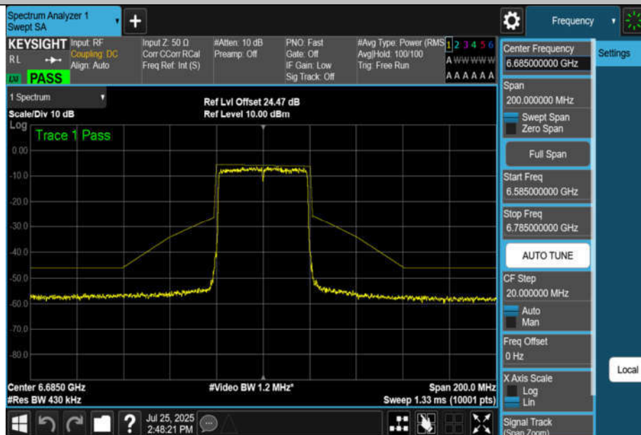
NTNV-11BE40MIMO-Ant4-6685-PASS
