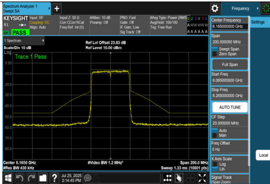
NTNV-11BE40MIMO-Ant1-6165-PASS
