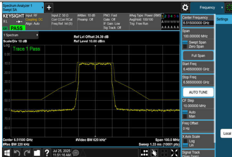
NTNV-11BE20MIMO-Ant2-6515-PASS
