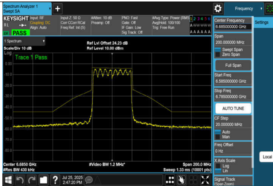
NTNV-11BE40MIMO-Ant3-6685-PASS
