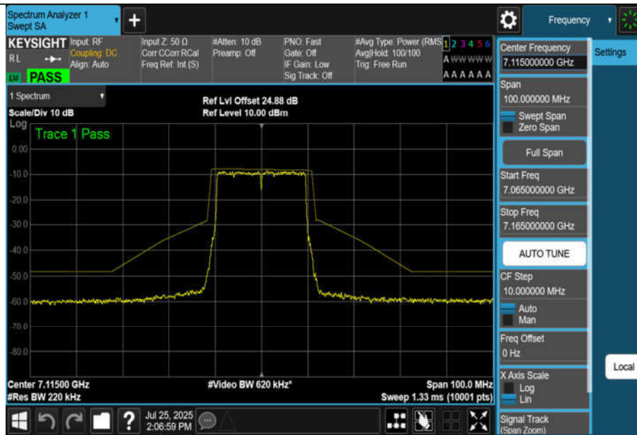
NTNV-11BE20MIMO-Ant3-7115-PASS
