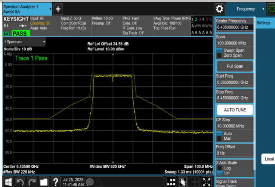
NTNV-11BE20MIMO-Ant4-6435-PASS
