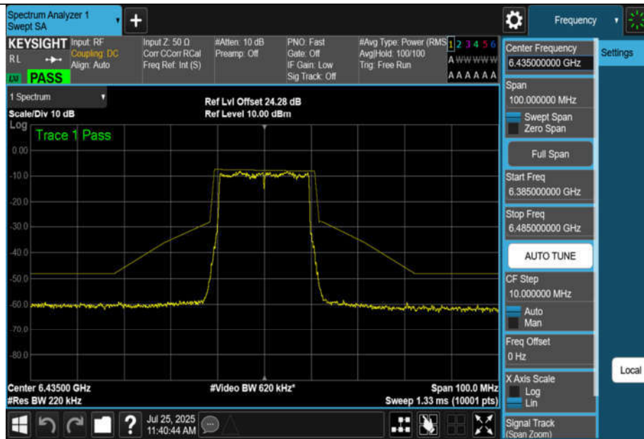
NTNV-11BE20MIMO-Ant3-6435-PASS
