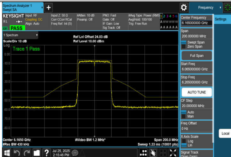
NTNV-11BE40MIMO-Ant2-6165-PASS
