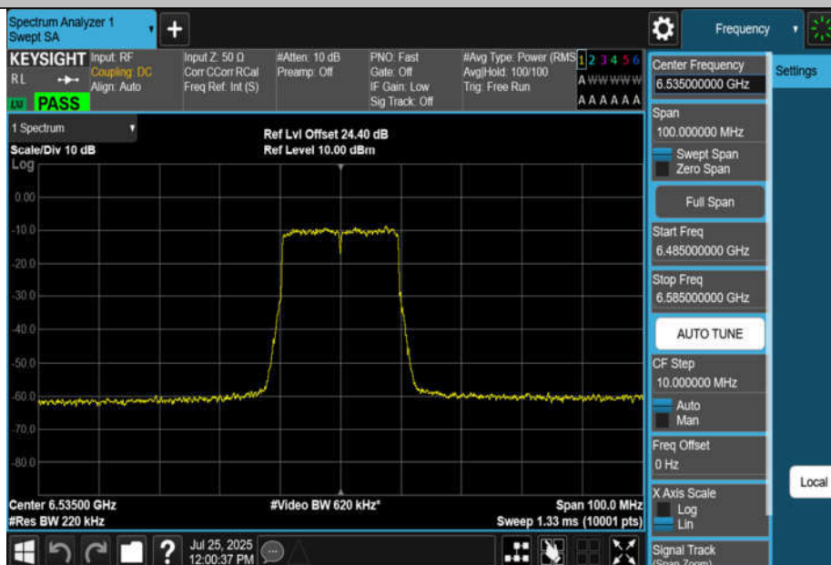
NTNV-11BE20MIMO-Ant2-6535-PASS
