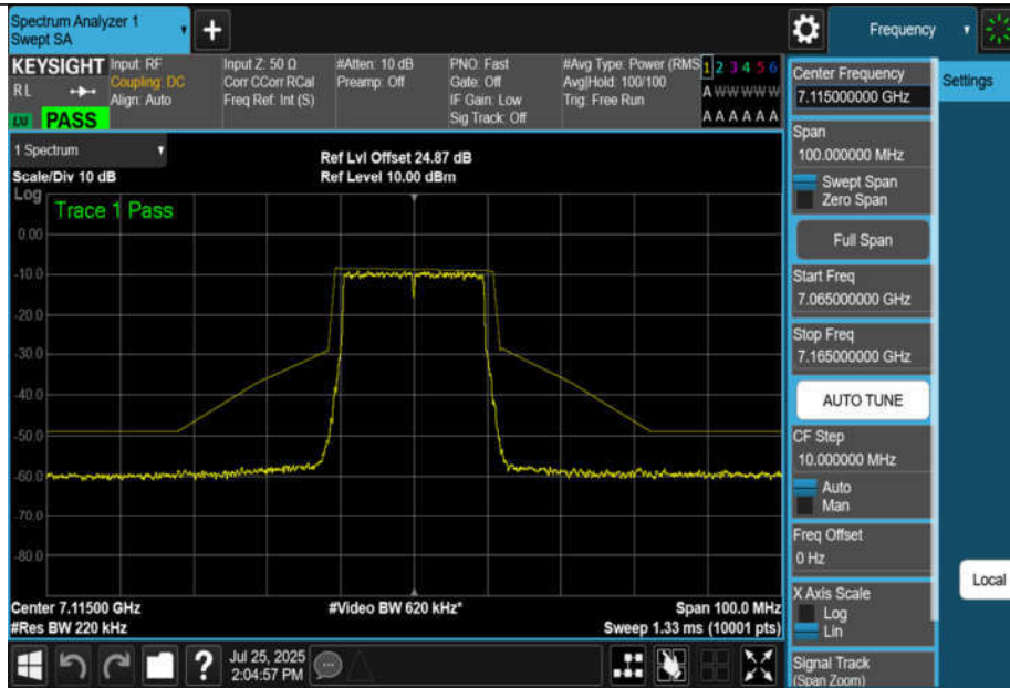
NTNV-11BE20MIMO-Ant1-7115-PASS
