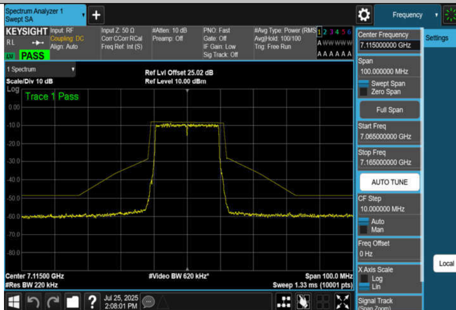
NTNV-11BE20MIMO-Ant4-7115-PASS
