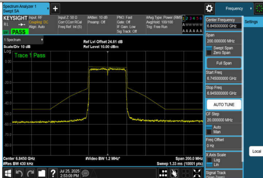
NTNV-11BE40MIMO-Ant4-6845-PASS
