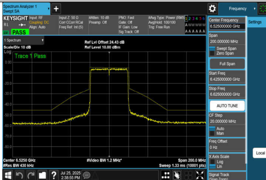
NTNV-11BE40MIMO-Ant4-6525-PASS
