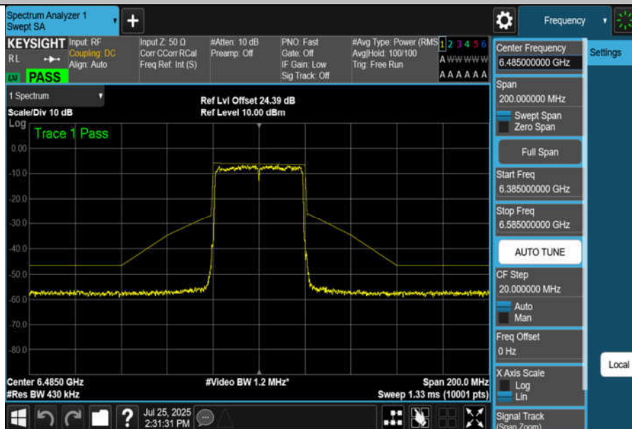
NTNV-11BE40MIMO-Ant2-6485-PASS
