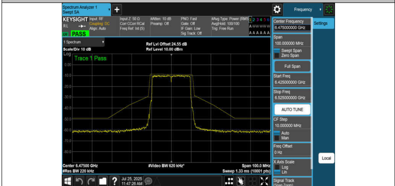
NTNV-11BE20MIMO-Ant4-6475-PASS
