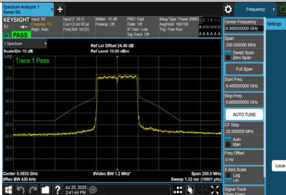
NTNV-11BE40MIMO-Ant2-6565-PASS
