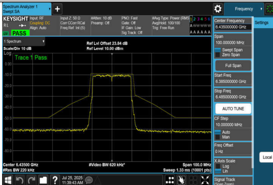
NTNV-11BE20MIMO-Ant2-6435-PASS
