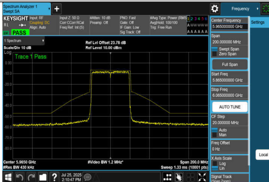
NTNV-11BE40MIMO-Ant2-5965-PASS
