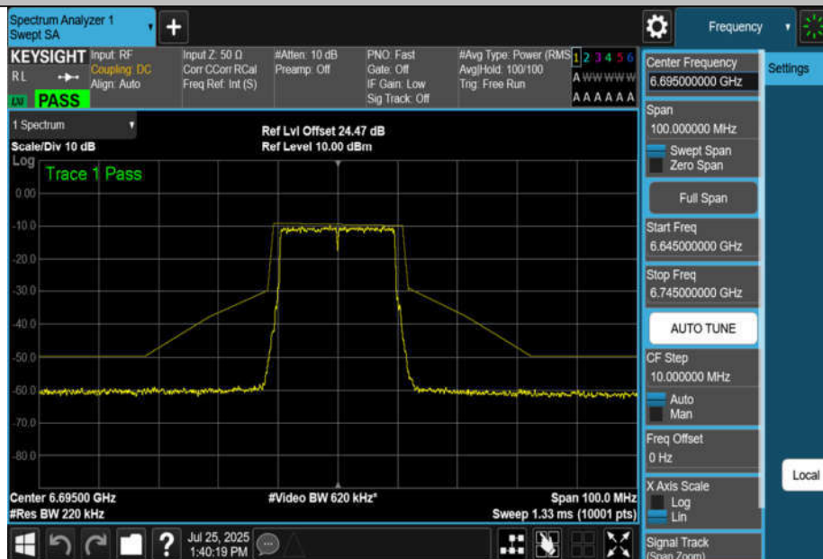
NTNV-11BE20MIMO-Ant4-6695-PASS
