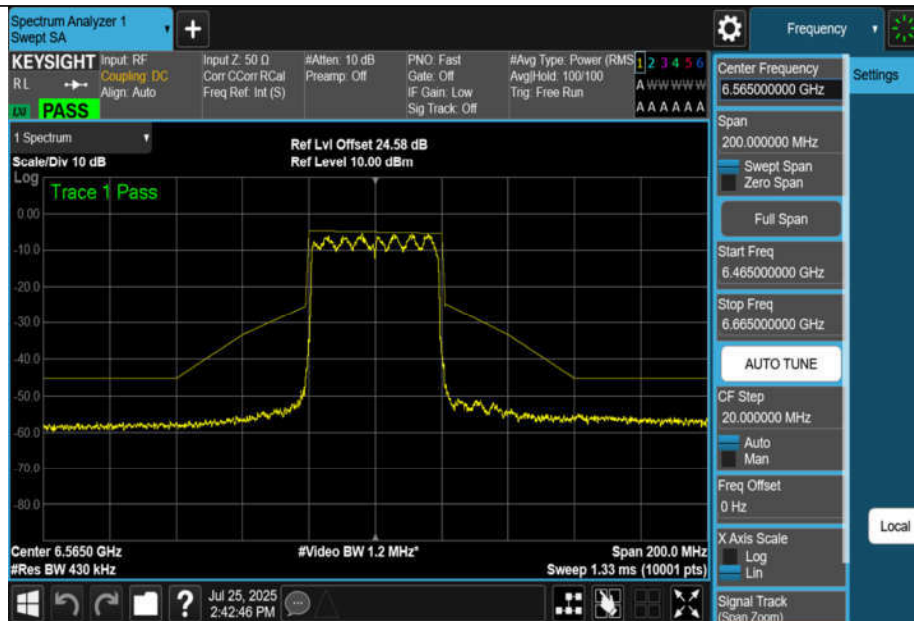
NTNV-11BE40MIMO-Ant3-6565-PASS
