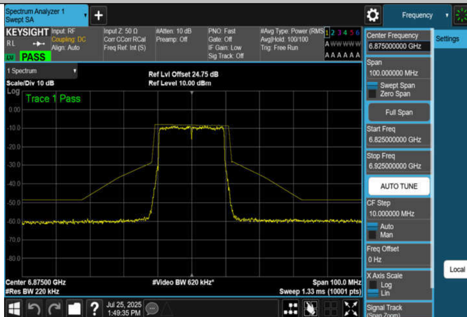
NTNV-11BE20MIMO-Ant3-6875-PASS
