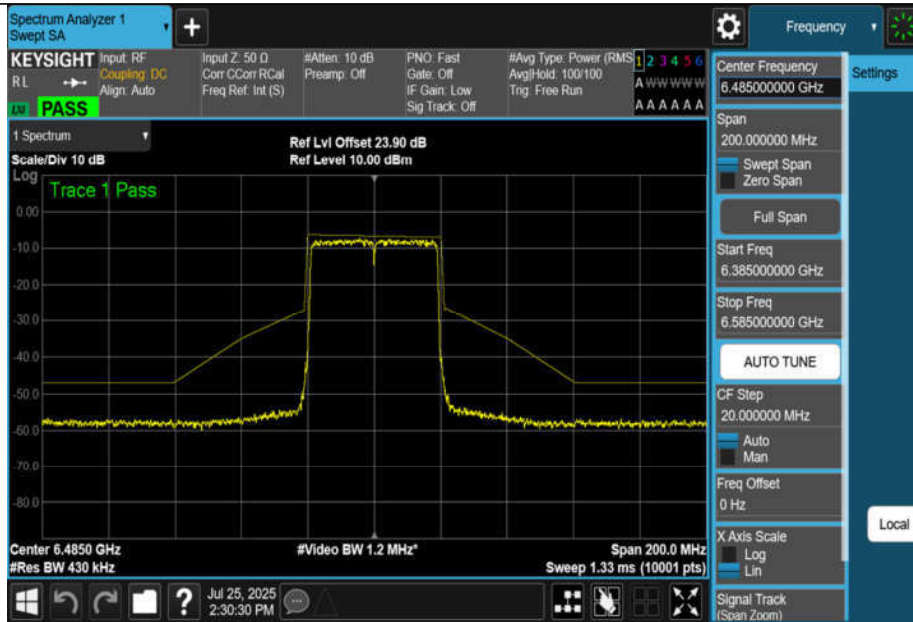
NTNV-11BE40MIMO-Ant1-6485-PASS
