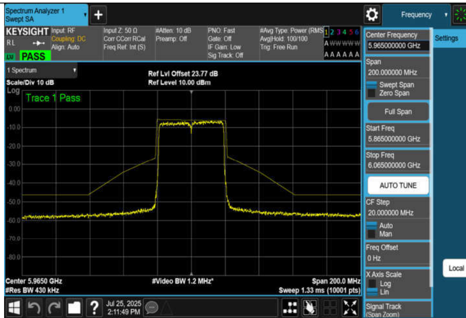
NTNV-11BE40MIMO-Ant3-5965-PASS
