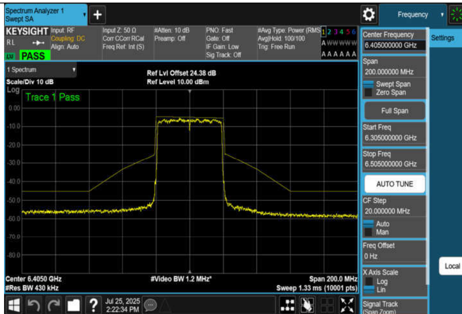
NTNV-11BE40MIMO-Ant3-6405-PASS
