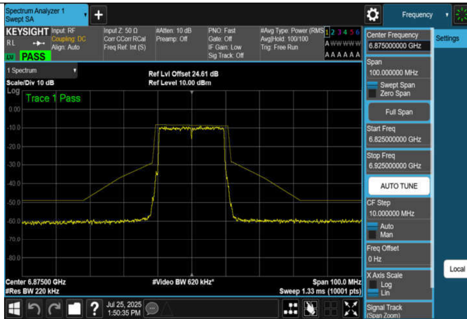
NTNV-11BE20MIMO-Ant4-6875-PASS
