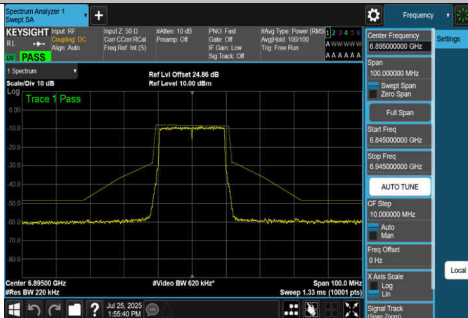
NTNV-11BE20MIMO-Ant4-6895-PASS
