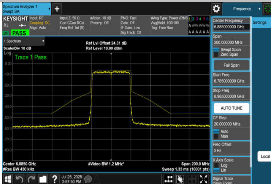
NTNV-11BE40MIMO-Ant2-6885-PASS
