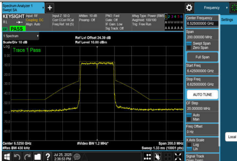
NTNV-11BE40MIMO-Ant2-6525-PASS
