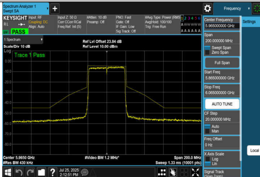
NTNV-11BE40MIMO-Ant4-5965-PASS
