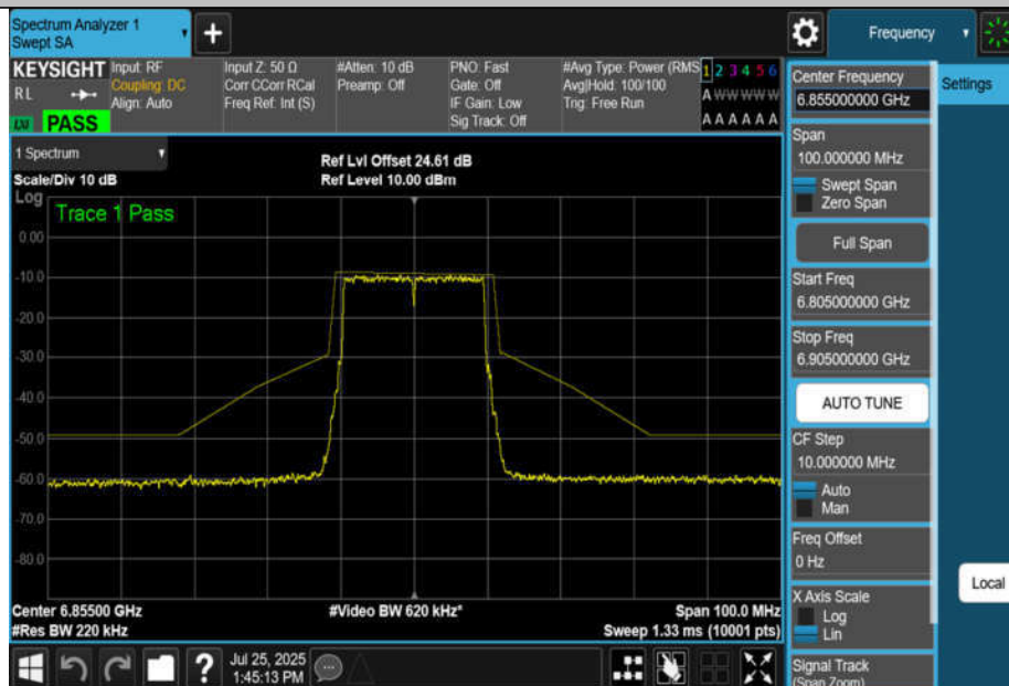
NTNV-11BE20MIMO-Ant4-6855-PASS
