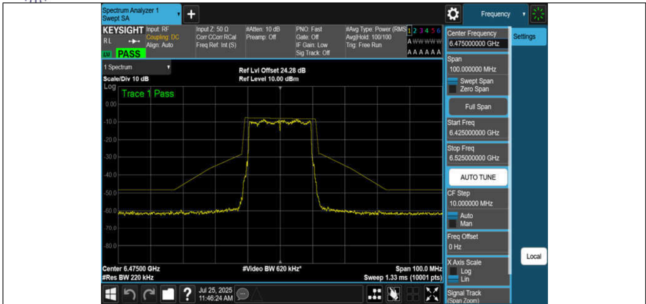
NTNV-11BE20MIMO-Ant3-6475-PASS
