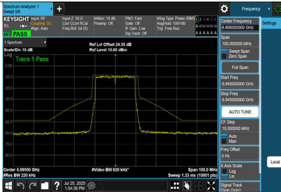
NTNV-11BE20MIMO-Ant3-6895-PASS
