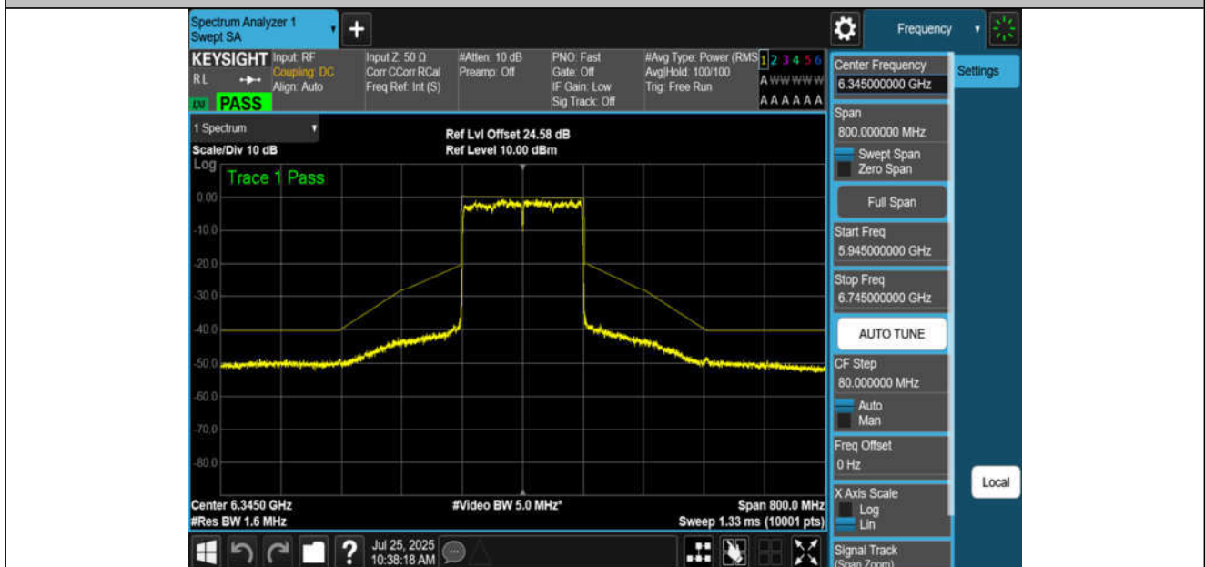
NTNV-11AX160MIMO-Ant4-6345-PASS
