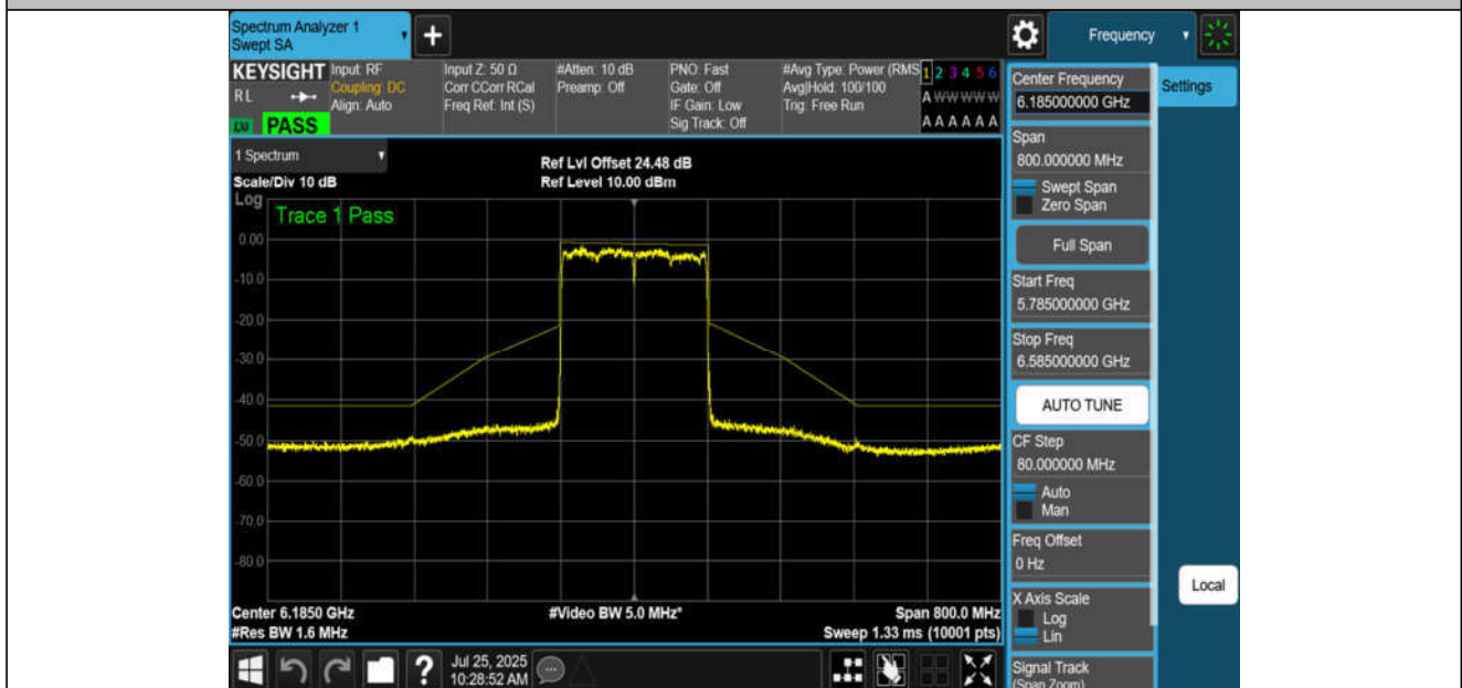
NTNV-11AX160MIMO-Ant2-6185-PASS
