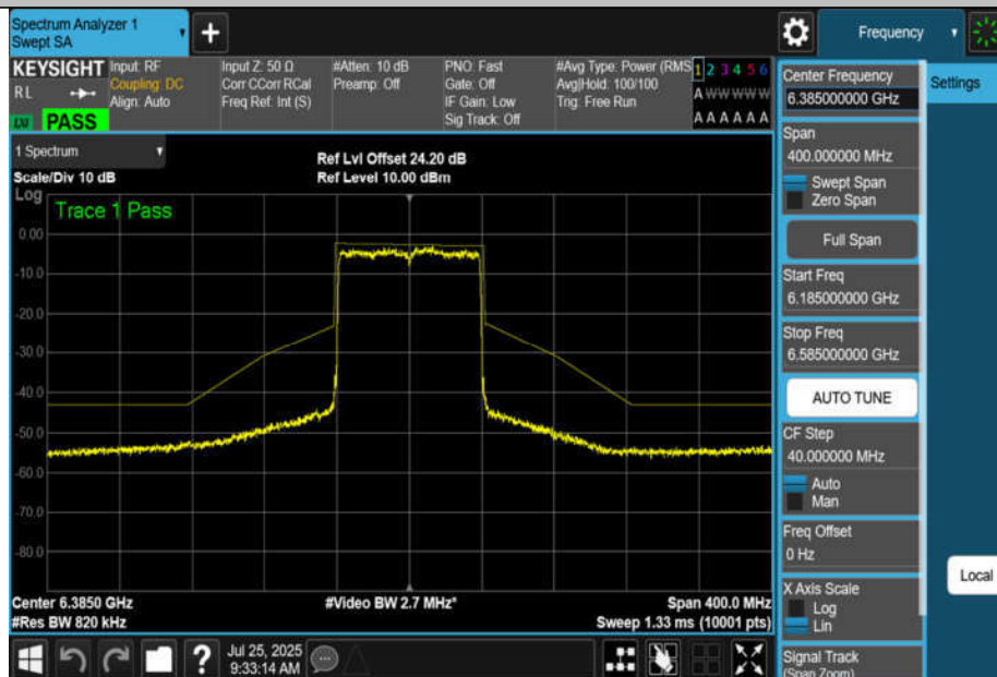
NTNV-11AX80MIMO-Ant4-6385-PASS
