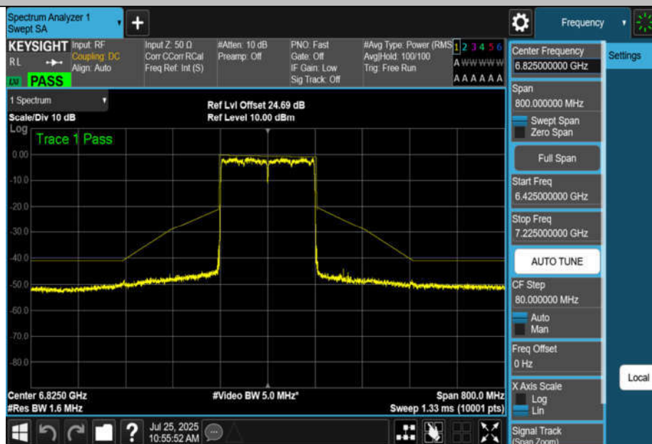
NTNV-11AX160MIMO-Ant4-6825-PASS
