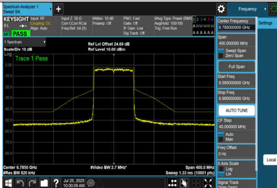
NTNV-11AX80MIMO-Ant4-6785-PASS
