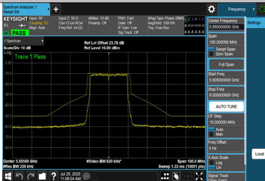
NTNV-11BE20MIMO-Ant2-5955-PASS
