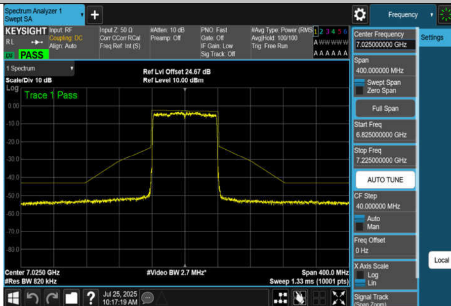
NTNV-11AX80MIMO-Ant4-7025-PASS
