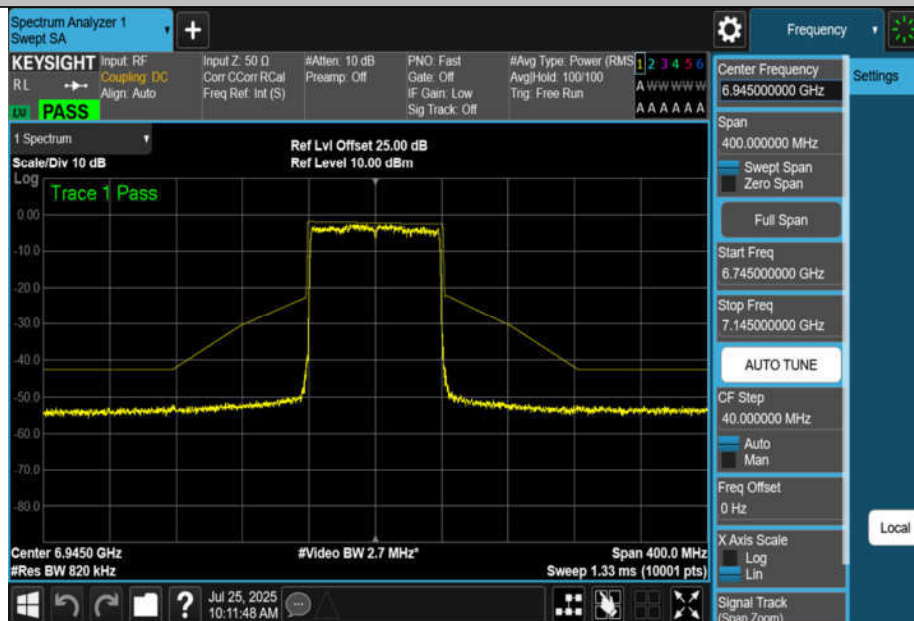
NTNV-11AX80MIMO-Ant4-6945-PASS
