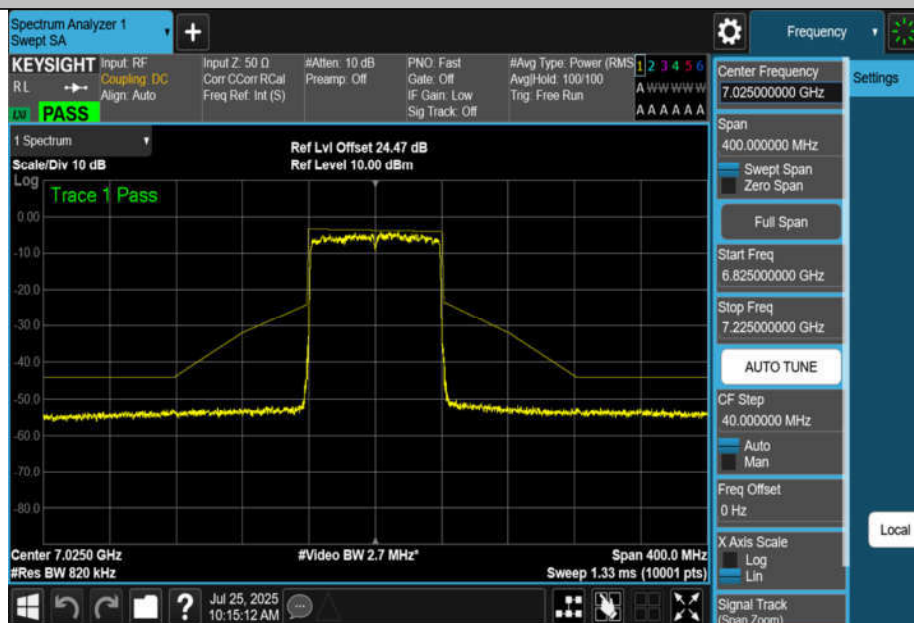
NTNV-11AX80MIMO-Ant2-7025-PASS
