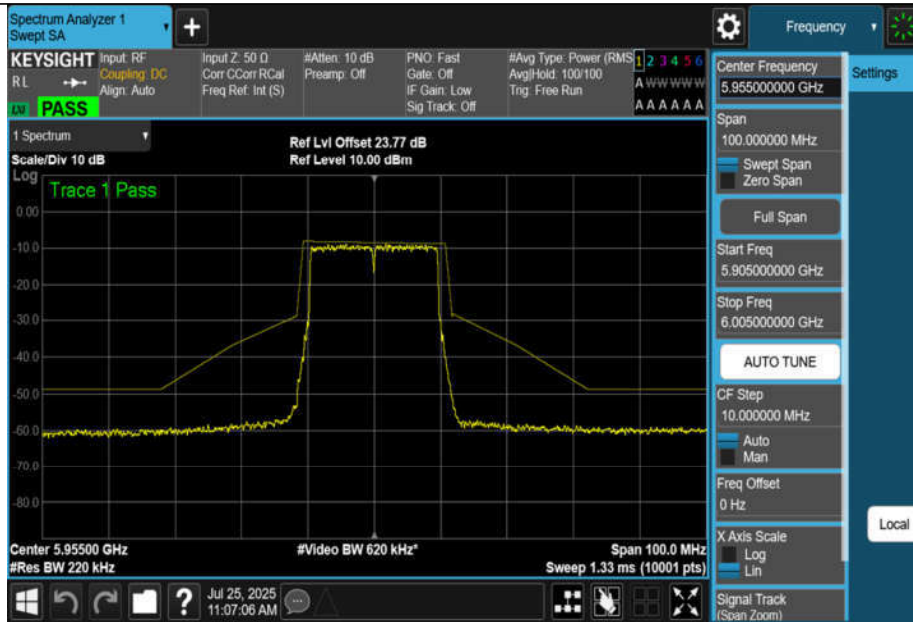
NTNV-11BE20MIMO-Ant3-5955-PASS
