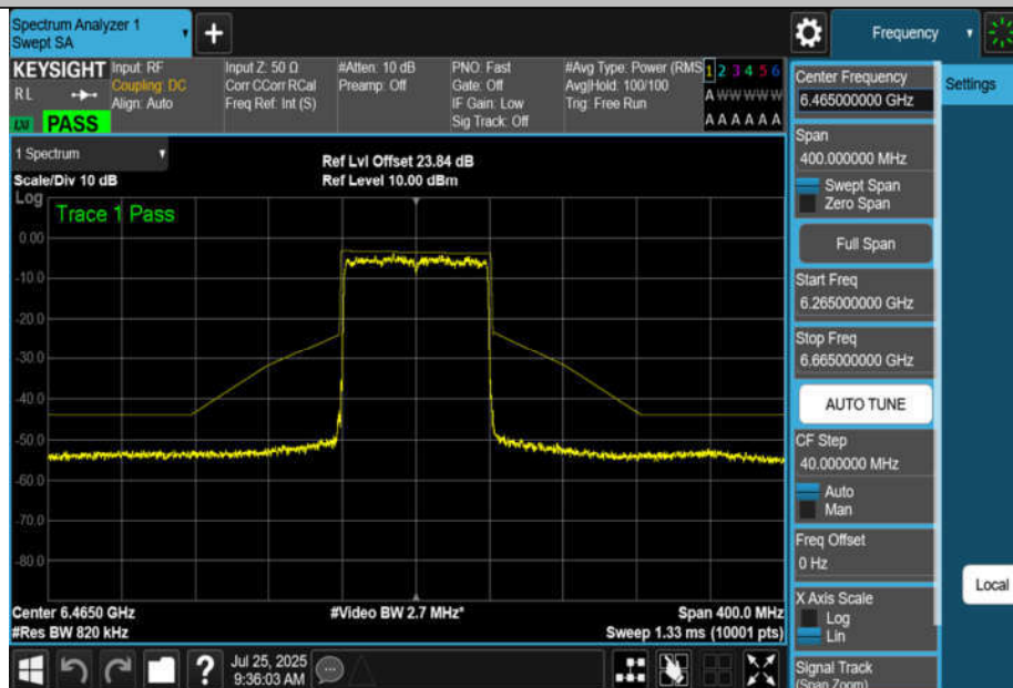
NTNV-11AX80MIMO-Ant2-6465-PASS
