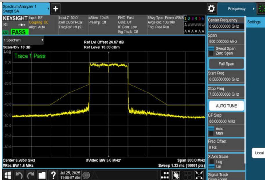
NTNV-11AX160MIMO-Ant4-6985-PASS
