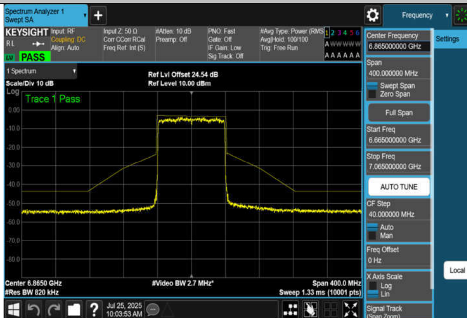
NTNV-11AX80MIMO-Ant2-6865-PASS
