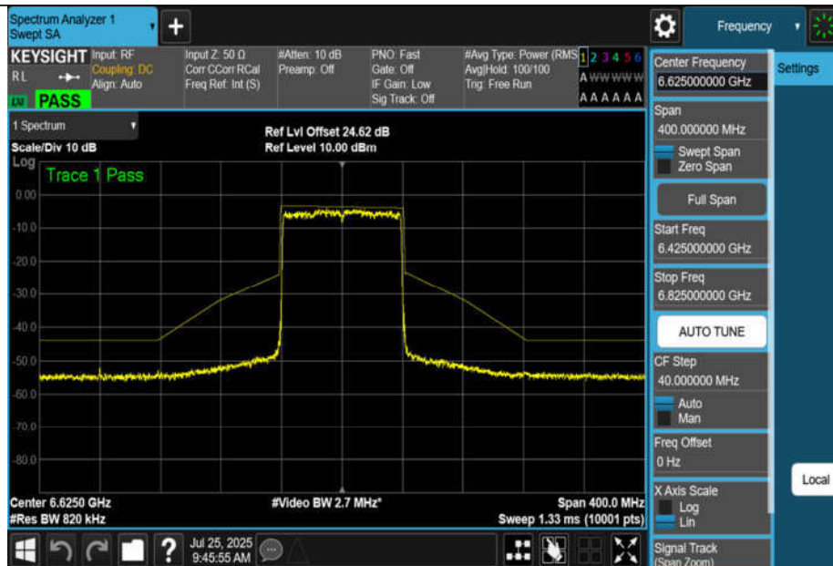
NTNV-11AX80MIMO-Ant1-6625-PASS
