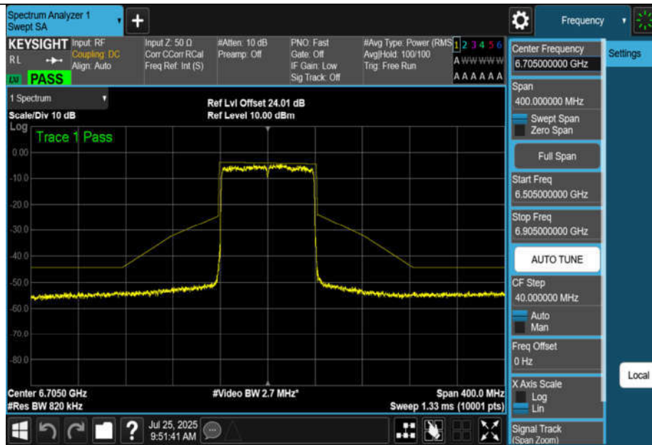
NTNV-11AX80MIMO-Ant1-6705-PASS
