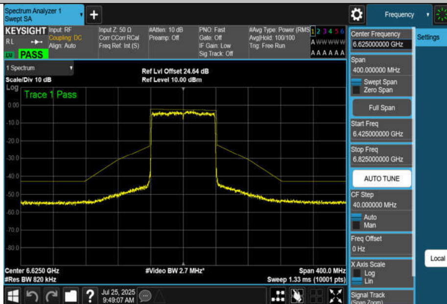
NTNV-11AX80MIMO-Ant4-6625-PASS
