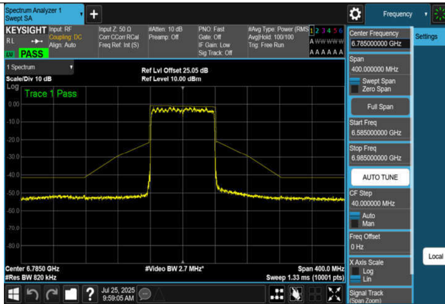
NTNV-11AX80MIMO-Ant3-6785-PASS
