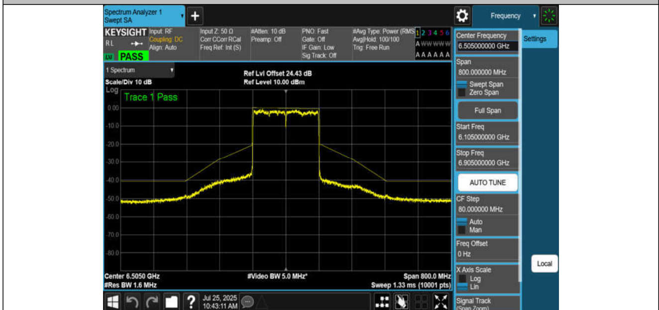
NTNV-11AX160MIMO-Ant4-6505-PASS
