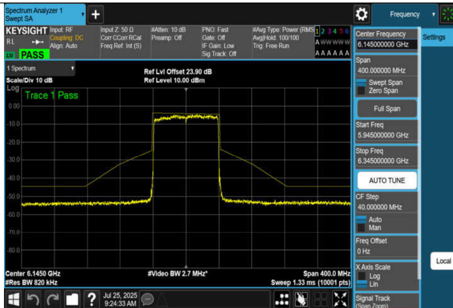
NTNV-11AX80MIMO-Ant1-6145-PASS
