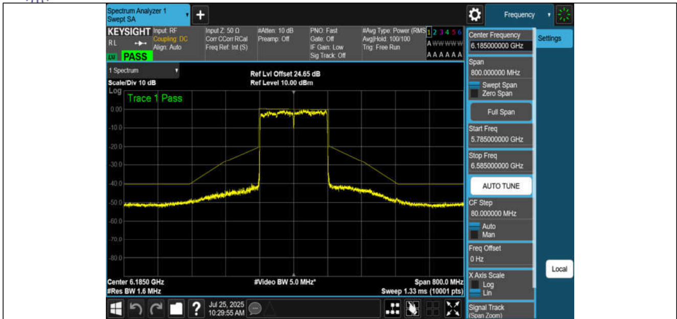
NTNV-11AX160MIMO-Ant3-6185-PASS
