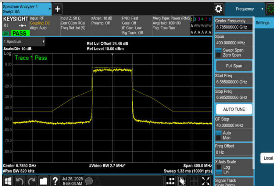
NTNV-11AX80MIMO-Ant2-6785-PASS
