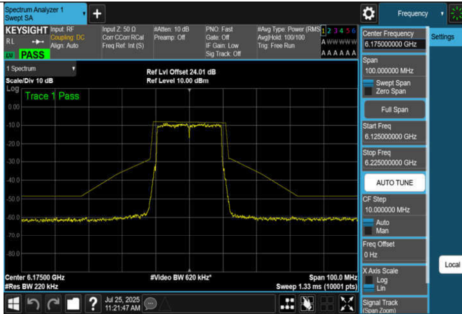
NTNV-11BE20MIMO-Ant3-6175-PASS
