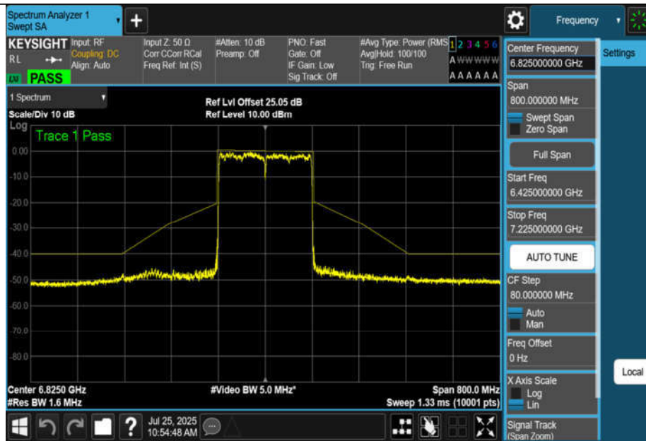
NTNV-11AX160MIMO-Ant3-6825-PASS
