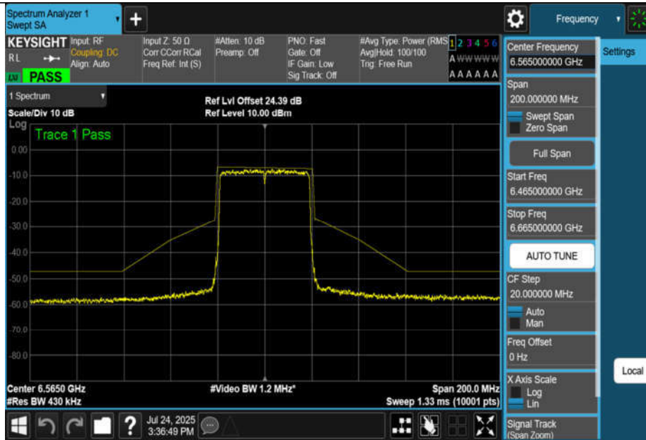
NTNV-11AX40MIMO-Ant1-6565-PASS
