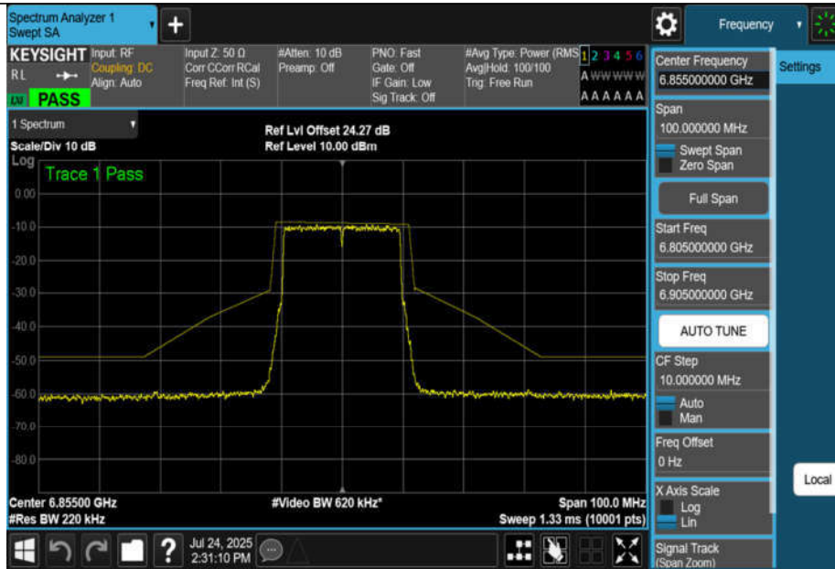
NTNV-11AX20MIMO-Ant1-6855-PASS
