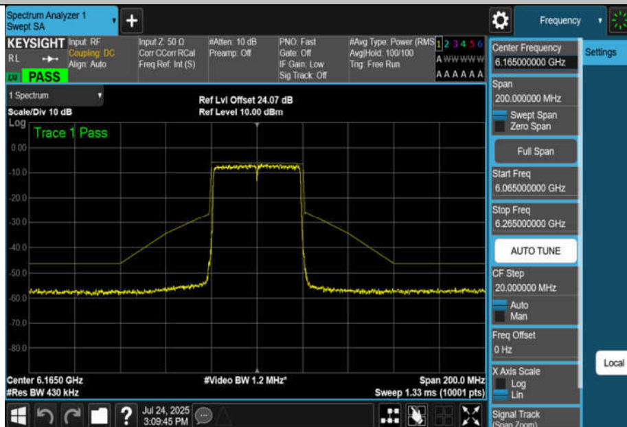
NTNV-11AX40MIMO-Ant4-6165-PASS
