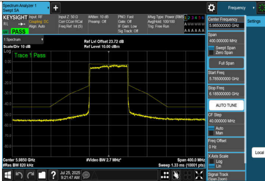
NTNV-11AX80MIMO-Ant3-5985-PASS
