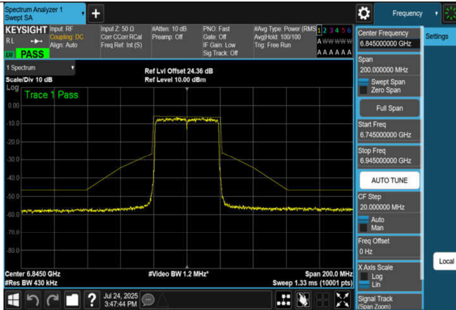
NTNV-11AX40MIMO-Ant1-6845-PASS
