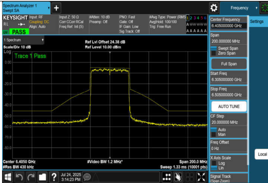
NTNV-11AX40MIMO-Ant3-6405-PASS
