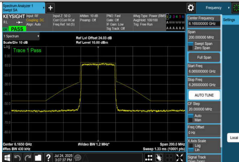
NTNV-11AX40MIMO-Ant2-6165-PASS
