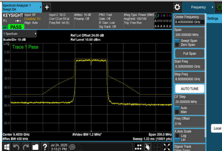
NTNV-11AX40MIMO-Ant2-6405-PASS
