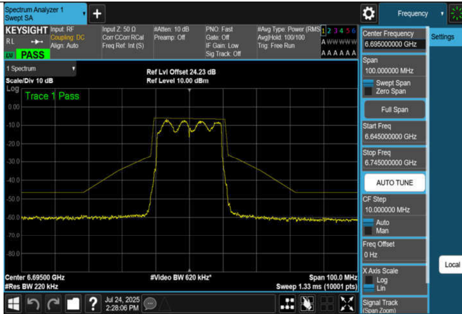
NTNV-11AX20MIMO-Ant3-6695-PASS
