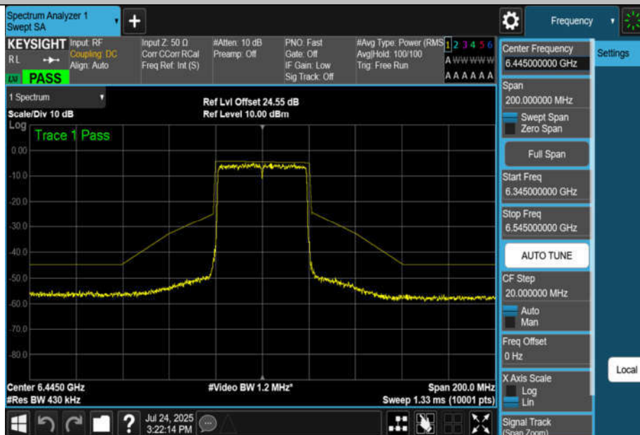
NTNV-11AX40MIMO-Ant4-6445-PASS
