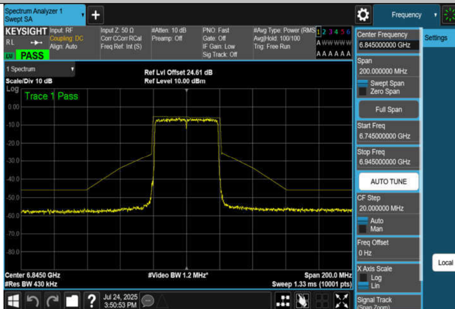
NTNV-11AX40MIMO-Ant4-6845-PASS
