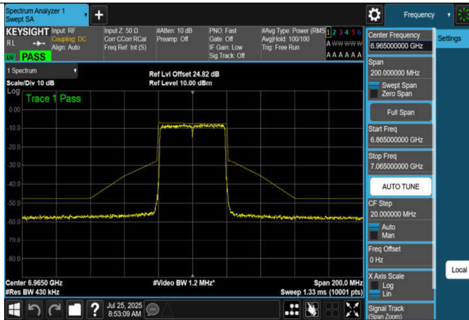
NTNV-11AX40MIMO-Ant1-6965-PASS
