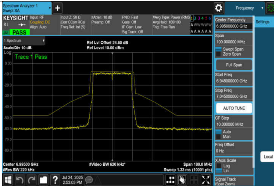
NTNV-11AX20MIMO-Ant3-6995-PASS
