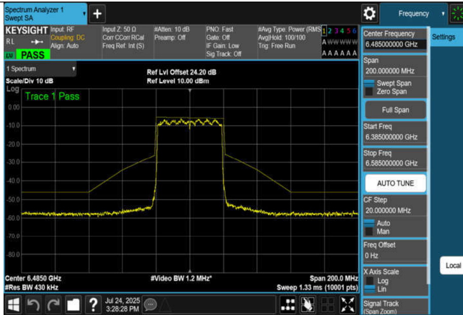
NTNV-11AX40MIMO-Ant3-6485-PASS
