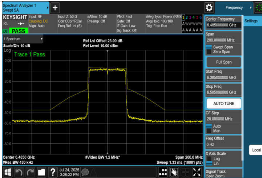
NTNV-11AX40MIMO-Ant1-6485-PASS
