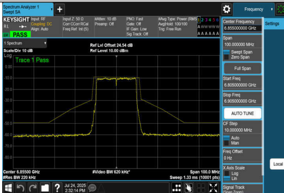
NTNV-11AX20MIMO-Ant2-6855-PASS
