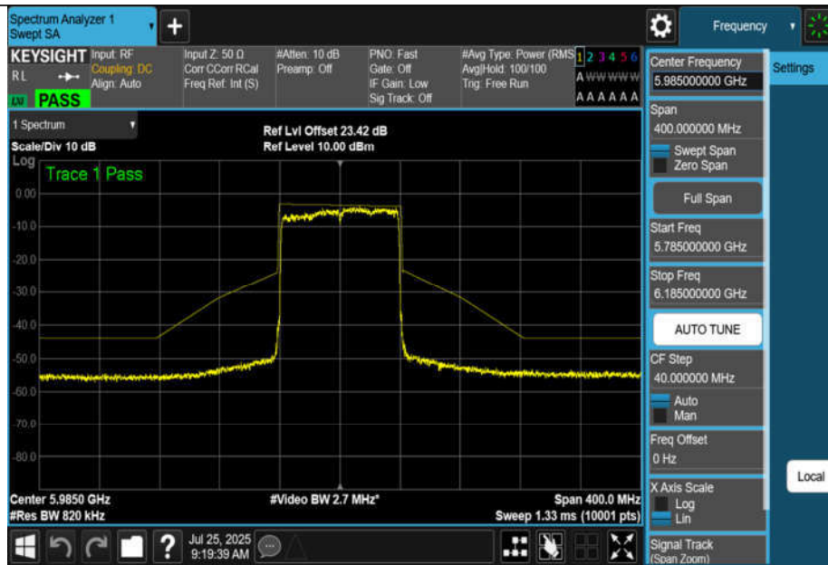
NTNV-11AX80MIMO-Ant1-5985-PASS
