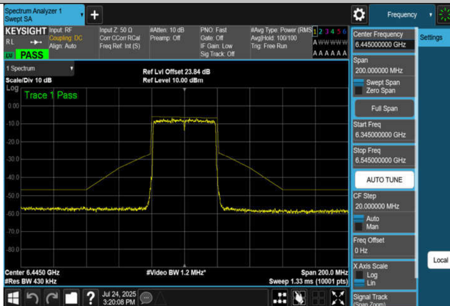
NTNV-11AX40MIMO-Ant2-6445-PASS
