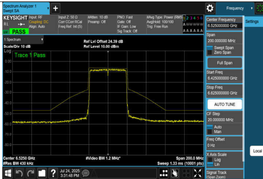
NTNV-11AX40MIMO-Ant1-6525-PASS
