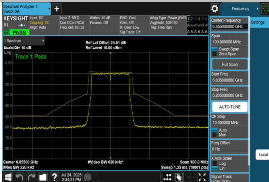
NTNV-11AX20MIMO-Ant4-6855-PASS
