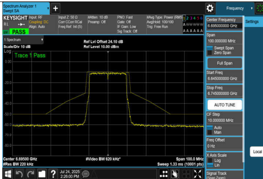
NTNV-11AX20MIMO-Ant1-6695-PASS
