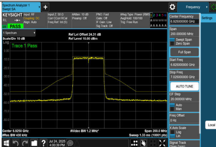
NTNV-11AX40MIMO-Ant2-6925-PASS
