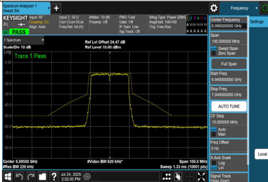
NTNV-11AX20MIMO-Ant2-6995-PASS
