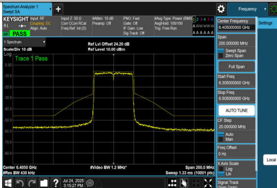
NTNV-11AX40MIMO-Ant4-6405-PASS
