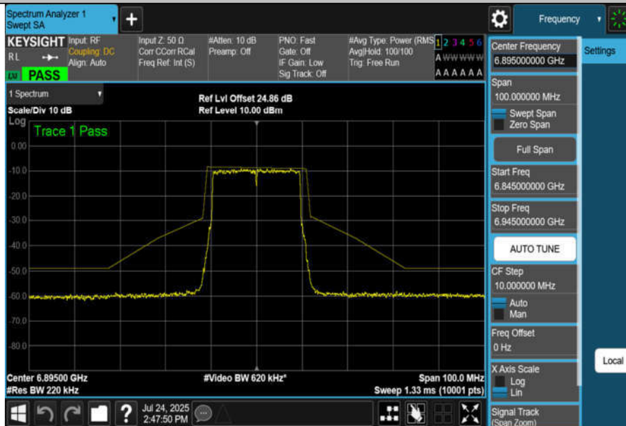
NTNV-11AX20MIMO-Ant4-6895-PASS
