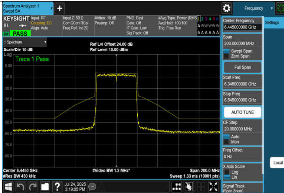
NTNV-11AX40MIMO-Ant1-6445-PASS
