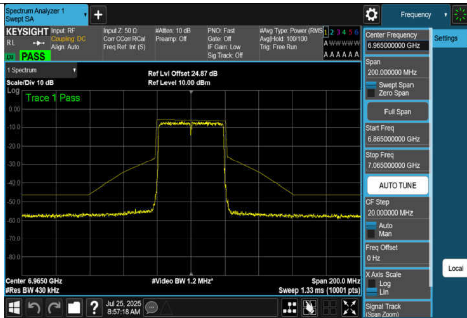
NTNV-11AX40MIMO-Ant3-6965-PASS
