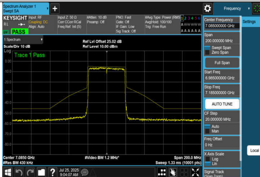
NTNV-11AX40MIMO-Ant4-7085-PASS
