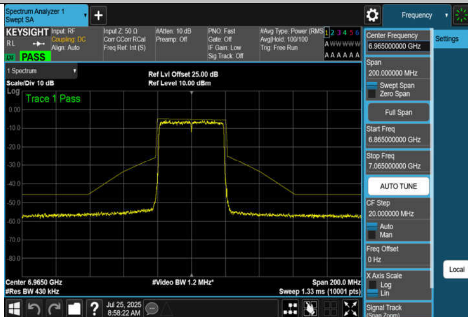
NTNV-11AX40MIMO-Ant4-6965-PASS
