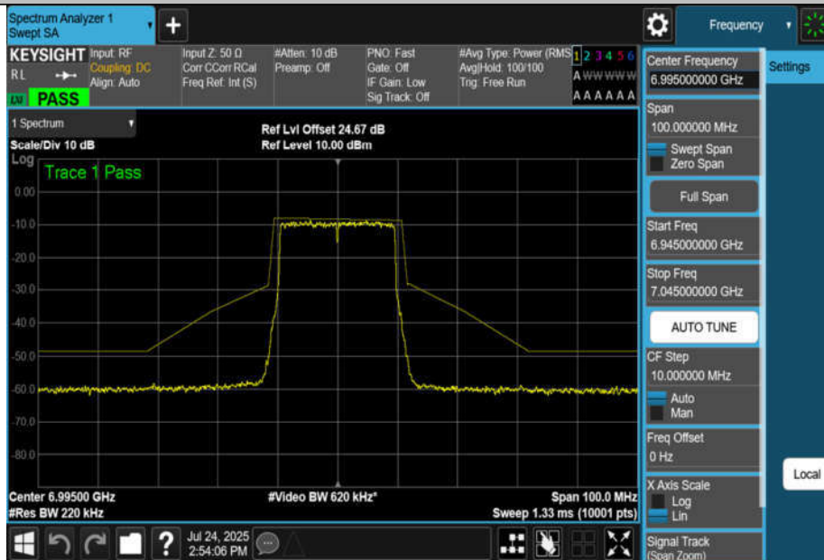
NTNV-11AX20MIMO-Ant4-6995-PASS
