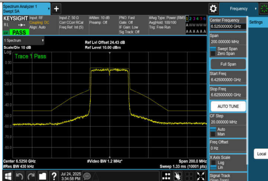
NTNV-11AX40MIMO-Ant4-6525-PASS
