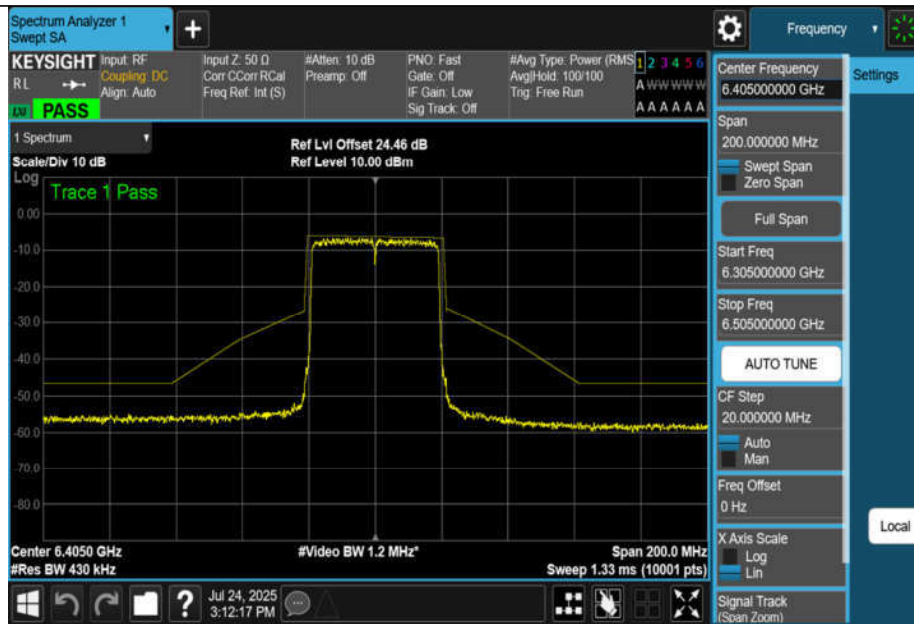
NTNV-11AX40MIMO-Ant1-6405-PASS
