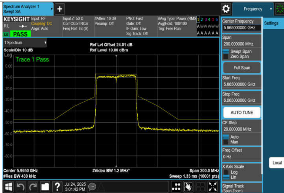
NTNV-11AX40MIMO-Ant1-5965-PASS
