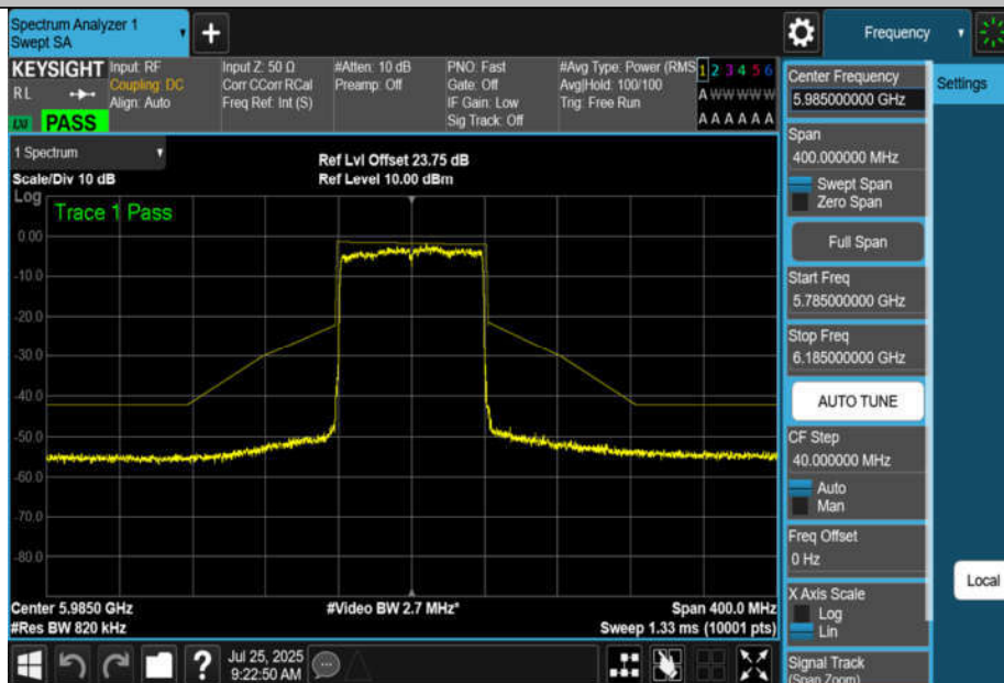
NTNV-11AX80MIMO-Ant4-5985-PASS
