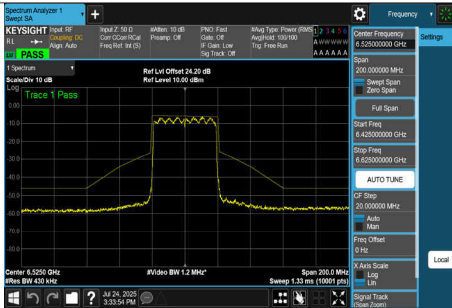
NTNV-11AX40MIMO-Ant3-6525-PASS
