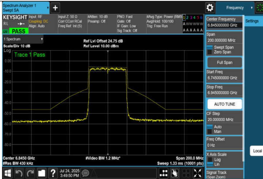
NTNV-11AX40MIMO-Ant3-6845-PASS
