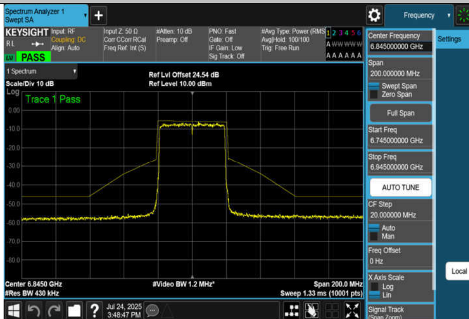
NTNV-11AX40MIMO-Ant2-6845-PASS
