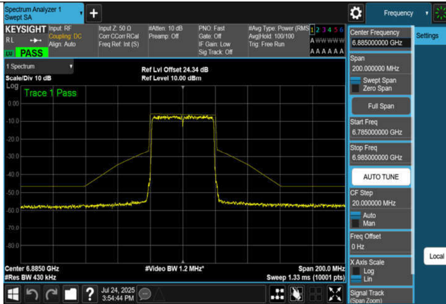
NTNV-11AX40MIMO-Ant1-6885-PASS
