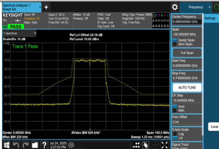
NTNV-11AX20MIMO-Ant2-6695-PASS
