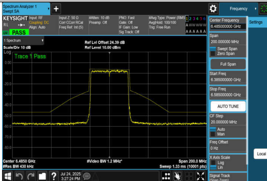
NTNV-11AX40MIMO-Ant2-6485-PASS
