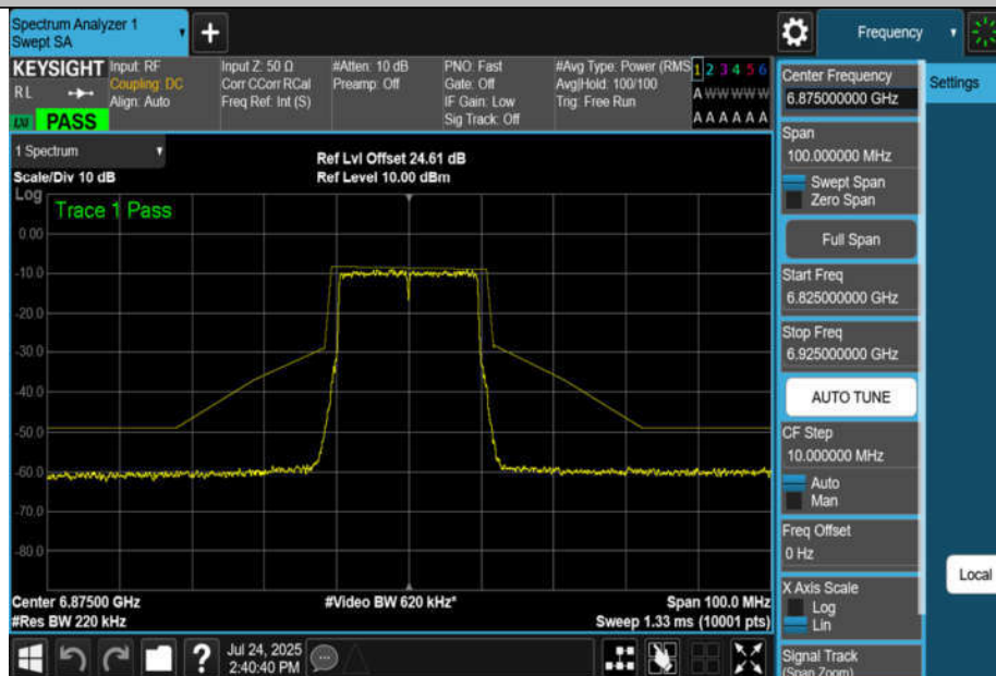
NTNV-11AX20MIMO-Ant4-6875-PASS
