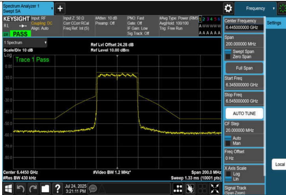
NTNV-11AX40MIMO-Ant3-6445-PASS
