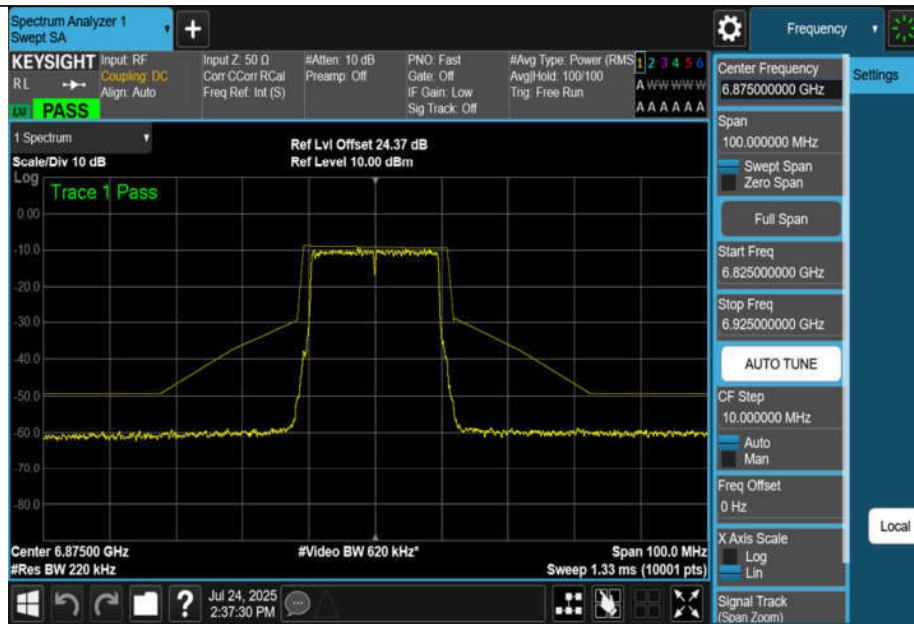
NTNV-11AX20MIMO-Ant1-6875-PASS
