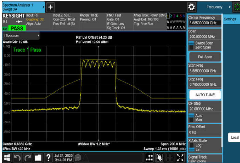
NTNV-11AX40MIMO-Ant3-6685-PASS
