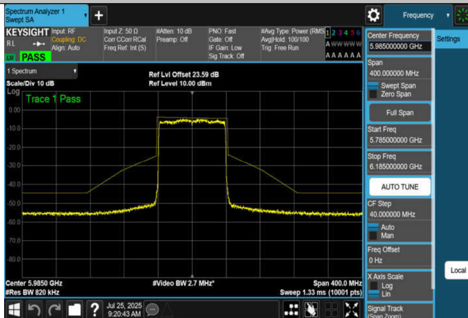
NTNV-11AX80MIMO-Ant2-5985-PASS
