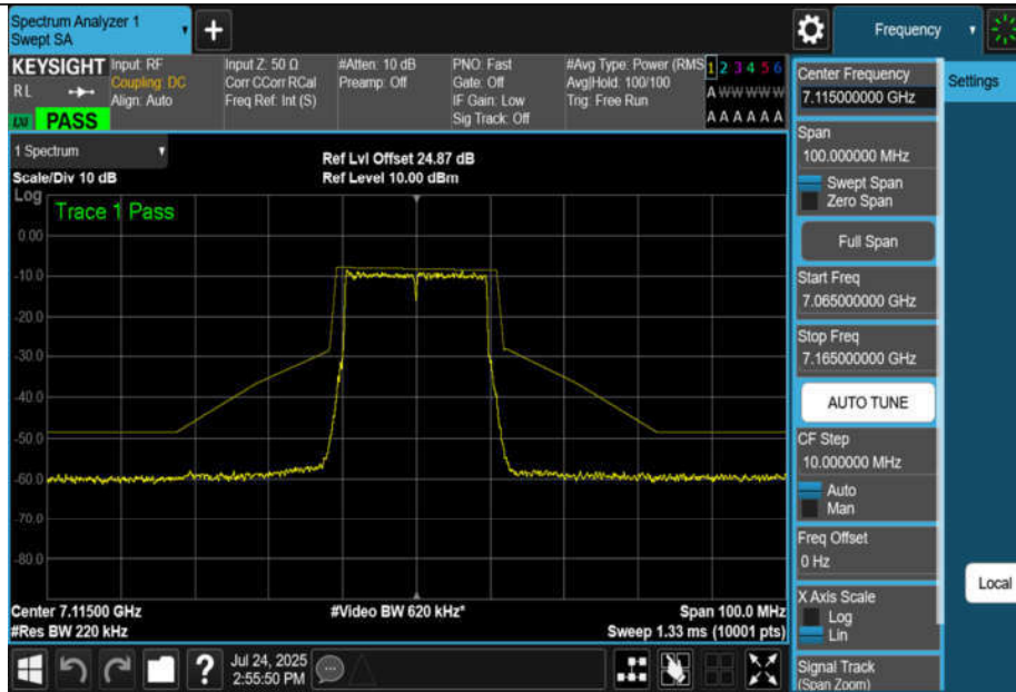
NTNV-11AX20MIMO-Ant1-7115-PASS
