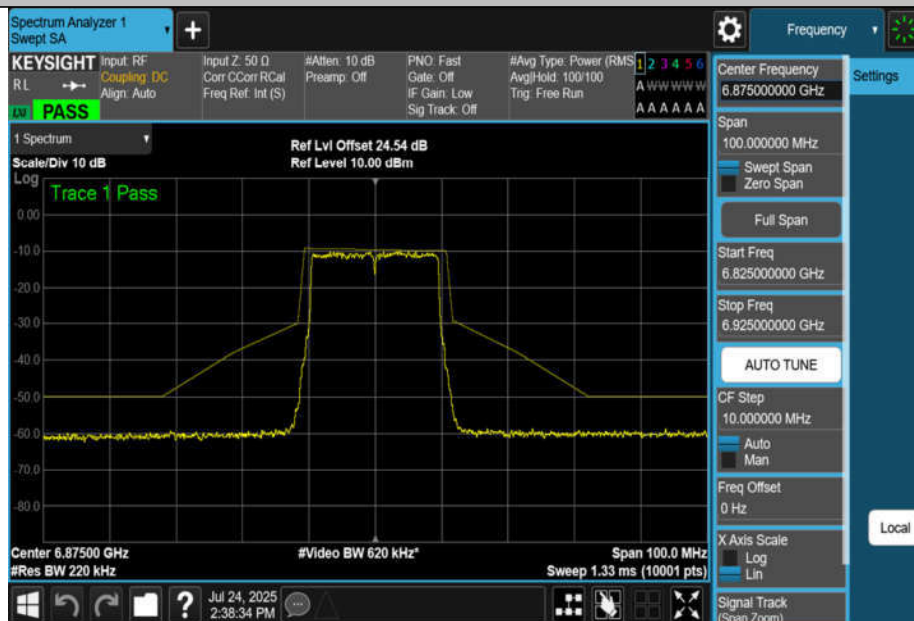
NTNV-11AX20MIMO-Ant2-6875-PASS
