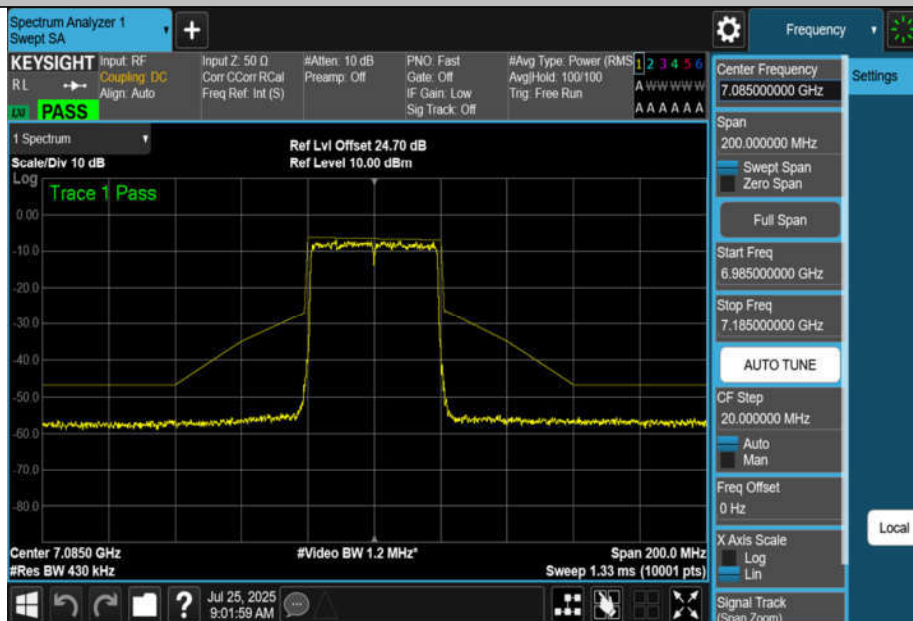
NTNV-11AX40MIMO-Ant2-7085-PASS
