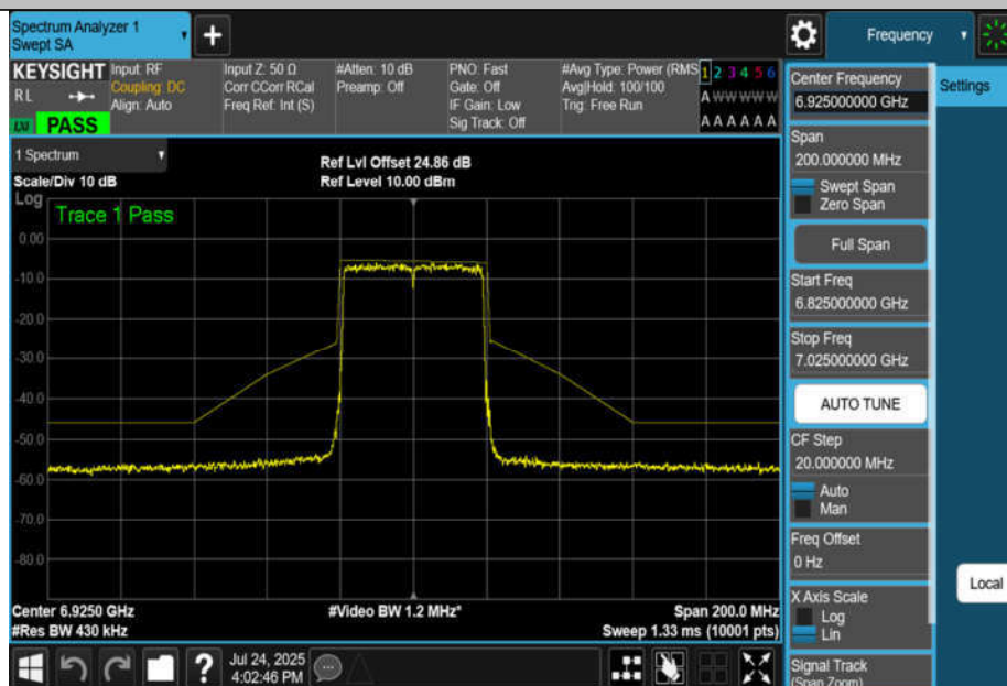
NTNV-11AX40MIMO-Ant4-6925-PASS
