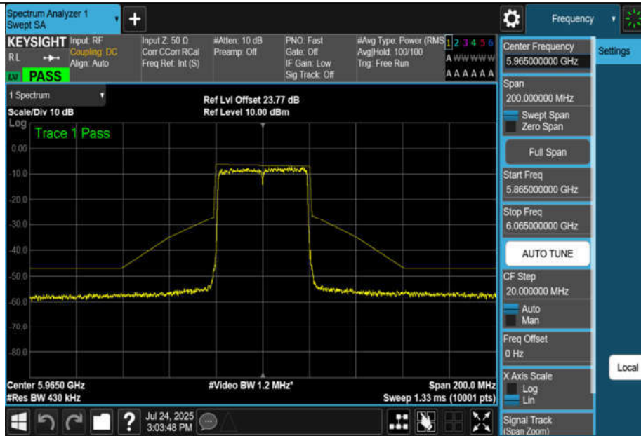
NTNV-11AX40MIMO-Ant3-5965-PASS
