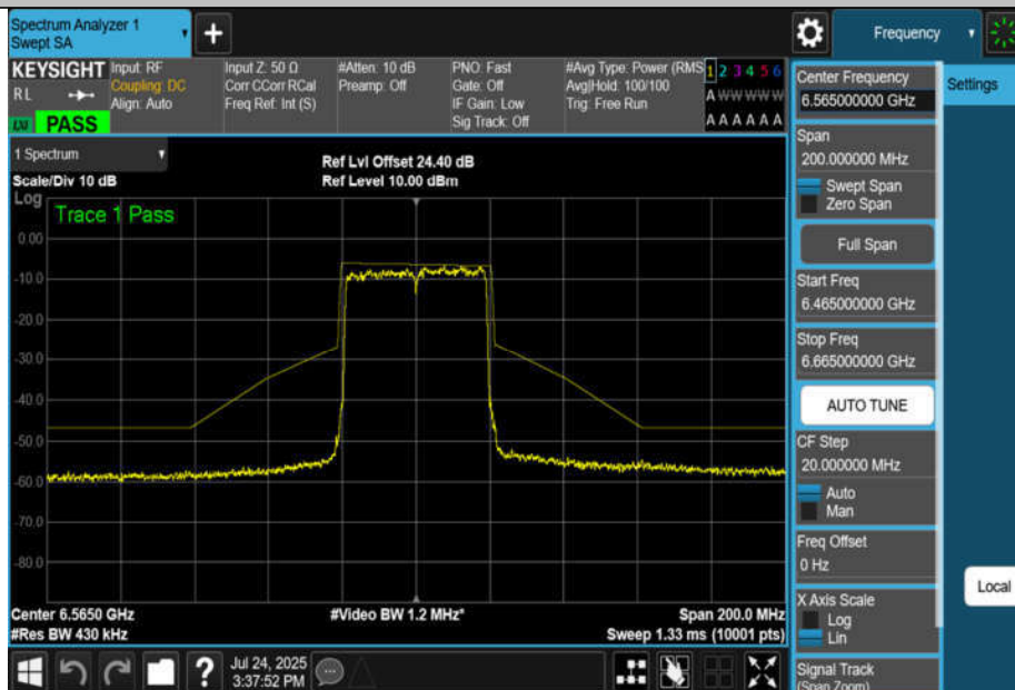
NTNV-11AX40MIMO-Ant2-6565-PASS
