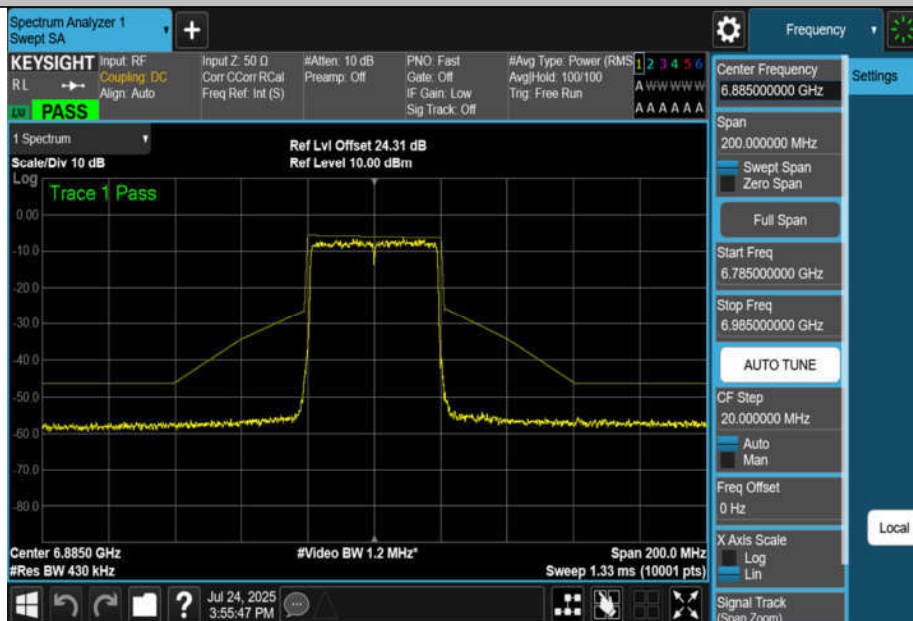
NTNV-11AX40MIMO-Ant2-6885-PASS
