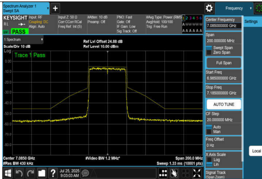
NTNV-11AX40MIMO-Ant3-7085-PASS
