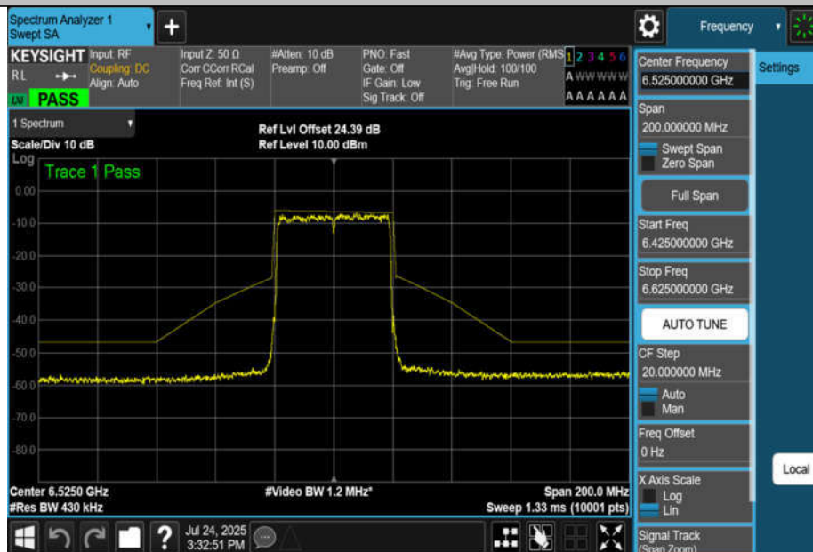
NTNV-11AX40MIMO-Ant2-6525-PASS
