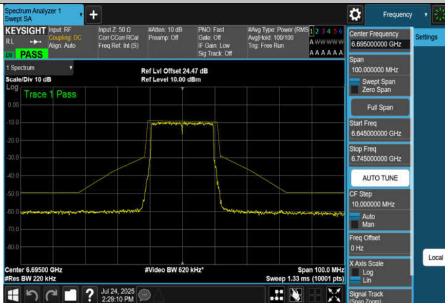
NTNV-11AX20MIMO-Ant4-6695-PASS
