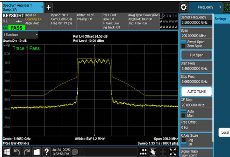
NTNV-11AX40MIMO-Ant3-6565-PASS
