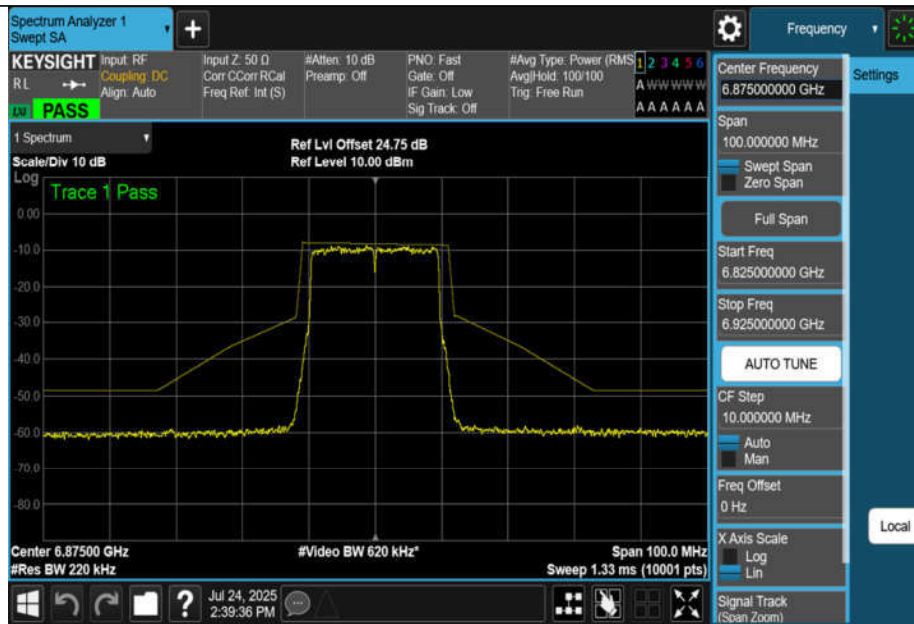
NTNV-11AX20MIMO-Ant3-6875-PASS
