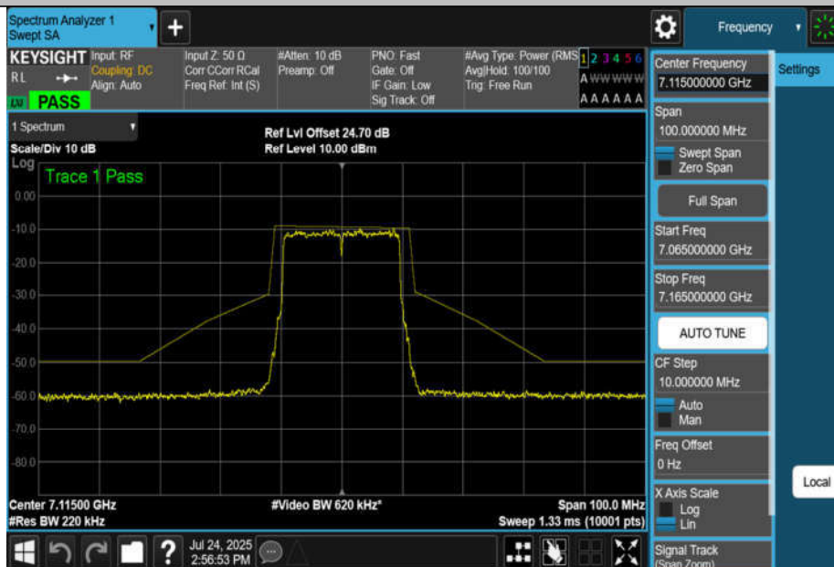
NTNV-11AX20MIMO-Ant2-7115-PASS
