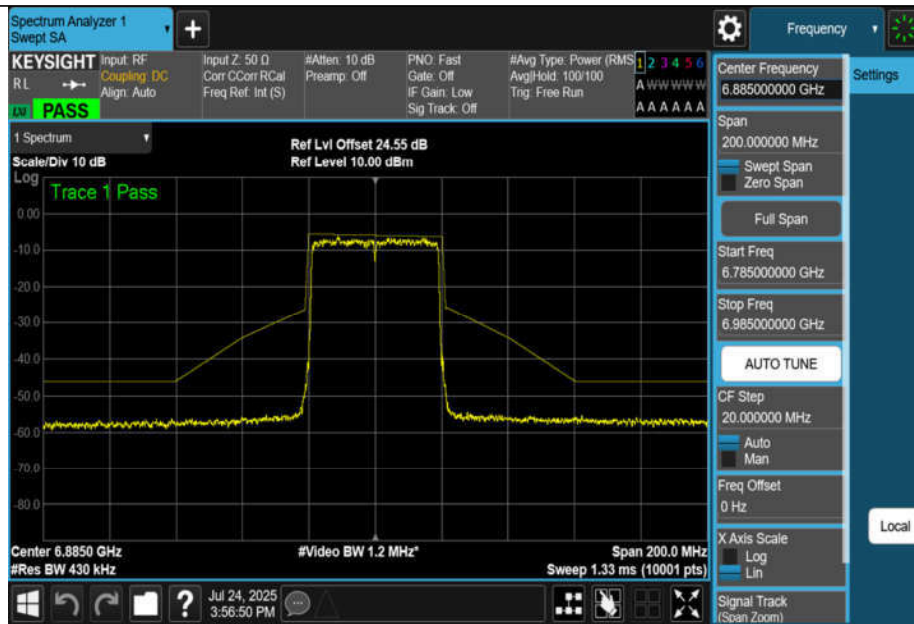
NTNV-11AX40MIMO-Ant3-6885-PASS
