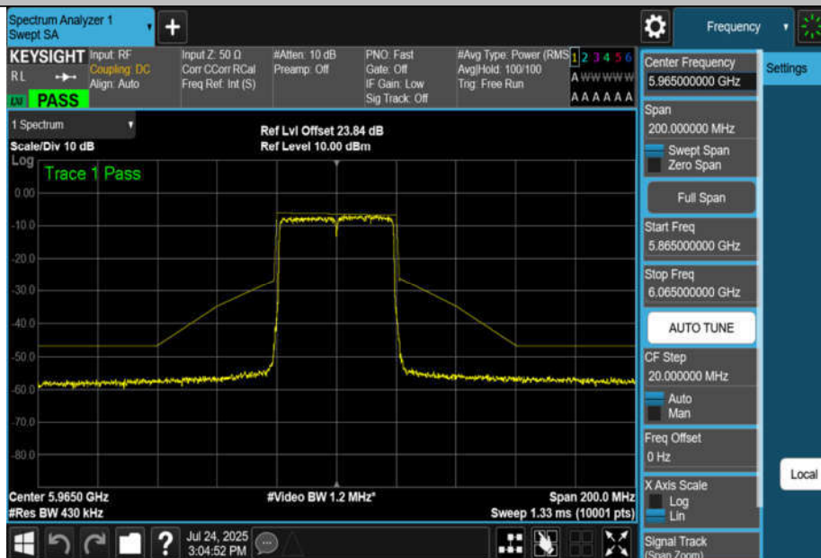
NTNV-11AX40MIMO-Ant4-5965-PASS
