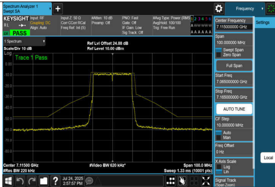
NTNV-11AX20MIMO-Ant3-7115-PASS
