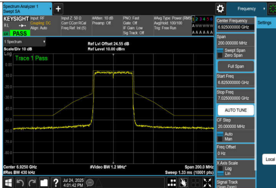
NTNV-11AX40MIMO-Ant3-6925-PASS
