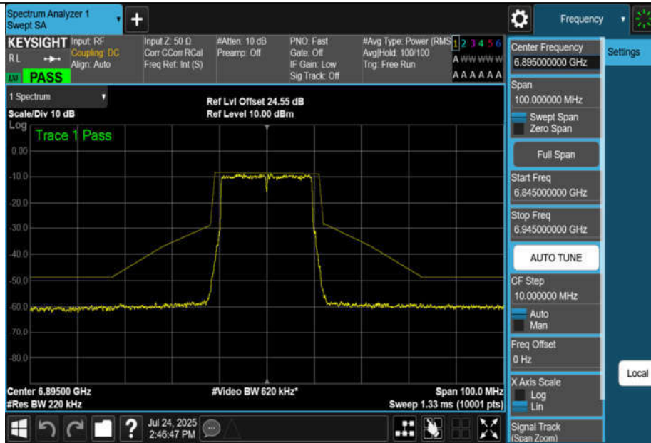
NTNV-11AX20MIMO-Ant3-6895-PASS
