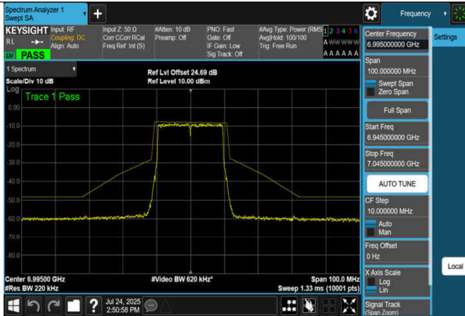
NTNV-11AX20MIMO-Ant1-6995-PASS
