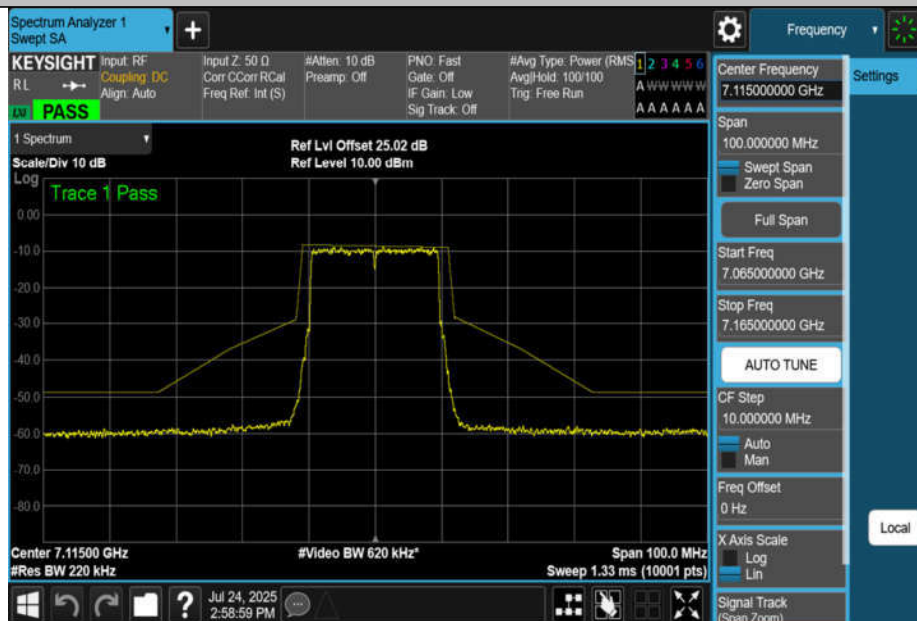
NTNV-11AX20MIMO-Ant4-7115-PASS
