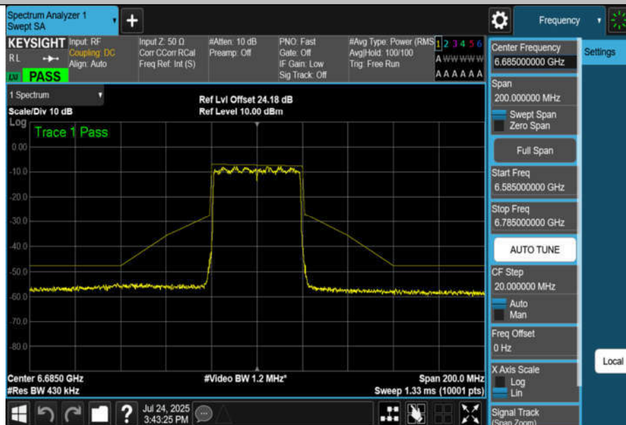
NTNV-11AX40MIMO-Ant2-6685-PASS
