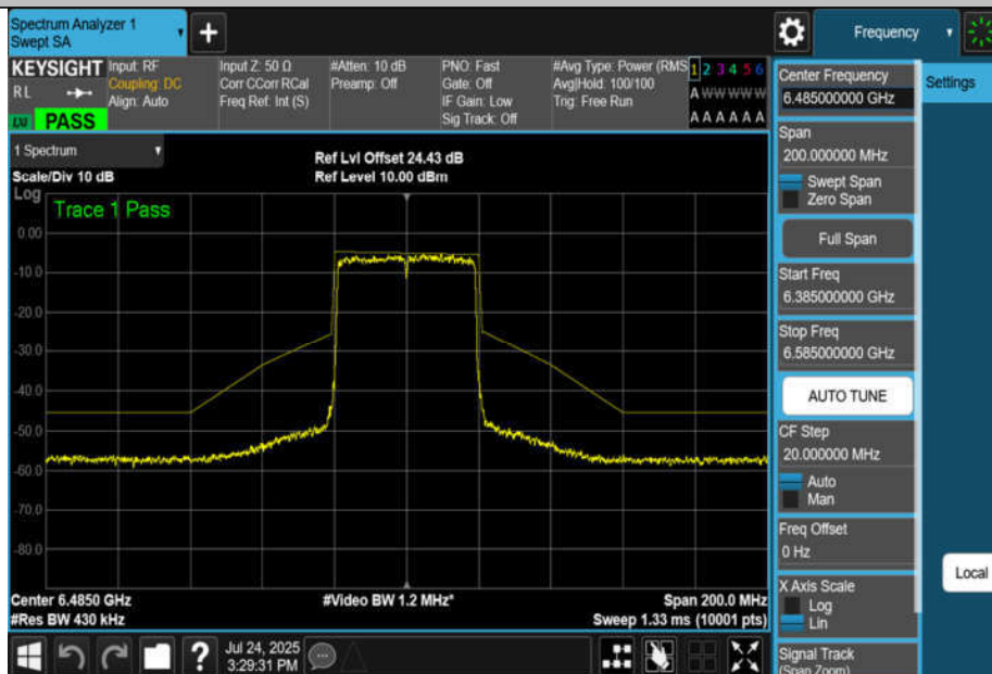
NTNV-11AX40MIMO-Ant4-6485-PASS
