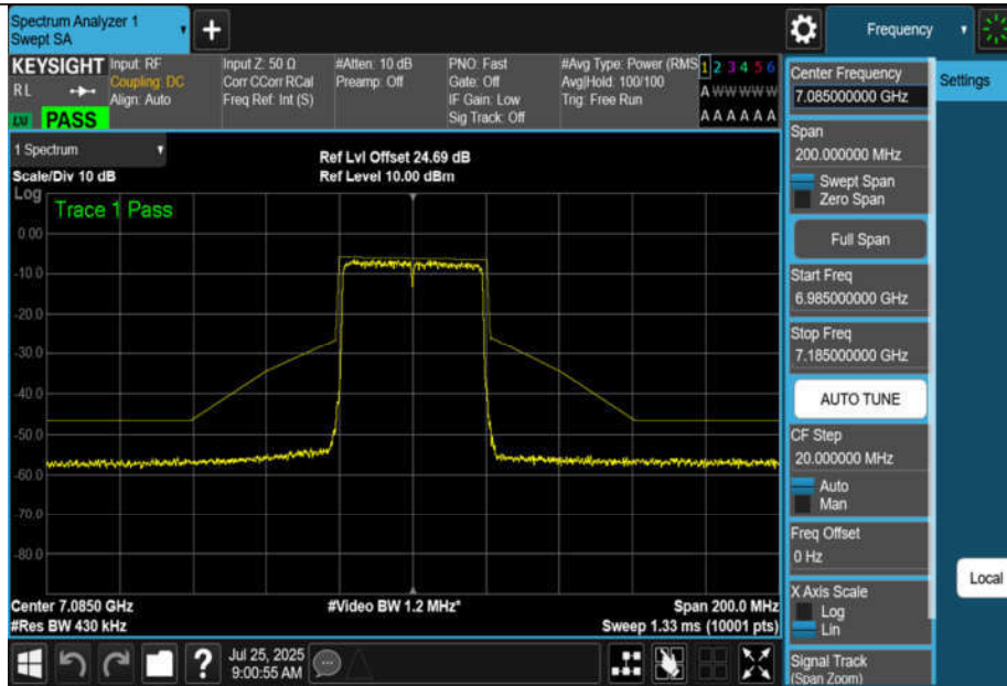
NTNV-11AX40MIMO-Ant1-7085-PASS
