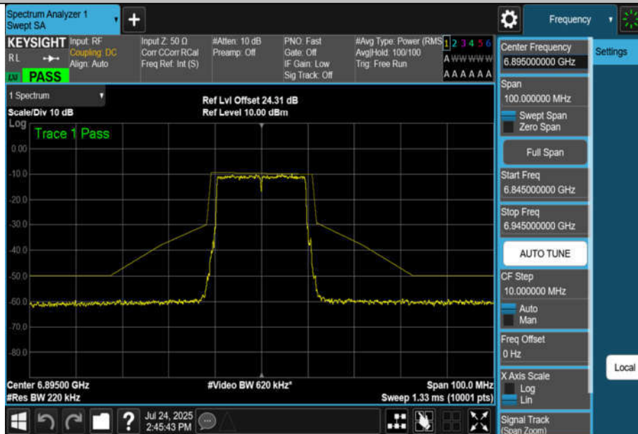
NTNV-11AX20MIMO-Ant2-6895-PASS
