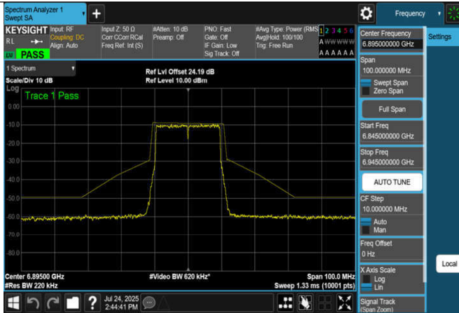
NTNV-11AX20MIMO-Ant1-6895-PASS
