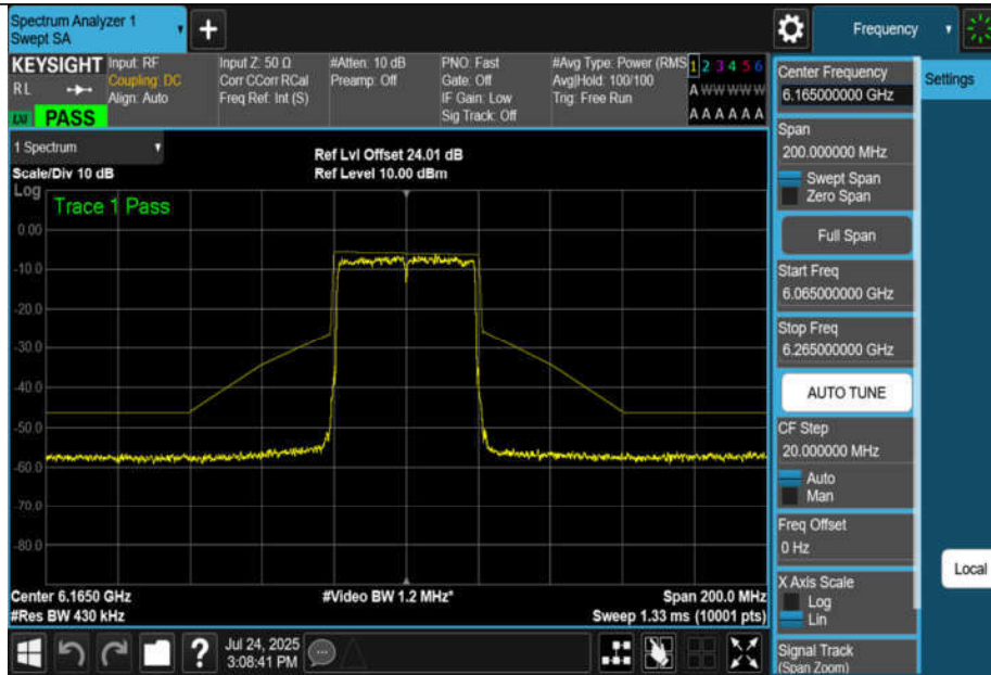
NTNV-11AX40MIMO-Ant3-6165-PASS
