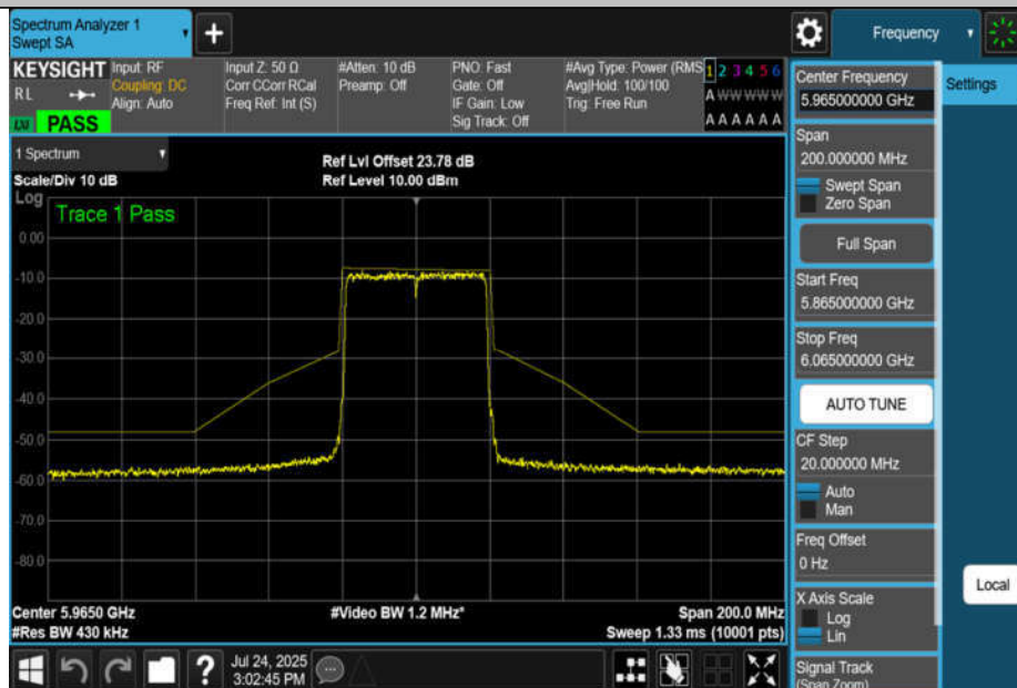
NTNV-11AX40MIMO-Ant2-5965-PASS
