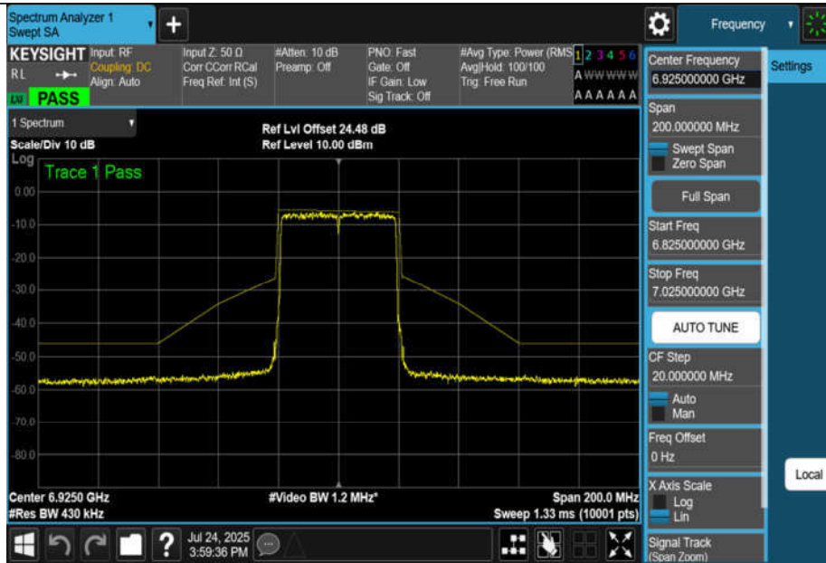
NTNV-11AX40MIMO-Ant1-6925-PASS
