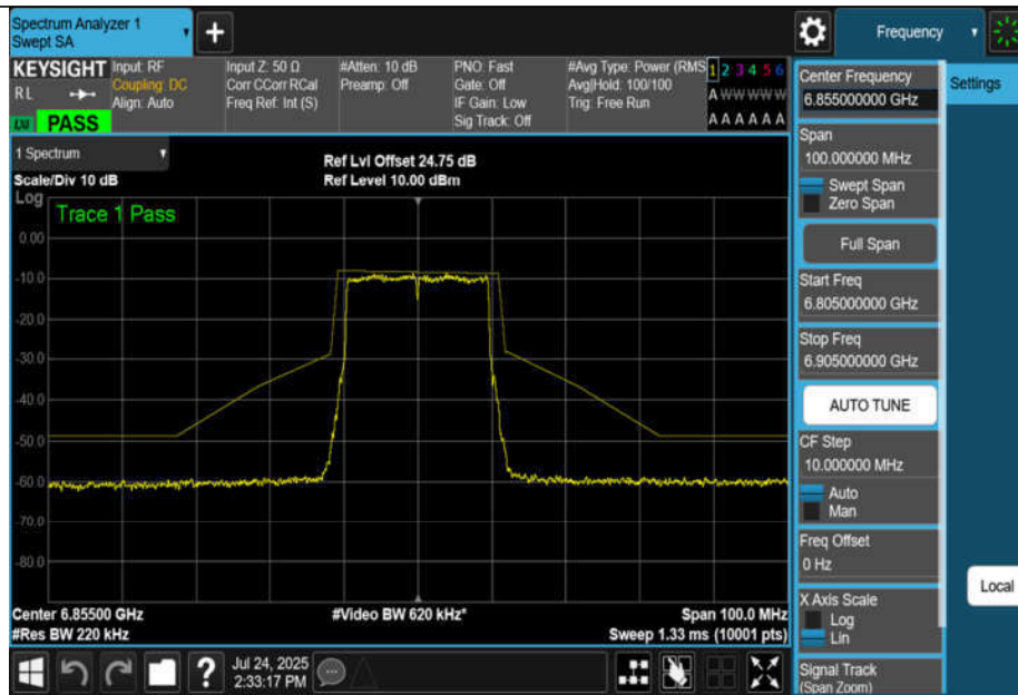
NTNV-11AX20MIMO-Ant3-6855-PASS
