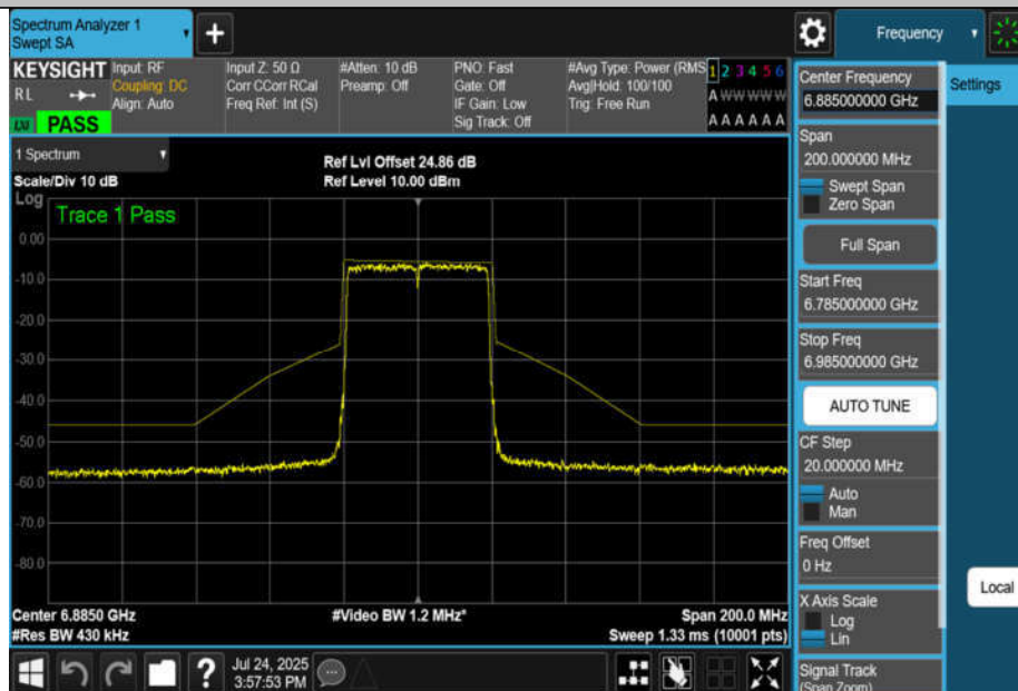
NTNV-11AX40MIMO-Ant4-6885-PASS
