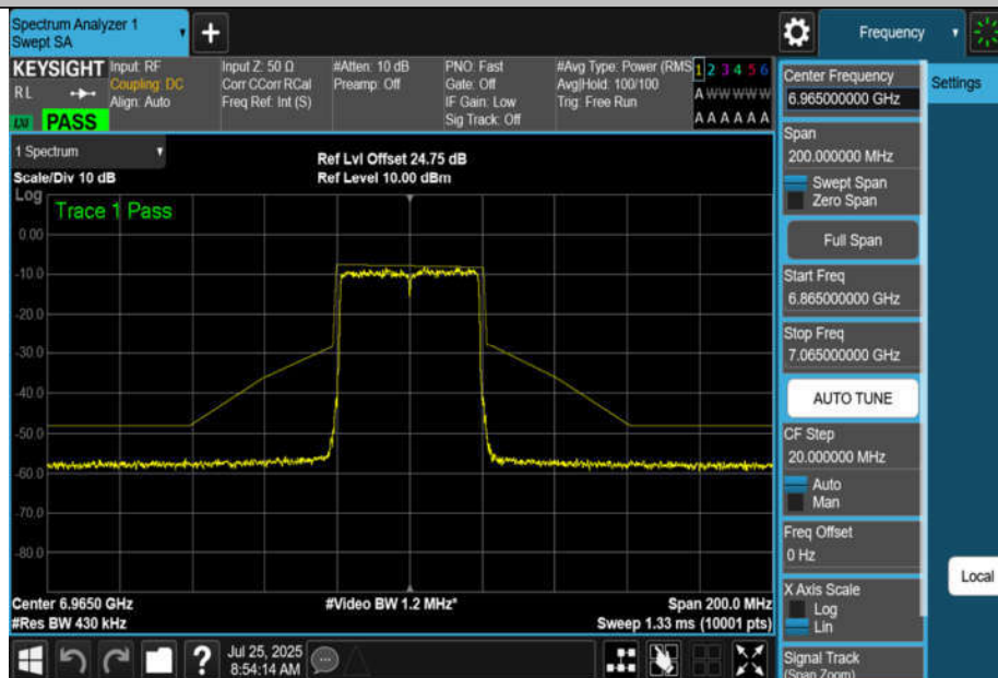
NTNV-11AX40MIMO-Ant2-6965-PASS
