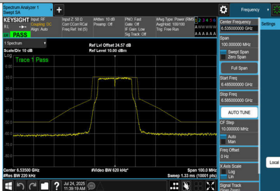
NTNV-11A-CDD-Ant4-6535-PASS
