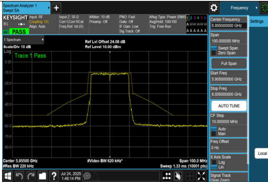
NTNV-11AX20MIMO-Ant1-5955-PASS
