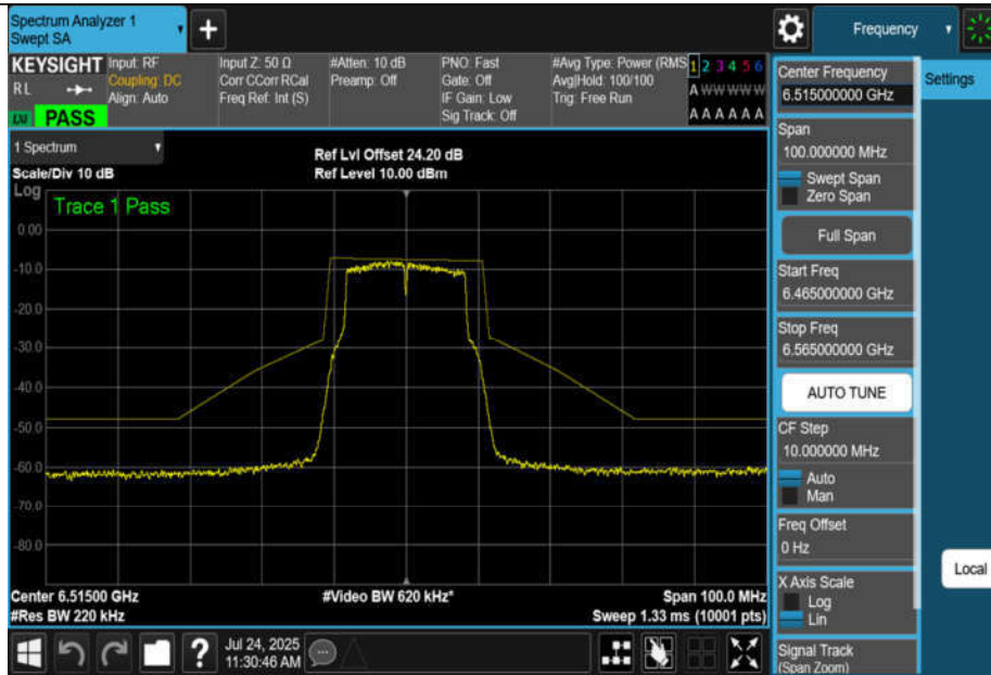
NTNV-11A-CDD-Ant3-6515-PASS
