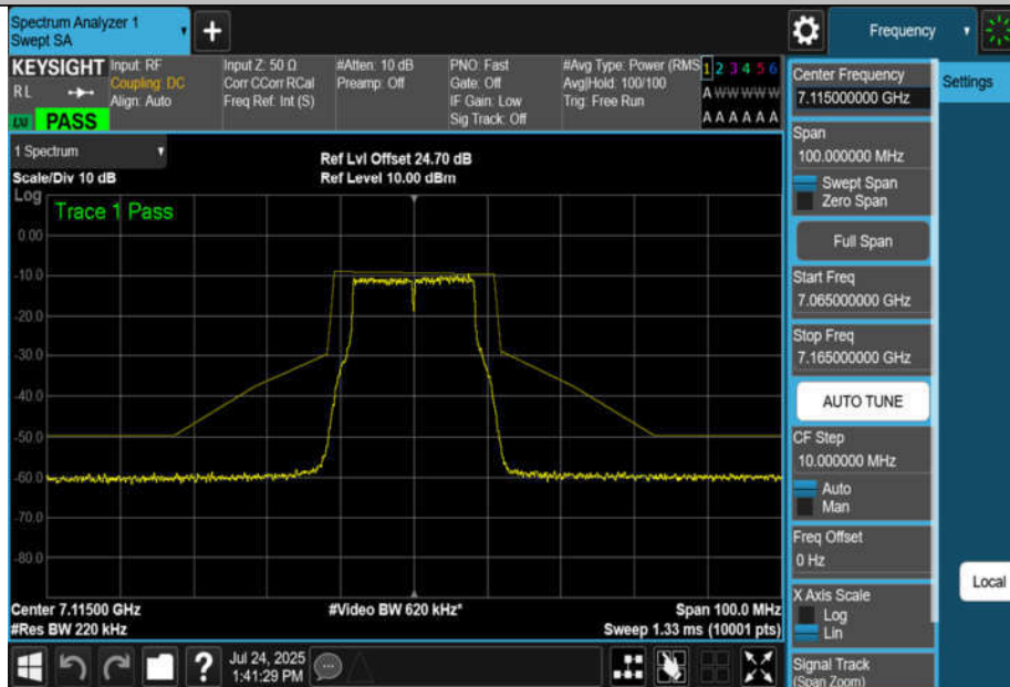
NTNV-11A-CDD-Ant2-7115-PASS
