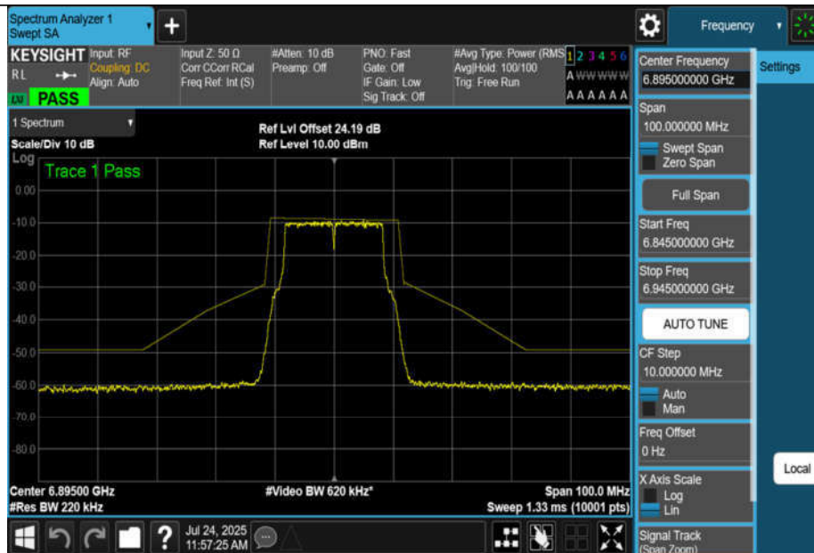
NTNV-11A-CDD-Ant1-6895-PASS
