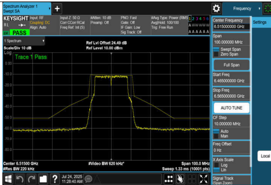
NTNV-11A-CDD-Ant1-6515-PASS
