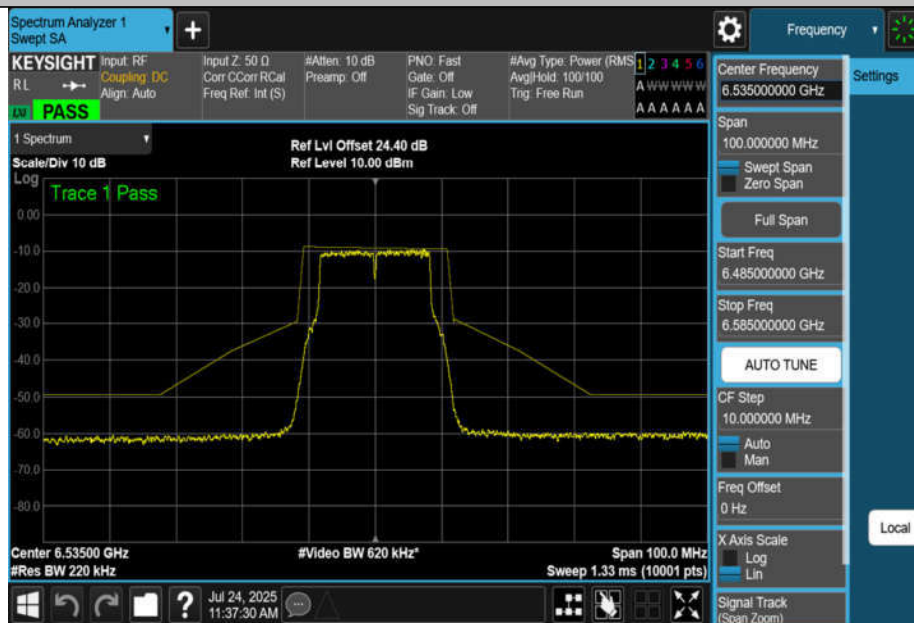
NTNV-11A-CDD-Ant2-6535-PASS
