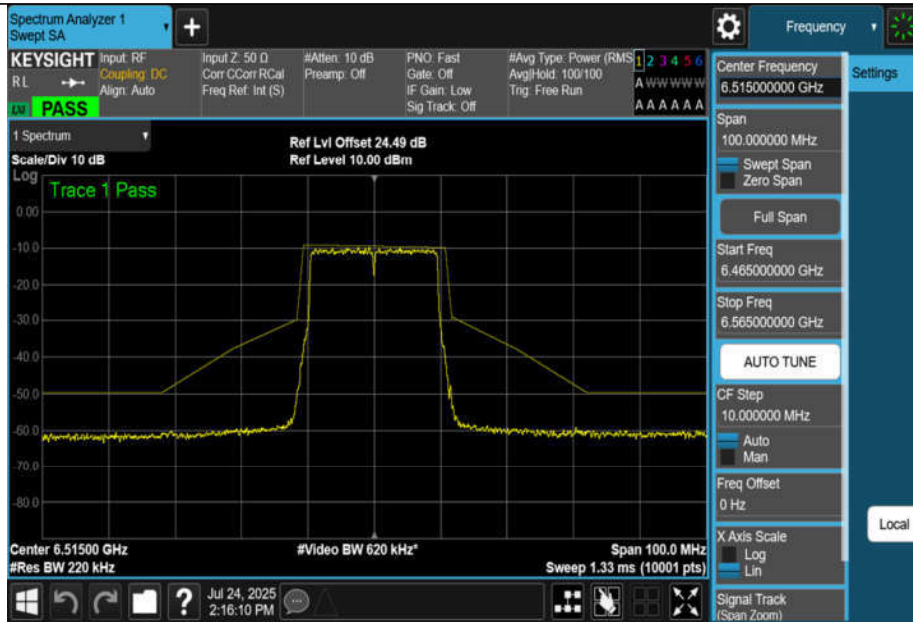
NTNV-11AX20MIMO-Ant1-6515-PASS
