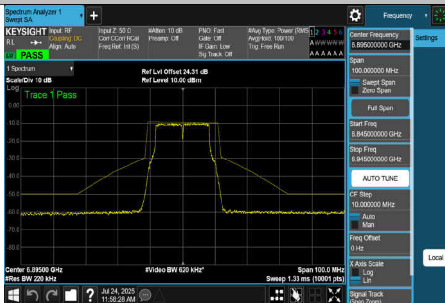
NTNV-11A-CDD-Ant2-6895-PASS
