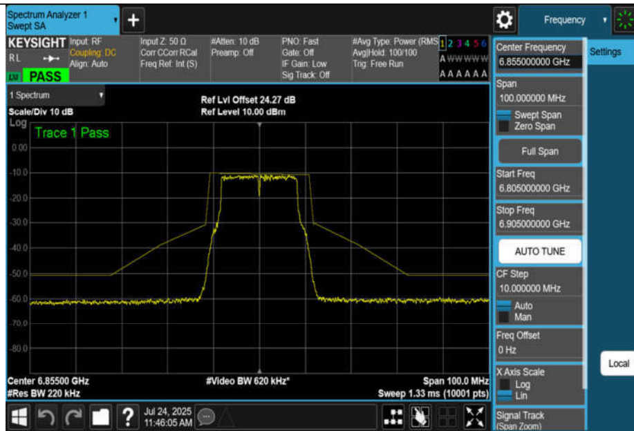
NTNV-11A-CDD-Ant1-6855-PASS
