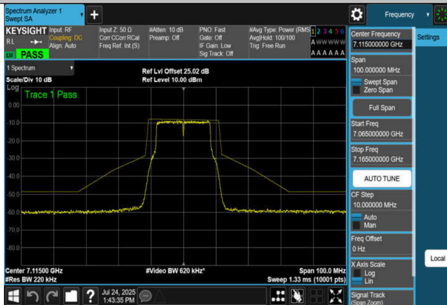
NTNV-11A-CDD-Ant4-7115-PASS
