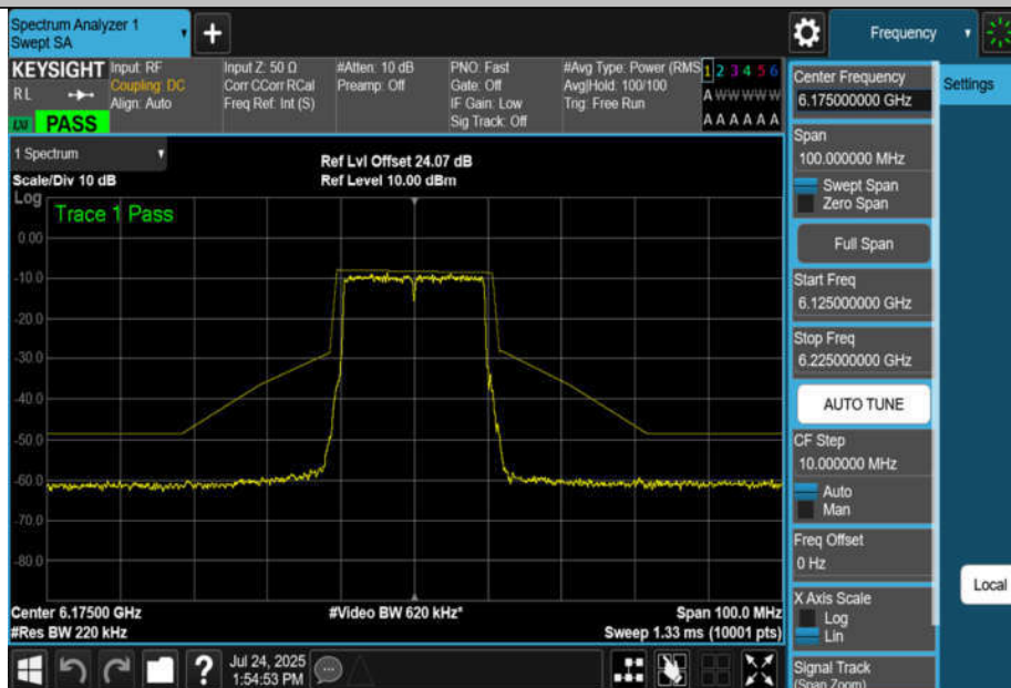
NTNV-11AX20MIMO-Ant4-6175-PASS
