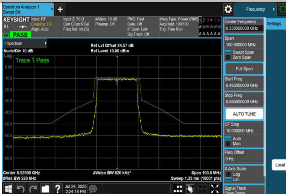
NTNV-11AX20MIMO-Ant4-6535-PASS
