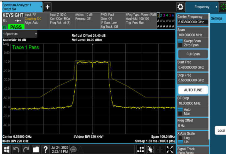
NTNV-11AX20MIMO-Ant2-6535-PASS
