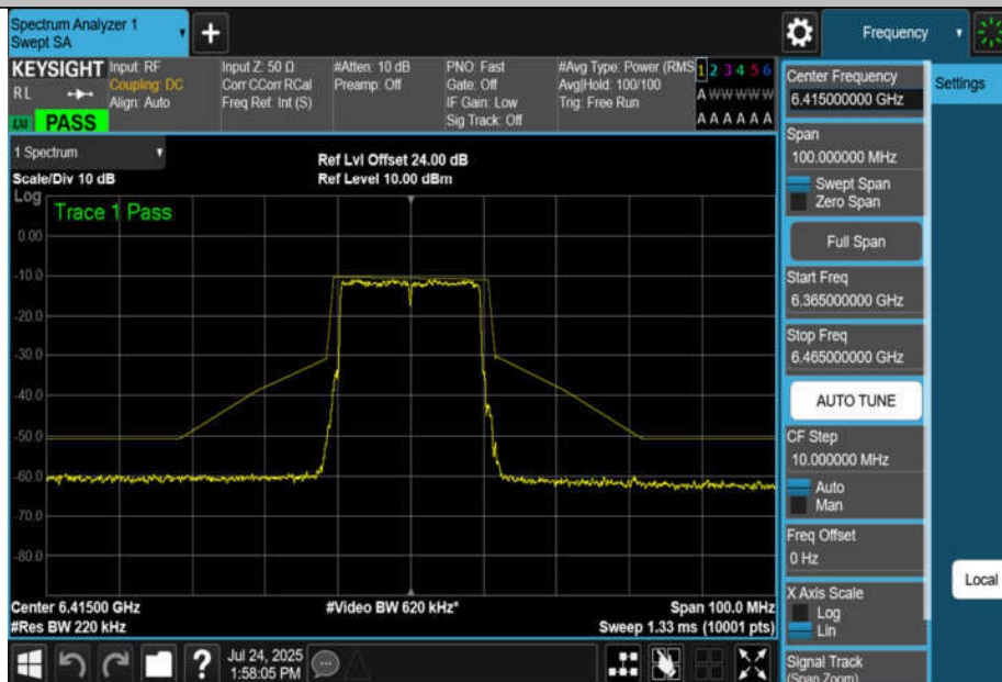
NTNV-11AX20MIMO-Ant2-6415-PASS
