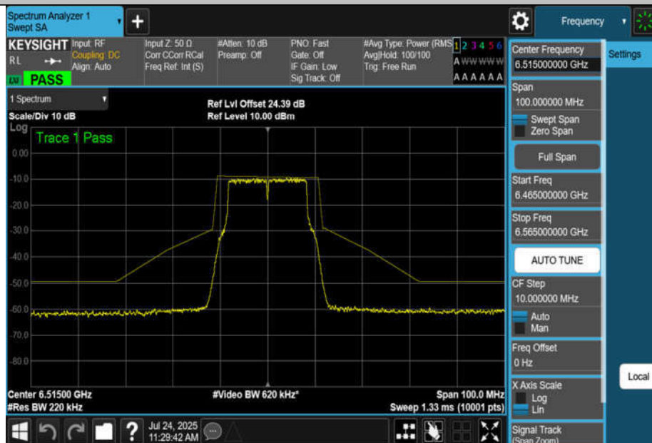
NTNV-11A-CDD-Ant2-6515-PASS
