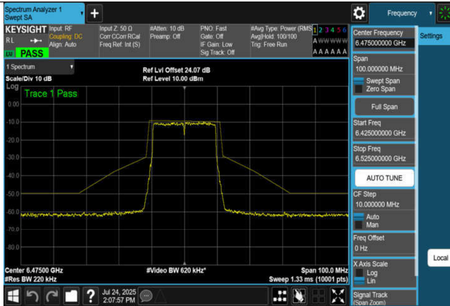
NTNV-11AX20MIMO-Ant1-6475-PASS
