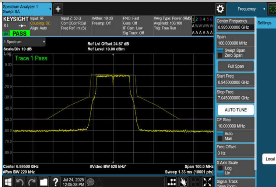
NTNV-11A-CDD-Ant4-6995-PASS
