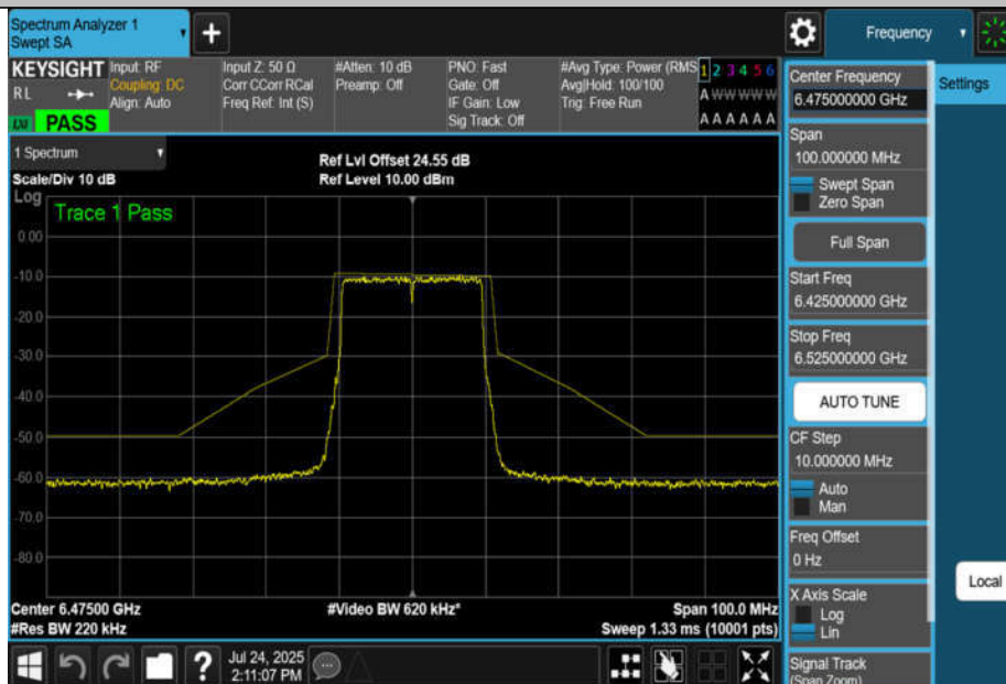
NTNV-11AX20MIMO-Ant4-6475-PASS
