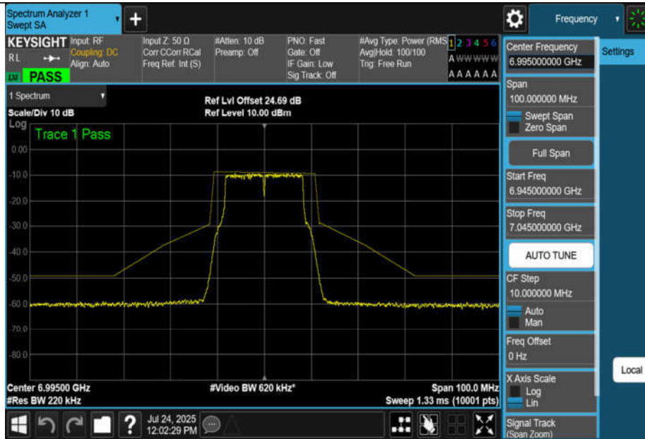
NTNV-11A-CDD-Ant1-6995-PASS
