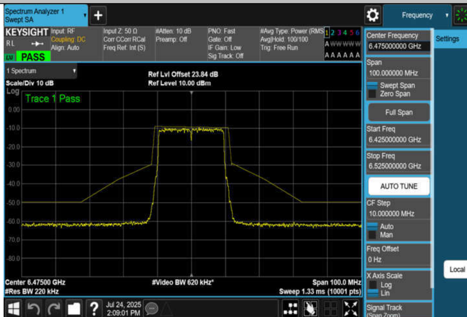
NTNV-11AX20MIMO-Ant2-6475-PASS
