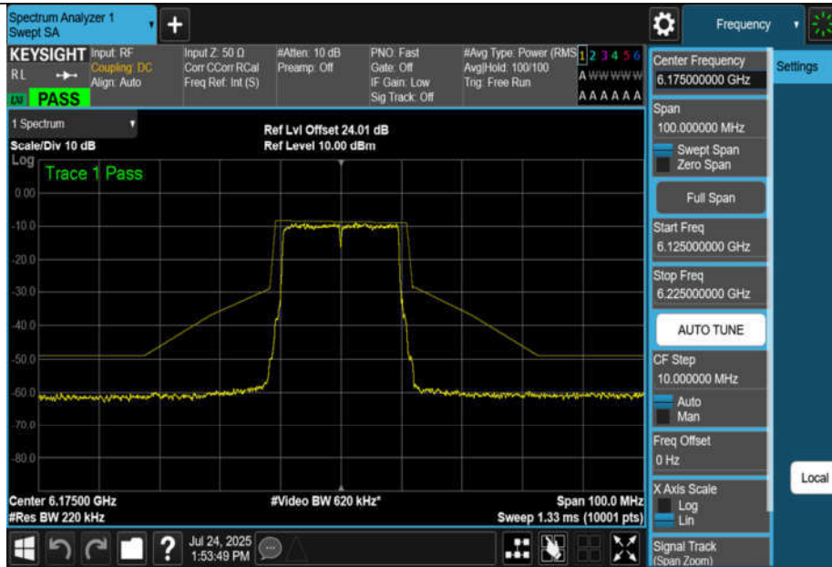
NTNV-11AX20MIMO-Ant3-6175-PASS
