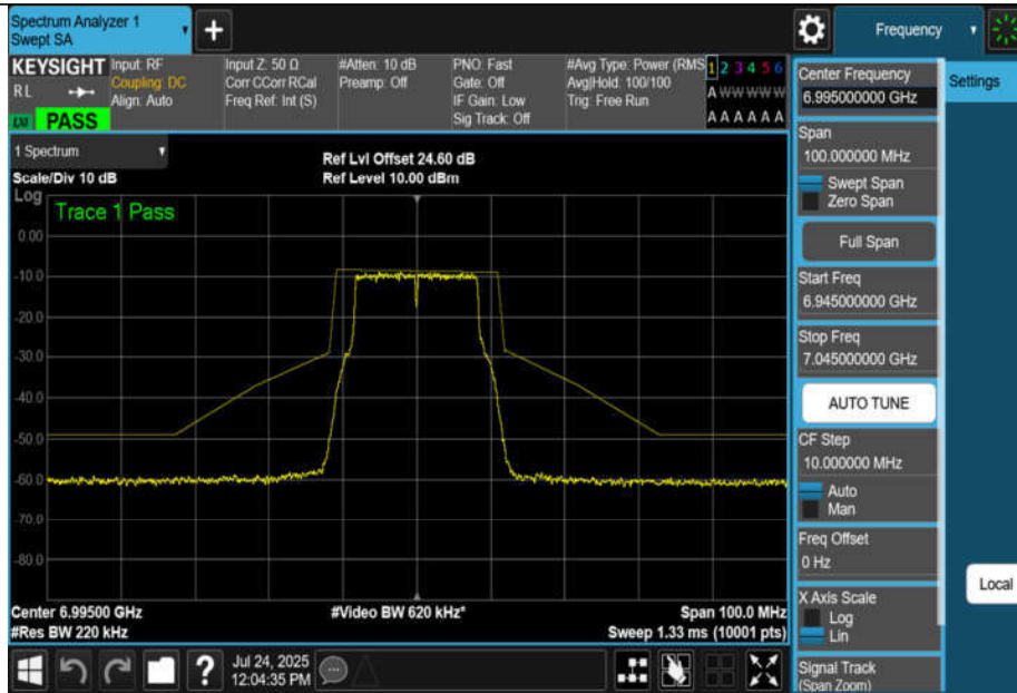
NTNV-11A-CDD-Ant3-6995-PASS
