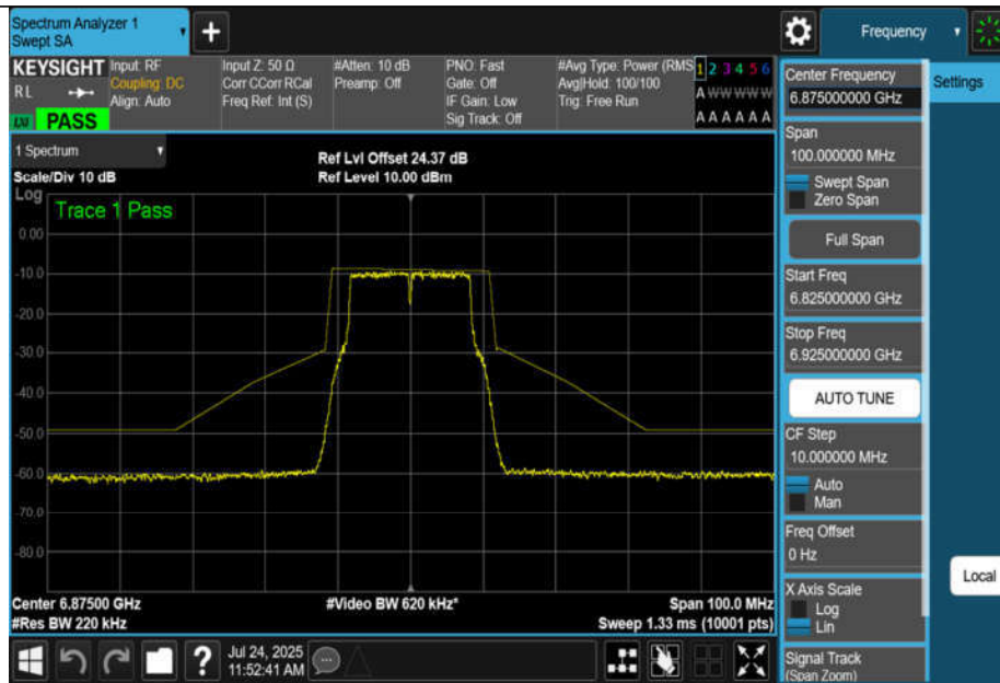
NTNV-11A-CDD-Ant1-6875-PASS
