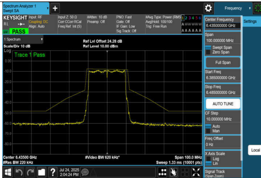
NTNV-11AX20MIMO-Ant3-6435-PASS
