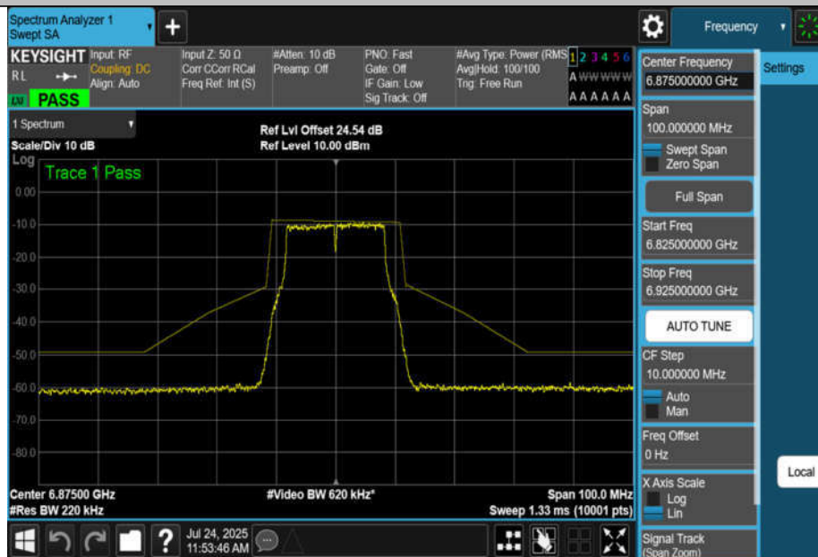
NTNV-11A-CDD-Ant2-6875-PASS
