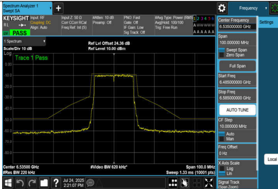
NTNV-11AX20MIMO-Ant1-6535-PASS
