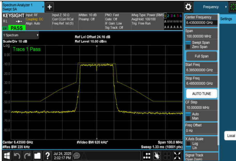
NTNV-11AX20MIMO-Ant1-6435-PASS
