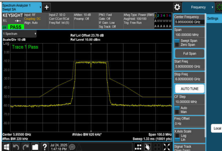
NTNV-11AX20MIMO-Ant2-5955-PASS
