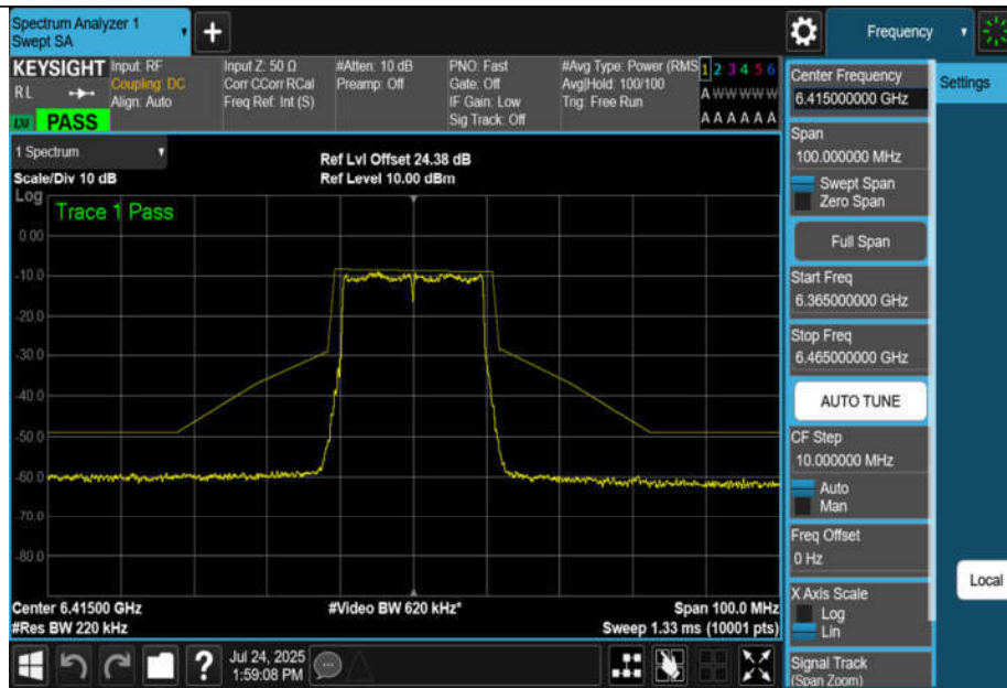
NTNV-11AX20MIMO-Ant3-6415-PASS
