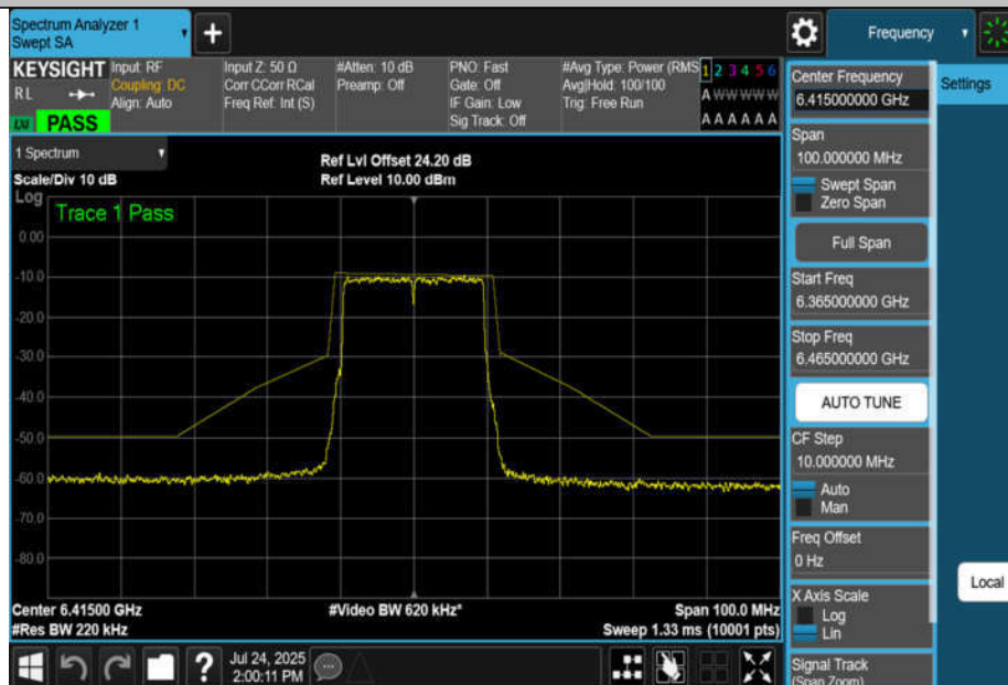
NTNV-11AX20MIMO-Ant4-6415-PASS
