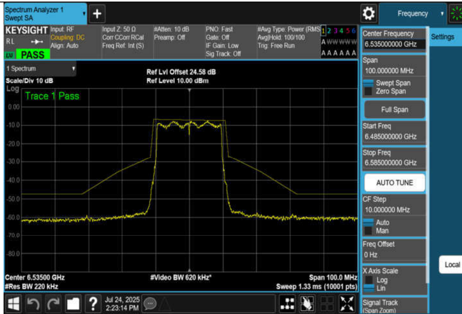
NTNV-11AX20MIMO-Ant3-6535-PASS
