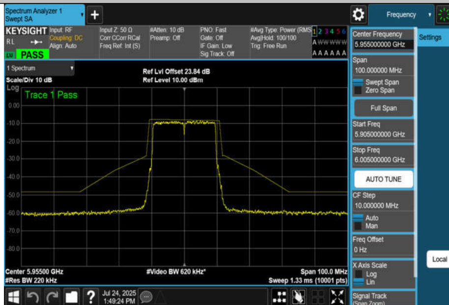
NTNV-11AX20MIMO-Ant4-5955-PASS
