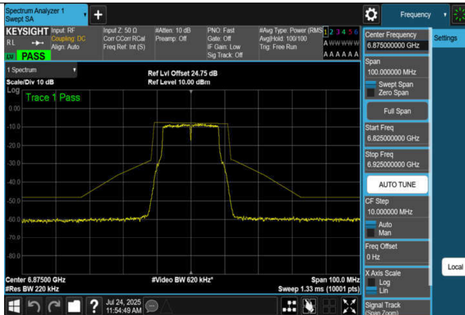
NTNV-11A-CDD-Ant3-6875-PASS
