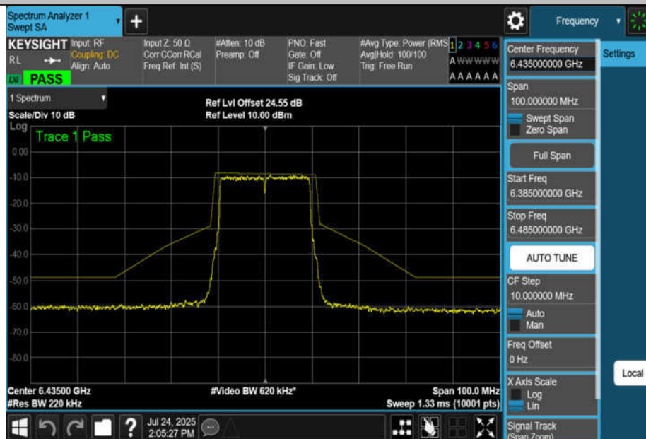
NTNV-11AX20MIMO-Ant4-6435-PASS
