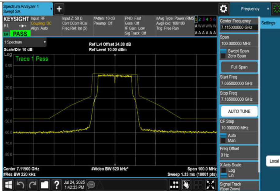
NTNV-11A-CDD-Ant3-7115-PASS
