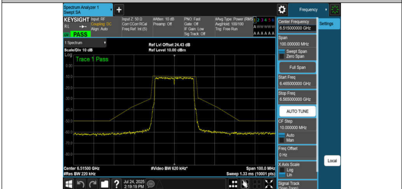
NTNV-11AX20MIMO-Ant4-6515-PASS
