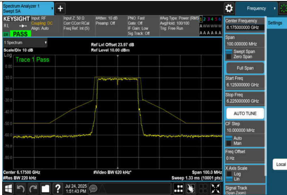
NTNV-11AX20MIMO-Ant1-6175-PASS
