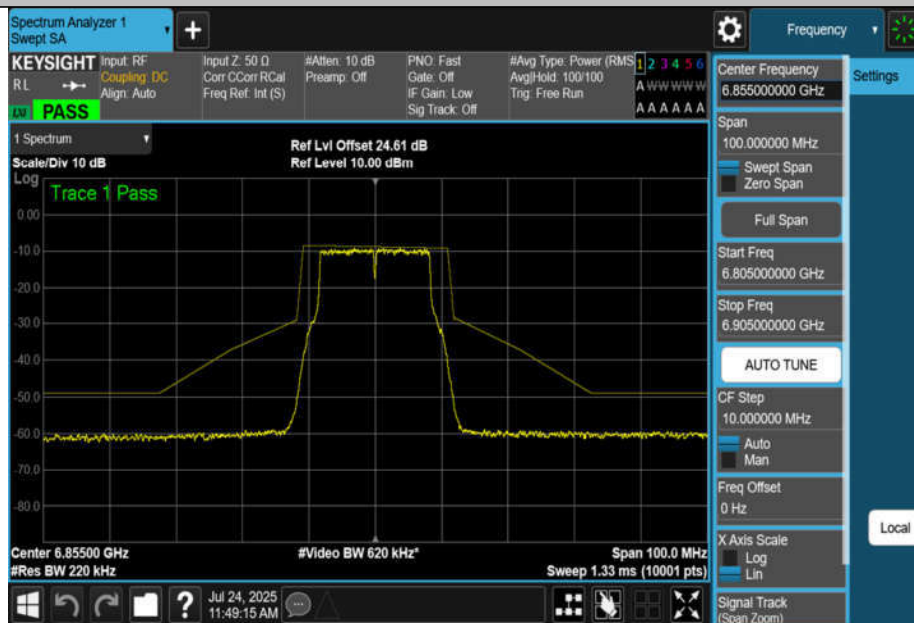
NTNV-11A-CDD-Ant4-6855-PASS
