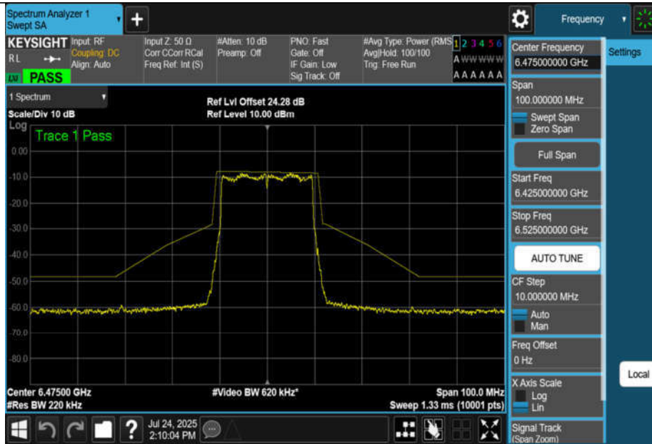
NTNV-11AX20MIMO-Ant3-6475-PASS
