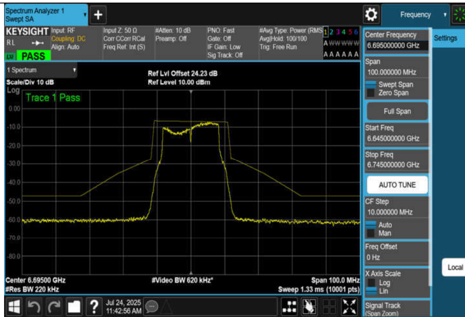
NTNV-11A-CDD-Ant3-6695-PASS
