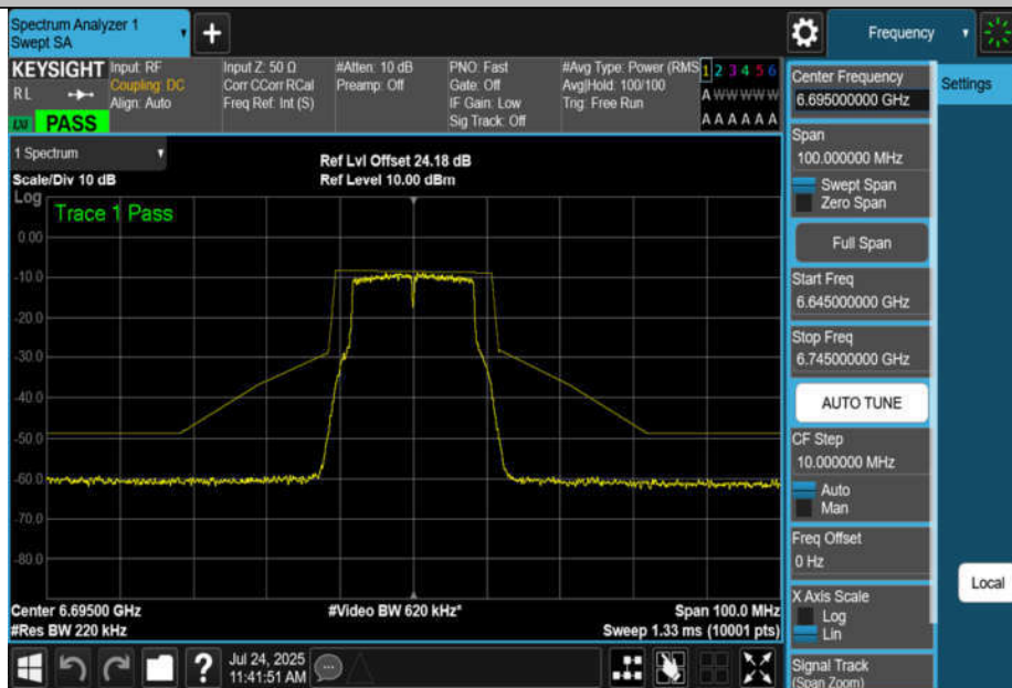
NTNV-11A-CDD-Ant2-6695-PASS
