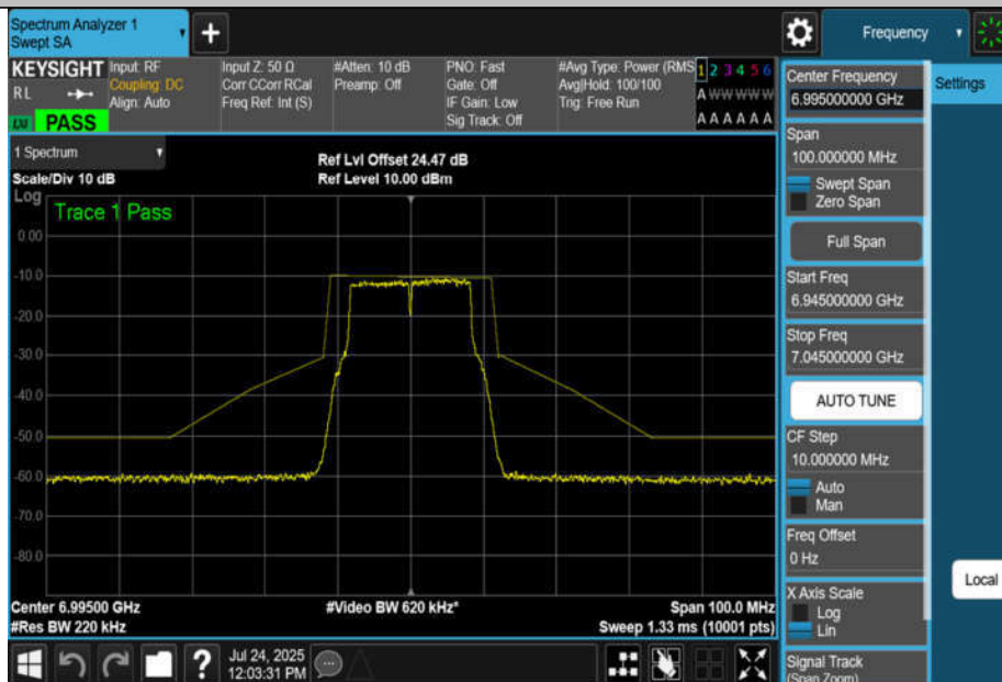
NTNV-11A-CDD-Ant2-6995-PASS
