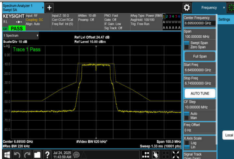
NTNV-11A-CDD-Ant4-6695-PASS
