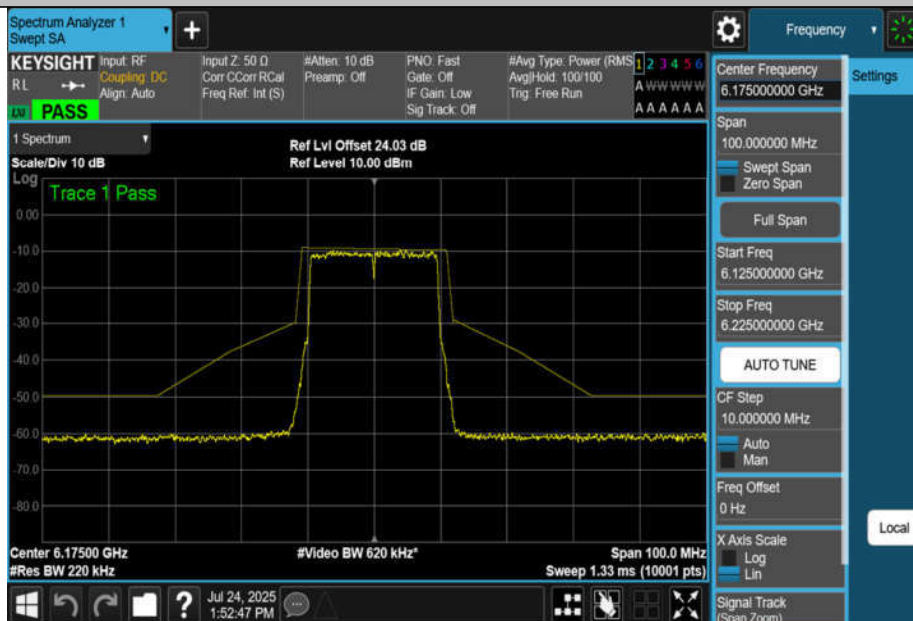
NTNV-11AX20MIMO-Ant2-6175-PASS
