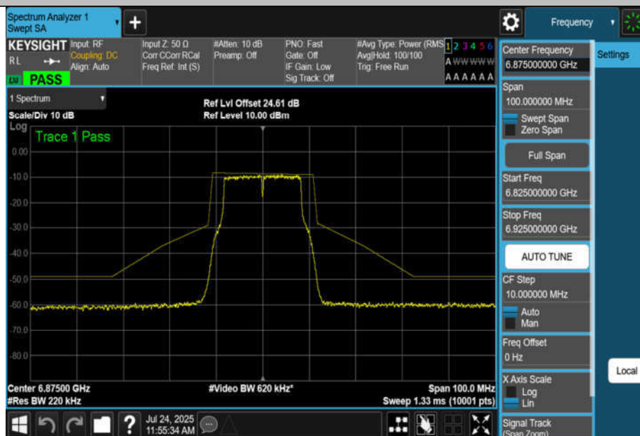
NTNV-11A-CDD-Ant4-6875-PASS
