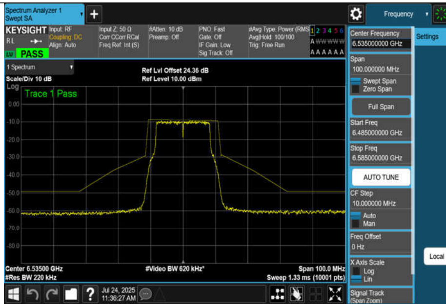
NTNV-11A-CDD-Ant1-6535-PASS
