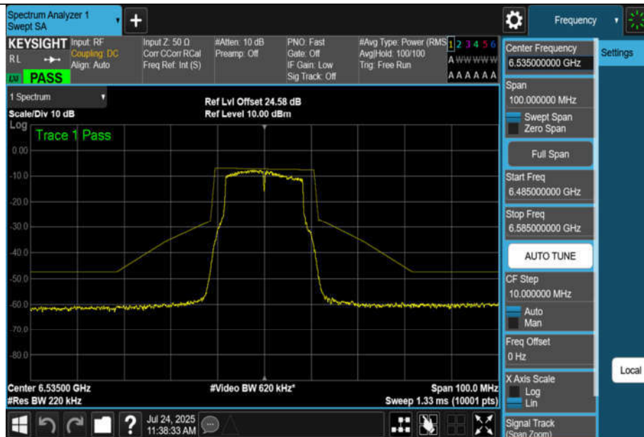
NTNV-11A-CDD-Ant3-6535-PASS
