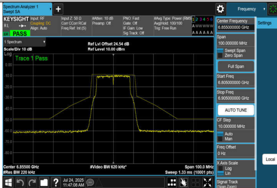
NTNV-11A-CDD-Ant2-6855-PASS
