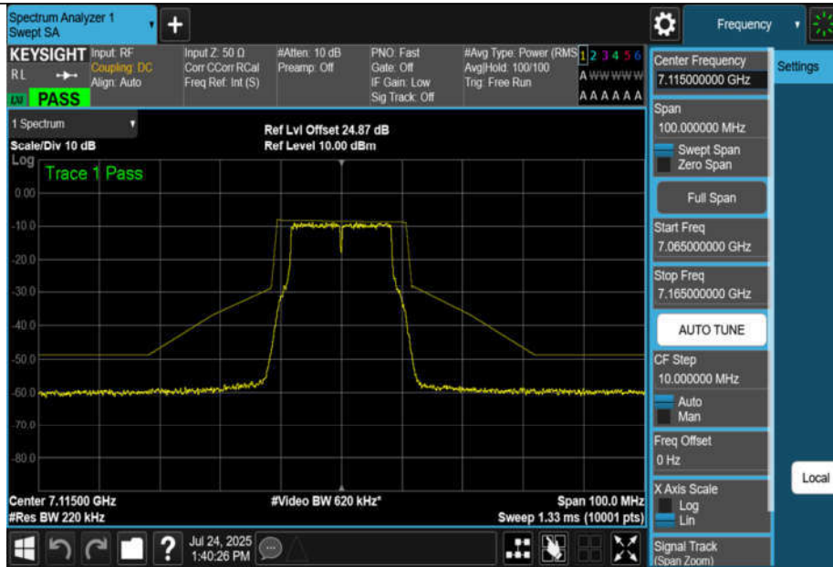
NTNV-11A-CDD-Ant1-7115-PASS
