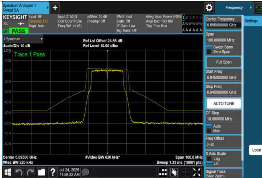
NTNV-11A-CDD-Ant3-6895-PASS
