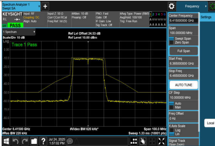
NTNV-11AX20MIMO-Ant1-6415-PASS
