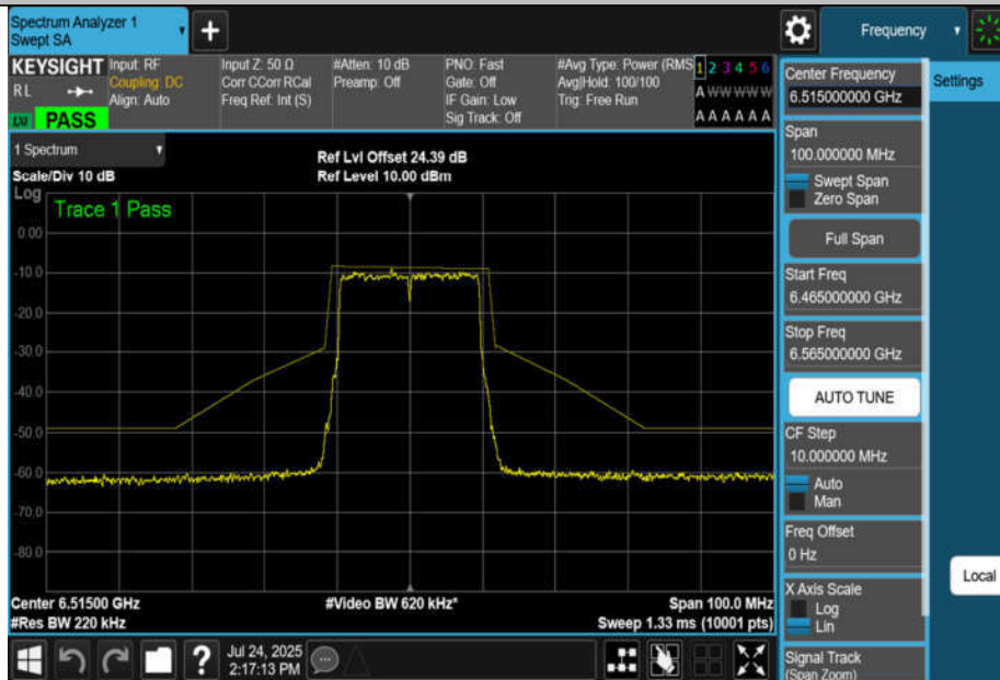
NTNV-11AX20MIMO-Ant2-6515-PASS
