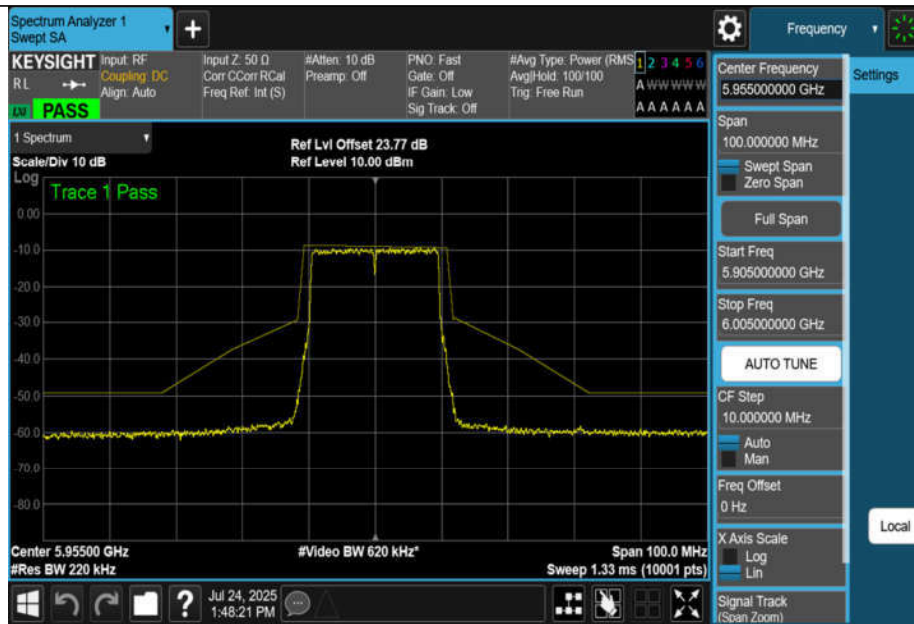
NTNV-11AX20MIMO-Ant3-5955-PASS
