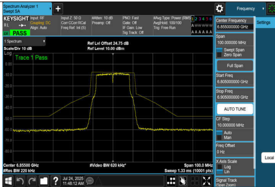
NTNV-11A-CDD-Ant3-6855-PASS
