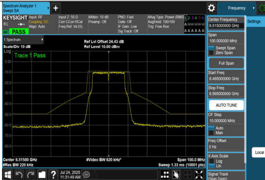
NTNV-11A-CDD-Ant4-6515-PASS
