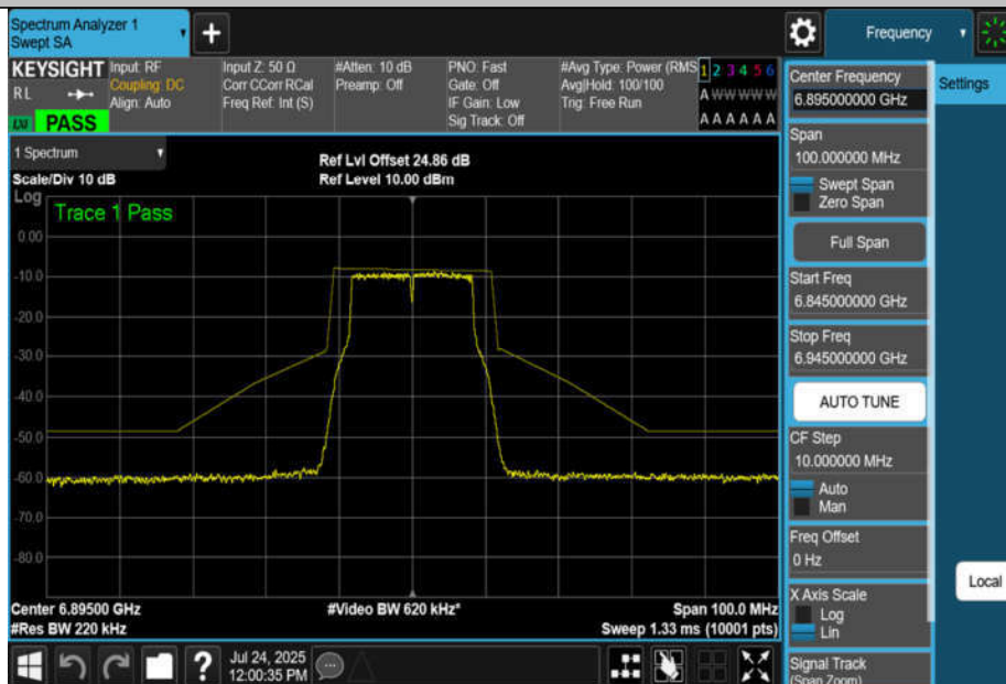
NTNV-11A-CDD-Ant4-6895-PASS
