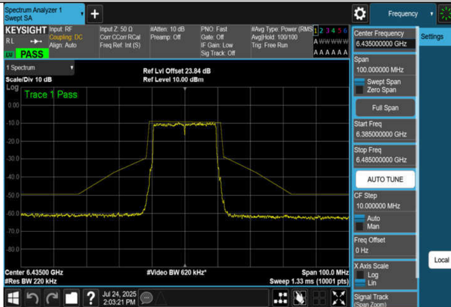
NTNV-11AX20MIMO-Ant2-6435-PASS
