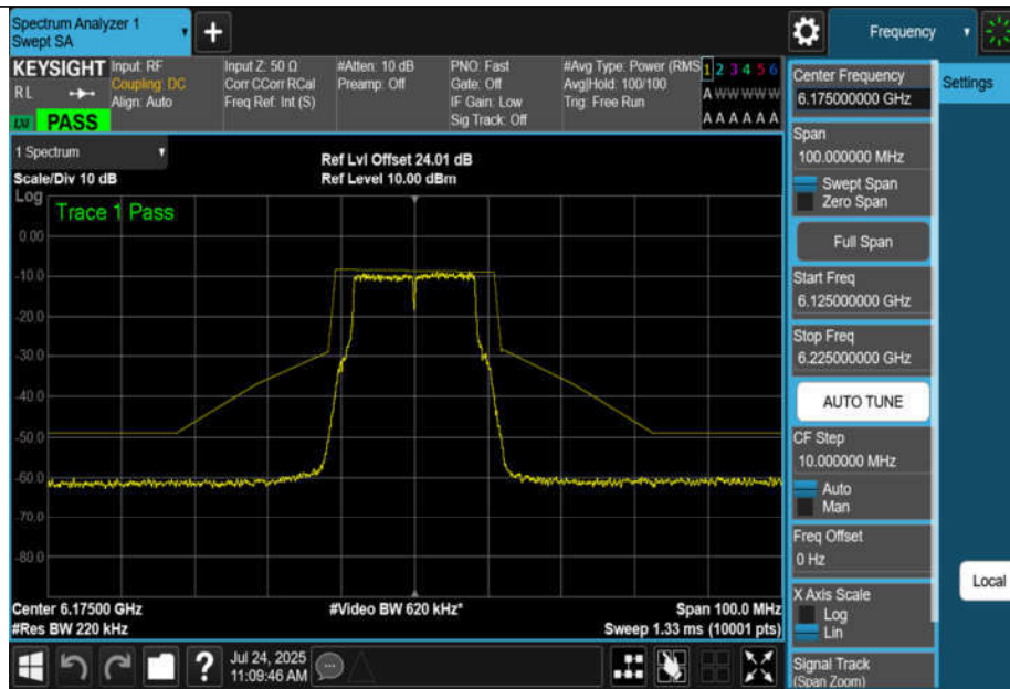
NTNV-11A-CDD-Ant3-6175-PASS
