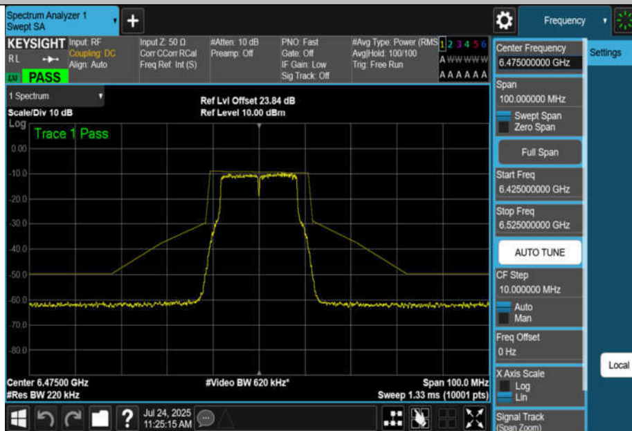
NTNV-11A-CDD-Ant2-6475-PASS
