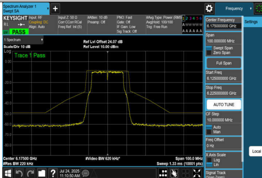
NTNV-11A-CDD-Ant4-6175-PASS
