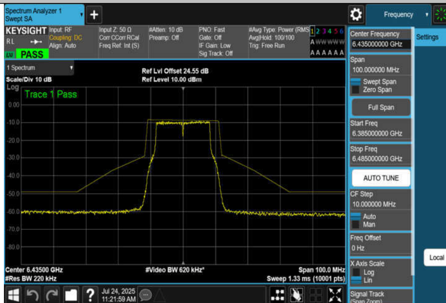
NTNV-11A-CDD-Ant4-6435-PASS
