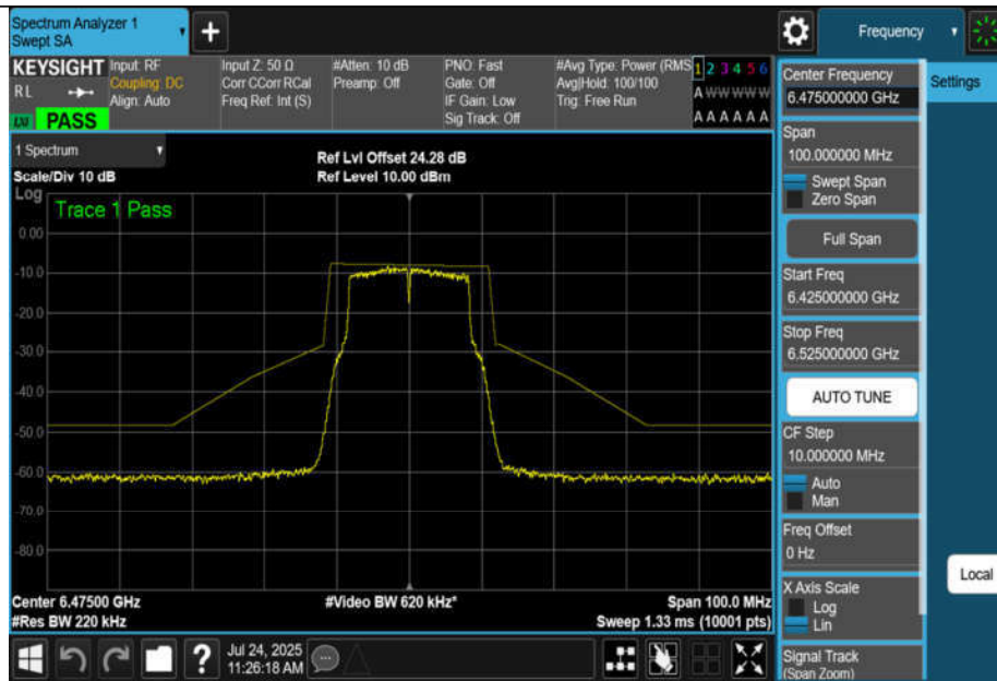
NTNV-11A-CDD-Ant3-6475-PASS
