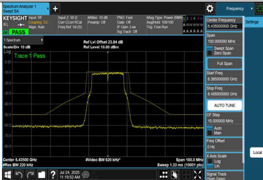
NTNV-11A-CDD-Ant2-6435-PASS
