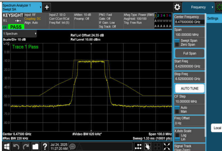
NTNV-11A-CDD-Ant4-6475-PASS
