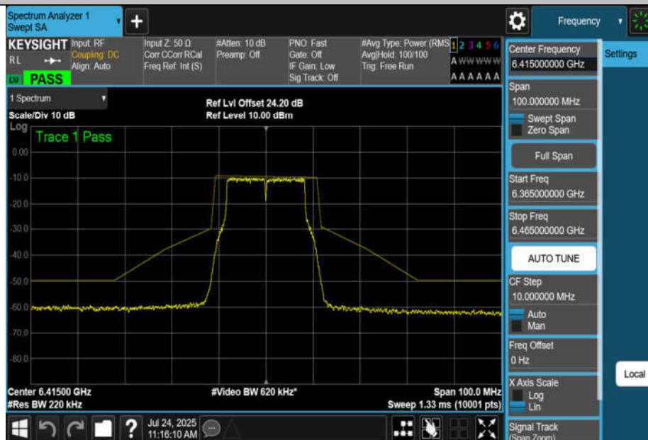
NTNV-11A-CDD-Ant4-6415-PASS
