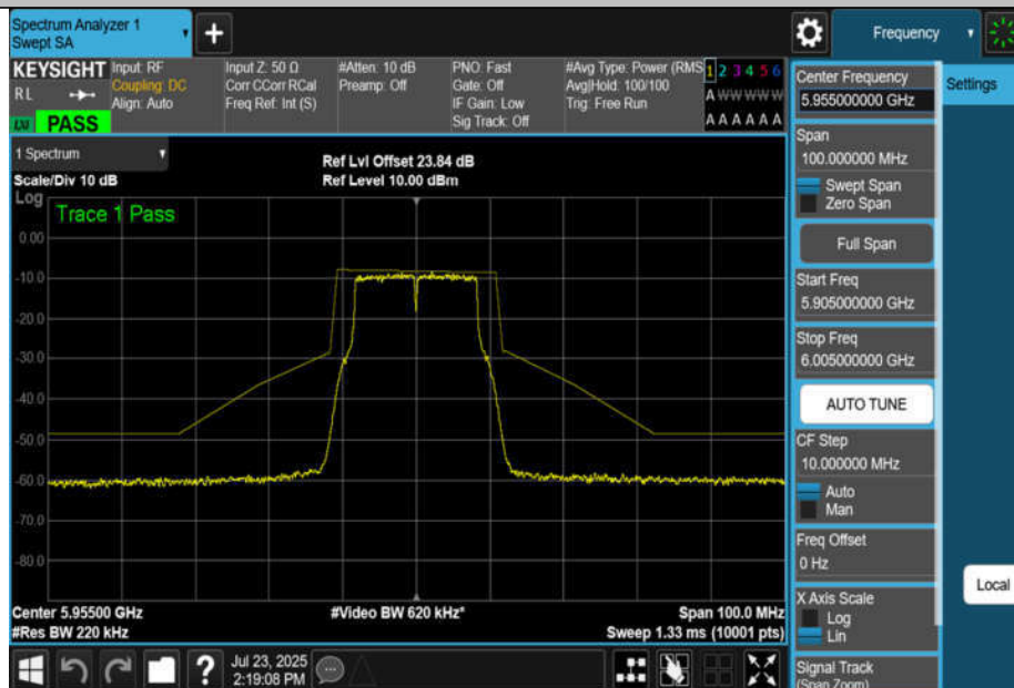
NTNV-11A-CDD-Ant4-5955-PASS
