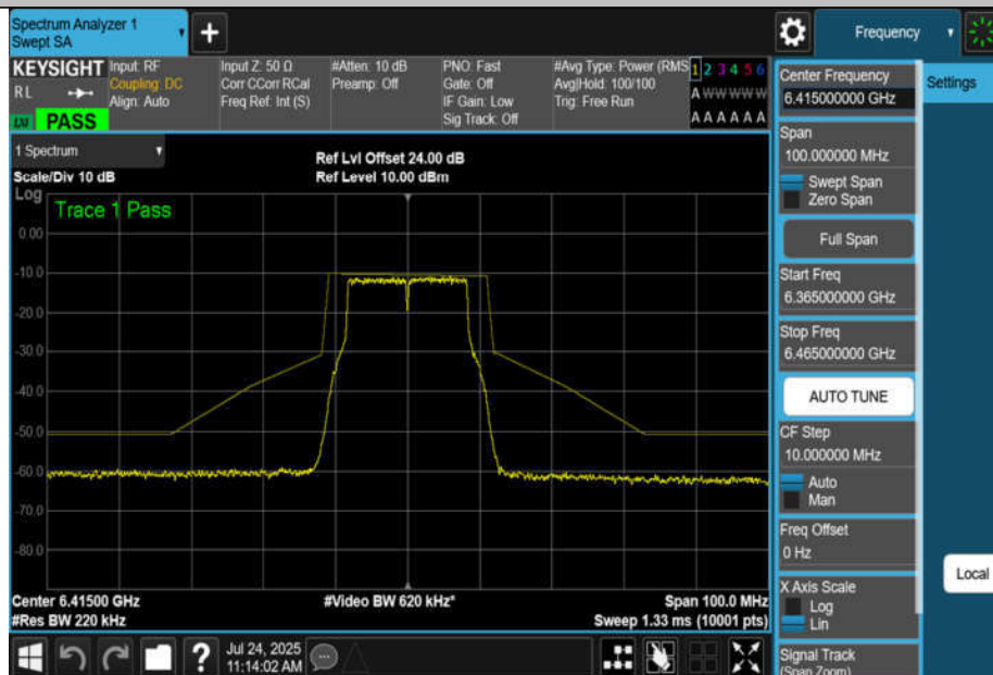
NTNV-11A-CDD-Ant2-6415-PASS
