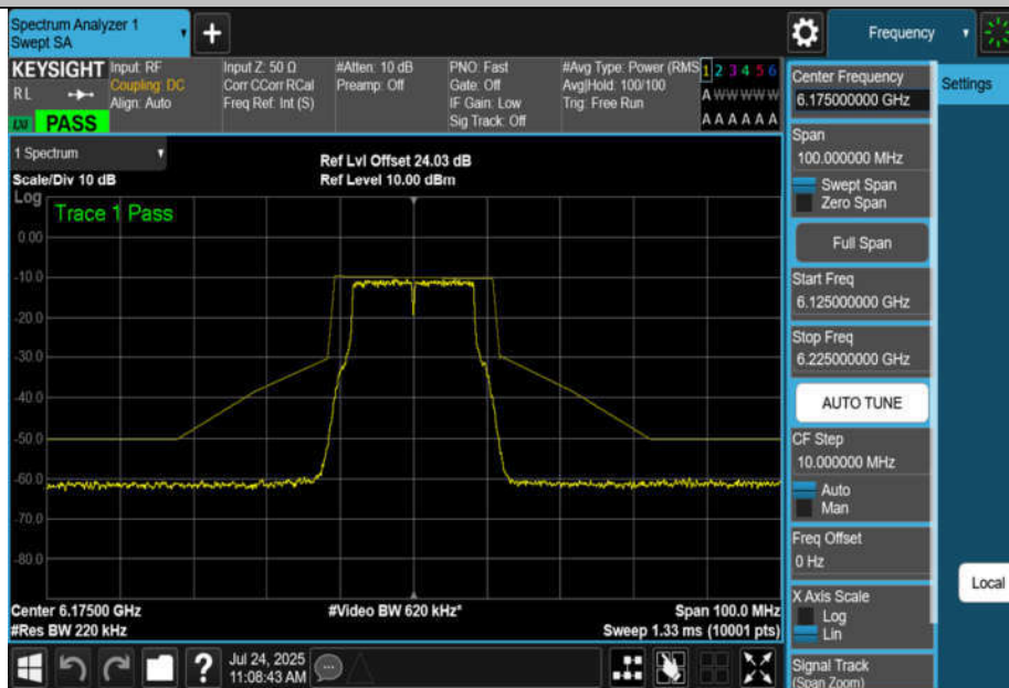
NTNV-11A-CDD-Ant2-6175-PASS
