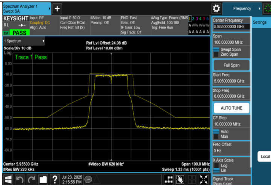
NTVN-11A-CDD-Ant1-5955-PASS
