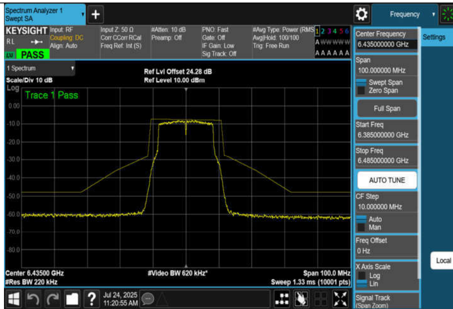
NTNV-11A-CDD-Ant3-6435-PASS
