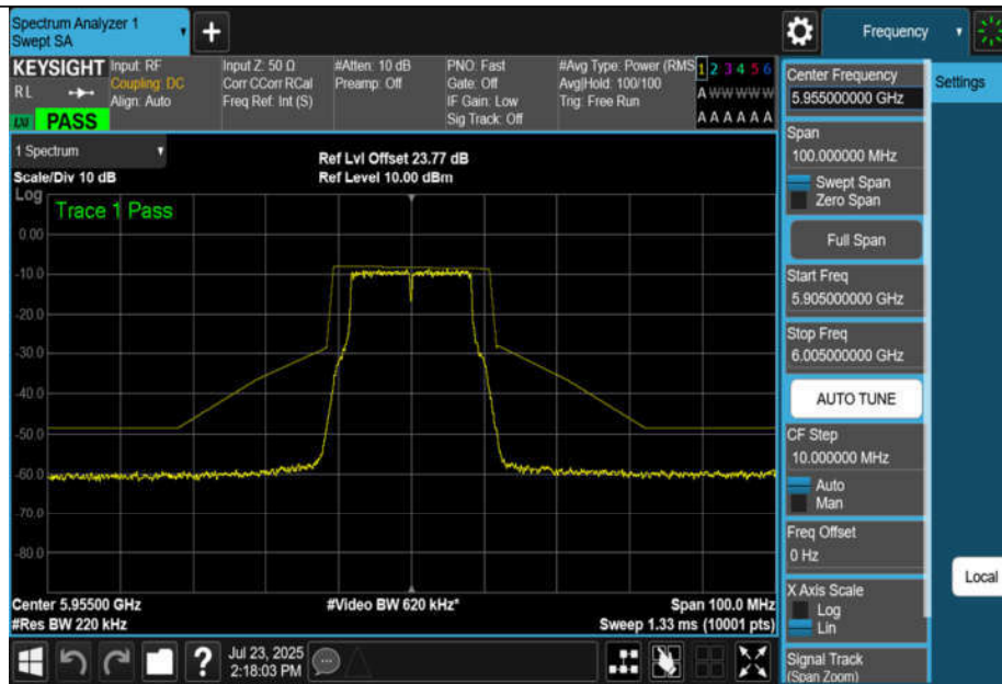
NTNV-11A-CDD-Ant3-5955-PASS
