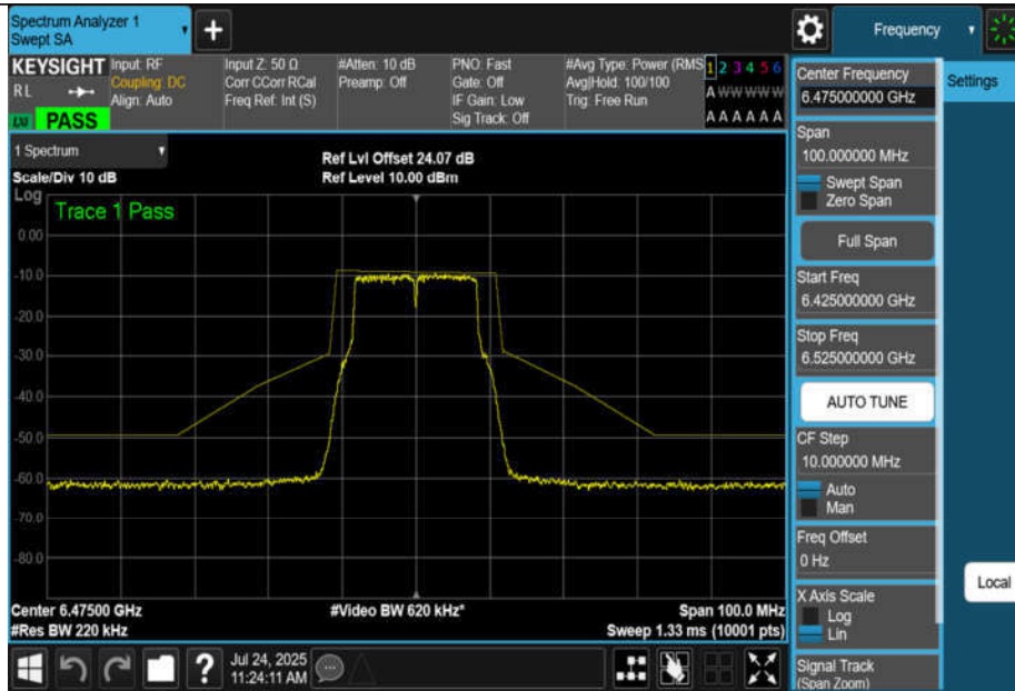
NTNV-11A-CDD-Ant1-6475-PASS
