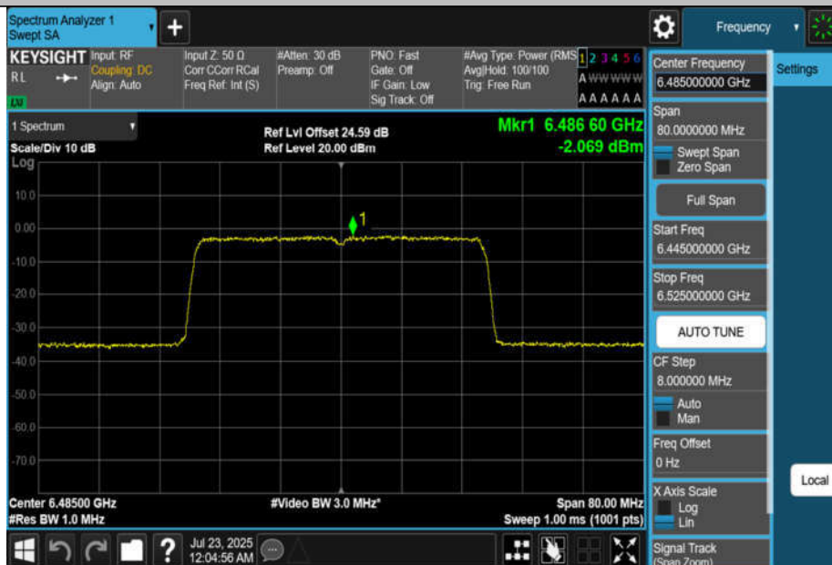
11BE40MIMO-Ant4-6485-PASS
