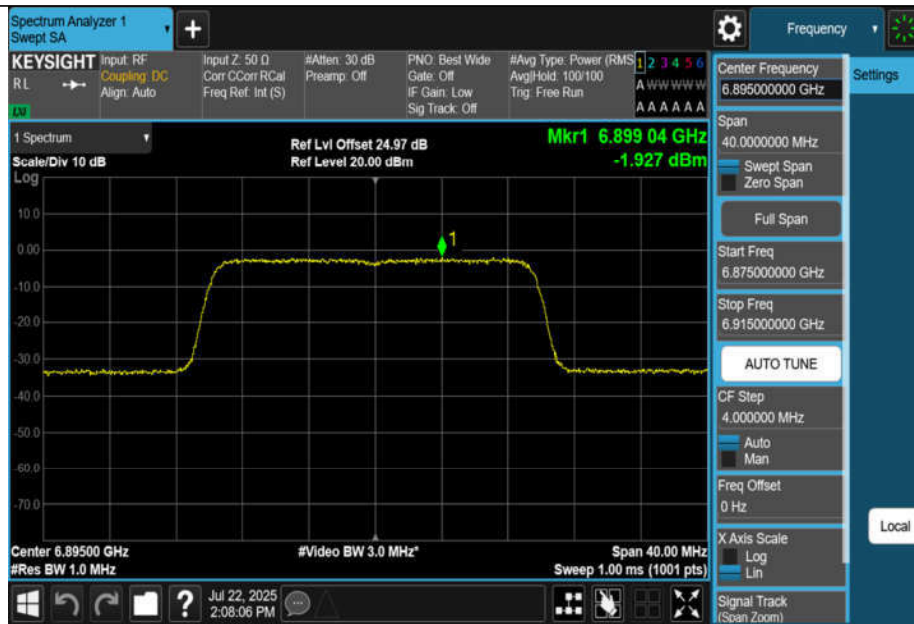
11BE20MIMO-Ant4-6895-PASS
