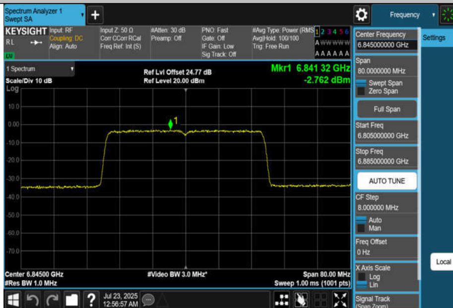
11BE40MIMO-Ant4-6845-PASS
