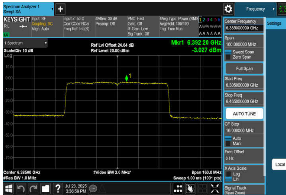
11BE80MIMO-Ant1-6385-PASS
