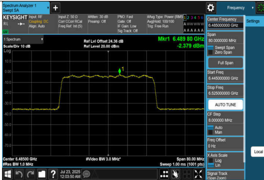
11BE40MIMO-Ant3-6485-PASS
