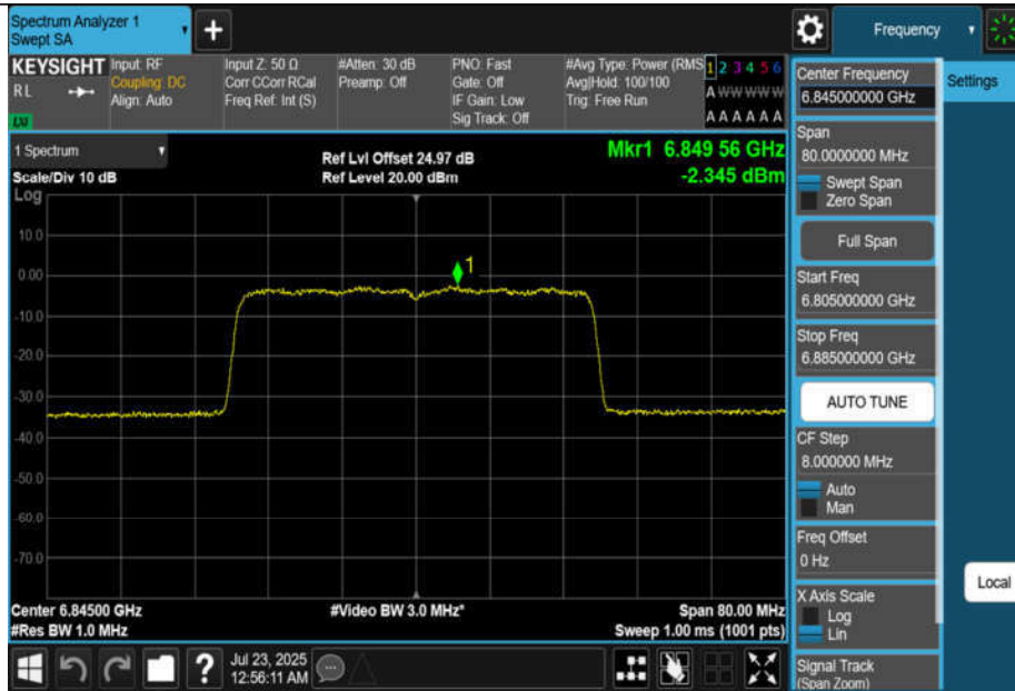
11BE40MIMO-Ant3-6845-PASS
