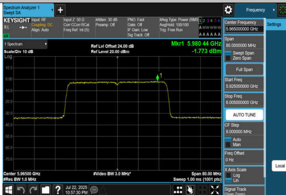
11BE40MIMO-Ant4-5965-PASS
