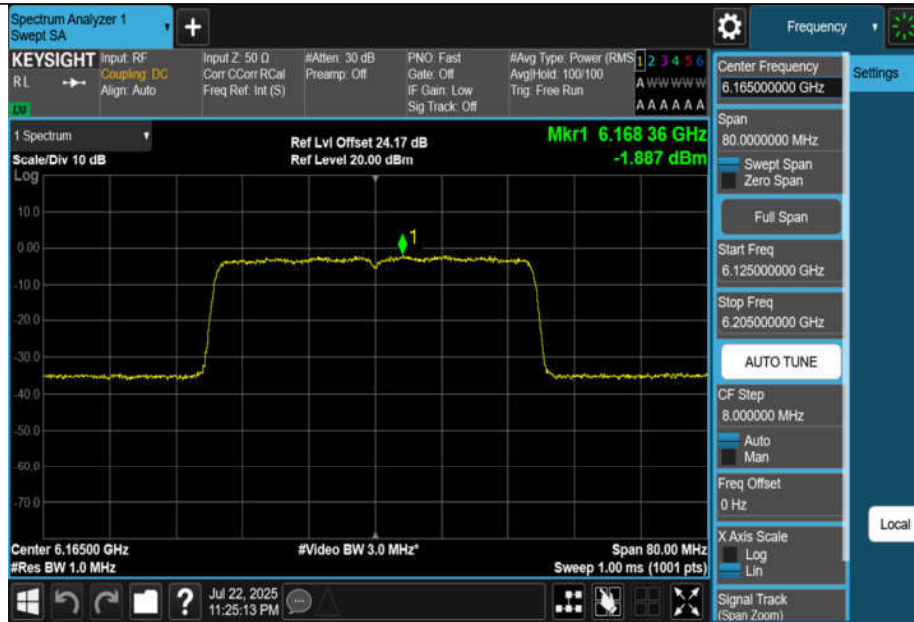
11BE40MIMO-Ant3-6165-PASS
