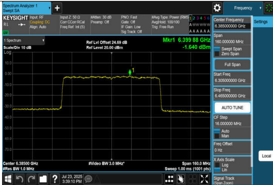
11BE80MIMO-Ant3-6385-PASS
