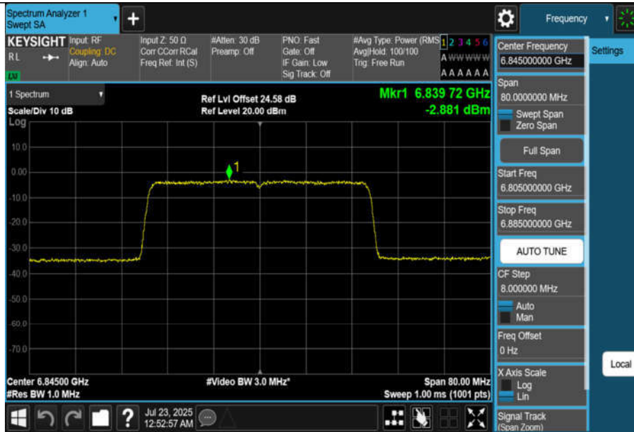
11BE40MIMO-Ant1-6845-PASS
