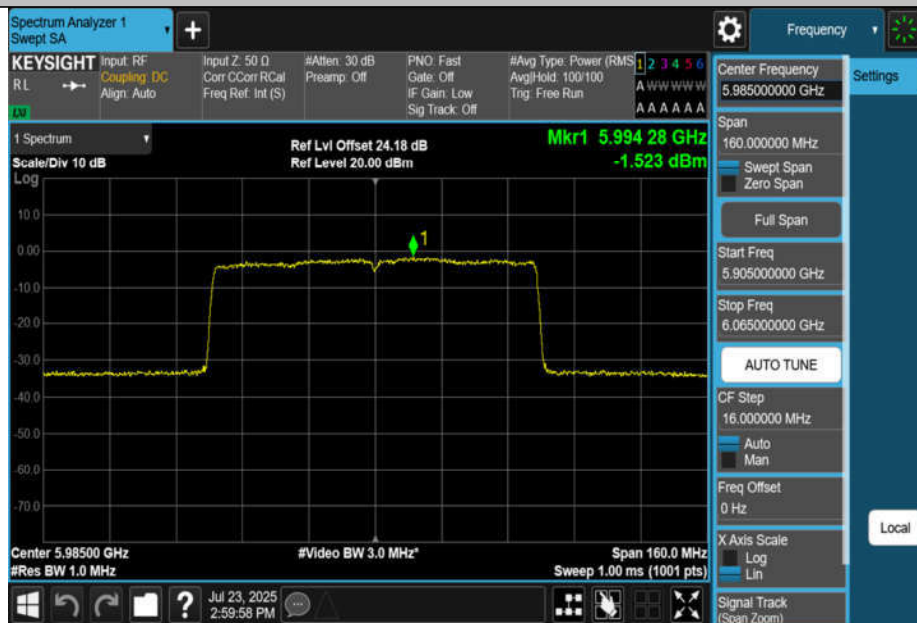
11BE80MIMO-Ant4-5985-PASS
