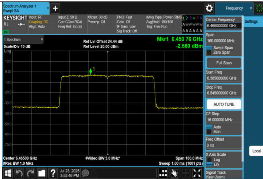
11BE80MIMO-Ant1-6465-PASS
