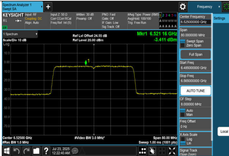
11BE40MIMO-Ant1-6525-PASS
