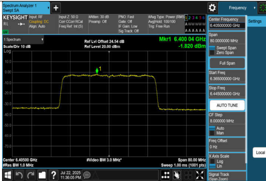
11BE40MIMO-Ant3-6405-PASS
