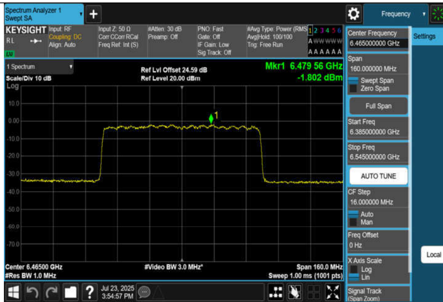
11BE80MIMO-Ant3-6465-PASS
