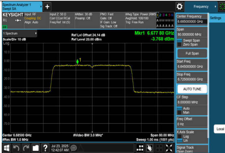
11BE40MIMO-Ant1-6685-PASS
