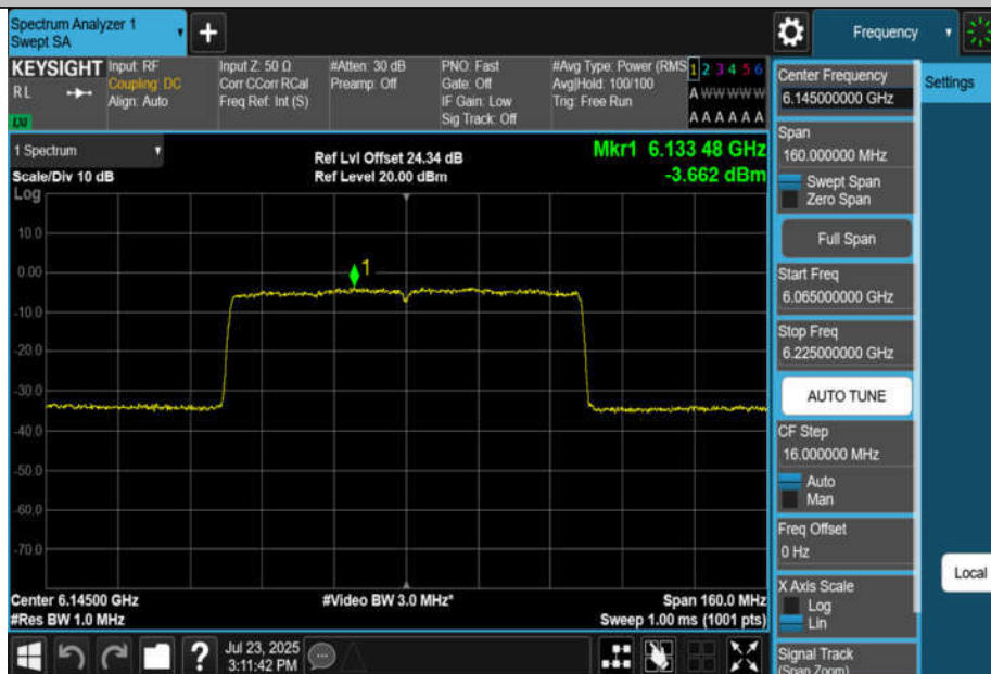
11BE80MIMO-Ant2-6145-PASS
