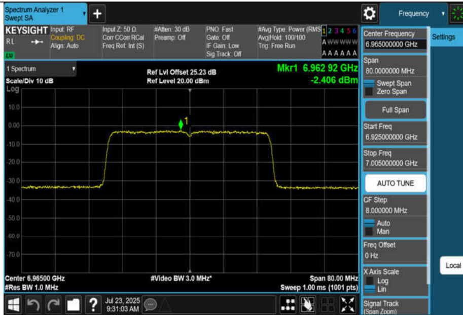
11BE40MIMO-Ant1-6965-PASS
