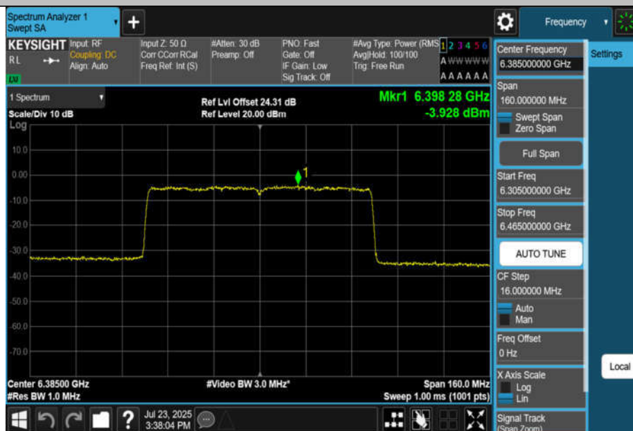
11BE80MIMO-Ant2-6385-PASS
