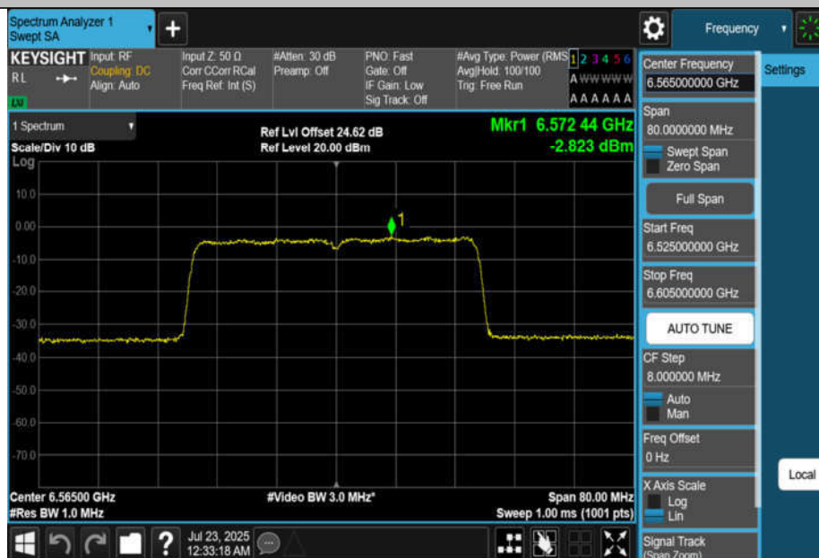
11BE40MIMO-Ant2-6565-PASS
