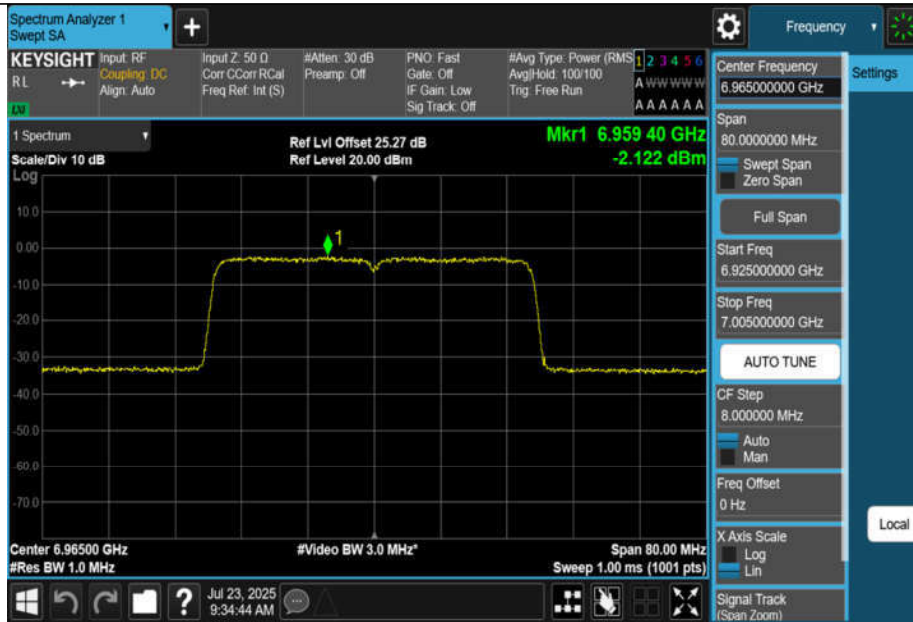
11BE40MIMO-Ant3-6965-PASS
