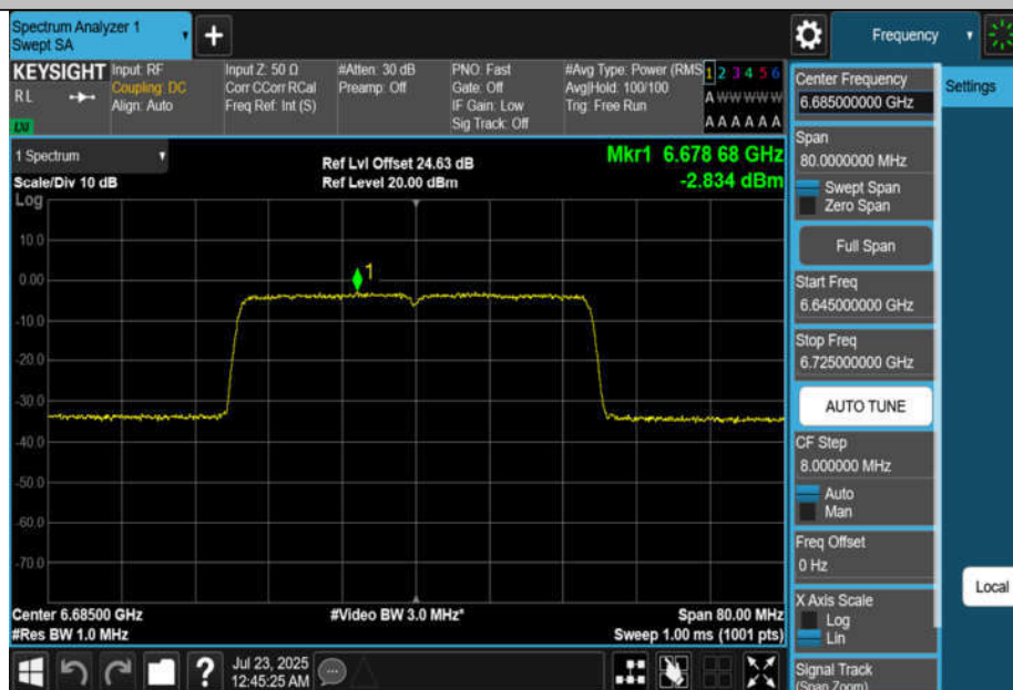
11BE40MIMO-Ant4-6685-PASS
