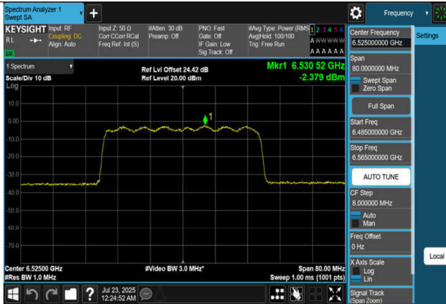
11BE40MIMO-Ant3-6525-PASS
