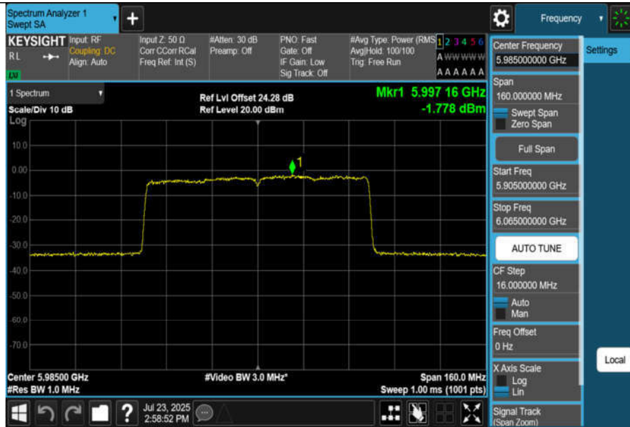
11BE80MIMO-Ant3-5985-PASS
