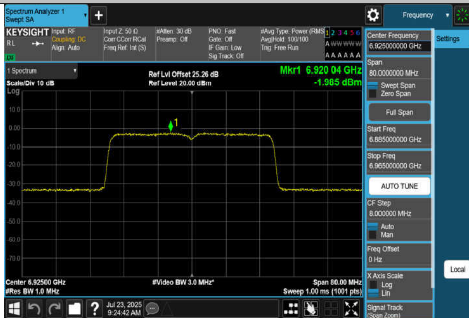
11BE40MIMO-Ant4-6925-PASS
