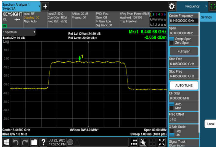
11BE40MIMO-Ant3-6445-PASS
