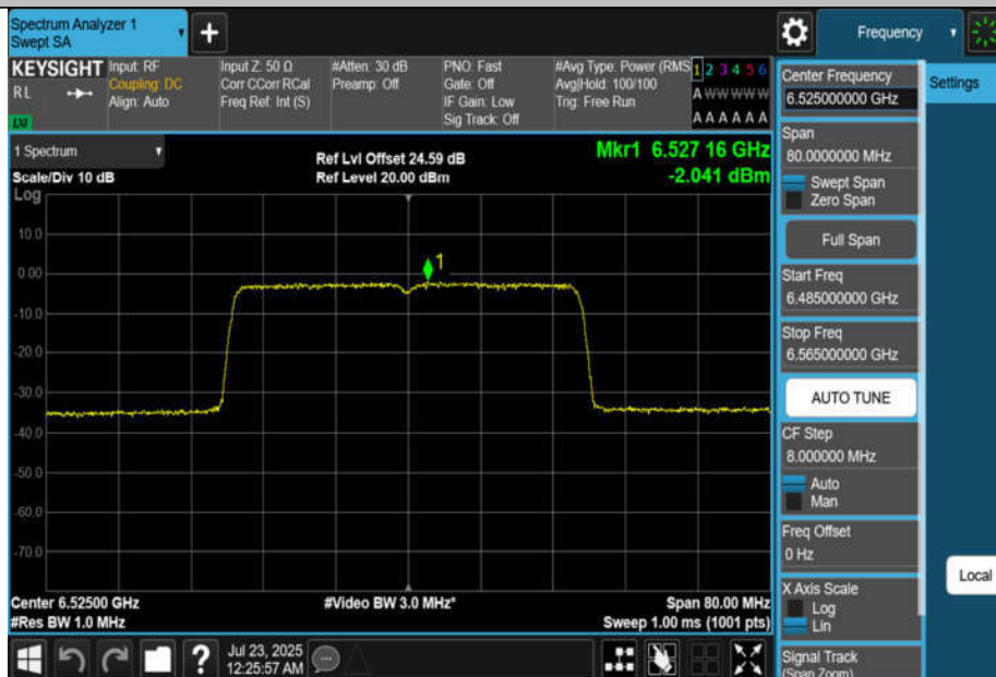
11BE40MIMO-Ant4-6525-PASS
