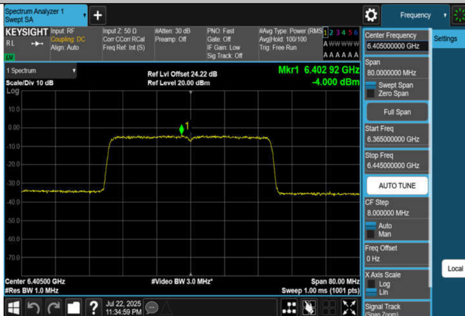
11BE40MIMO-Ant2-6405-PASS
