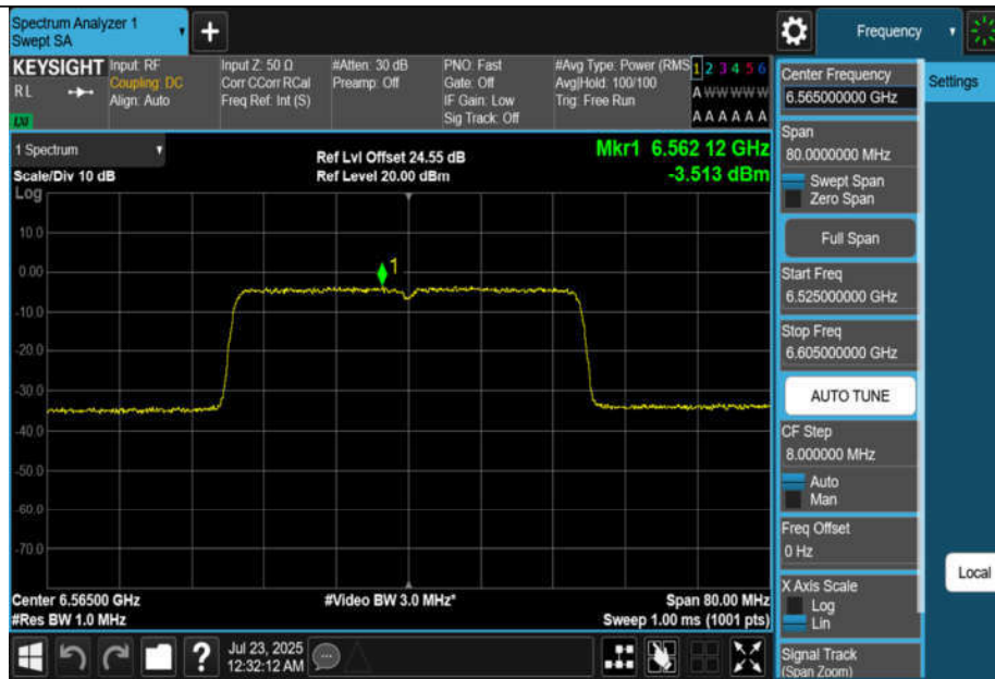
11BE40MIMO-Ant1-6565-PASS
