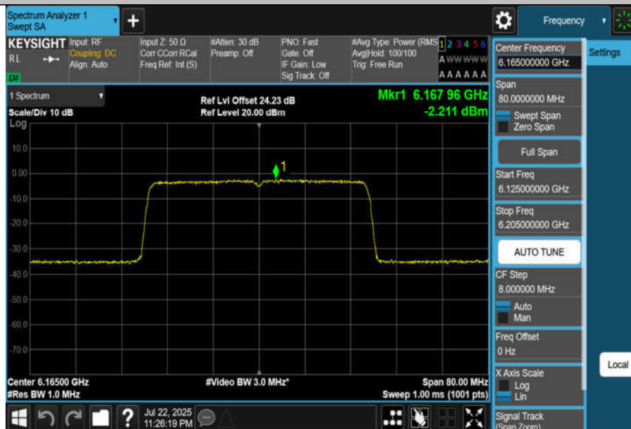
11BE40MIMO-Ant4-6165-PASS
