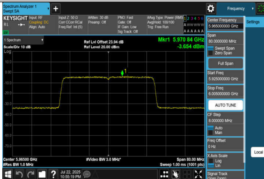
11BE40MIMO-Ant2-5965-PASS
