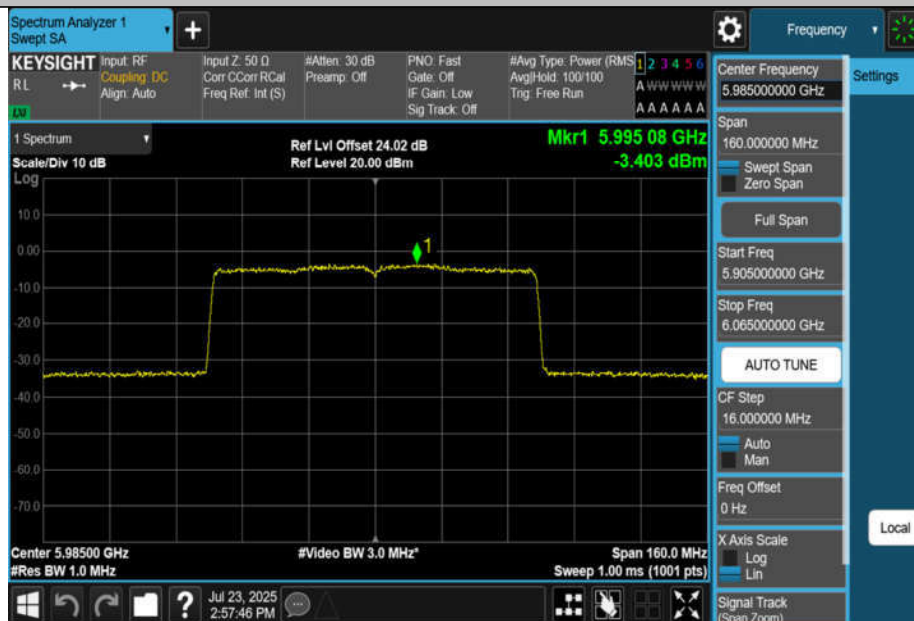
11BE80MIMO-Ant2-5985-PASS
