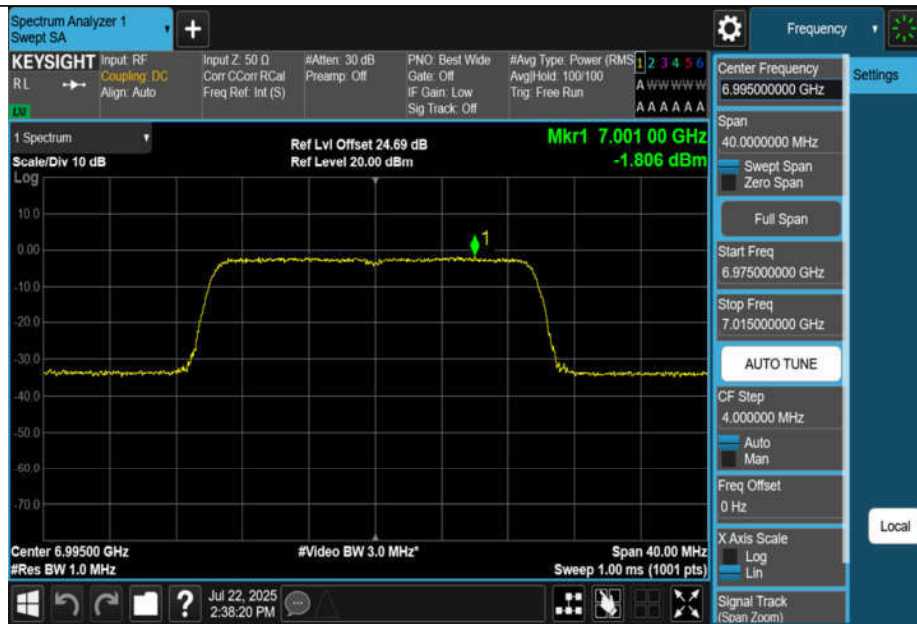
11BE20MIMO-Ant3-6995-PASS
