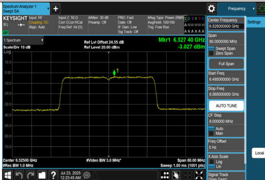
11BE40MIMO-Ant2-6525-PASS
