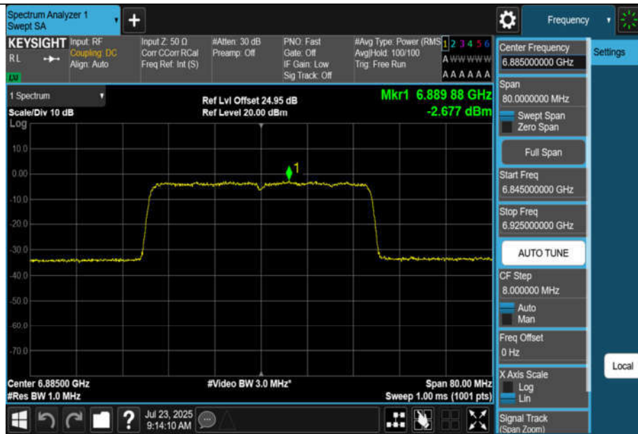
11BE40MIMO-Ant3-6885-PASS
