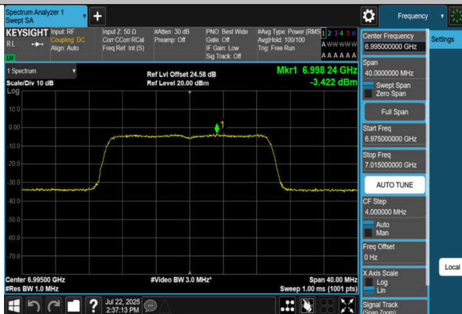
11BE20MIMO-Ant2-6995-PASS
