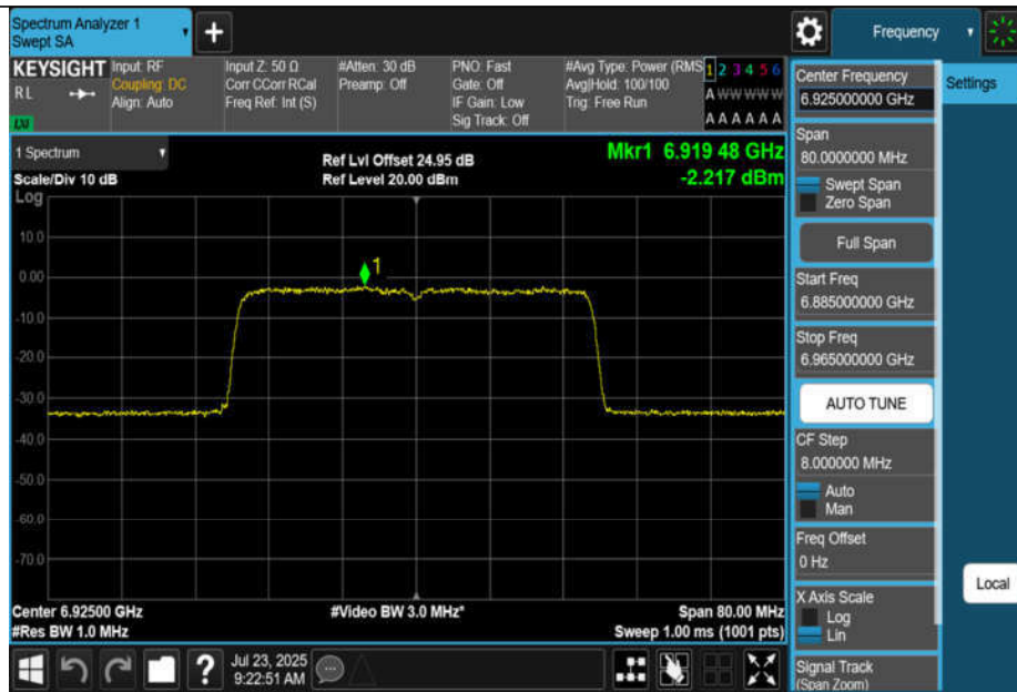
11BE40MIMO-Ant3-6925-PASS
