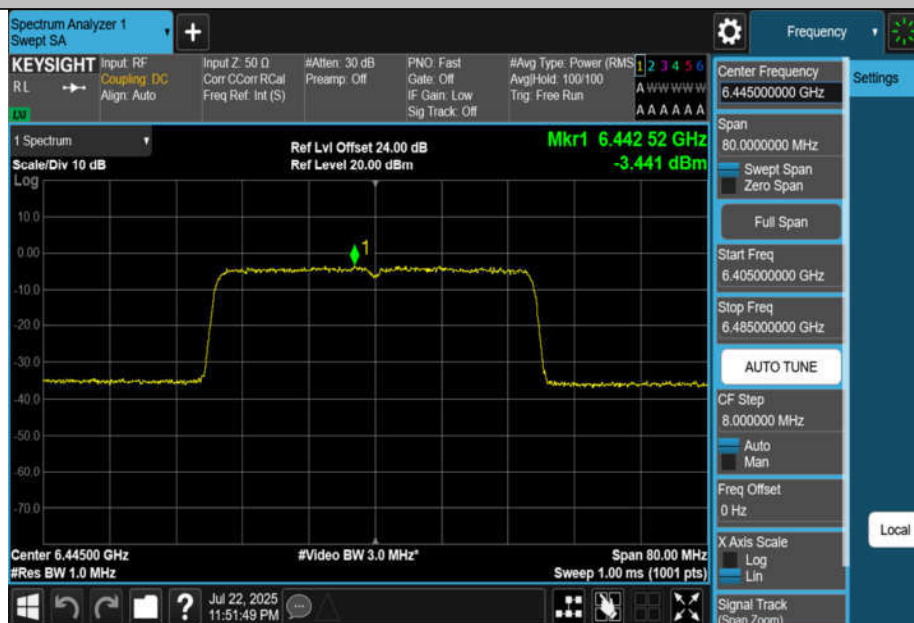
11BE40MIMO-Ant2-6445-PASS
