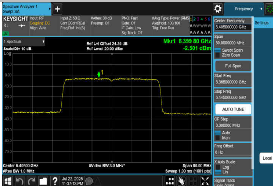
11BE40MIMO-Ant4-6405-PASS
