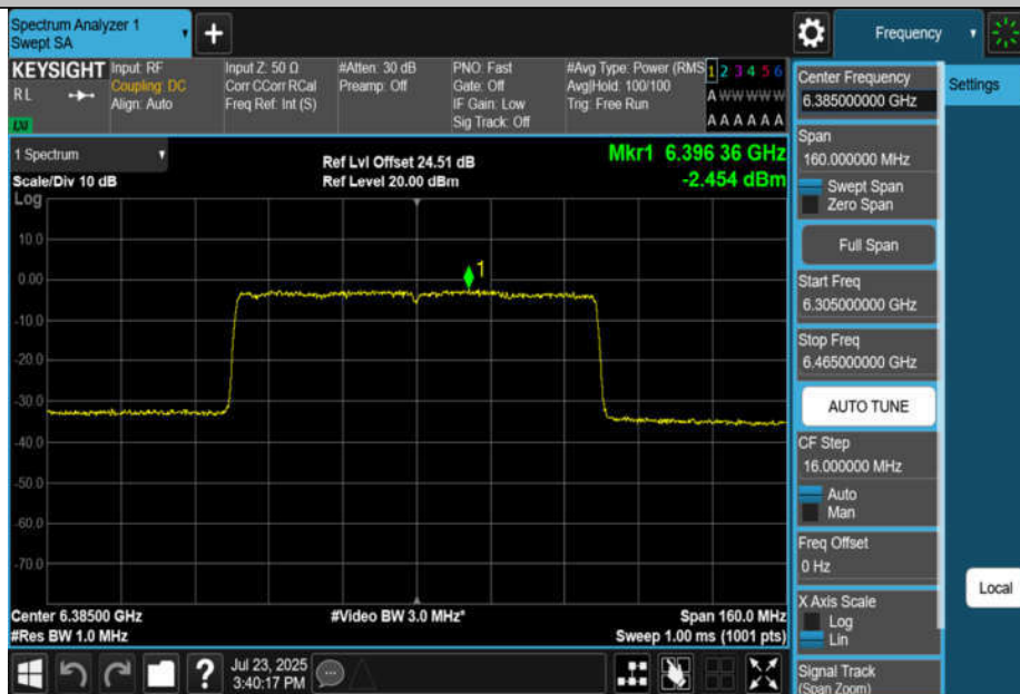
11BE80MIMO-Ant4-6385-PASS
