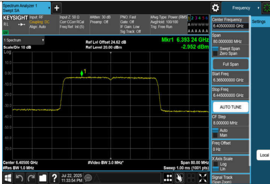
11BE40MIMO-Ant1-6405-PASS
