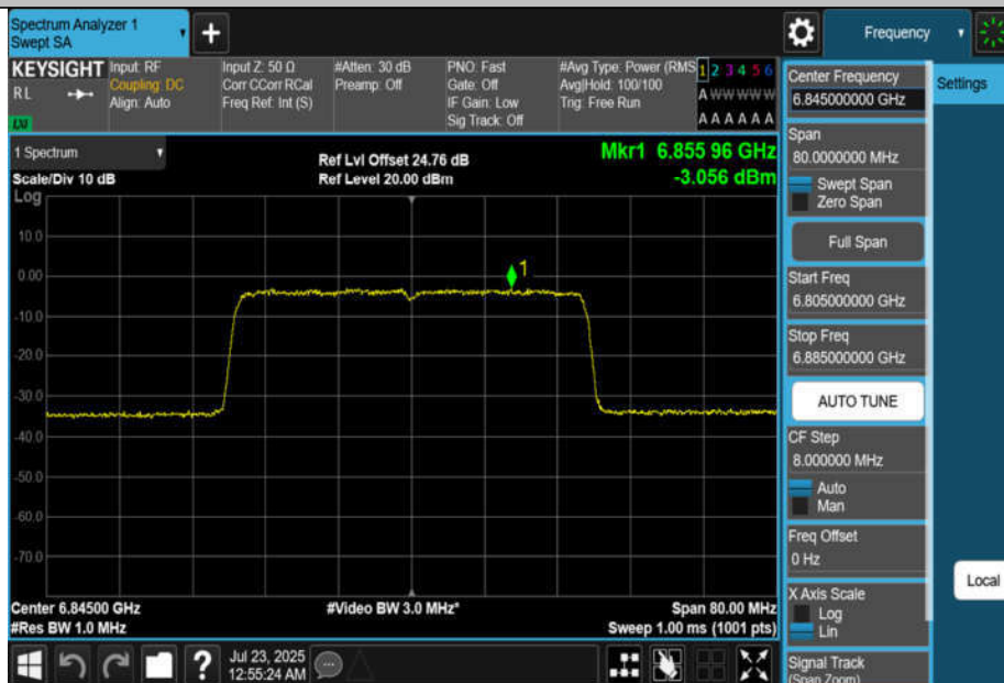
11BE40MIMO-Ant2-6845-PASS
