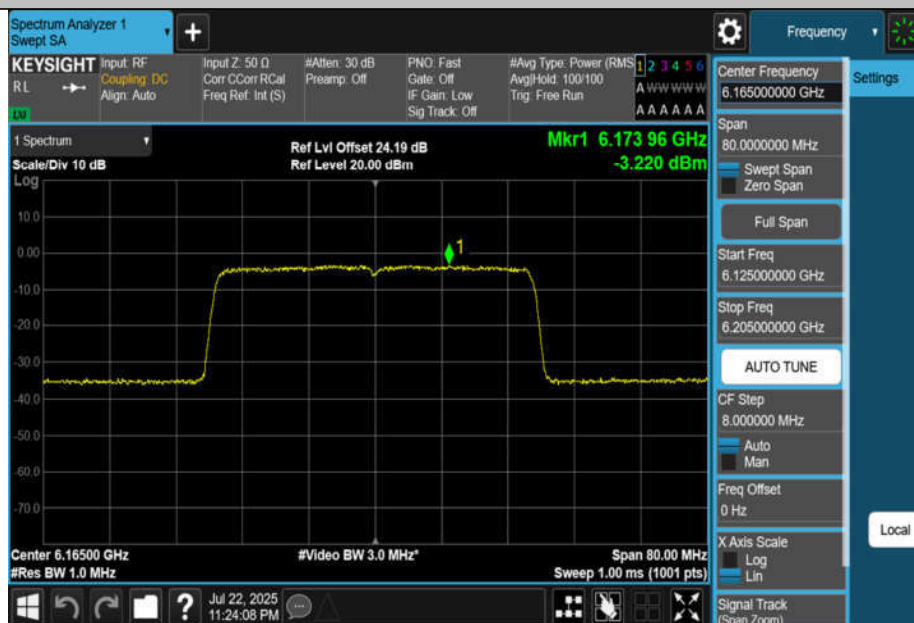
11BE40MIMO-Ant2-6165-PASS
