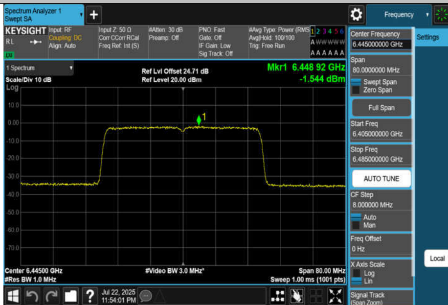
11BE40MIMO-Ant4-6445-PASS
