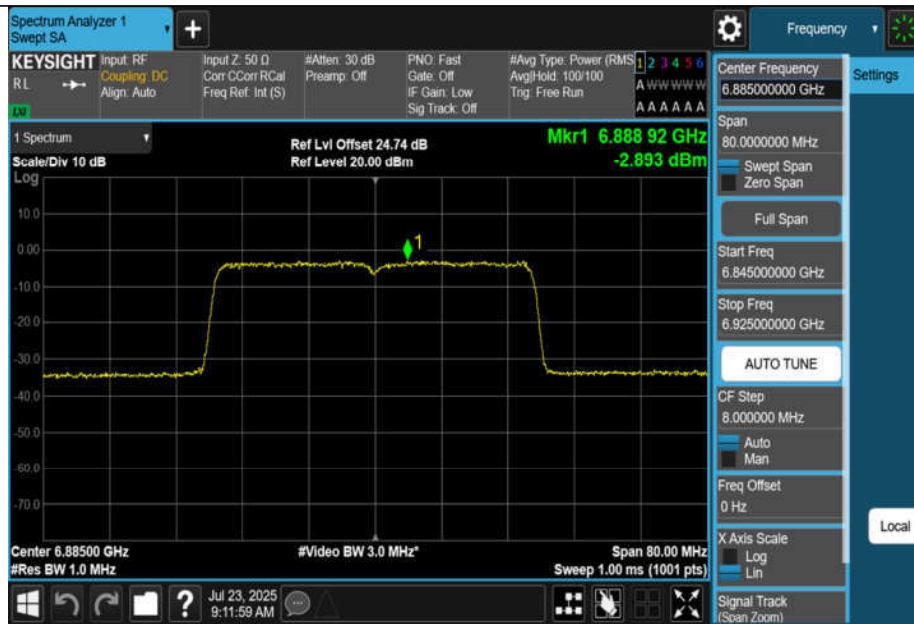
11BE40MIMO-Ant1-6885-PASS
