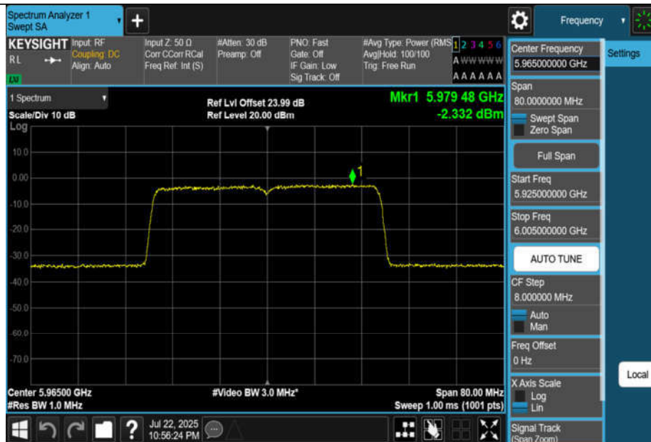
11BE40MIMO-Ant3-5965-PASS
