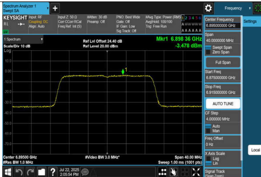
11BE20MIMO-Ant2-6895-PASS
