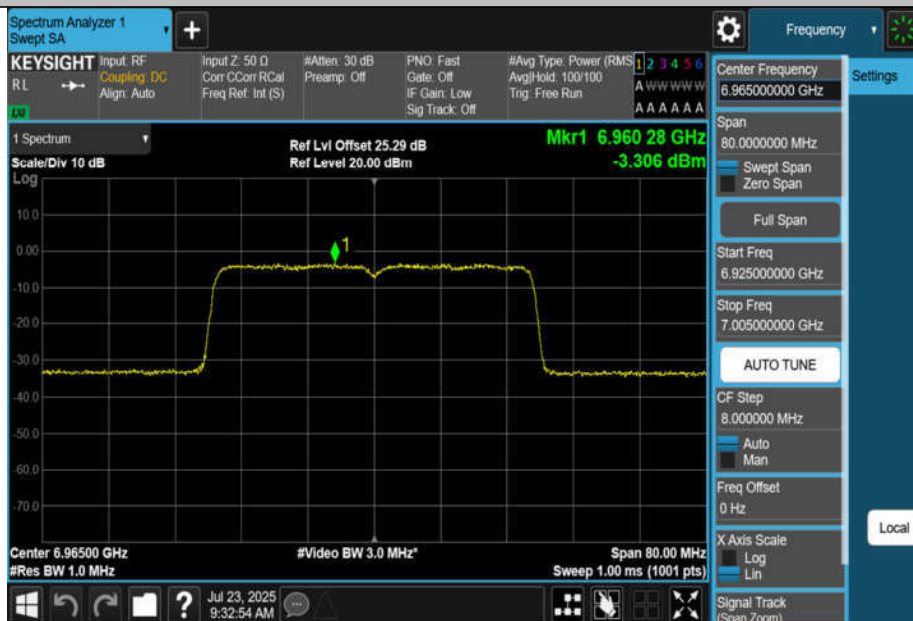
11BE40MIMO-Ant2-6965-PASS
