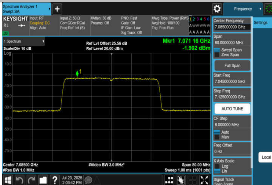
11BE40MIMO-Ant4-7085-PASS
