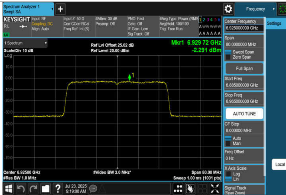
11BE40MIMO-Ant1-6925-PASS
