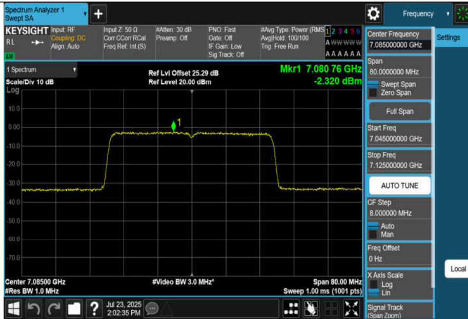
11BE40MIMO-Ant3-7085-PASS
