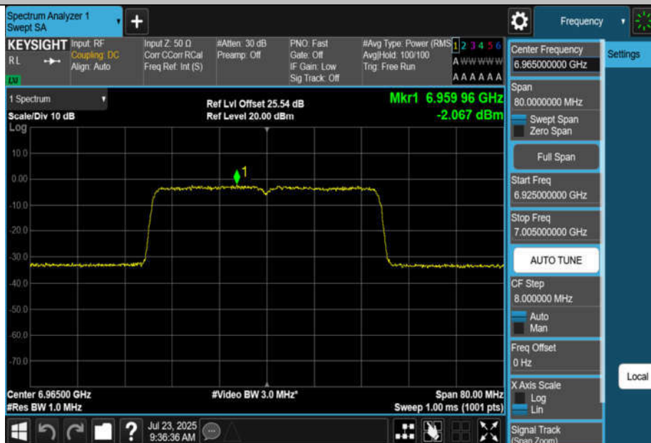
11BE40MIMO-Ant4-6965-PASS
