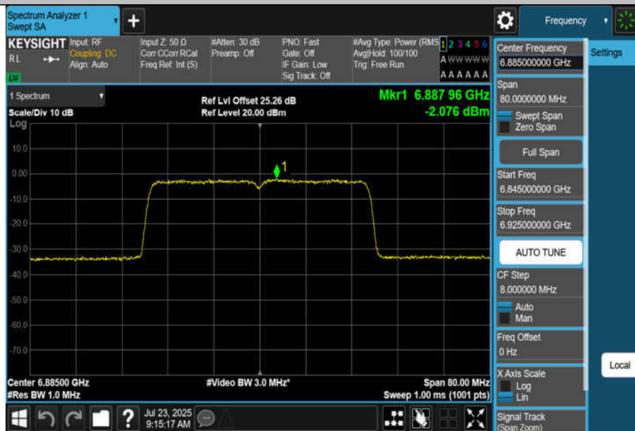
11BE40MIMO-Ant4-6885-PASS
