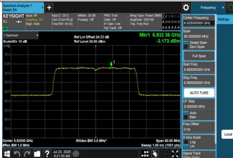
11BE40MIMO-Ant2-6925-PASS
