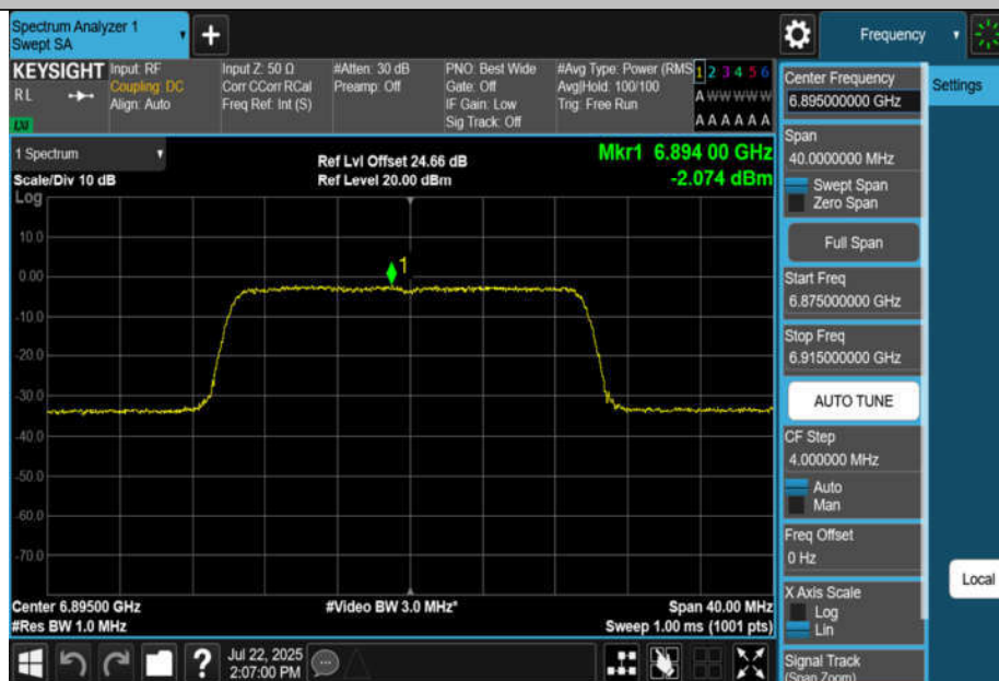
11BE20MIMO-Ant3-6895-PASS
