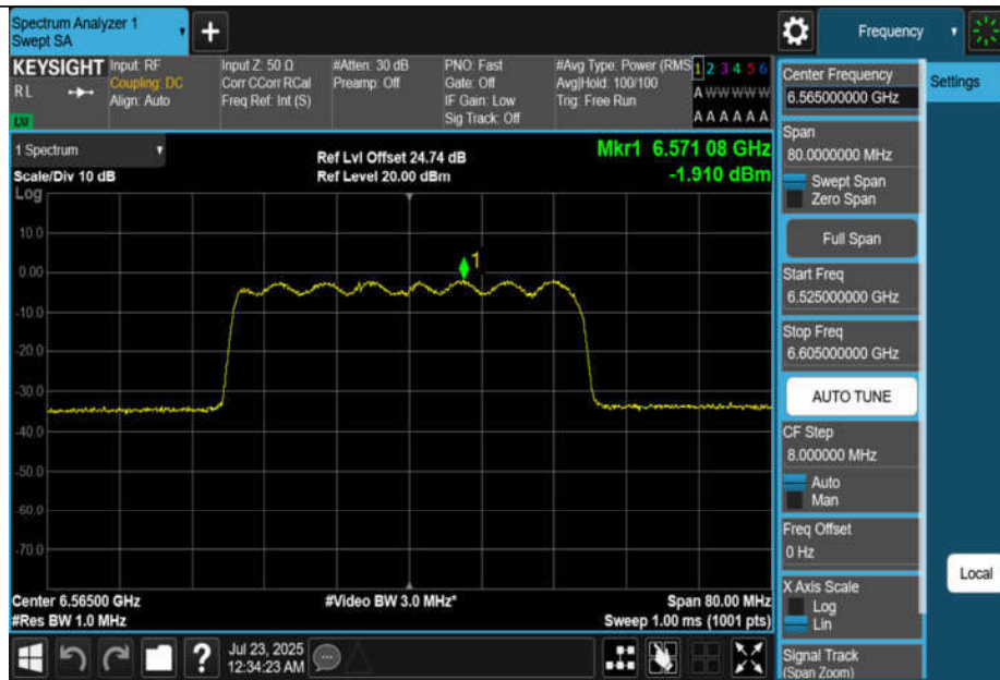
11BE40MIMO-Ant3-6565-PASS
