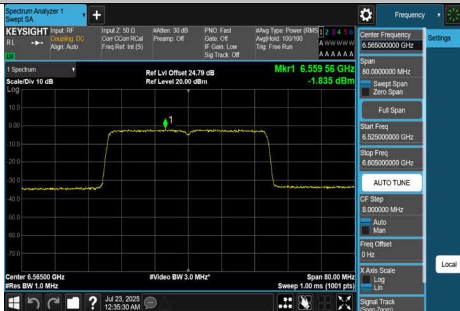
11BE40MIMO-Ant4-6565-PASS
