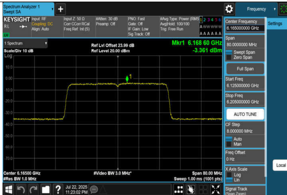
11BE40MIMO-Ant1-6165-PASS
