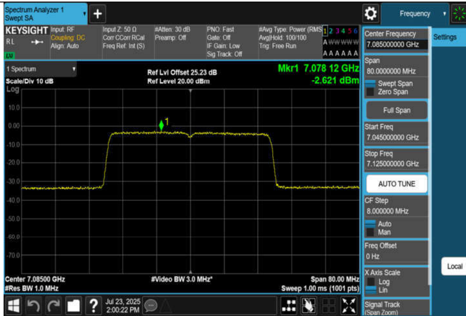
11BE40MIMO-Ant1-7085-PASS
