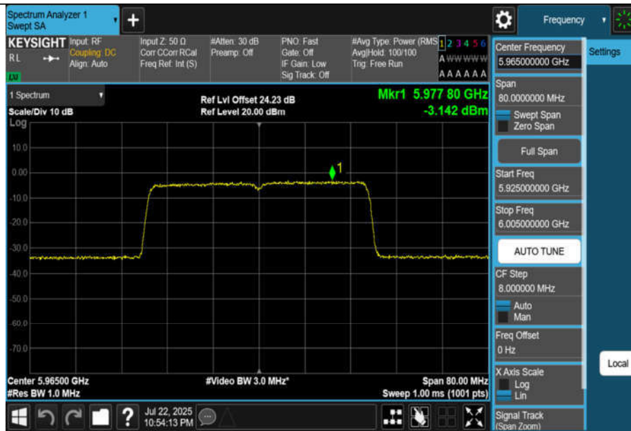
11BE40MIMO-Ant1-5965-PASS
