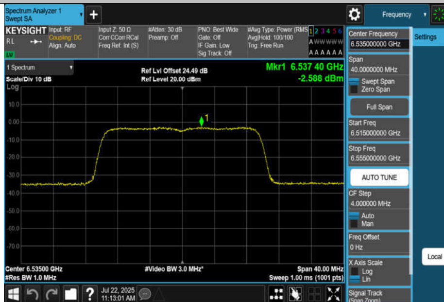
11BE20MIMO-Ant2-6535-PASS
