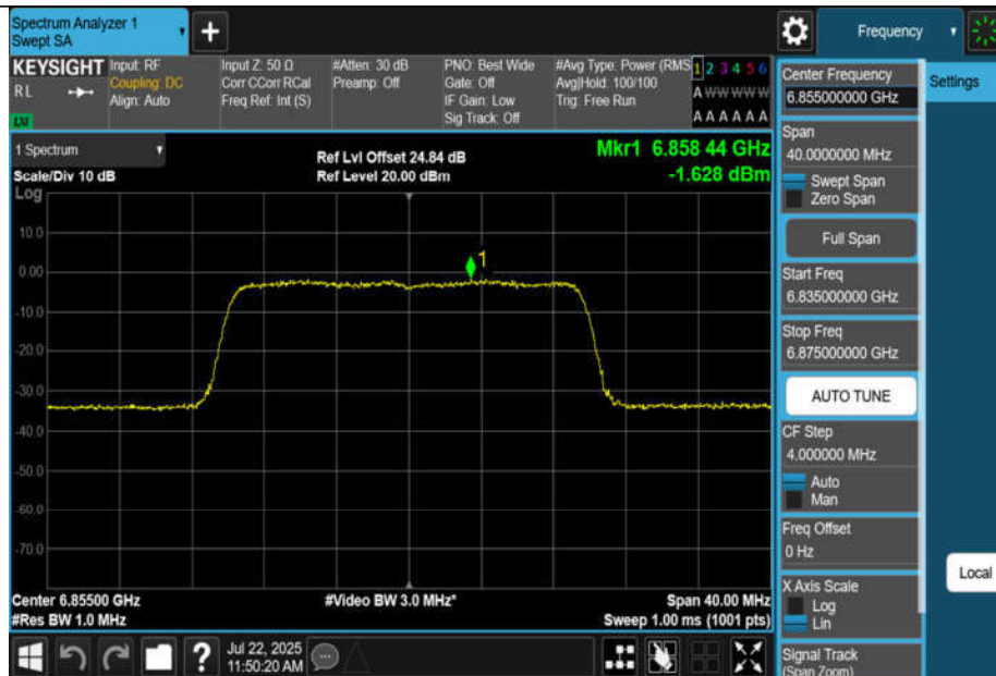
11BE20MIMO-Ant3-6855-PASS
