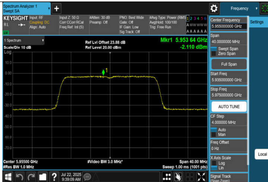
11BE20MIMO-Ant3-5955-PASS
