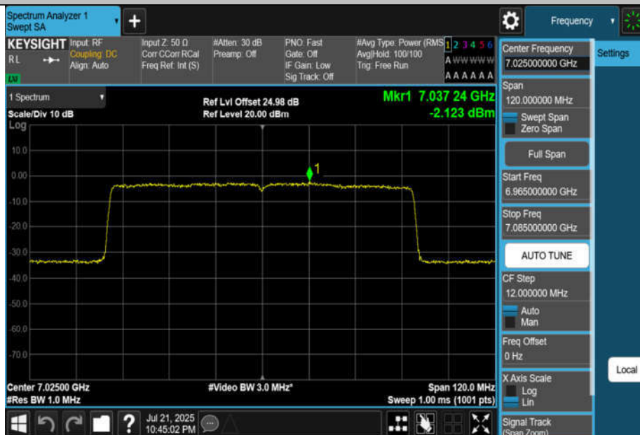
11AX80MIMO-Ant4-7025-PASS
