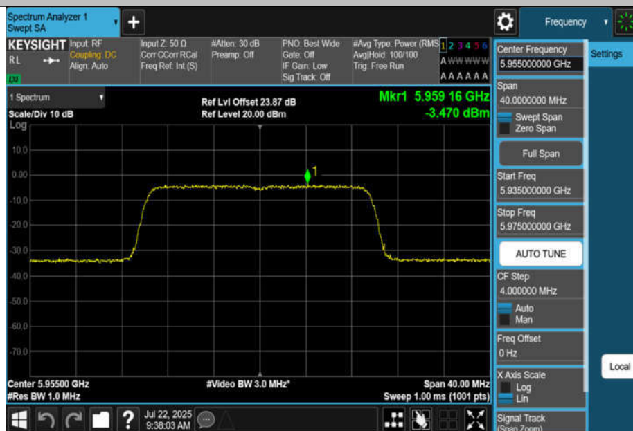
11BE20MIMO-Ant2-5955-PASS
