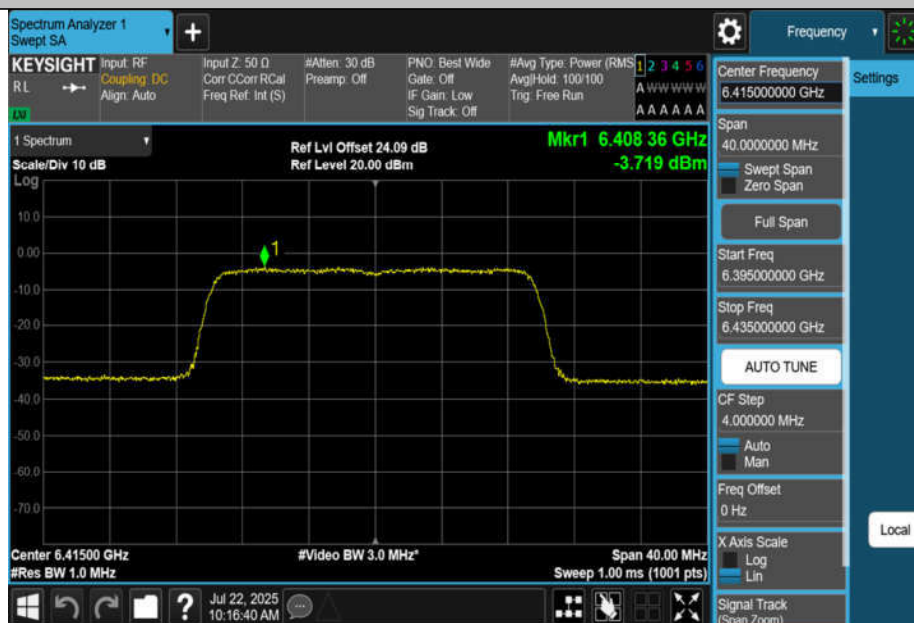
11BE20MIMO-Ant2-6415-PASS
