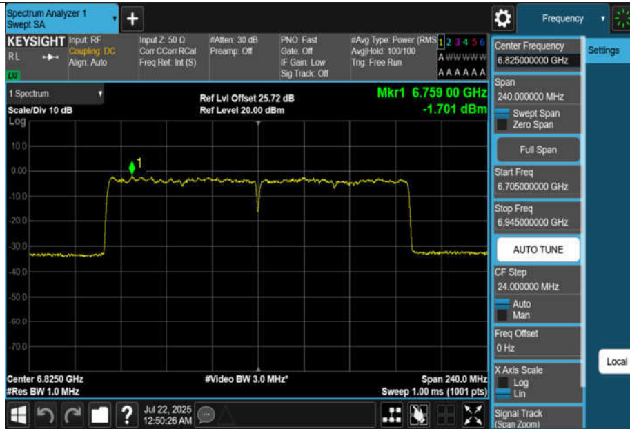
11AX160MIMO-Ant3-6825-PASS
