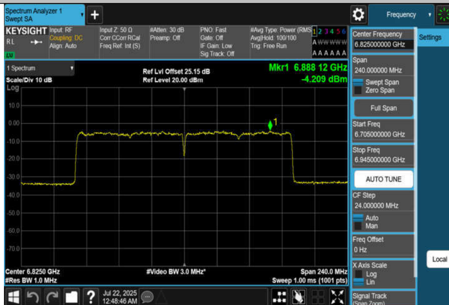
11AX160MIMO-Ant2-6825-PASS
