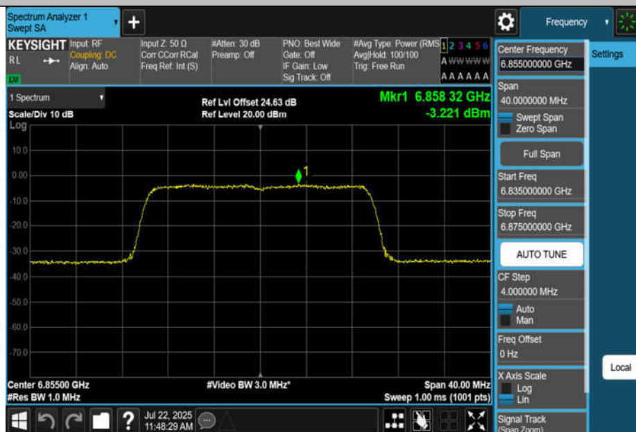
11BE20MIMO-Ant2-6855-PASS
