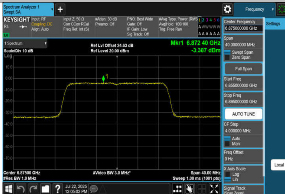
11BE20MIMO-Ant2-6875-PASS
