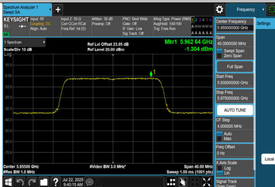
11BE20MIMO-Ant4-5955-PASS
