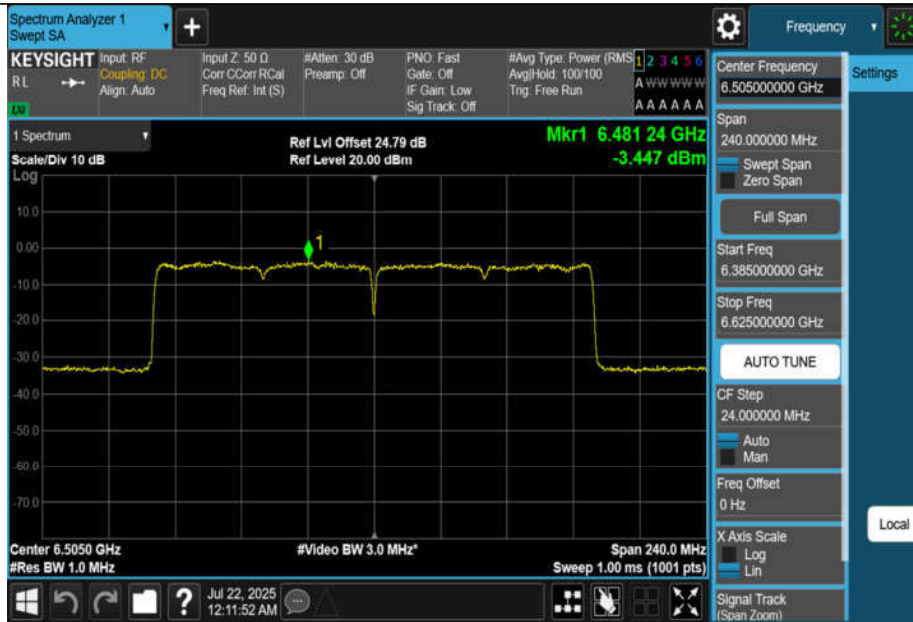
11AX160MIMO-Ant1-6505-PASS
