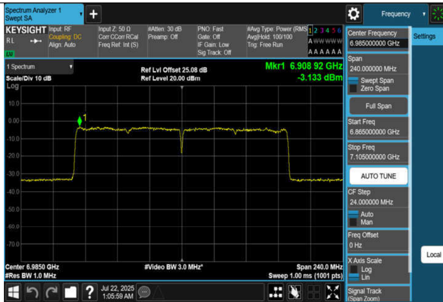
11AX160MIMO-Ant1-6985-PASS
