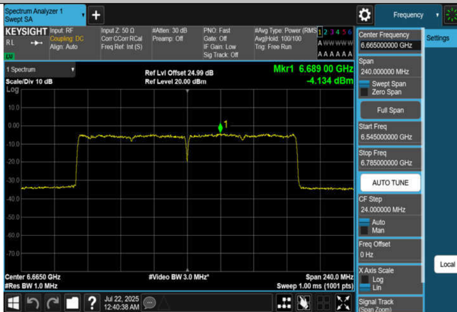
11AX160MIMO-Ant4-6665-PASS
