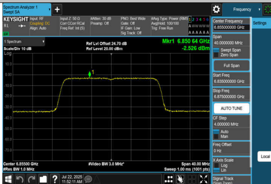
11BE20MIMO-Ant4-6855-PASS
