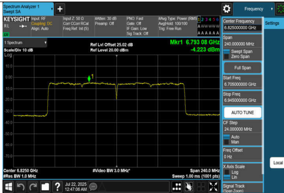
11AX160MIMO-Ant1-6825-PASS
