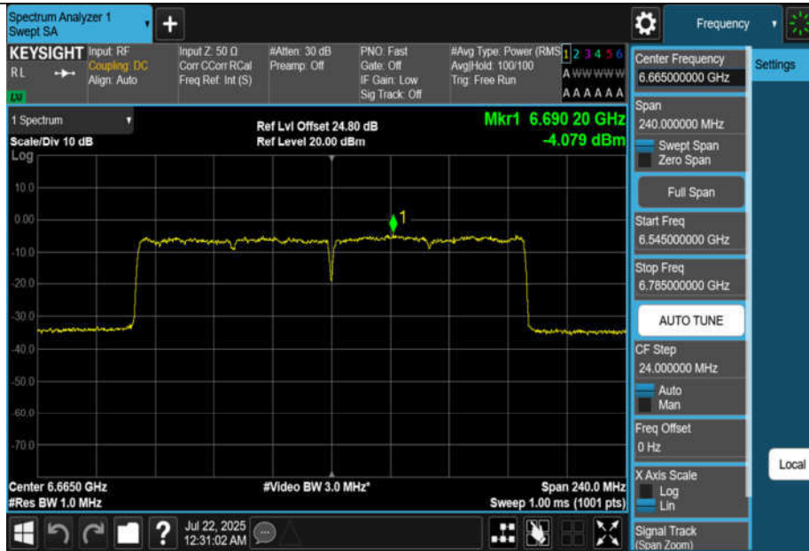
11AX160MIMO-Ant1-6665-PASS
