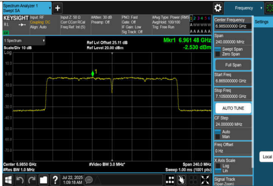
11AX160MIMO-Ant3-6985-PASS
