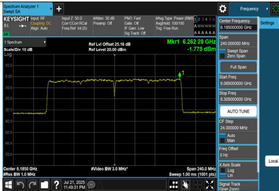
11AX160MIMO-Ant3-6185-PASS
