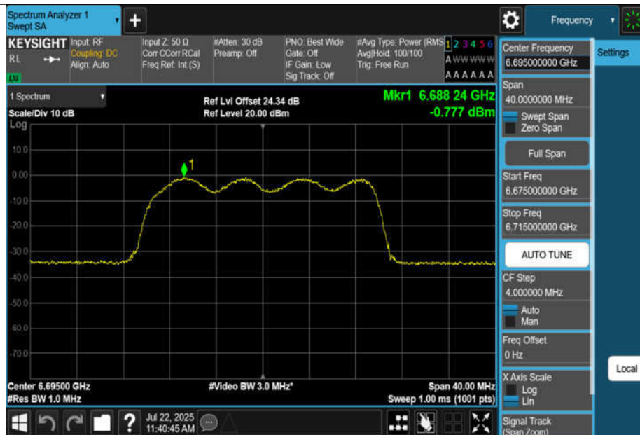
11BE20MIMO-Ant3-6695-PASS
