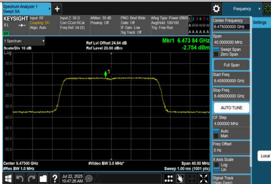
11BE20MIMO-Ant4-6475-PASS
