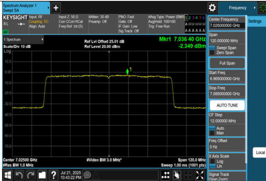
11AX80MIMO-Ant3-7025-PASS
