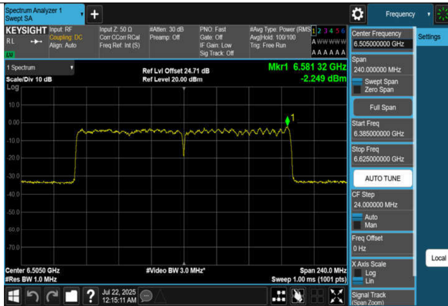
11AX160MIMO-Ant3-6505-PASS
