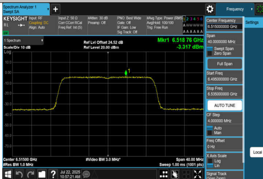
11BE20MIMO-Ant4-6515-PASS
