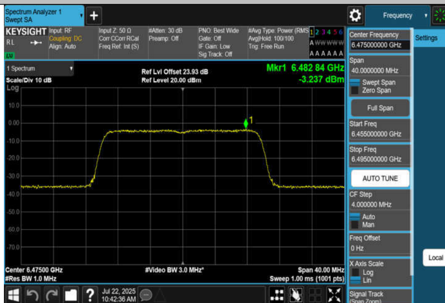
11BE20MIMO-Ant2-6475-PASS
