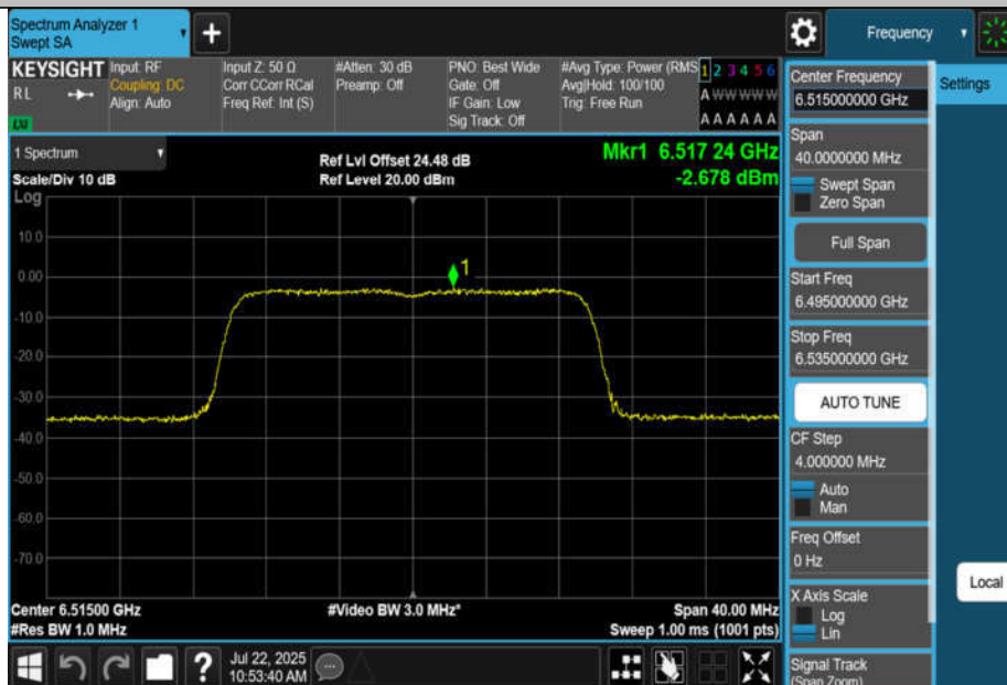
11BE20MIMO-Ant2-6515-PASS
