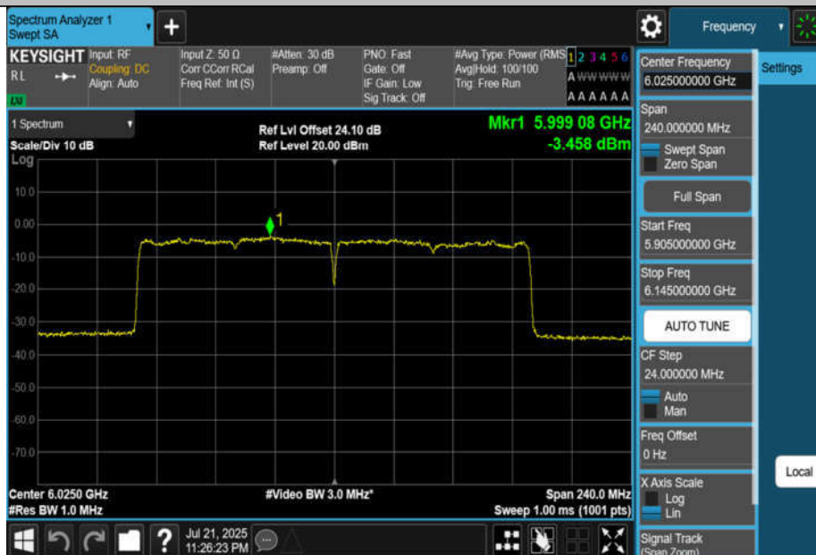
11AX160MIMO-Ant2-6025-PASS
