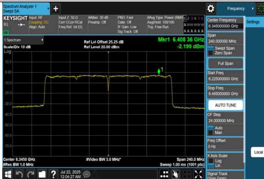
11AX160MIMO-Ant4-6345-PASS
