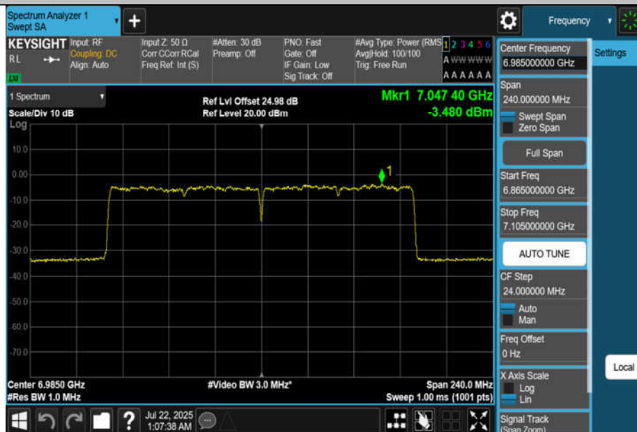
11AX160MIMO-Ant2-6985-PASS
