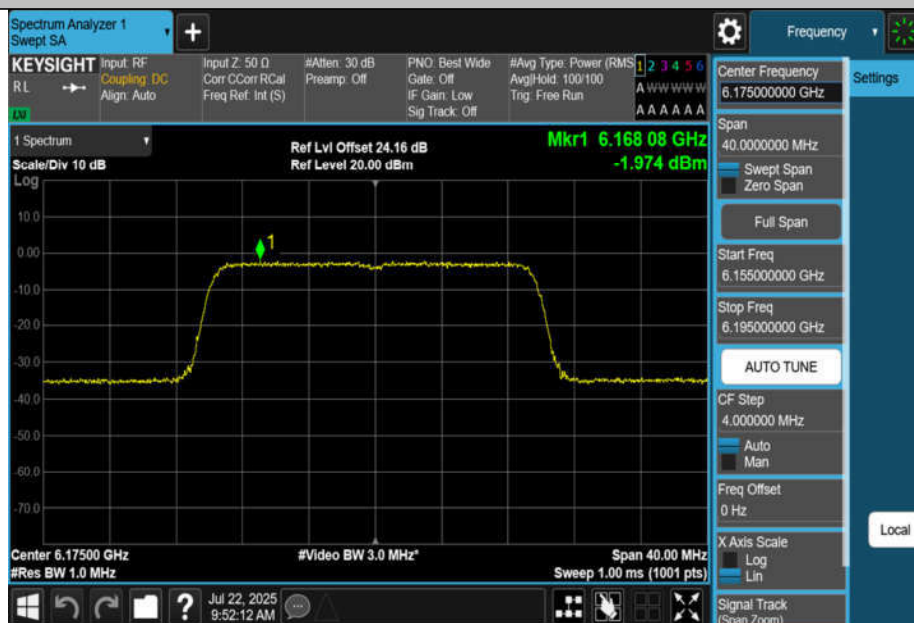
11BE20MIMO-Ant4-6175-PASS
