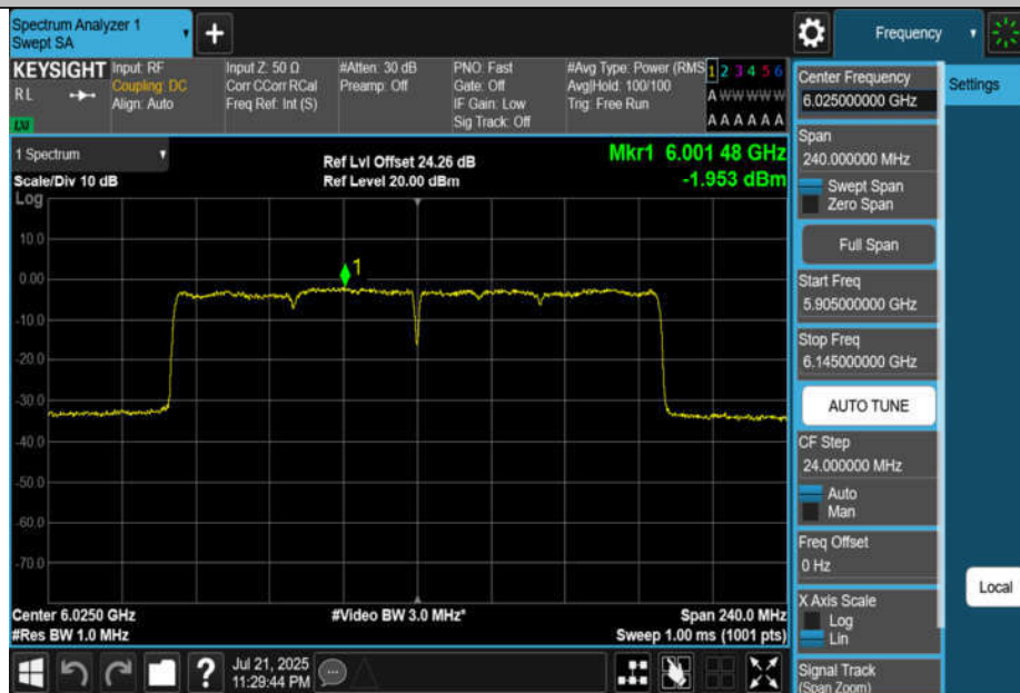
11AX160MIMO-Ant4-6025-PASS
