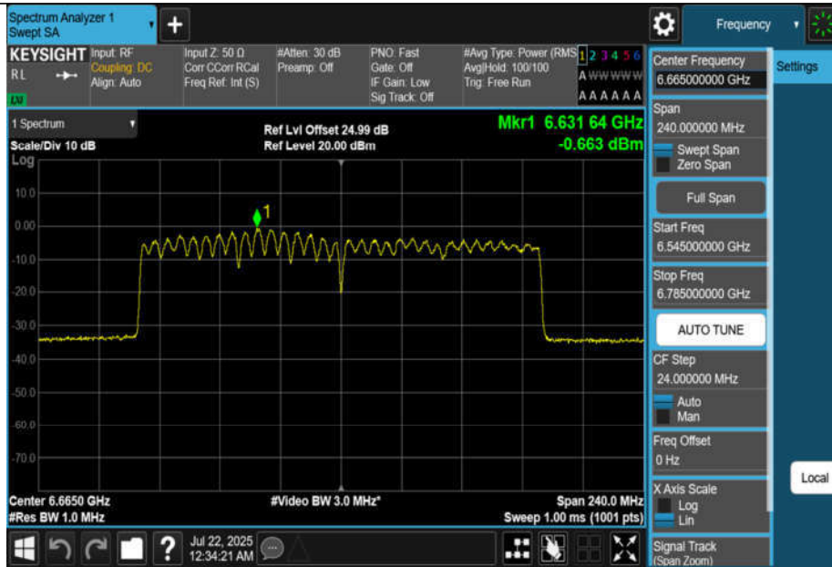
11AX160MIMO-Ant3-6665-PASS
