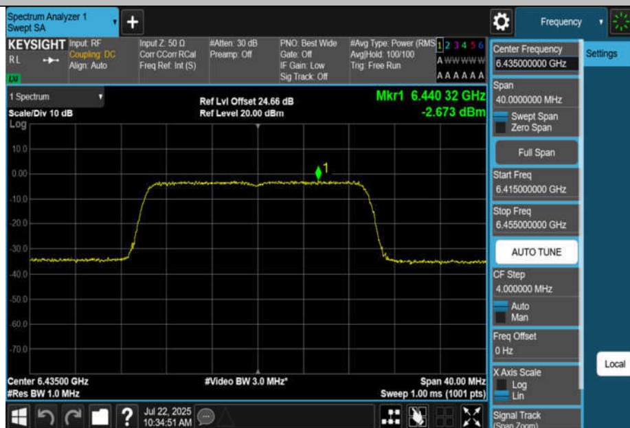
11BE20MIMO-Ant4-6435-PASS
