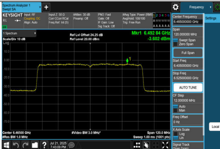
11AX80MIMO-Ant2-6465-PASS
