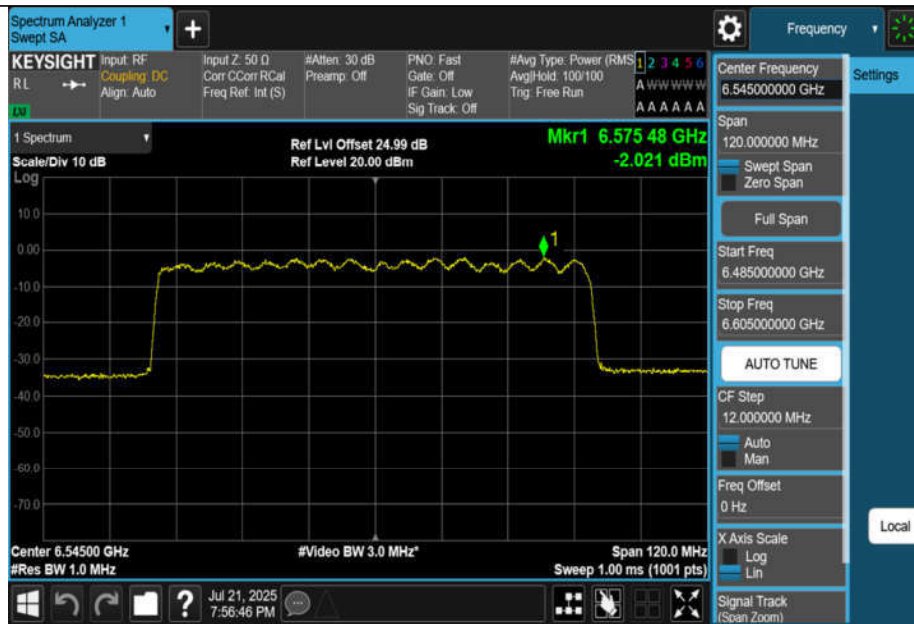
11AX80MIMO-Ant3-6545-PASS
