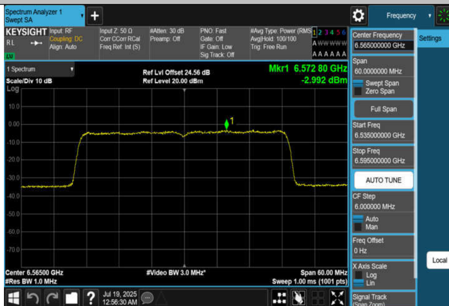
11AX40MIMO-Ant2-6565-PASS
