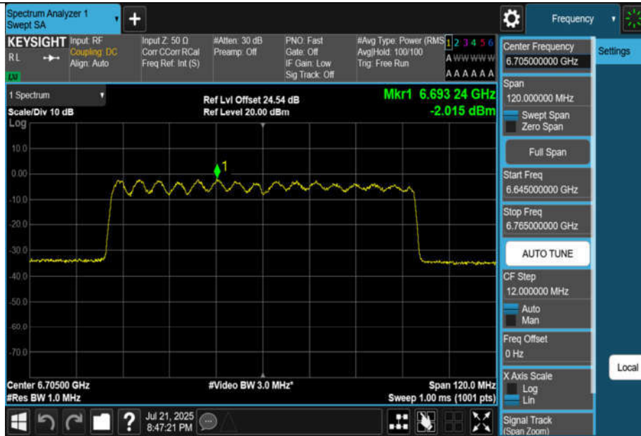
11AX80MIMO-Ant3-6705-PASS
