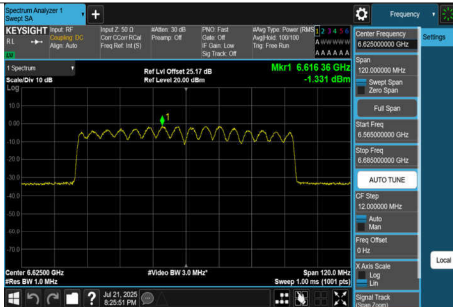
11AX80MIMO-Ant3-6625-PASS
