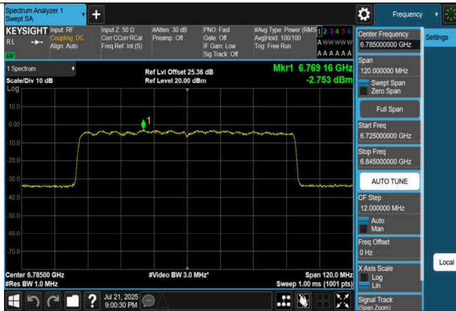
11AX80MIMO-Ant3-6785-PASS
