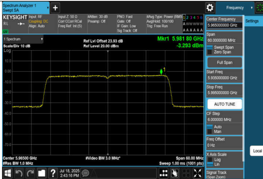
11AX40MIMO-Ant3-5965-PASS
