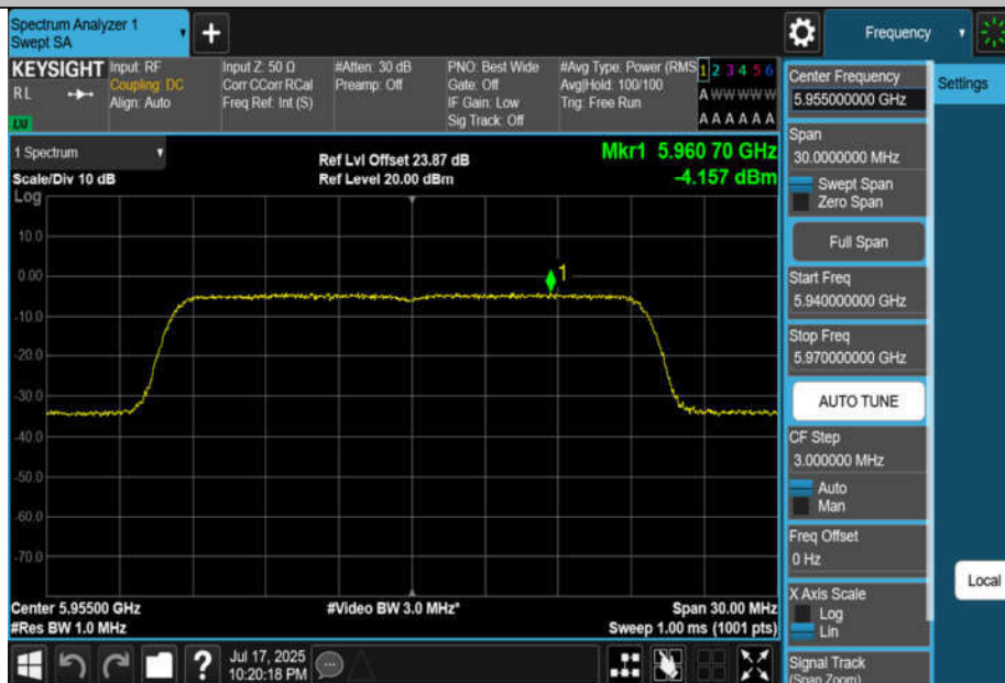
11AX20MIMO-Ant2-5955-PASS
