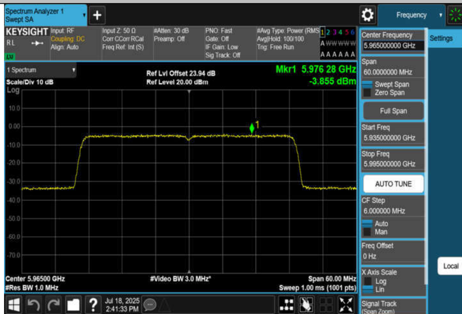
11AX40MIMO-Ant2-5965-PASS
