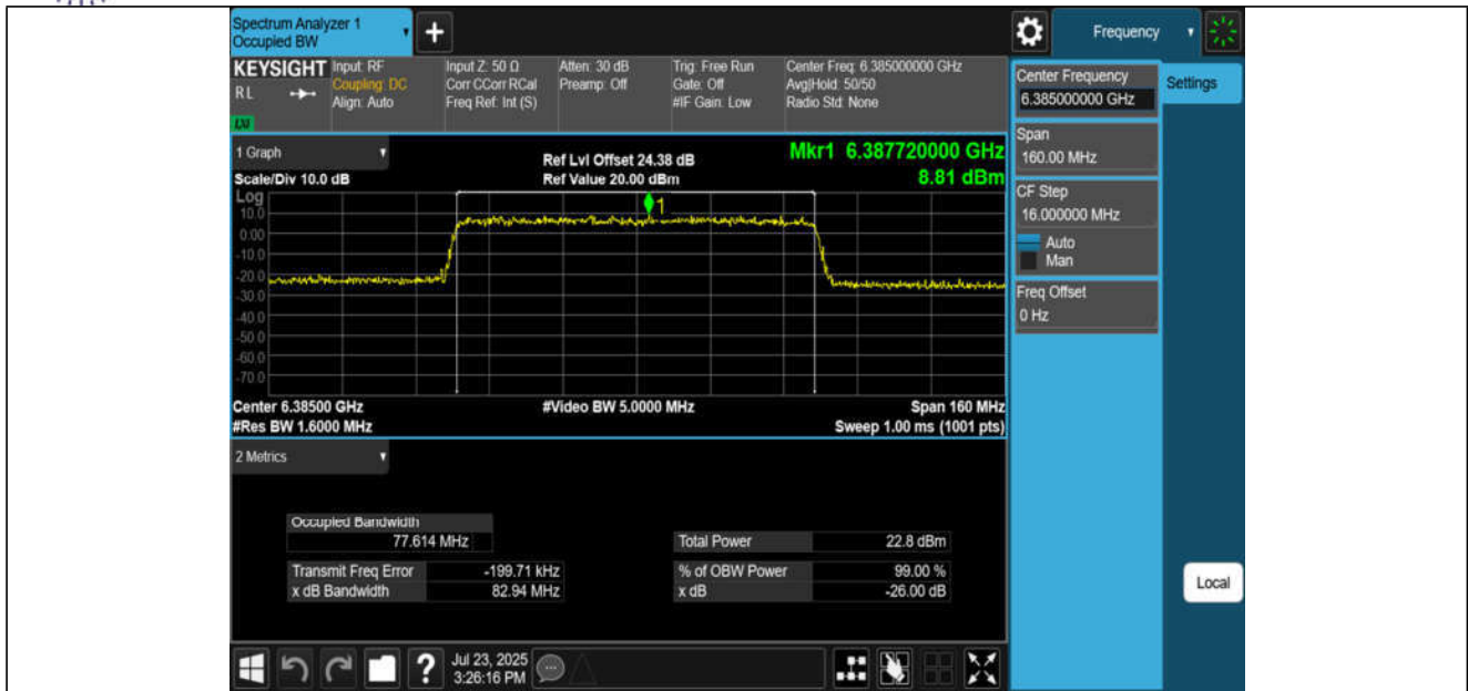
11BE80MIMO-Ant3-6385-PASS
