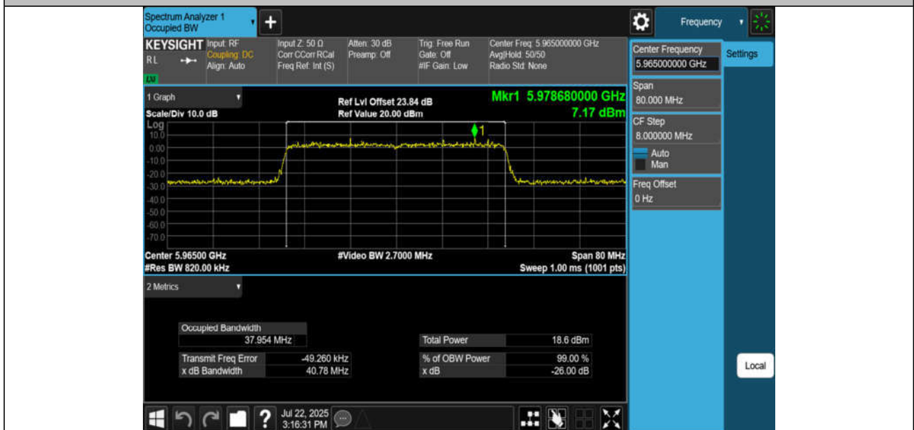
11BE40MIMO-Ant4-5965-PASS
