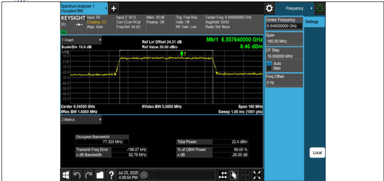
11BE80MIMO-Ant1-6545-PASS
