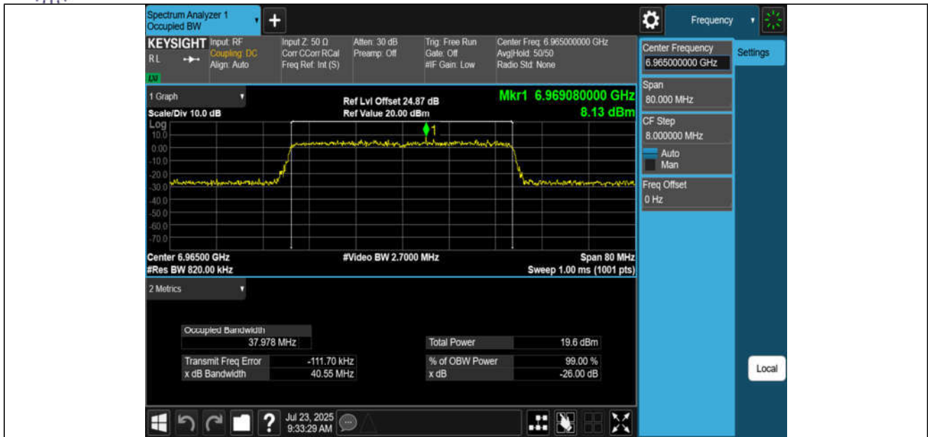
11BE40MIMO-Ant3-6965-PASS
