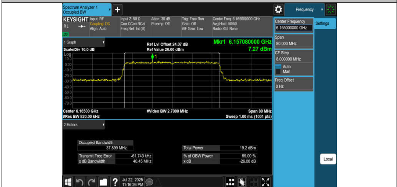
11BE40MIMO-Ant4-6165-PASS
