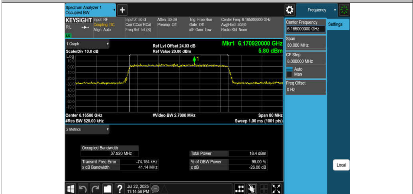
11BE40MIMO-Ant2-6165-PASS
