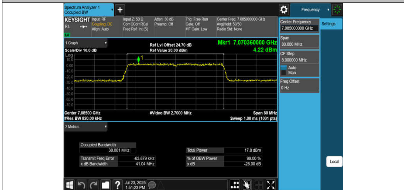
11BE40MIMO-Ant2-7085-PASS
