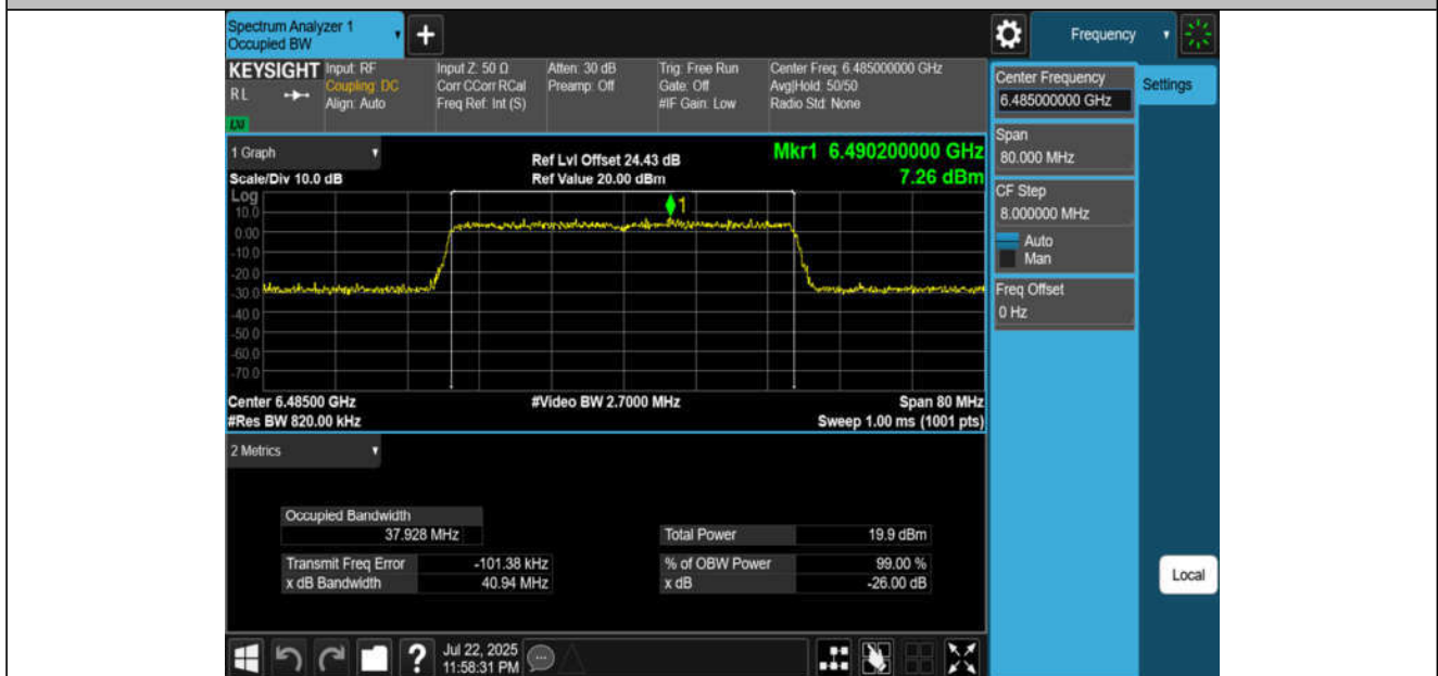
11BE40MIMO-Ant4-6485-PASS
