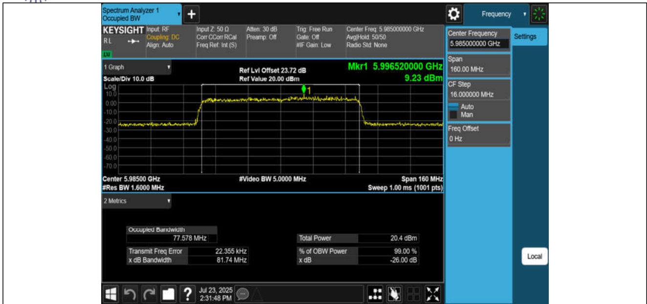
11BE80MIMO-Ant3-5985-PASS
