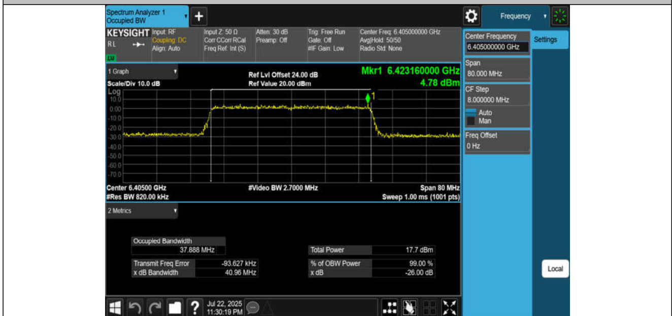
11BE40MIMO-Ant2-6405-PASS
