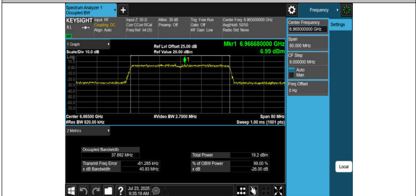
11BE40MIMO-Ant4-6965-PASS
