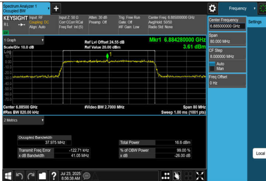
11BE40MIMO-Ant3-6885-PASS
