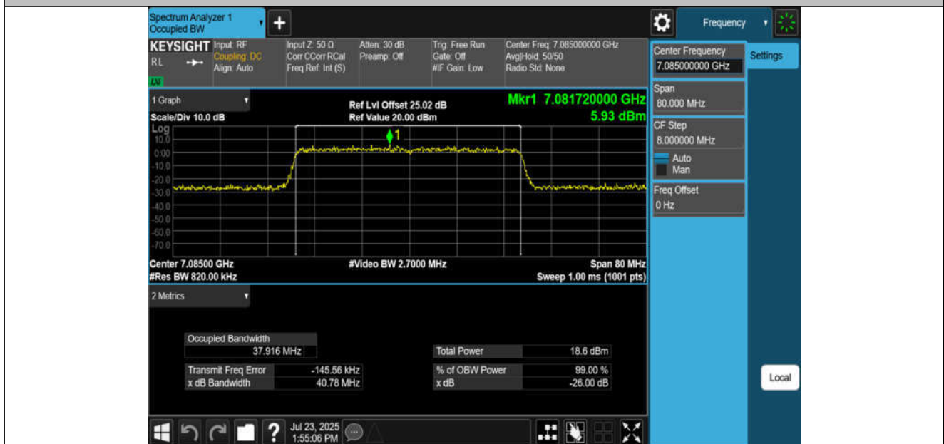
11BE40MIMO-Ant4-7085-PASS
