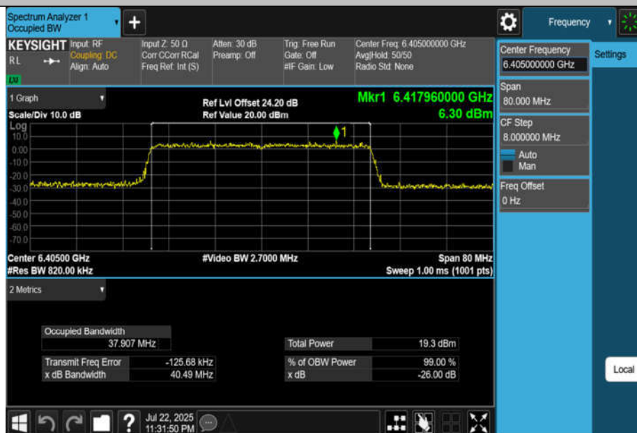
11BE40MIMO-Ant4-6405-PASS
