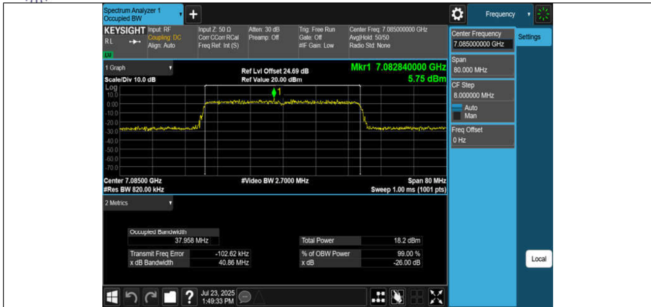
11BE40MIMO-Ant1-7085-PASS
