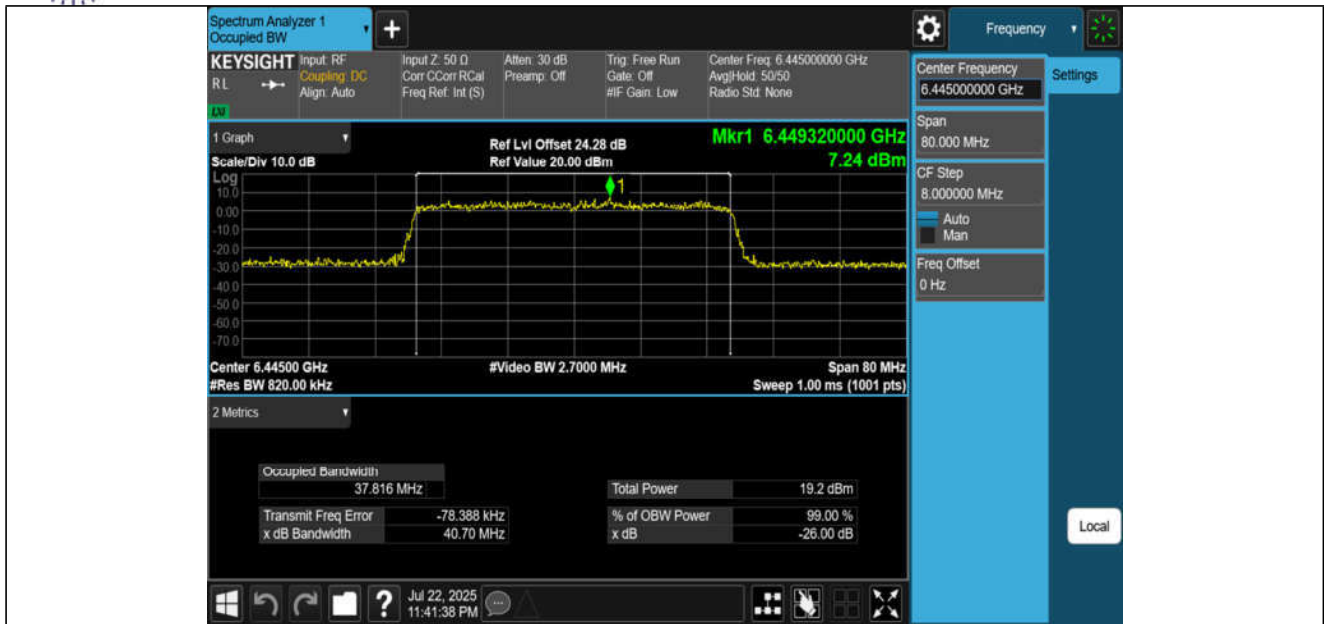
11BE40MIMO-Ant3-6445-PASS
