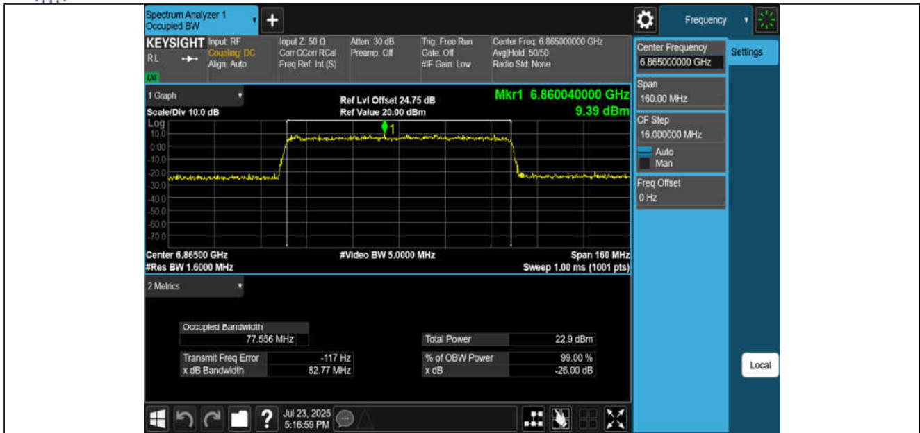
11BE80MIMO-Ant3-6865-PASS
