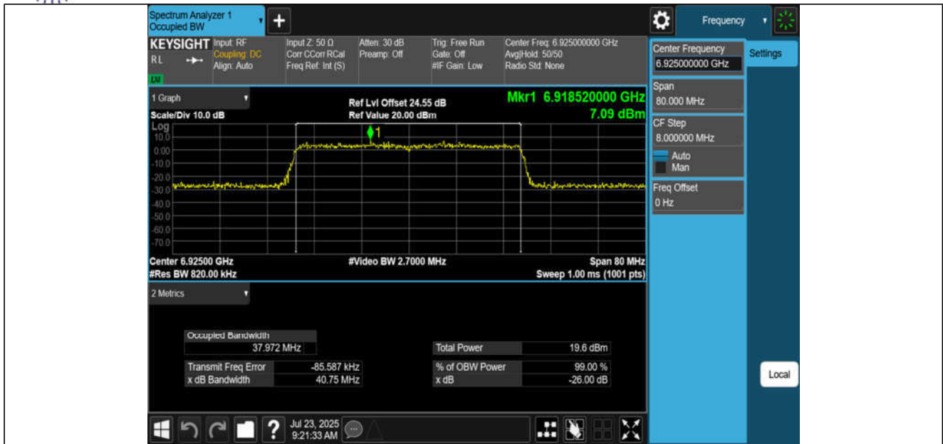
11BE40MIMO-Ant3-6925-PASS
