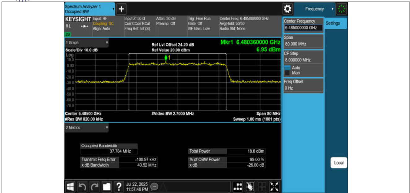
11BE40MIMO-Ant3-6485-PASS
