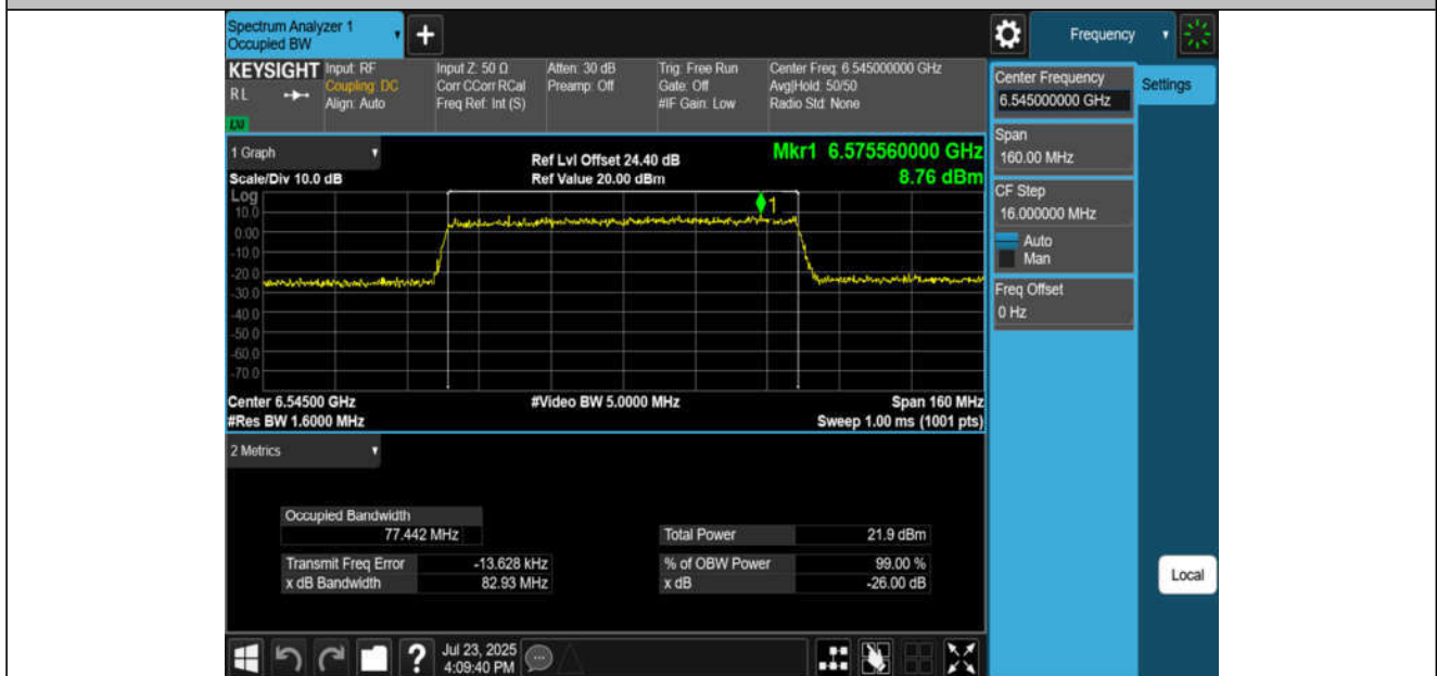
11BE80MIMO-Ant2-6545-PASS
