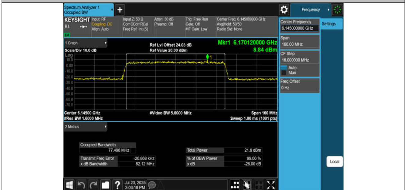
11BE80MIMO-Ant2-6145-PASS
