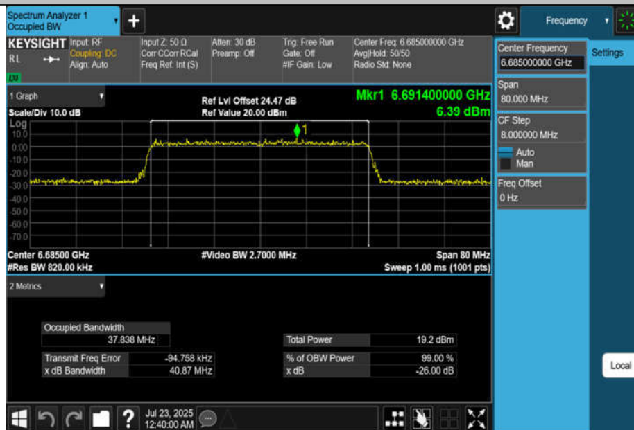
11BE40MIMO-Ant4-6685-PASS
