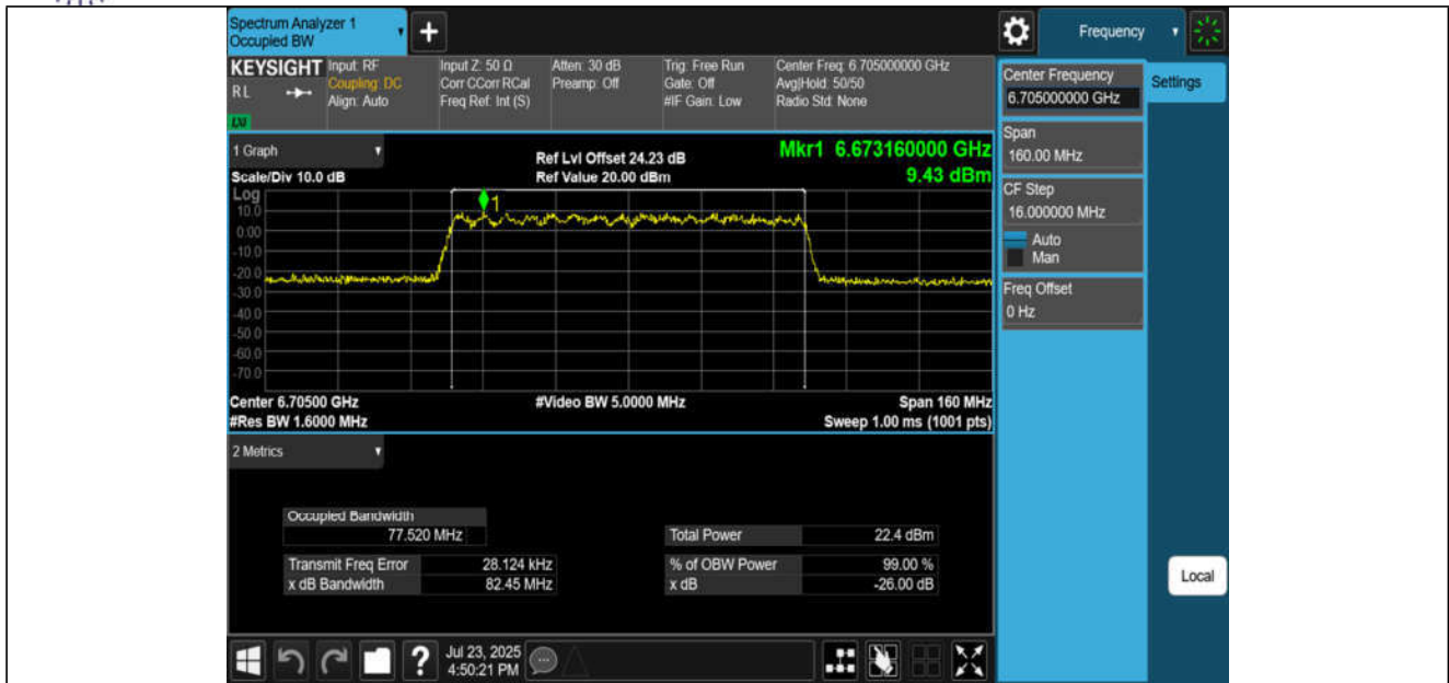
11BE80MIMO-Ant3-6705-PASS
