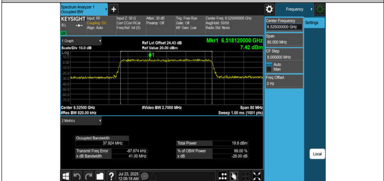
11BE40MIMO-Ant4-6525-PASS
