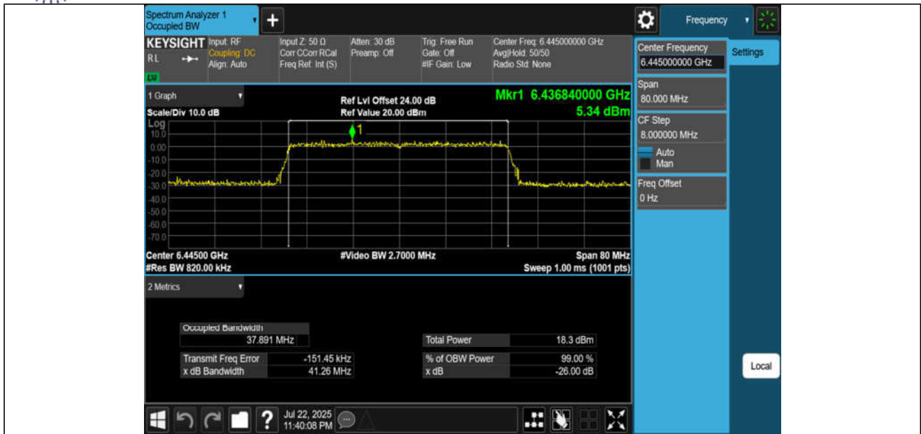
11BE40MIMO-Ant1-6445-PASS
