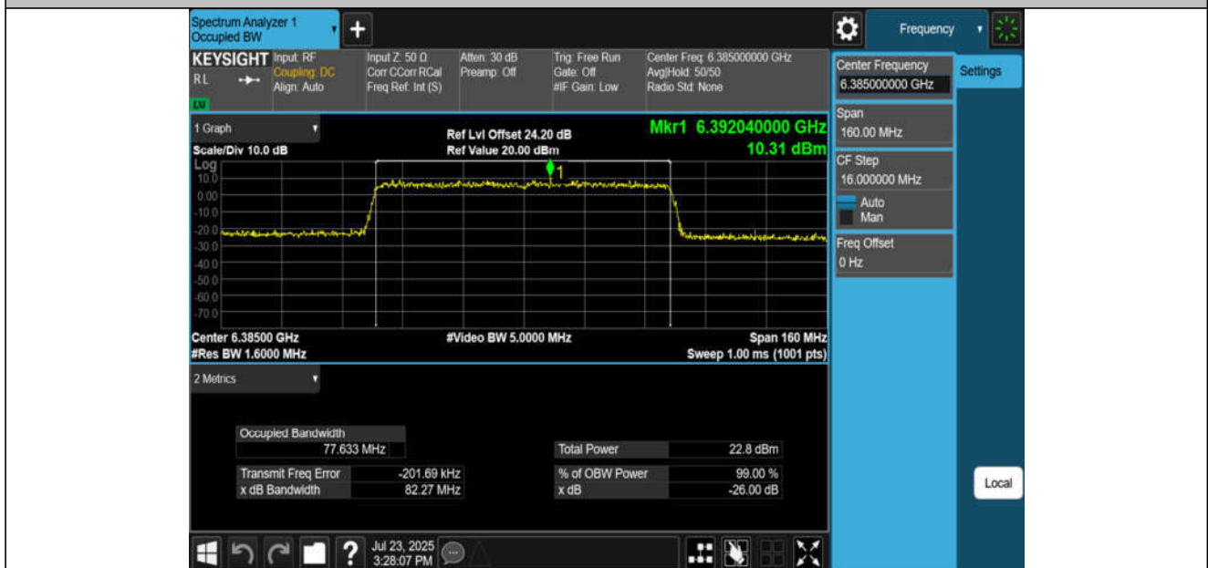
11BE80MIMO-Ant4-6385-PASS
