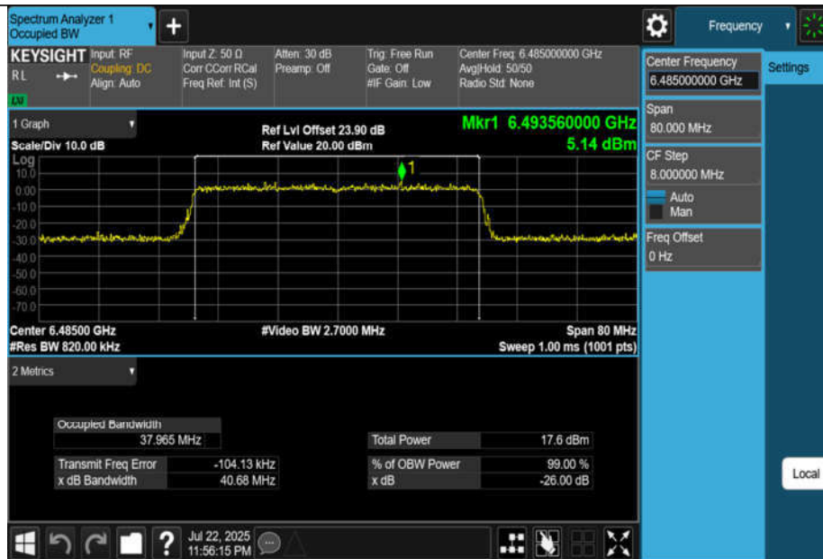
11BE40MIMO-Ant1-6485-PASS
