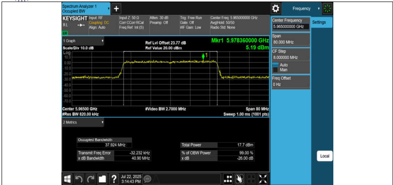
11BE40MIMO-Ant3-5965-PASS
