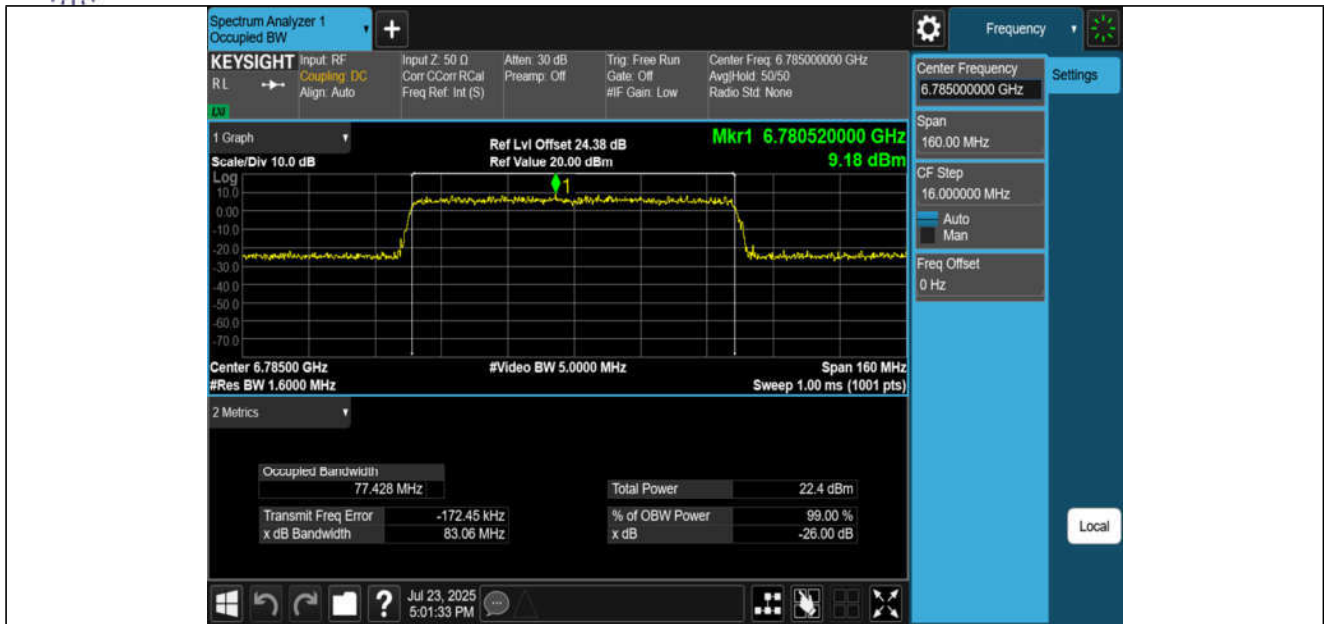
11BE80MIMO-Ant1-6785-PASS
