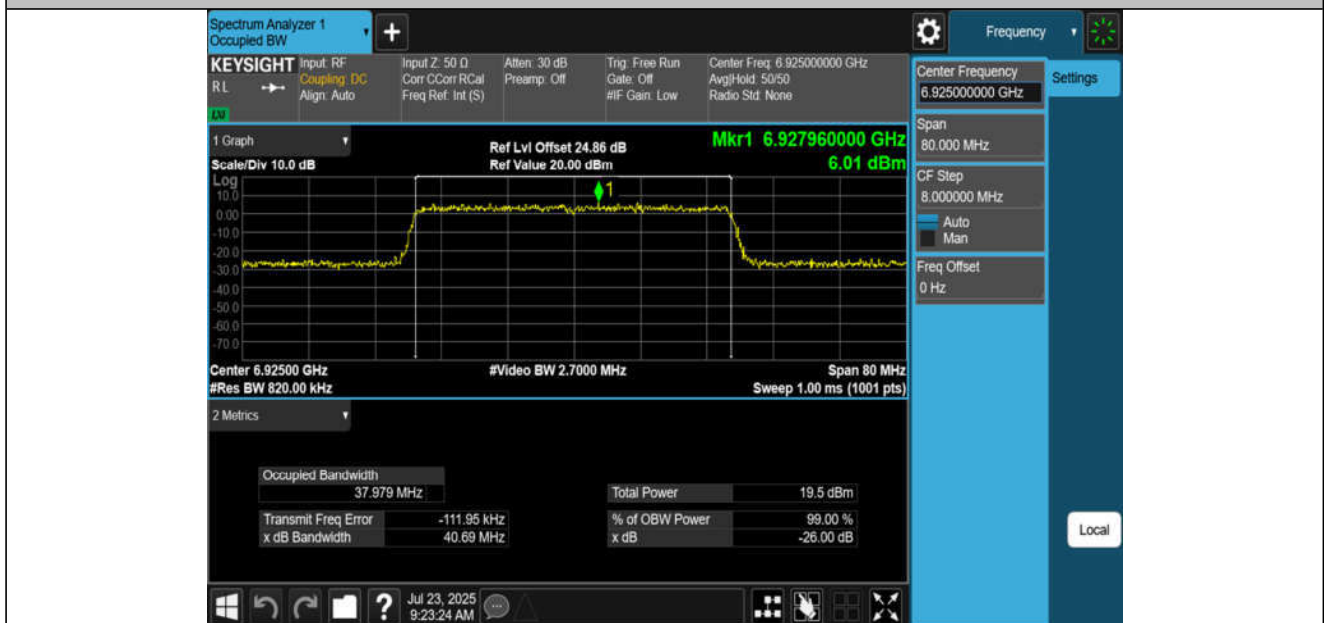
11BE40MIMO-Ant4-6925-PASS
