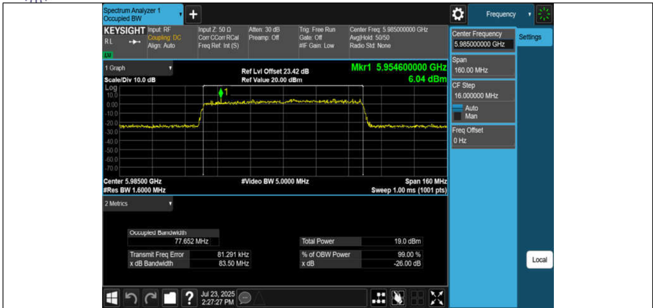
11BE80MIMO-Ant1-5985-PASS
