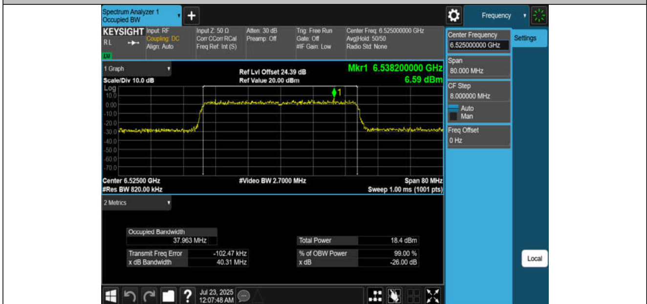
11BE40MIMO-Ant2-6525-PASS
