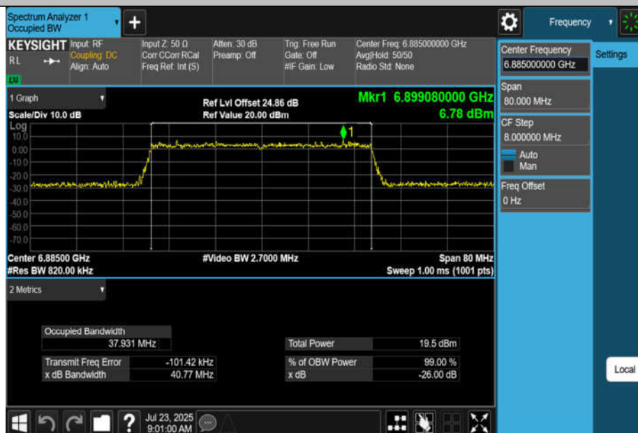
11BE40MIMO-Ant4-6885-PASS
