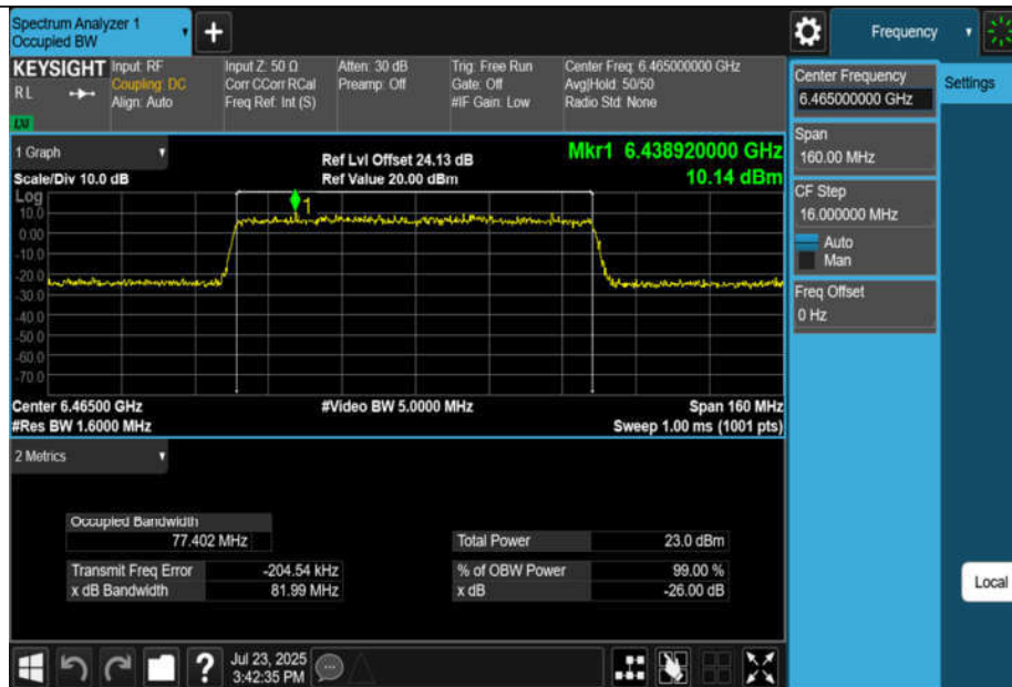
11BE80MIMO-Ant1-6465-PASS
