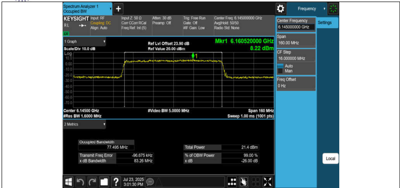
11BE80MIMO-Ant1-6145-PASS
