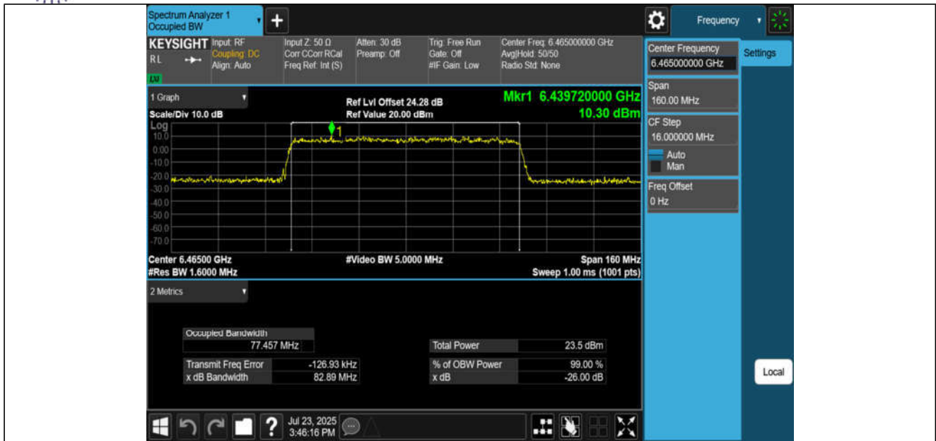
11BE80MIMO-Ant3-6465-PASS
