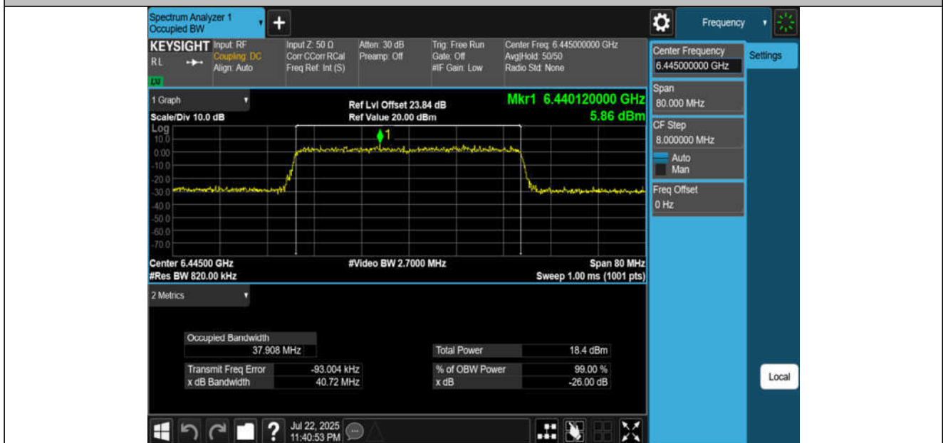
11BE40MIMO-Ant2-6445-PASS
