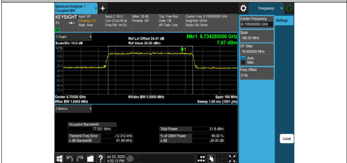
11BE80MIMO-Ant4-6705-PASS
