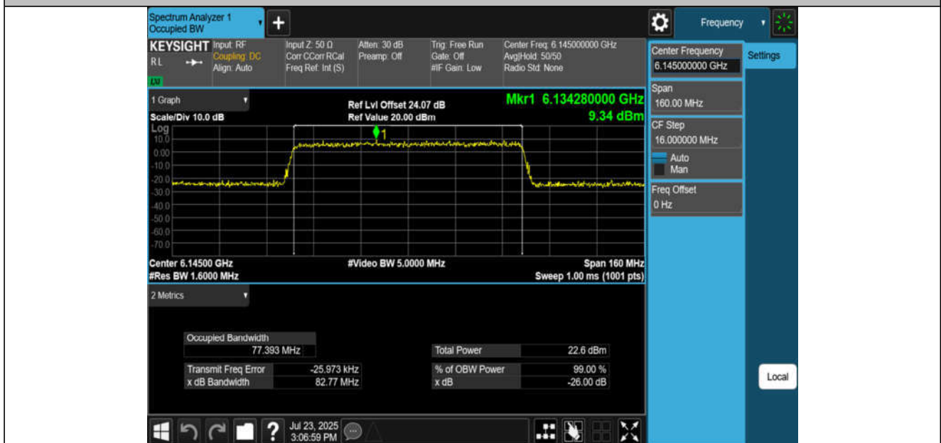
11BE80MIMO-Ant4-6145-PASS
