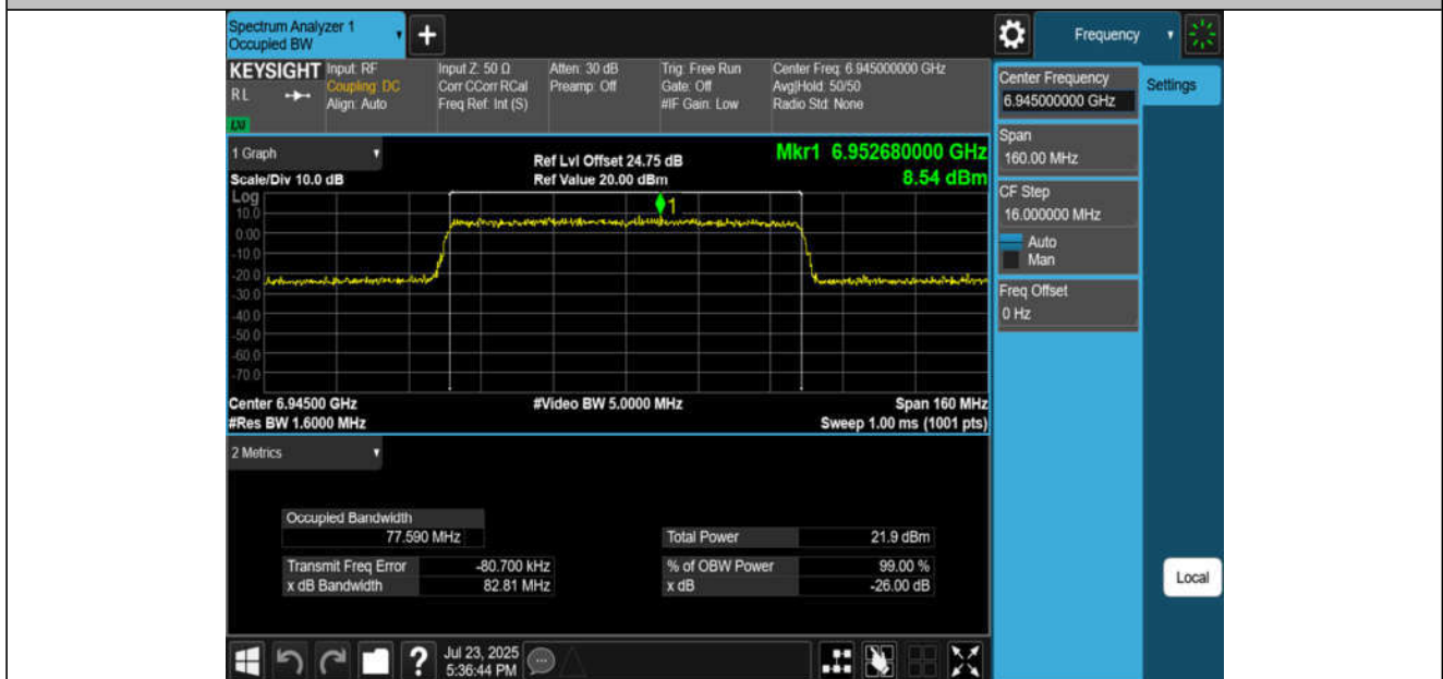
11BE80MIMO-Ant2-6945-PASS
