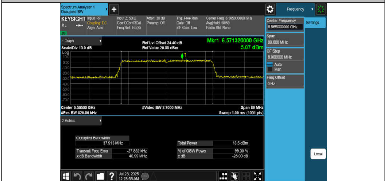
11BE40MIMO-Ant2-6565-PASS
