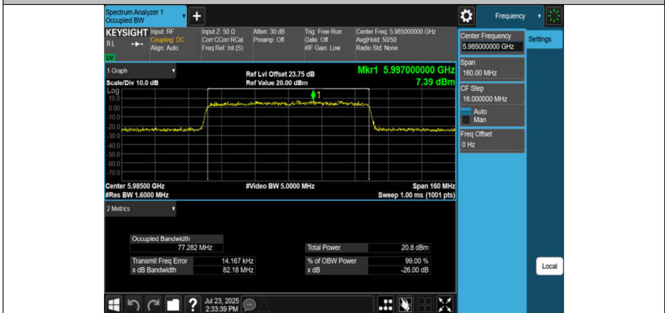
11BE80MIMO-Ant4-5985-PASS
