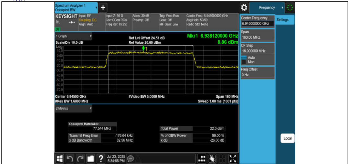
11BE80MIMO-Ant1-6945-PASS
