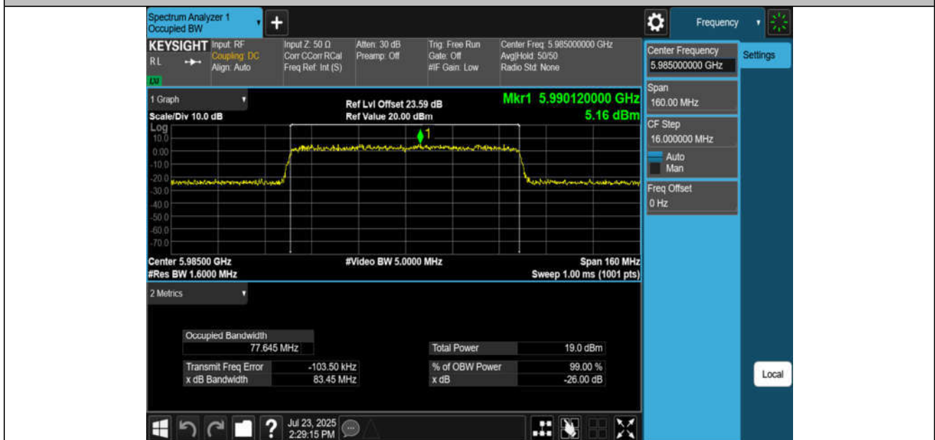
11BE80MIMO-Ant2-5985-PASS
