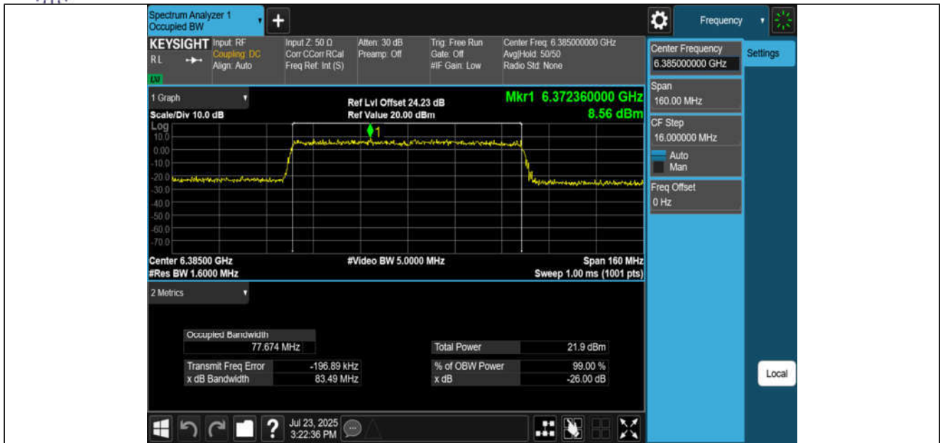
11BE80MIMO-Ant1-6385-PASS
