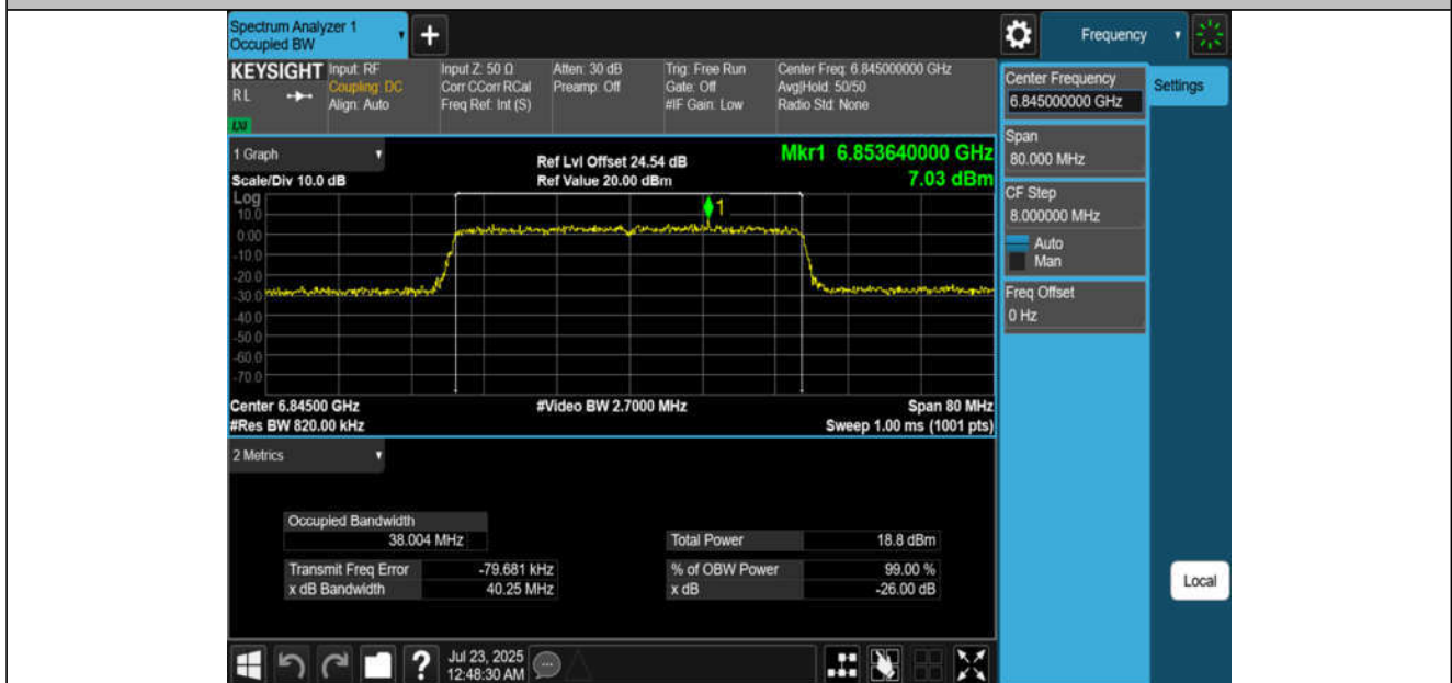
11BE40MIMO-Ant2-6845-PASS
