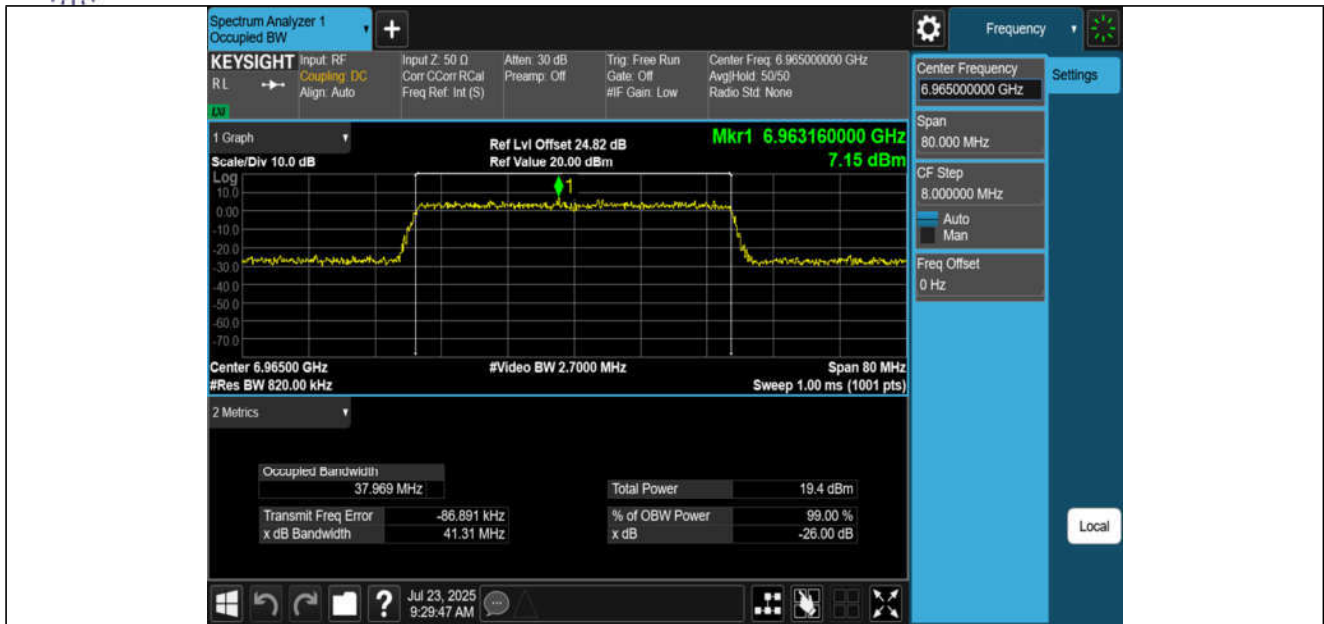
11BE40MIMO-Ant1-6965-PASS
