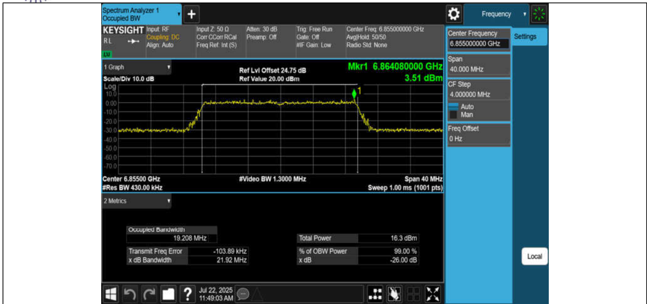
11BE20MIMO-Ant3-6855-PASS
