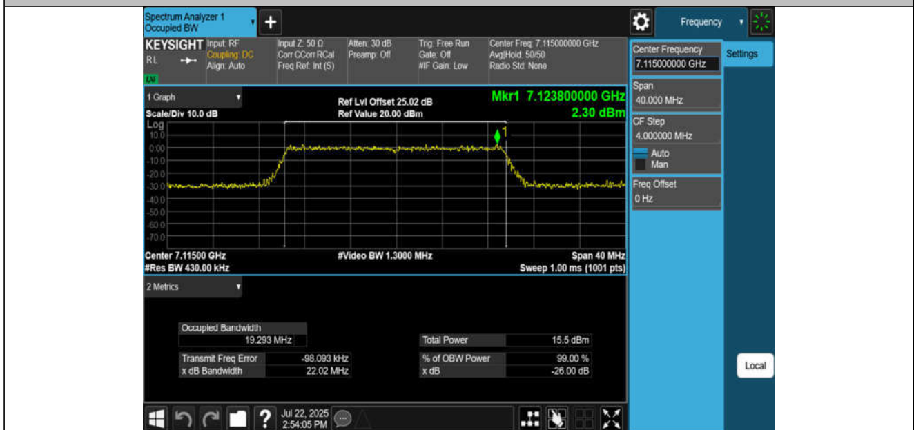
11BE20MIMO-Ant4-7115-PASS
