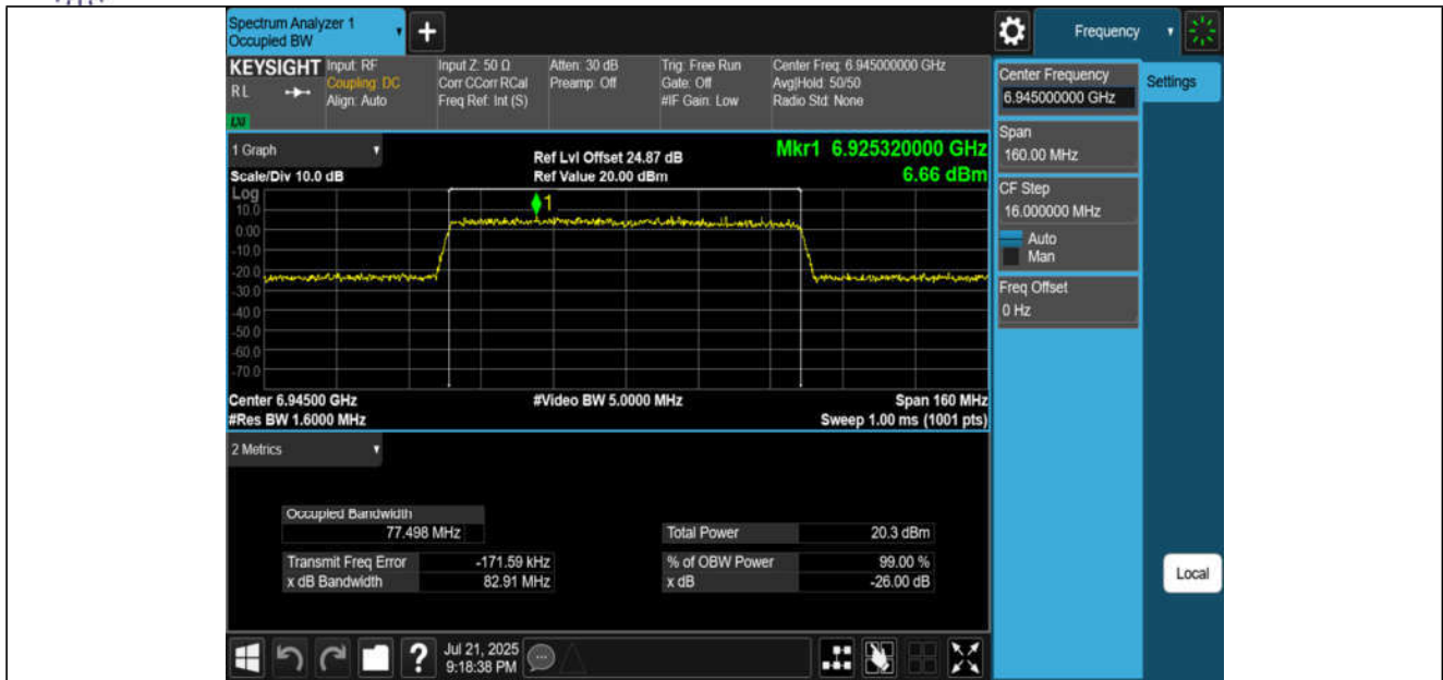
11AX80MIMO-Ant3-6945-PASS
