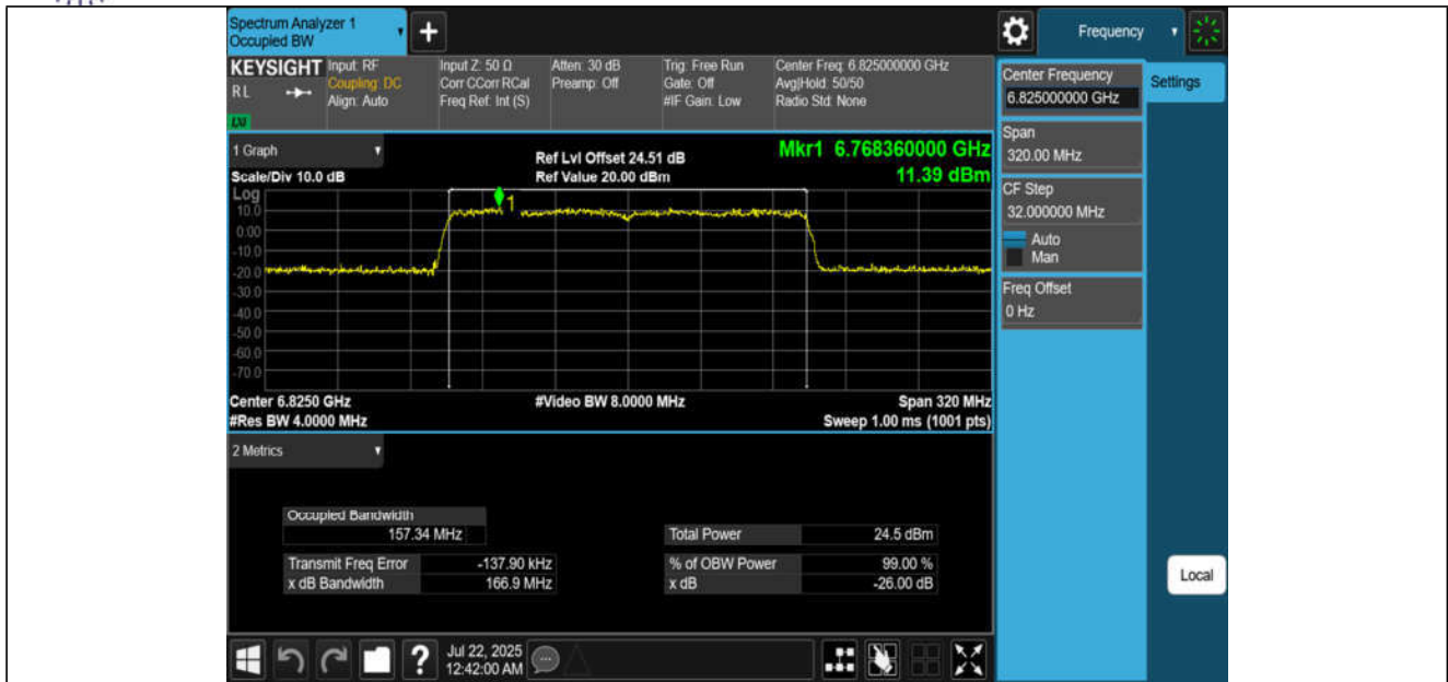
11AX160MIMO-Ant1-6825-PASS
