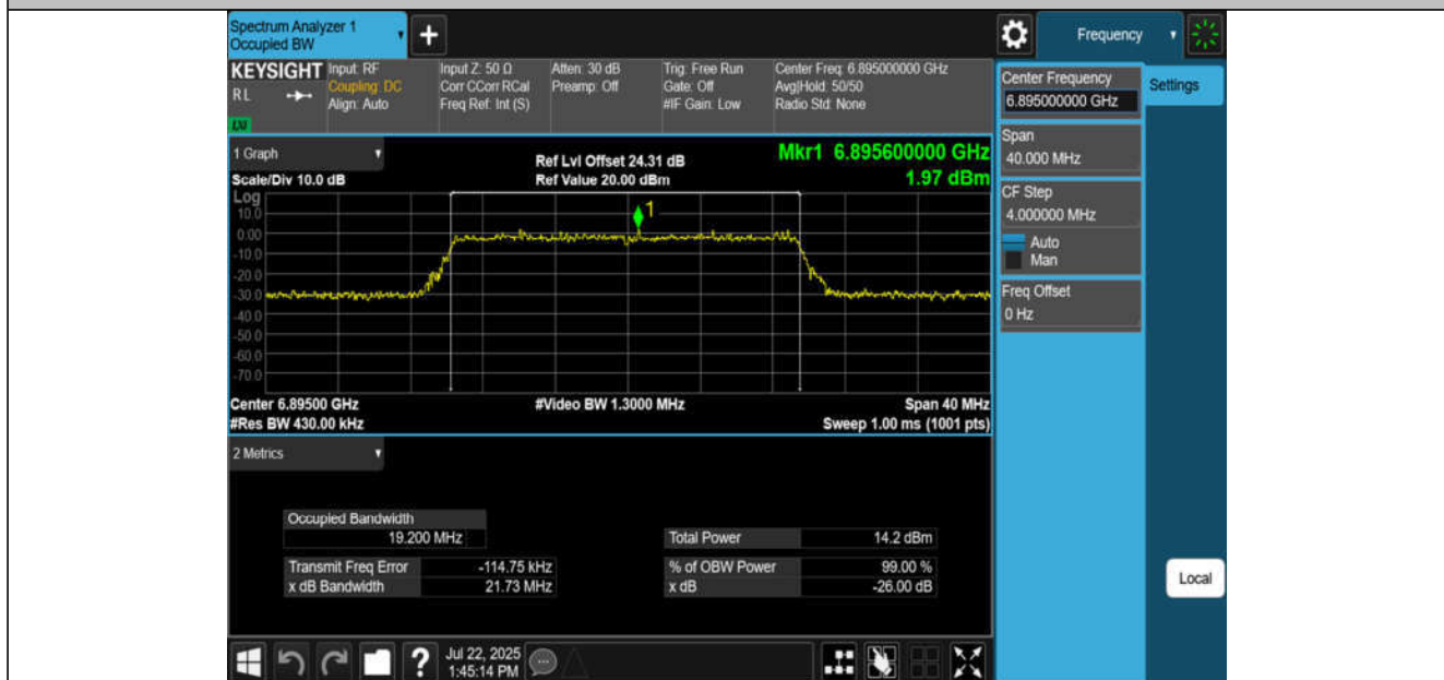
11BE20MIMO-Ant2-6895-PASS
