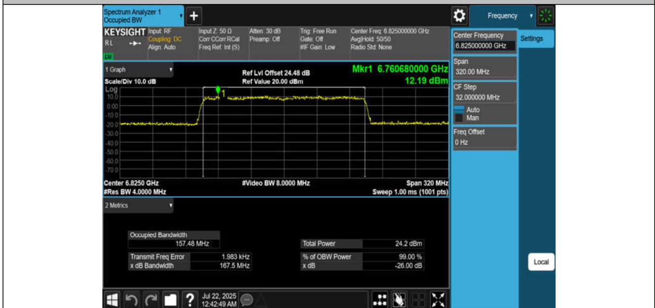
11AX160MIMO-Ant2-6825-PASS
