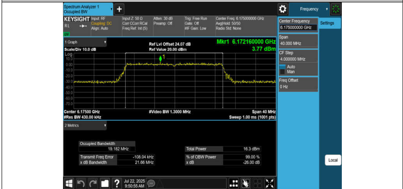
11BE20MIMO-Ant4-6175-PASS
