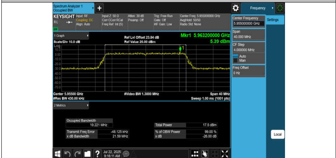
11BE20MIMO-Ant4-5955-PASS
