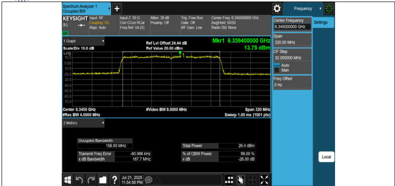
11AX160MIMO-Ant3-6345-PASS
