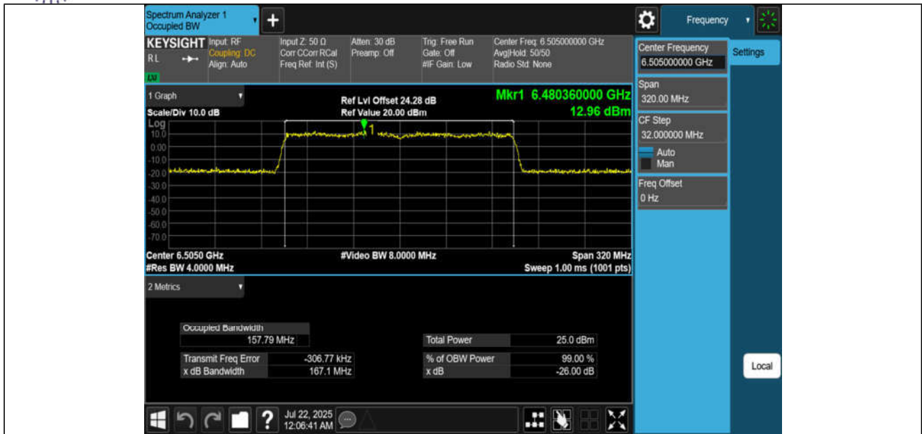
11AX160MIMO-Ant1-6505-PASS
