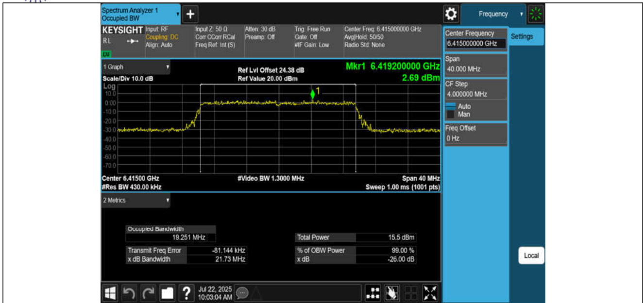
11BE20MIMO-Ant3-6415-PASS
