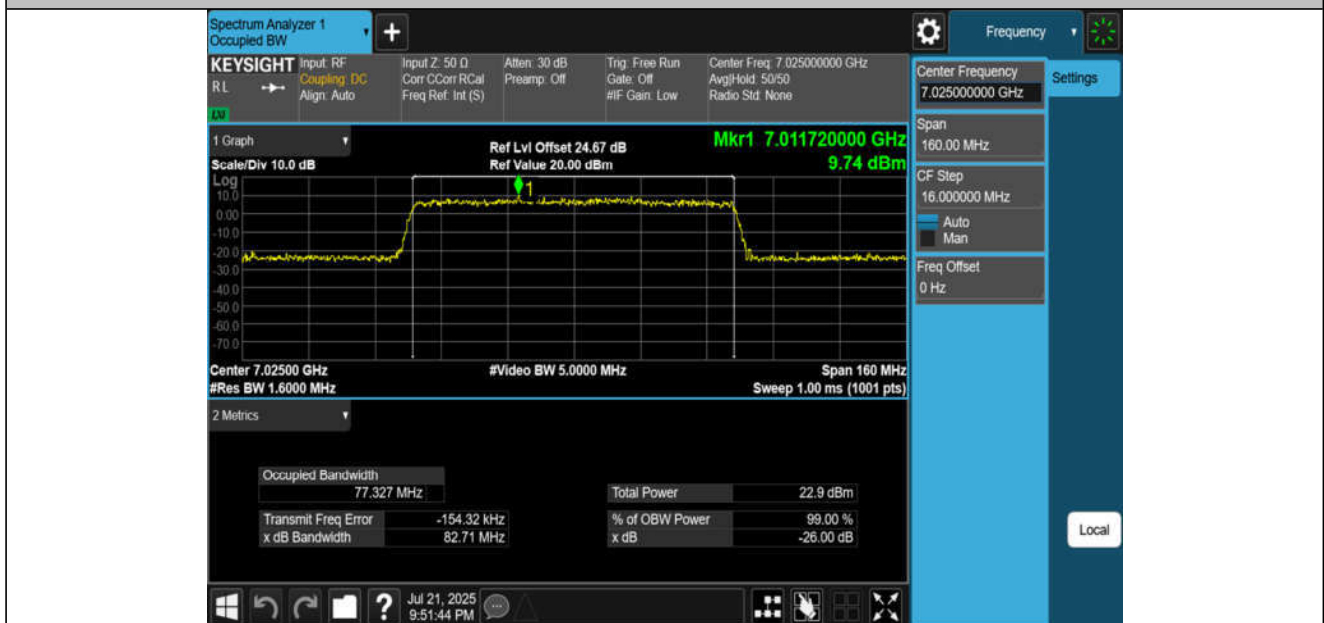
11AX80MIMO-Ant4-7025-PASS
