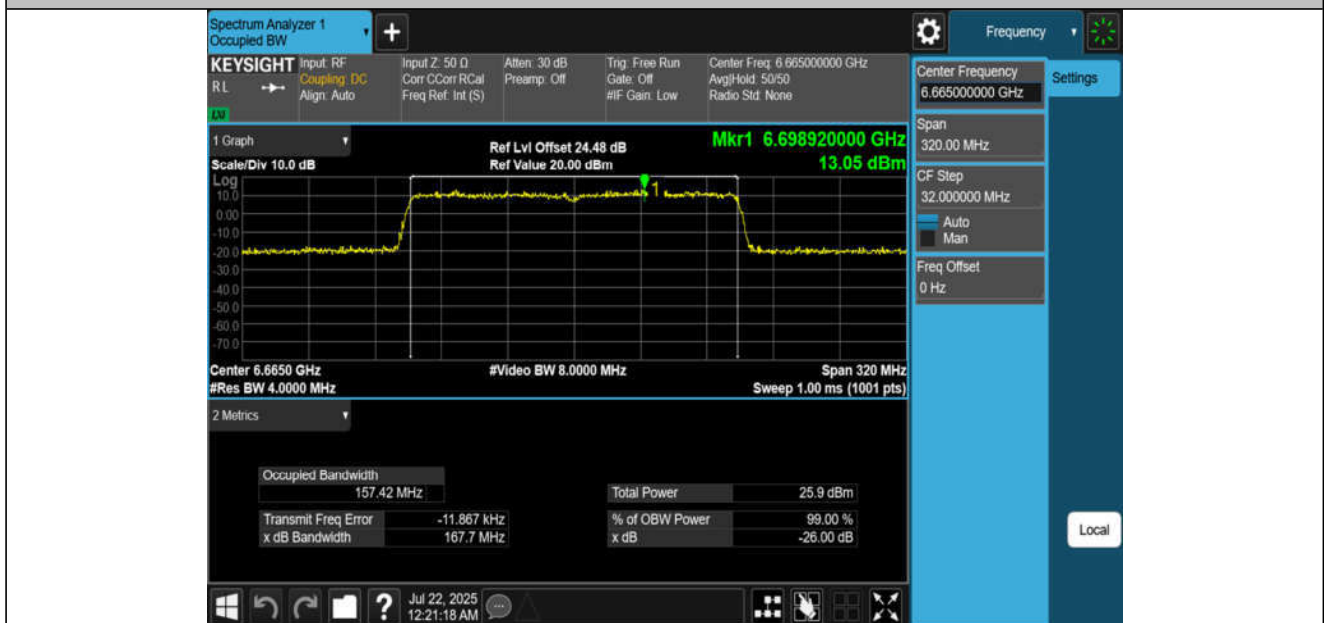
11AX160MIMO-Ant4-6665-PASS
