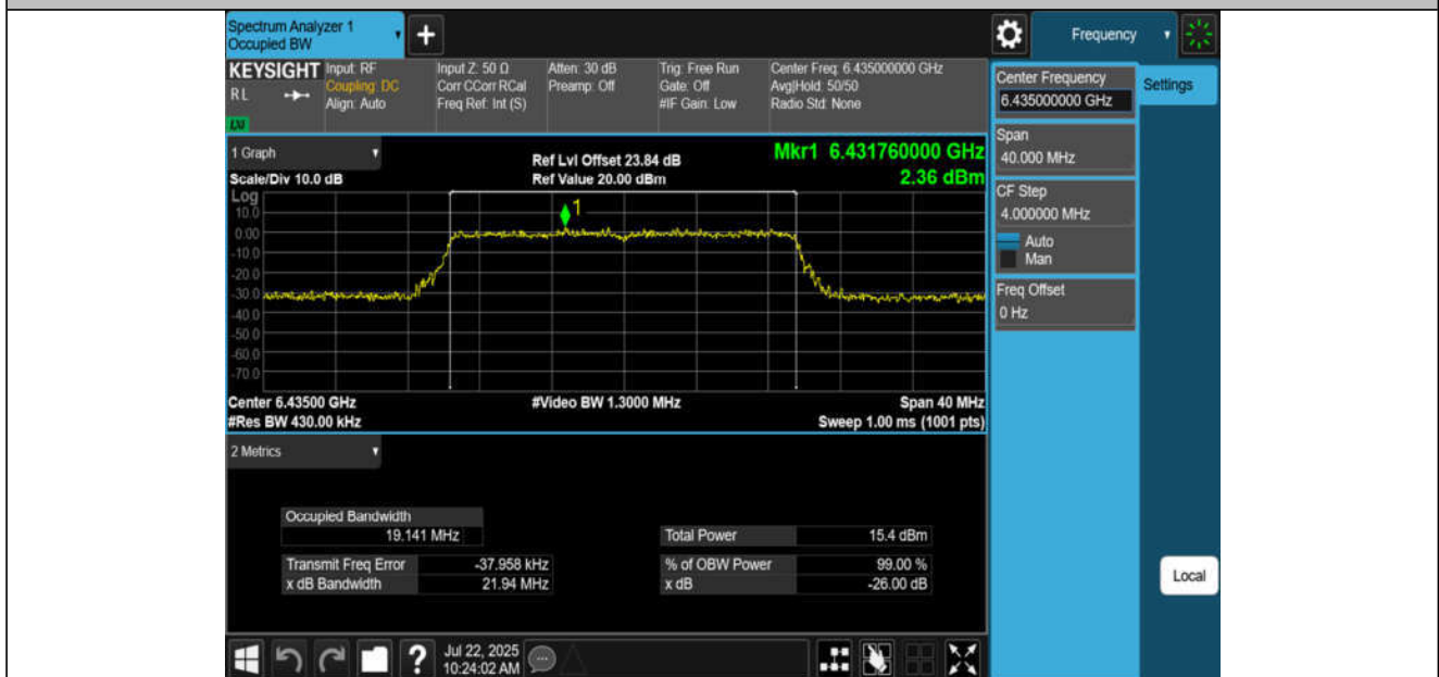
11BE20MIMO-Ant2-6435-PASS
