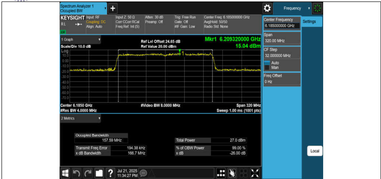
11AX160MIMO-Ant3-6185-PASS
