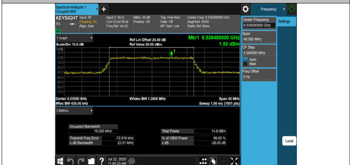
11BE20MIMO-Ant2-6535-PASS
