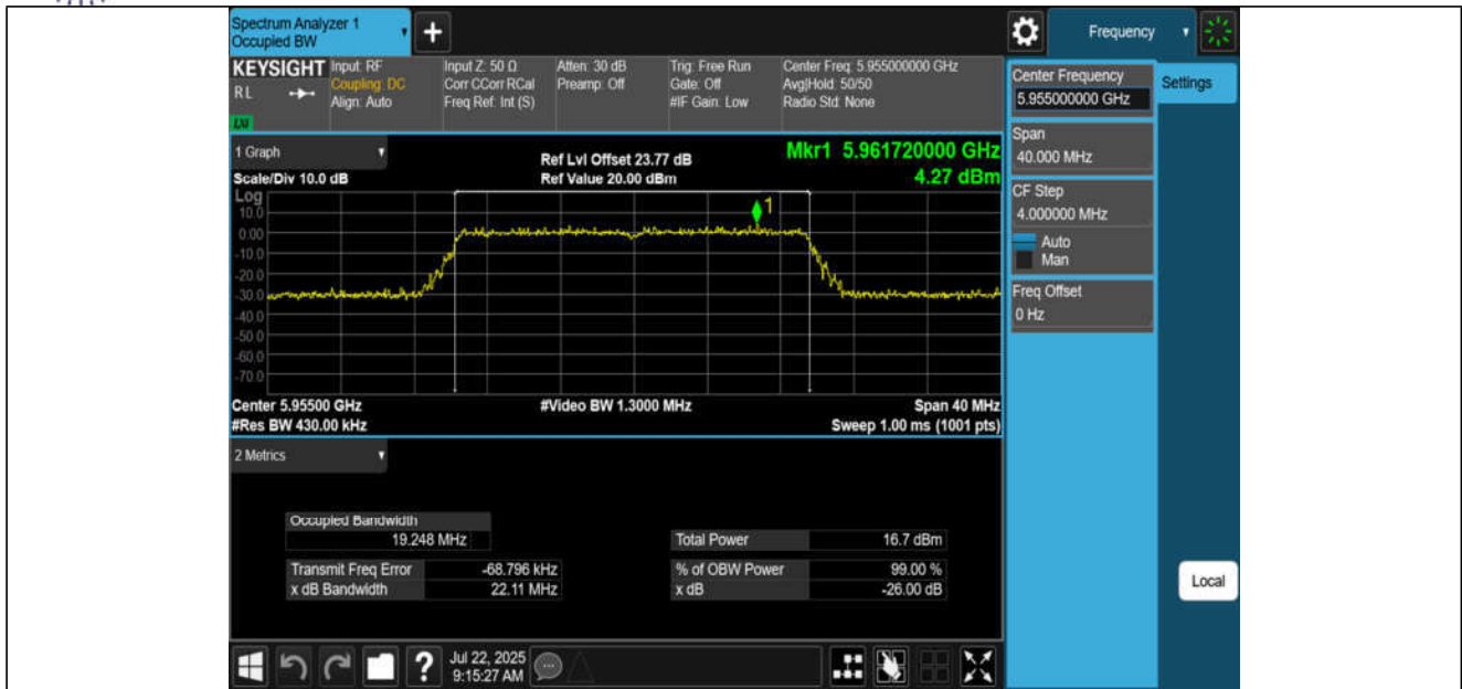
11BE20MIMO-Ant3-5955-PASS
