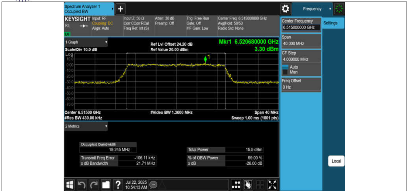
11BE20MIMO-Ant3-6515-PASS
