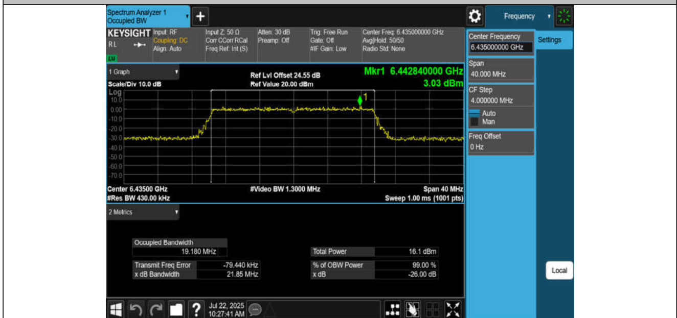
11BE20MIMO-Ant4-6435-PASS
