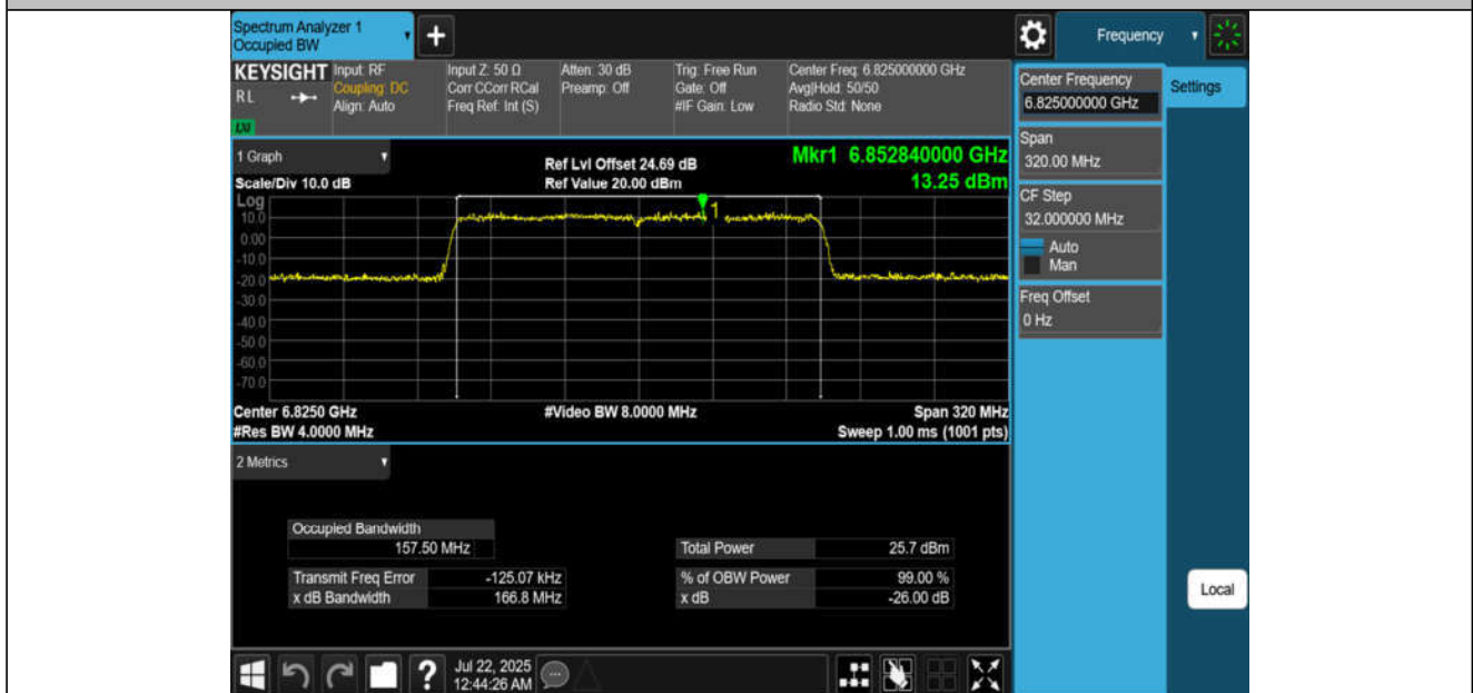
11AX160MIMO-Ant4-6825-PASS
