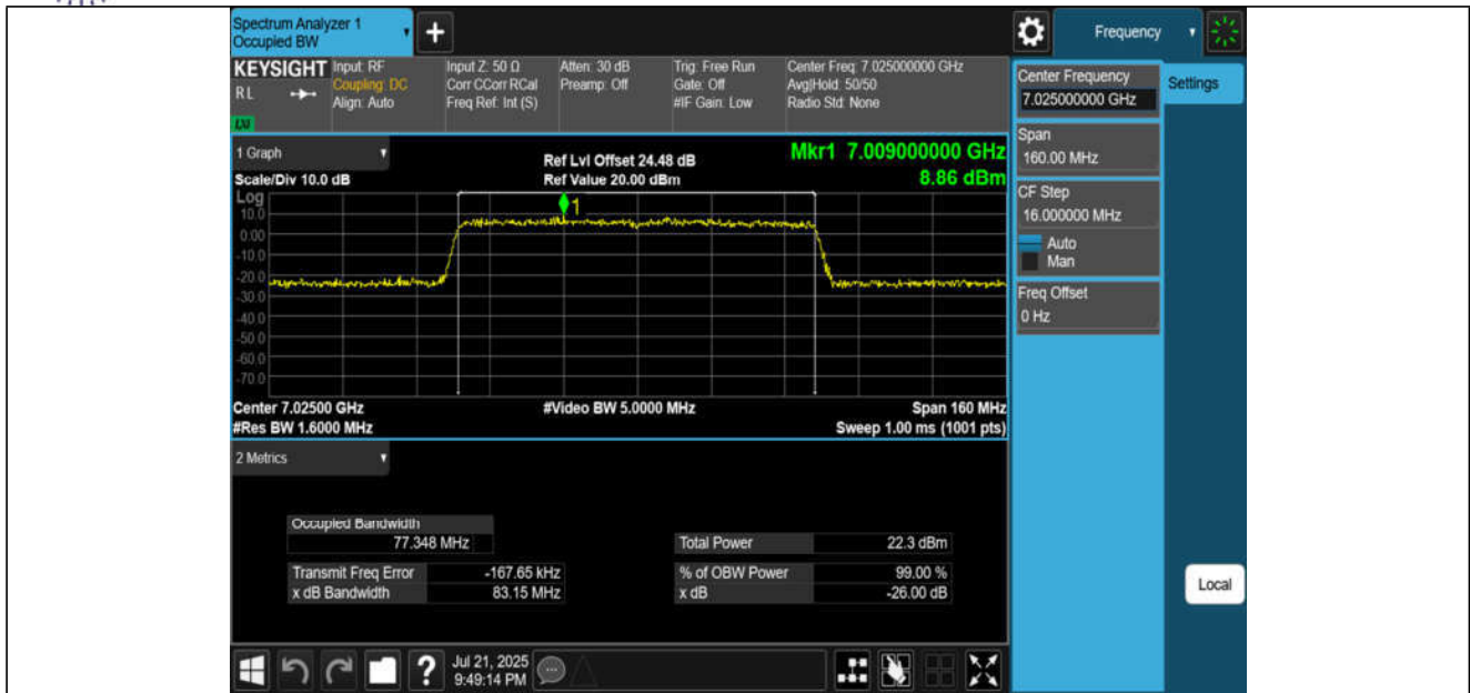
11AX80MIMO-Ant1-7025-PASS
