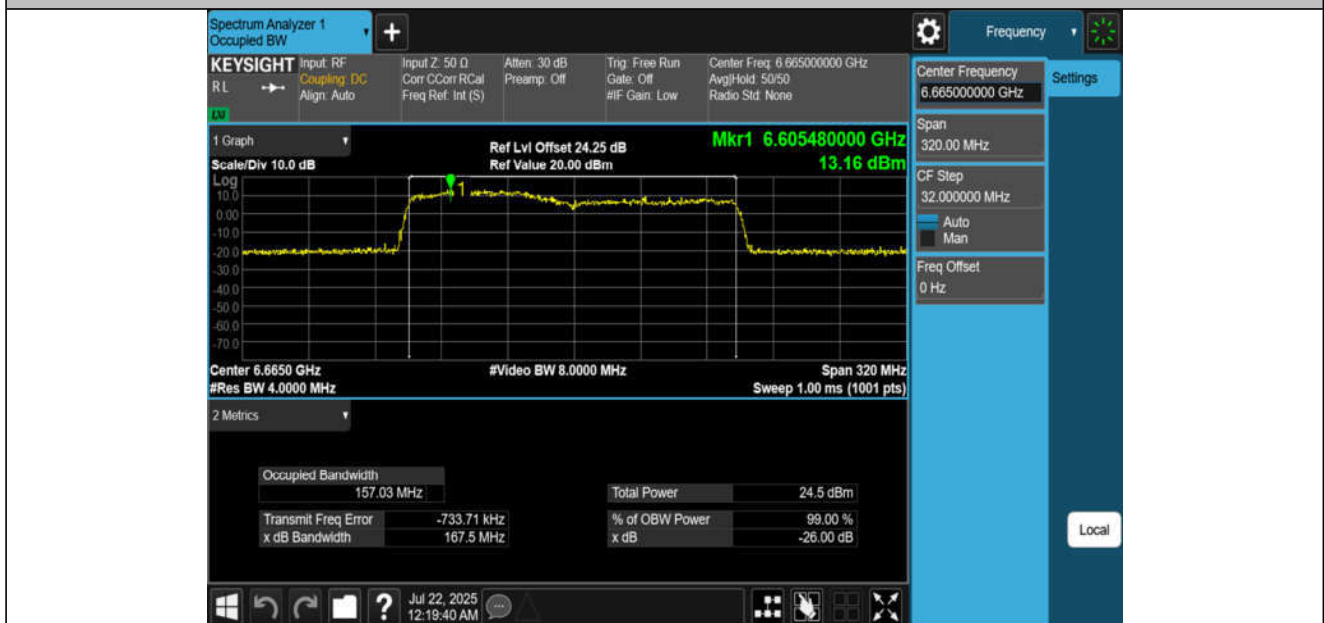
11AX160MIMO-Ant2-6665-PASS
