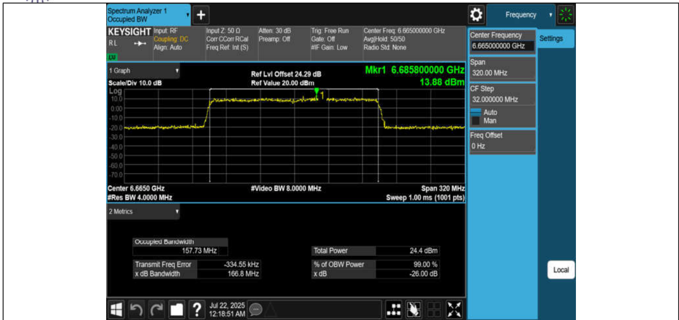
11AX160MIMO-Ant1-6665-PASS
