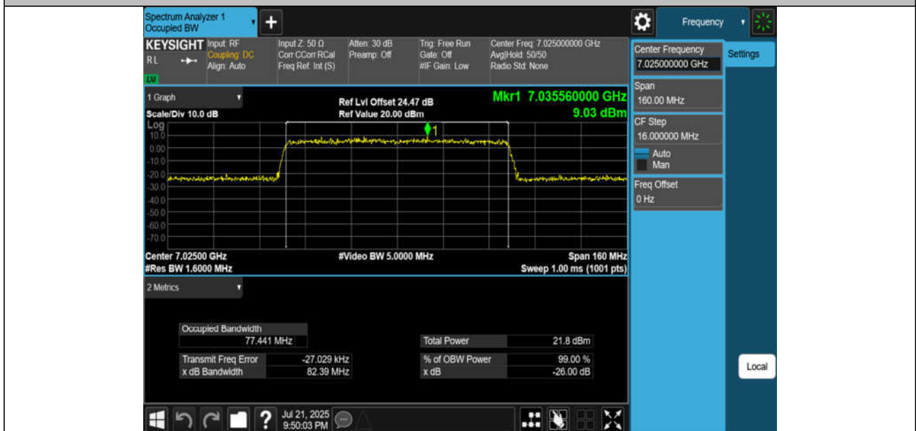
11AX80MIMO-Ant2-7025-PASS
