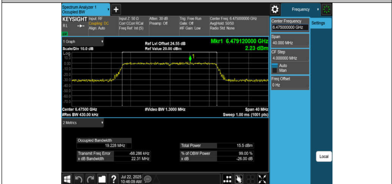
11BE20MIMO-Ant4-6475-PASS
