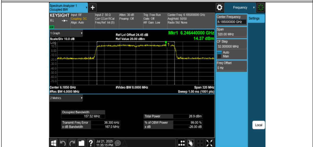
11AX160MIMO-Ant4-6185-PASS
