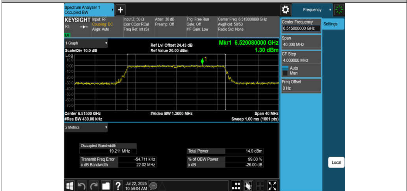
11BE20MIMO-Ant4-6515-PASS
