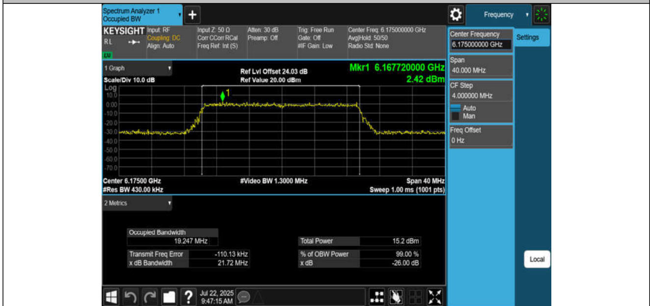
11BE20MIMO-Ant2-6175-PASS
