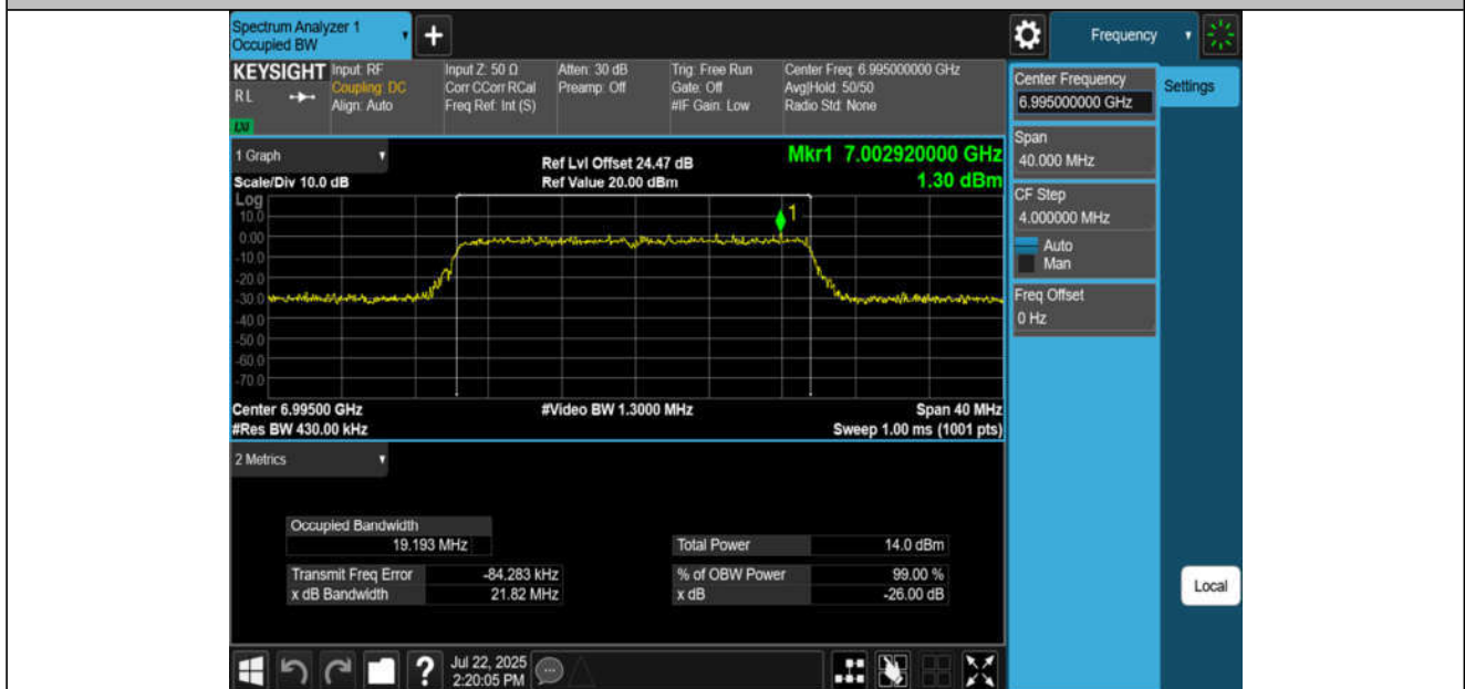
11BE20MIMO-Ant2-6995-PASS
