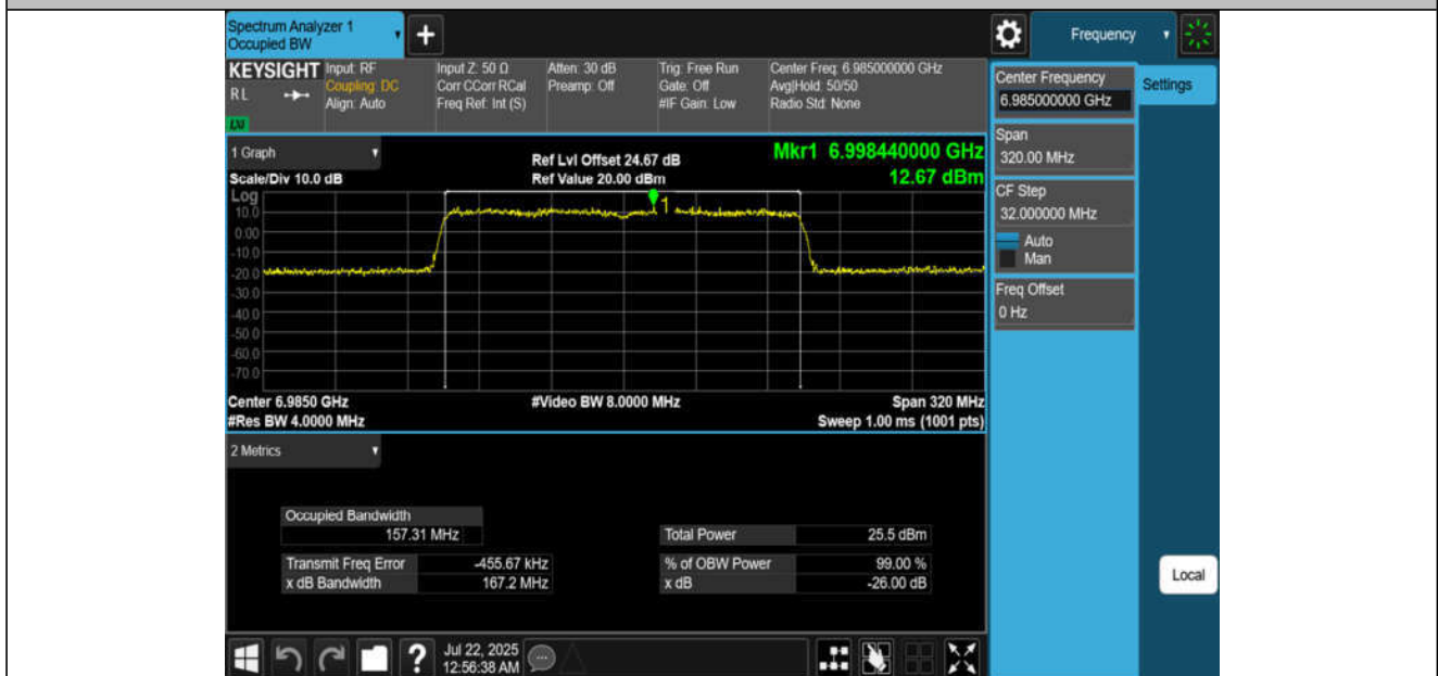
11AX160MIMO-Ant4-6985-PASS
