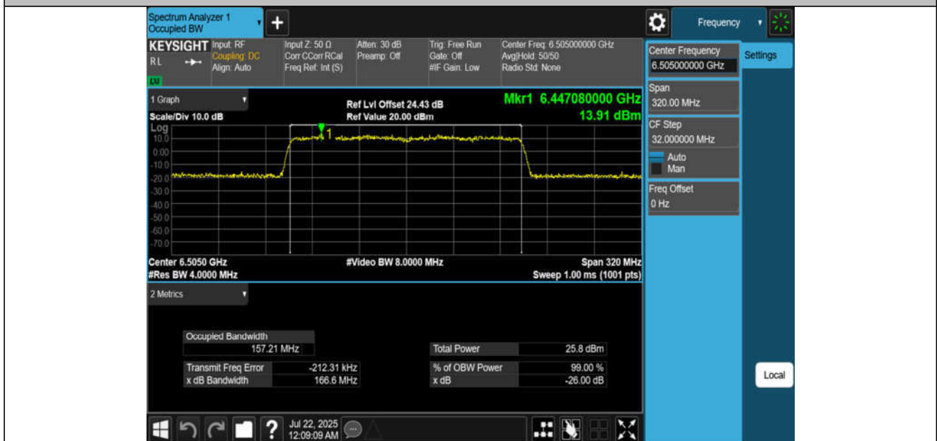
11AX160MIMO-Ant4-6505-PASS
