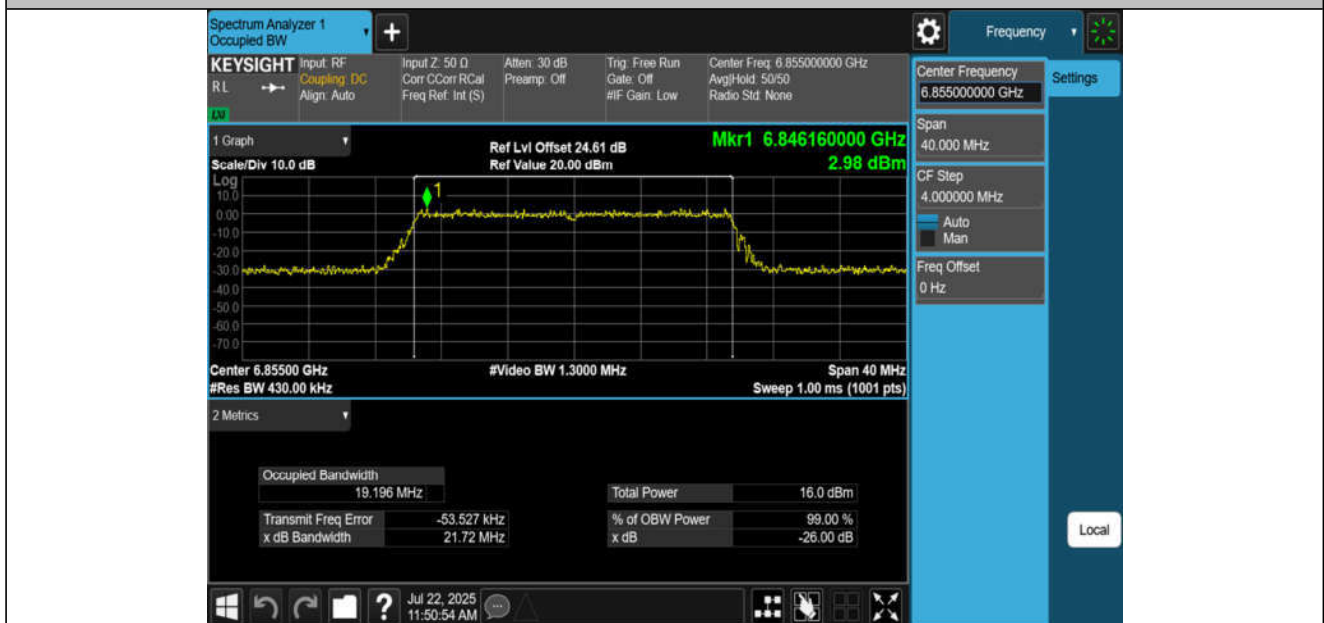
11BE20MIMO-Ant4-6855-PASS
