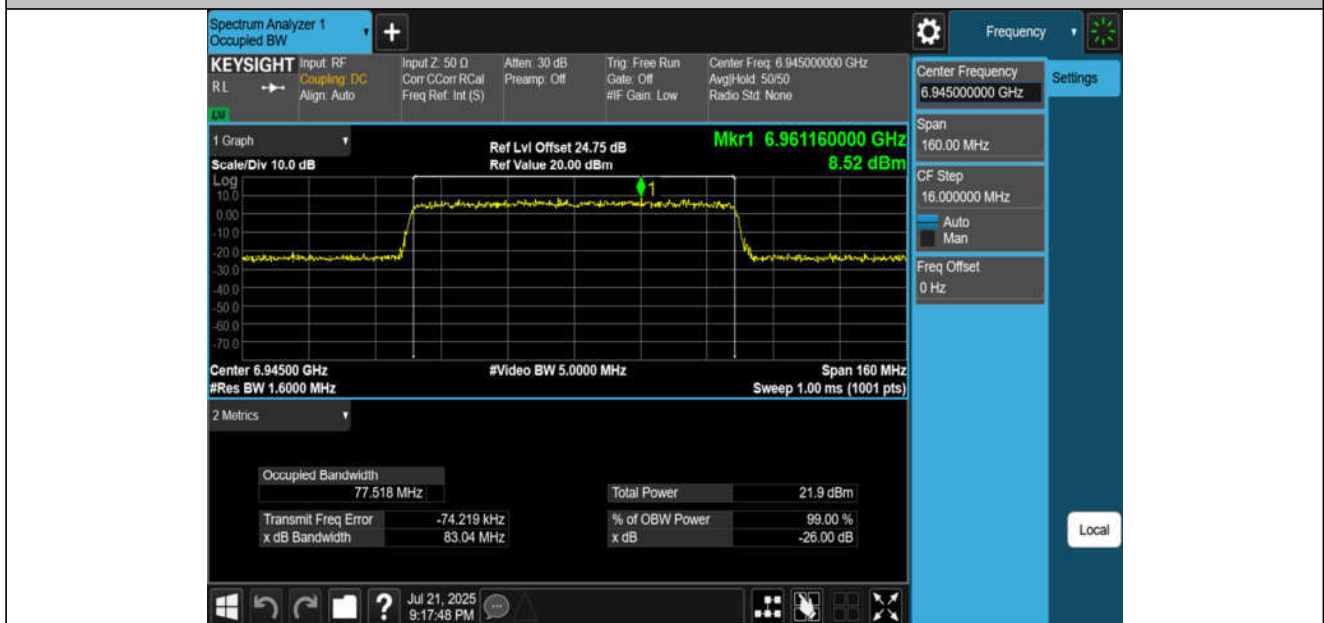
11AX80MIMO-Ant2-6945-PASS
