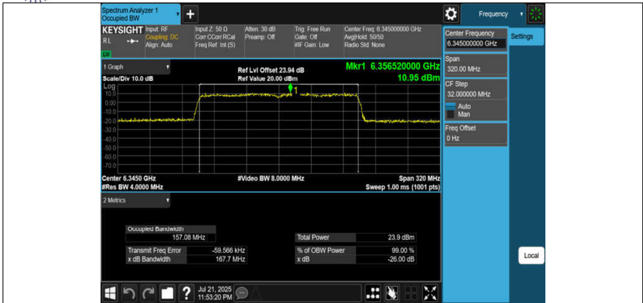
11AX160MIMO-Ant1-6345-PASS
