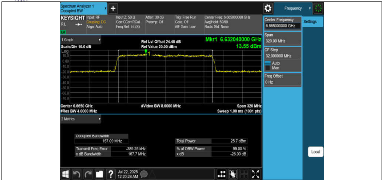
11AX160MIMO-Ant3-6665-PASS
