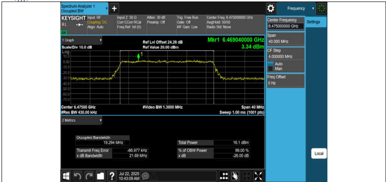
11BE20MIMO-Ant3-6475-PASS
