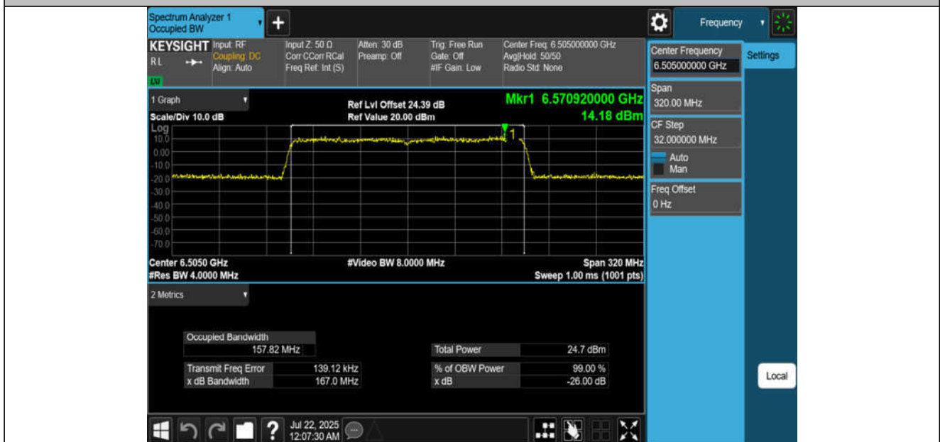
11AX160MIMO-Ant2-6505-PASS
