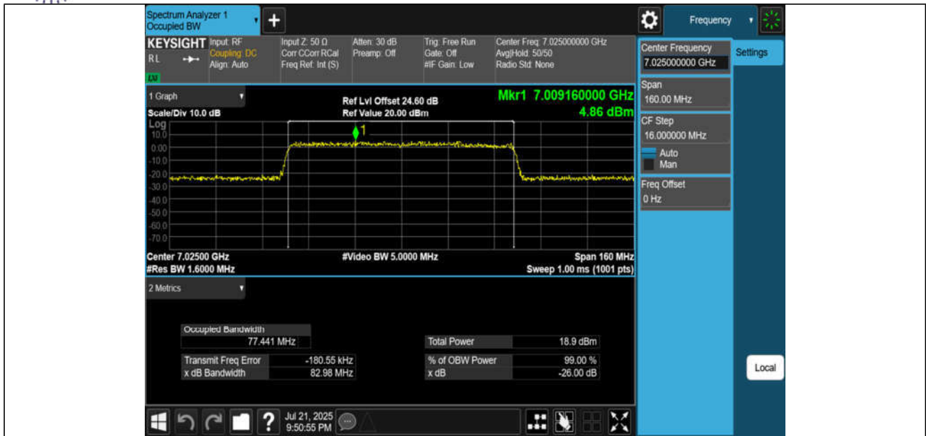
11AX80MIMO-Ant3-7025-PASS
