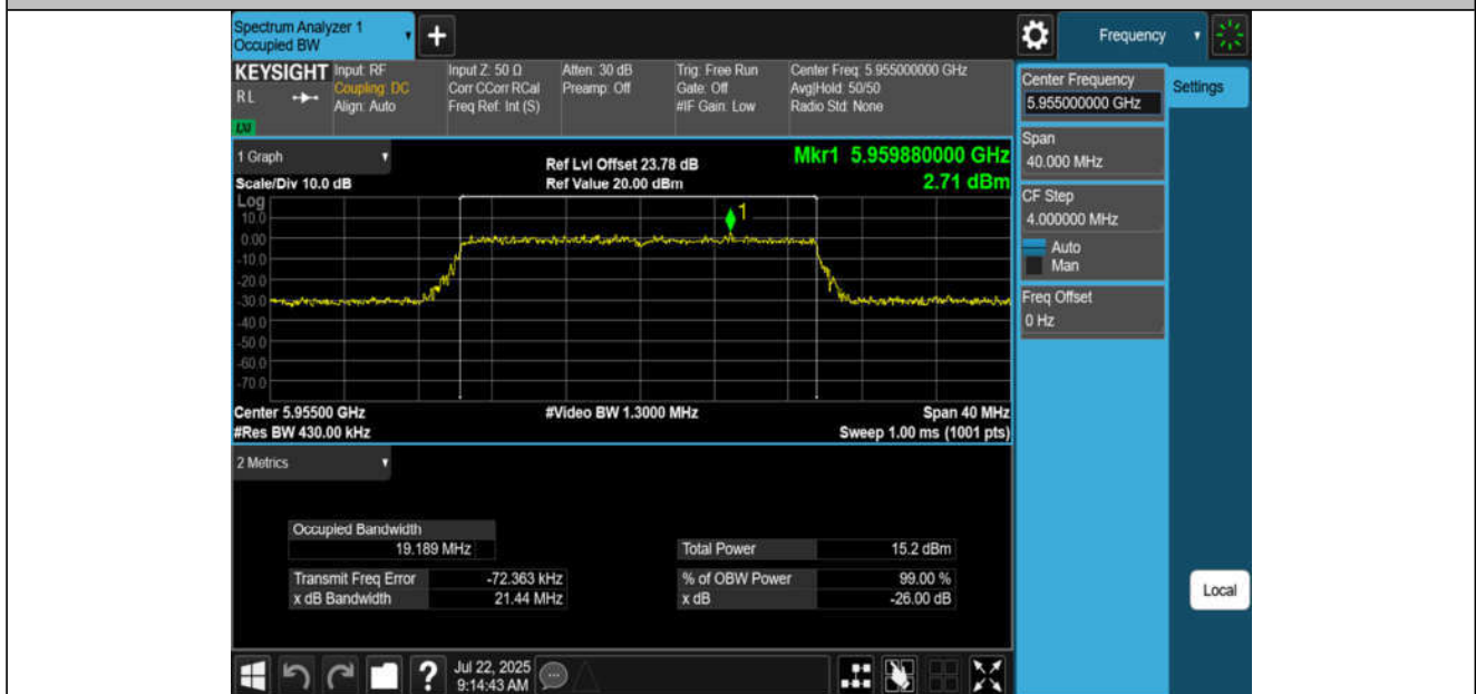
11BE20MIMO-Ant2-5955-PASS
