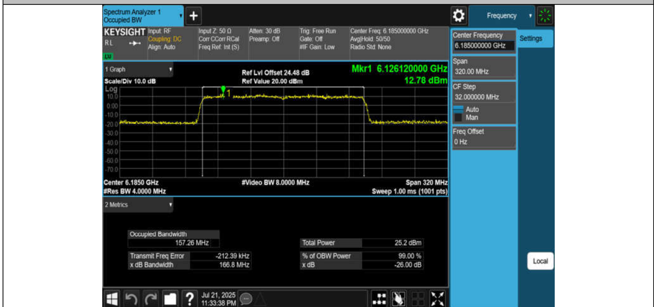
11AX160MIMO-Ant2-6185-PASS
