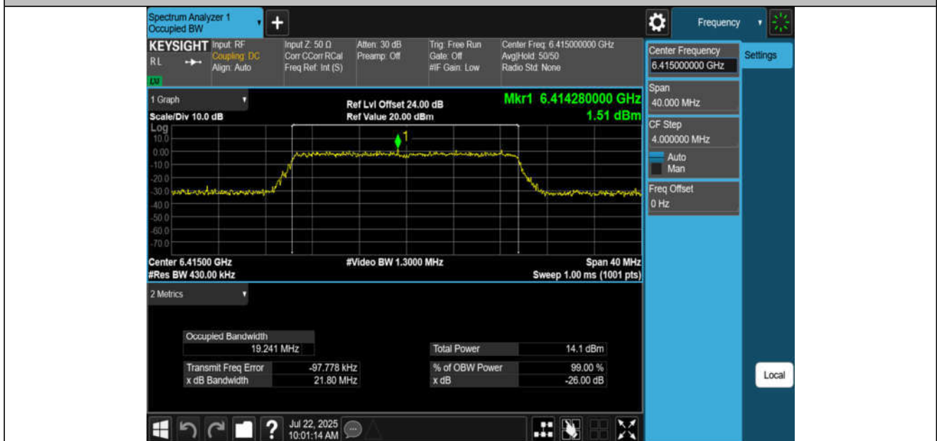
11BE20MIMO-Ant2-6415-PASS
