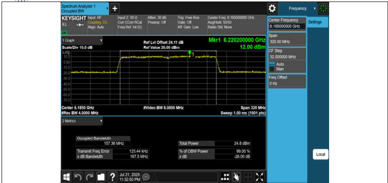
11AX160MIMO-Ant1-6185-PASS
