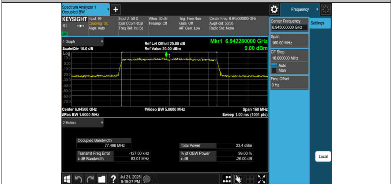
11AX80MIMO-Ant4-6945-PASS
