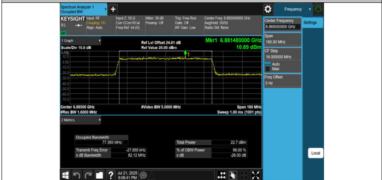
11AX80MIMO-Ant4-6865-PASS
