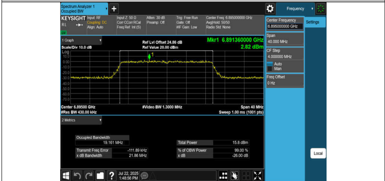
11BE20MIMO-Ant4-6895-PASS
