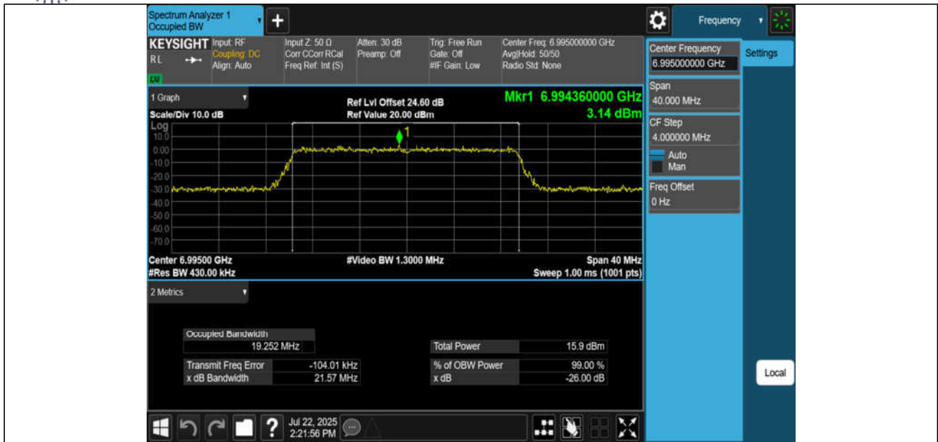
11BE20MIMO-Ant3-6995-PASS
