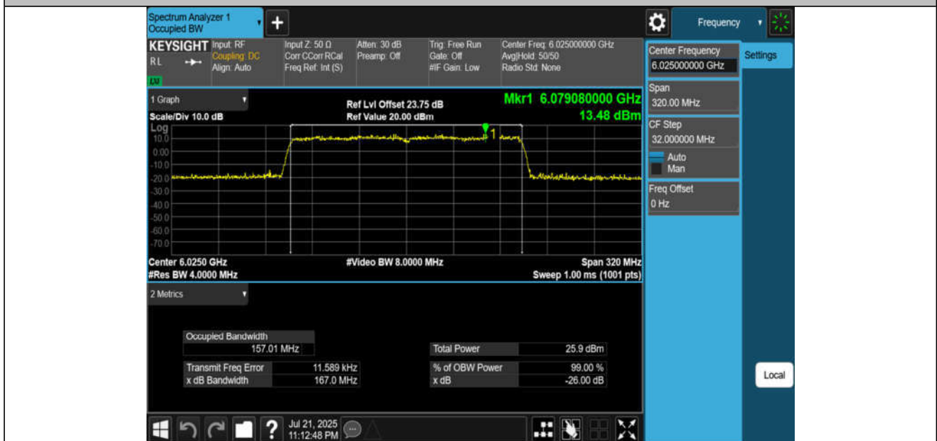
11AX160MIMO-Ant4-6025-PASS
