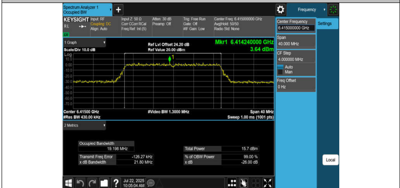
11BE20MIMO-Ant4-6415-PASS
