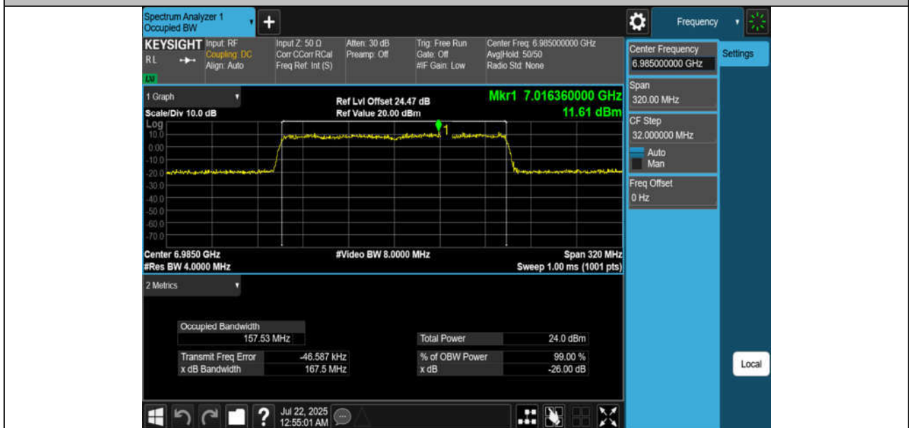
11AX160MIMO-Ant2-6985-PASS
