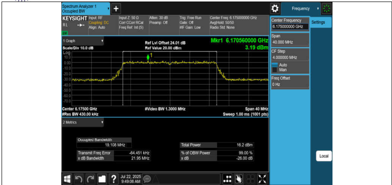
11BE20MIMO-Ant3-6175-PASS
