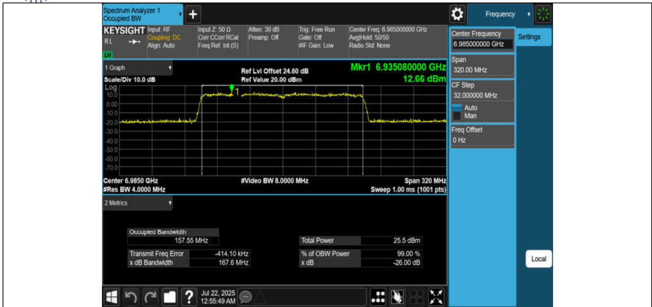
11AX160MIMO-Ant3-6985-PASS
