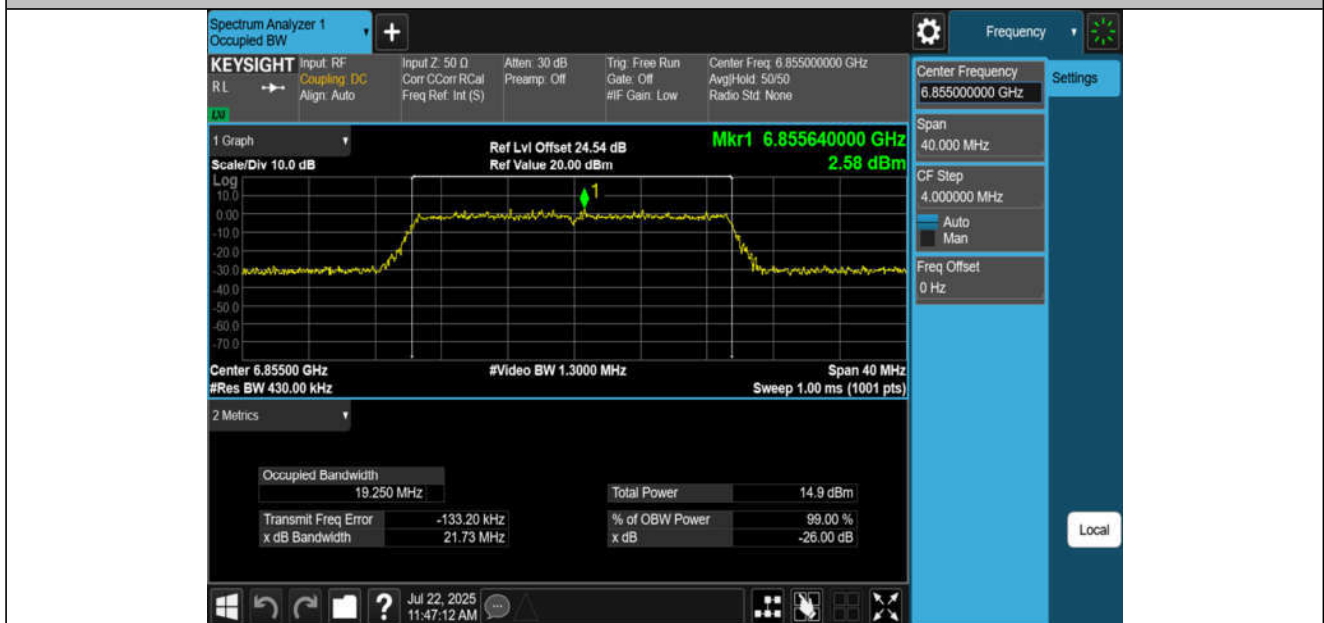
11BE20MIMO-Ant2-6855-PASS
