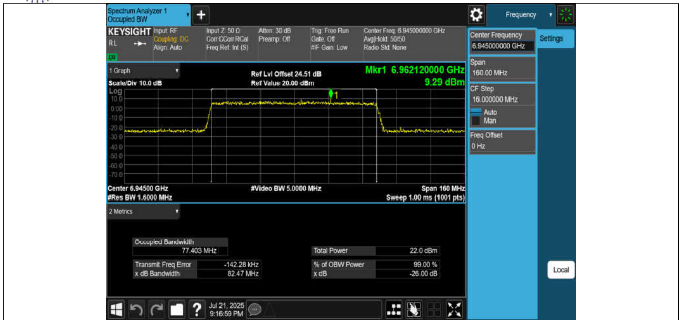
11AX80MIMO-Ant1-6945-PASS
