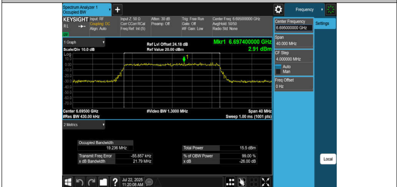
11BE20MIMO-Ant2-6695-PASS
