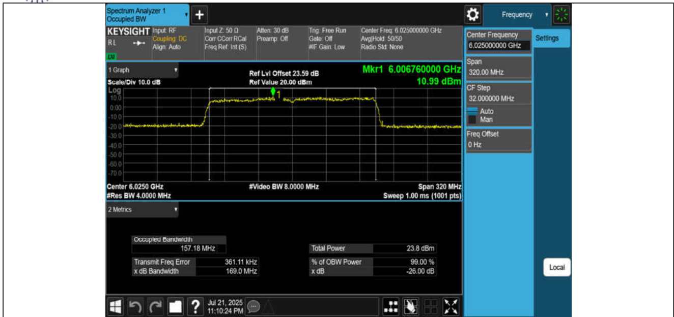
11AX160MIMO-Ant1-6025-PASS
