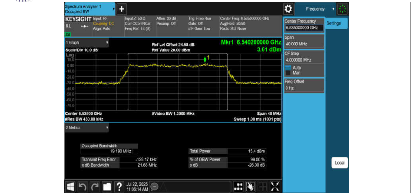
11BE20MIMO-Ant3-6535-PASS
