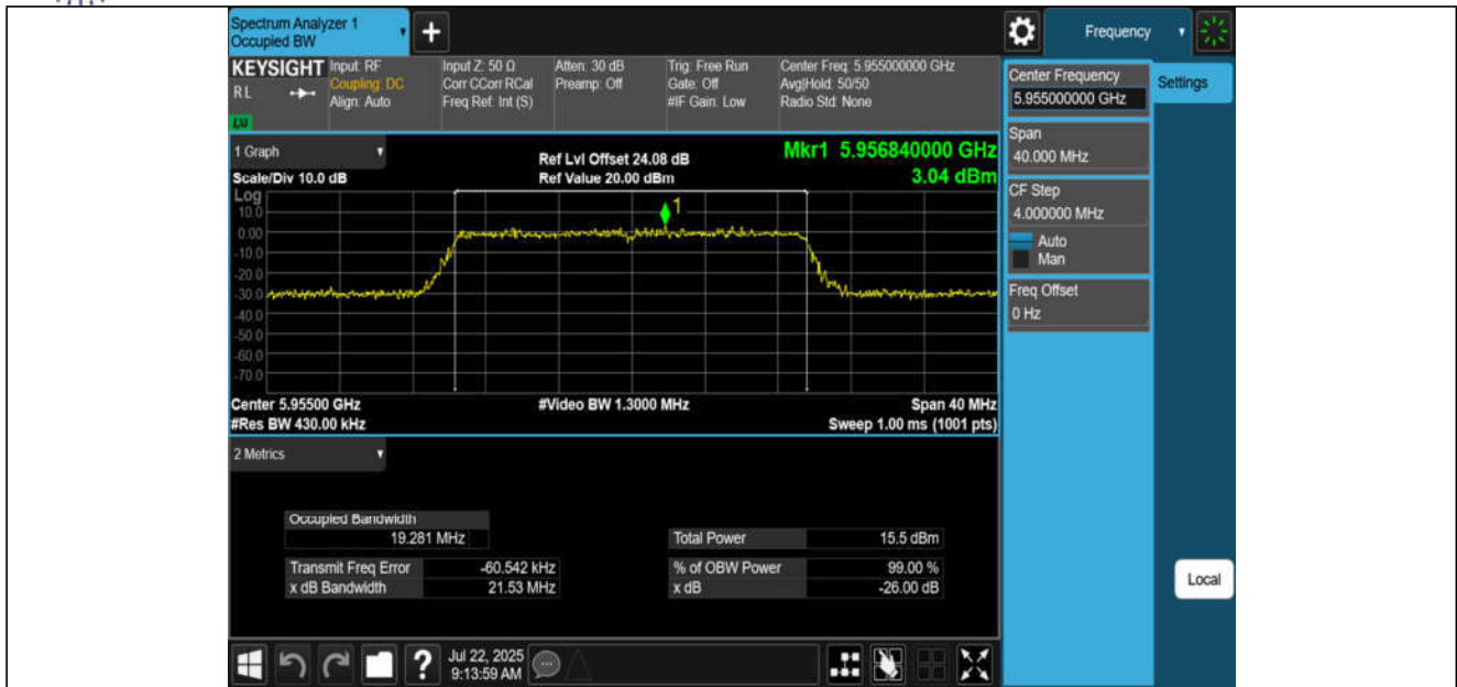
11BE20MIMO-Ant1-5955-PASS
