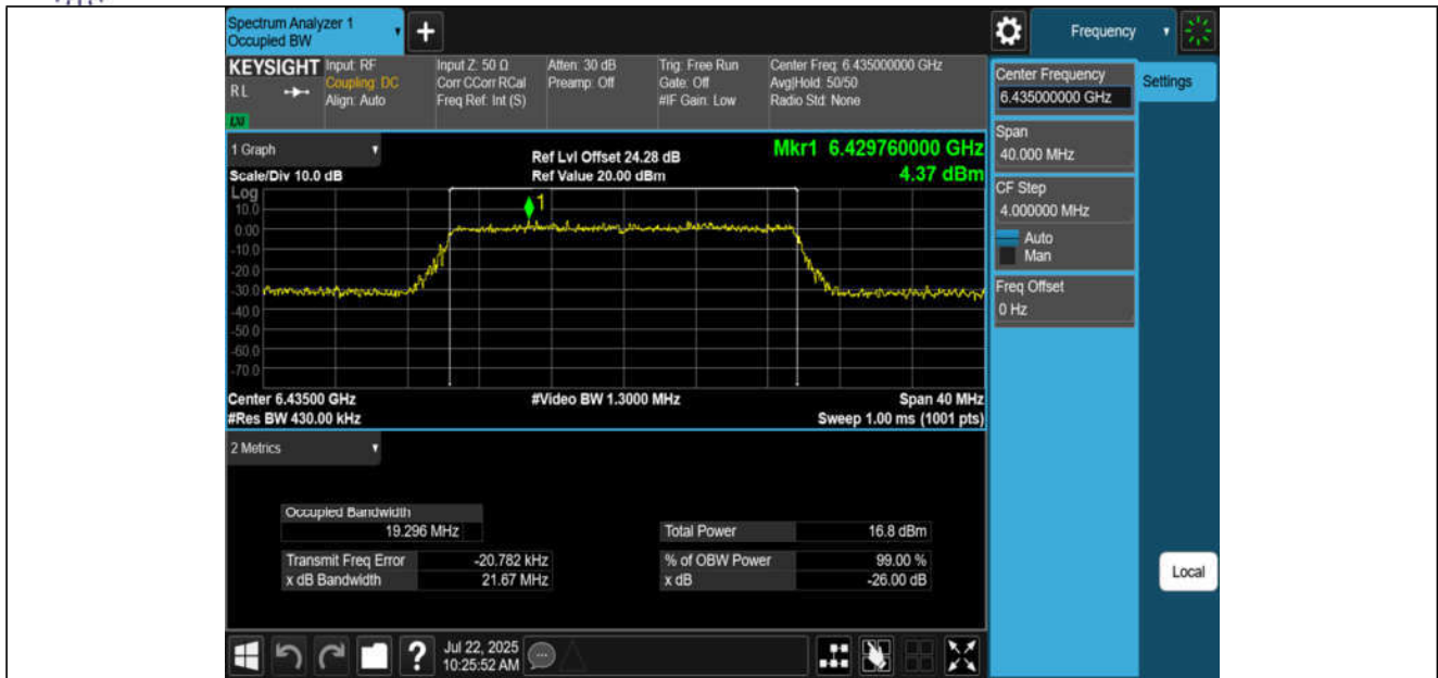
11BE20MIMO-Ant3-6435-PASS
