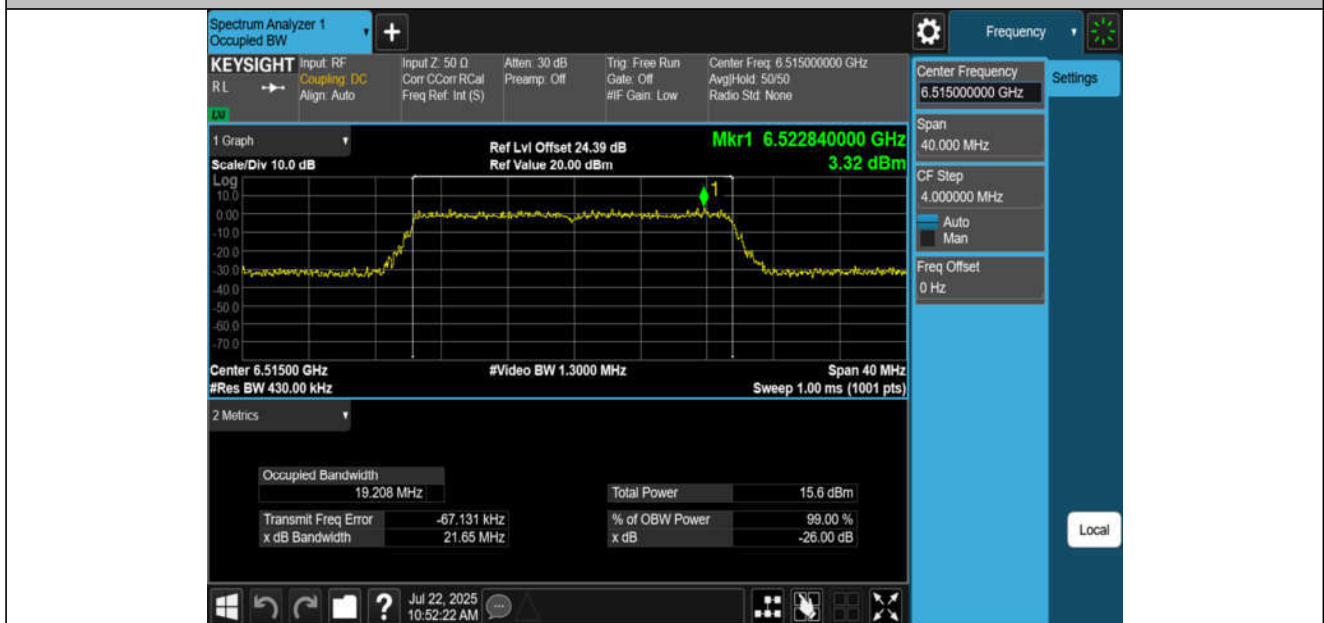
11BE20MIMO-Ant2-6515-PASS
