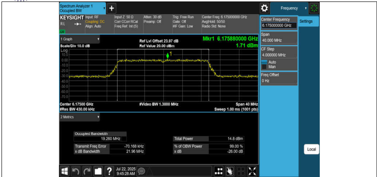
11BE20MIMO-Ant1-6175-PASS
