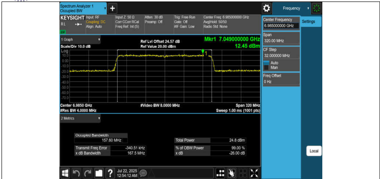
11AX160MIMO-Ant1-6985-PASS
