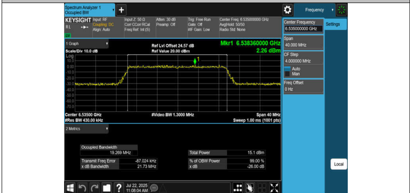
11BE20MIMO-Ant4-6535-PASS
