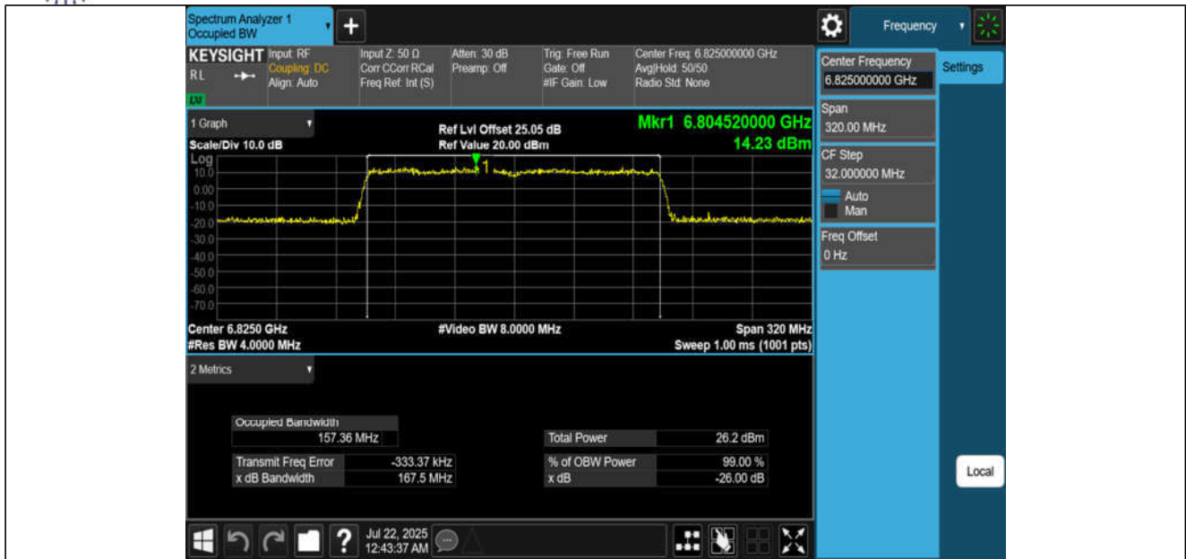
11AX160MIMO-Ant3-6825-PASS
