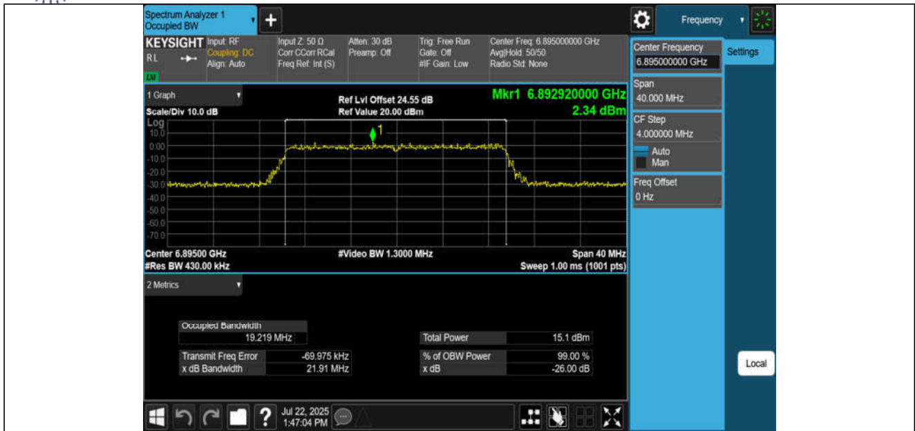
11BE20MIMO-Ant3-6895-PASS
