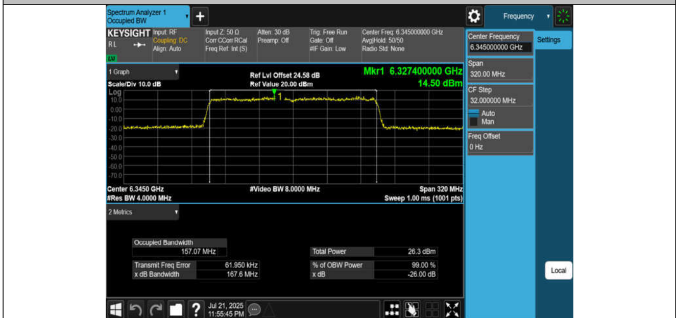
11AX160MIMO-Ant4-6345-PASS
