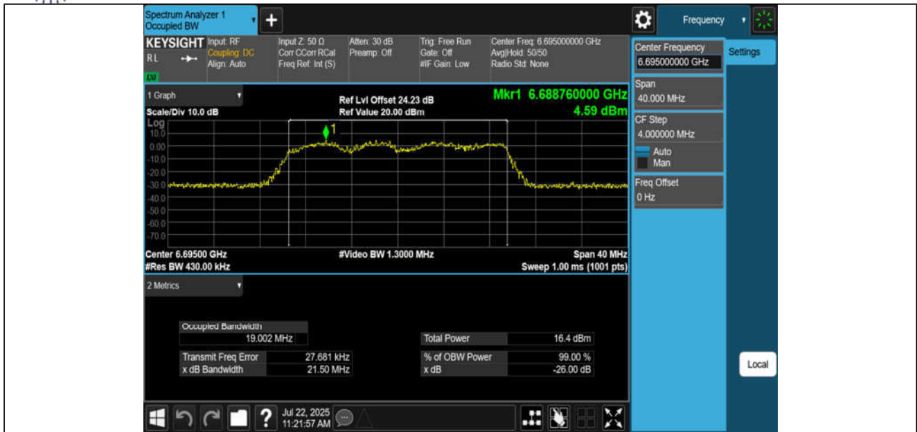
11BE20MIMO-Ant3-6695-PASS
