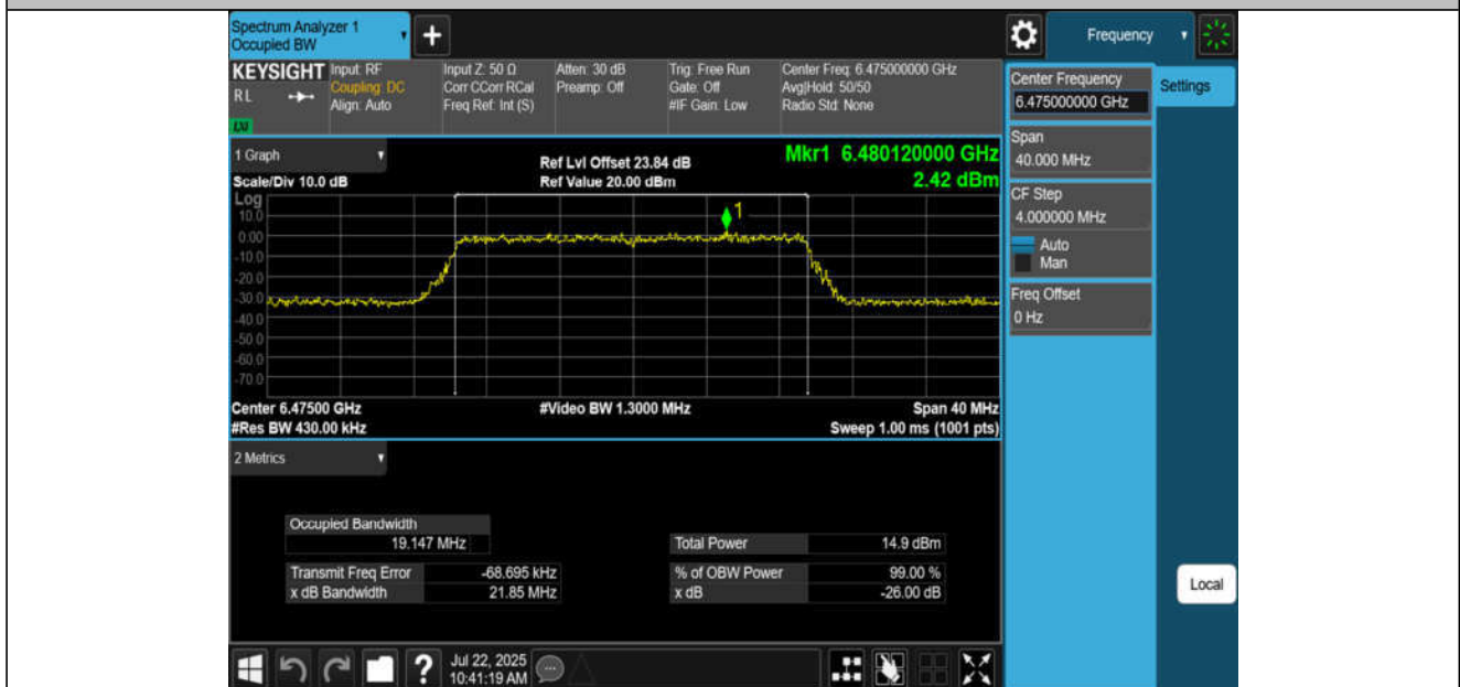
11BE20MIMO-Ant2-6475-PASS
