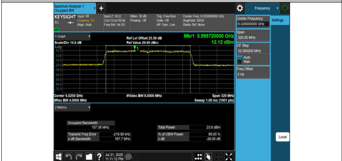
11AX160MIMO-Ant2-6025-PASS
