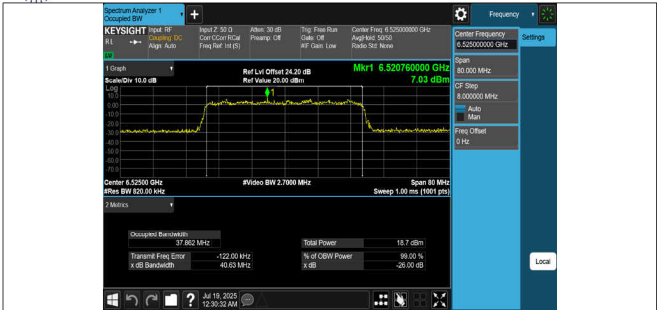
11AX40MIMO-Ant3-6525-PASS
