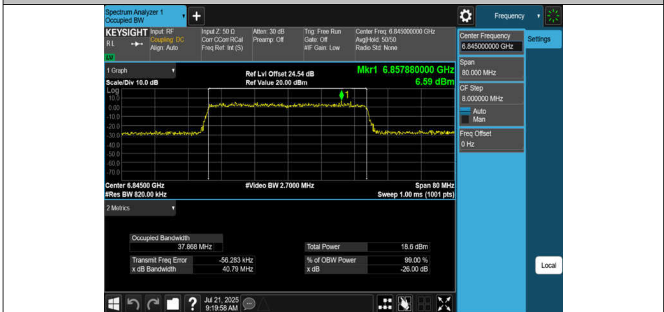
11AX40MIMO-Ant2-6845-PASS
