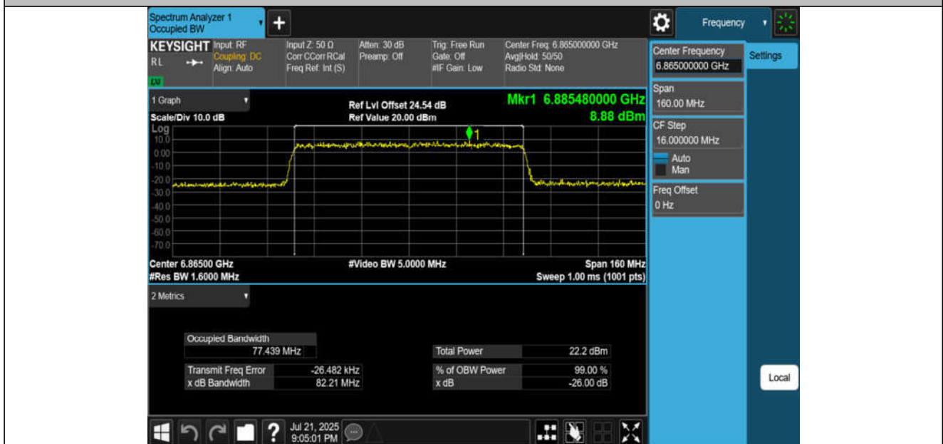
11AX80MIMO-Ant2-6865-PASS
