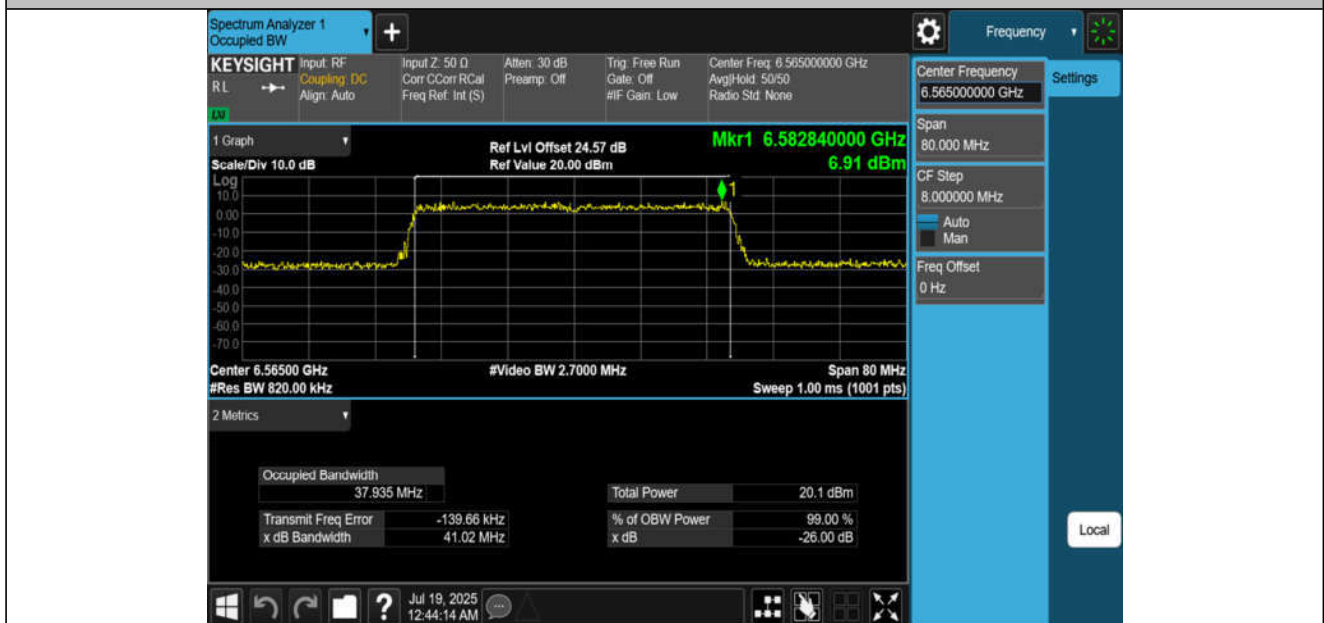
11AX40MIMO-Ant4-6565-PASS
