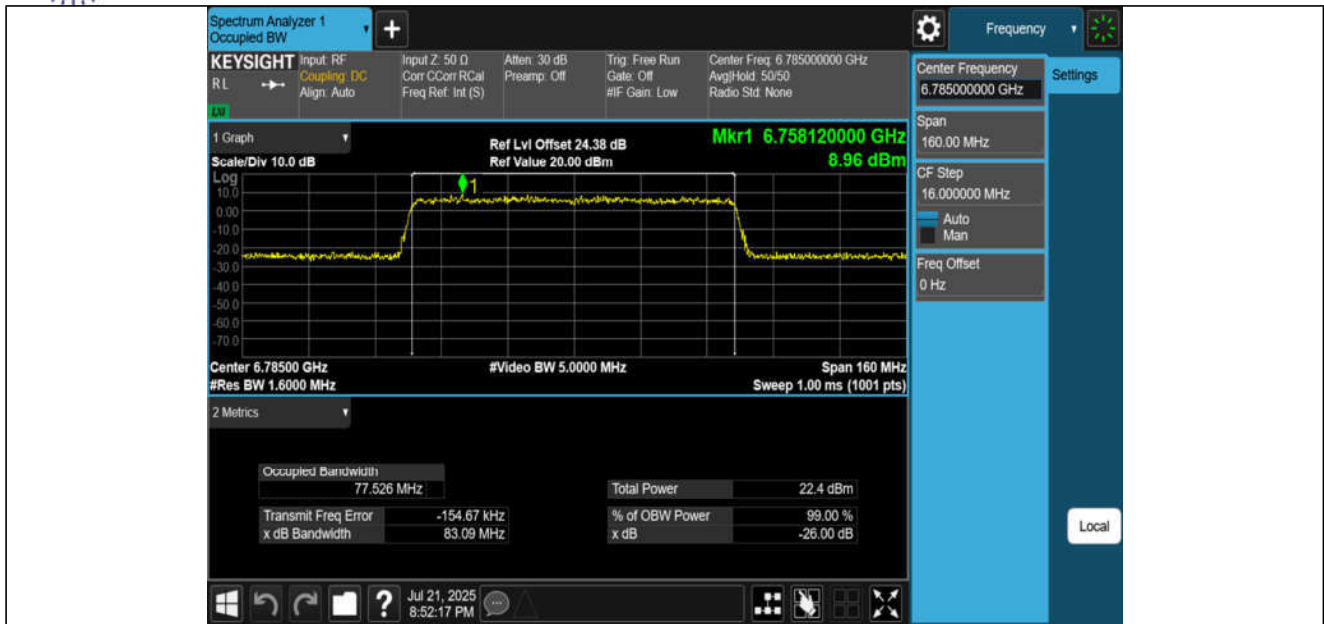
11AX80MIMO-Ant1-6785-PASS
