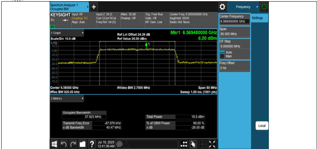
11AX40MIMO-Ant1-6565-PASS
