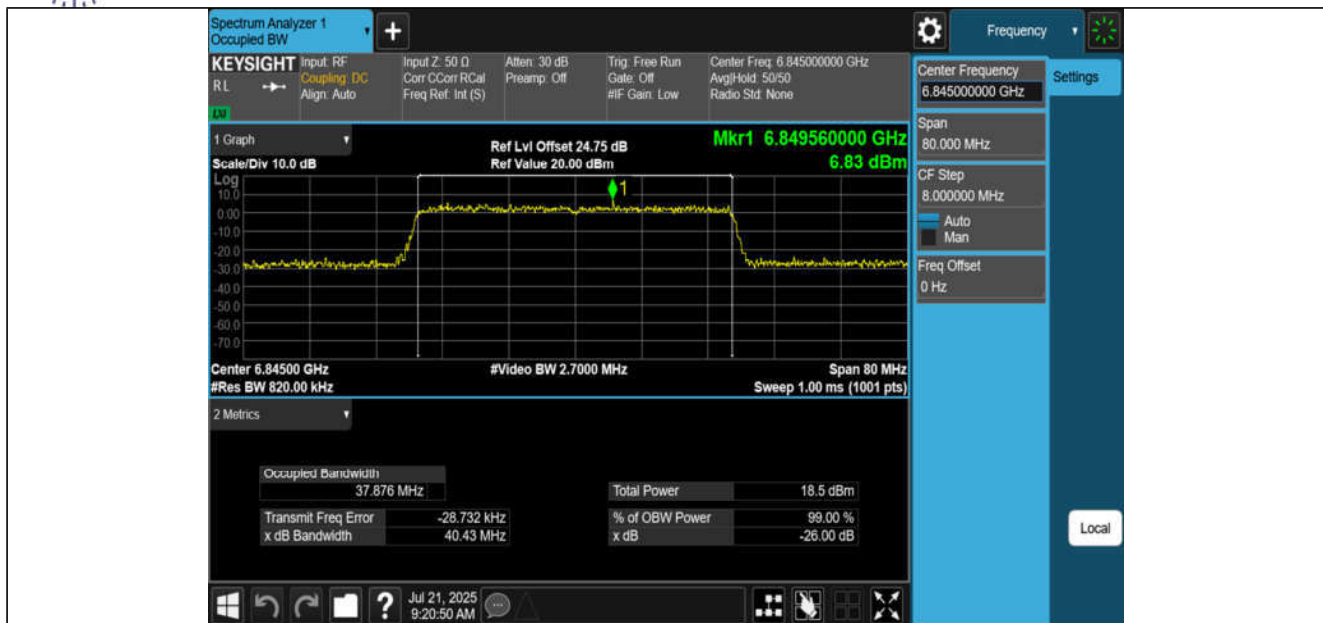
11AX40MIMO-Ant3-6845-PASS
