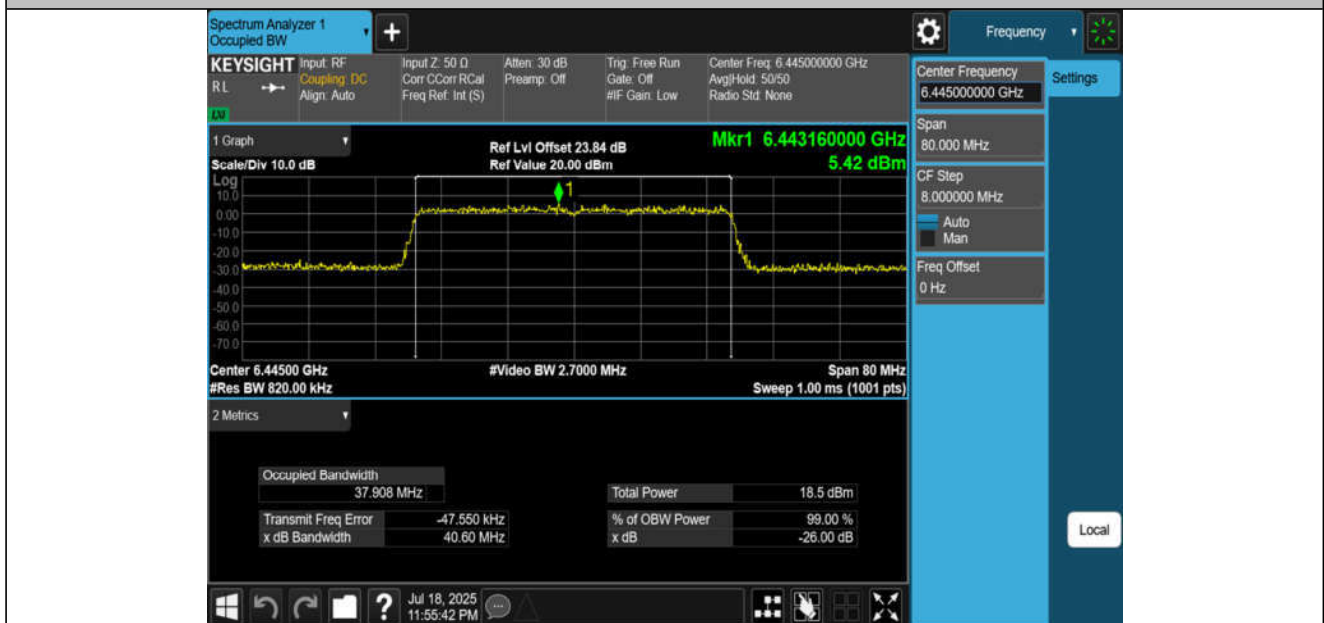
11AX40MIMO-Ant2-6445-PASS
