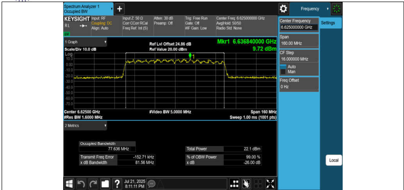
11AX80MIMO-Ant3-6625-PASS
