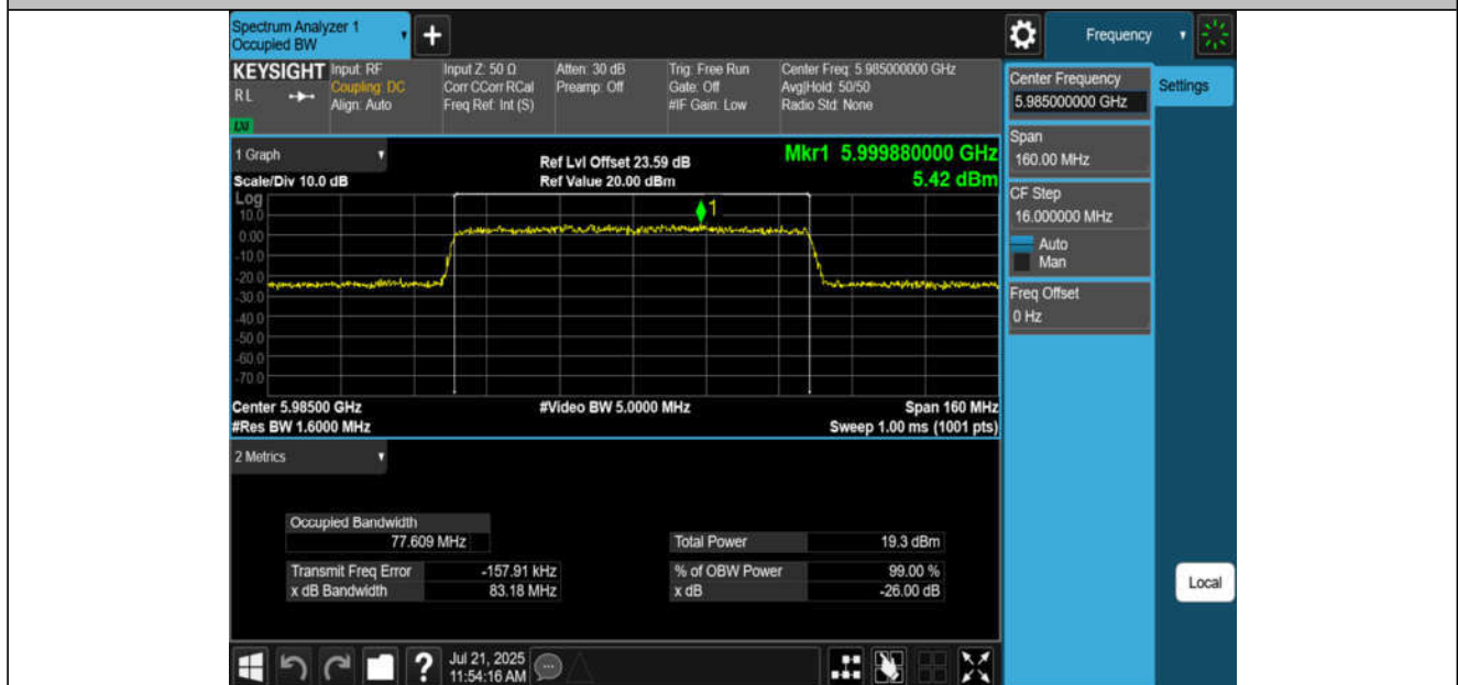
11AX80MIMO-Ant2-5985-PASS
