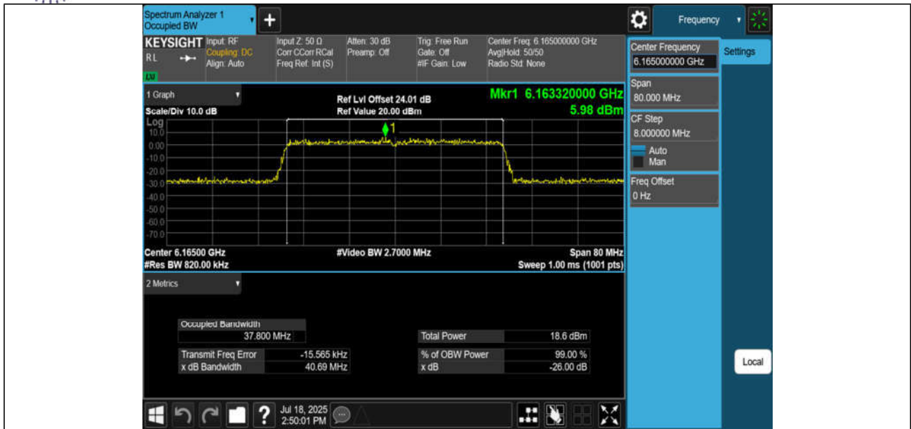
11AX40MIMO-Ant3-6165-PASS
