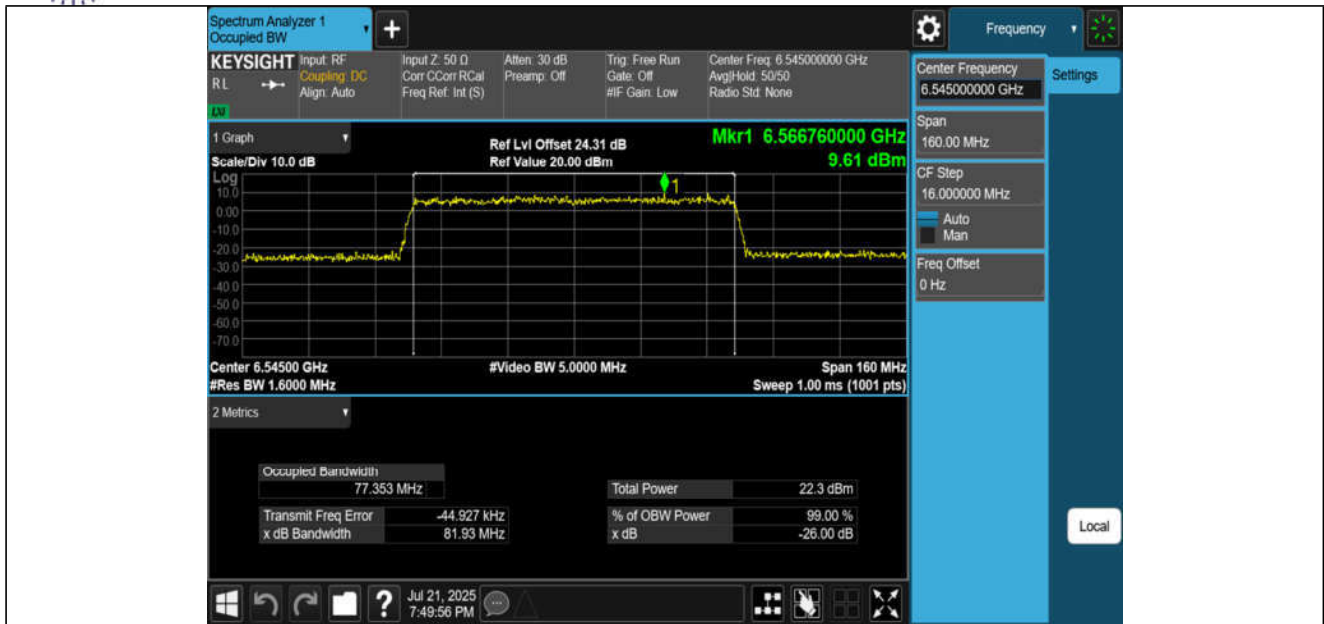
11AX80MIMO-Ant1-6545-PASS
