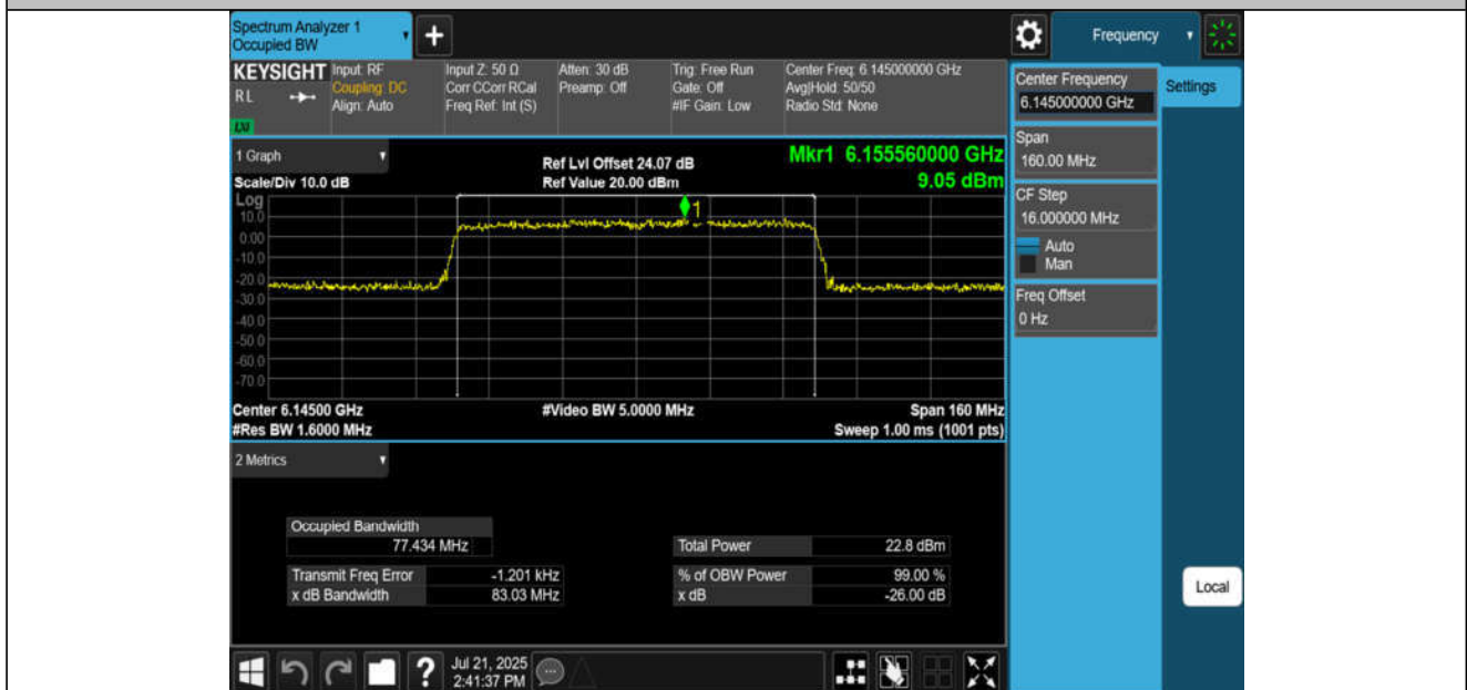
11AX80MIMO-Ant4-6145-PASS
