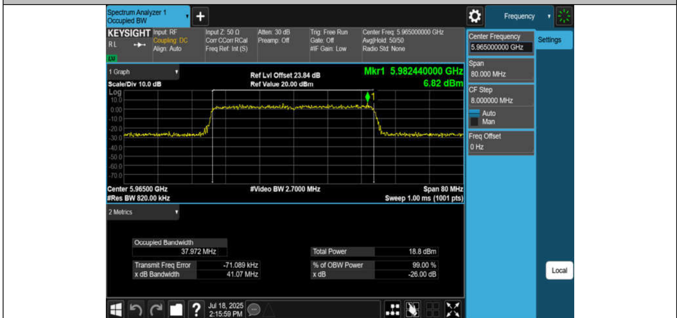
11AX40MIMO-Ant4-5965-PASS
