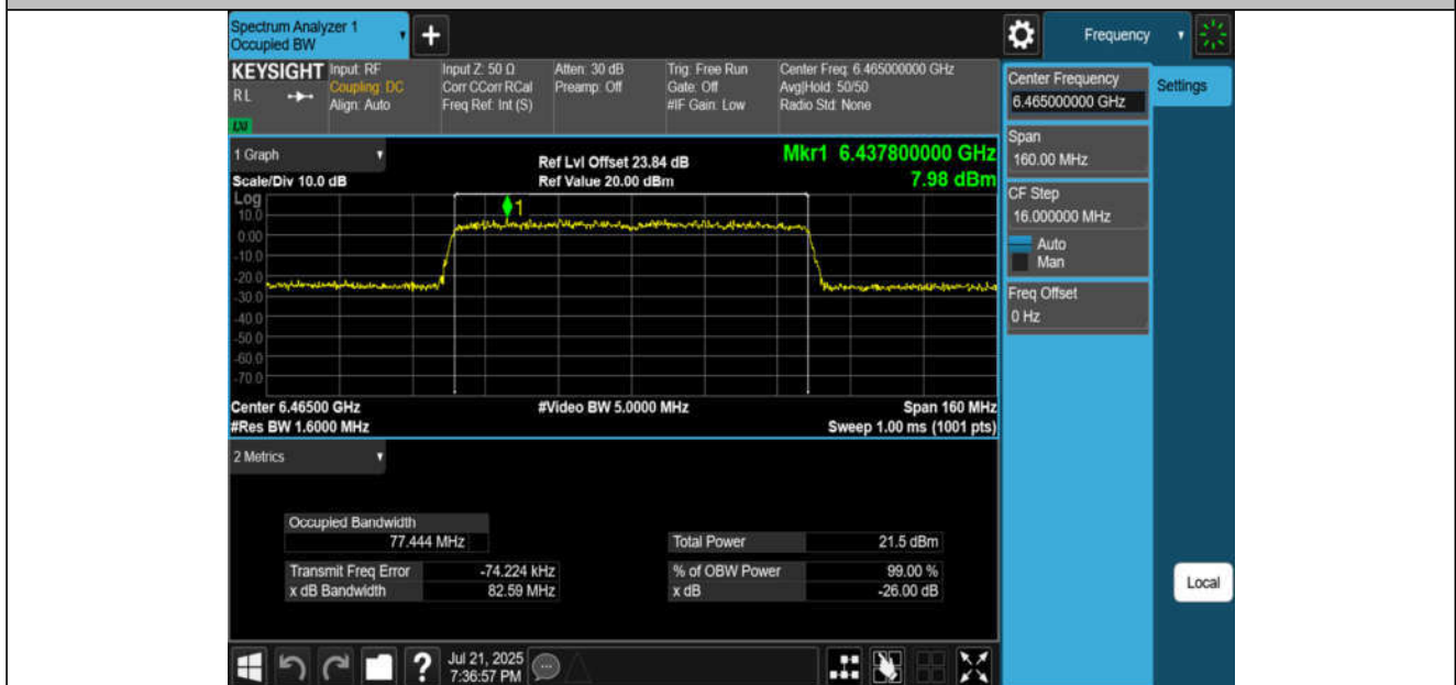
11AX80MIMO-Ant2-6465-PASS
