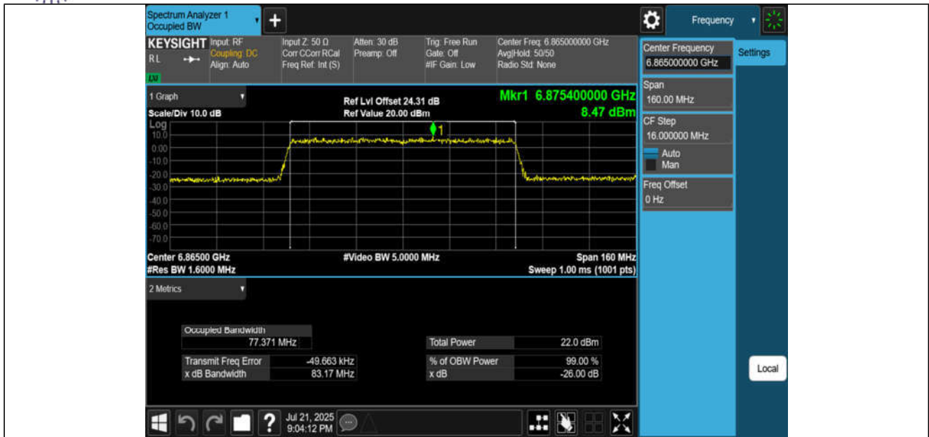
11AX80MIMO-Ant1-6865-PASS
