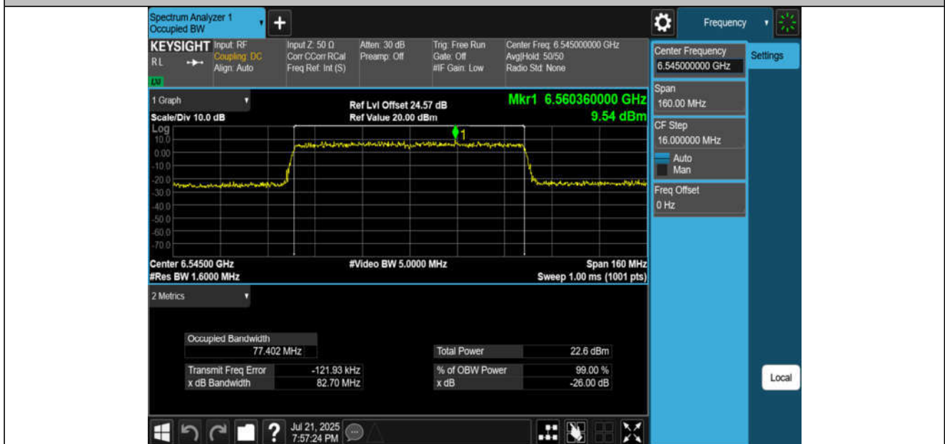
11AX80MIMO-Ant4-6545-PASS
