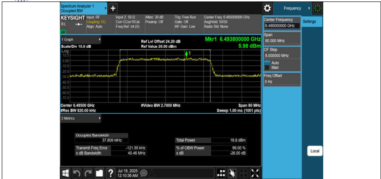
11AX40MIMO-Ant3-6485-PASS
