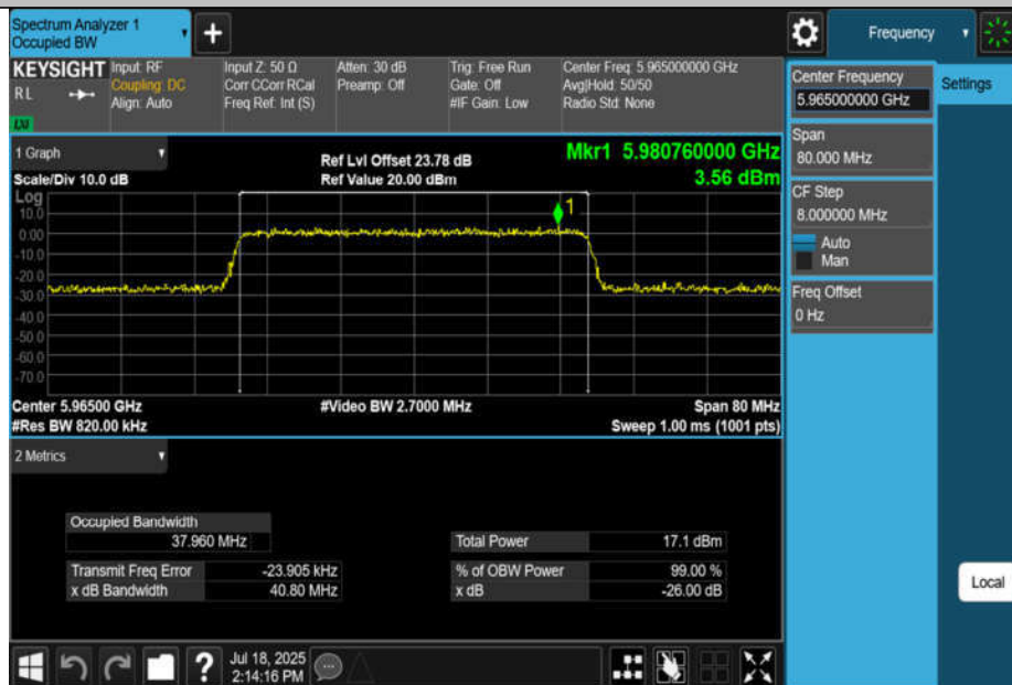
11AX40MIMO-Ant2-5965-PASS
