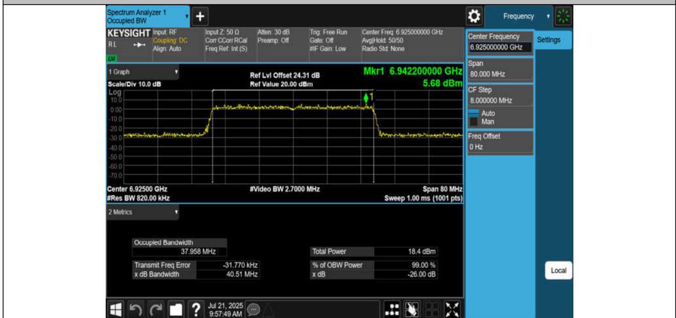
11AX40MIMO-Ant2-6925-PASS
