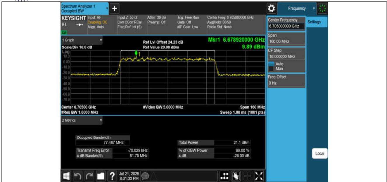
11AX80MIMO-Ant3-6705-PASS
