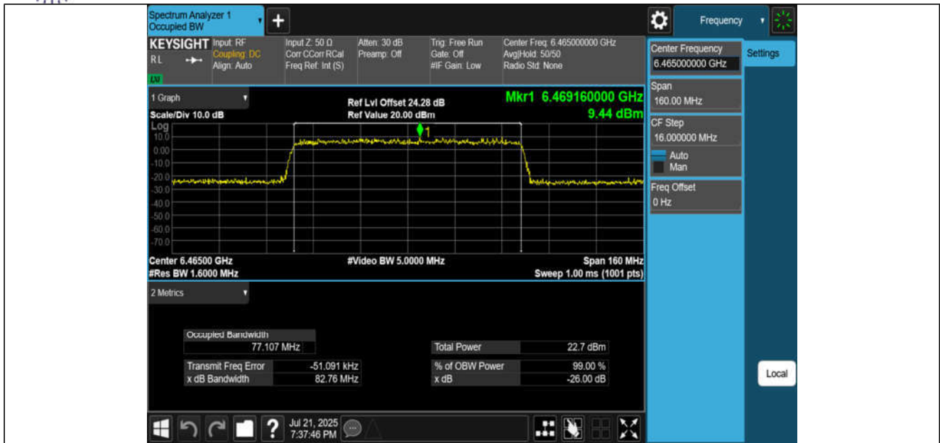
11AX80MIMO-Ant3-6465-PASS
