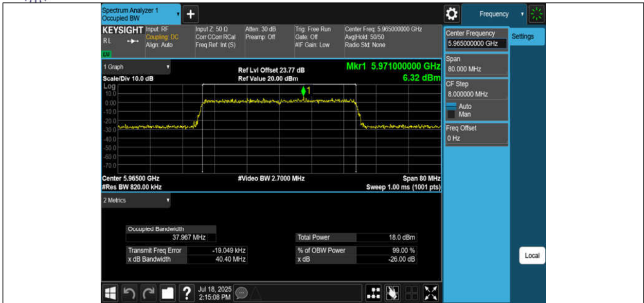
11AX40MIMO-Ant3-5965-PASS
