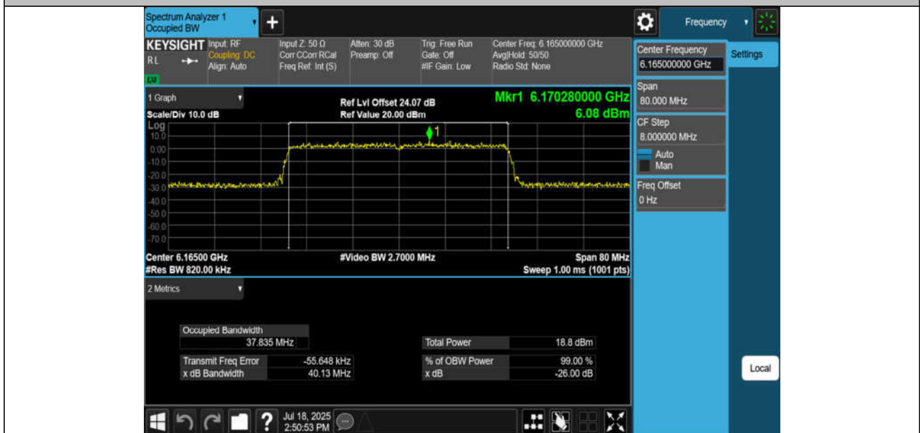
11AX40MIMO-Ant4-6165-PASS
