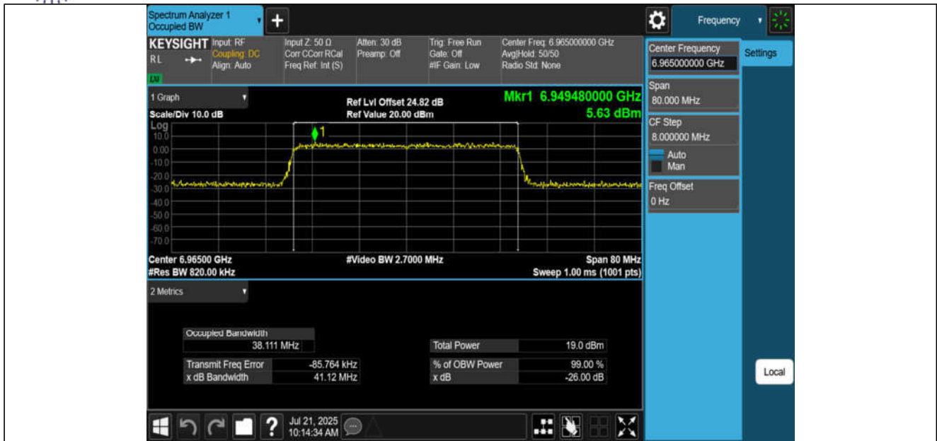
11AX40MIMO-Ant1-6965-PASS
