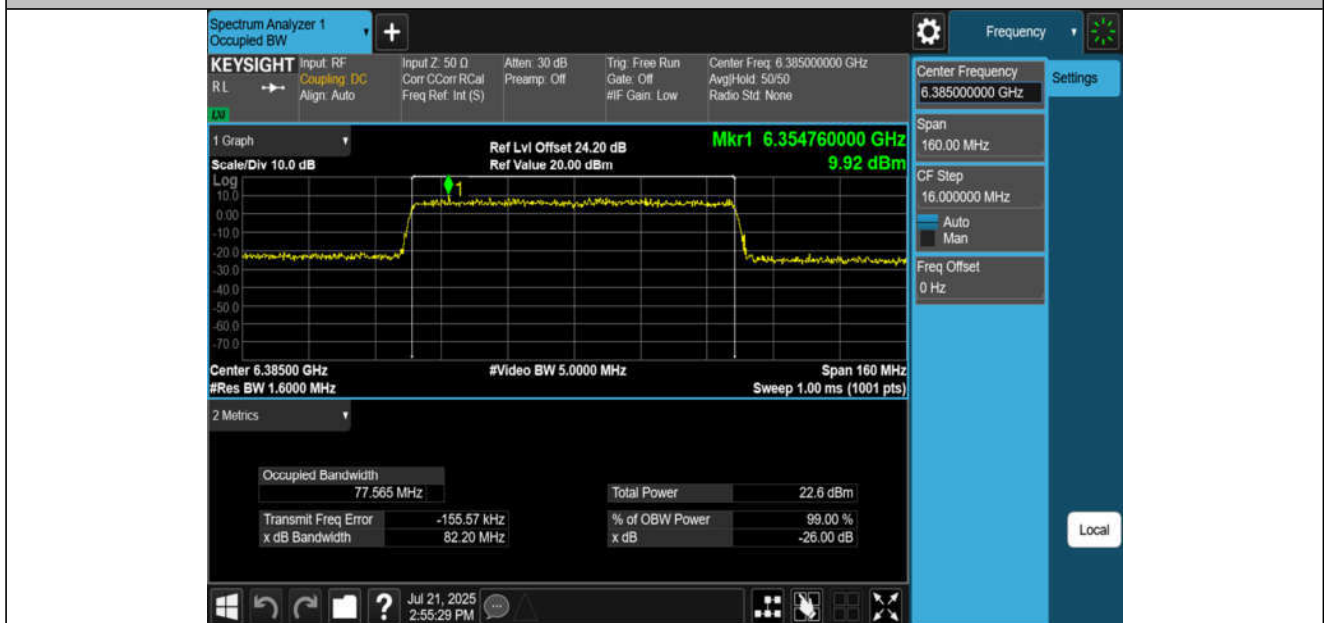
11AX80MIMO-Ant4-6385-PASS
