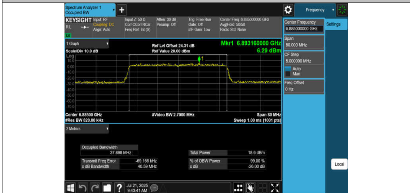
11AX40MIMO-Ant2-6885-PASS
