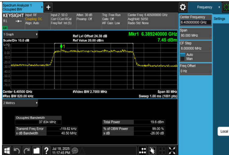
11AX40MIMO-Ant3-6405-PASS
