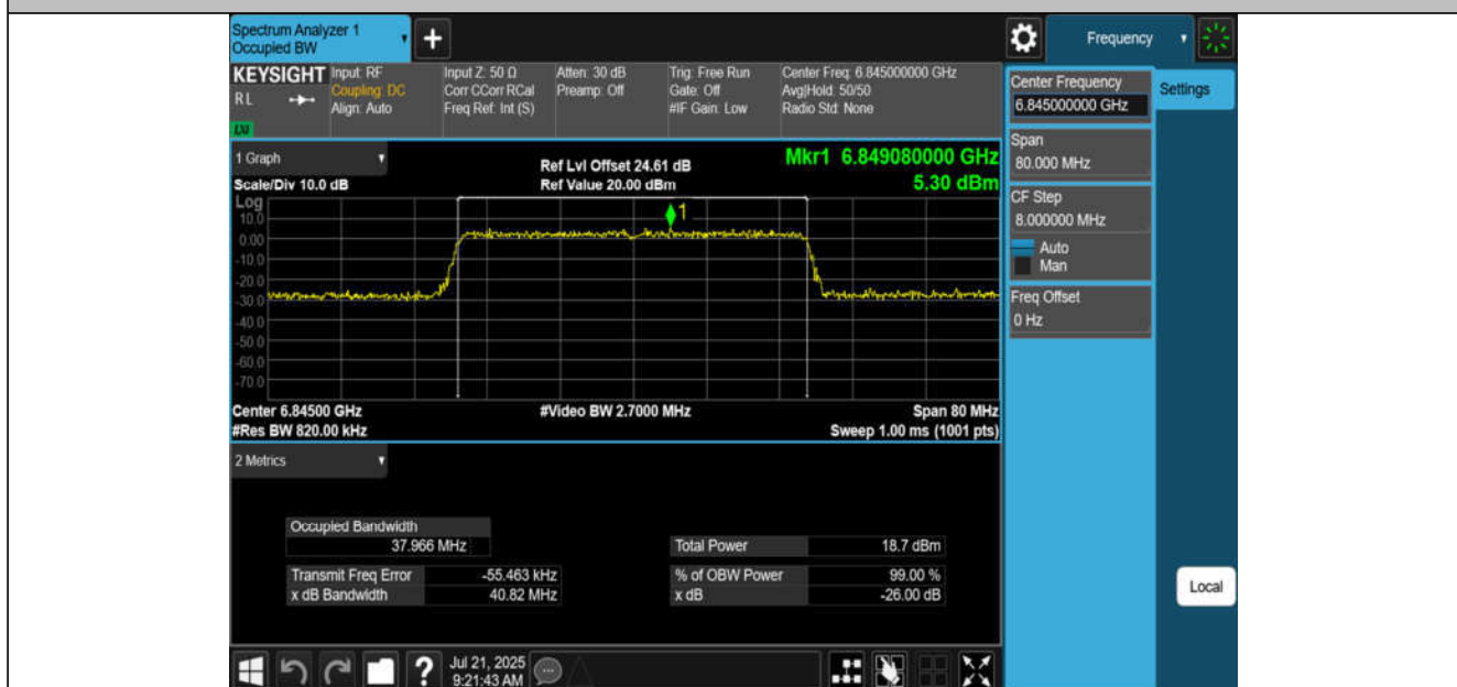
11AX40MIMO-Ant4-6845-PASS
