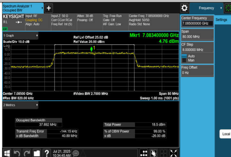
11AX40MIMO-Ant4-7085-PASS
