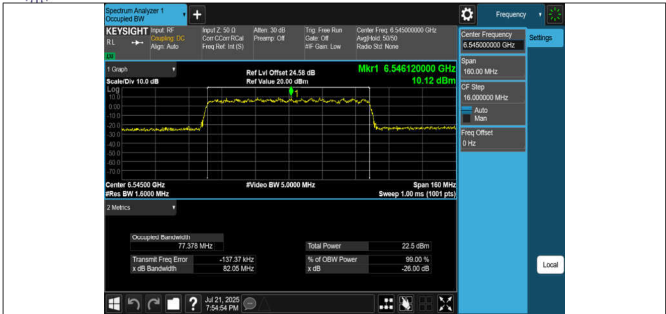
11AX80MIMO-Ant3-6545-PASS
