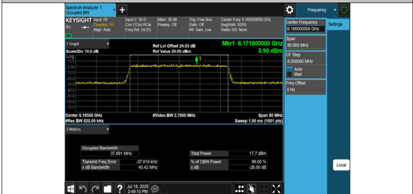
11AX40MIMO-Ant2-6165-PASS
