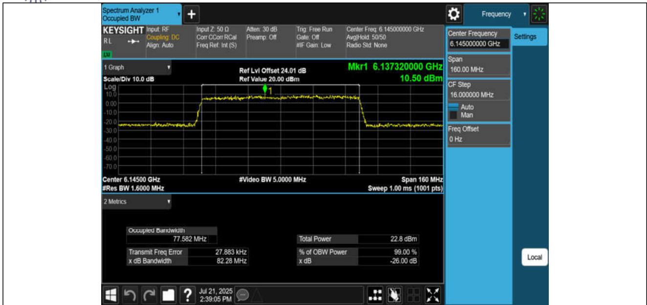
11AX80MIMO-Ant3-6145-PASS
