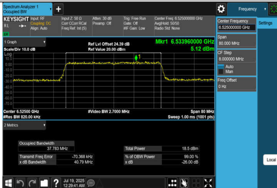
11AX40MIMO-Ant2-6525-PASS
