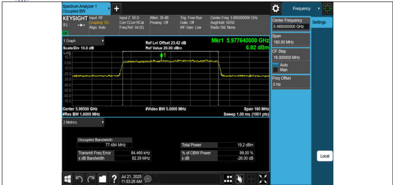
11AX80MIMO-Ant1-5985-PASS
