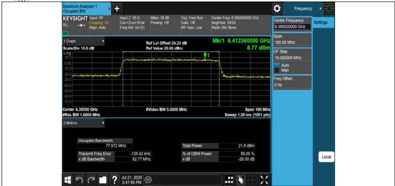
11AX80MIMO-Ant1-6385-PASS
