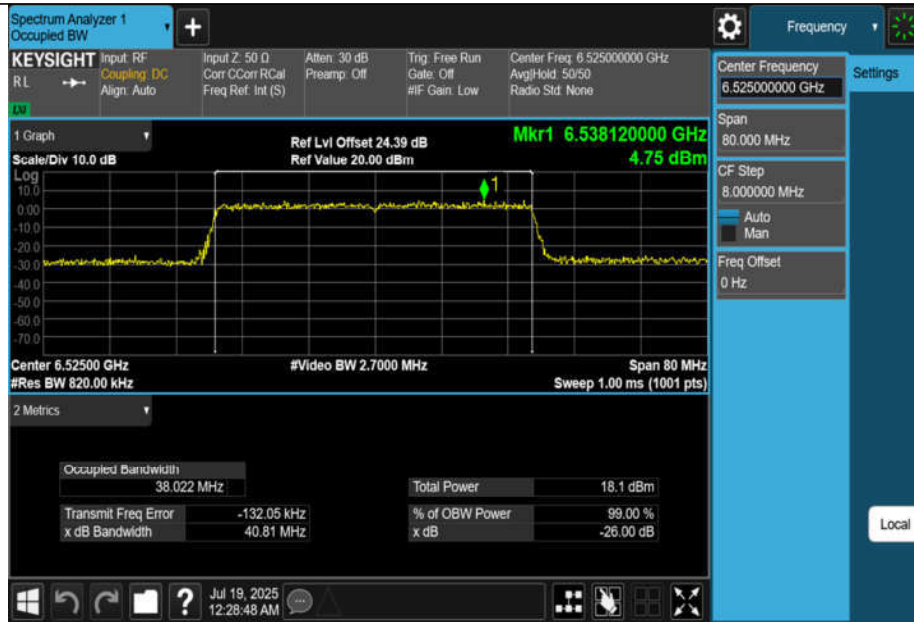
11AX40MIMO-Ant1-6525-PASS
