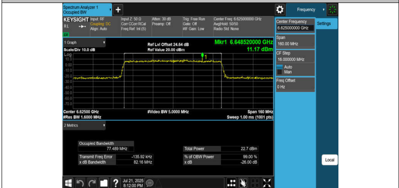
11AX80MIMO-Ant4-6625-PASS
