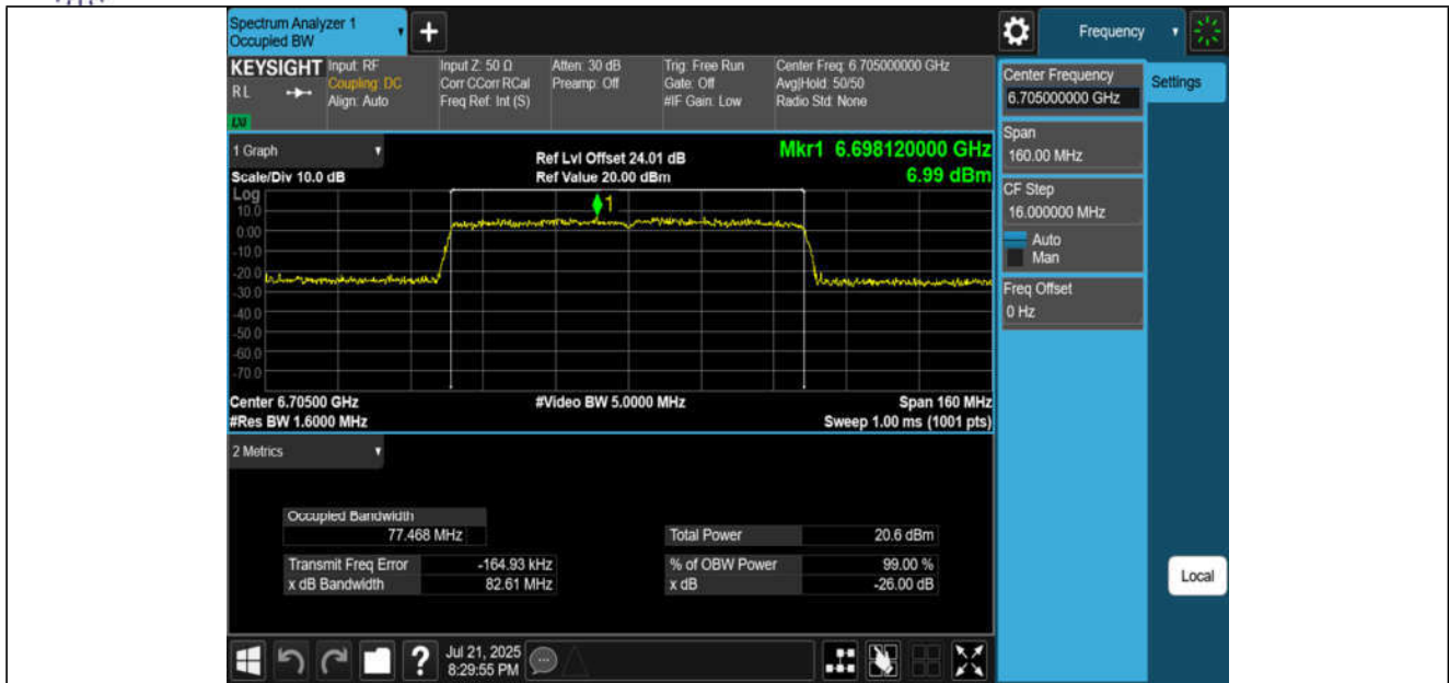
11AX80MIMO-Ant1-6705-PASS
