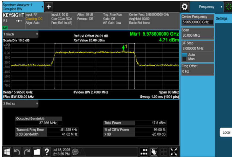
11AX40MIMO-Ant1-5965-PASS
