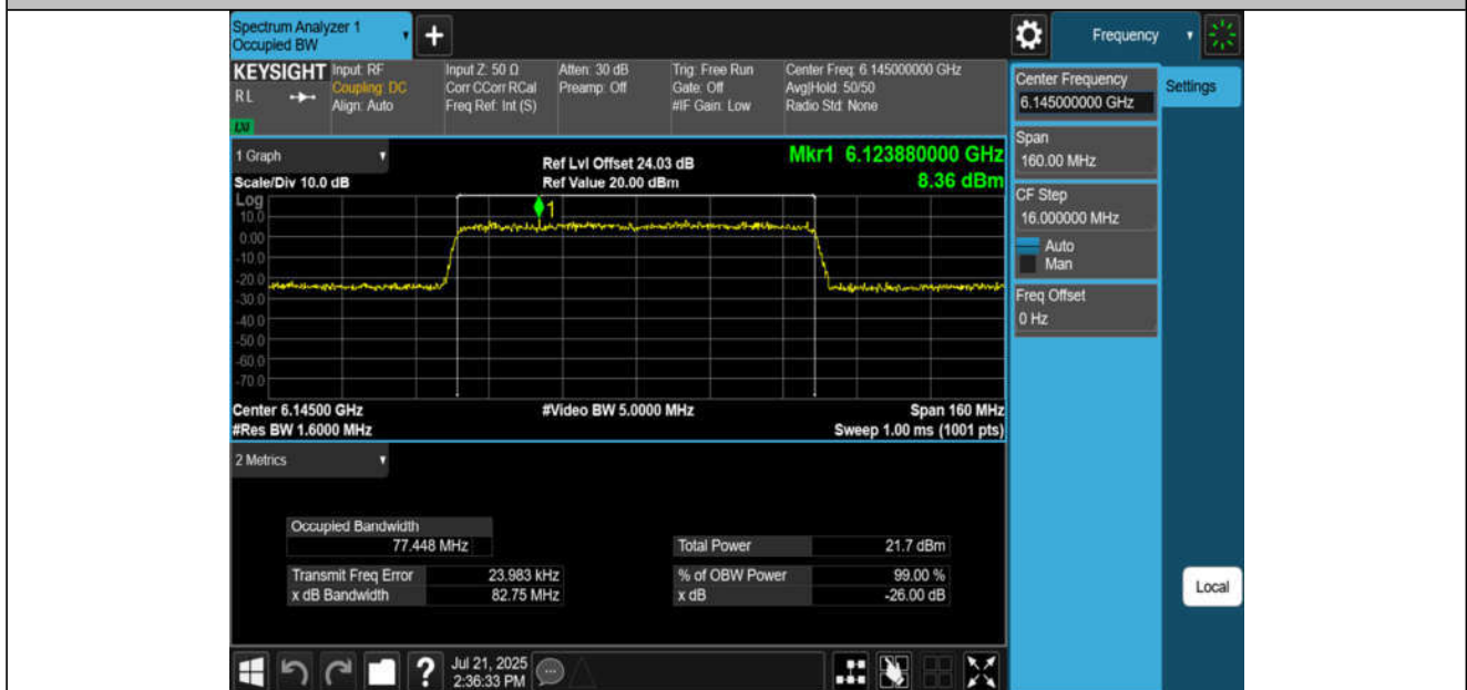
11AX80MIMO-Ant2-6145-PASS
