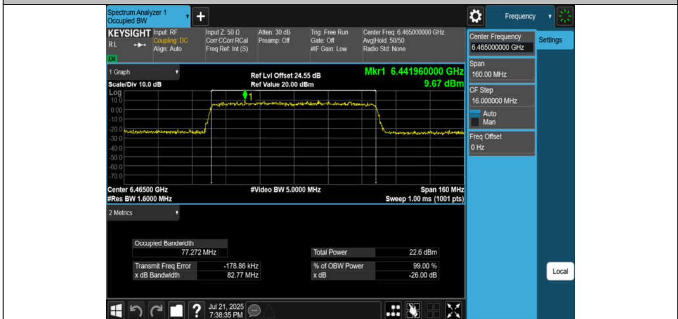
11AX80MIMO-Ant4-6465-PASS
