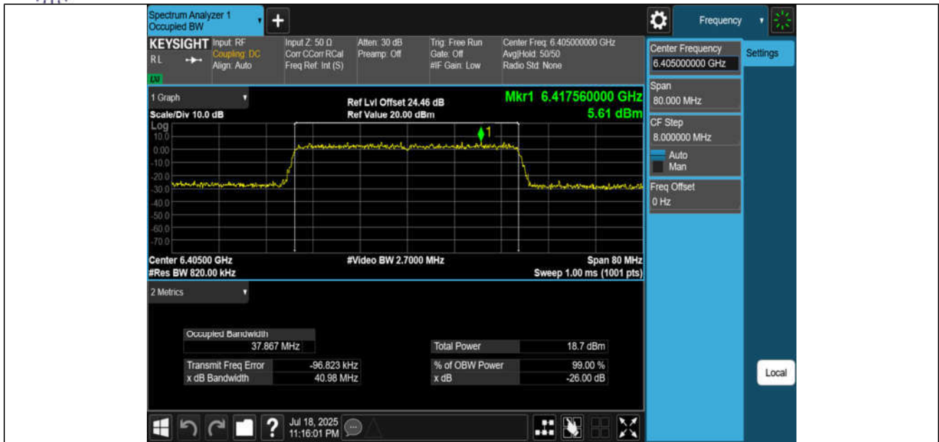
11AX40MIMO-Ant1-6405-PASS
