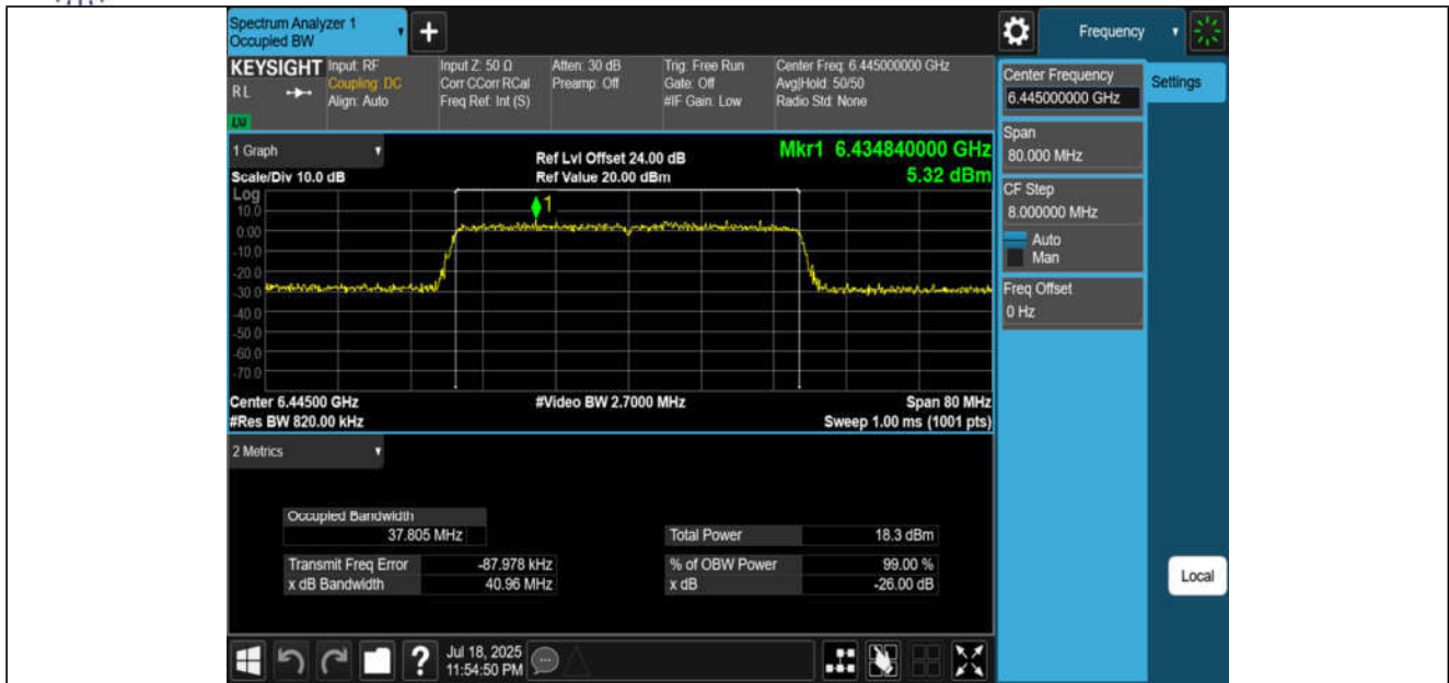
11AX40MIMO-Ant1-6445-PASS
