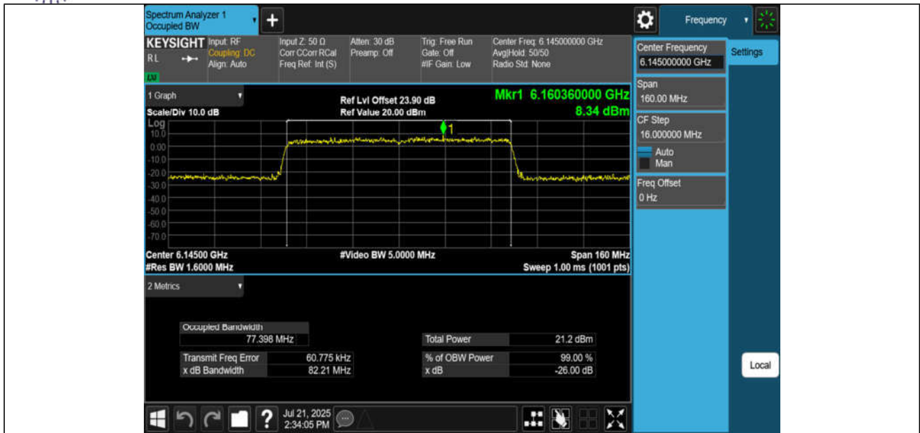
11AX80MIMO-Ant1-6145-PASS
