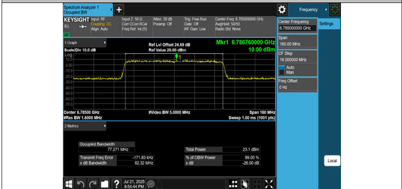
11AX80MIMO-Ant4-6785-PASS
