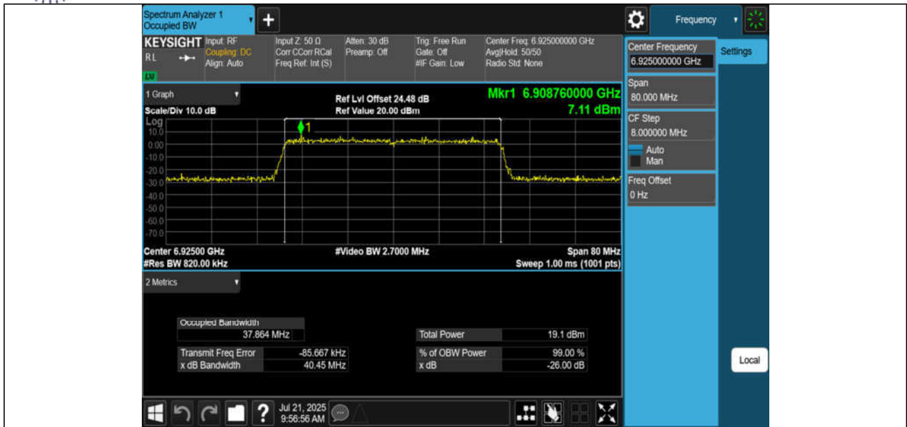
11AX40MIMO-Ant1-6925-PASS
