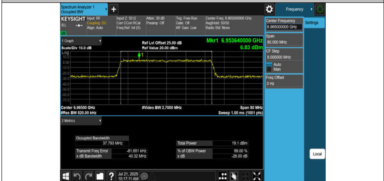
11AX40MIMO-Ant4-6965-PASS
