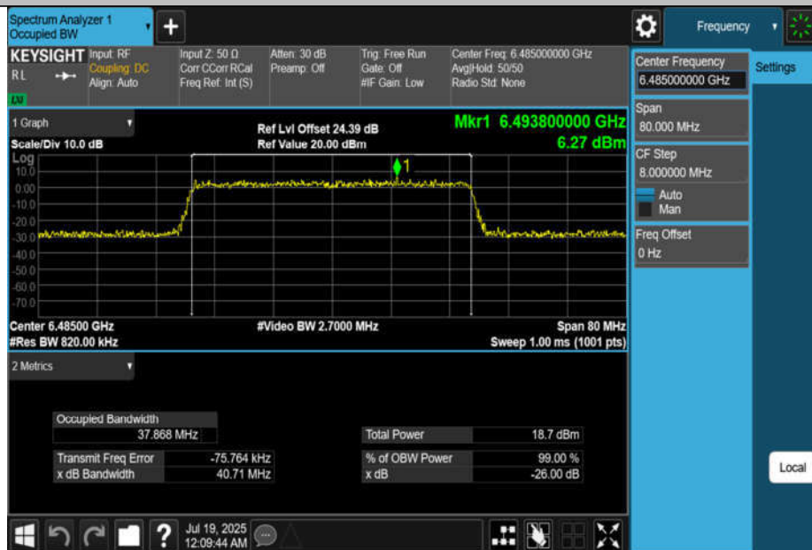
11AX40MIMO-Ant2-6485-PASS
