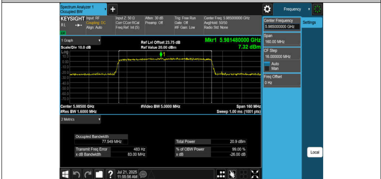
11AX80MIMO-Ant4-5985-PASS
