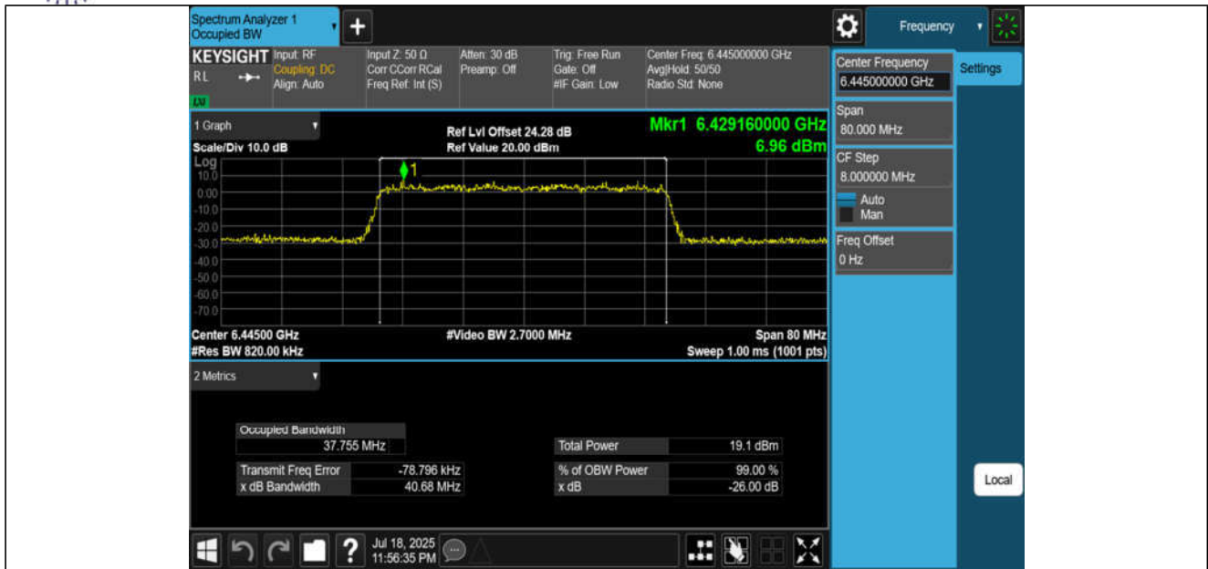
11AX40MIMO-Ant3-6445-PASS
