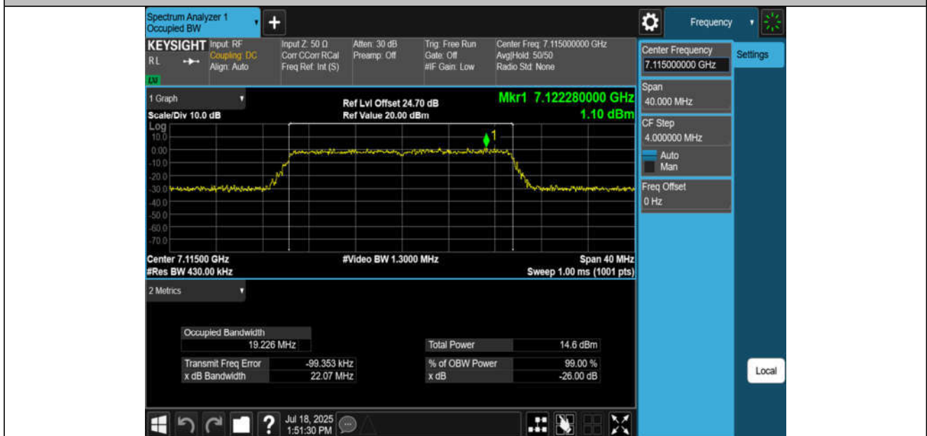
11AX20MIMO-Ant2-7115-PASS
