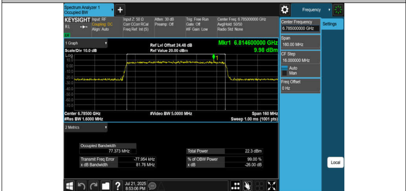
11AX80MIMO-Ant2-6785-PASS
