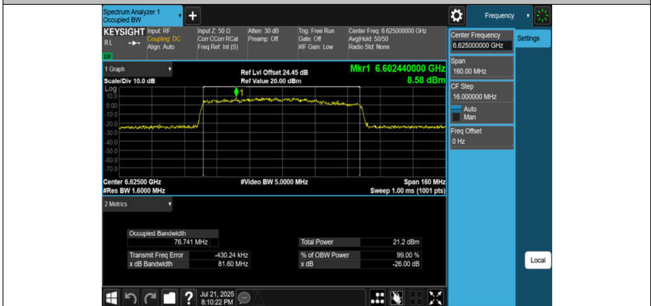
11AX80MIMO-Ant2-6625-PASS
