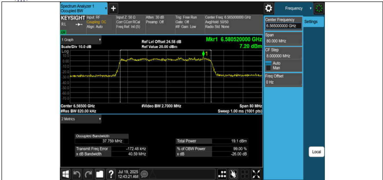
11AX40MIMO-Ant3-6565-PASS
