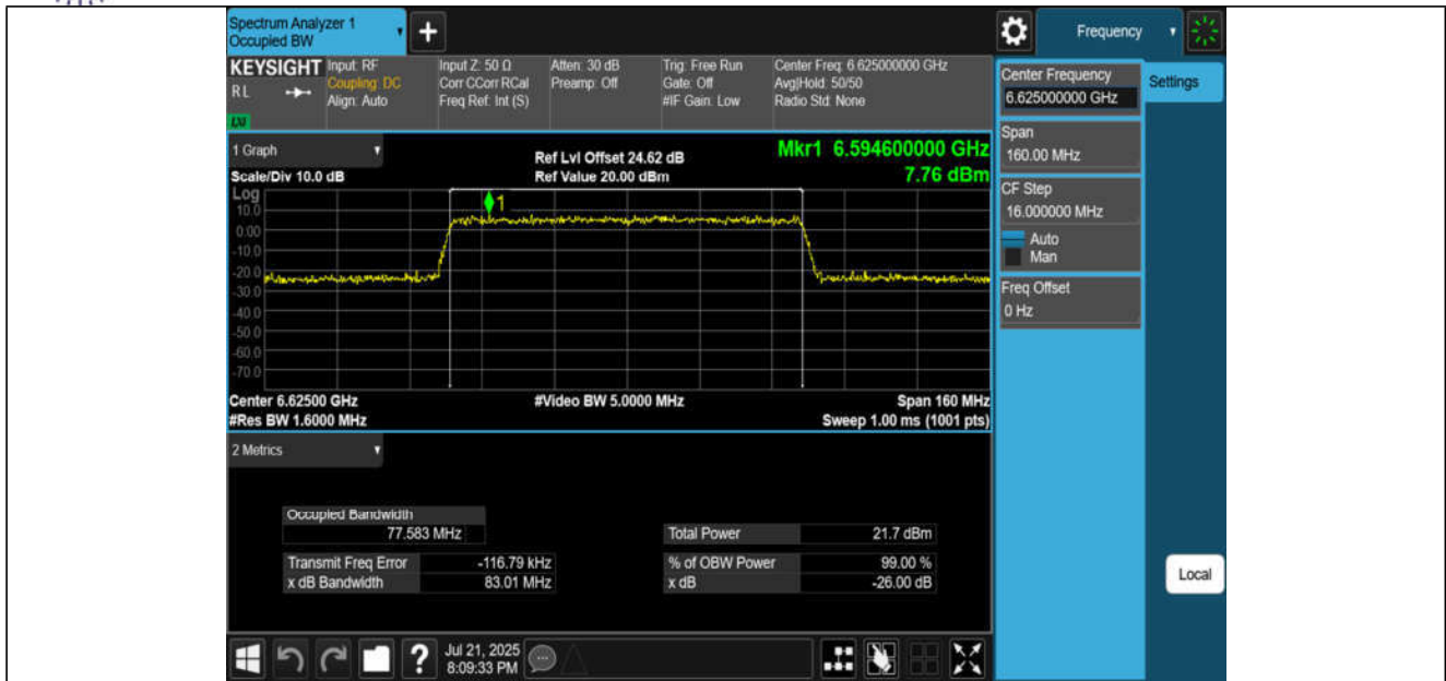
11AX80MIMO-Ant1-6625-PASS
