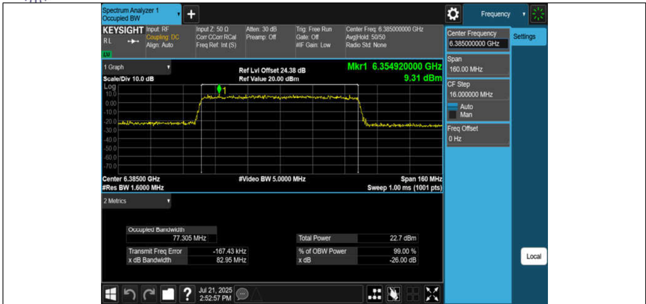
11AX80MIMO-Ant3-6385-PASS
