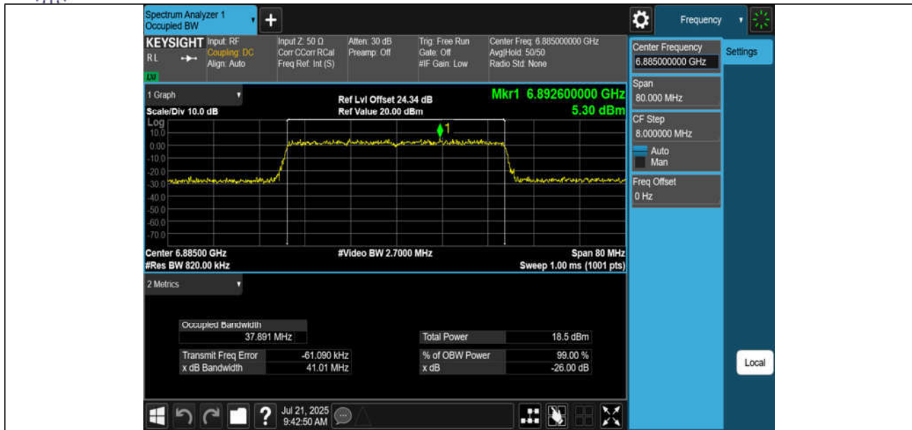
11AX40MIMO-Ant1-6885-PASS
