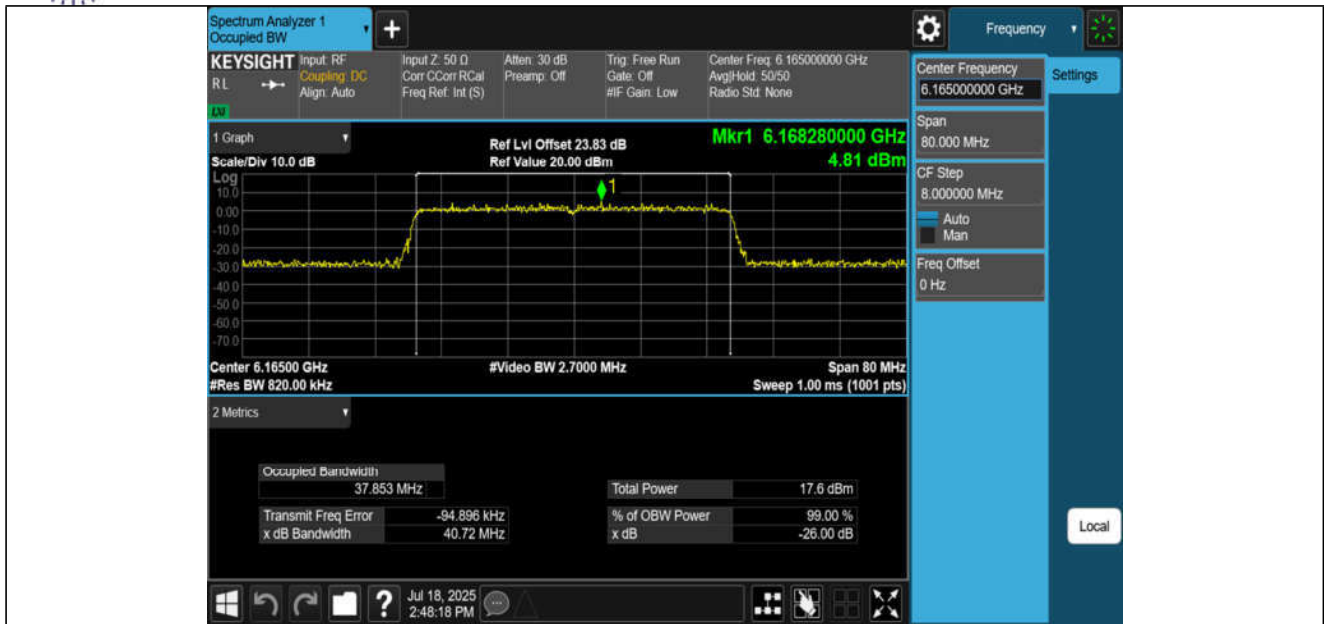
11AX40MIMO-Ant1-6165-PASS
