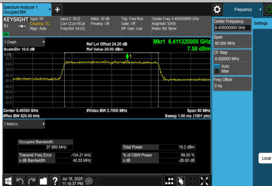
11AX40MIMO-Ant4-6405-PASS
