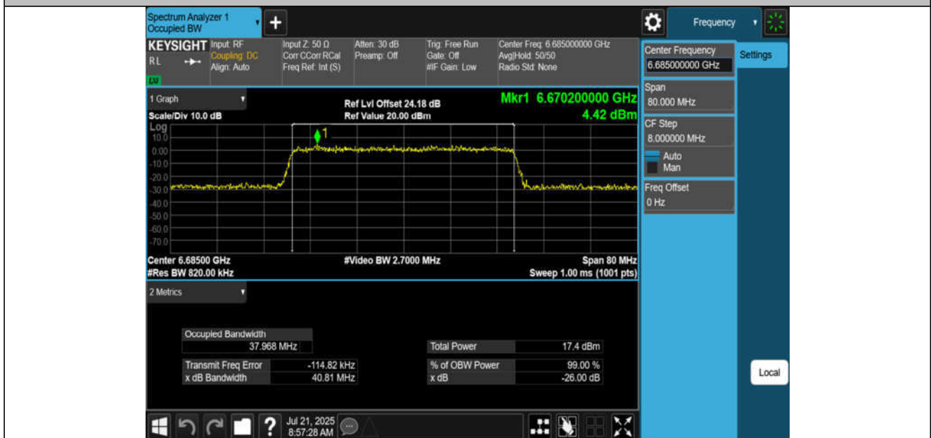
11AX40MIMO-Ant2-6685-PASS
