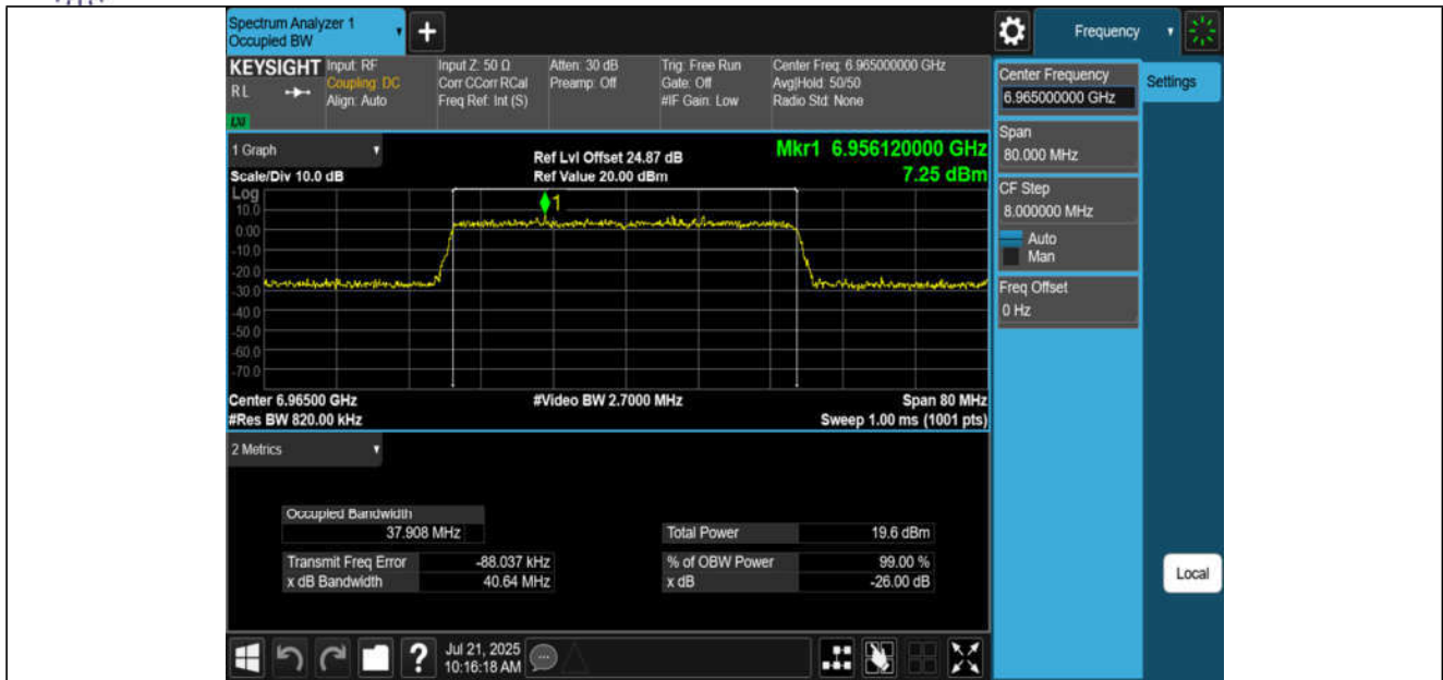
11AX40MIMO-Ant3-6965-PASS
