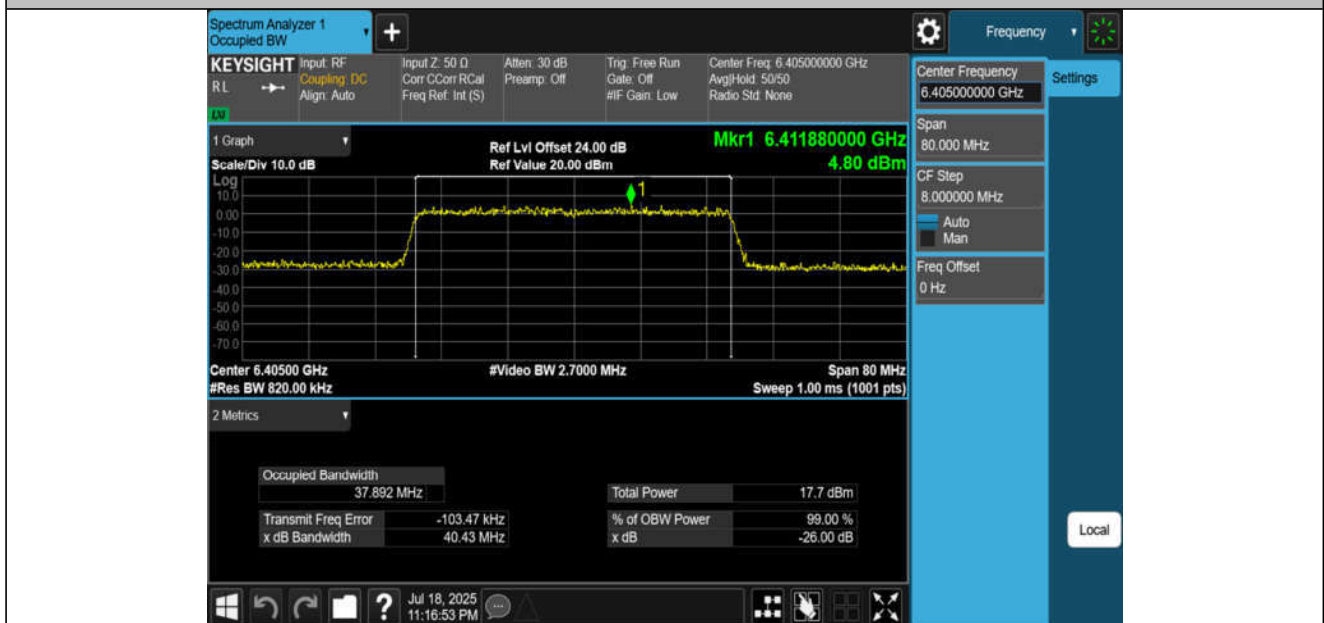
11AX40MIMO-Ant2-6405-PASS
