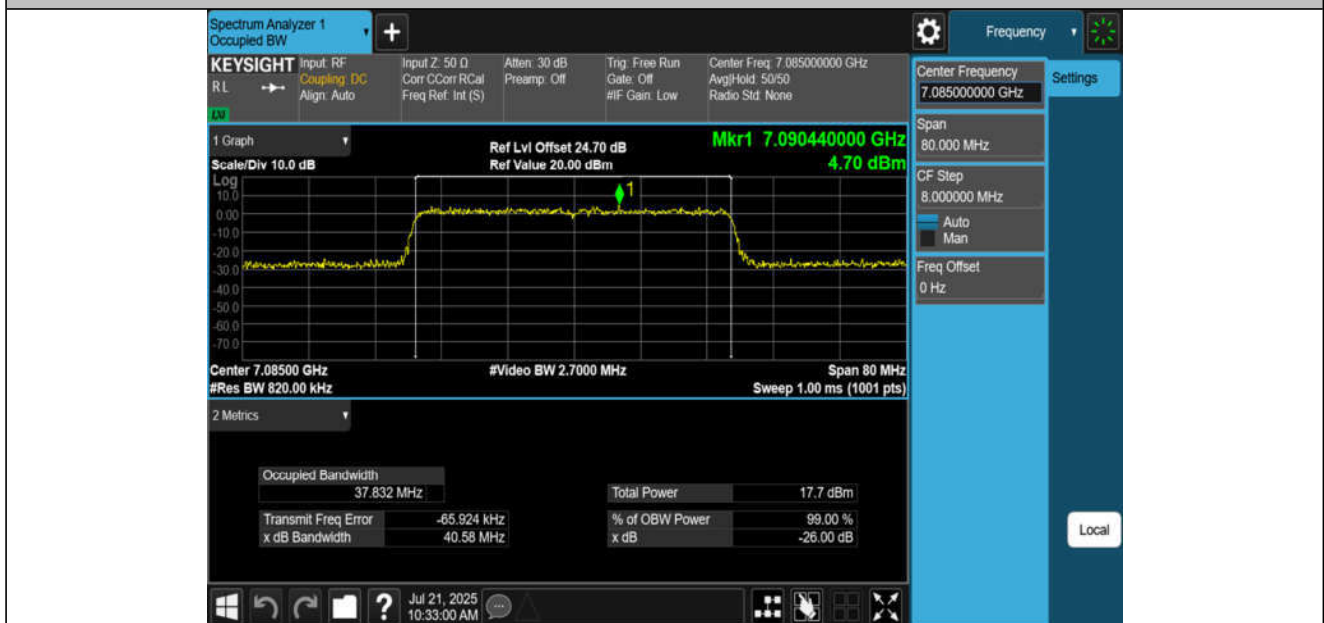
11AX40MIMO-Ant2-7085-PASS
