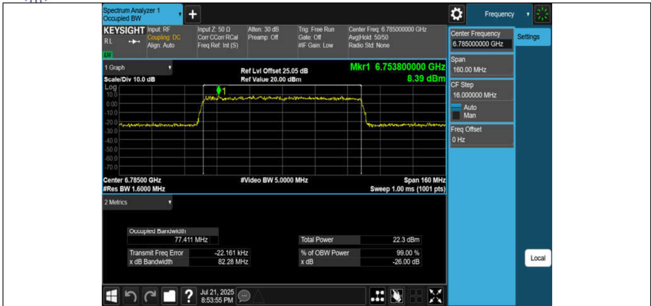
11AX80MIMO-Ant3-6785-PASS
