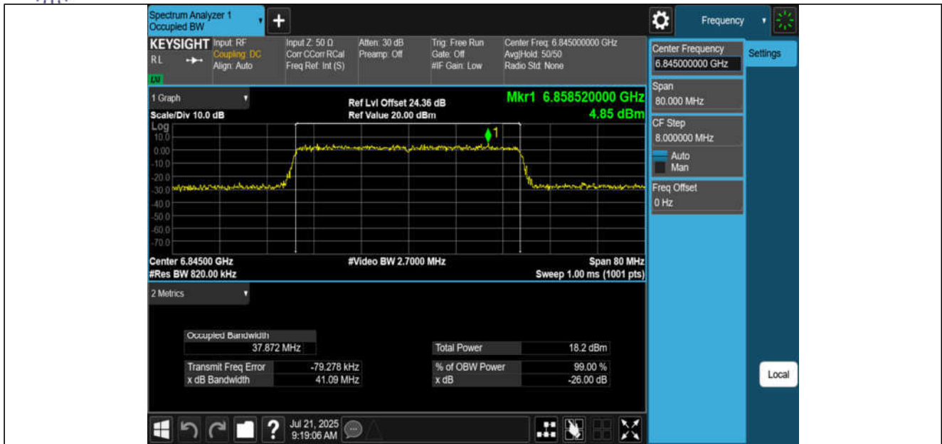
11AX40MIMO-Ant1-6845-PASS
