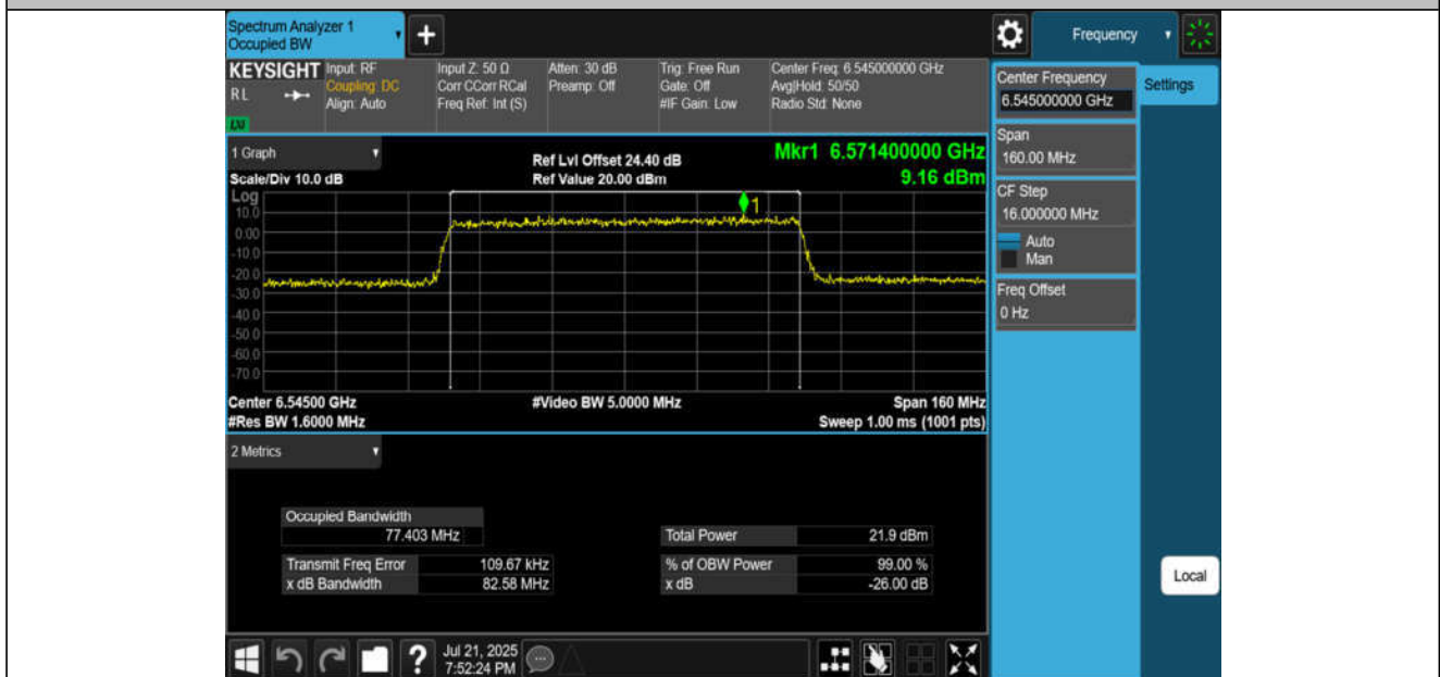
11AX80MIMO-Ant2-6545-PASS
