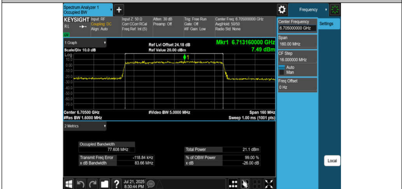
11AX80MIMO-Ant2-6705-PASS
