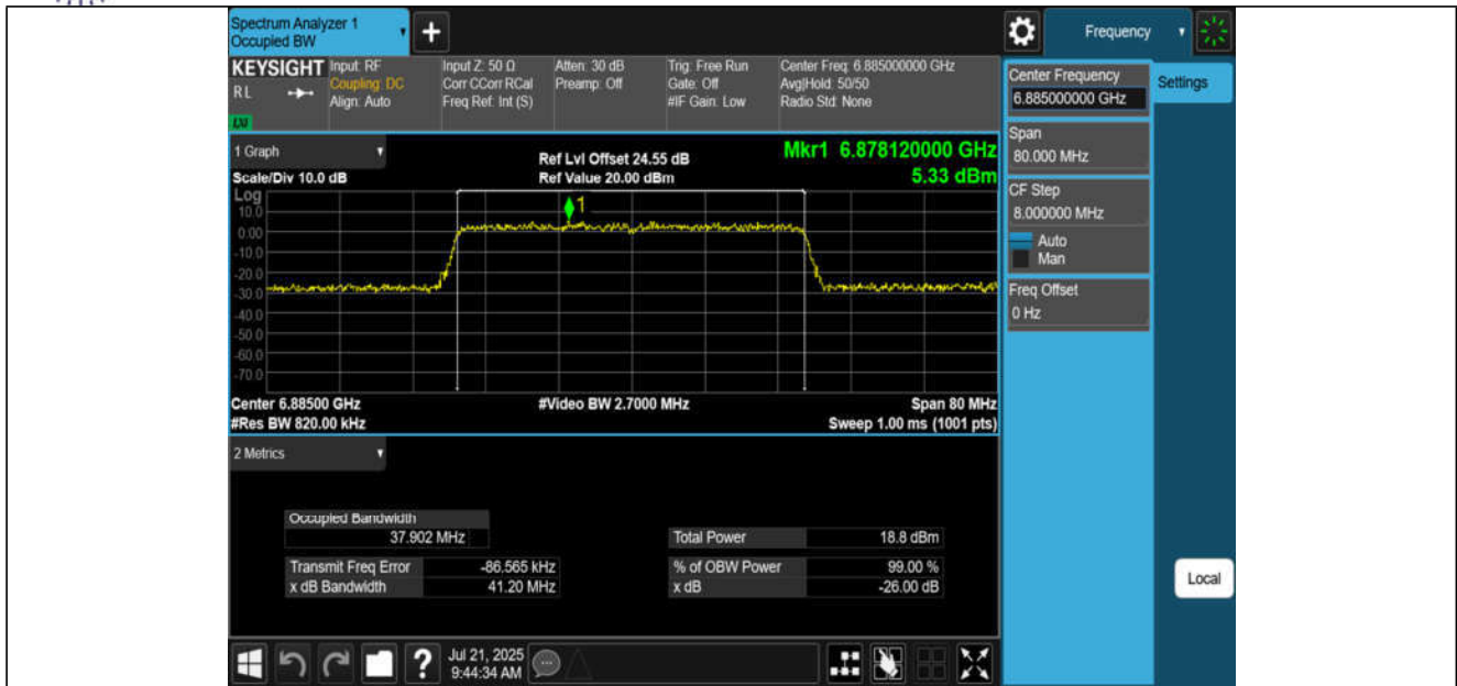
11AX40MIMO-Ant3-6885-PASS
