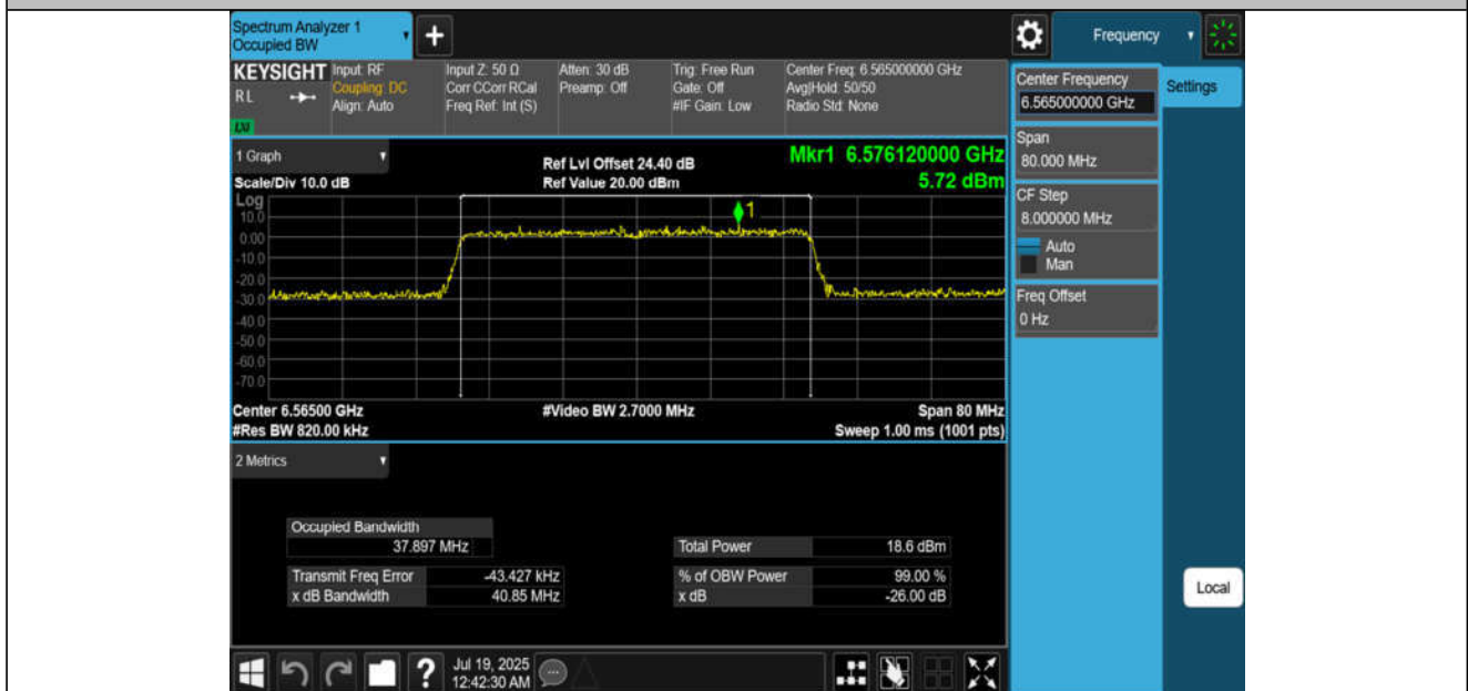
11AX40MIMO-Ant2-6565-PASS
