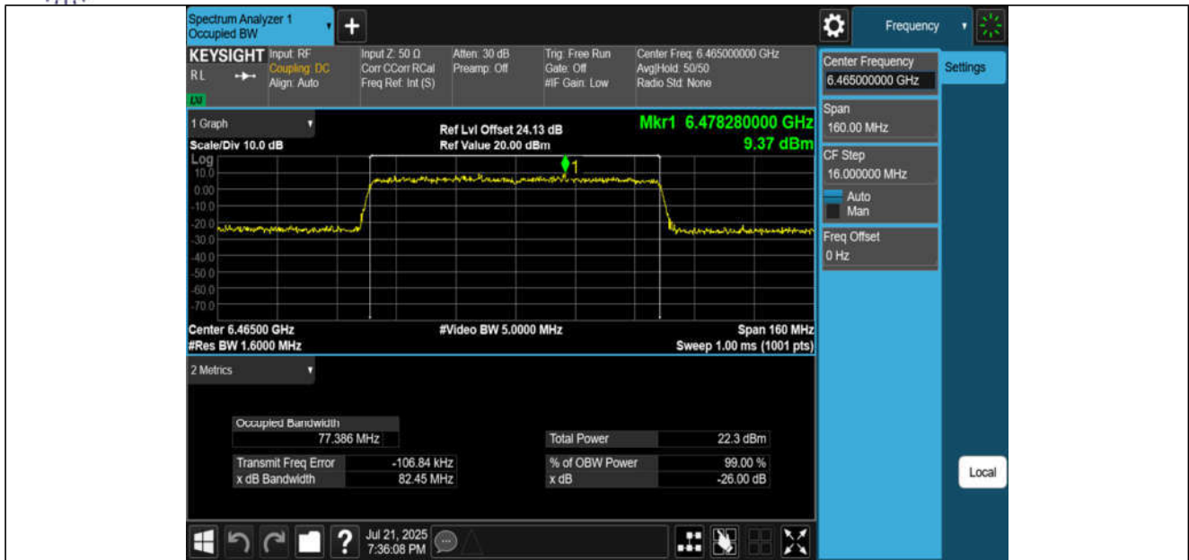
11AX80MIMO-Ant1-6465-PASS
