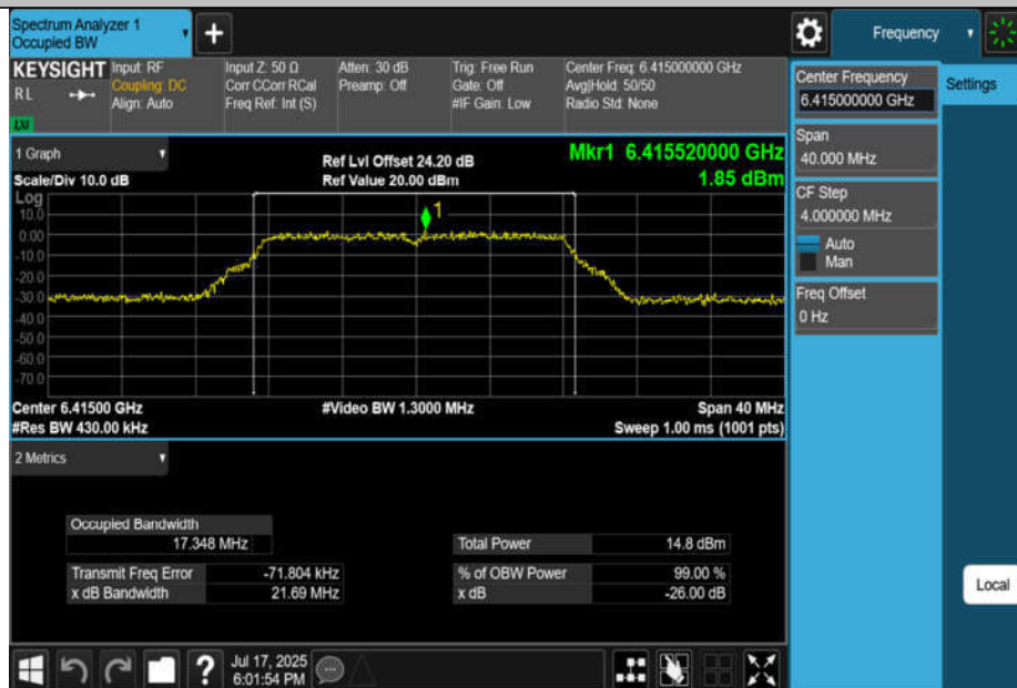
11A-CDD-Ant4-6415-PASS
