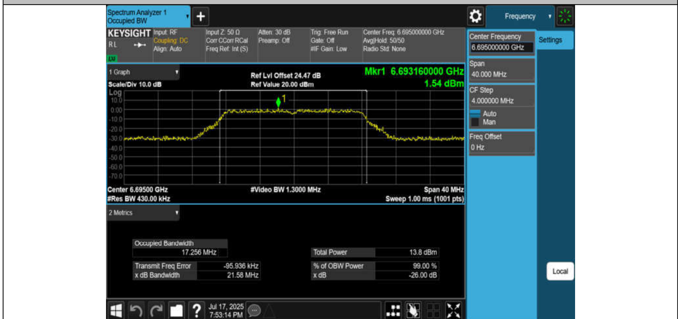
11A-CDD-Ant4-6695-PASS
