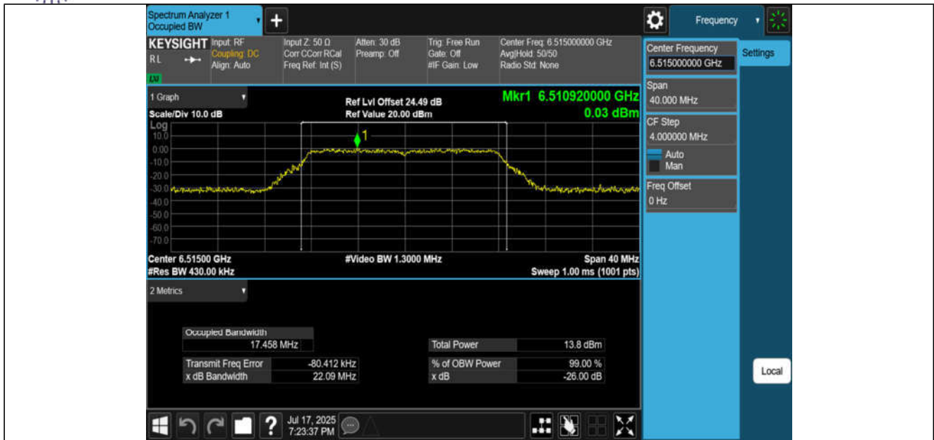
11A-CDD-Ant1-6515-PASS
