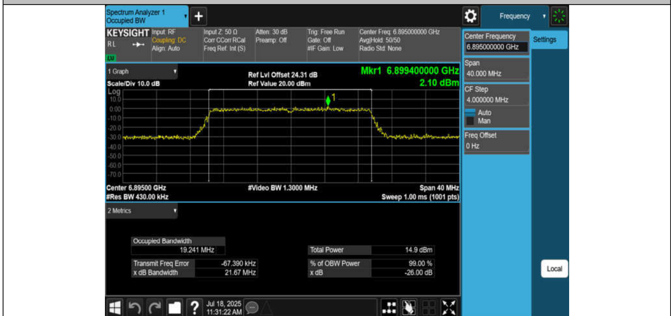
11AX20MIMO-Ant2-6895-PASS
