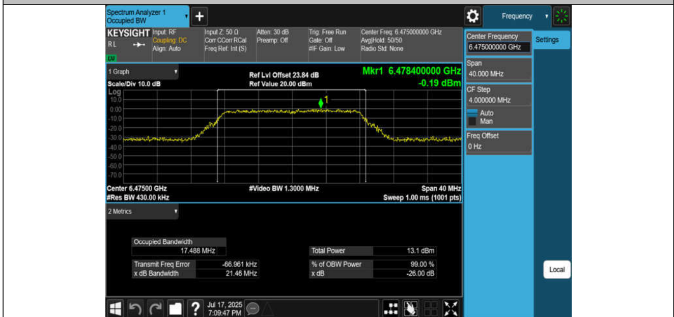
11A-CDD-Ant2-6475-PASS
