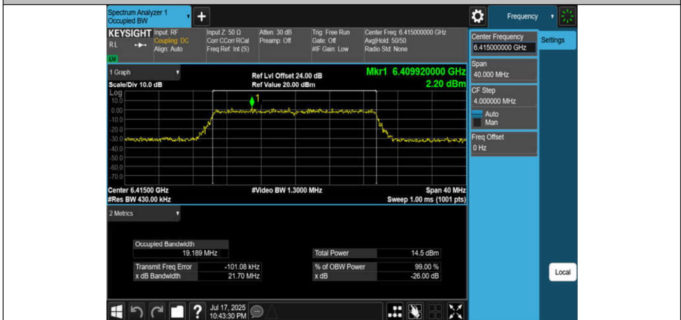
11AX20MIMO-Ant2-6415-PASS
