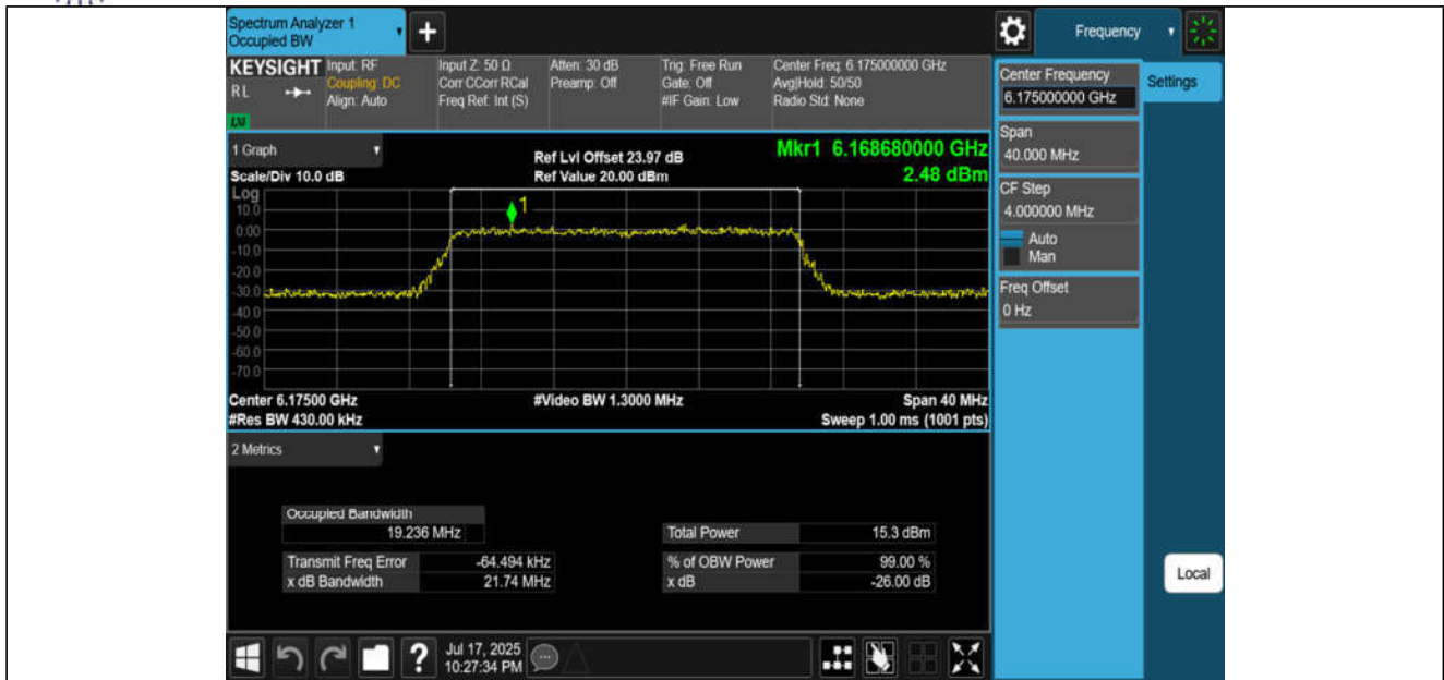
11AX20MIMO-Ant1-6175-PASS
