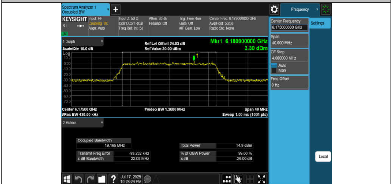
11AX20MIMO-Ant2-6175-PASS
