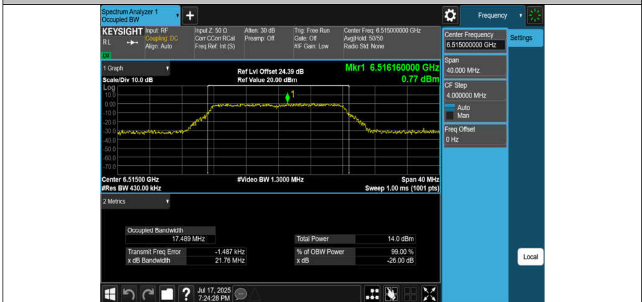
11A-CDD-Ant2-6515-PASS
