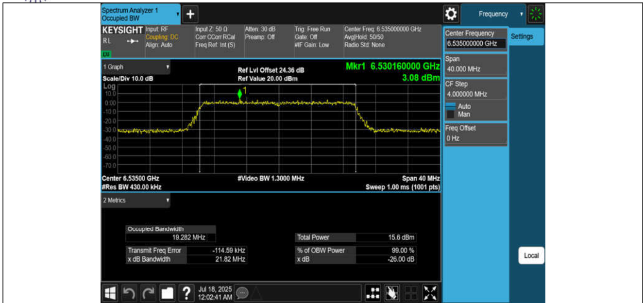
11AX20MIMO-Ant1-6535-PASS
