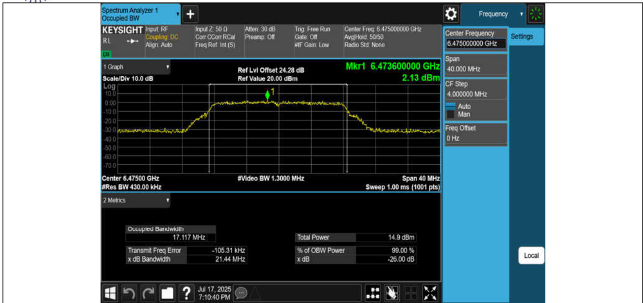
11A-CDD-Ant3-6475-PASS
