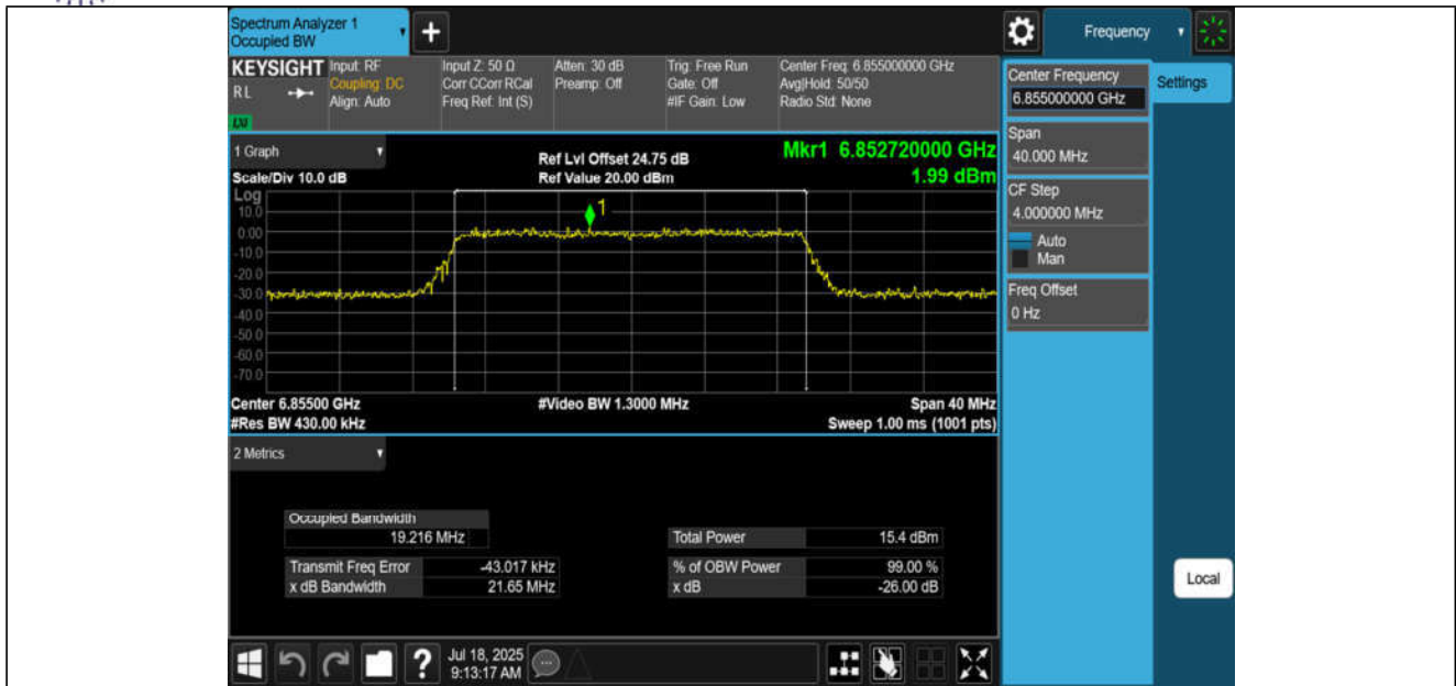
11AX20MIMO-Ant3-6855-PASS
