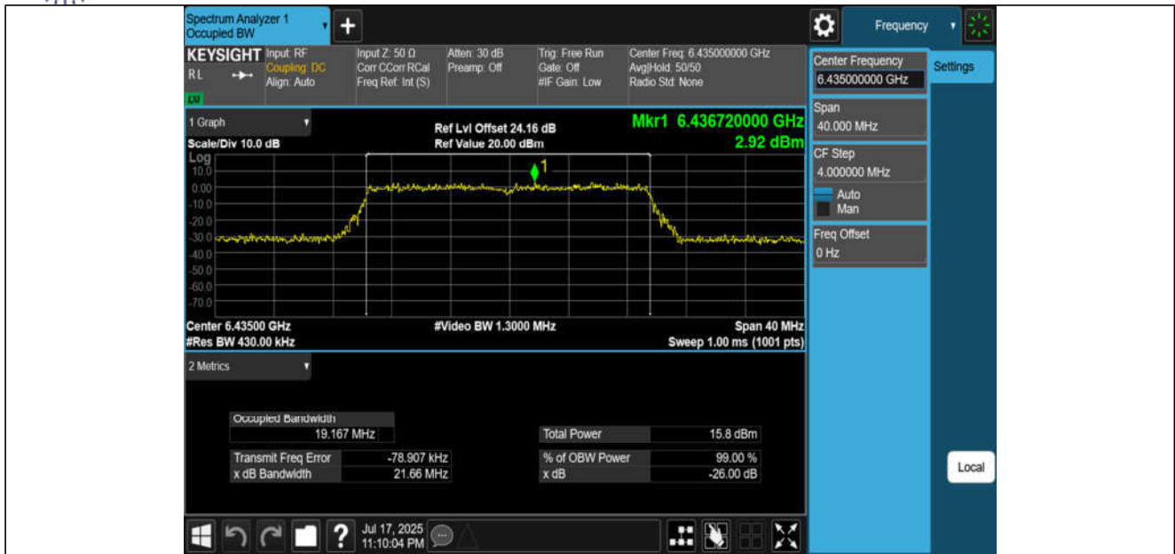
11AX20MIMO-Ant1-6435-PASS
