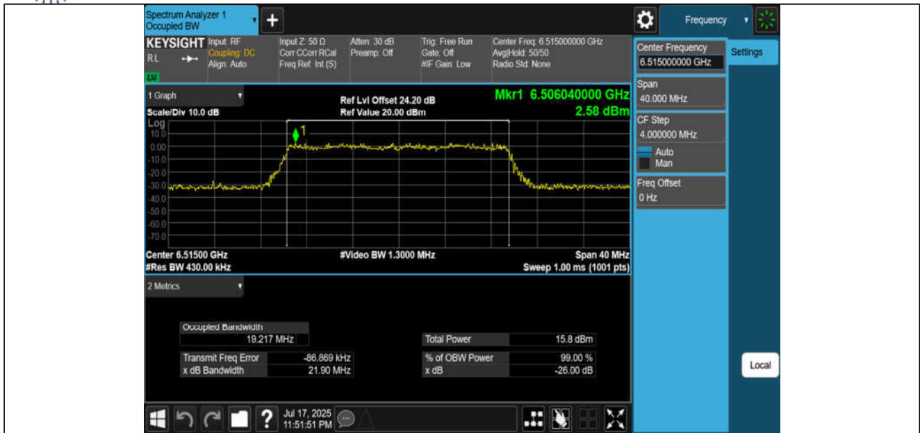
11AX20MIMO-Ant3-6515-PASS
