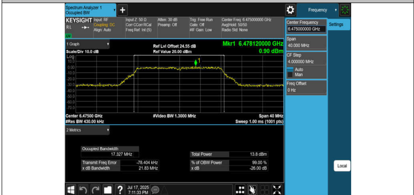
11A-CDD-Ant4-6475-PASS
