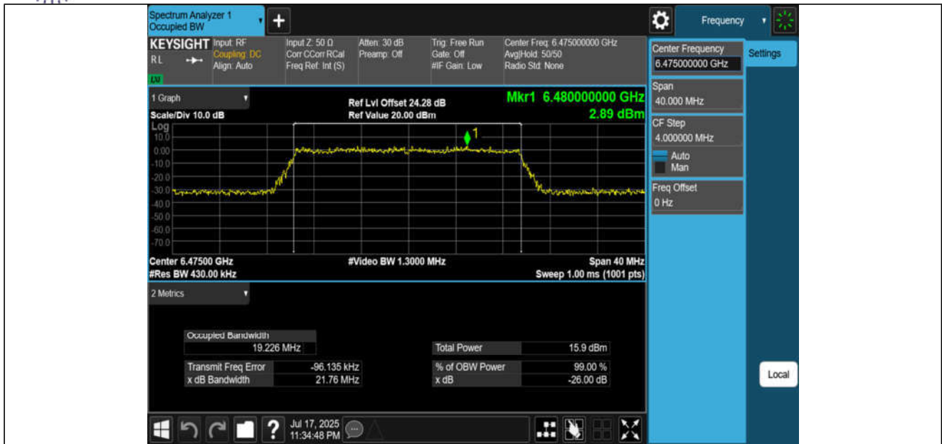
11AX20MIMO-Ant3-6475-PASS
