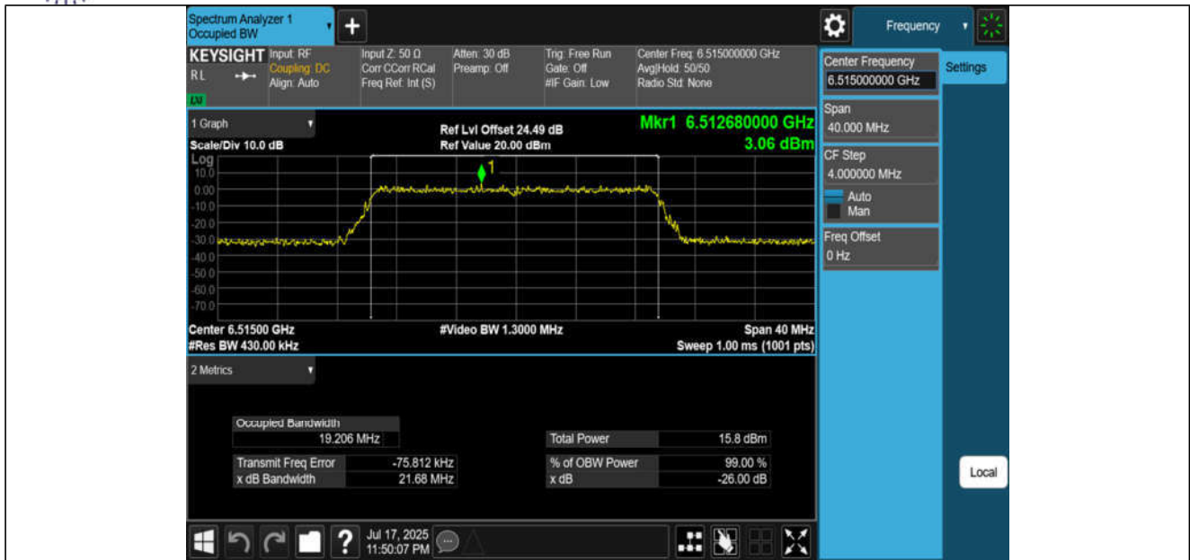
11AX20MIMO-Ant1-6515-PASS
