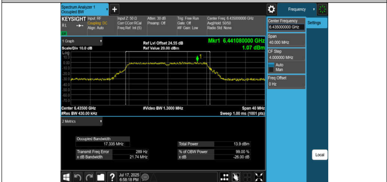
11A-CDD-Ant4-6435-PASS
