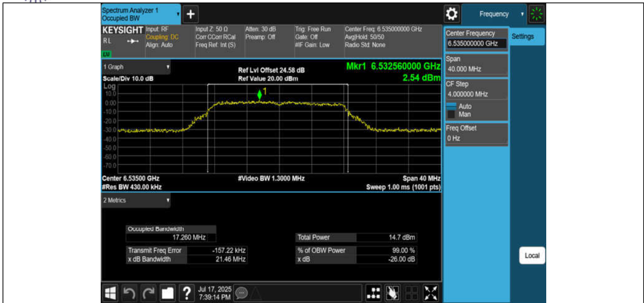
11A-CDD-Ant3-6535-PASS
