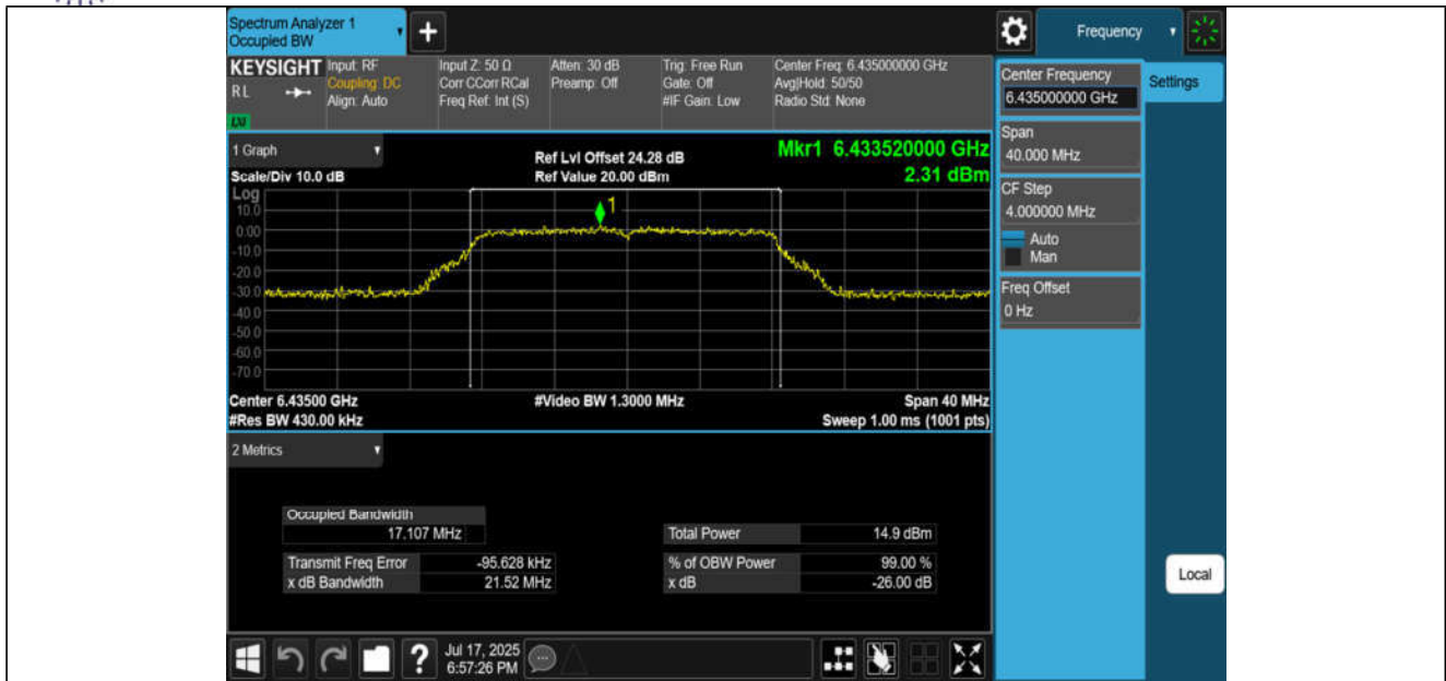
11A-CDD-Ant3-6435-PASS
