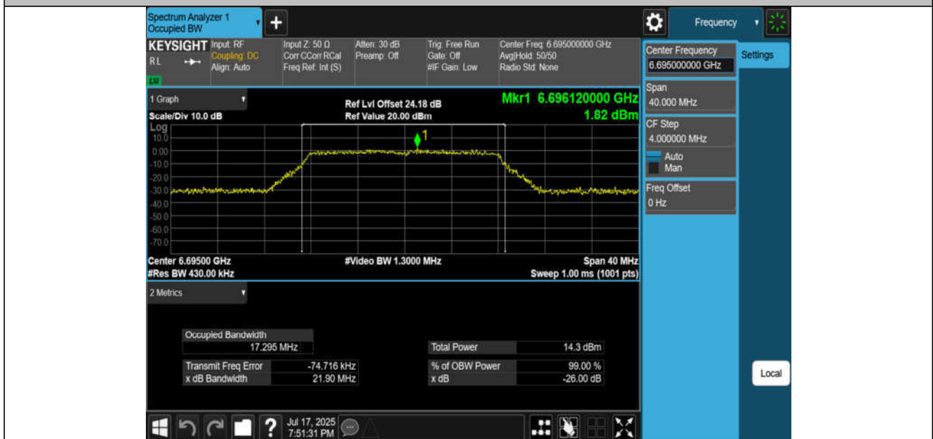
11A-CDD-Ant2-6695-PASS
