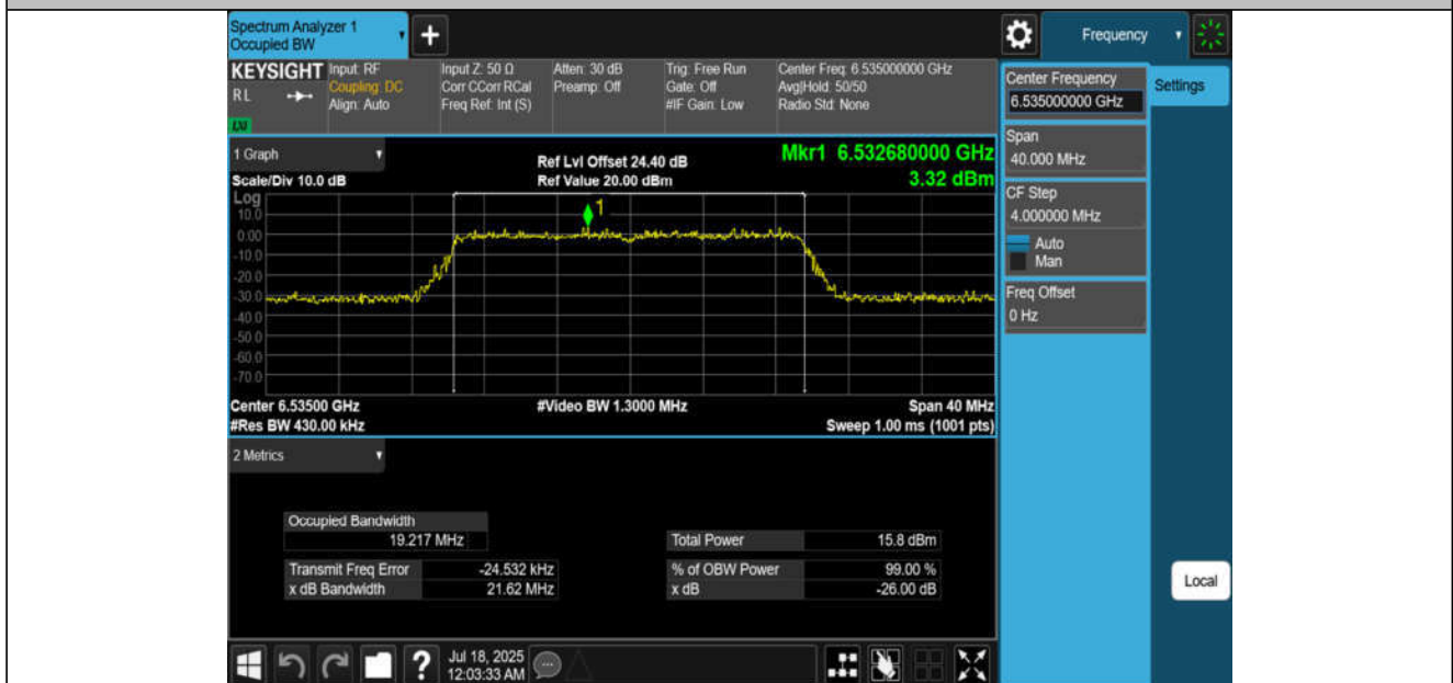
11AX20MIMO-Ant2-6535-PASS
