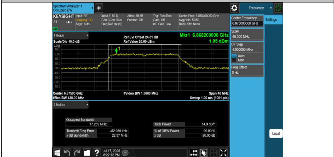
11A-CDD-Ant4-6875-PASS
