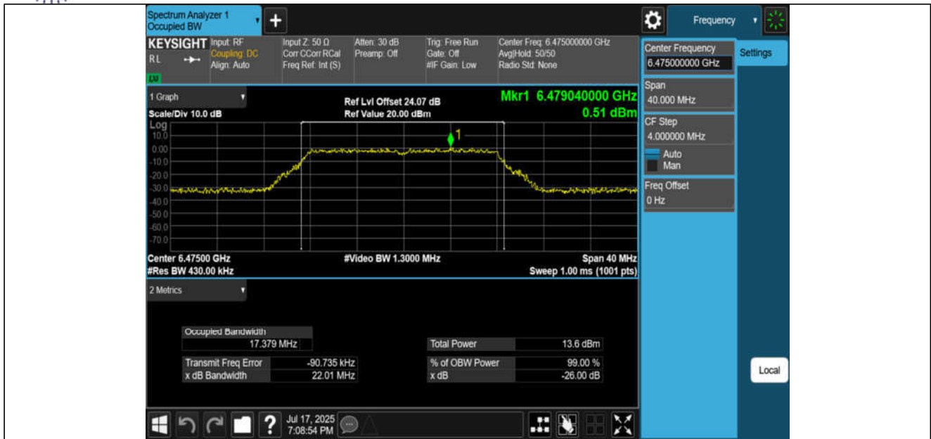
11A-CDD-Ant1-6475-PASS
