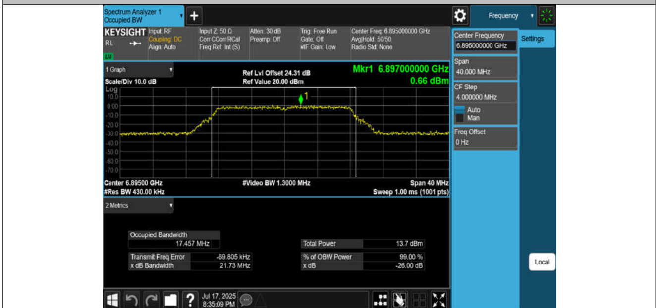
11A-CDD-Ant2-6895-PASS
