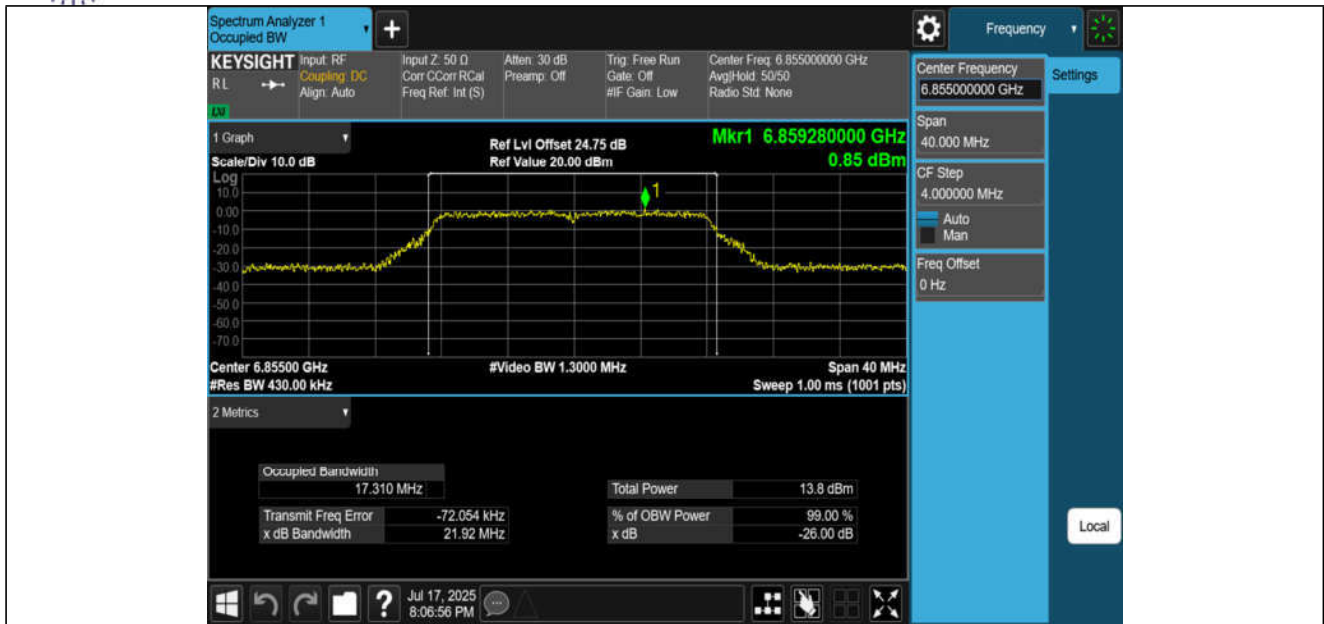
11A-CDD-Ant3-6855-PASS
