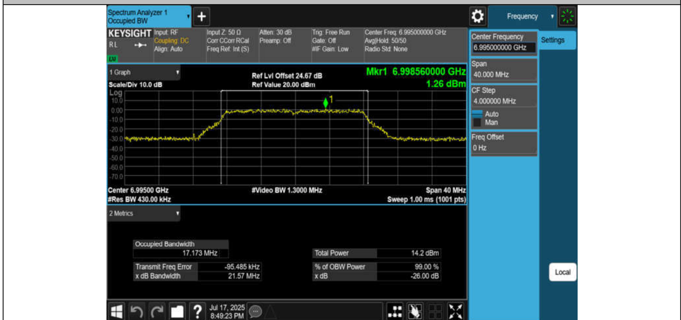
11A-CDD-Ant4-6995-PASS
