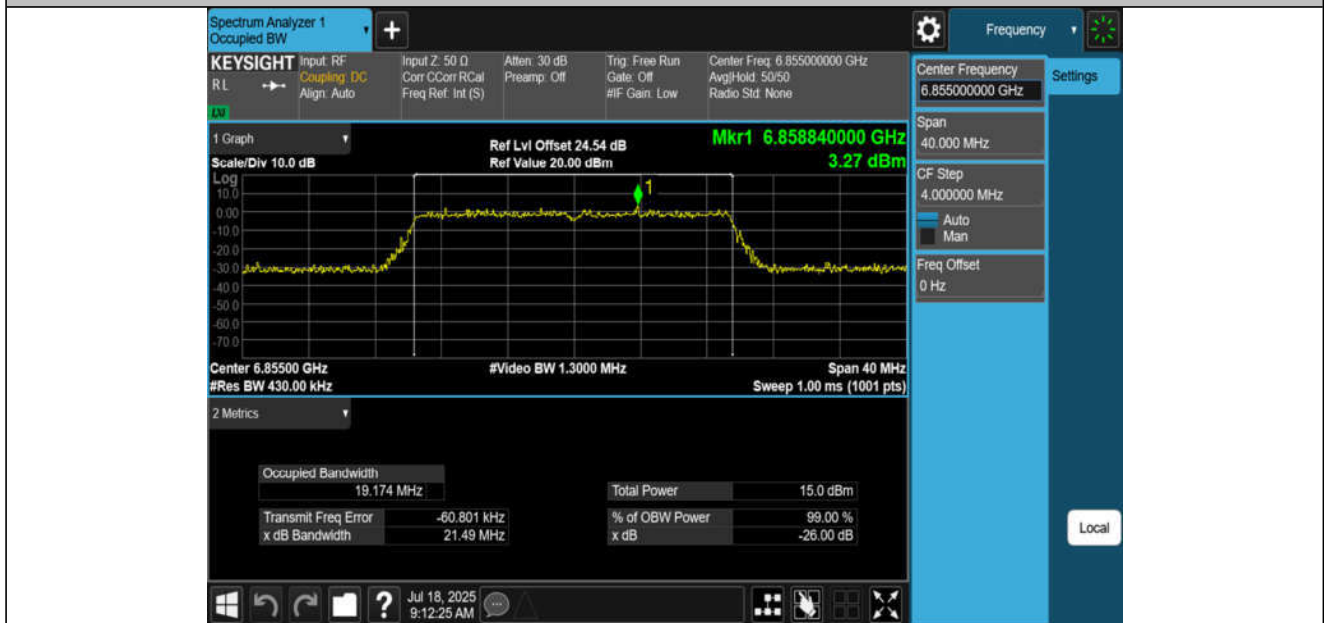
11AX20MIMO-Ant2-6855-PASS
