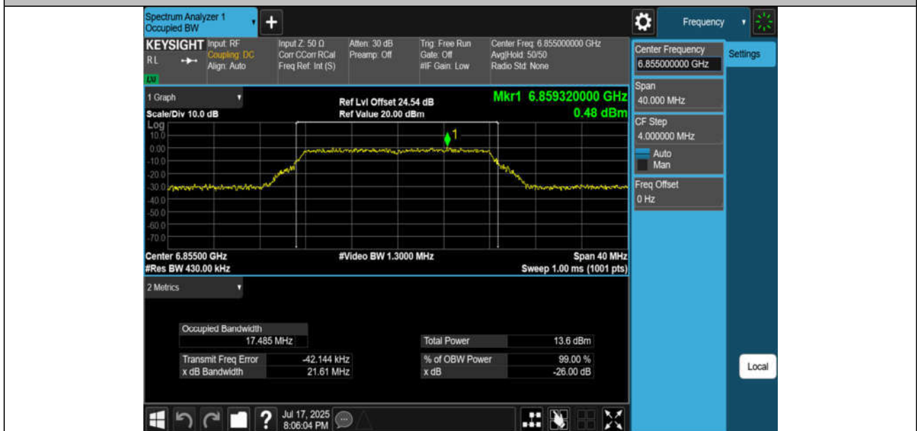
11A-CDD-Ant2-6855-PASS
