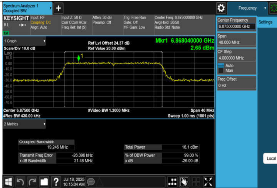
11AX20MIMO-Ant1-6875-PASS
