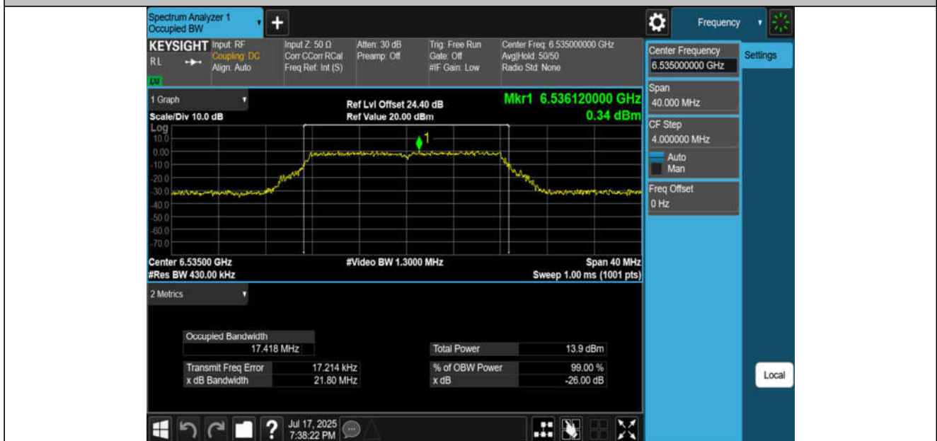
11A-CDD-Ant2-6535-PASS
