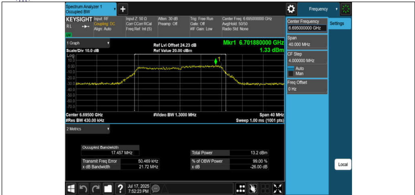
11A-CDD-Ant3-6695-PASS
