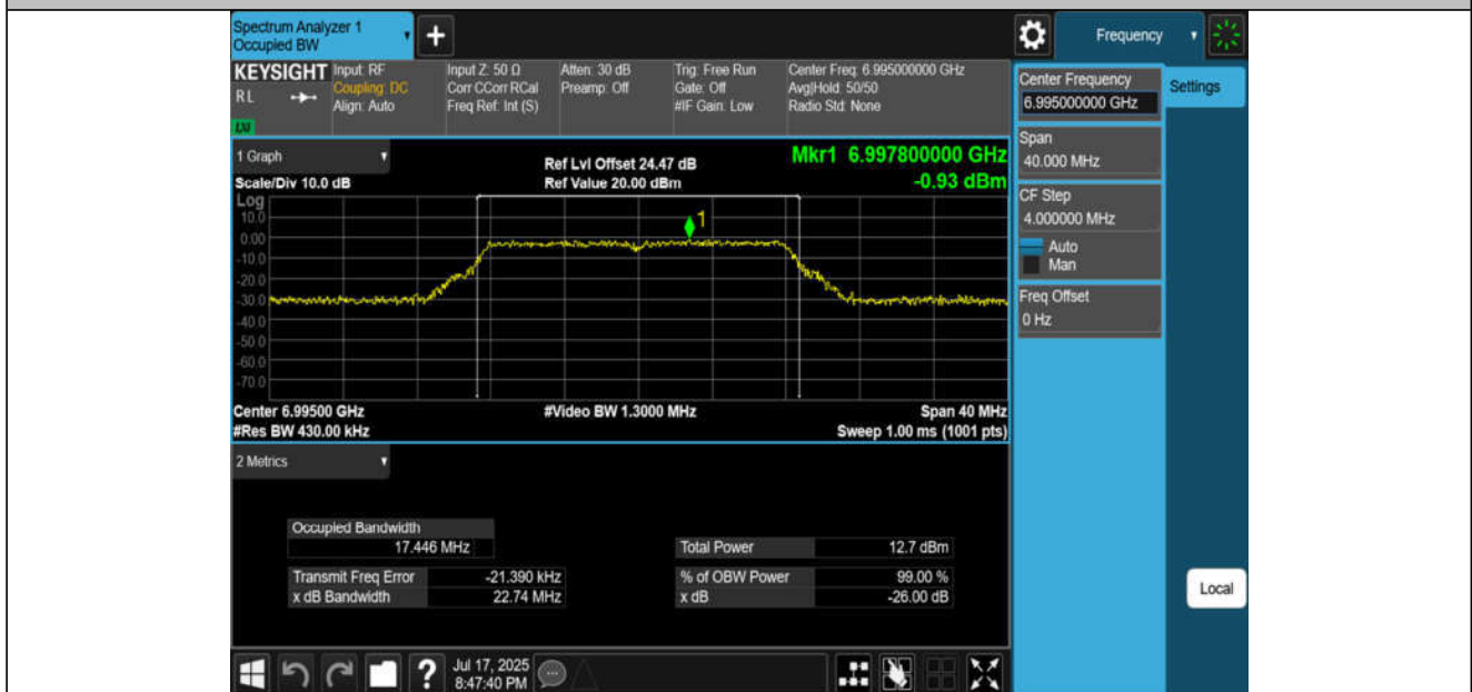
11A-CDD-Ant2-6995-PASS
