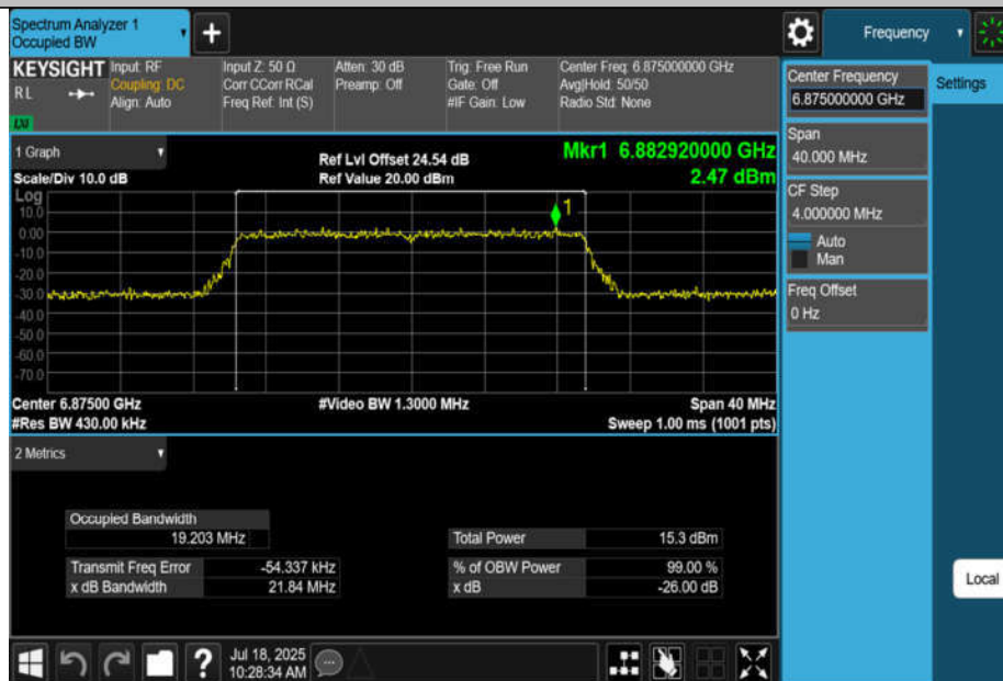
11AX20MIMO-Ant2-6875-PASS
