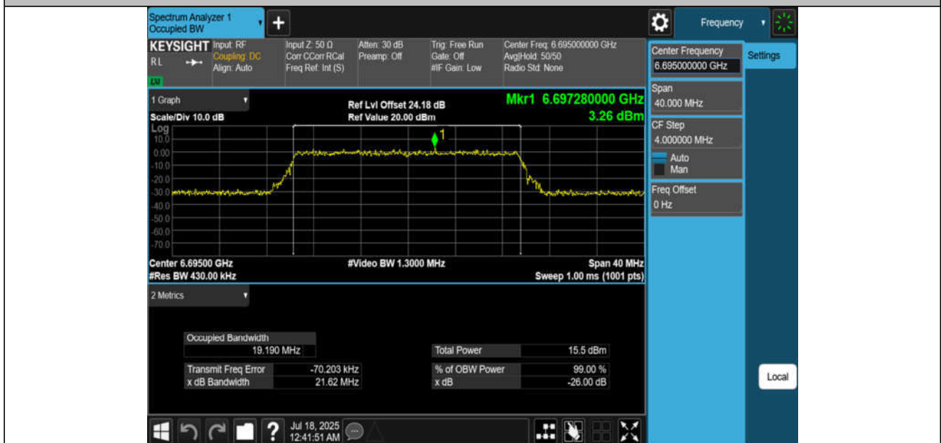
11AX20MIMO-Ant2-6695-PASS
