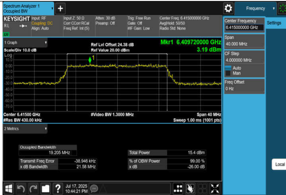
11AX20MIMO-Ant3-6415-PASS
