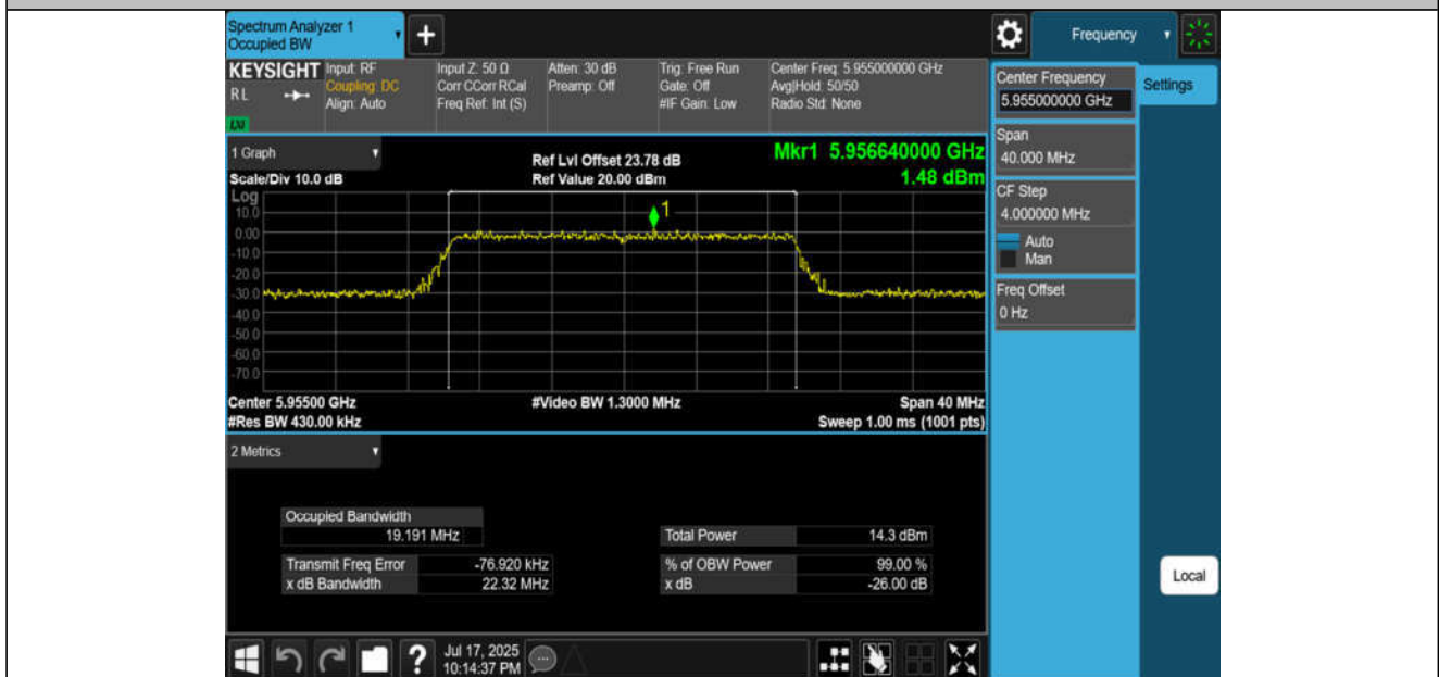
11AX20MIMO-Ant2-5955-PASS
