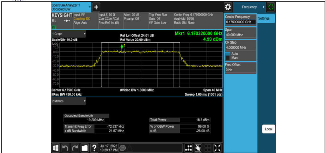
11AX20MIMO-Ant3-6175-PASS
