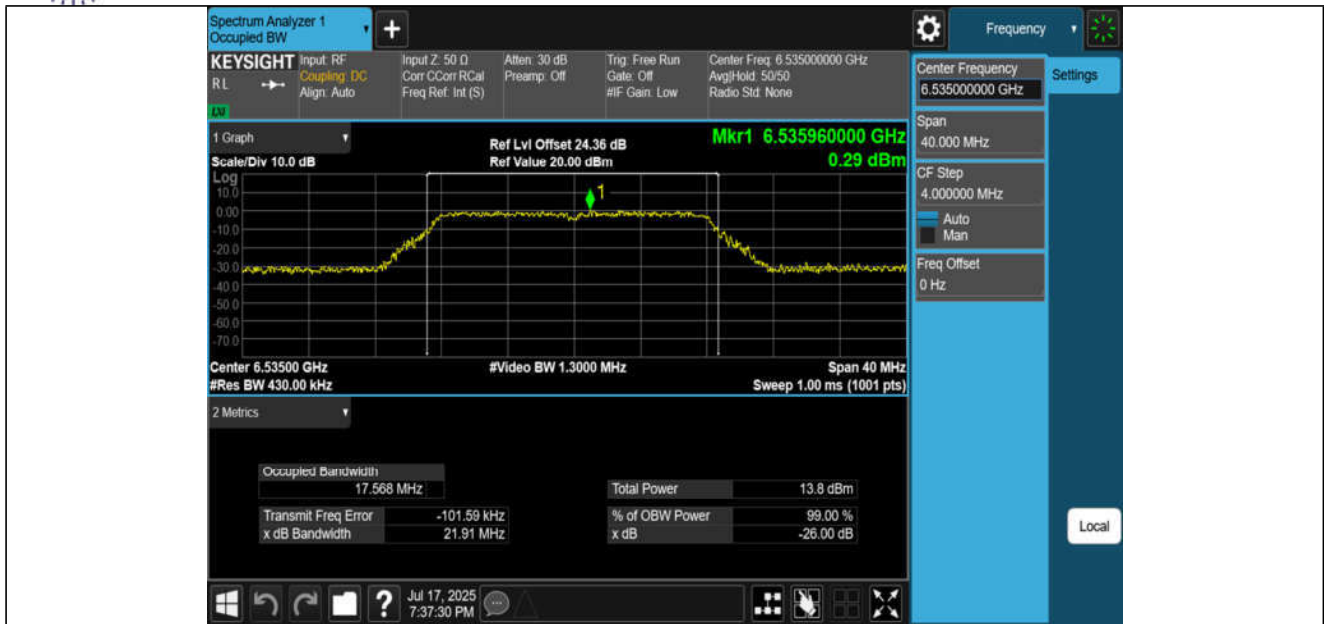
11A-CDD-Ant1-6535-PASS
