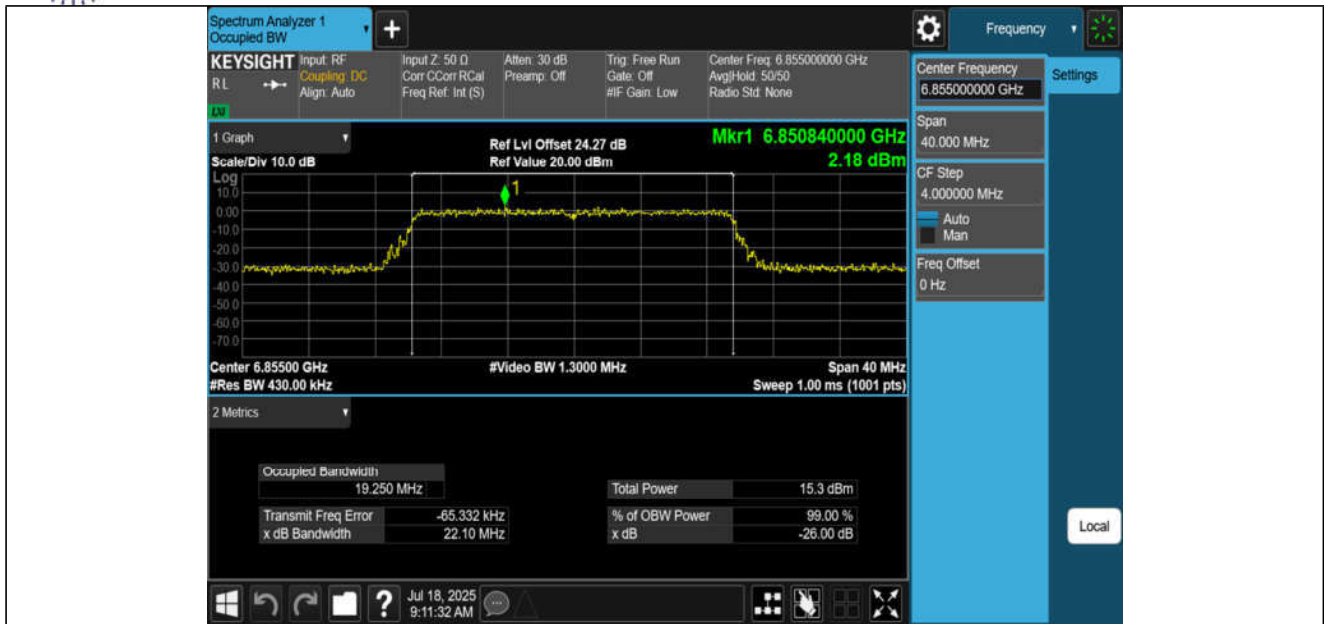
11AX20MIMO-Ant1-6855-PASS
