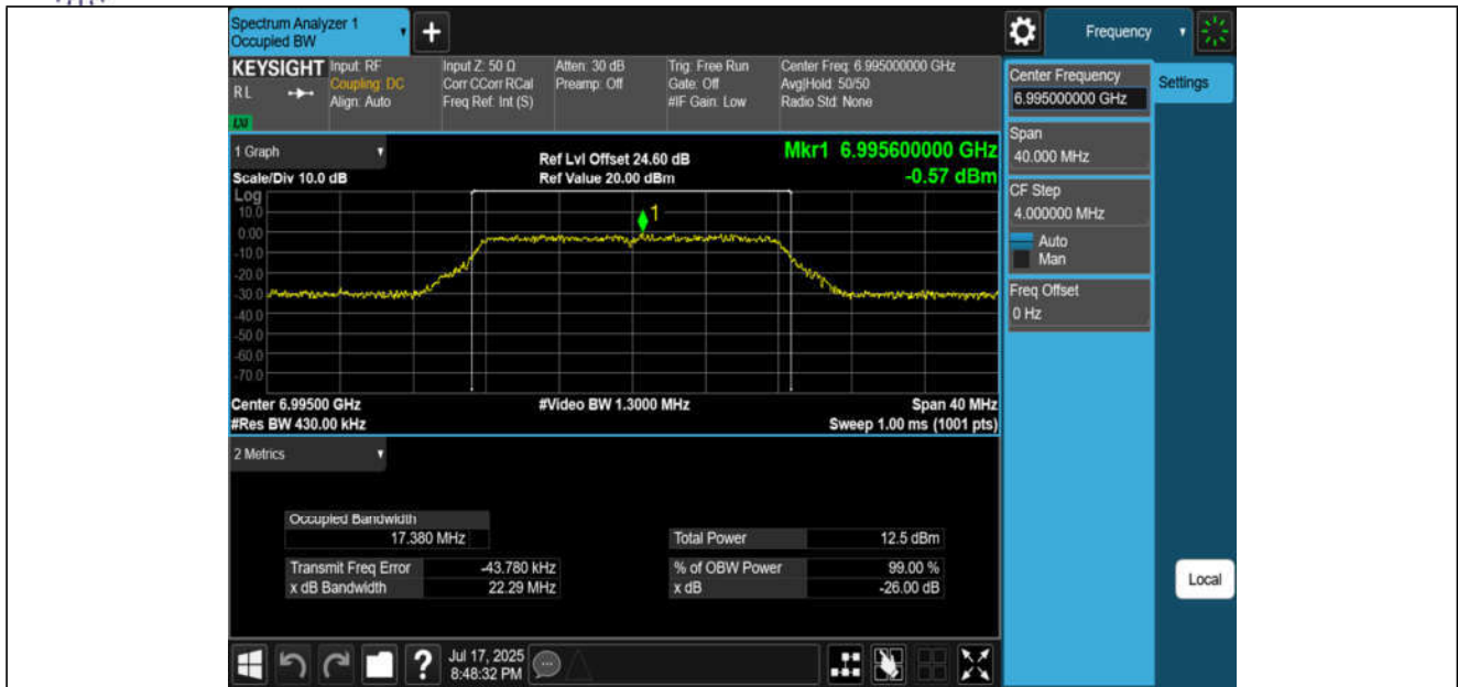
11A-CDD-Ant3-6995-PASS
