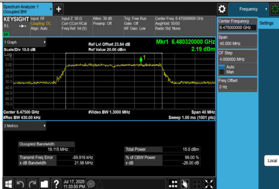
11AX20MIMO-Ant2-6475-PASS
