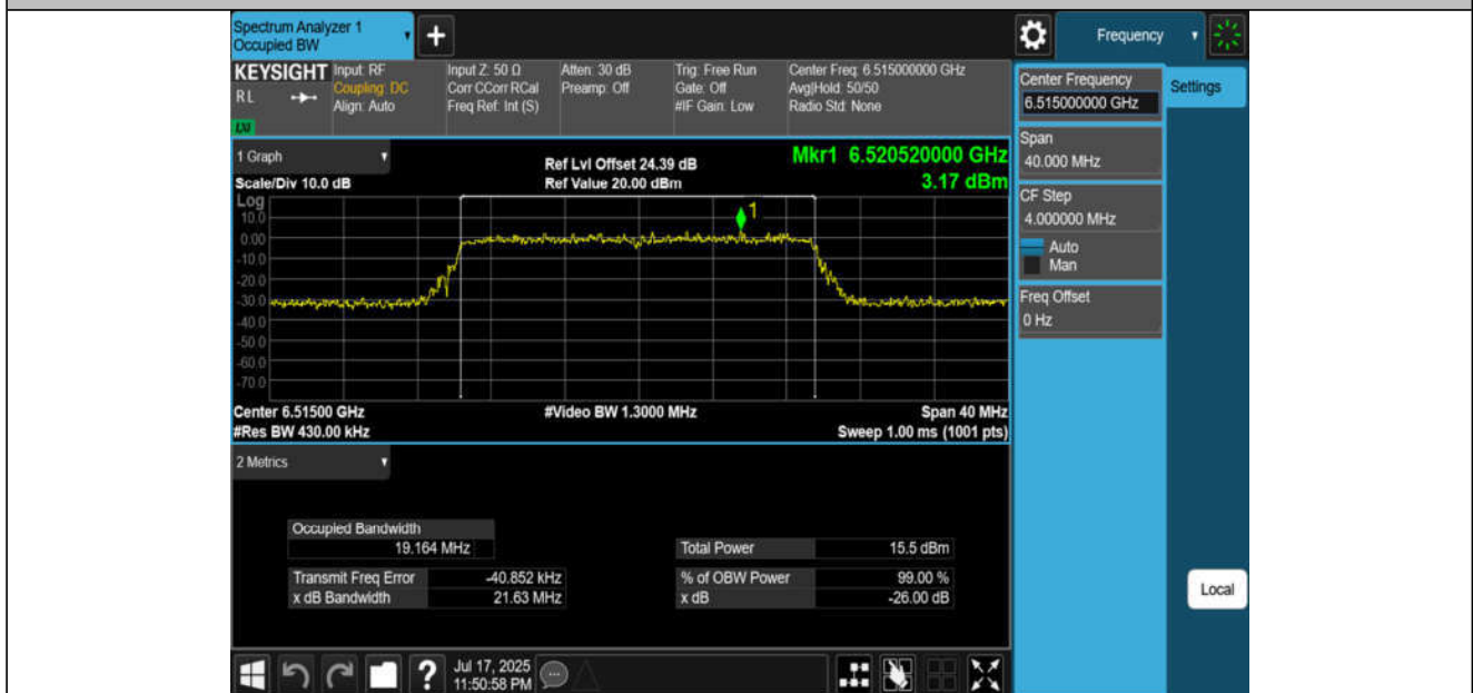
11AX20MIMO-Ant2-6515-PASS
