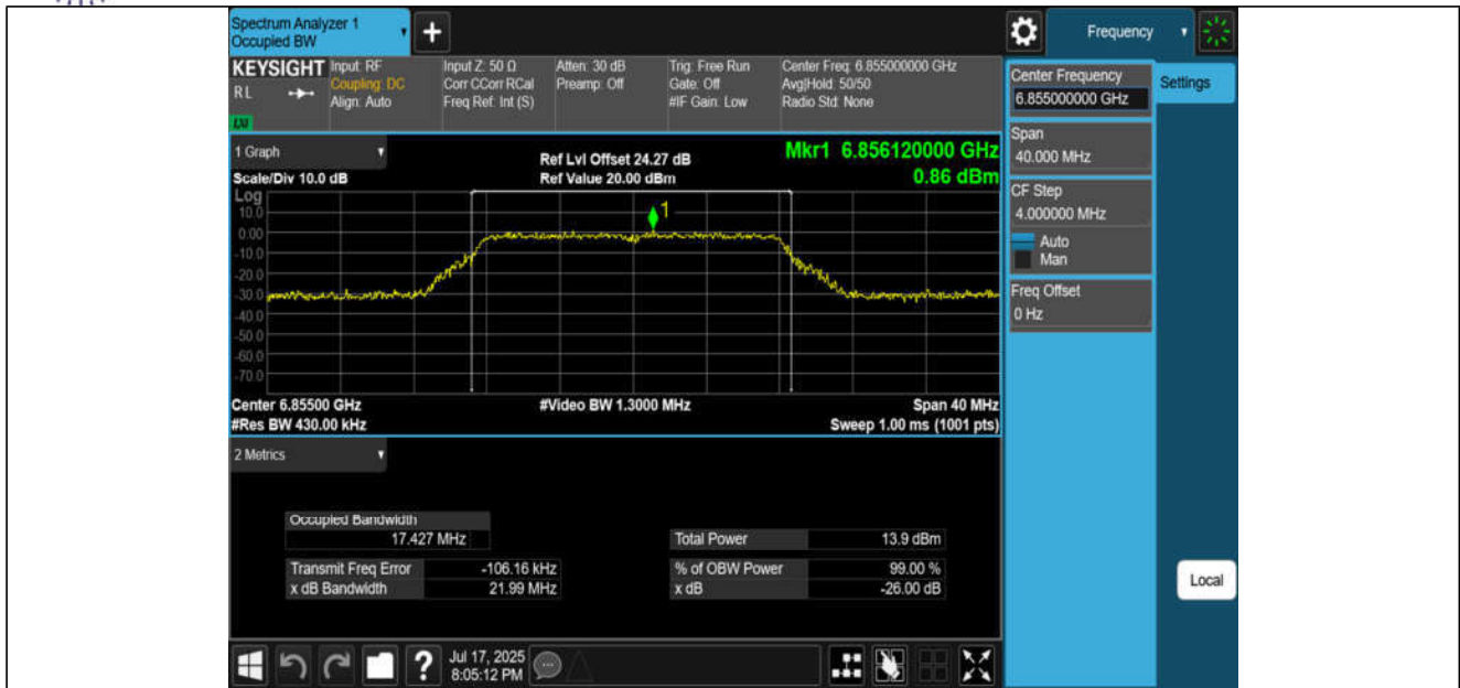
11A-CDD-Ant1-6855-PASS
