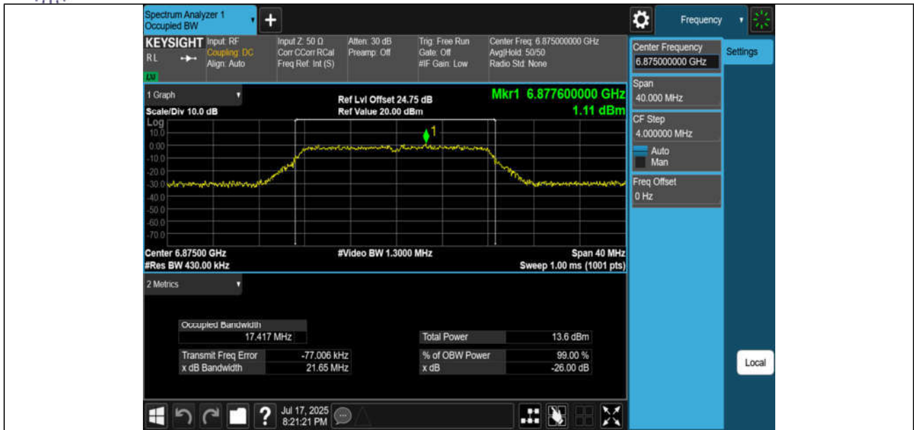
11A-CDD-Ant3-6875-PASS
