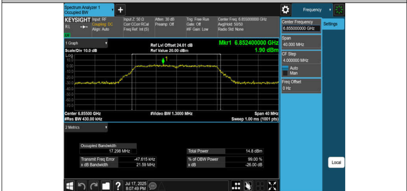
11A-CDD-Ant4-6855-PASS
