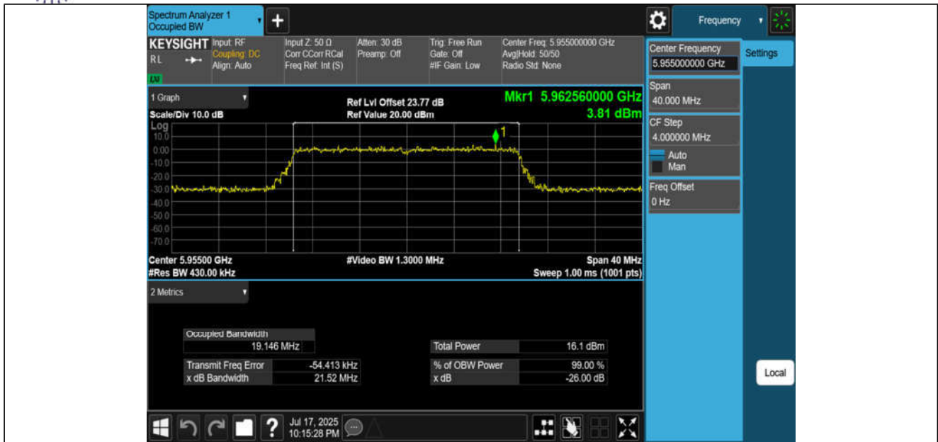
11AX20MIMO-Ant3-5955-PASS
