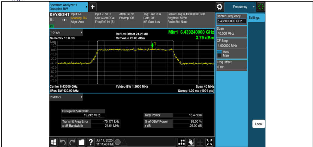
11AX20MIMO-Ant3-6435-PASS
