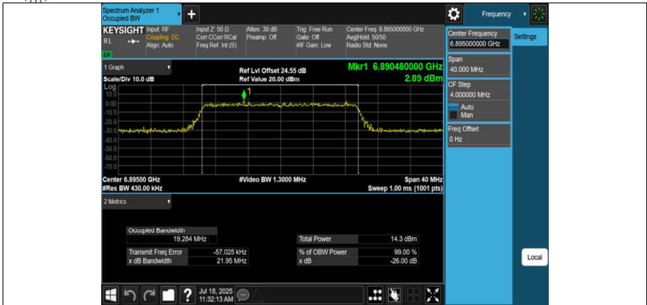
11AX20MIMO-Ant3-6895-PASS
