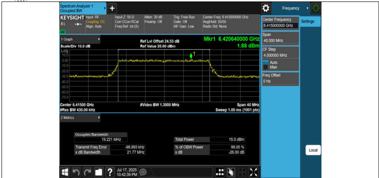
11AX20MIMO-Ant1-6415-PASS
