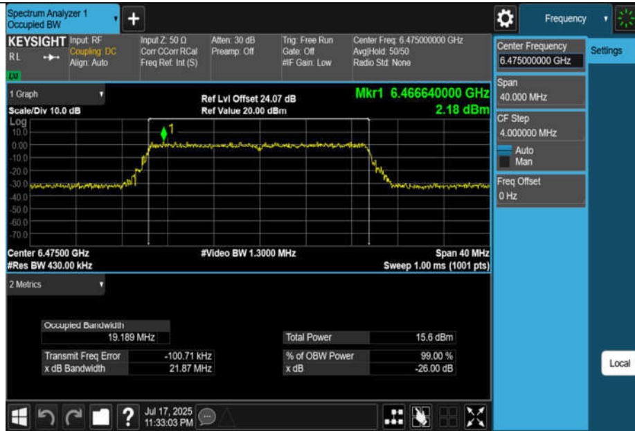
11AX20MIMO-Ant1-6475-PASS
