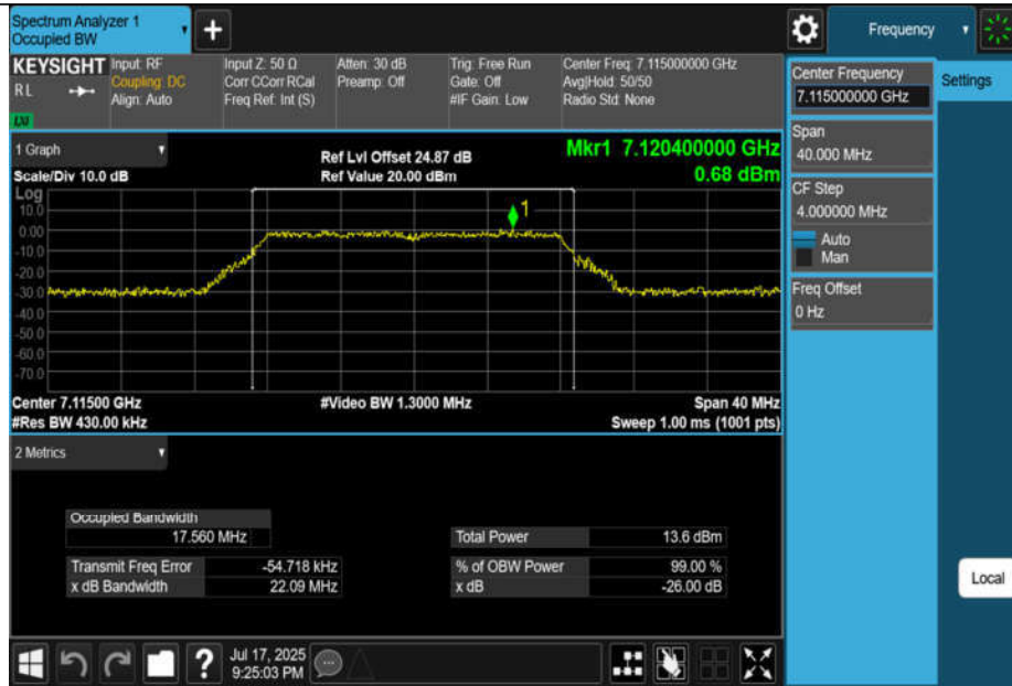
11A-CDD-Ant1-7115-PASS
