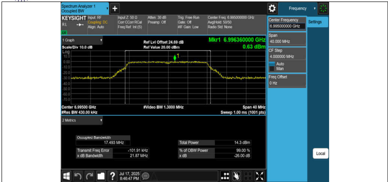
11A-CDD-Ant1-6995-PASS
