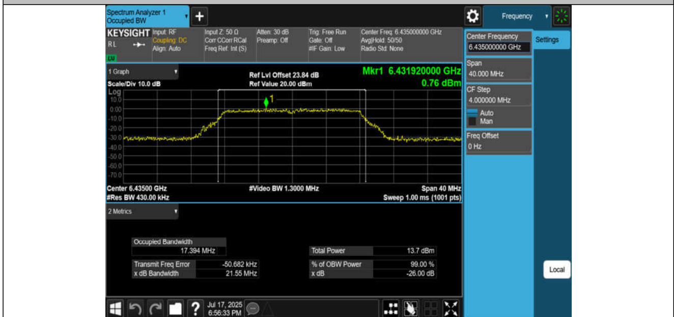
11A-CDD-Ant2-6435-PASS
