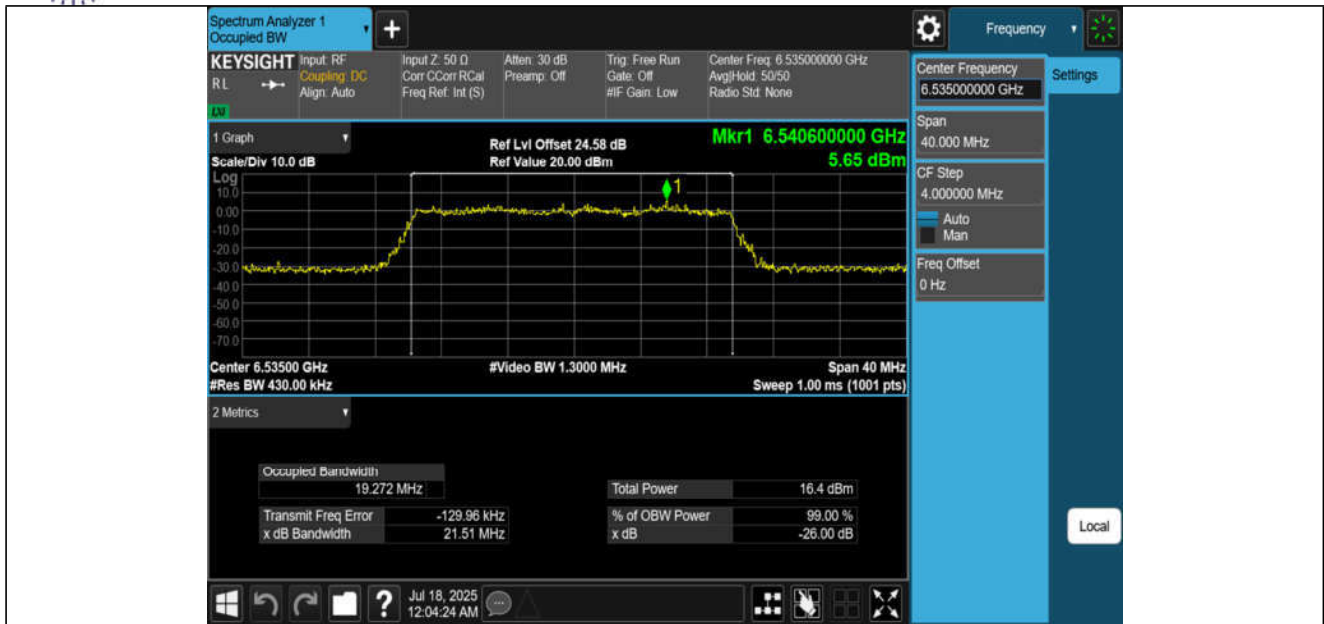
11AX20MIMO-Ant3-6535-PASS
