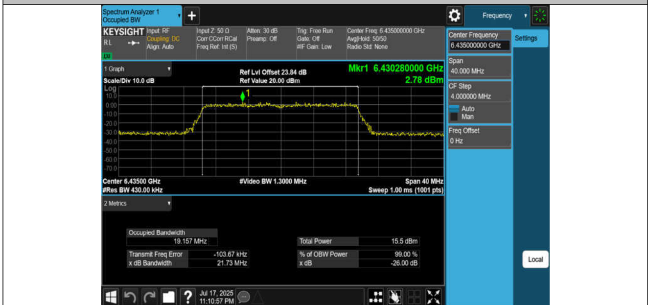
11AX20MIMO-Ant2-6435-PASS
