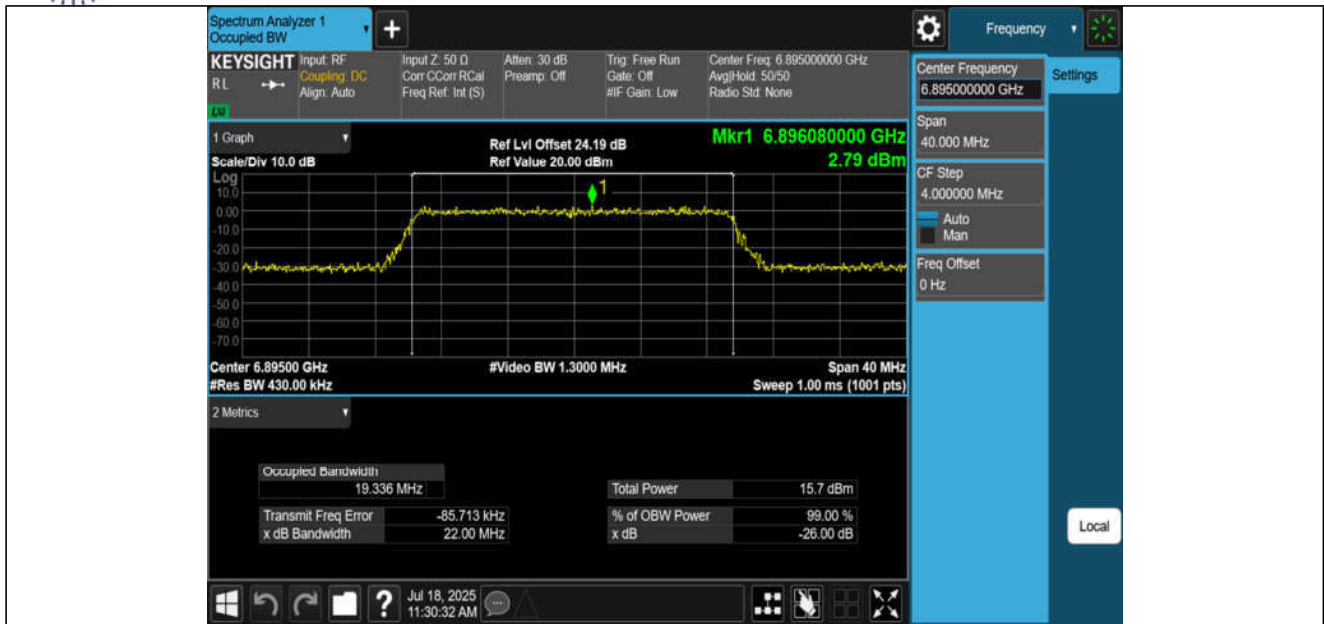
11AX20MIMO-Ant1-6895-PASS
