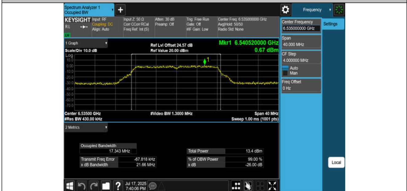
11A-CDD-Ant4-6535-PASS
