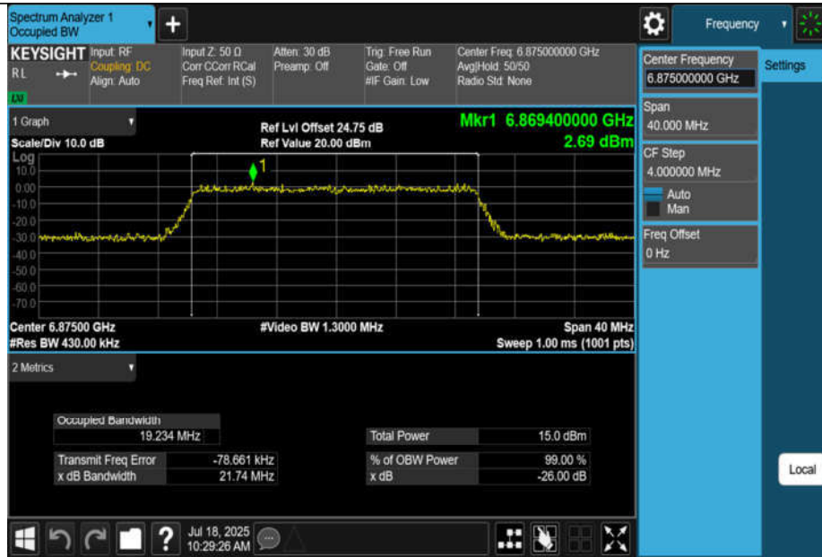
11AX20MIMO-Ant3-6875-PASS
