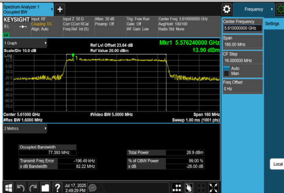
11BE80MIMO-Ant4-5610
