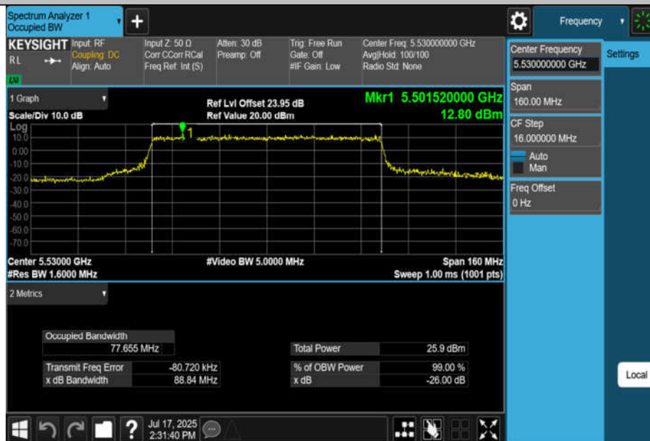
11BE80MIMO-Ant4-5530
