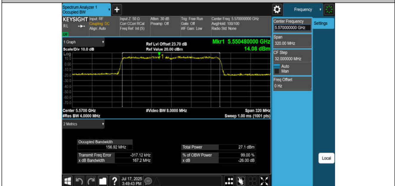
11BE160MIMO-Ant4-5570
