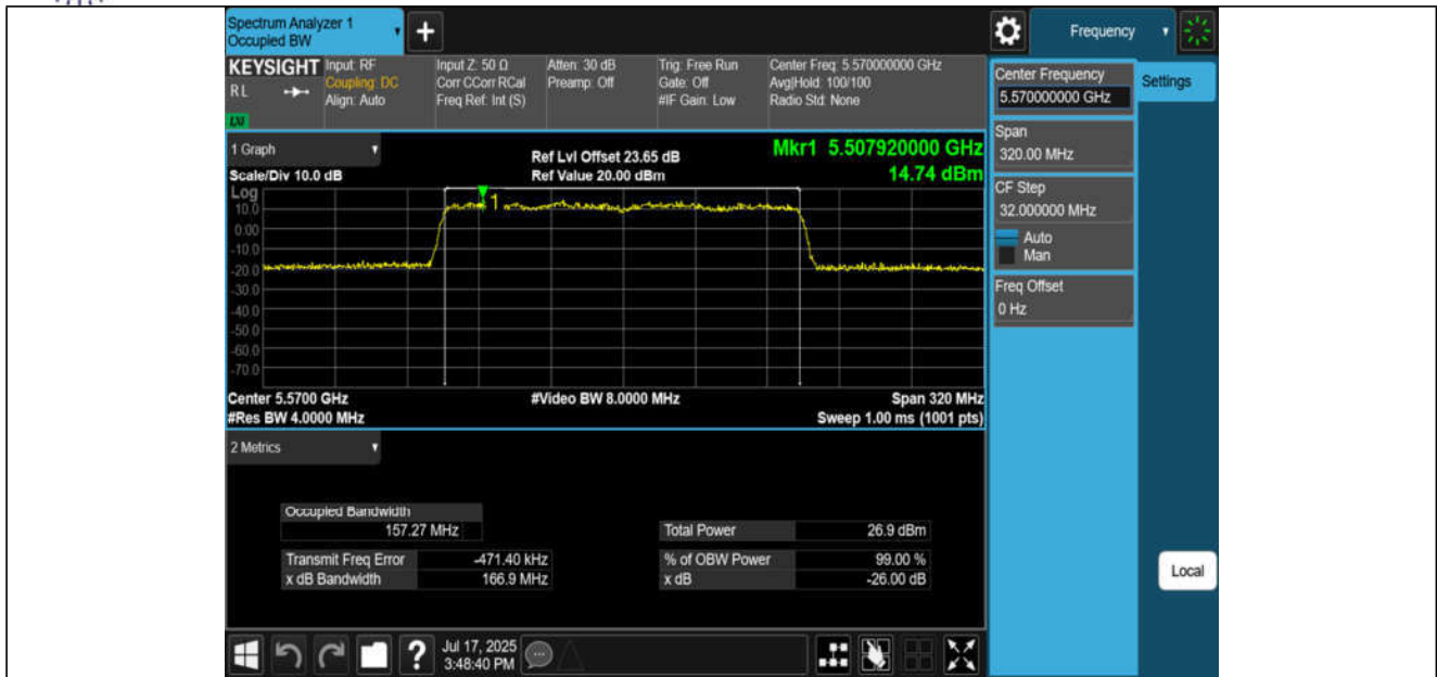
11BE160MIMO-Ant3-5570
