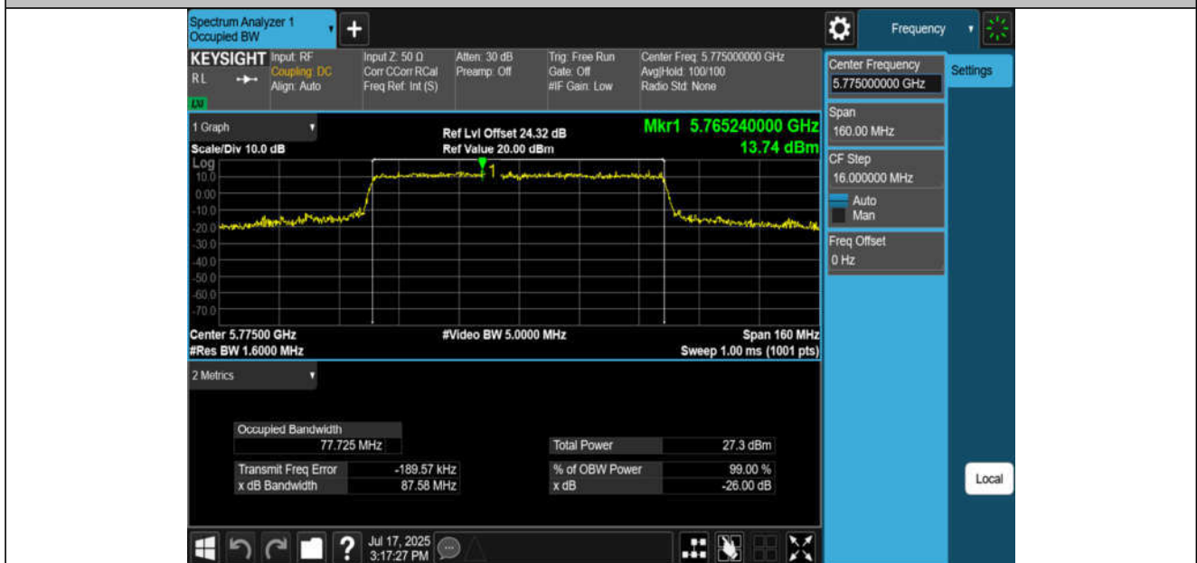
11BE80MIMO-Ant4-5775
