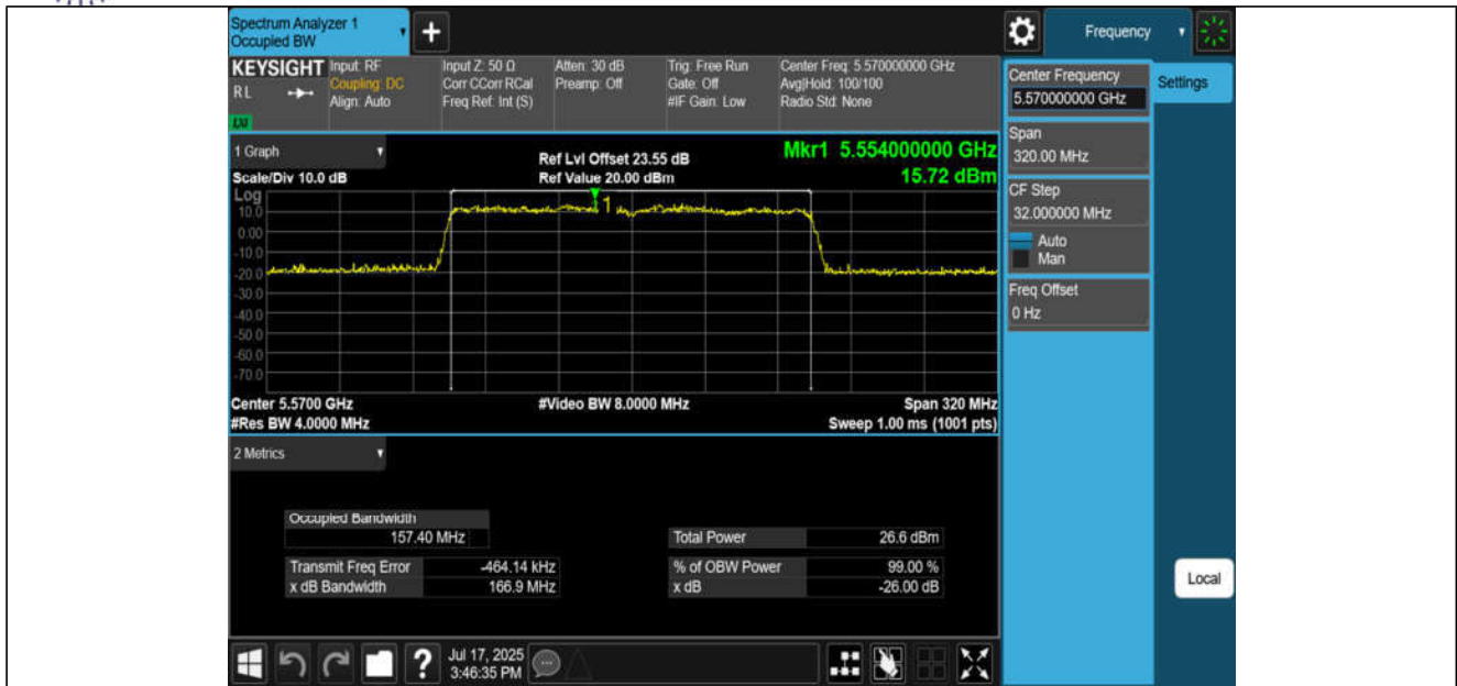
11BE160MIMO-Ant1-5570
