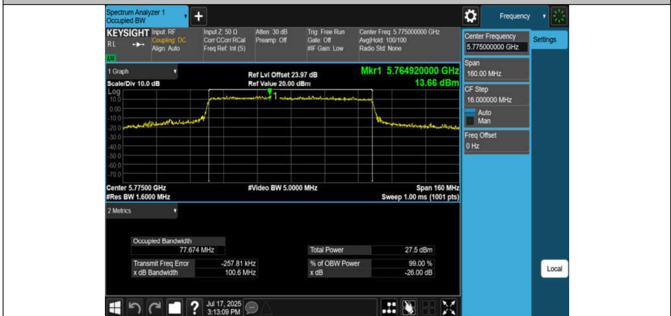
11BE80MIMO-Ant2-5775
