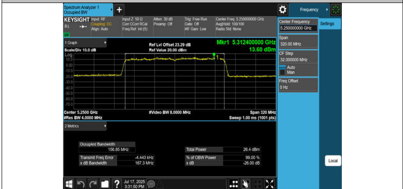
11BE160MIMO-Ant4-5250
