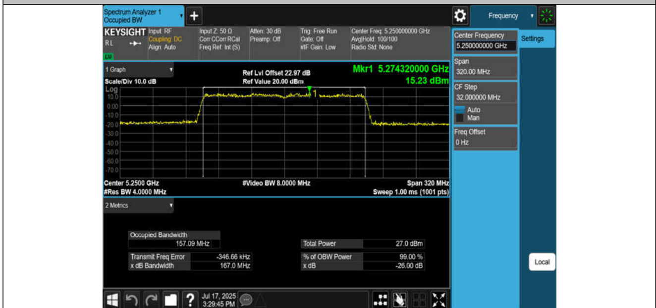
11BE160MIMO-Ant2-5250
