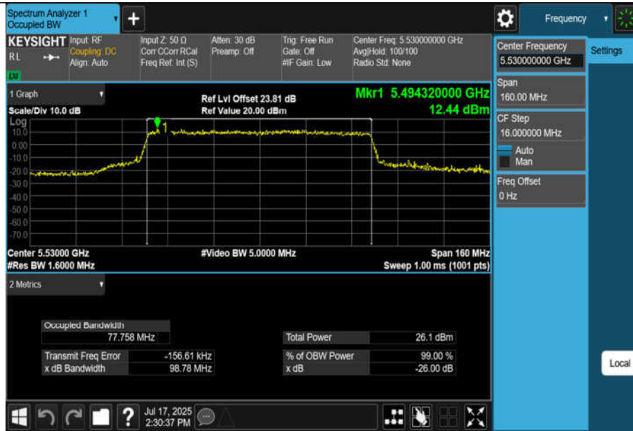
11BE80MIMO-Ant3-5530
