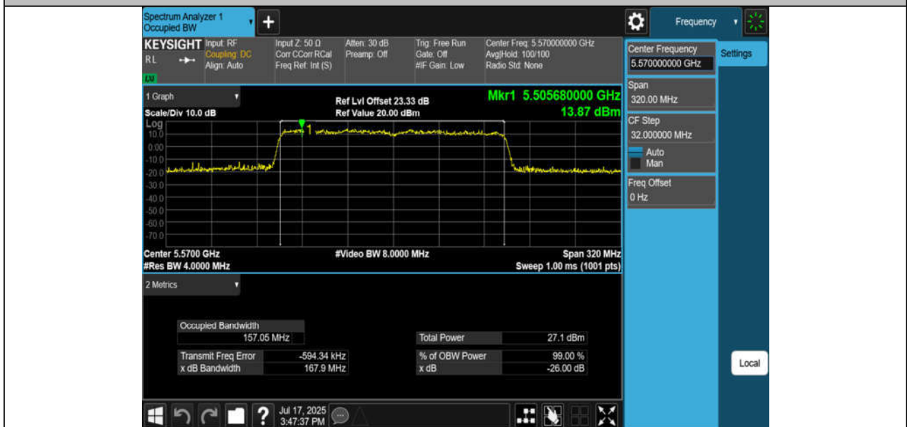
11BE160MIMO-Ant2-5570
