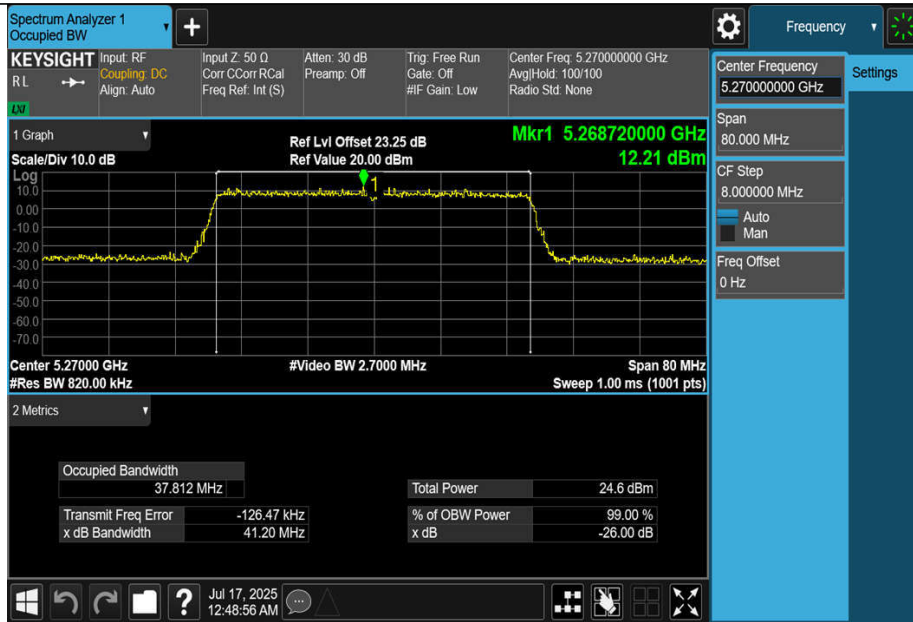
11BE40MIMO-Ant3-5270
