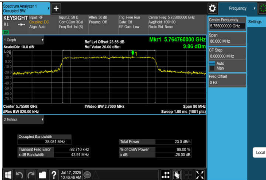
11BE40MIMO-Ant1-5755
