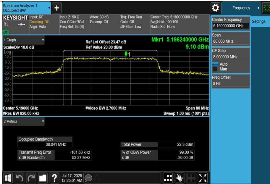
11BE40MIMO-Ant3-5190
