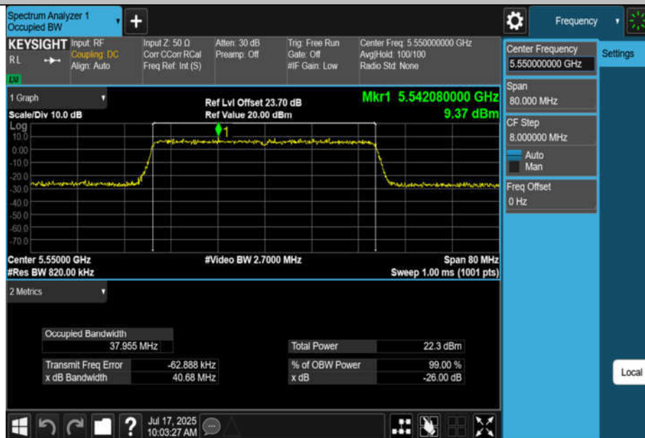
11BE40MIMO-Ant4-5550
