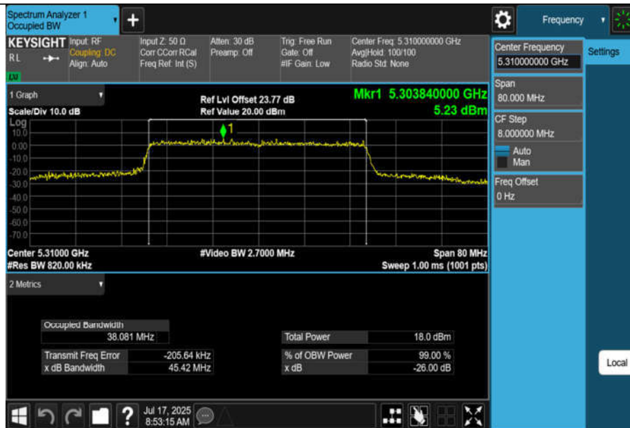
11BE40MIMO-Ant3-5310
