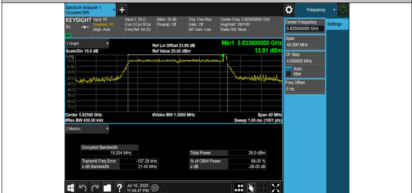
11BE20MIMO-Ant4-5825
