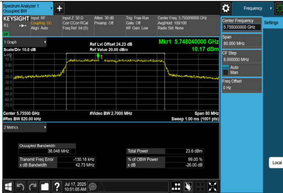
11BE40MIMO-Ant3-5755
