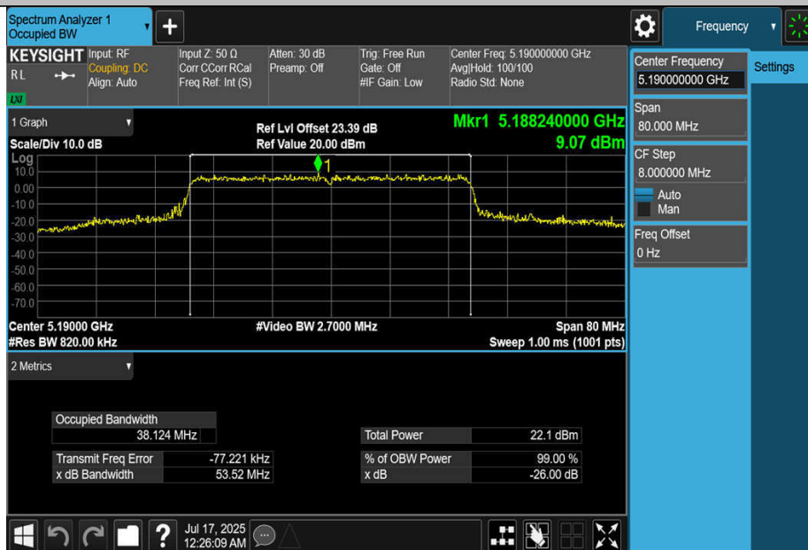
11BE40MIMO-Ant4-5190
