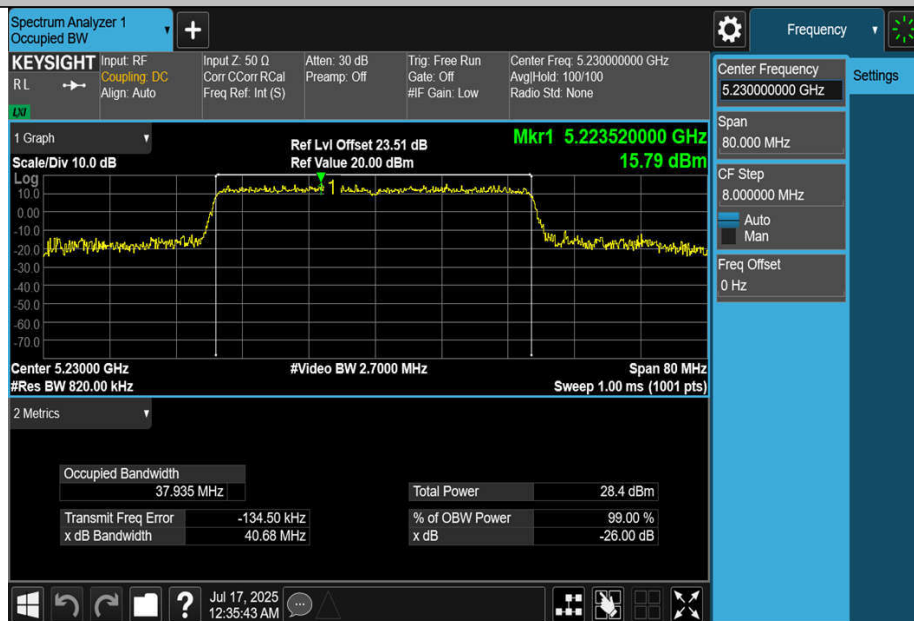
11BE40MIMO-Ant2-5230
