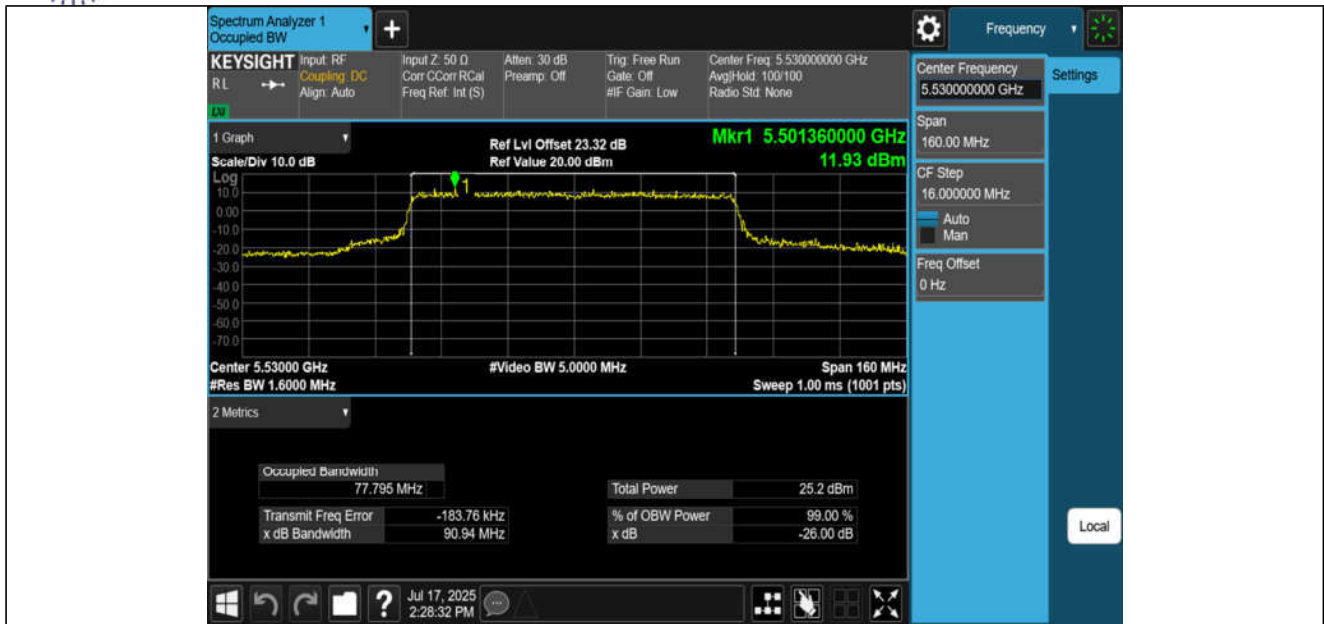
11BE80MIMO-Ant1-5530
