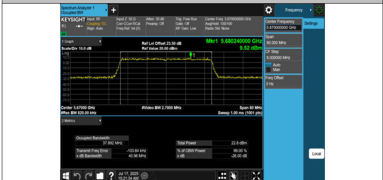
11BE40MIMO-Ant2-5670
