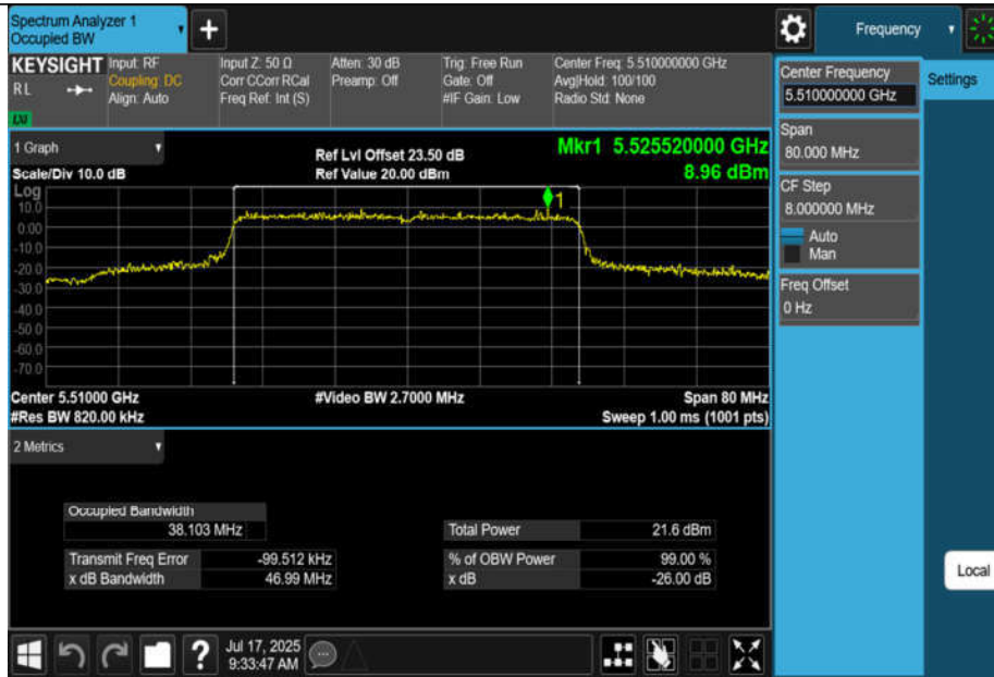
11BE40MIMO-Ant1-5510
