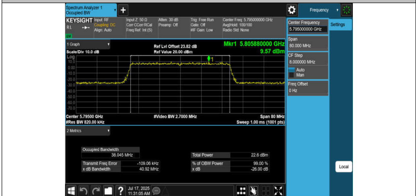
11BE40MIMO-Ant2-5795
