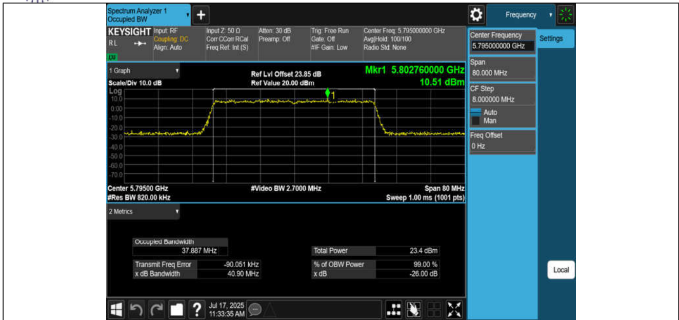
11BE40MIMO-Ant3-5795
