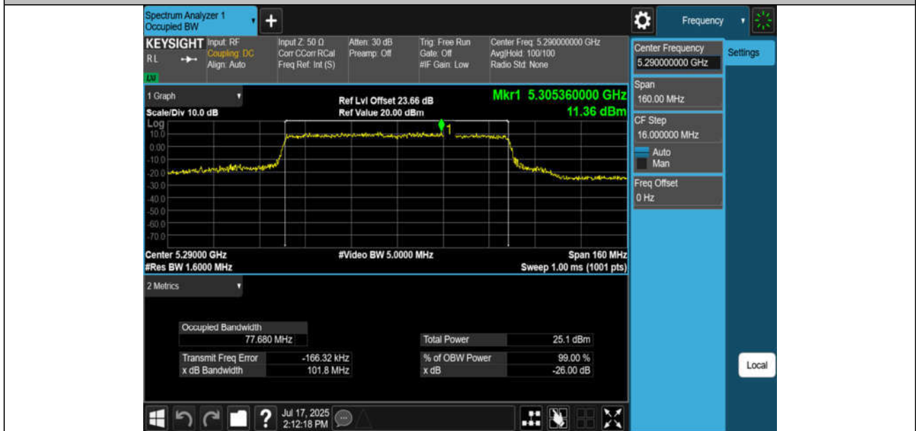
11BE80MIMO-Ant2-5290
