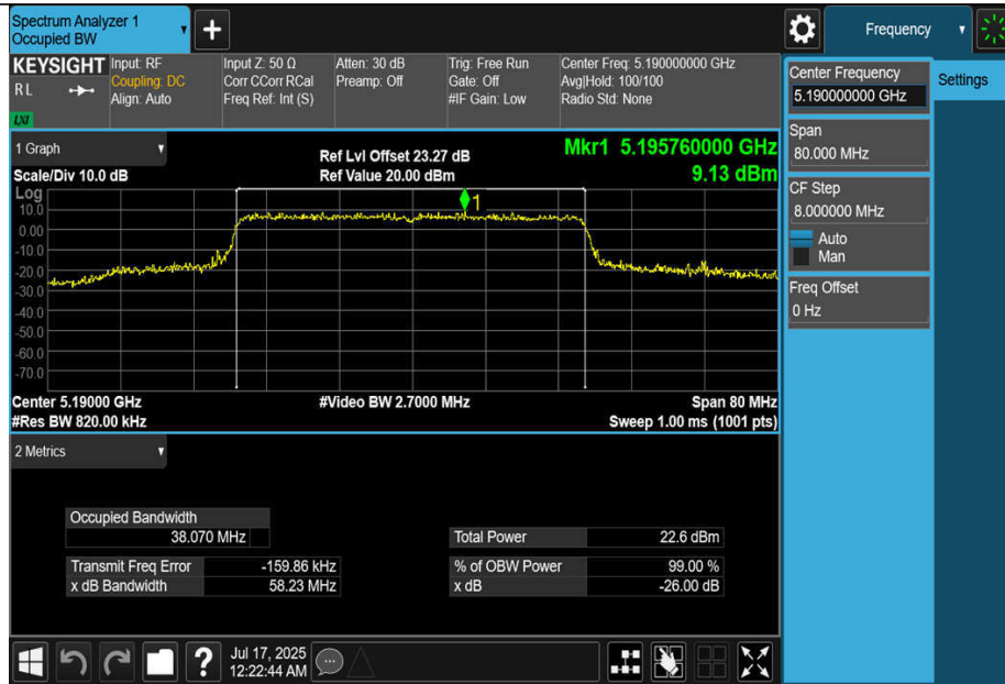
11BE40MIMO-Ant1-5190
