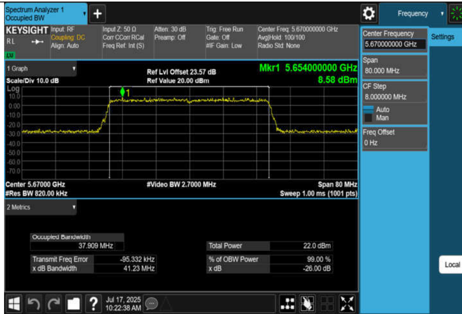
11BE40MIMO-Ant3-5670
