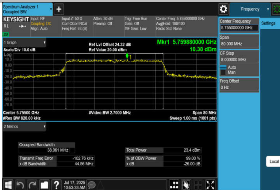
11BE40MIMO-Ant4-5755
