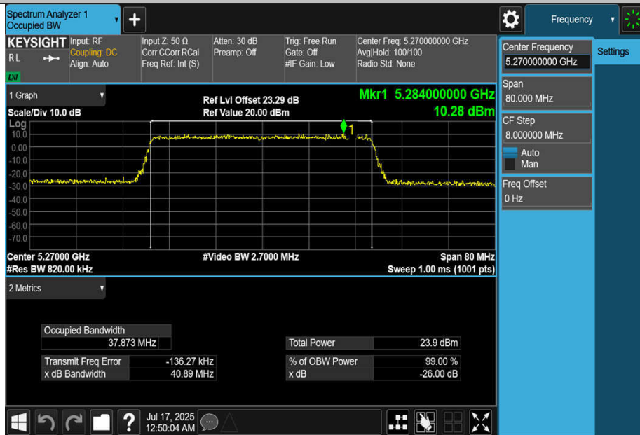
11BE40MIMO-Ant4-5270
