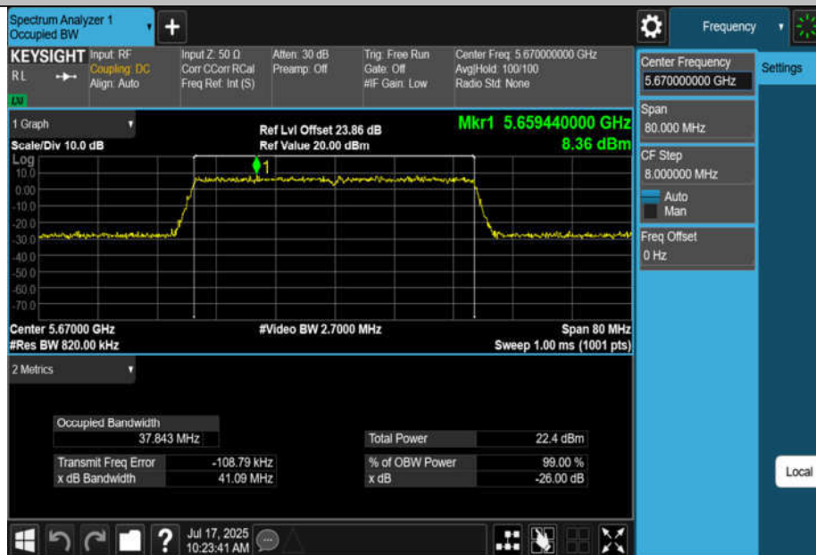
11BE40MIMO-Ant4-5670
