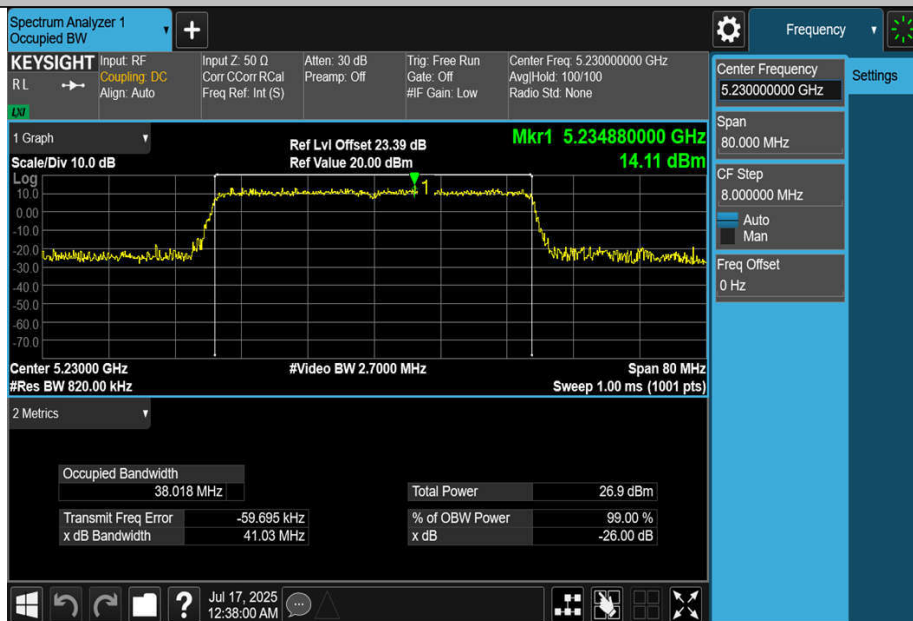
11BE40MIMO-Ant4-5230
