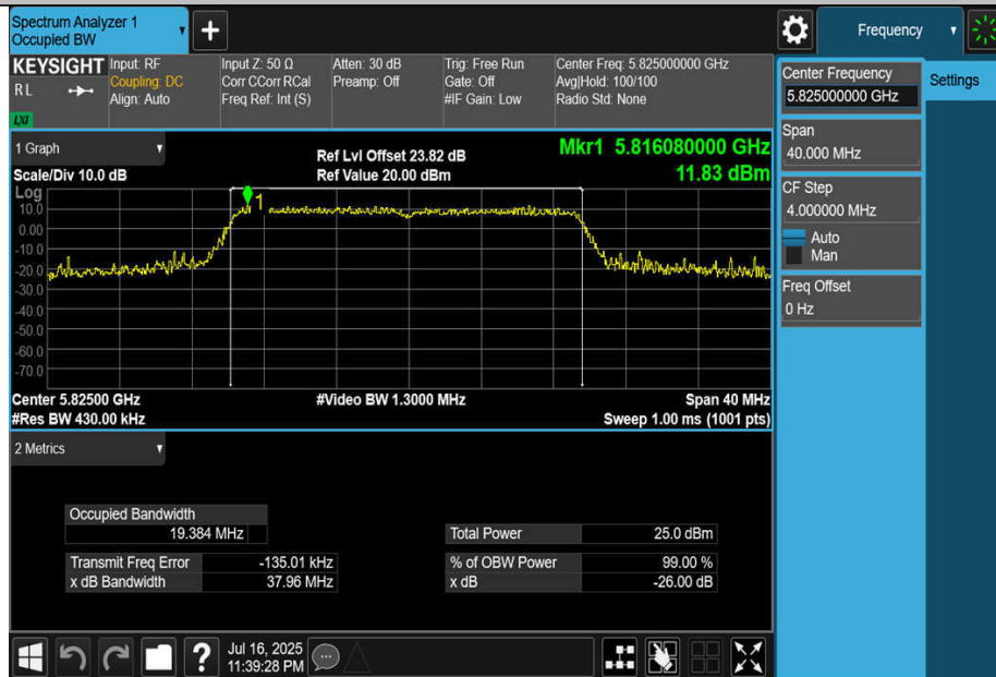
11BE20MIMO-Ant2-5825
