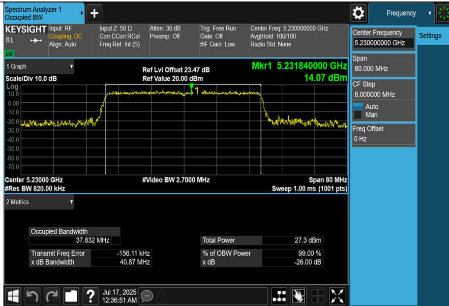
11BE40MIMO-Ant3-5230
