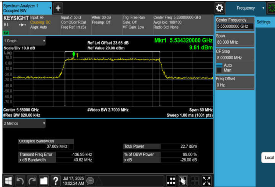
11BE40MIMO-Ant3-5550
