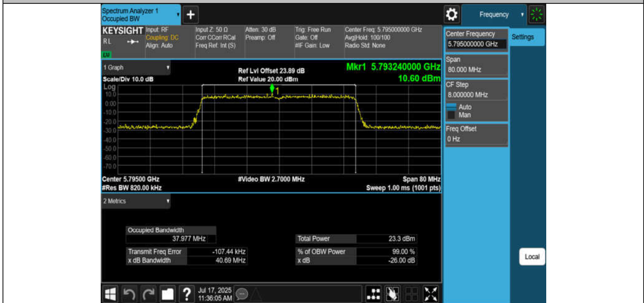
11BE40MIMO-Ant4-5795
