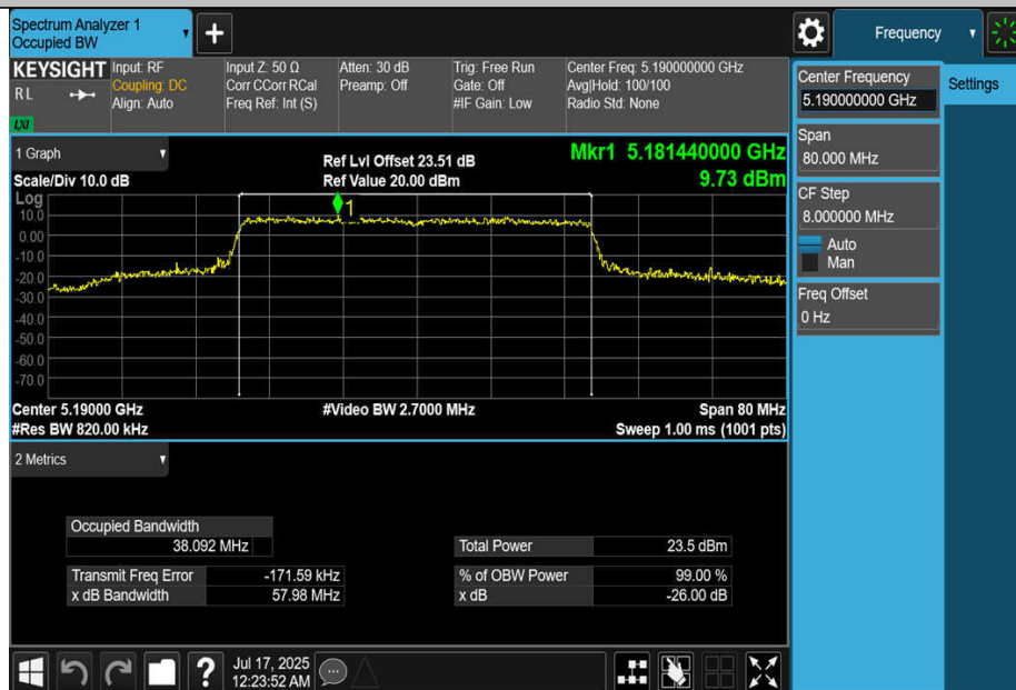
11BE40MIMO-Ant2-5190
