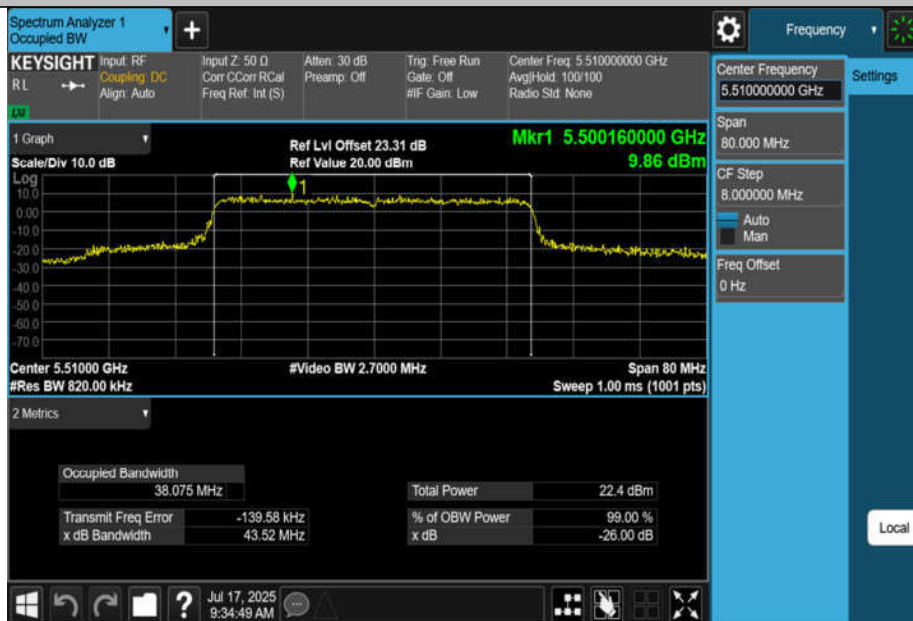
11BE40MIMO-Ant2-5510
