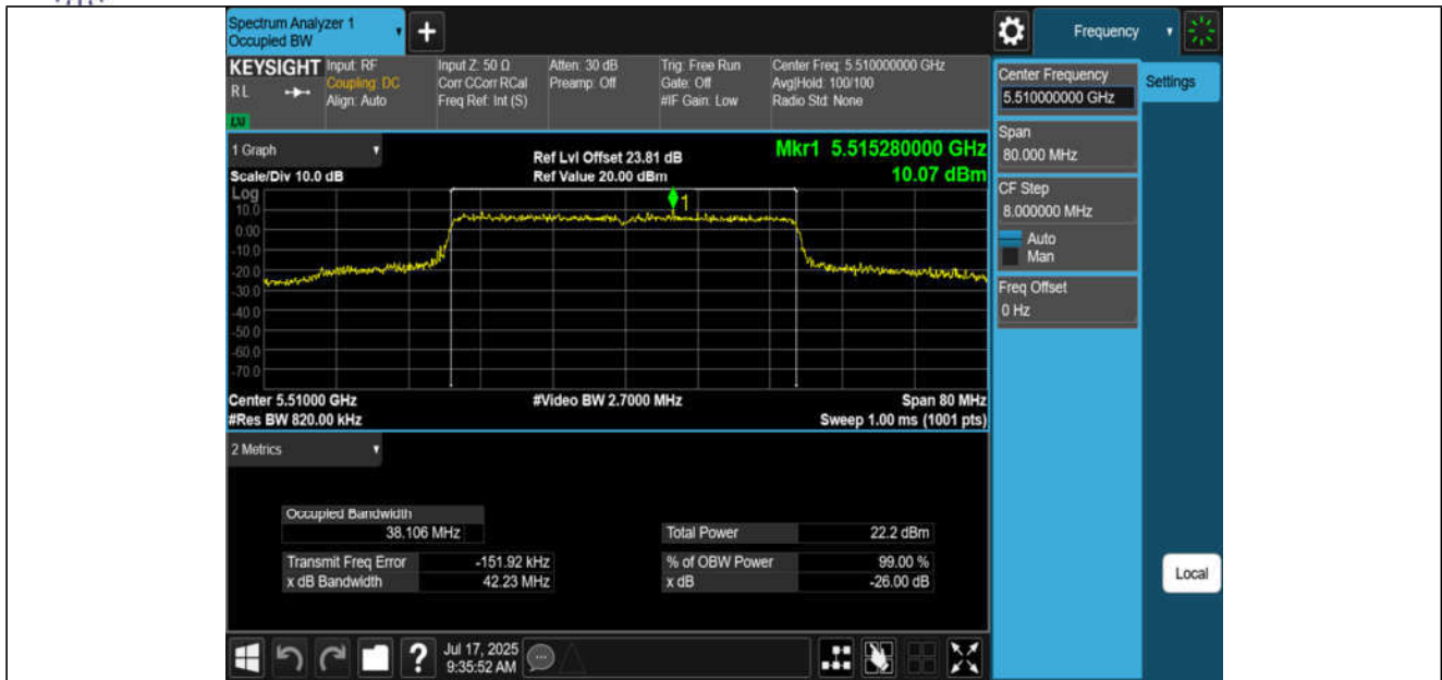
11BE40MIMO-Ant3-5510
