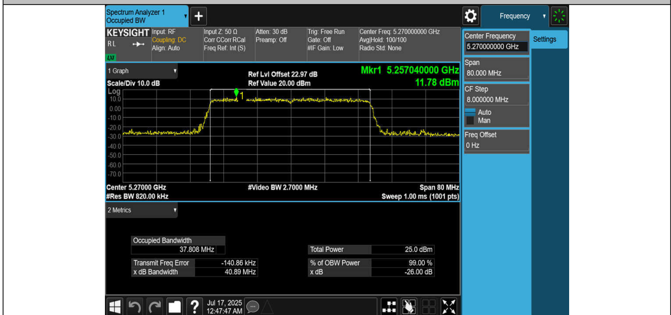
11BE40MIMO-Ant2-5270
