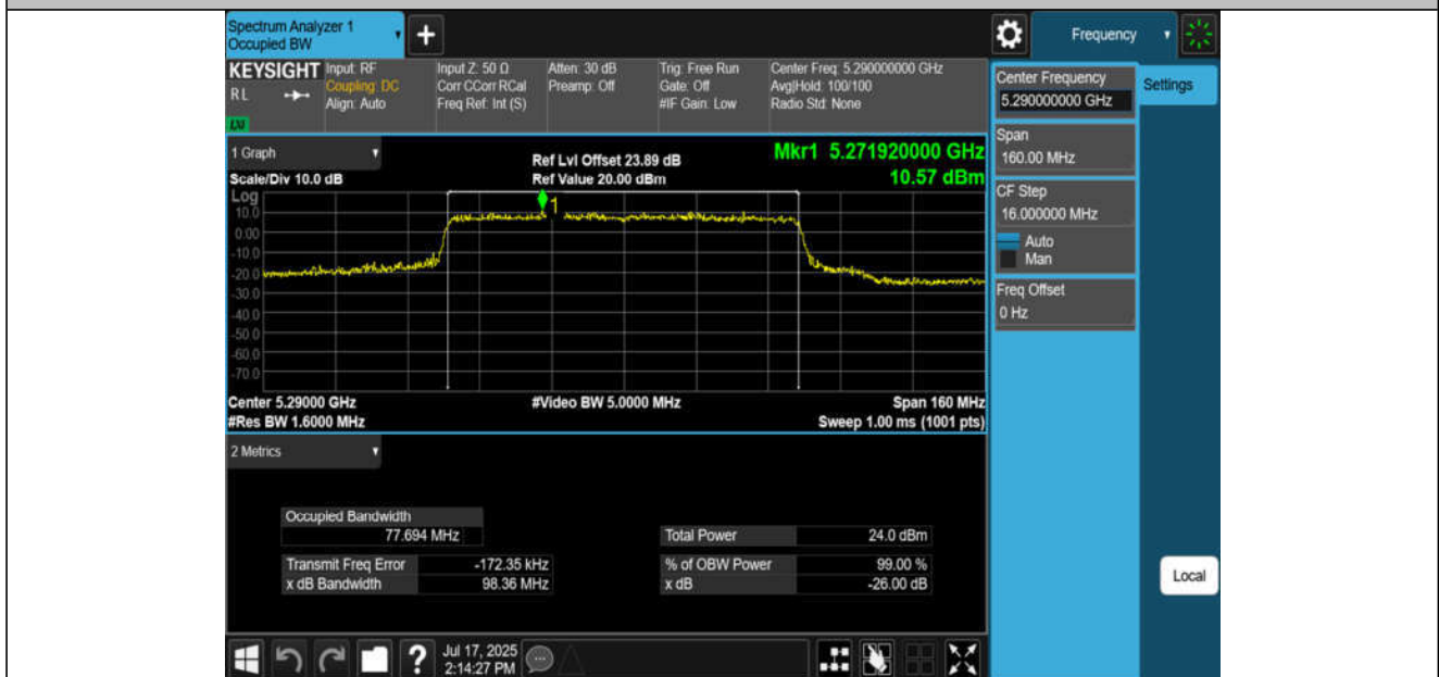
11BE80MIMO-Ant4-5290
