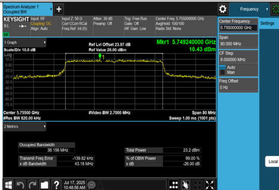
11BE40MIMO-Ant2-5755
