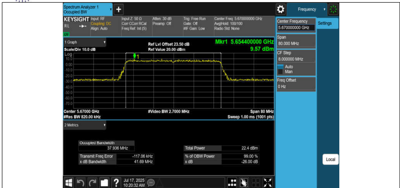
11BE40MIMO-Ant1-5670
