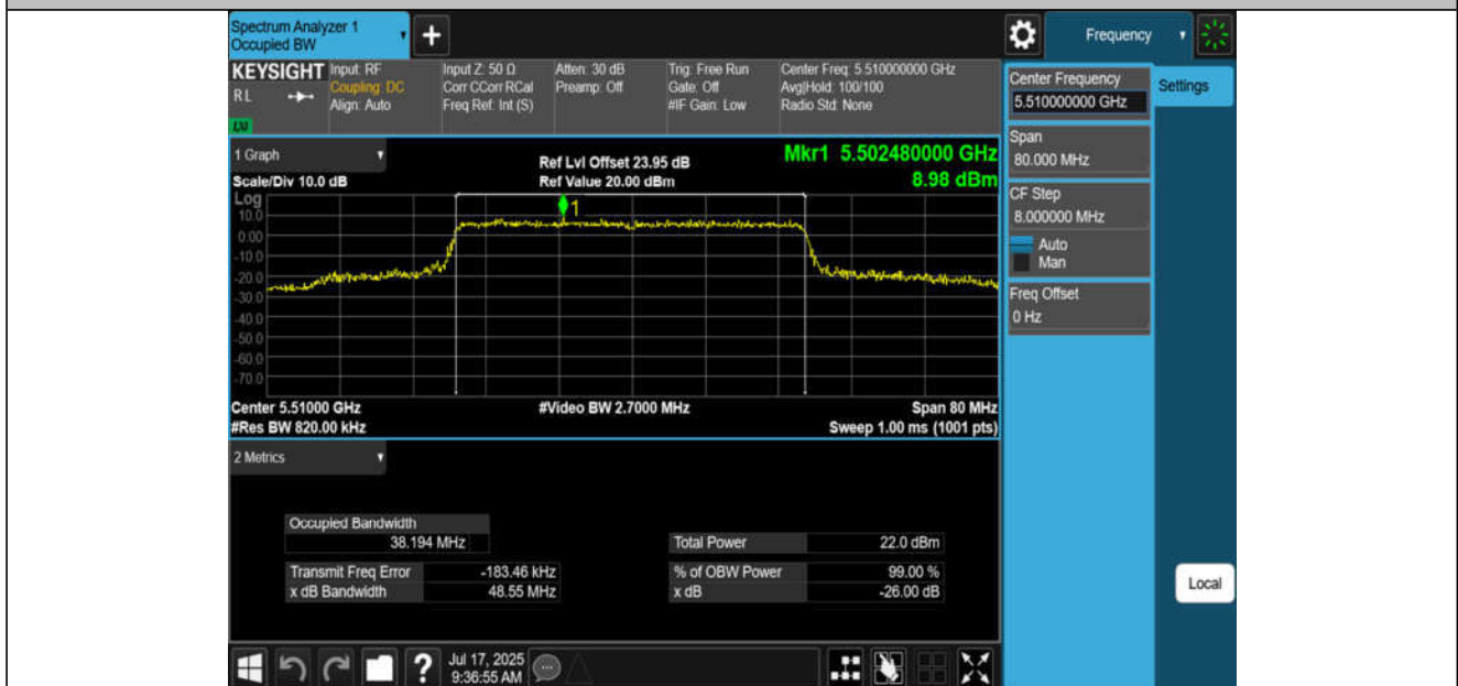
11BE40MIMO-Ant4-5510
