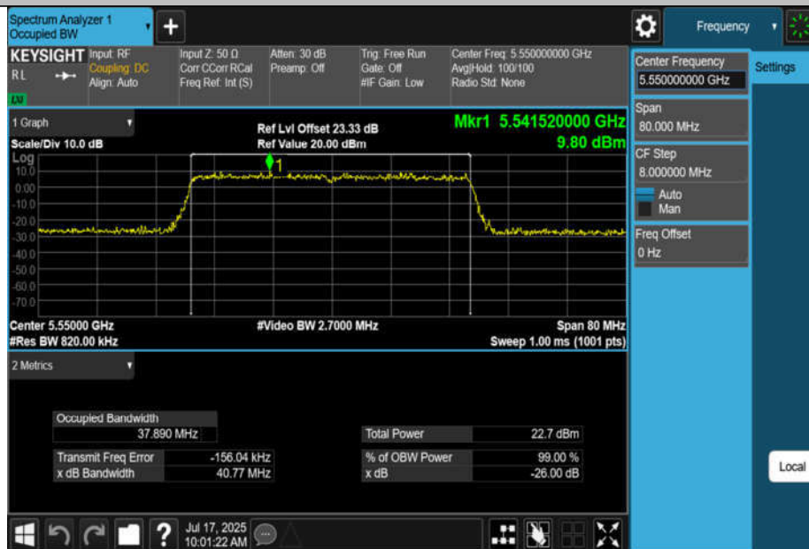
11BE40MIMO-Ant2-5550
