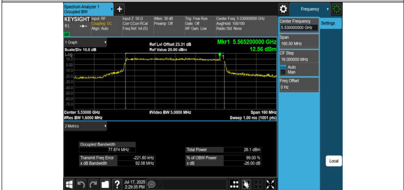
11BE80MIMO-Ant2-5530
