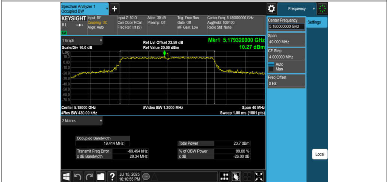
11BE20MIMO-Ant4-5180
