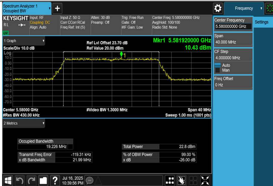
11BE20MIMO-Ant4-5580
