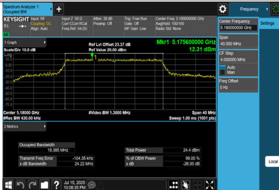
11BE20MIMO-Ant2-5180
