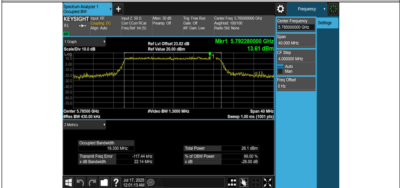
11BE20MIMO-Ant2-5785
