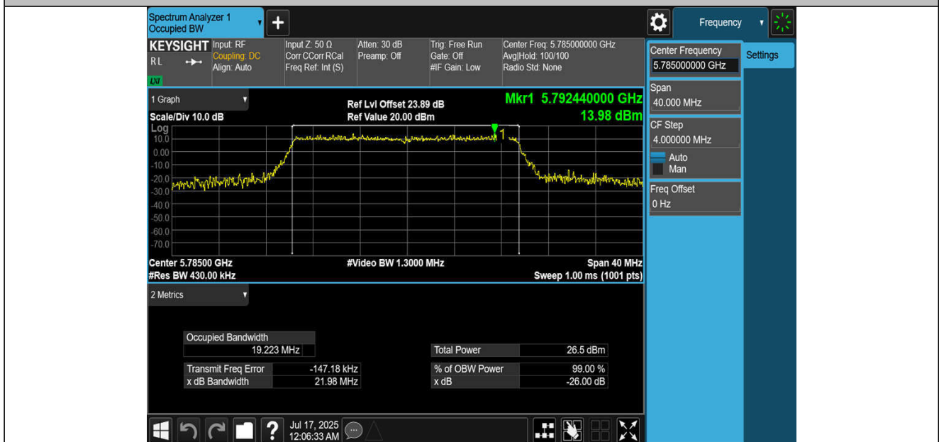
11BE20MIMO-Ant4-5785
