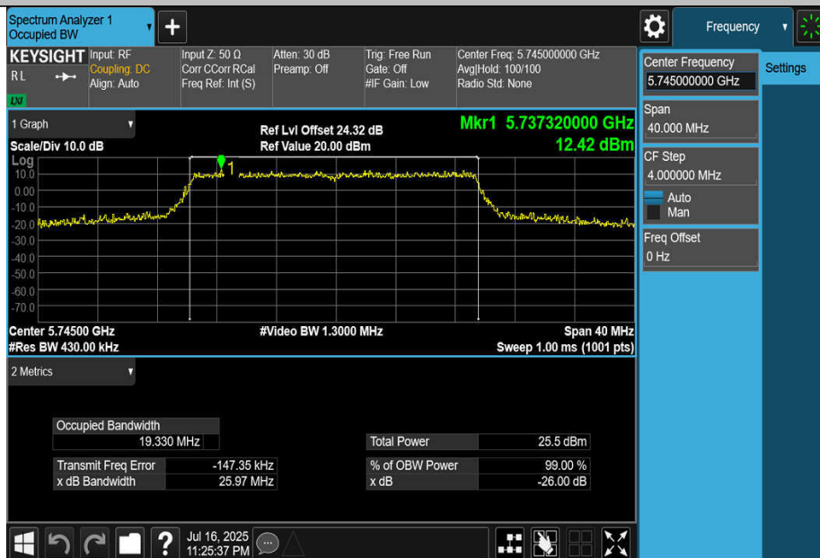
11BE20MIMO-Ant4-5745
