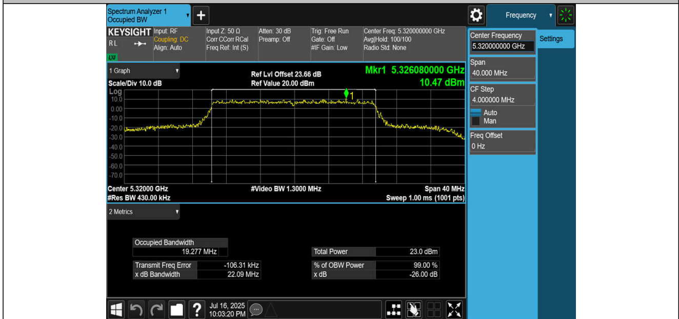
11BE20MIMO-Ant2-5320
