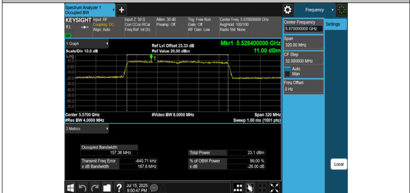
11AX160MIMO-Ant2-5570
