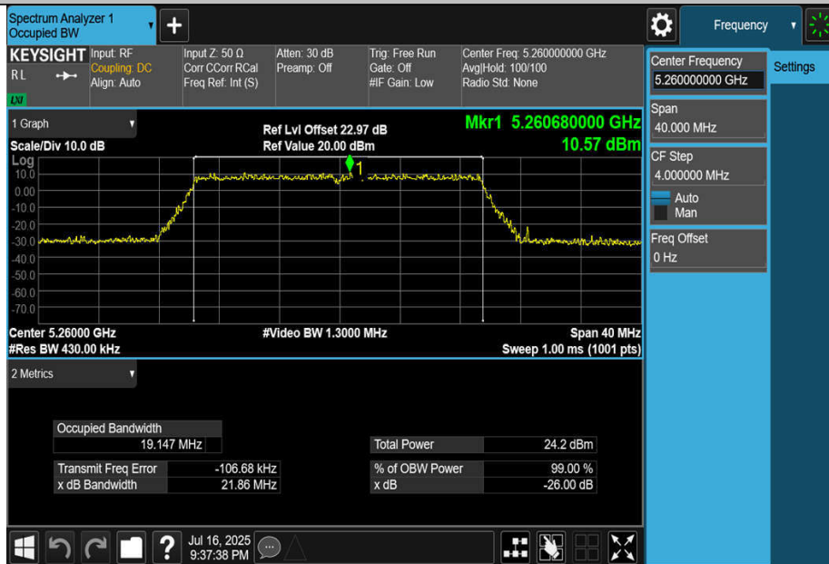
11BE20MIMO-Ant2-5260
