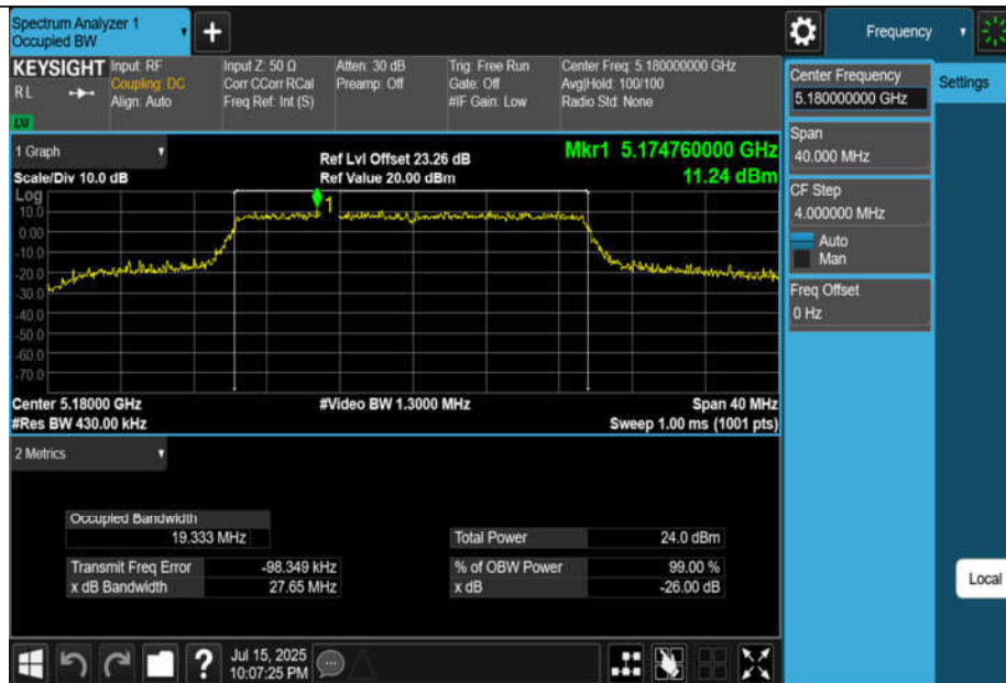
11BE20MIMO-Ant1-5180
