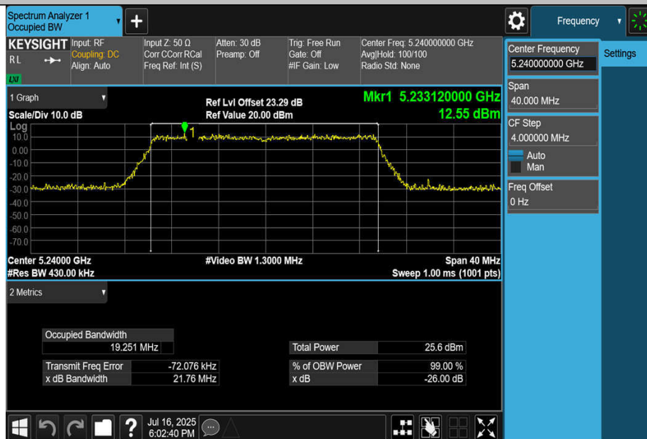
11BE20MIMO-Ant4-5240
