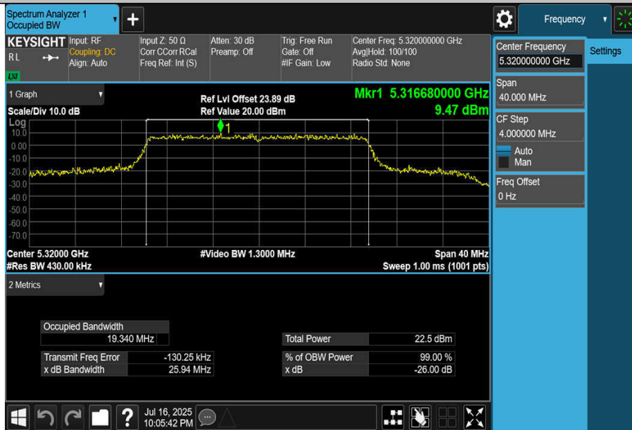
11BE20MIMO-Ant4-5320
