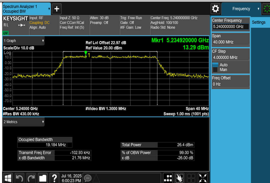
11BE20MIMO-Ant2-5240
