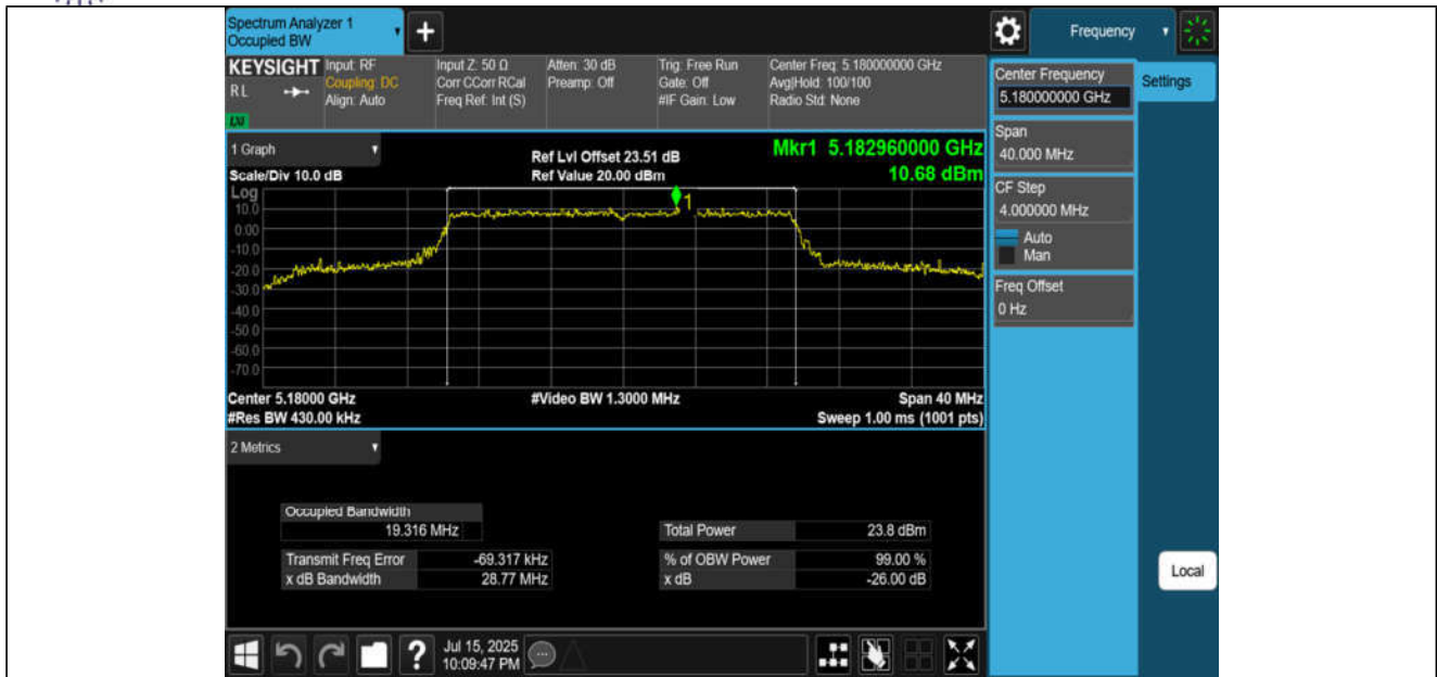
11BE20MIMO-Ant3-5180
