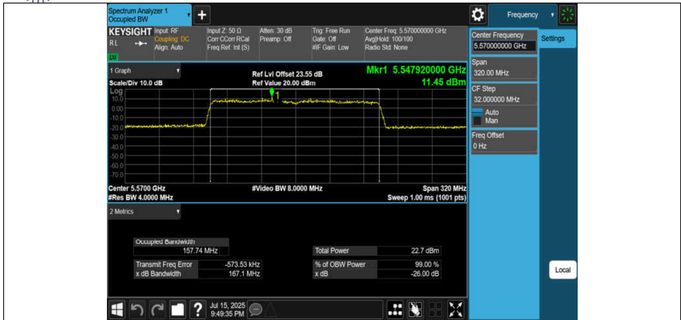
11AX160MIMO-Ant1-5570
