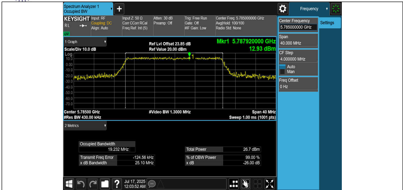
11BE20MIMO-Ant3-5785
