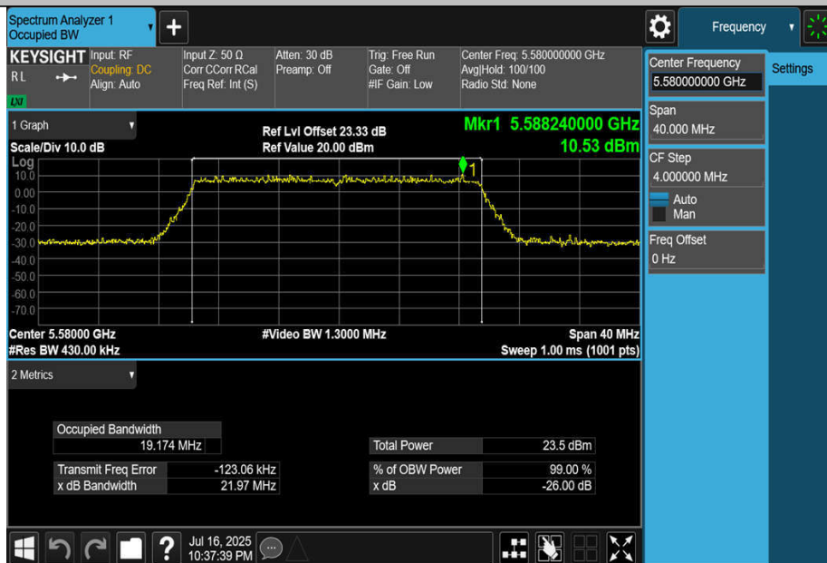
11BE20MIMO-Ant2-5580
