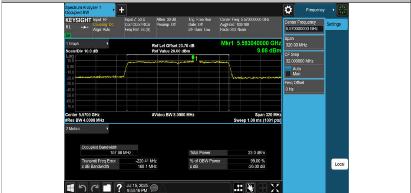
11AX160MIMO-Ant4-5570
