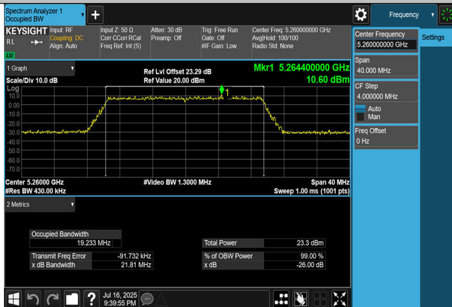
11BE20MIMO-Ant4-5260
