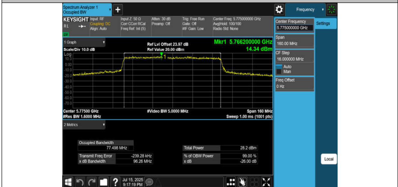
11AX80MIMO-Ant2-5775
