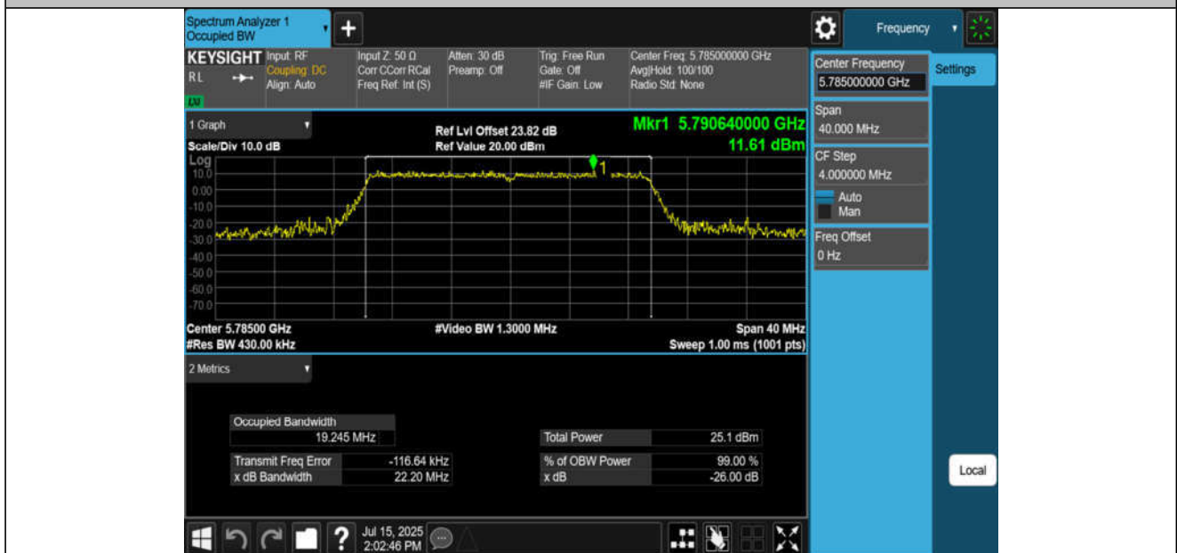
11AX20MIMO-Ant2-5785
