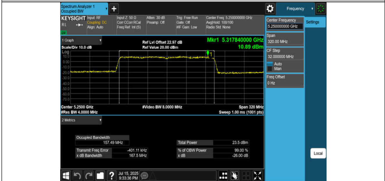
11AX160MIMO-Ant2-5250
