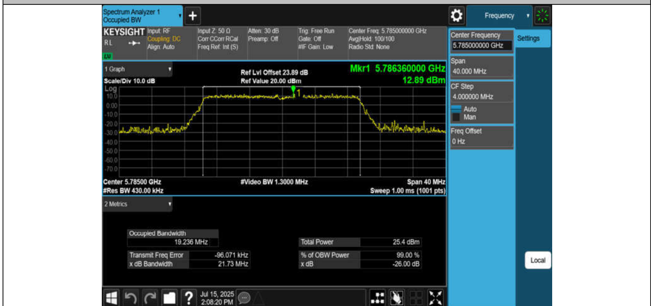
11AX20MIMO-Ant4-5785
