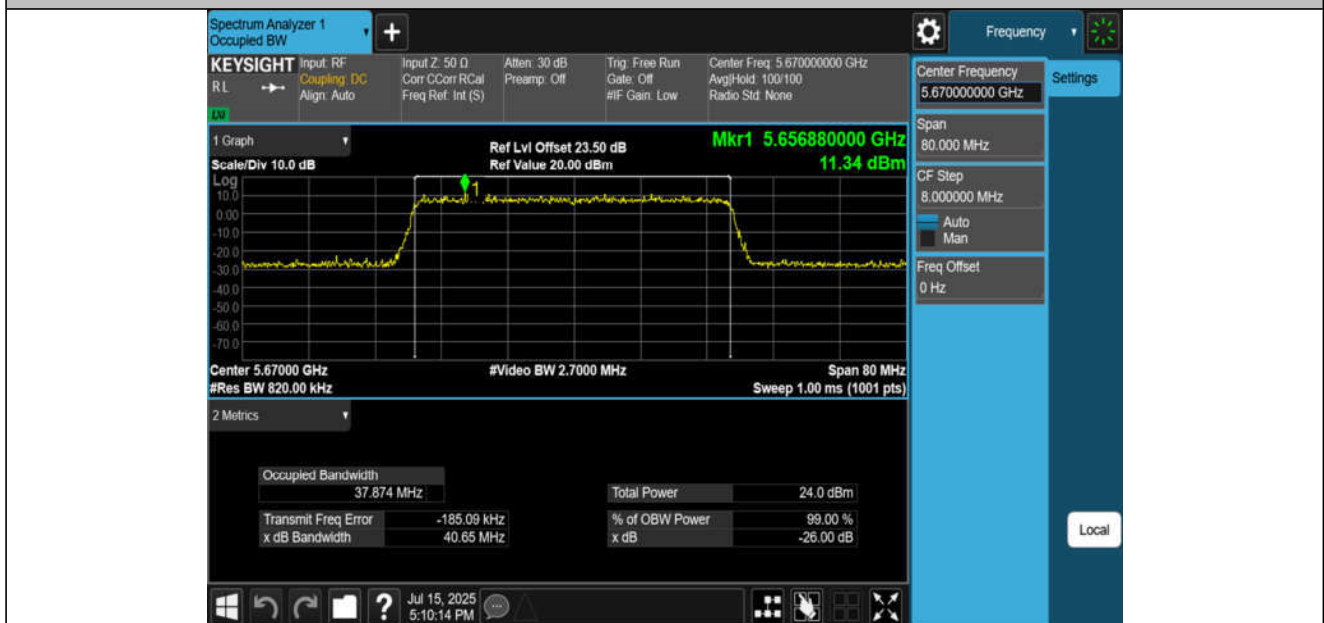
11AX40MIMO-Ant2-5670
