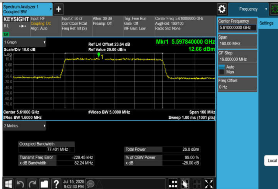
11AX80MIMO-Ant4-5610
