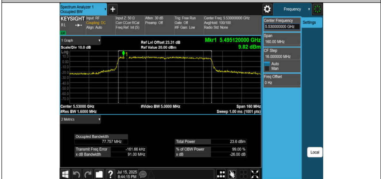
11AX80MIMO-Ant2-5530
