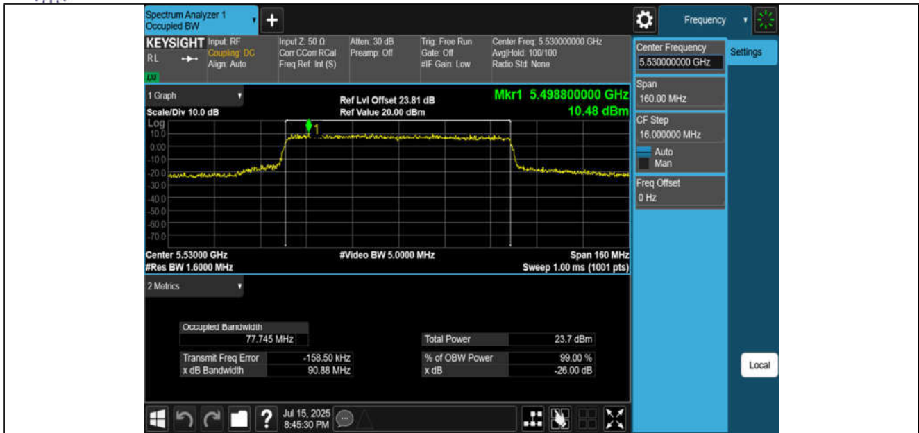
11AX80MIMO-Ant3-5530
