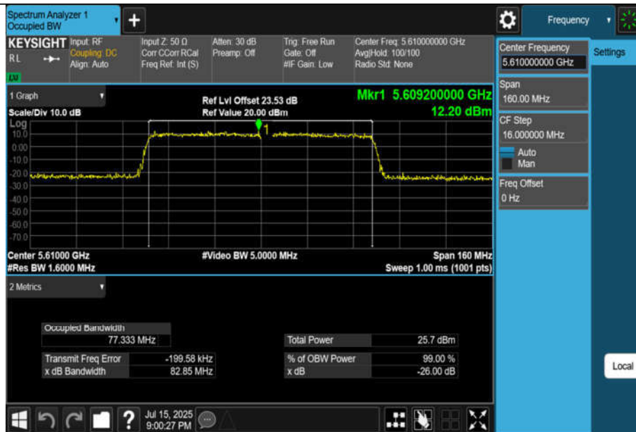
11AX80MIMO-Ant3-5610
