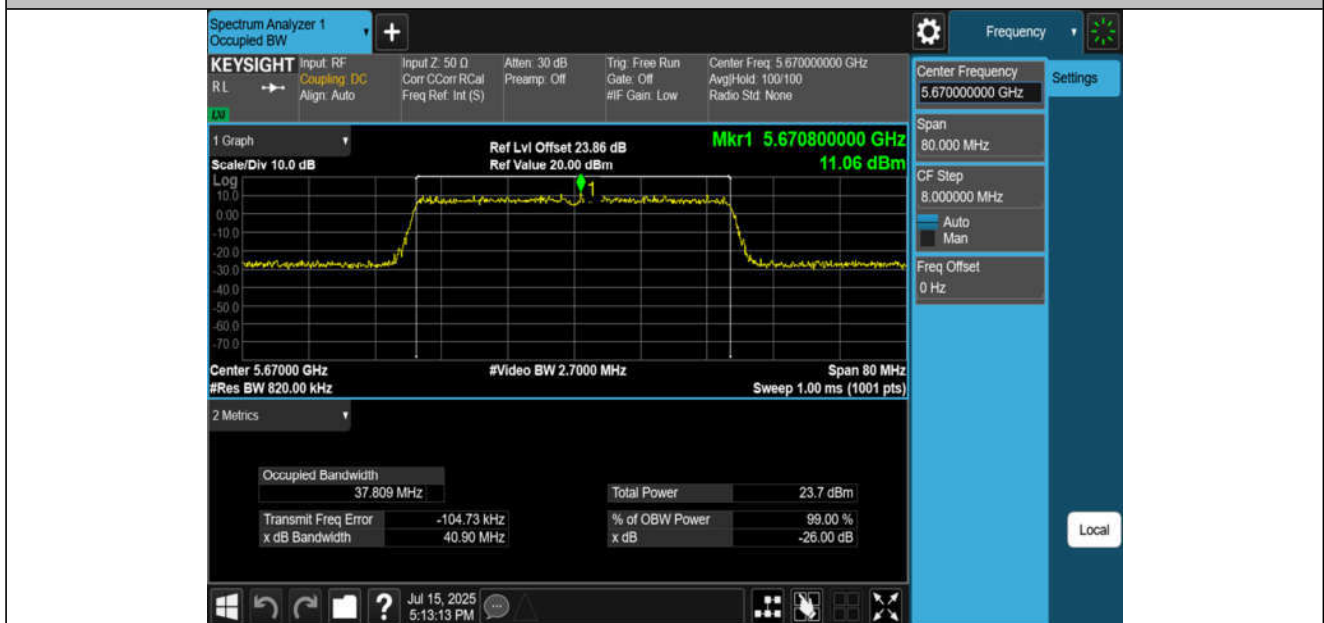
11AX40MIMO-Ant4-5670
