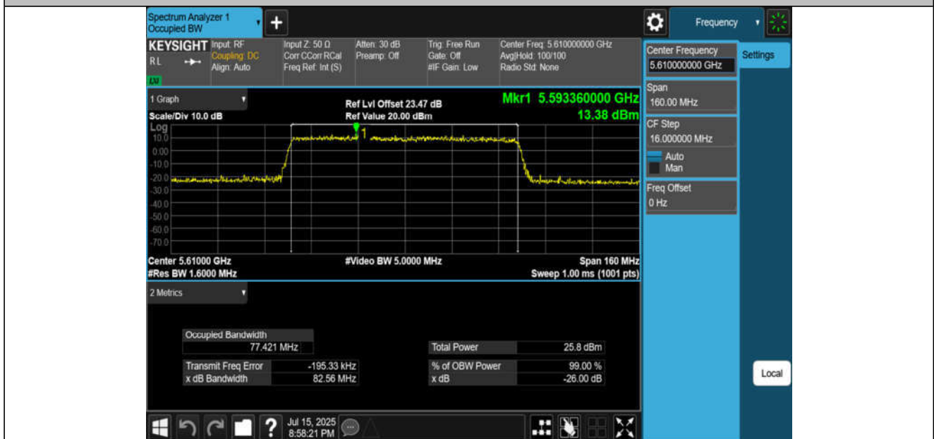
11AX80MIMO-Ant2-5610
