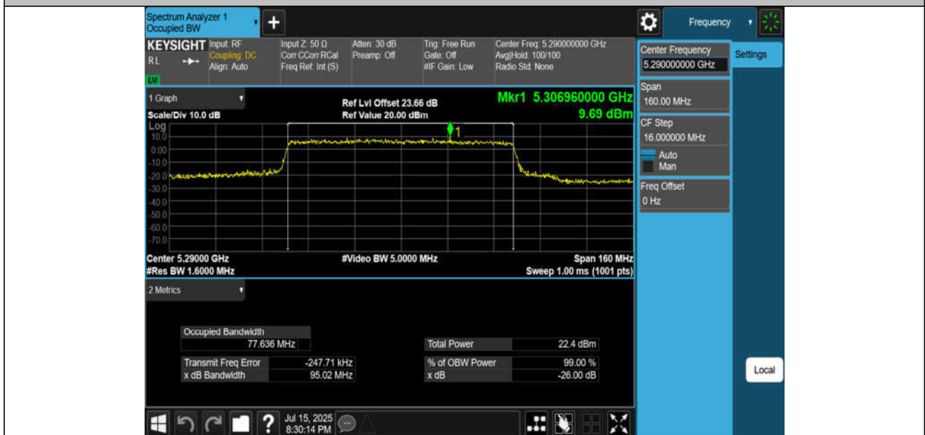
11AX80MIMO-Ant2-5290
