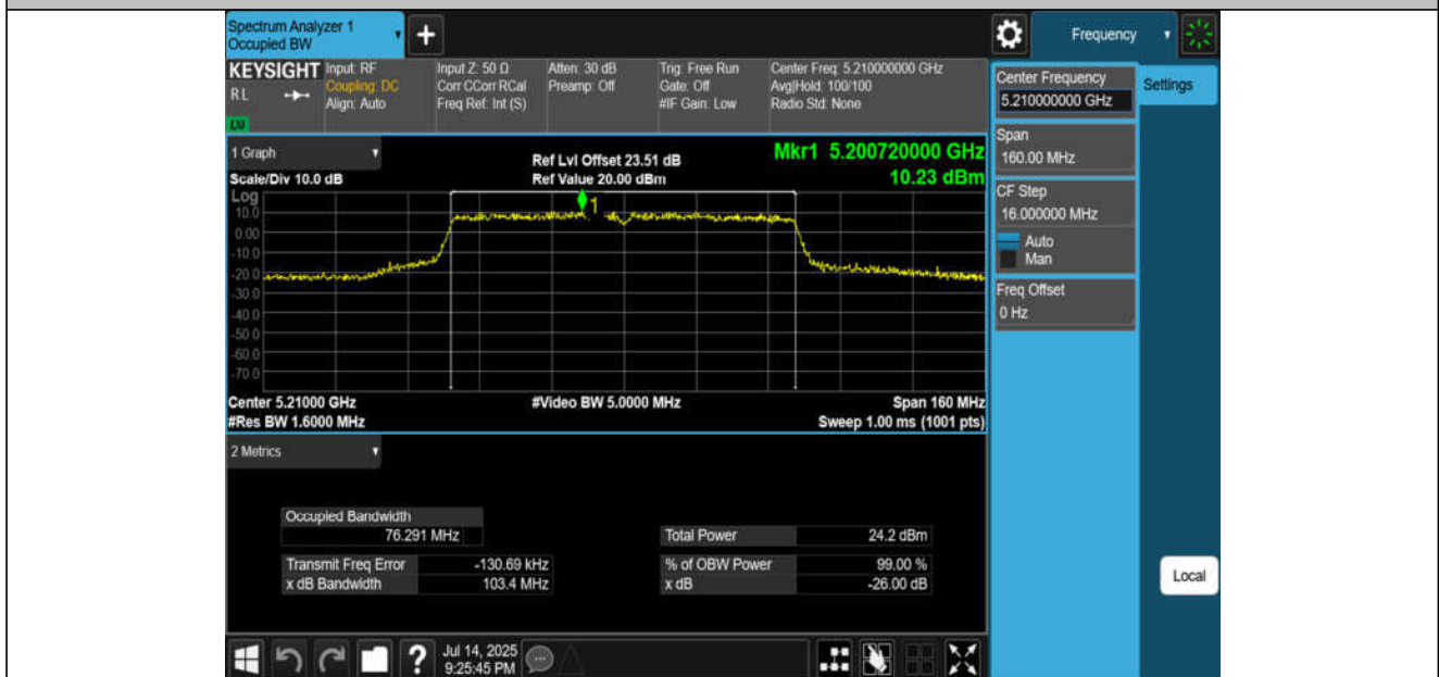
11AC80MIMO-Ant2-5210
