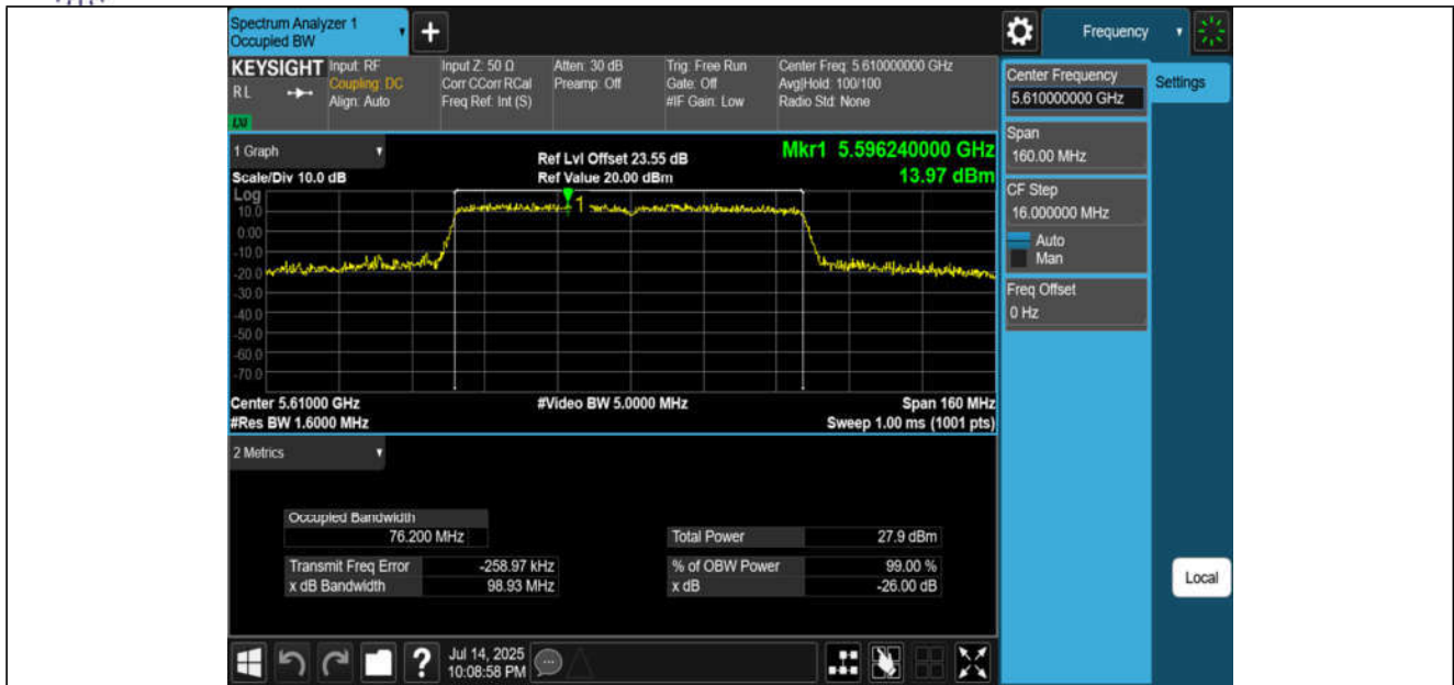
11AC80MIMO-Ant1-5610
