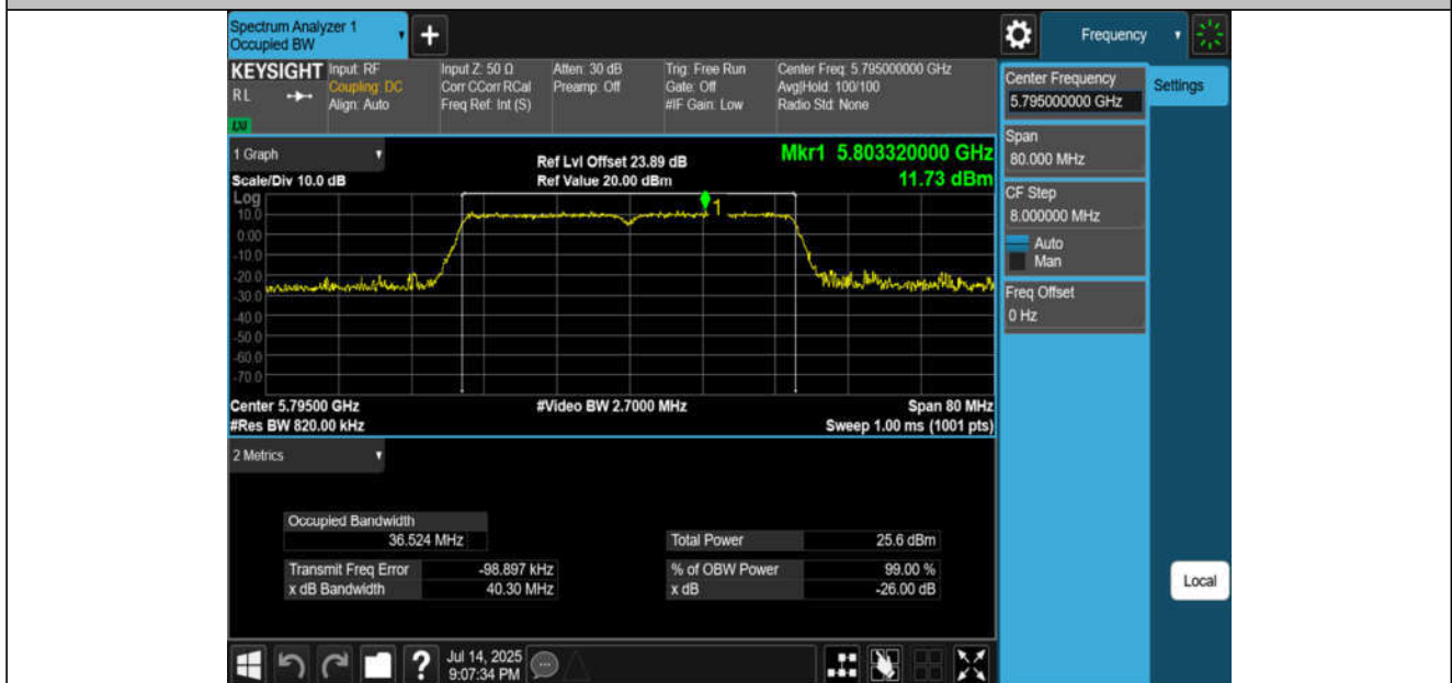
11AC40MIMO-Ant4-5795
