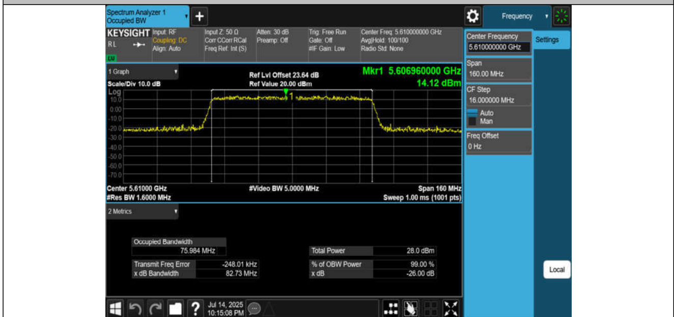
11AC80MIMO-Ant4-5610
