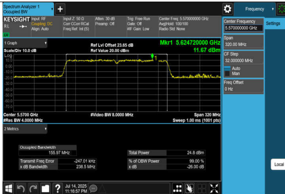
11AC160MIMO-Ant3-5570
