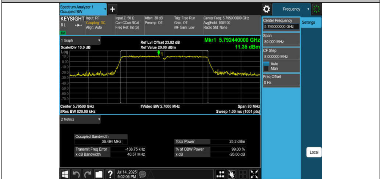
11AC40MIMO-Ant2-5795
