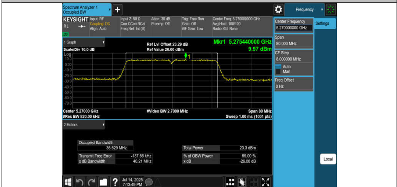
11AC40MIMO-Ant4-5270
