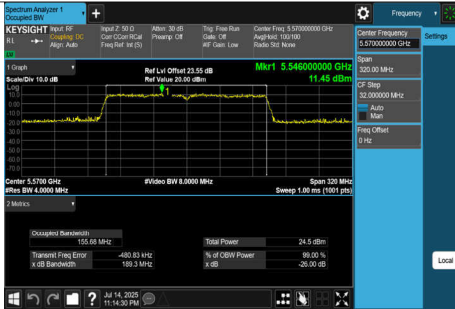
11AC160MIMO-Ant1-5570
