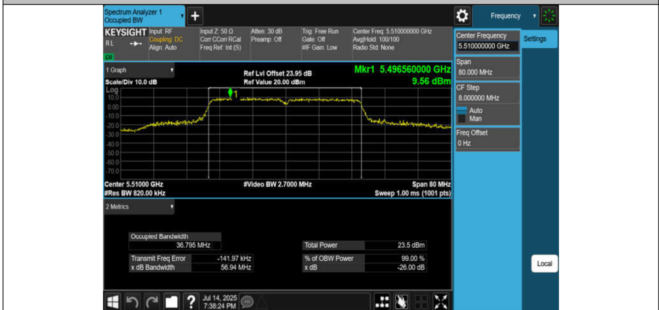
11AC40MIMO-Ant4-5510
