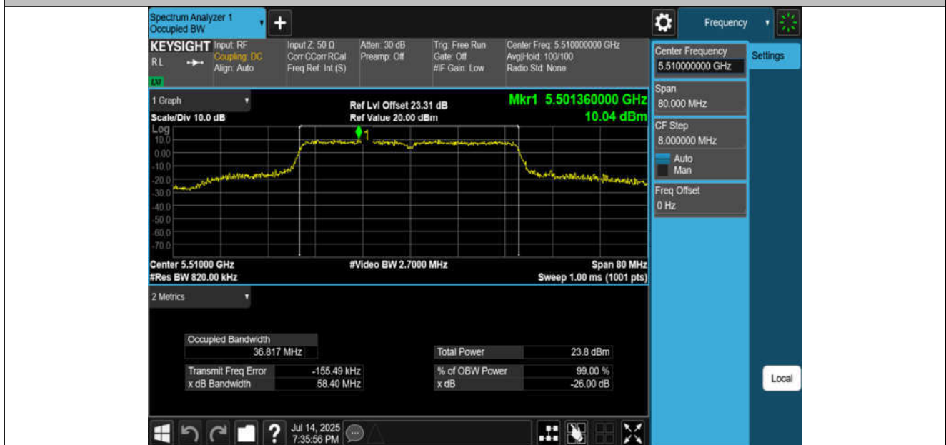
11AC40MIMO-Ant2-5510
