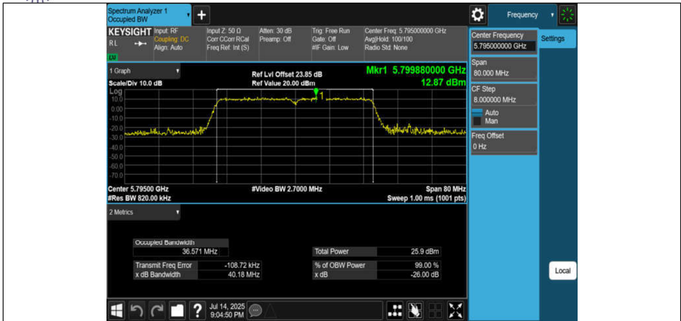
11AC40MIMO-Ant3-5795
