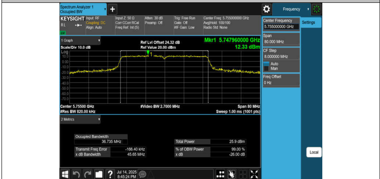
11AC40MIMO-Ant4-5755
