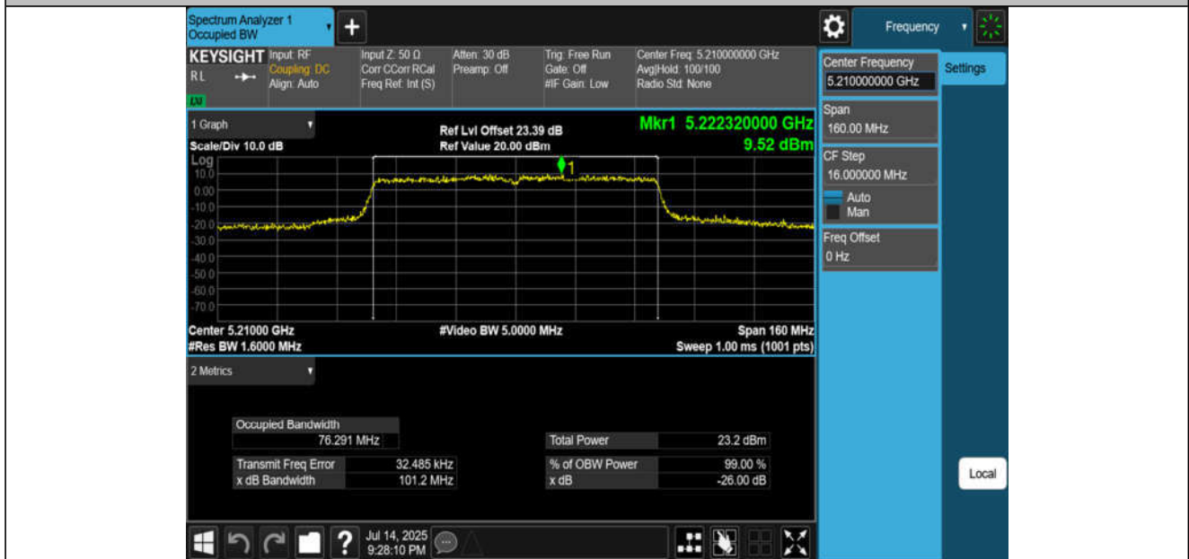
11AC80MIMO-Ant4-5210
