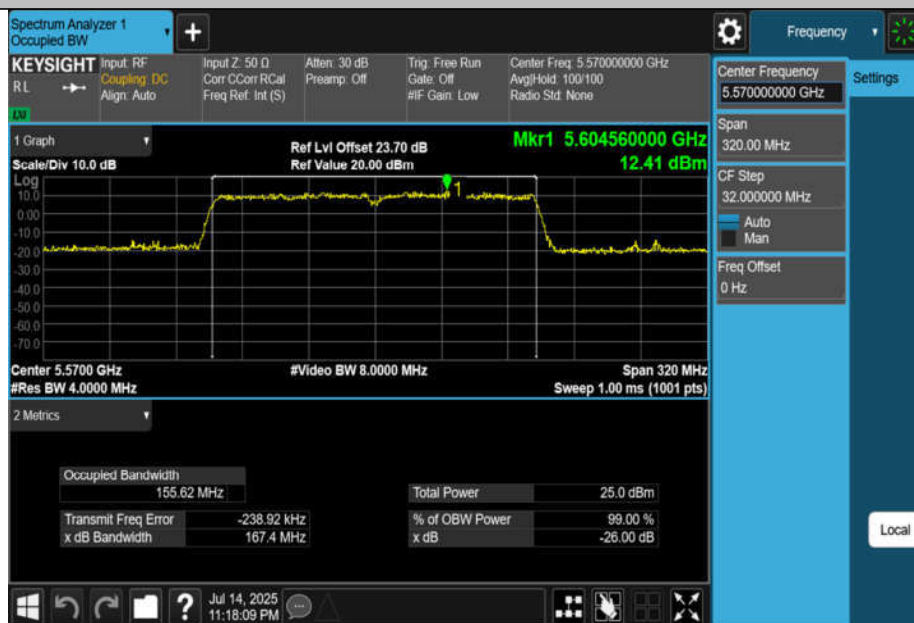
11AC160MIMO-Ant4-5570
