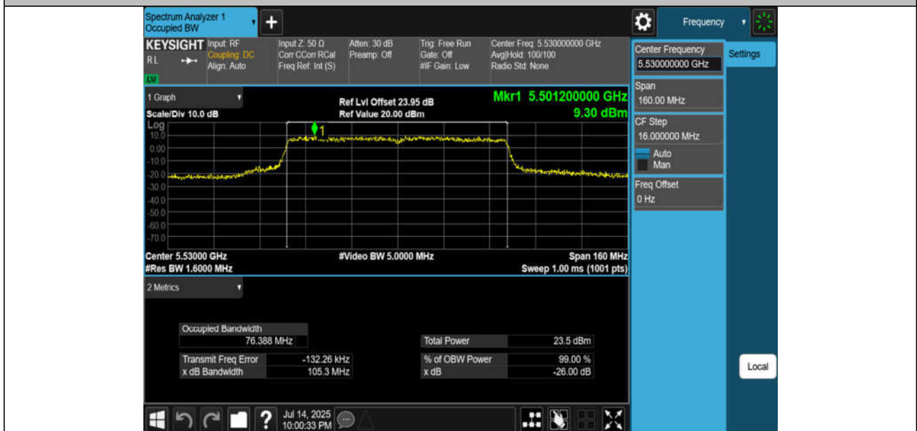
11AC80MIMO-Ant4-5530
