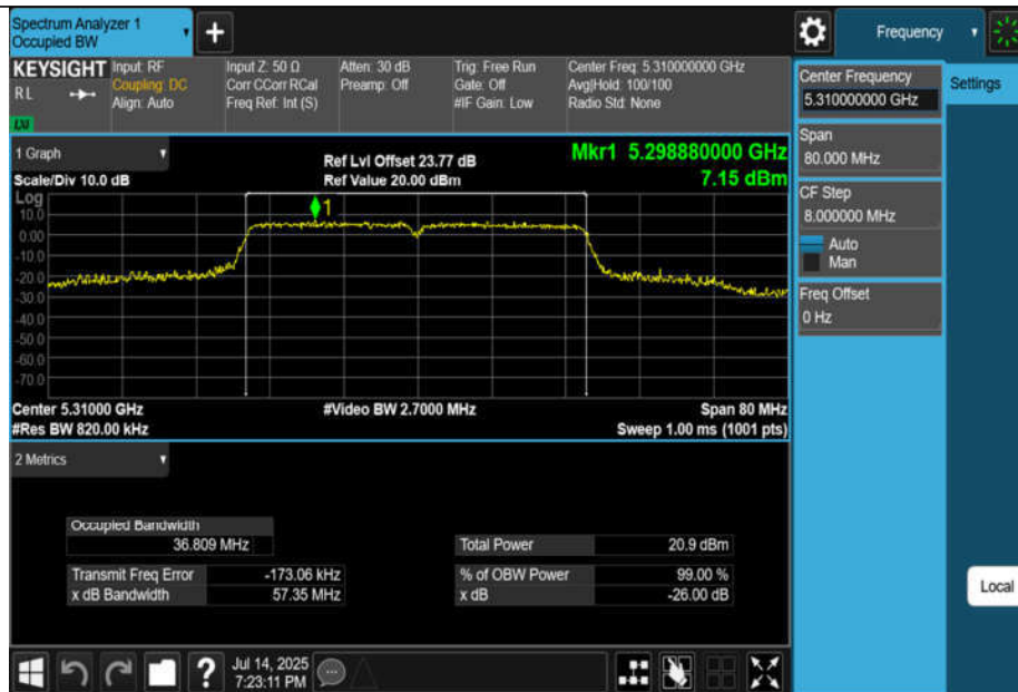
11AC40MIMO-Ant3-5310
