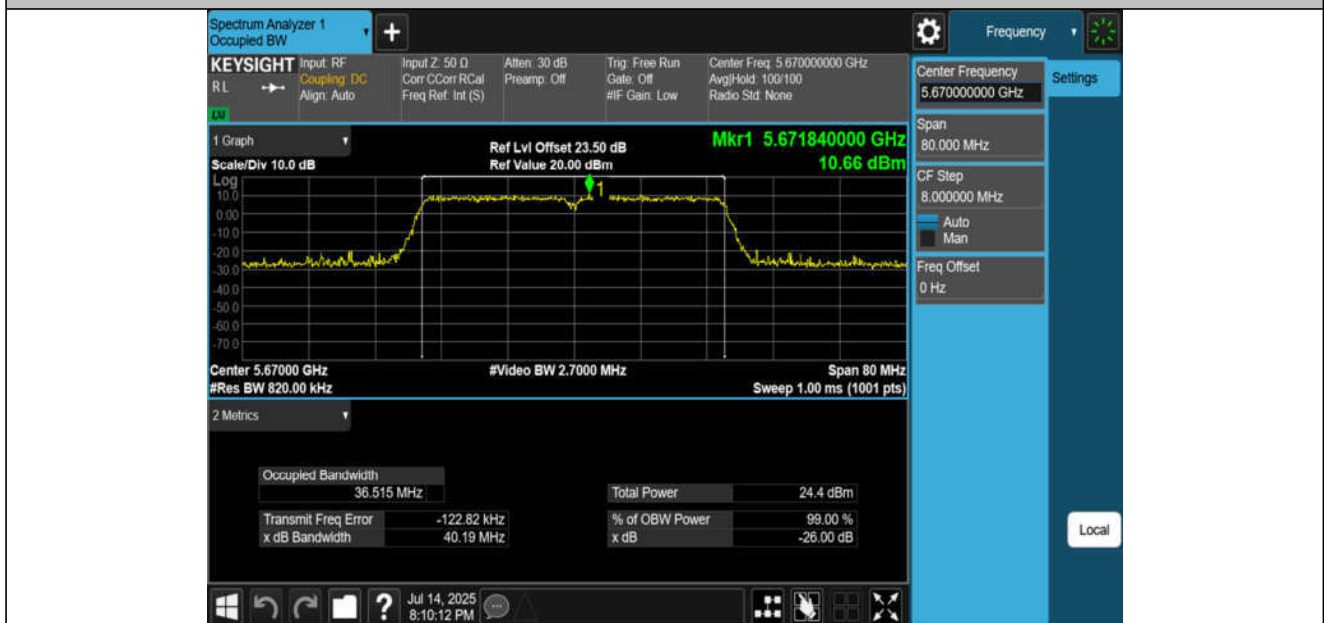
11AC40MIMO-Ant2-5670
