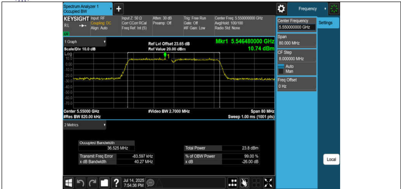
11AC40MIMO-Ant3-5550
