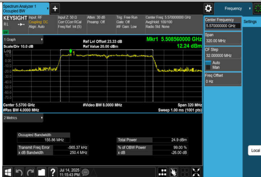
11AC160MIMO-Ant2-5570
