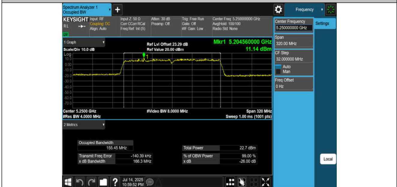
11AC160MIMO-Ant4-5250
