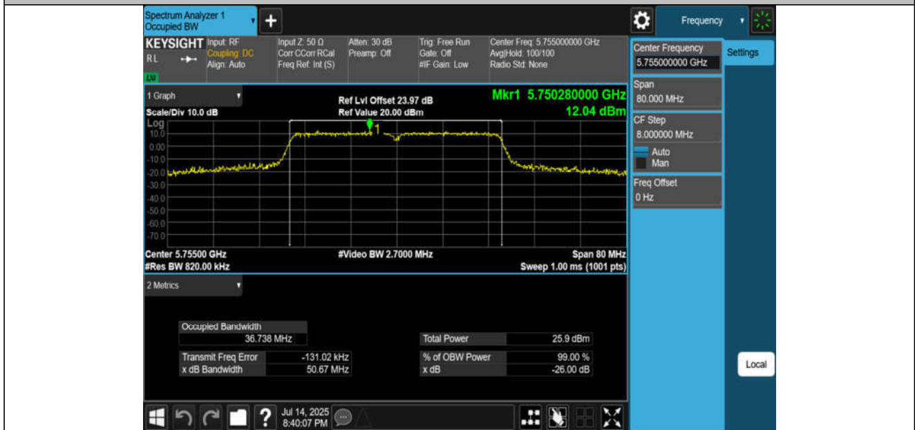
11AC40MIMO-Ant2-5755
