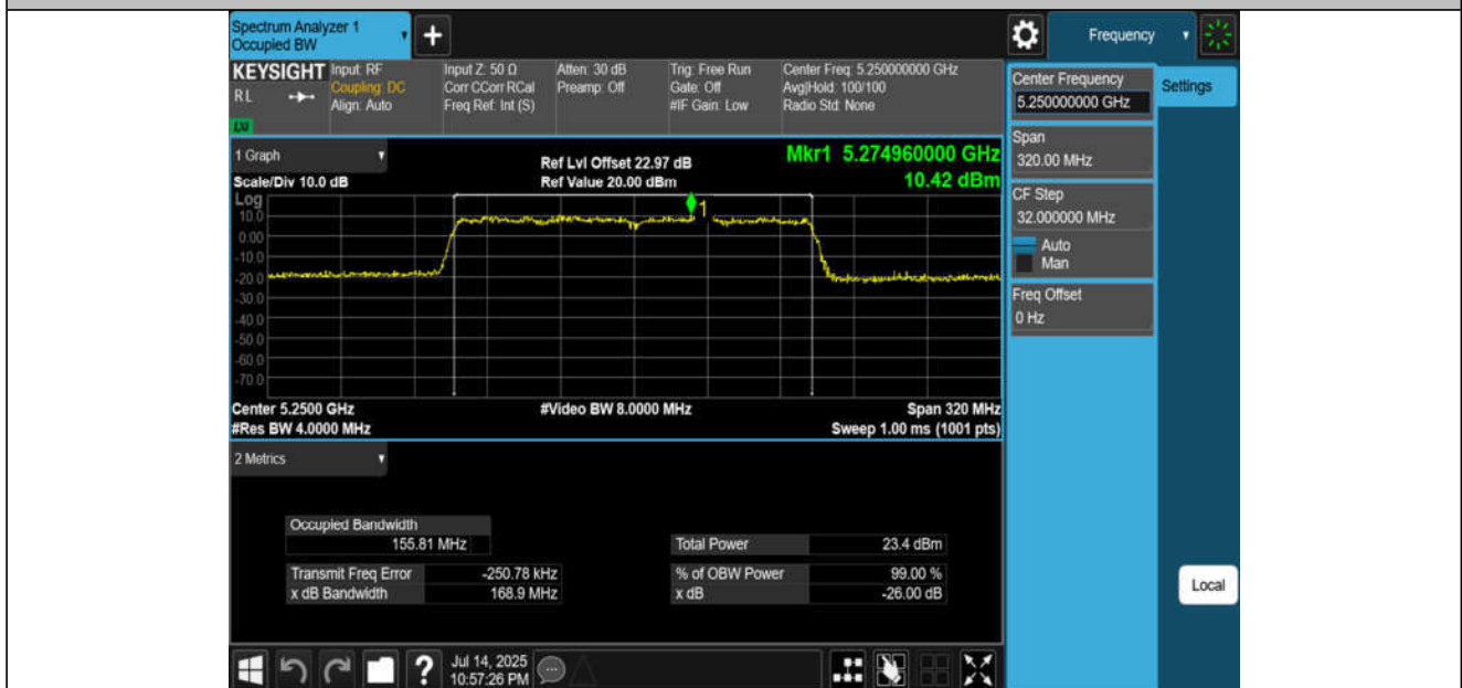
11AC160MIMO-Ant2-5250
