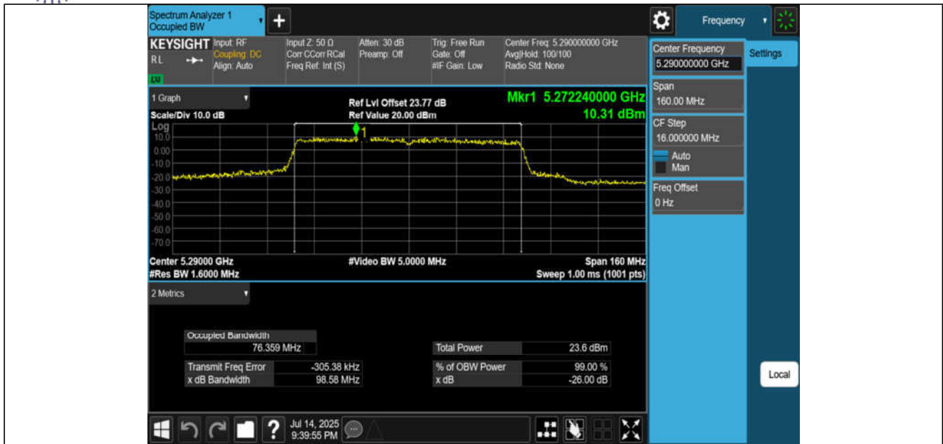
11AC80MIMO-Ant3-5290
