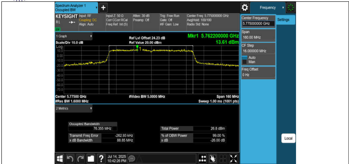
11AC80MIMO-Ant3-5775
