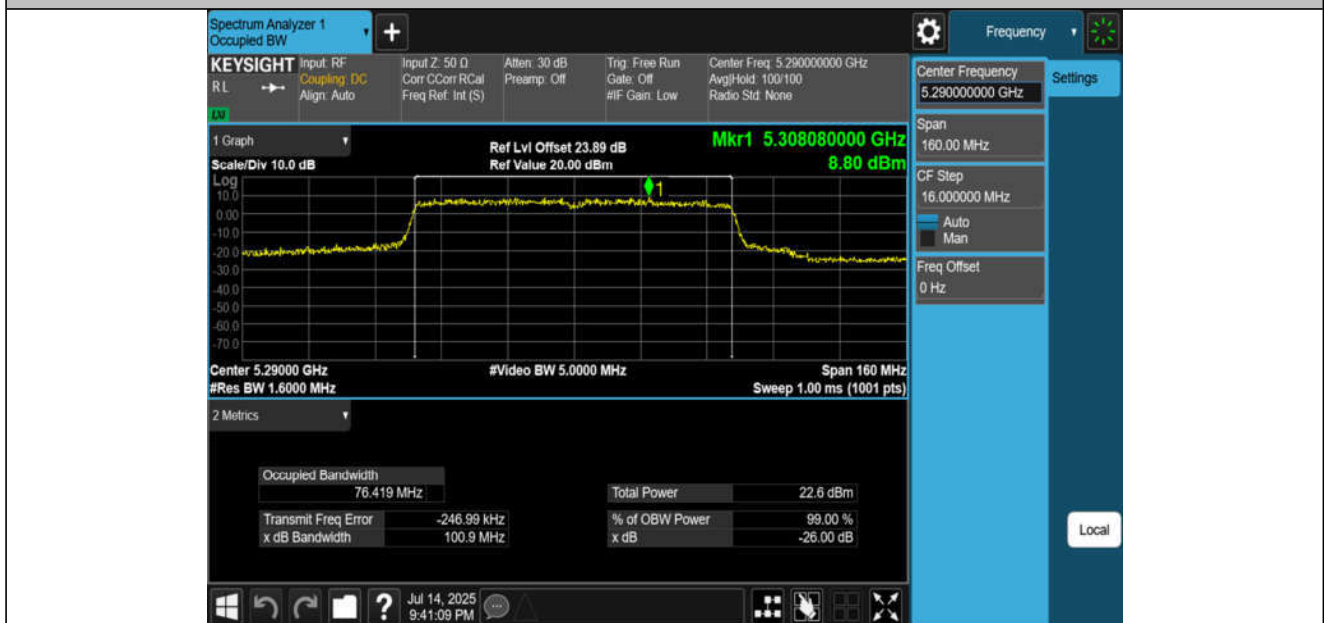
11AC80MIMO-Ant4-5290
