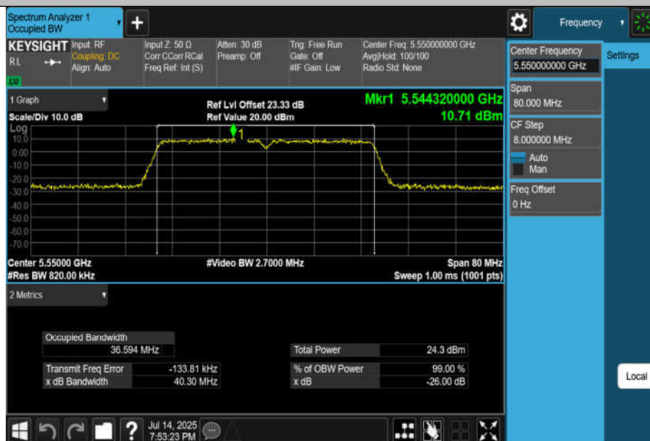
11AC40MIMO-Ant2-5550
