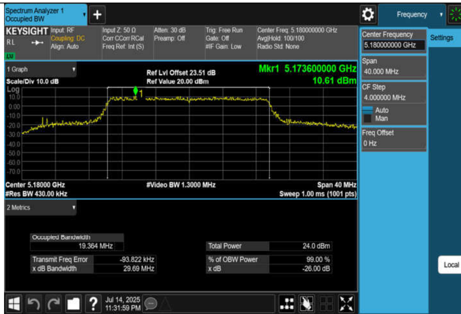
11AX20MIMO-Ant3-5180
