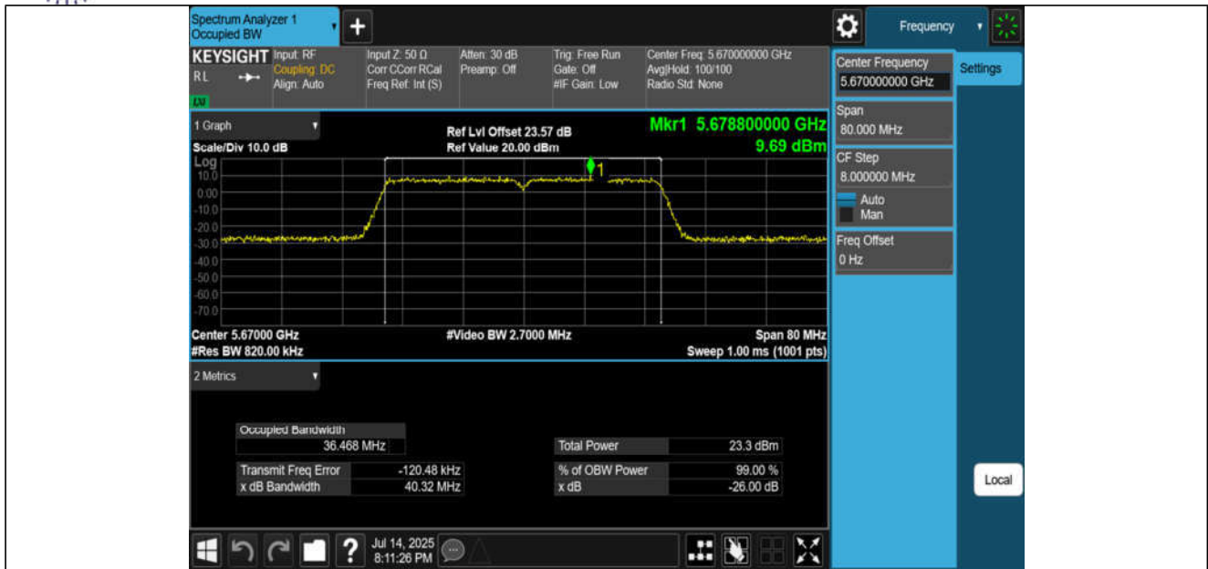
11AC40MIMO-Ant3-5670
