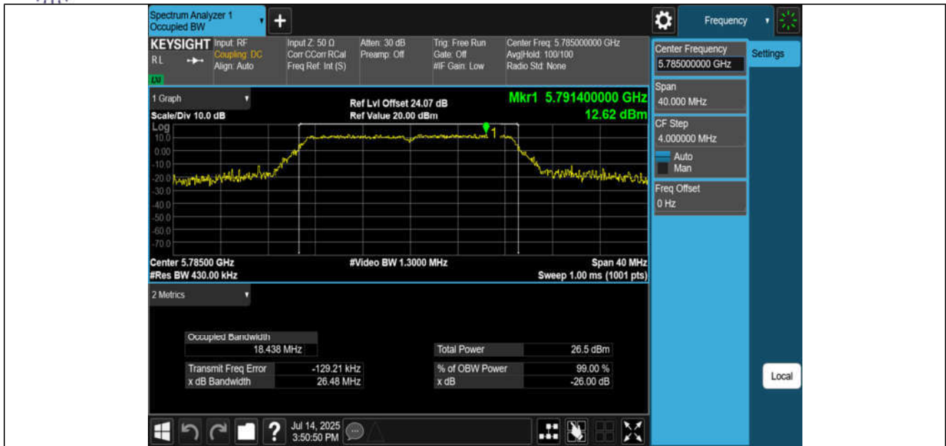
11AC20MIMO-Ant1-5785
