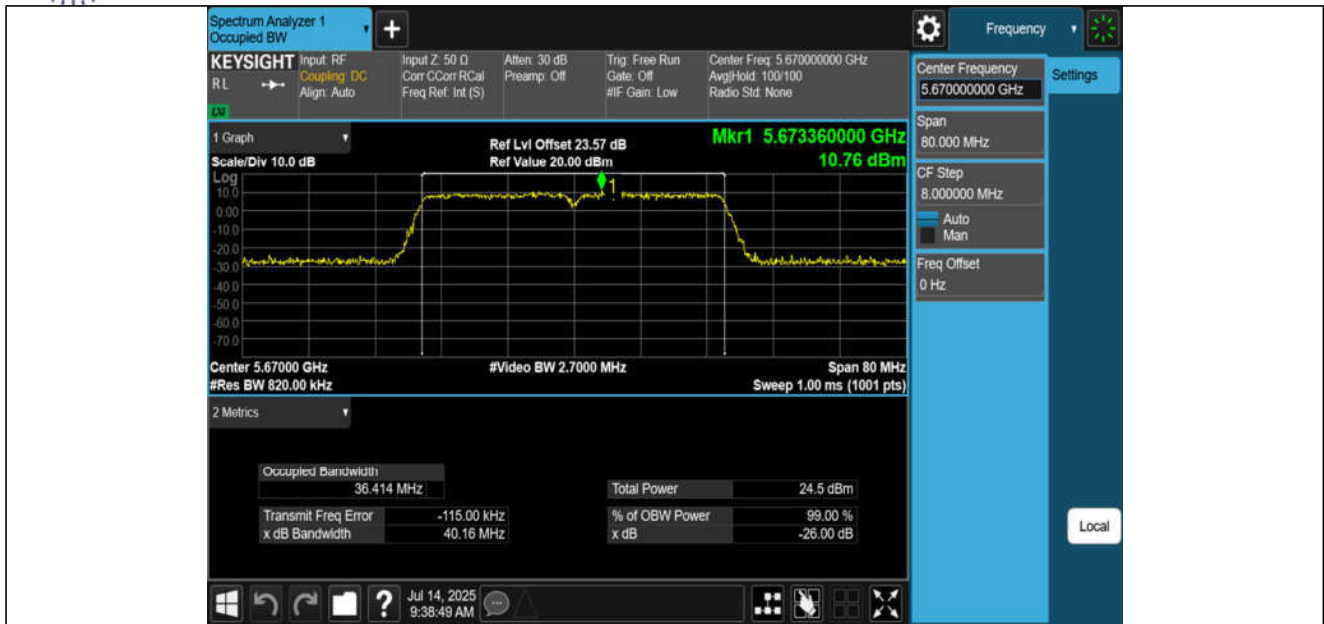
11N40MIMO-Ant3-5670
