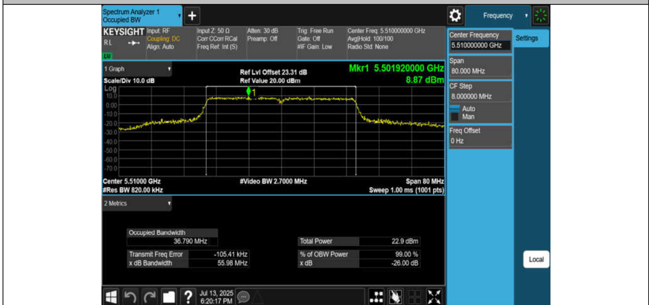
11N40MIMO-Ant2-5510
