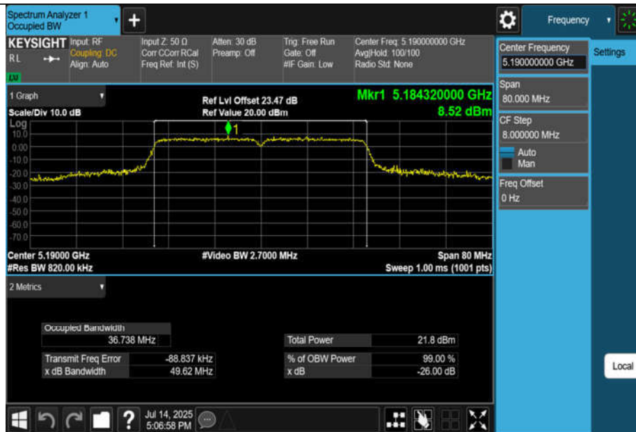
11AC40MIMO-Ant3-5190
