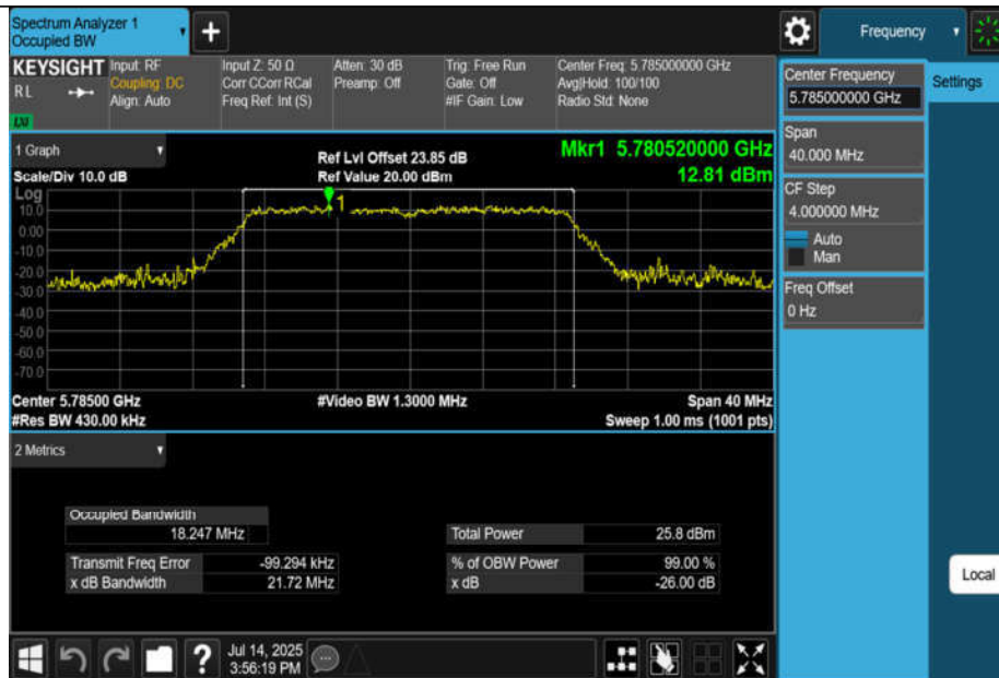
11AC20MIMO-Ant3-5785
