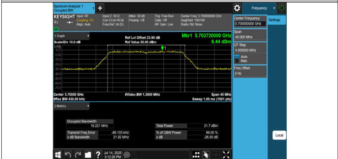
11AC20MIMO-Ant4-5700
