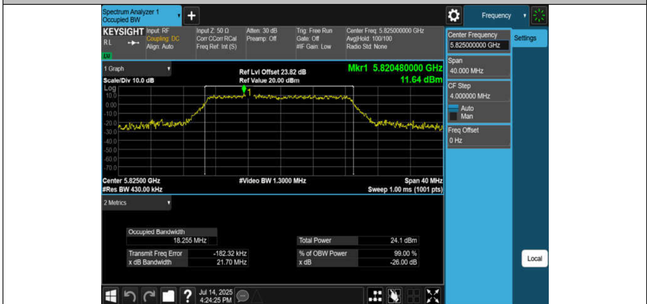
11AC20MIMO-Ant2-5825
