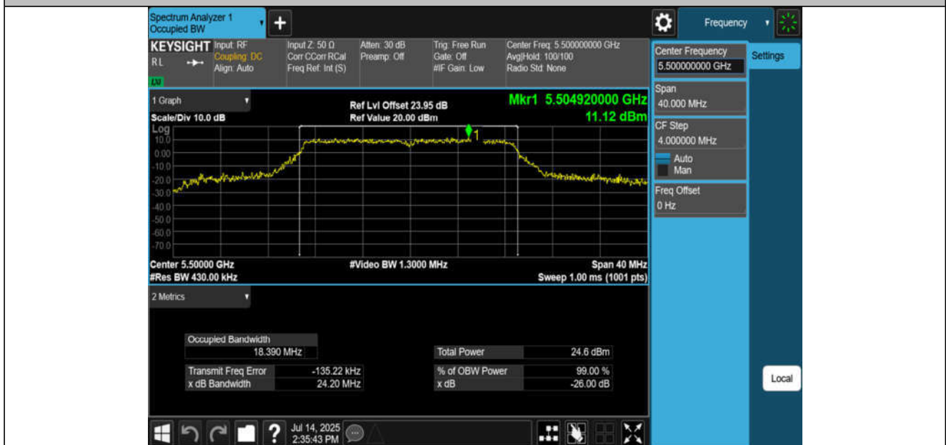
11AC20MIMO-Ant4-5500
