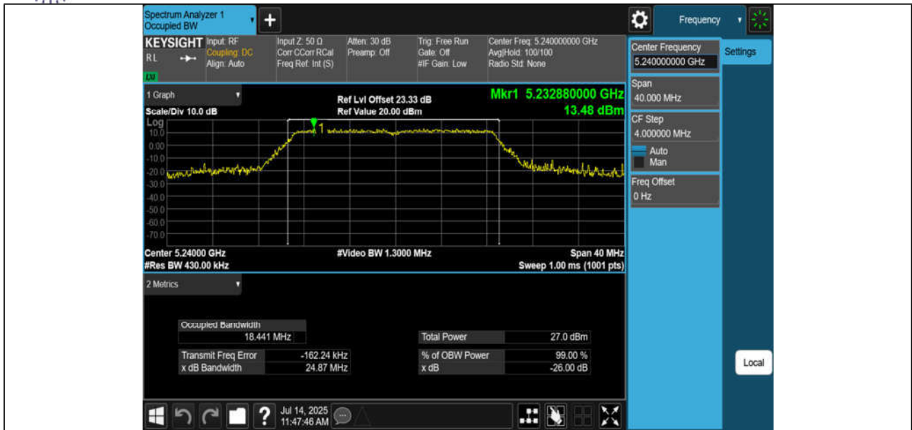
11AC20MIMO-Ant1-5240
