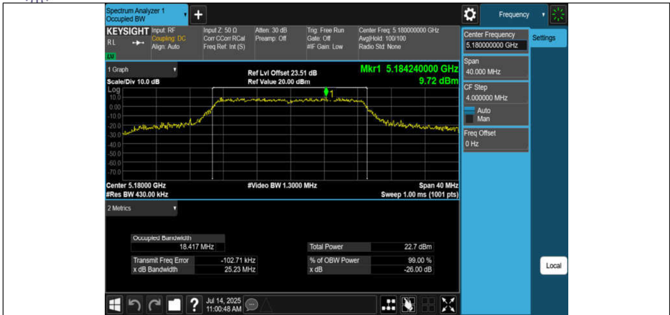
11AC20MIMO-Ant3-5180
