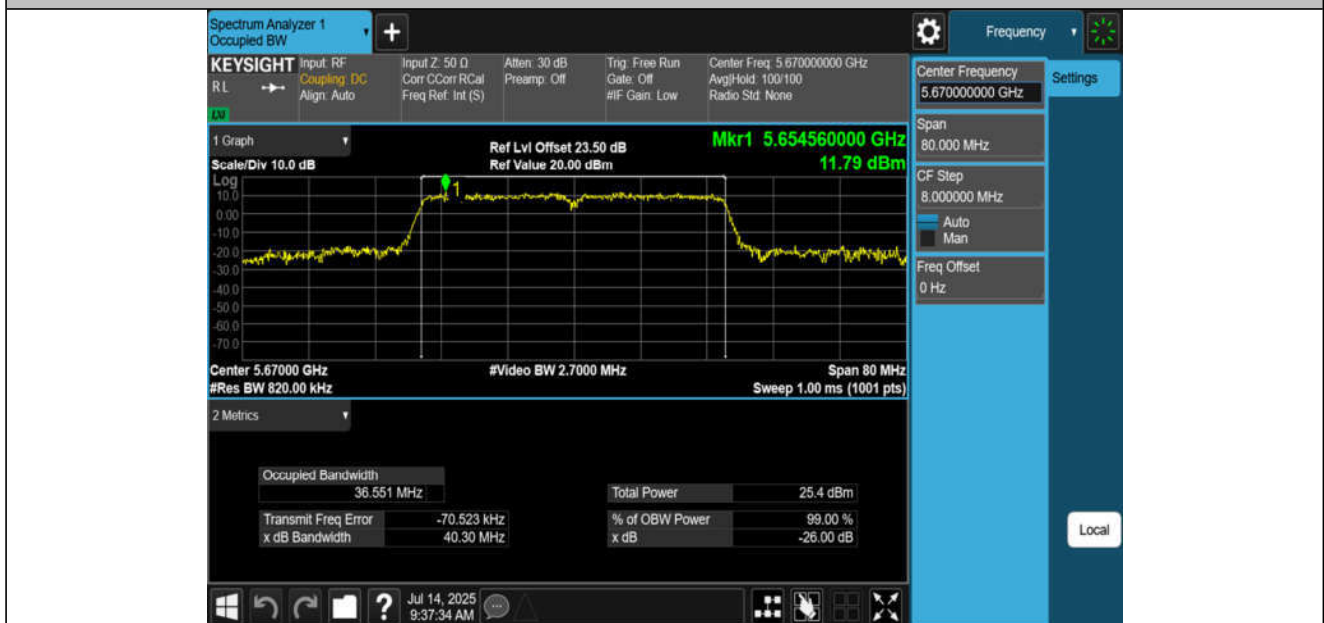
11N40MIMO-Ant2-5670
