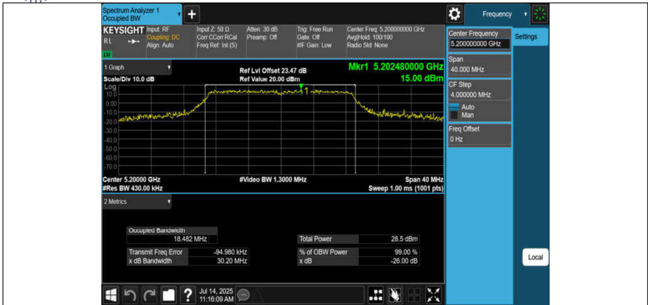
11AC20MIMO-Ant3-5200
