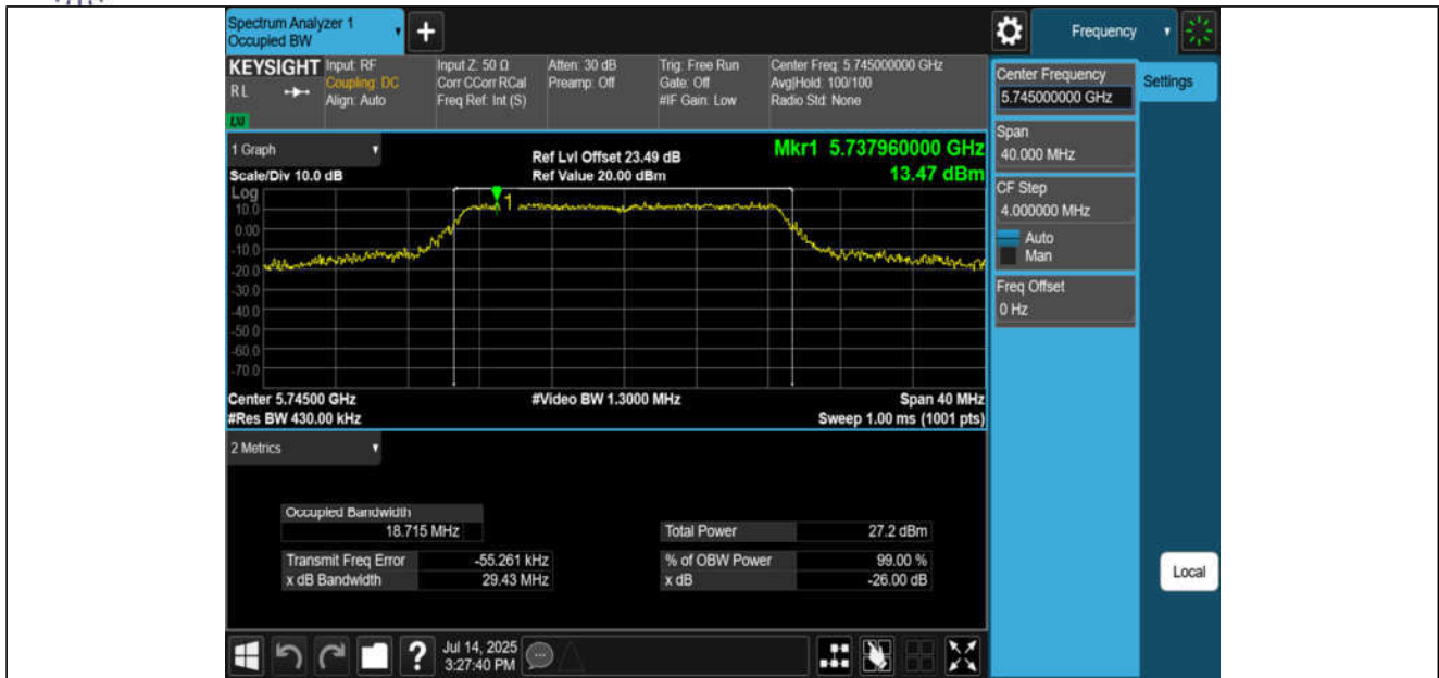
11AC20MIMO-Ant1-5745
