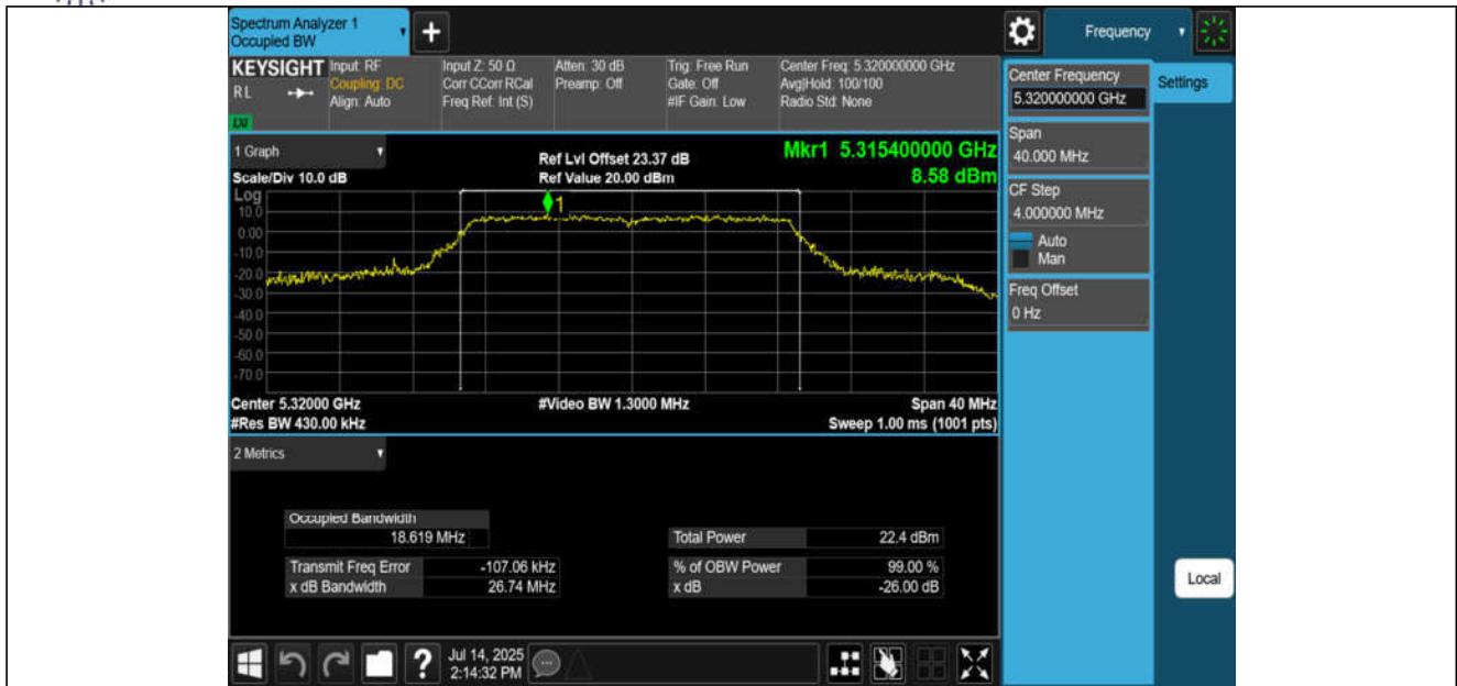
11AC20MIMO-Ant1-5320
