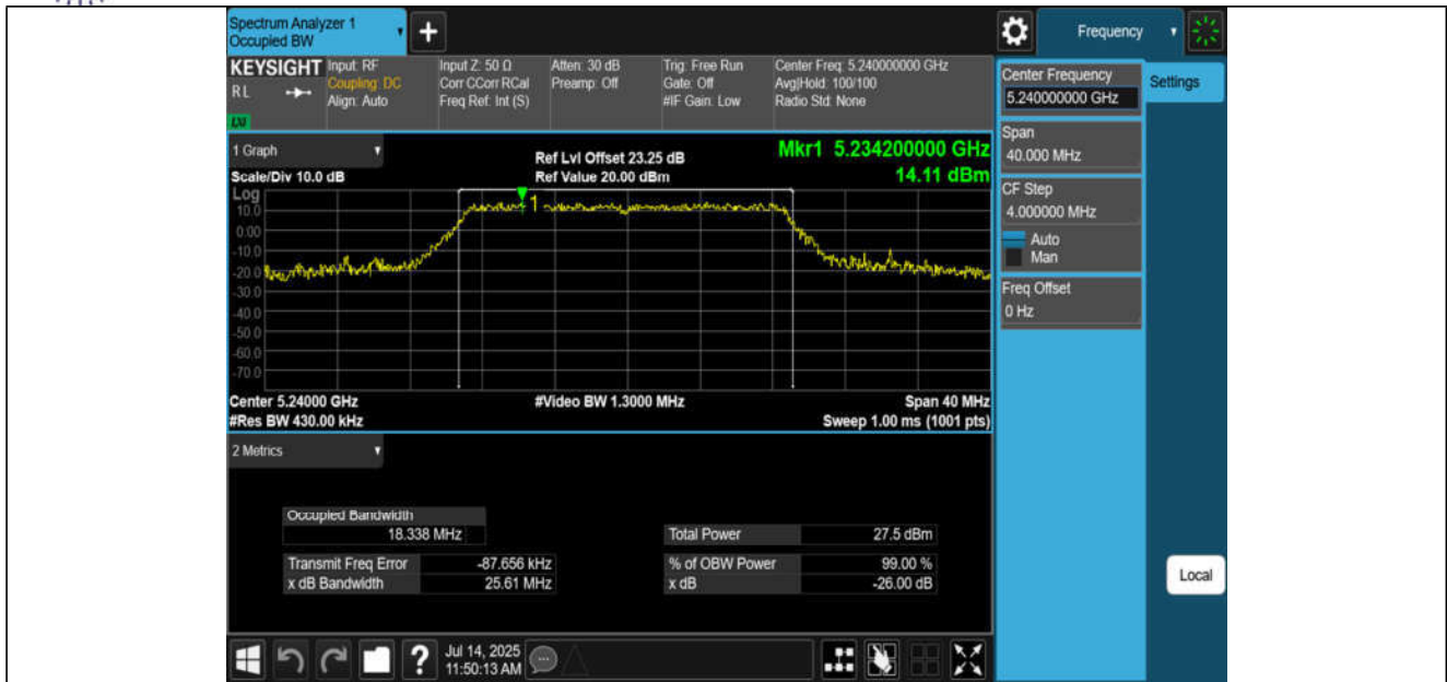
11AC20MIMO-Ant3-5240
