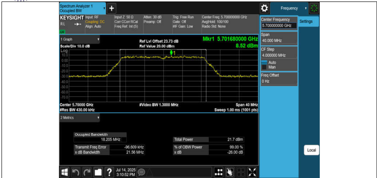
11AC20MIMO-Ant3-5700
