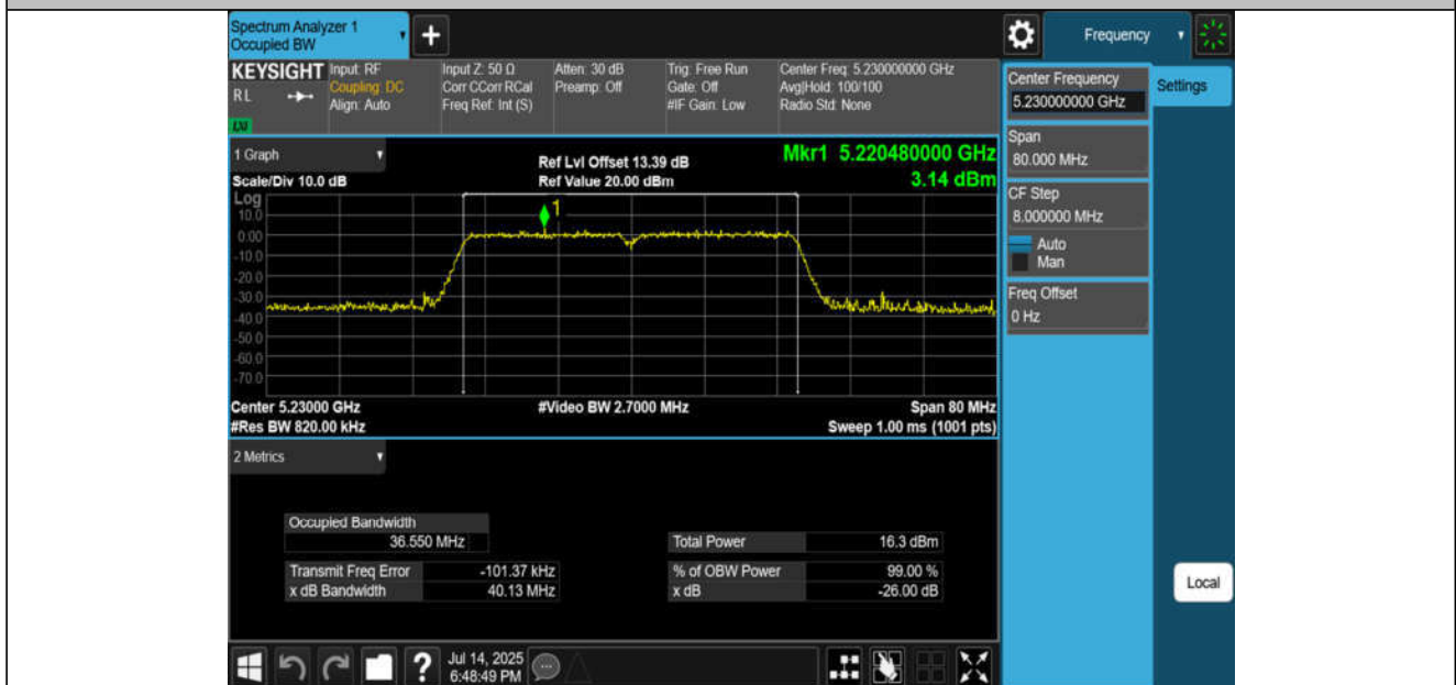
11AC40MIMO-Ant4-5230
