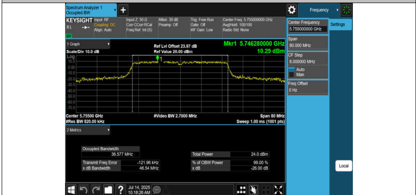
11N40MIMO-Ant2-5755
