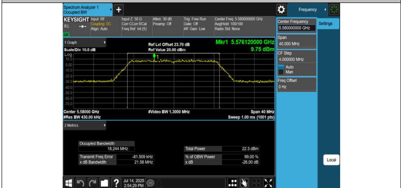
11AC20MIMO-Ant4-5580
