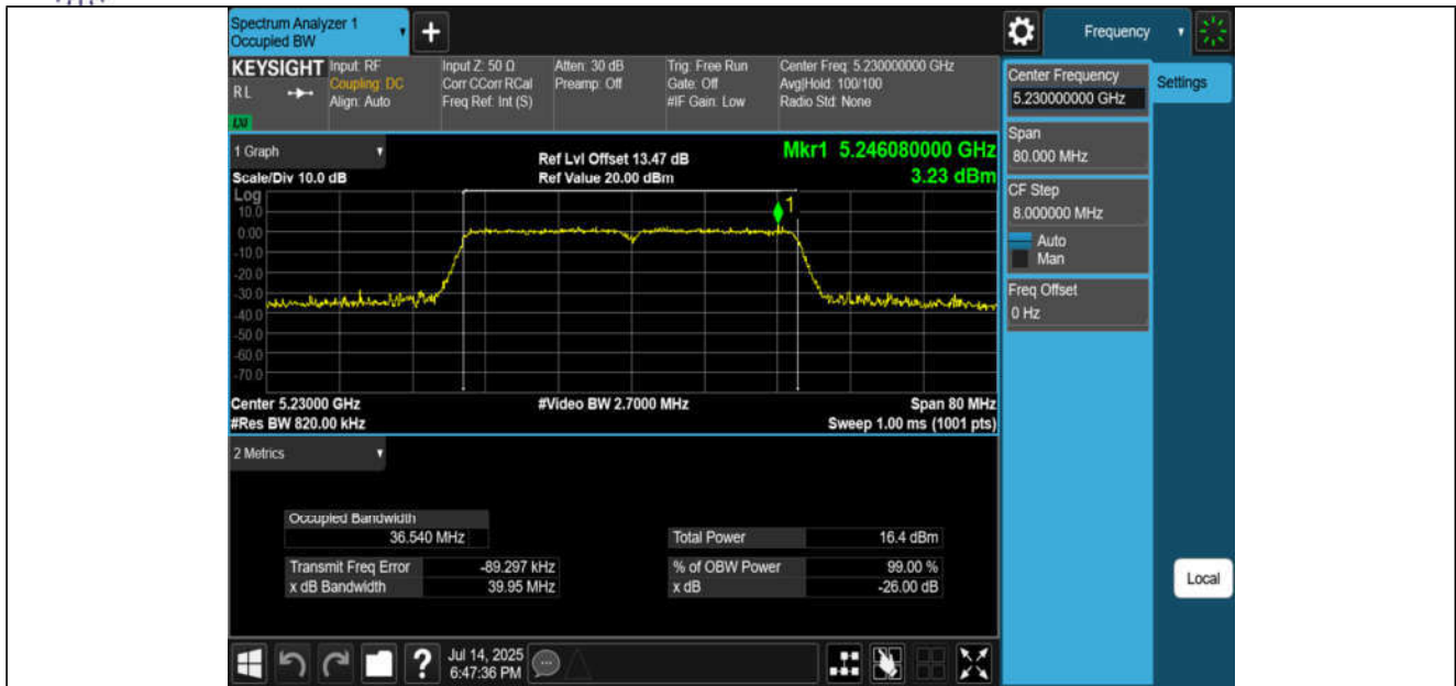
11AC40MIMO-Ant3-5230
