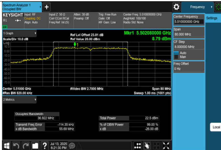
11N40MIMO-Ant3-5510
