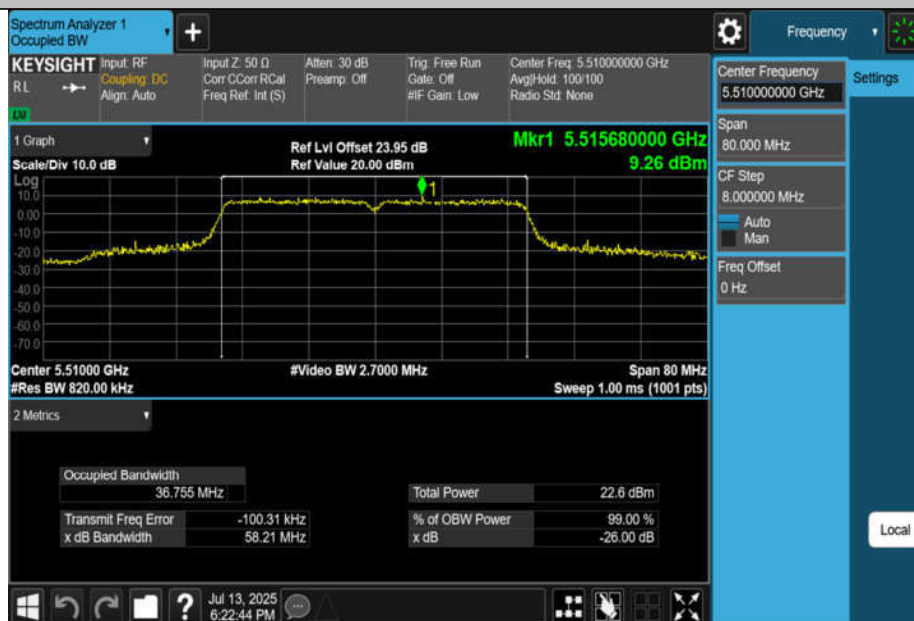
11N40MIMO-Ant4-5510
