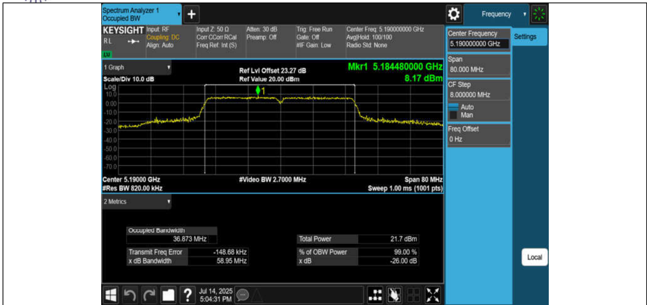
11AC40MIMO-Ant1-5190
