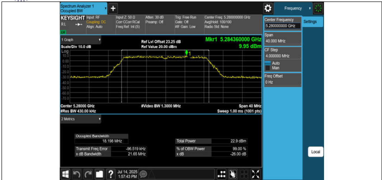
11AC20MIMO-Ant3-5280
