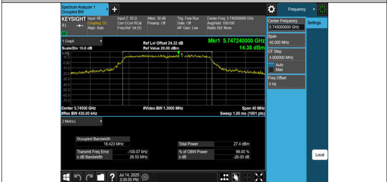
11AC20MIMO-Ant4-5745
