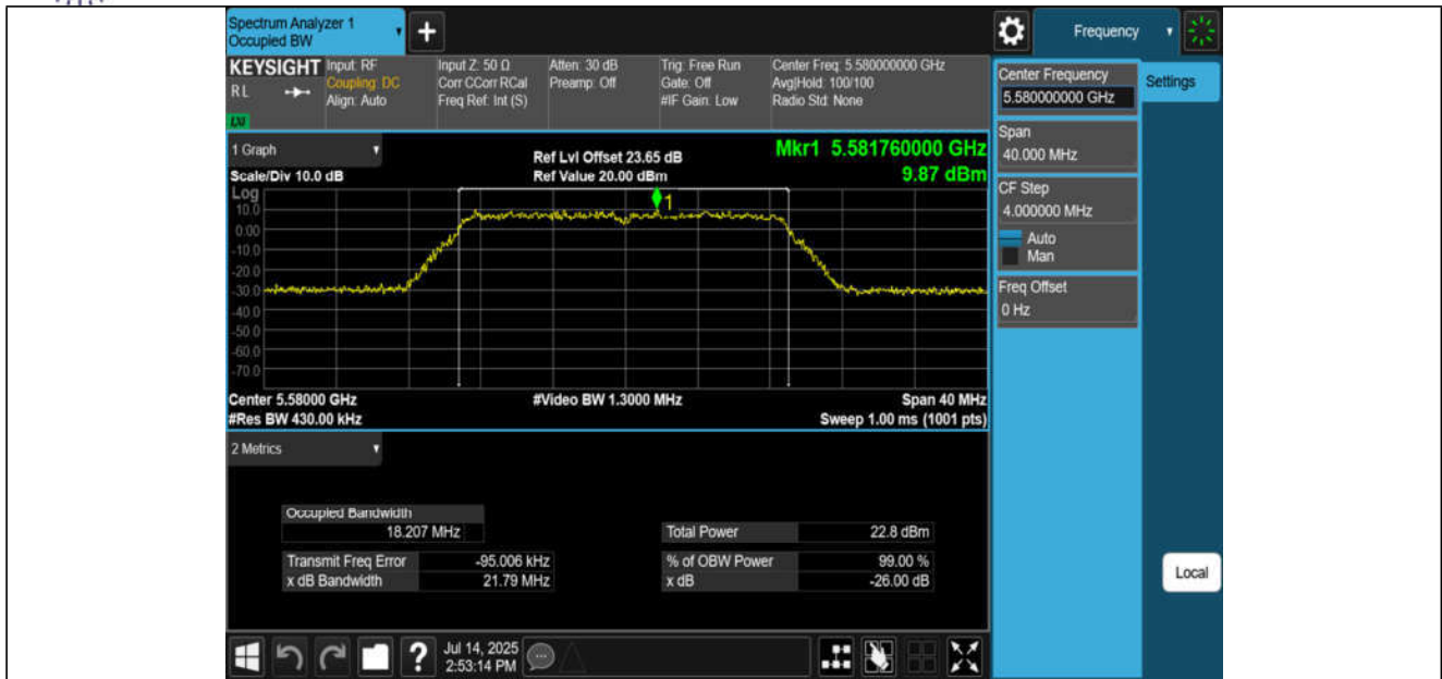
11AC20MIMO-Ant3-5580
