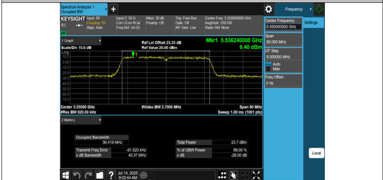
11N40MIMO-Ant2-5550
