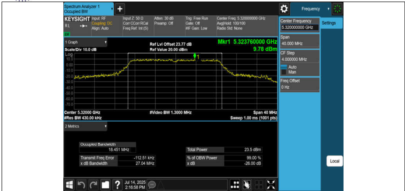
11AC20MIMO-Ant3-5320
