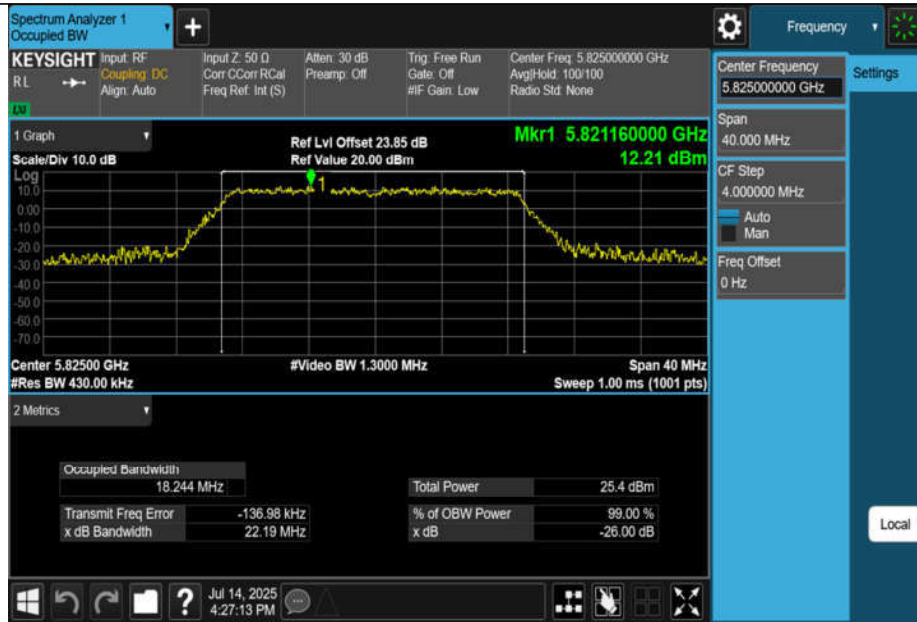
11AC20MIMO-Ant3-5825
