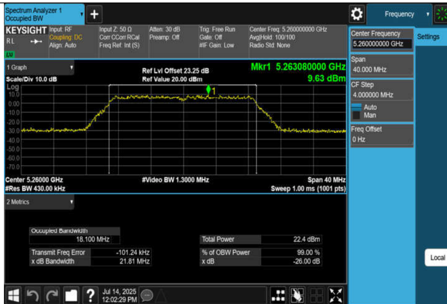
11AC20MIMO-Ant3-5260
