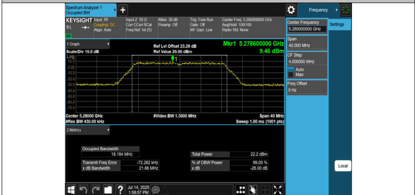
11AC20MIMO-Ant4-5280
