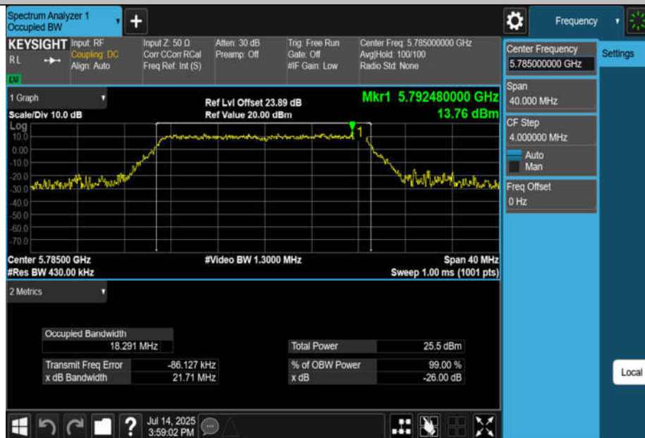
11AC20MIMO-Ant4-5785
