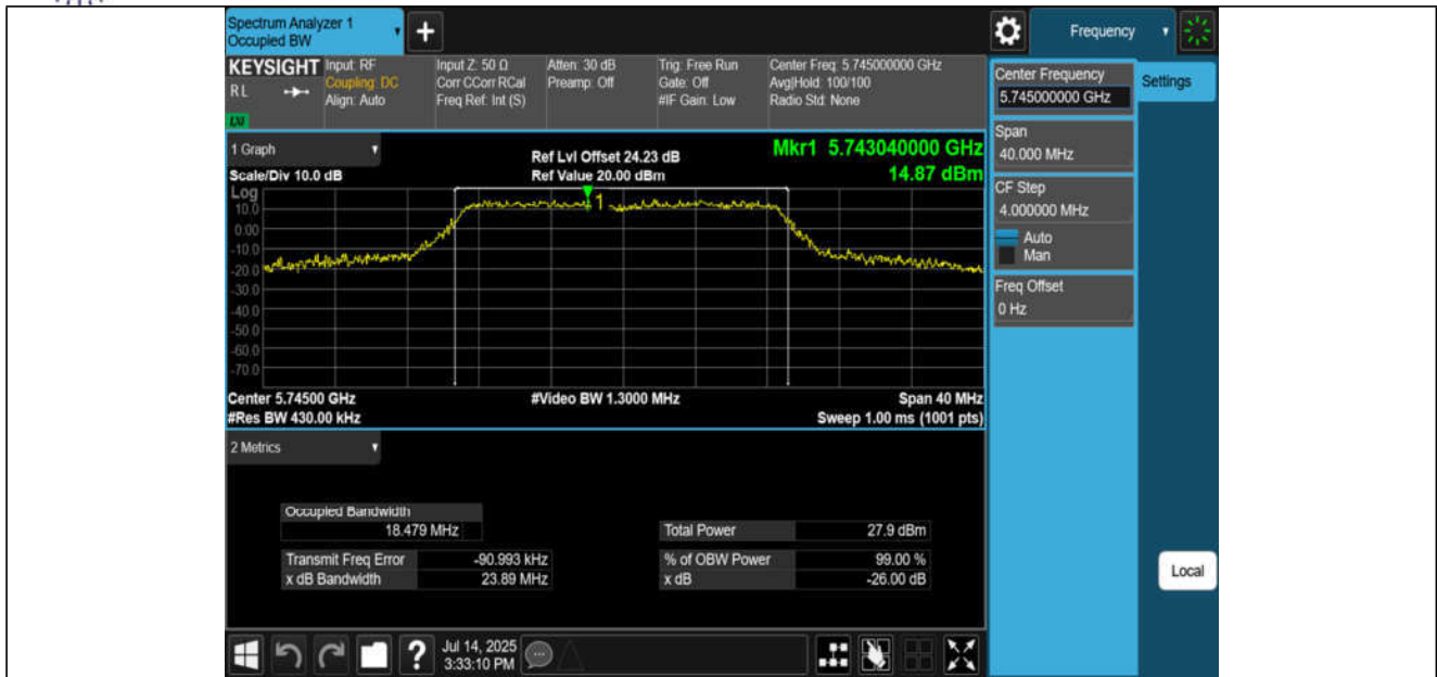
11AC20MIMO-Ant3-5745
