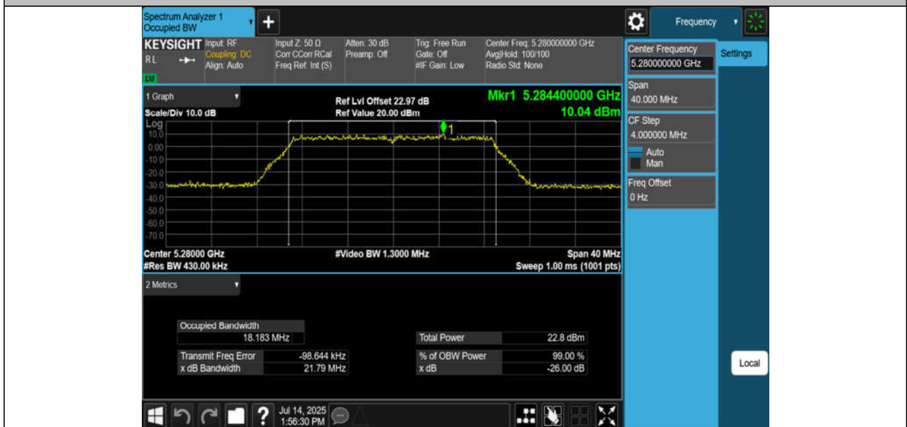
11AC20MIMO-Ant2-5280
