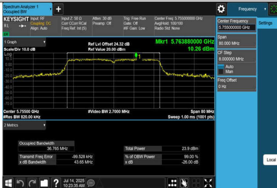
11N40MIMO-Ant4-5755
