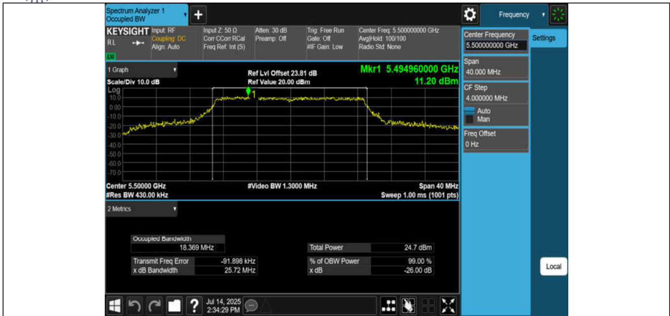
11AC20MIMO-Ant3-5500
