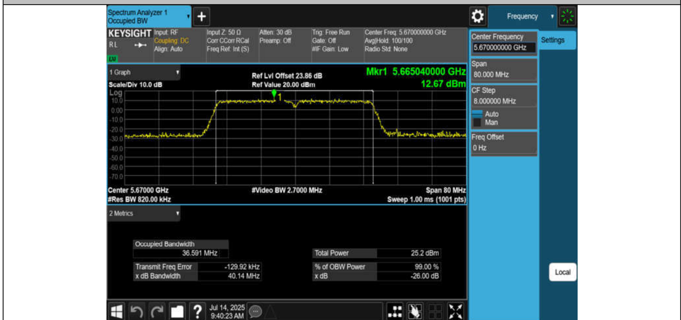
11N40MIMO-Ant4-5670
