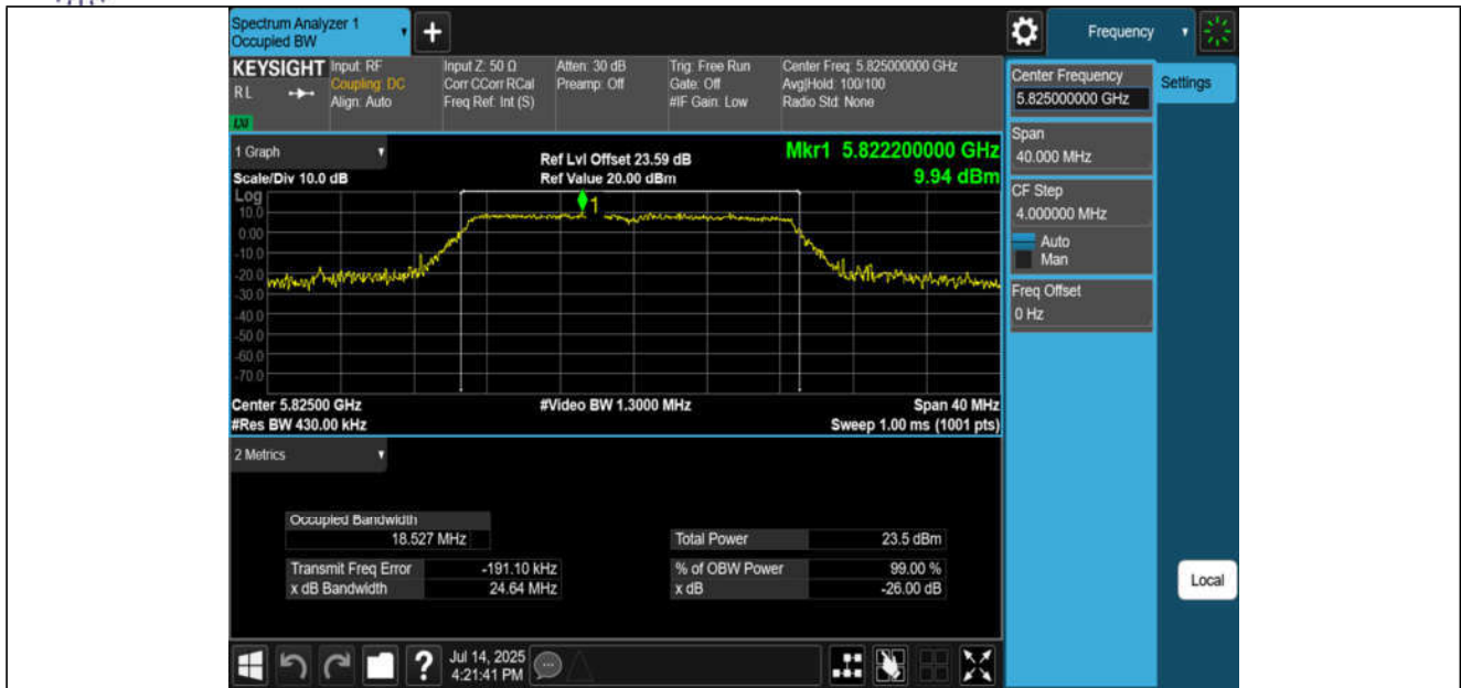
11AC20MIMO-Ant1-5825
