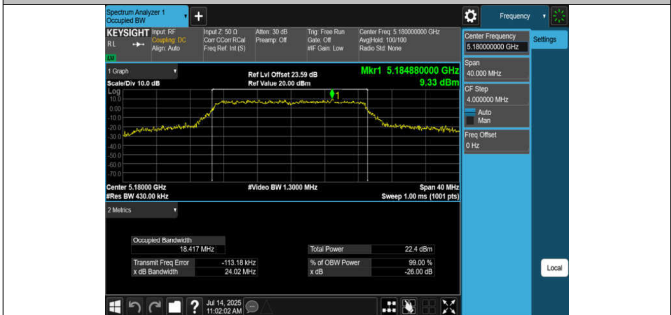
11AC20MIMO-Ant4-5180
