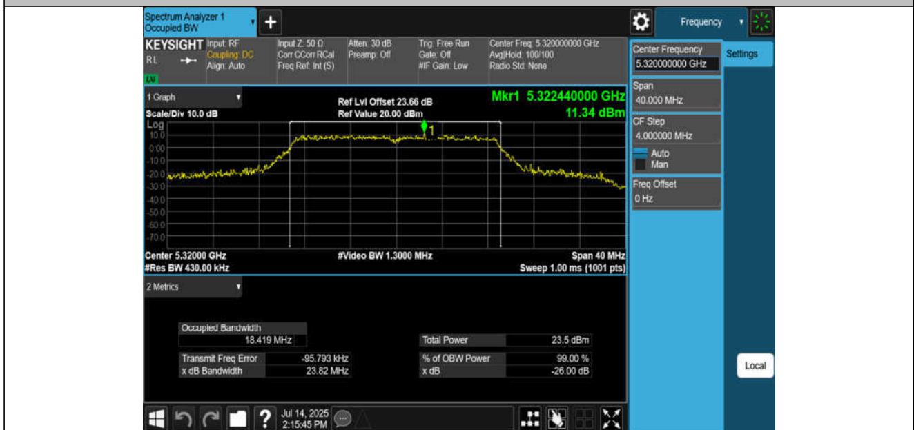
11AC20MIMO-Ant2-5320
