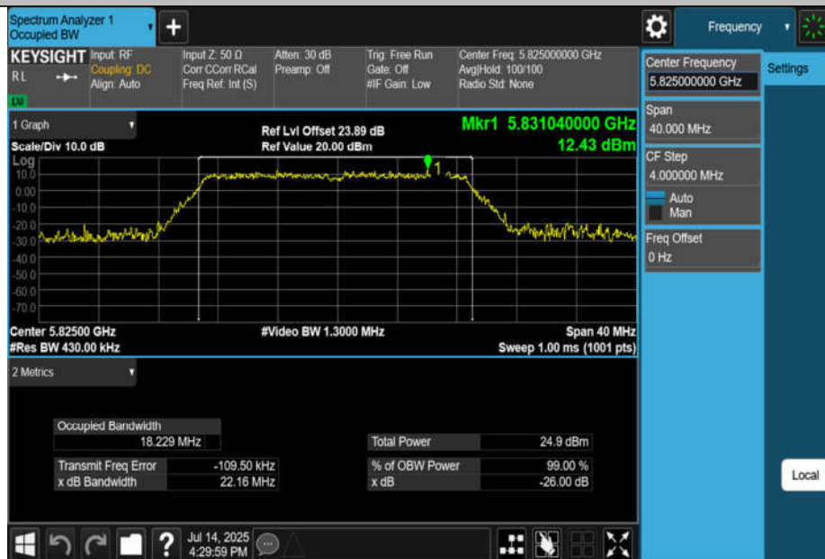
11AC20MIMO-Ant4-5825
