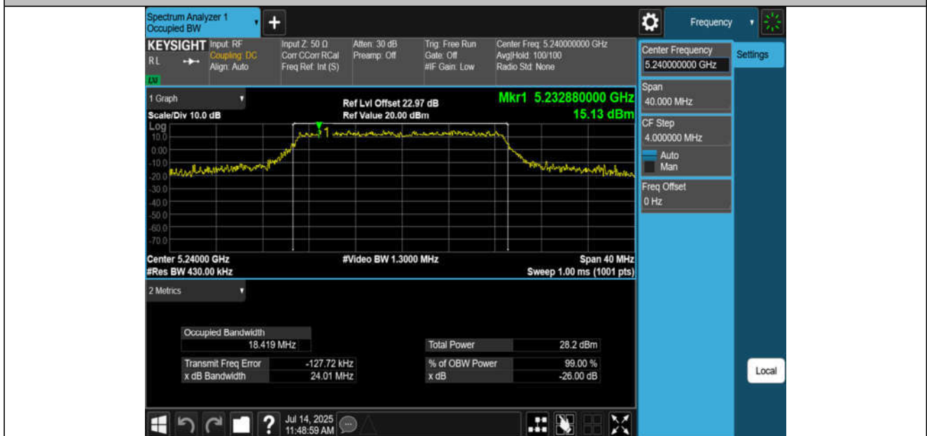
11AC20MIMO-Ant2-5240
