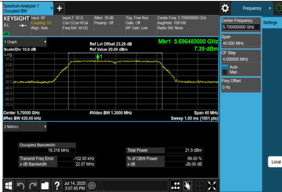
11AC20MIMO-Ant1-5700
