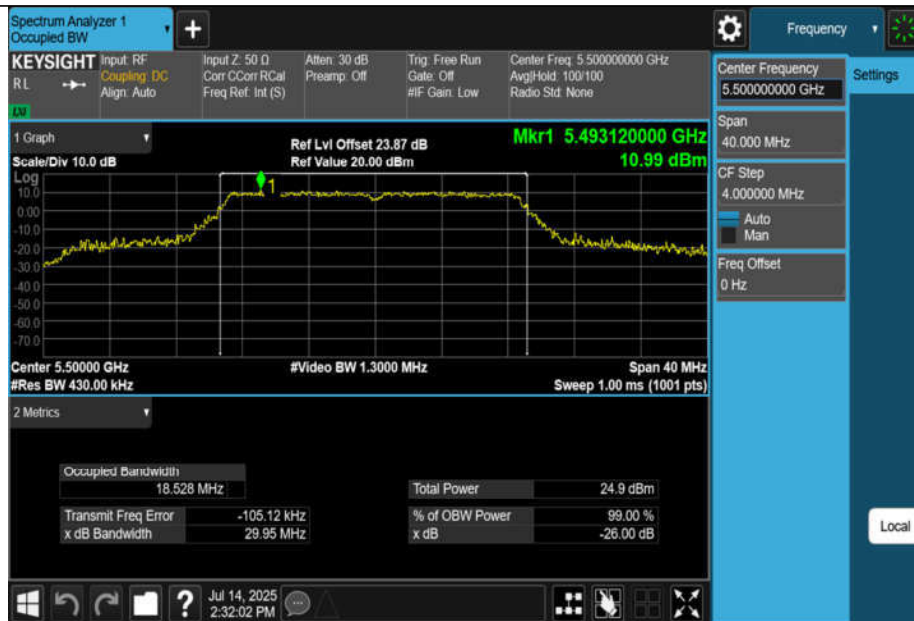
11AC20MIMO-Ant1-5500
