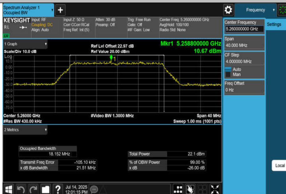
11AC20MIMO-Ant2-5260
