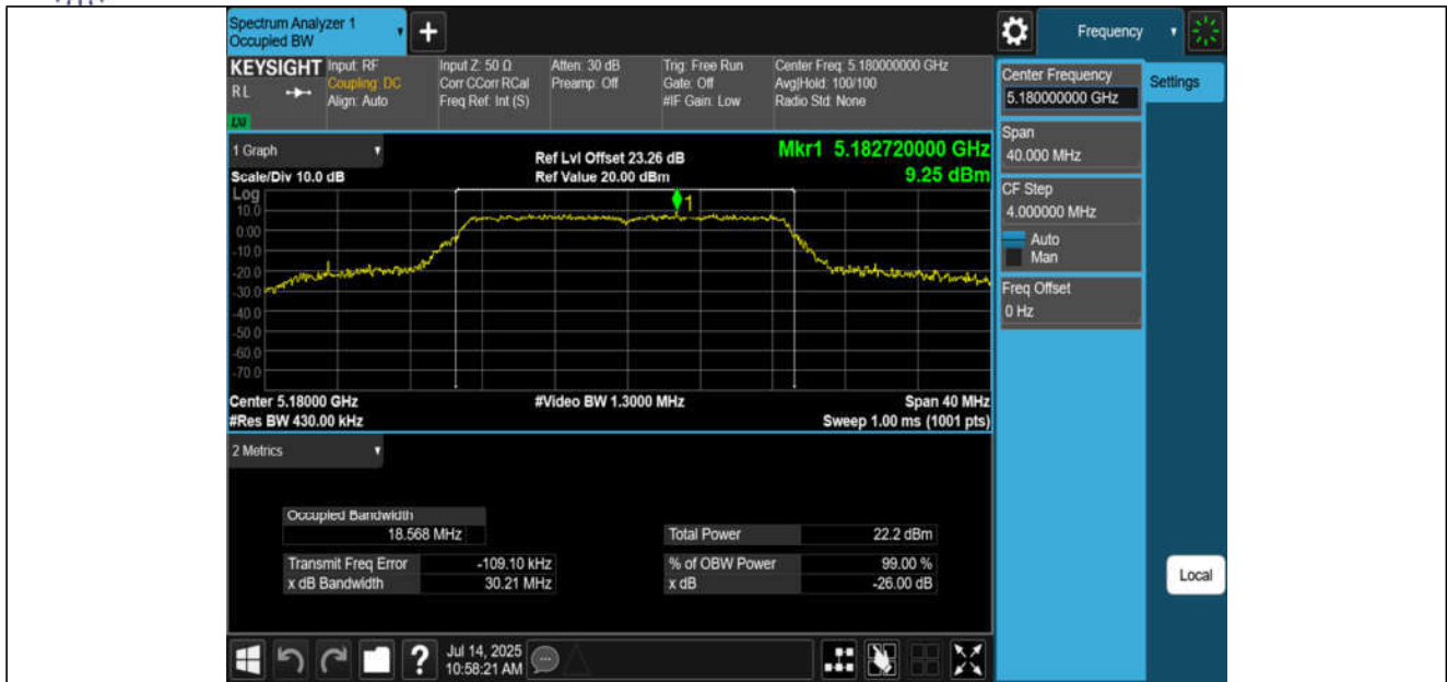
11AC20MIMO-Ant1-5180
