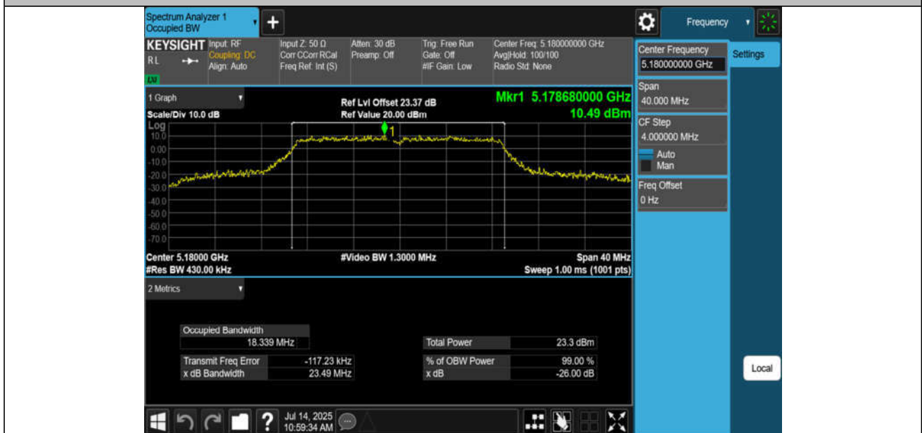
11AC20MIMO-Ant2-5180
