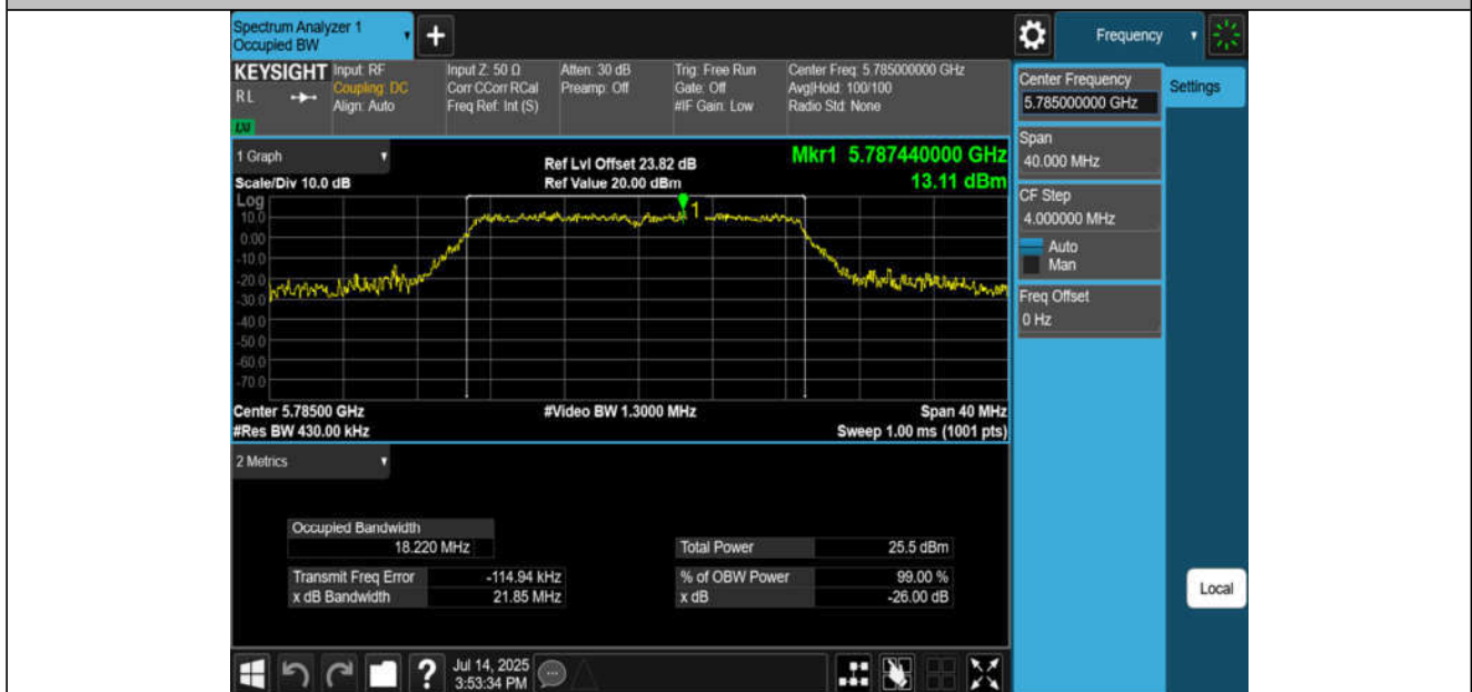
11AC20MIMO-Ant2-5785
