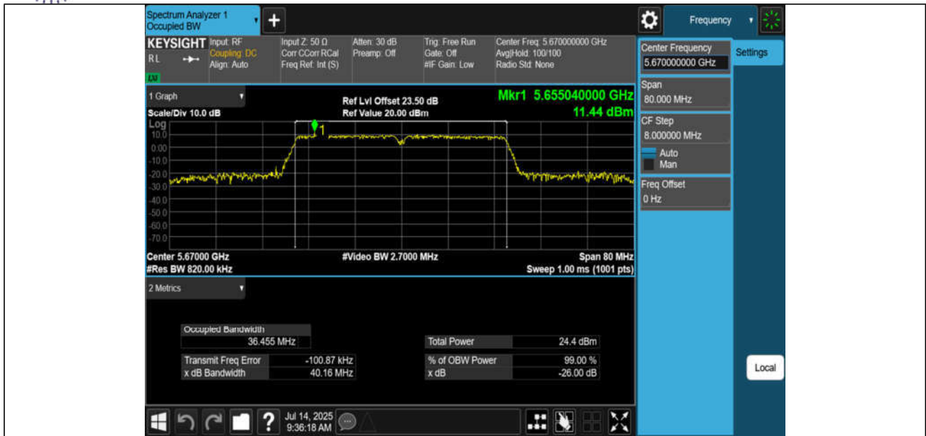
11N40MIMO-Ant1-5670
