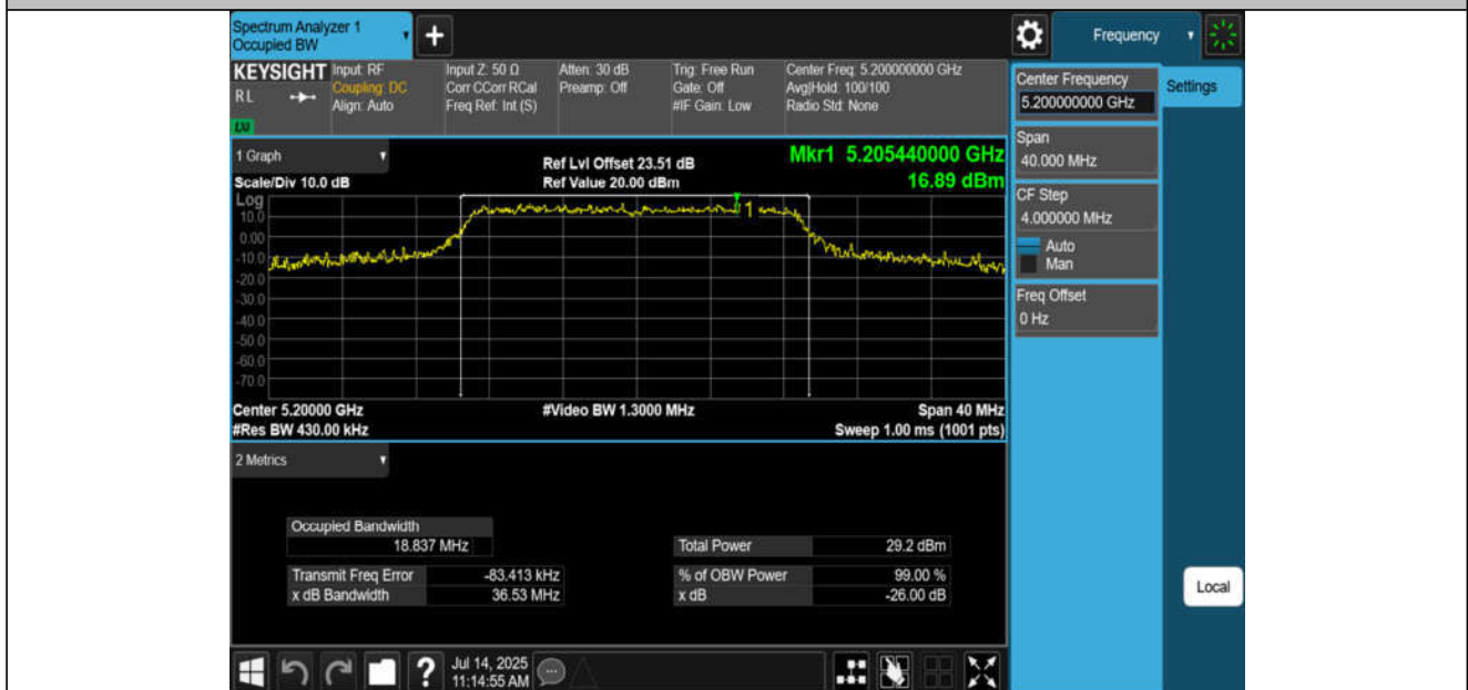
11AC20MIMO-Ant2-5200
