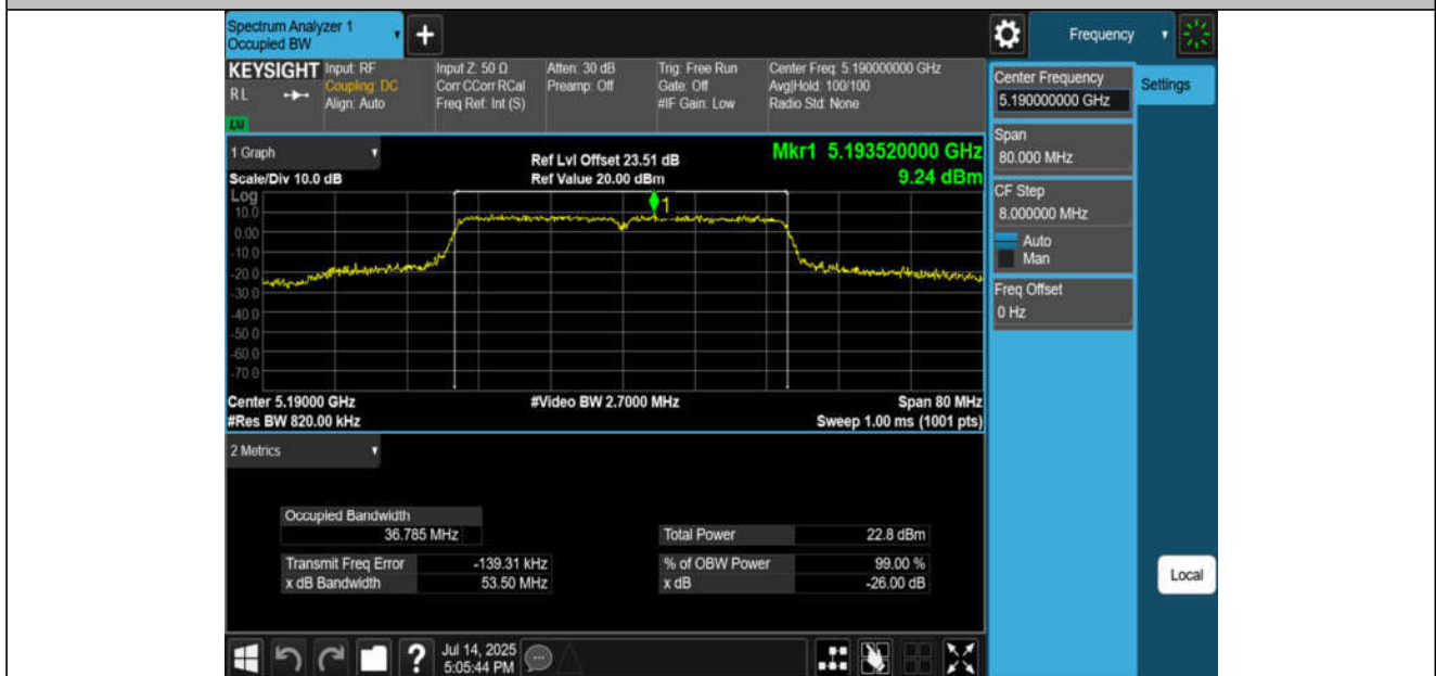
11AC40MIMO-Ant2-5190
