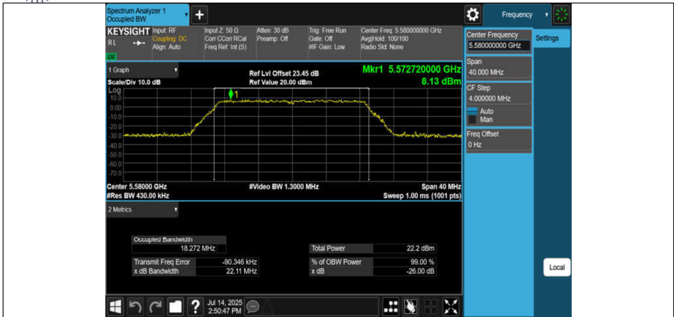
11AC20MIMO-Ant1-5580
