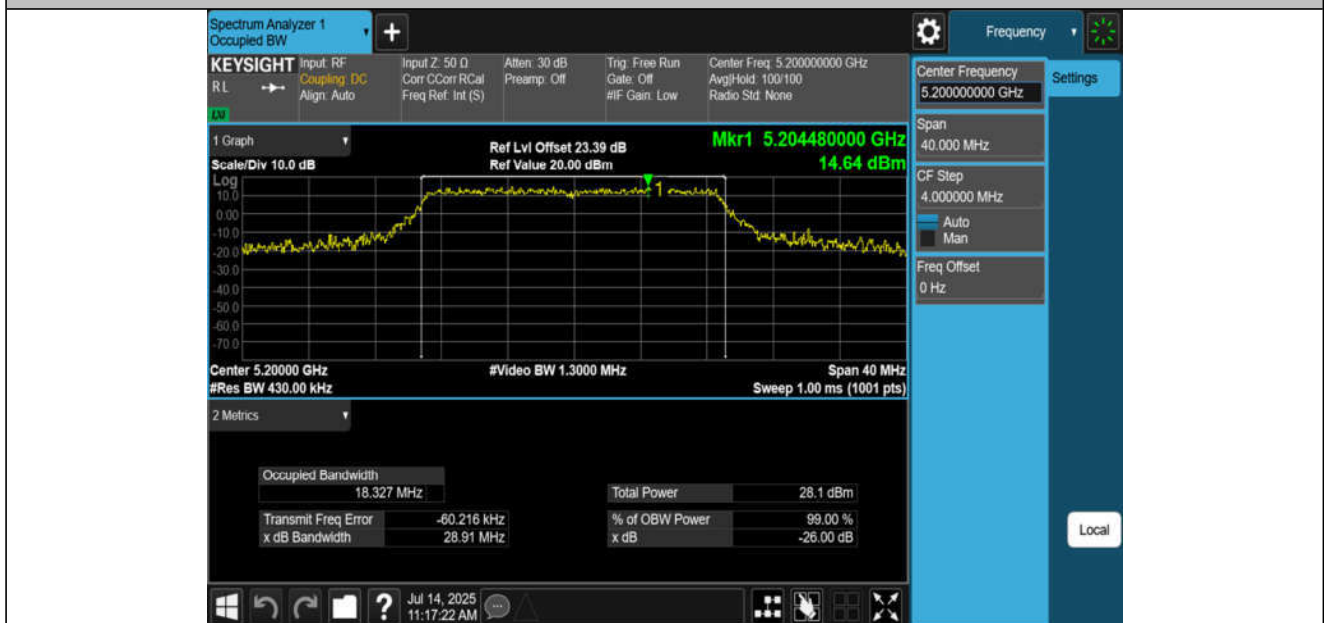
11AC20MIMO-Ant4-5200
