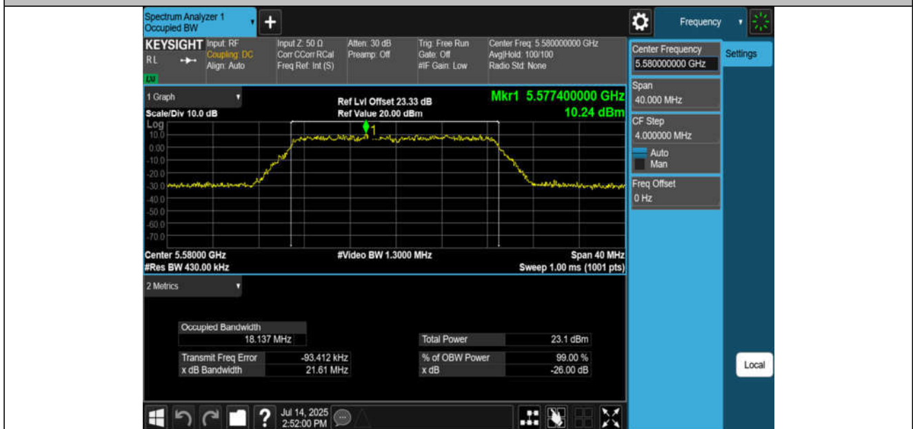
11AC20MIMO-Ant2-5580
