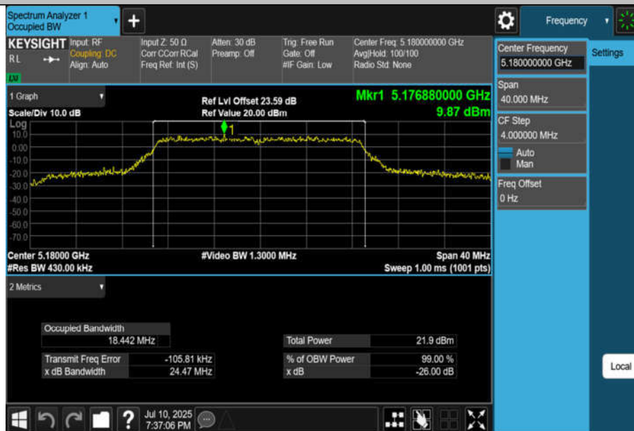
11N20MIMO-Ant4-5180
