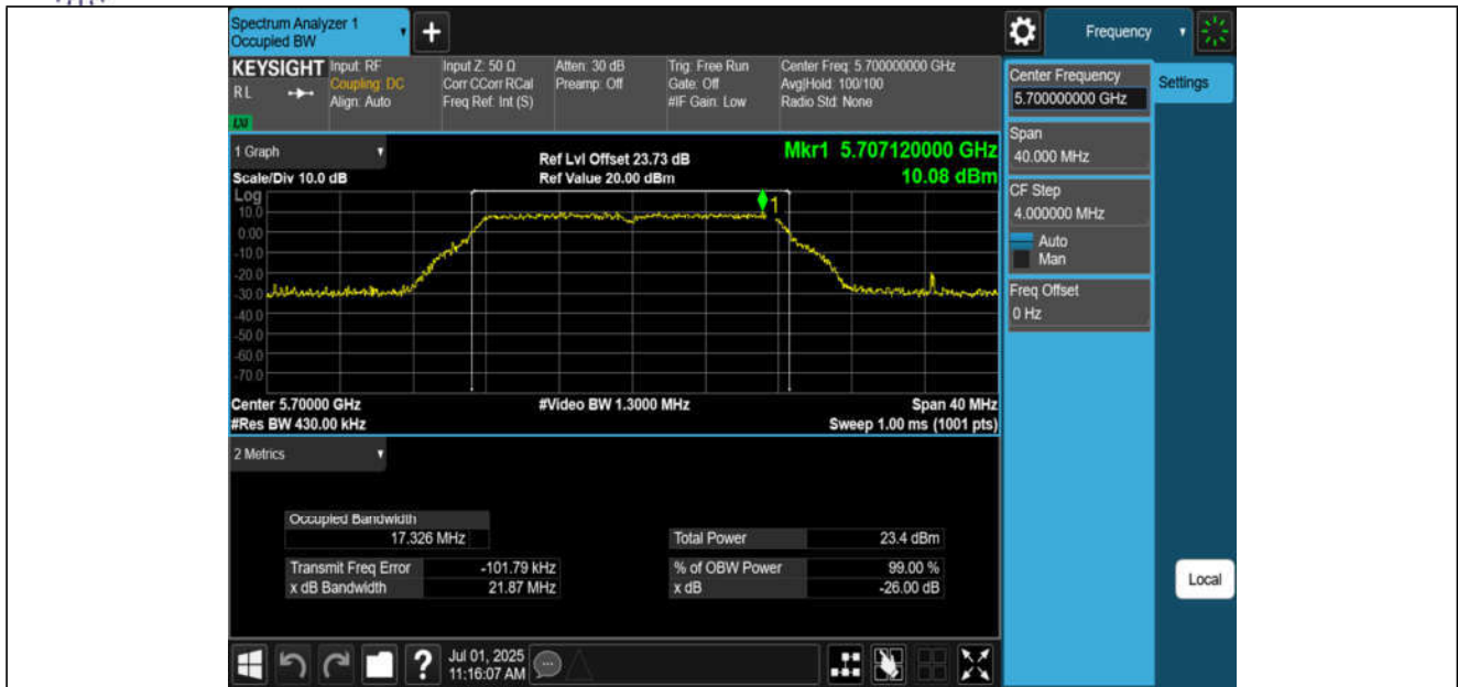
11A-CDD-Ant3-5700
