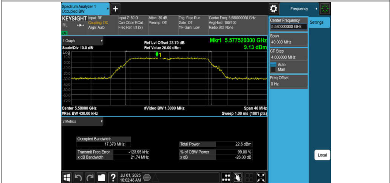
11A-CDD-Ant4-5580
