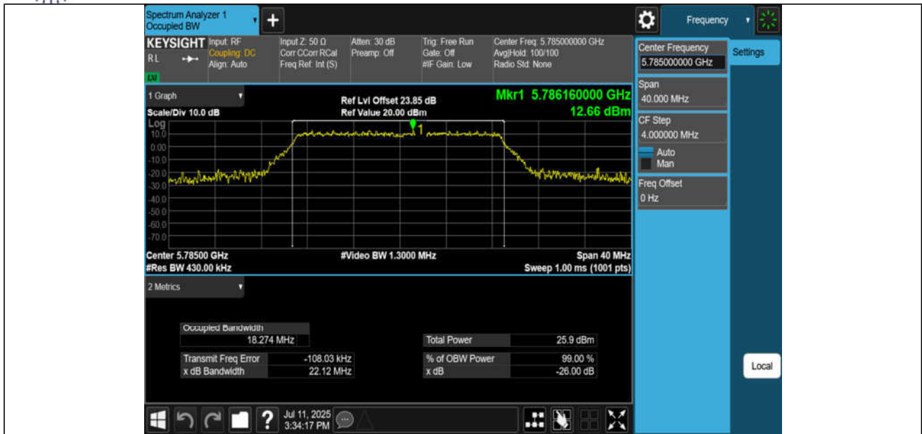
11N20MIMO-Ant3-5785
