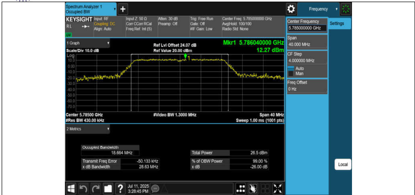
11N20MIMO-Ant1-5785
