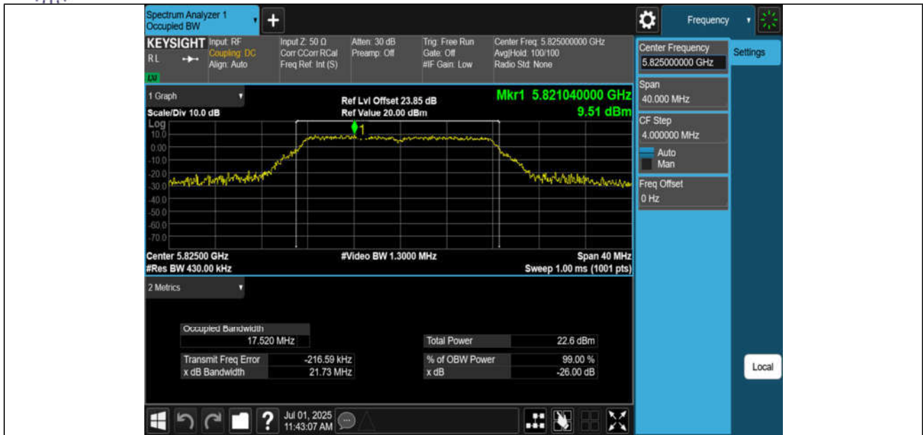
11A-CDD-Ant3-5825
