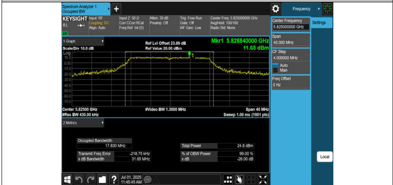
11A-CDD-Ant4-5825
