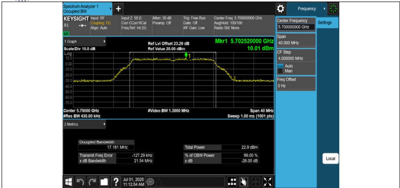
11A-CDD-Ant1-5700
