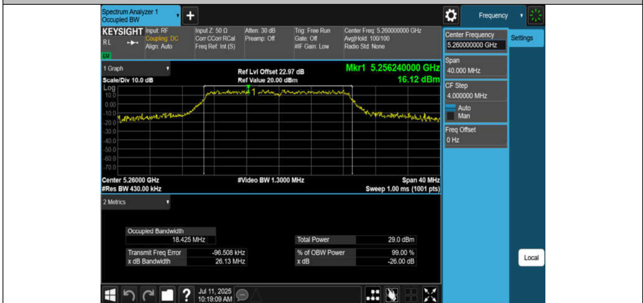
11N20MIMO-Ant2-5260
