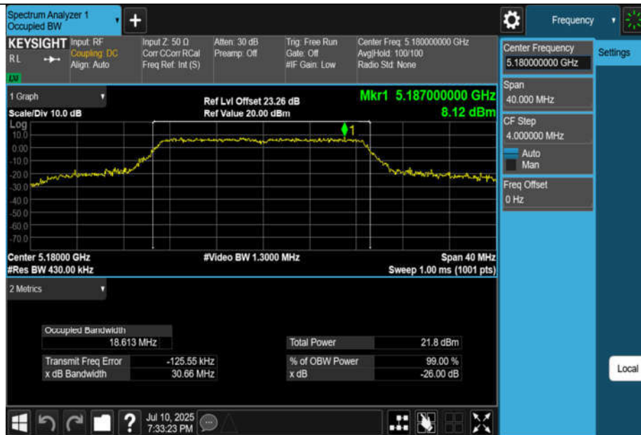
11N20MIMO-Ant1-5180
