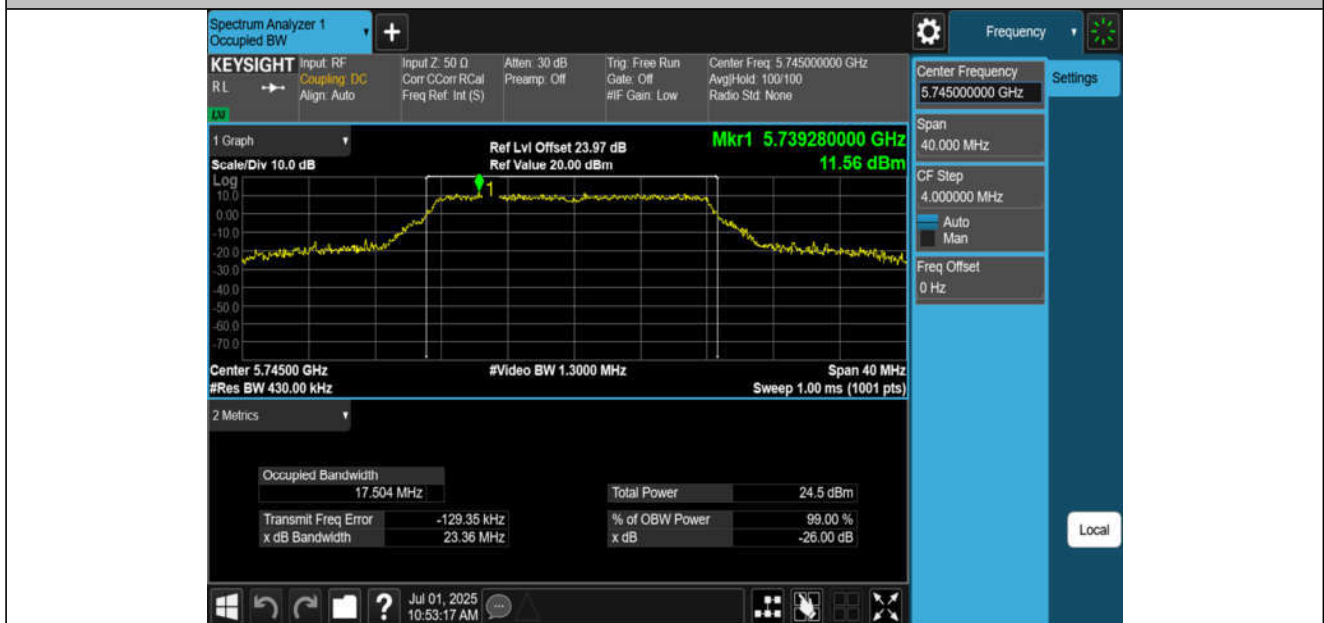
11A-CDD-Ant2-5745
