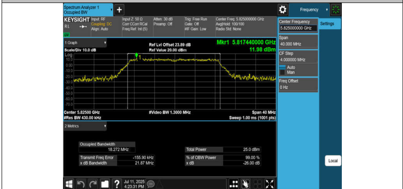
11N20MIMO-Ant4-5825
