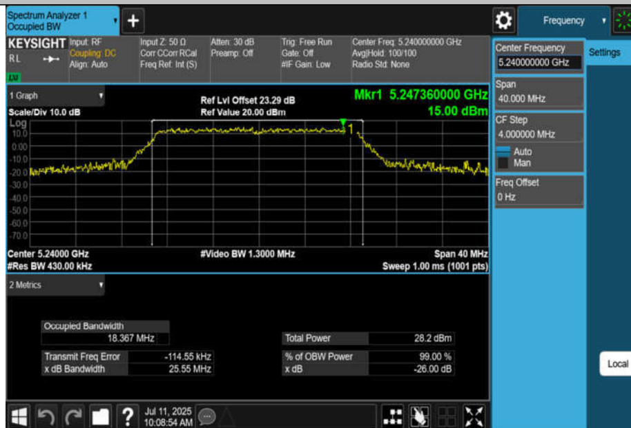
11N20MIMO-Ant4-5240
