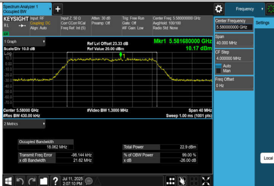
11N20MIMO-Ant2-5580
