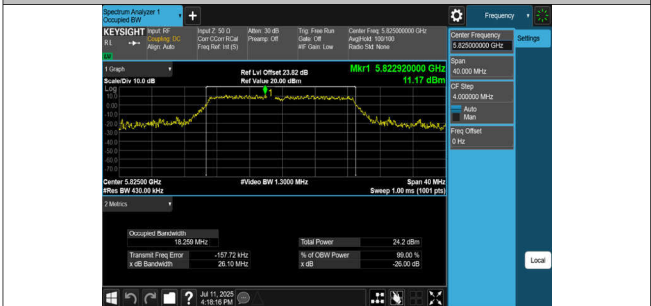
11N20MIMO-Ant2-5825
