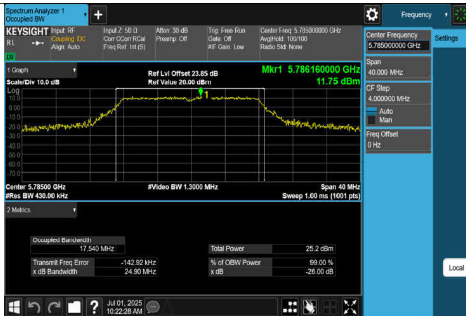
11A-CDD-Ant3-5785
