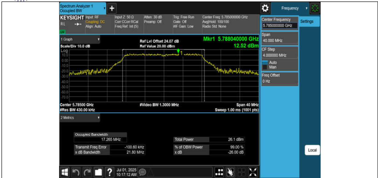
11A-CDD-Ant1-5785
