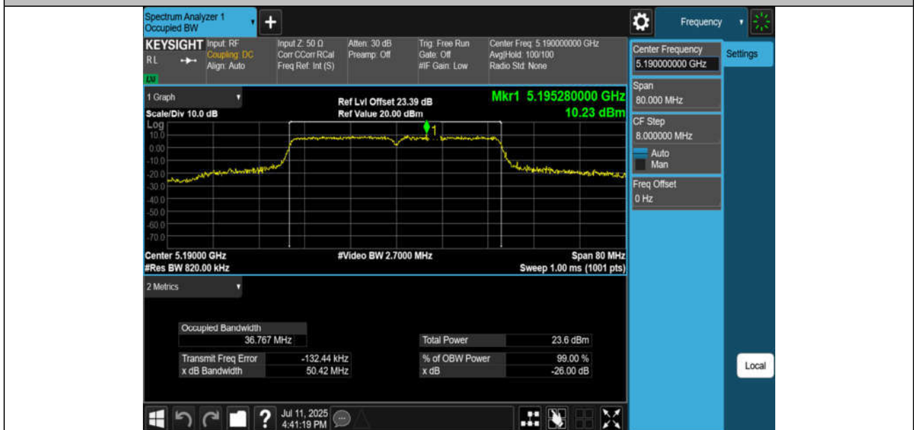
11N40MIMO-Ant4-5190
