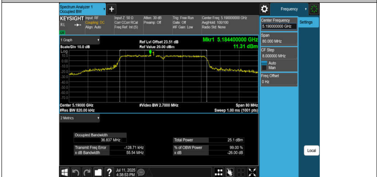
11N40MIMO-Ant2-5190
