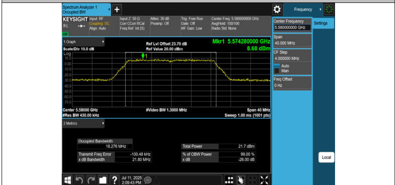
11N20MIMO-Ant4-5580
