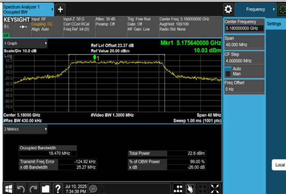
11N20MIMO-Ant2-5180
