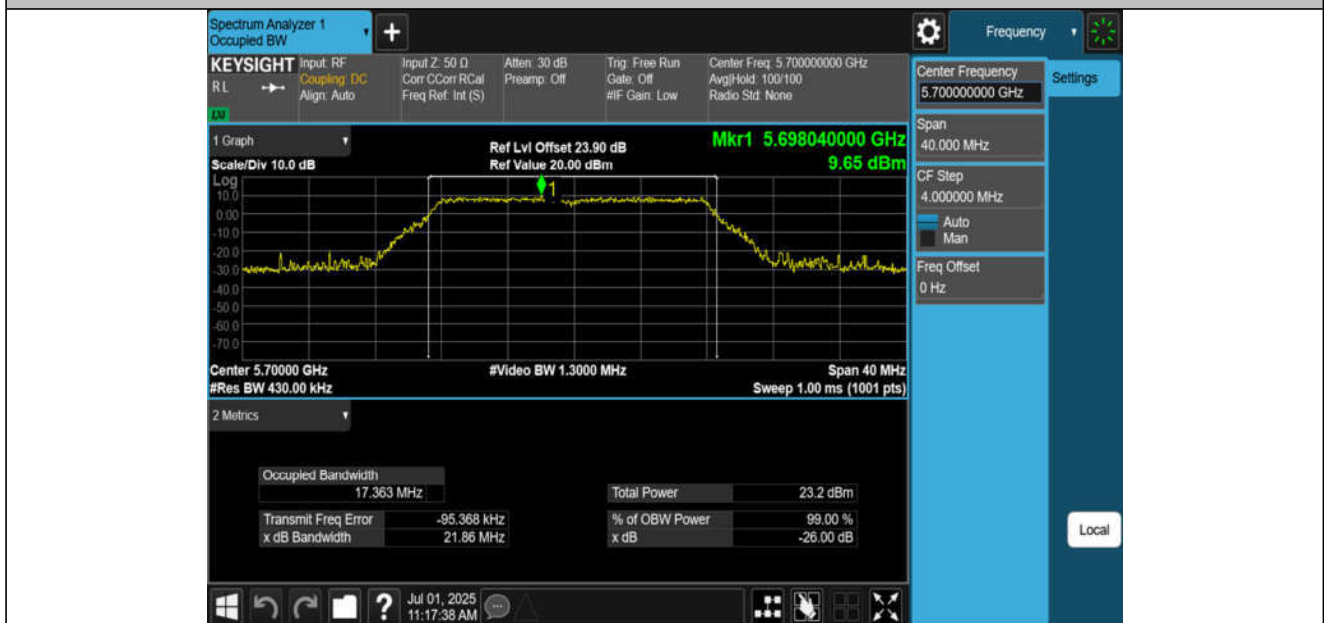
11A-CDD-Ant4-5700
