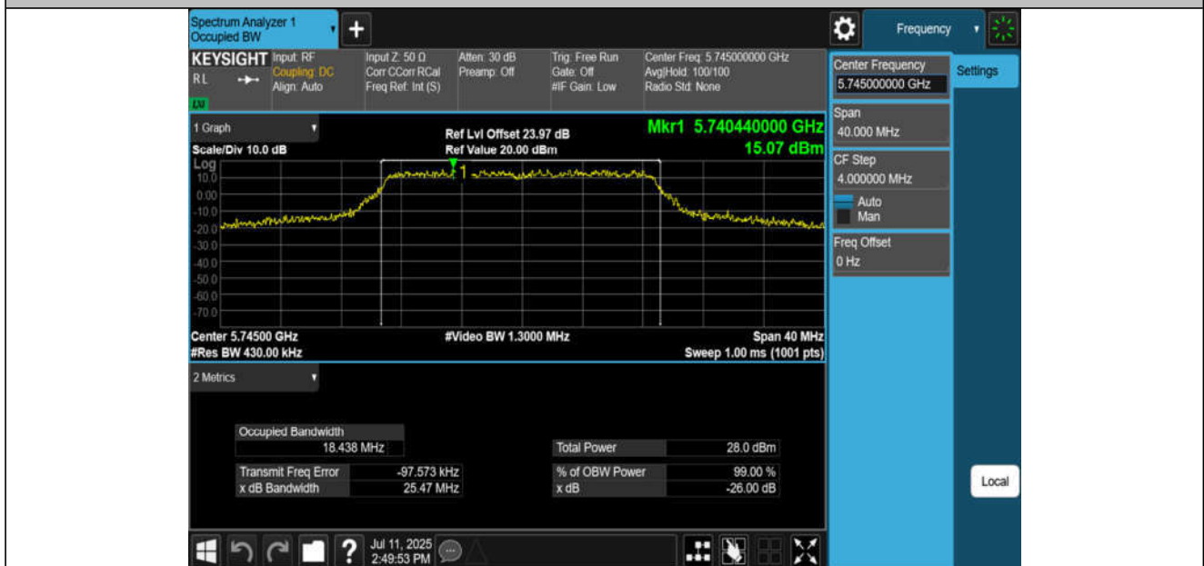
11N20MIMO-Ant2-5745
