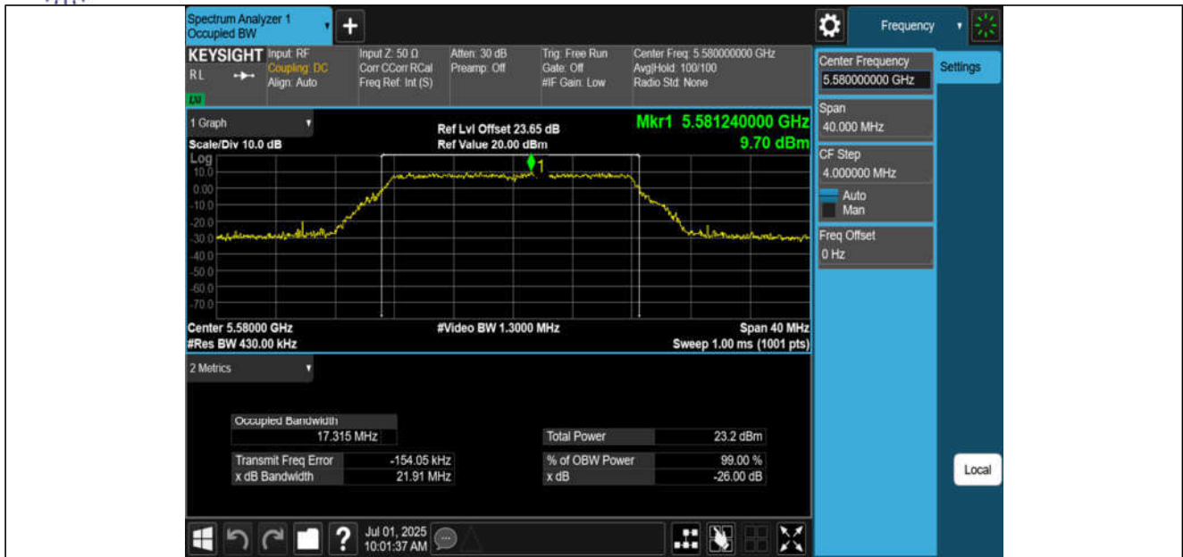
11A-CDD-Ant3-5580
