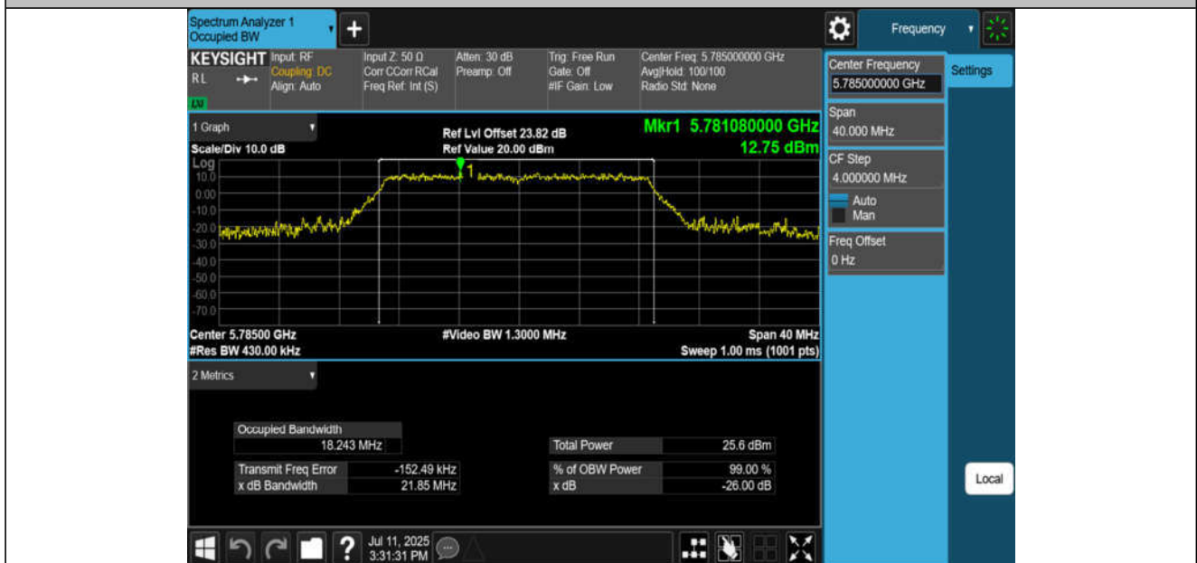
11N20MIMO-Ant2-5785
