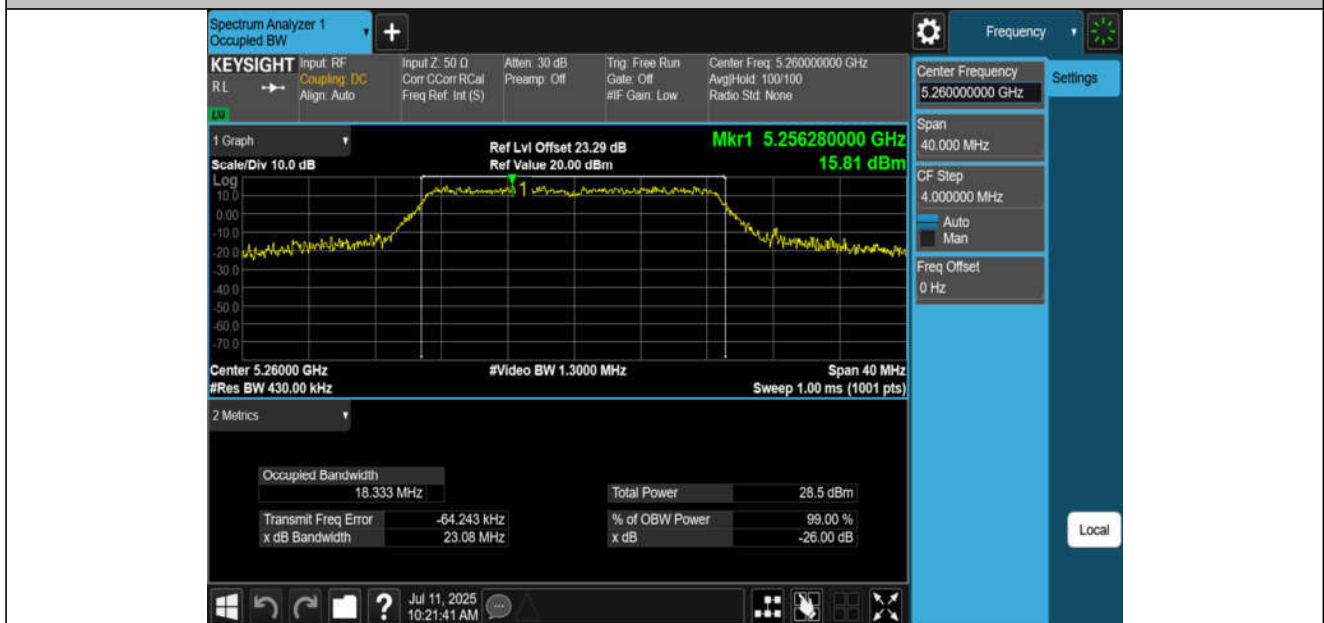
11N20MIMO-Ant4-5260
