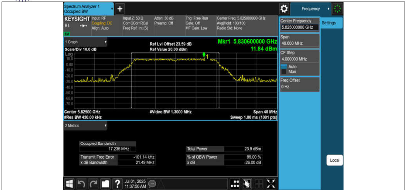
11A-CDD-Ant1-5825
