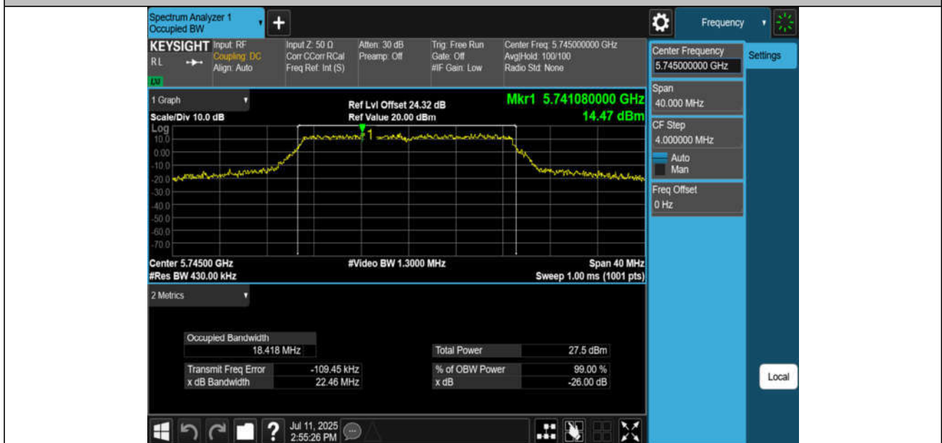
11N20MIMO-Ant4-5745
