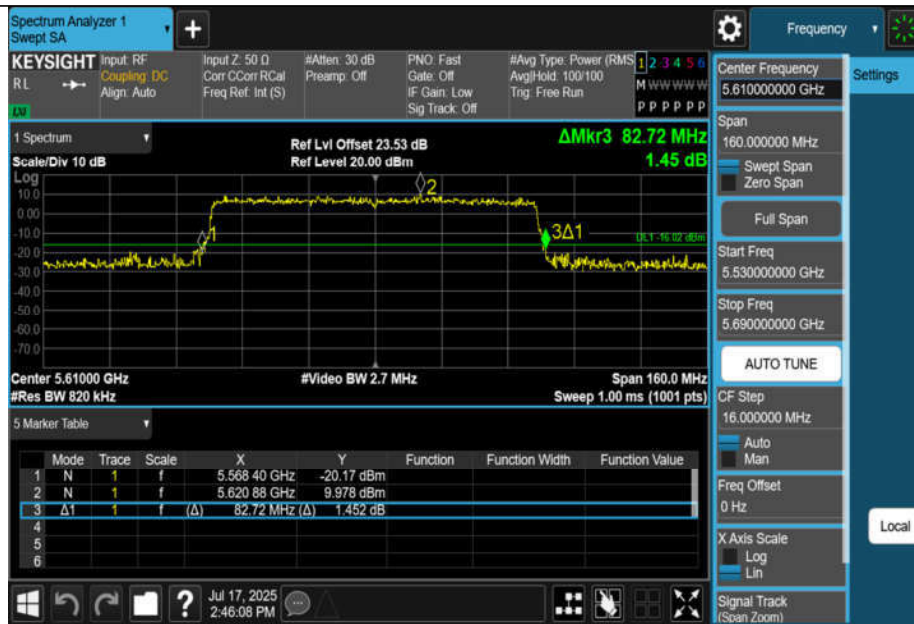
11BE80MIMO-Ant3-5610
