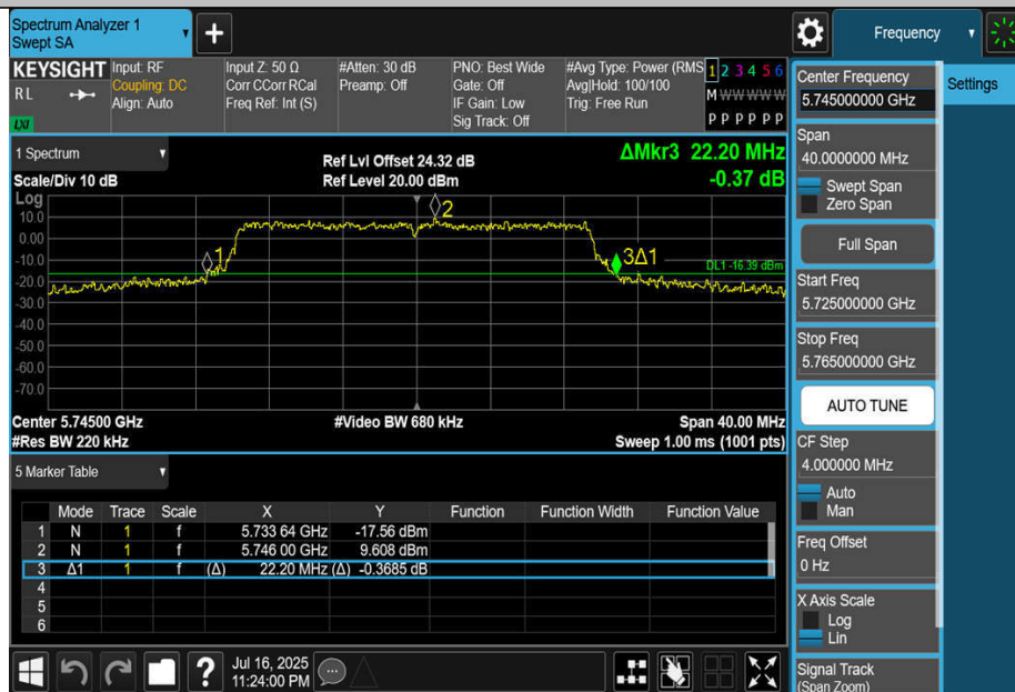
11BE20MIMO-Ant4-5745
