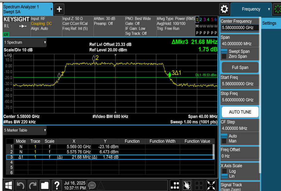
11BE20MIMO-Ant2-5580
