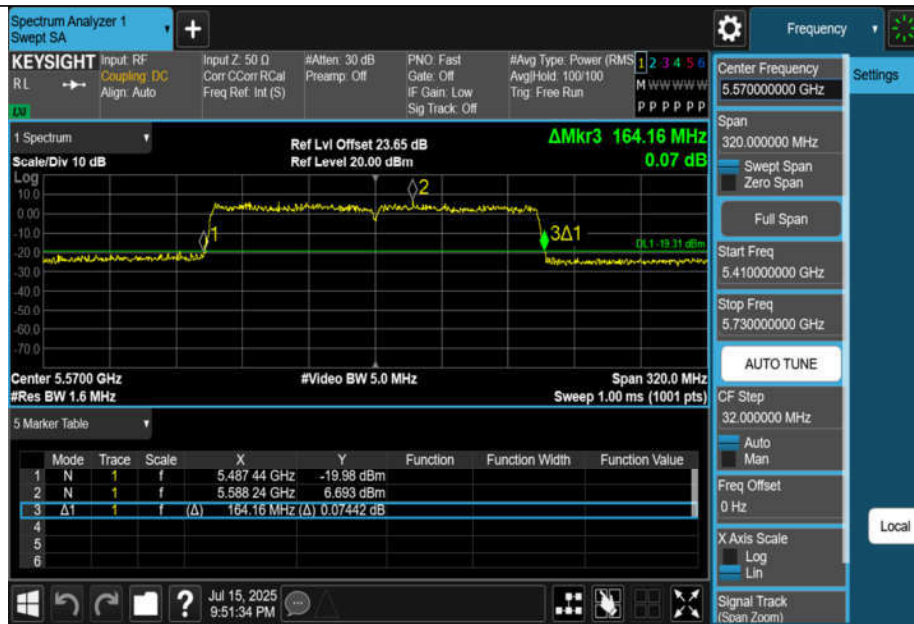
11AX160MIMO-Ant3-5570
