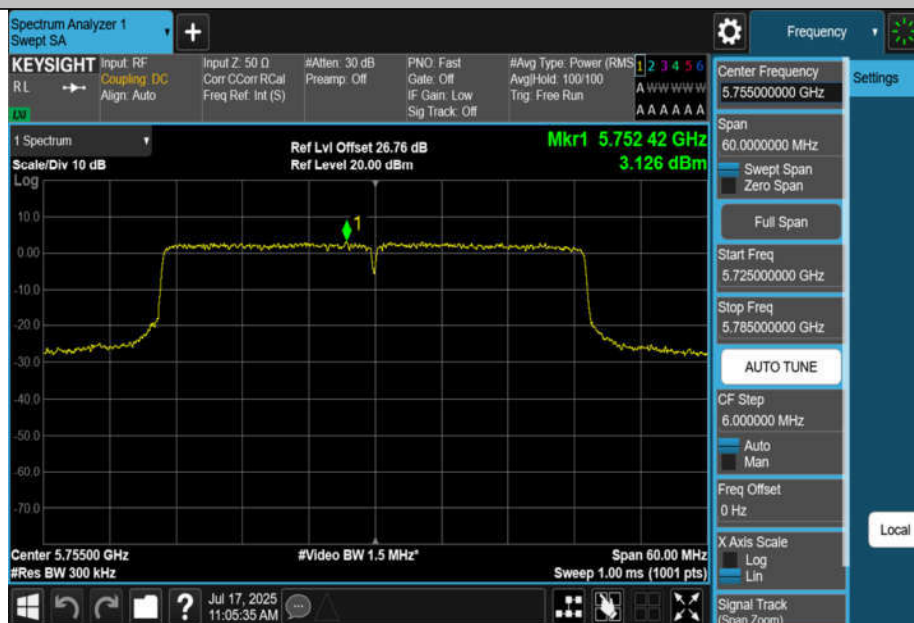
11BE40MIMO-Ant4-5755-PASS
