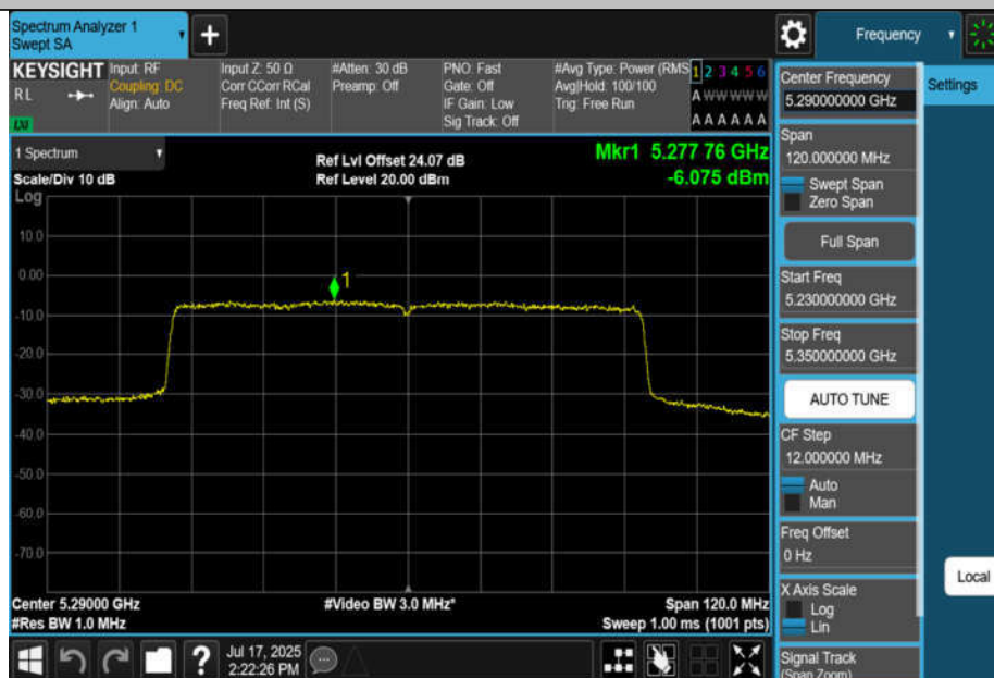
11BE80MIMO-Ant2-5290-PASS
