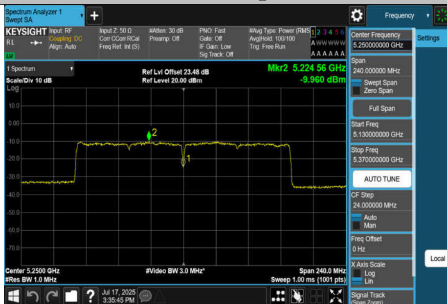
11BE160MIMO-Ant2-5250_UNII-1-PASS
