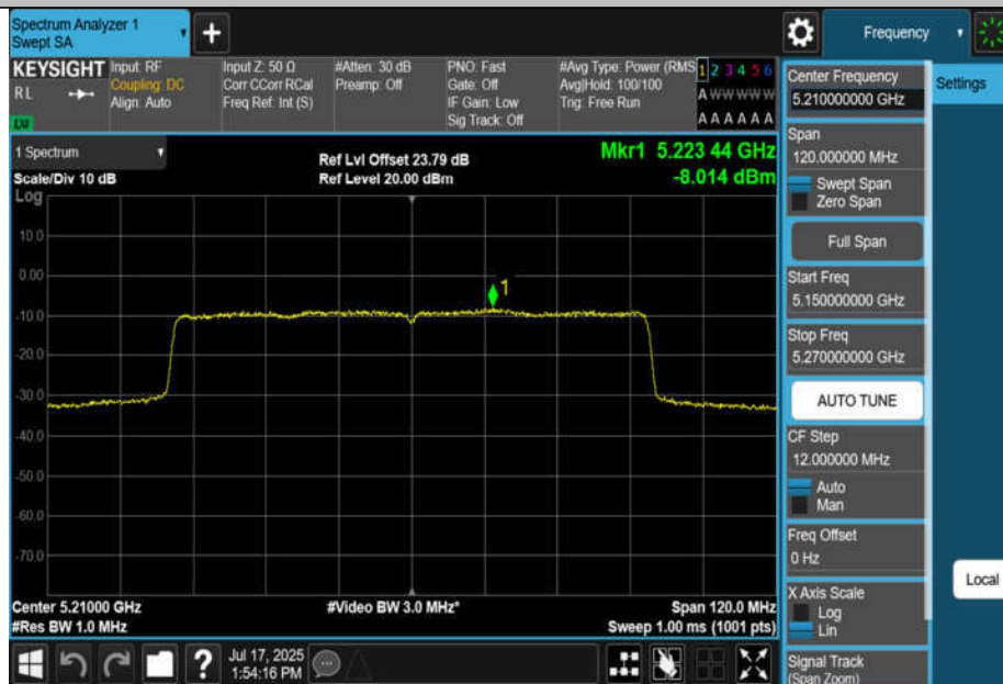
11BE80MIMO-Ant4-5210-PASS
