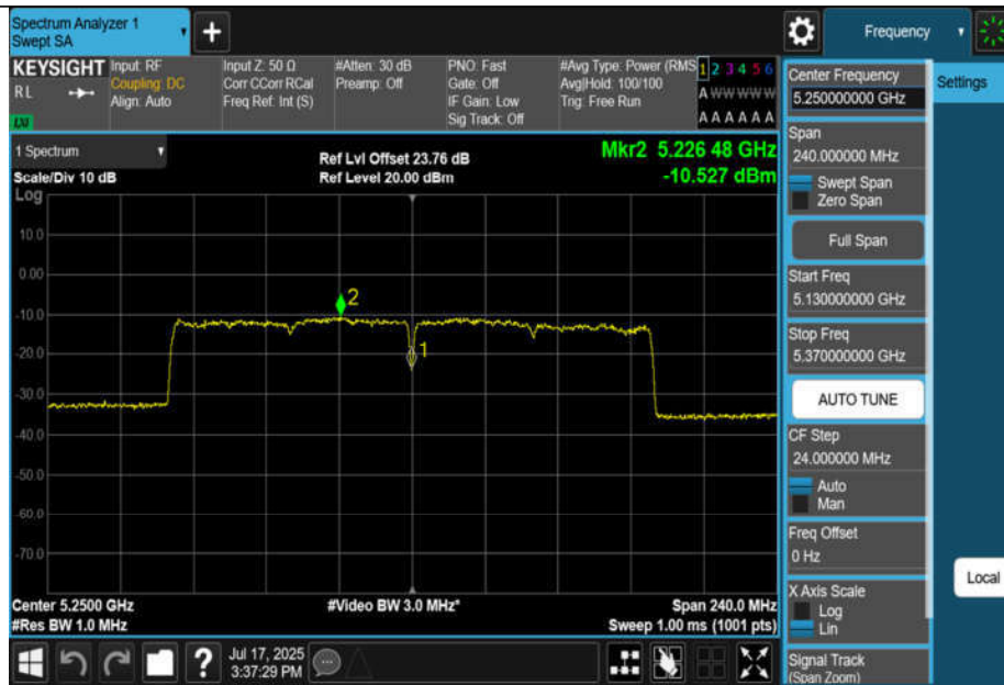
11BE160MIMO-Ant3-5250_UNII-1-PASS
