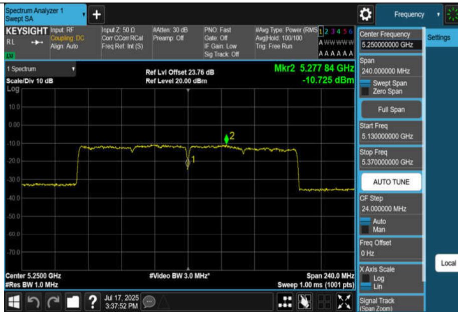
11BE160MIMO-Ant3-5250_UNII-2A-PASS
