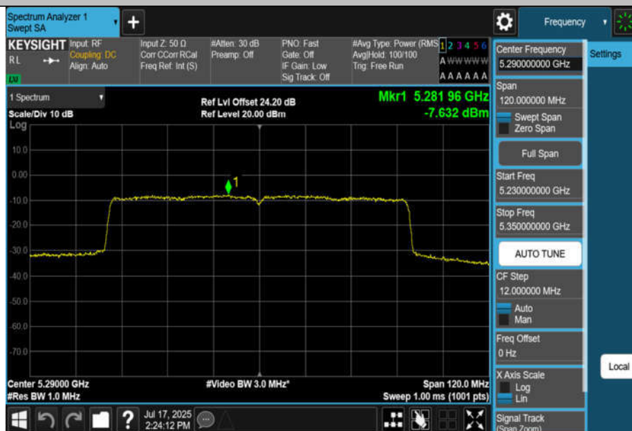
11BE80MIMO-Ant4-5290-PASS
