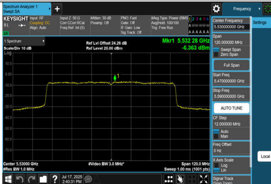
11BE80MIMO-Ant4-5530-PASS
