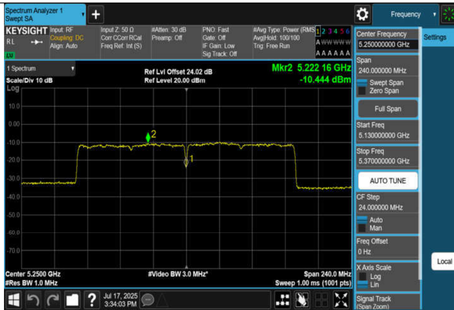
11BE160MIMO-Ant1-5250_UNII-1-PASS
