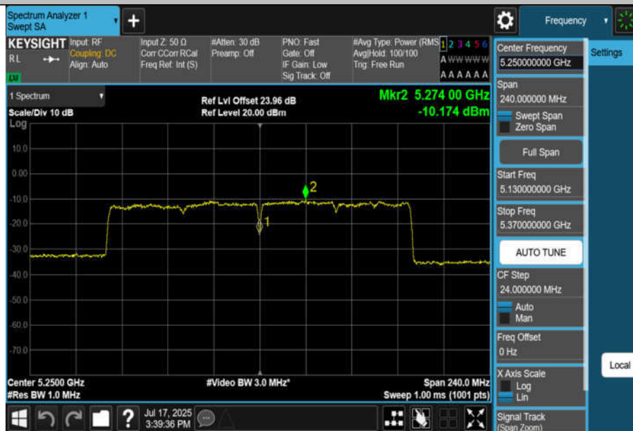
11BE160MIMO-Ant4-5250_UNII-2A-PASS
