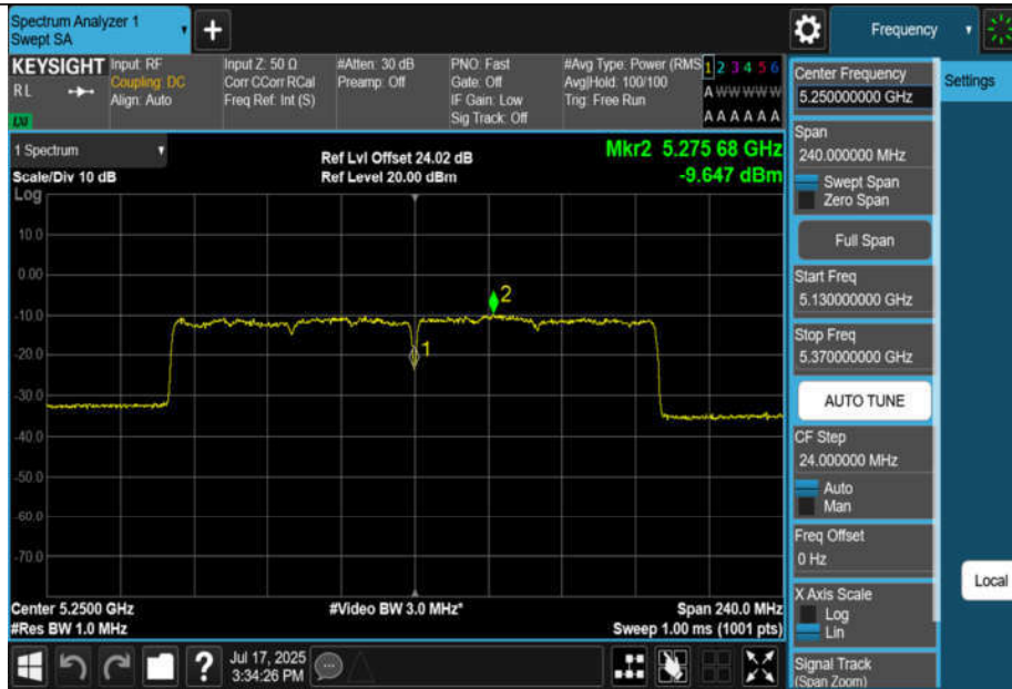
11BE160MIMO-Ant1-5250_UNII-2A-PASS
