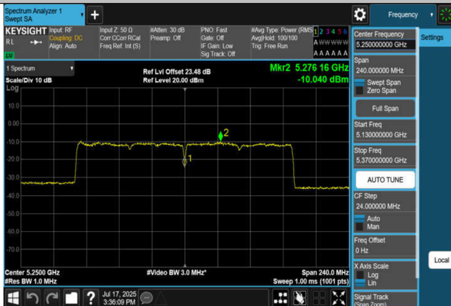
11BE160MIMO-Ant2-5250_UNII-2A-PASS
