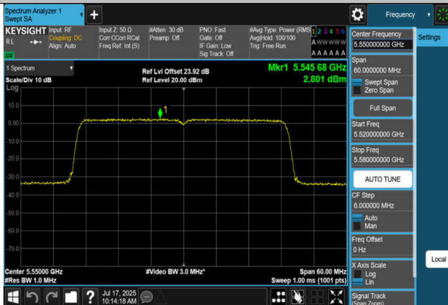
11BE40MIMO-Ant4-5550-PASS
