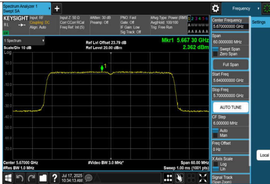
11BE40MIMO-Ant3-5670-PASS
