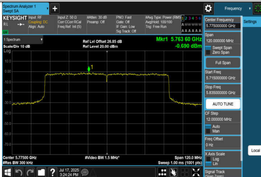
11BE80MIMO-Ant4-5775-PASS
