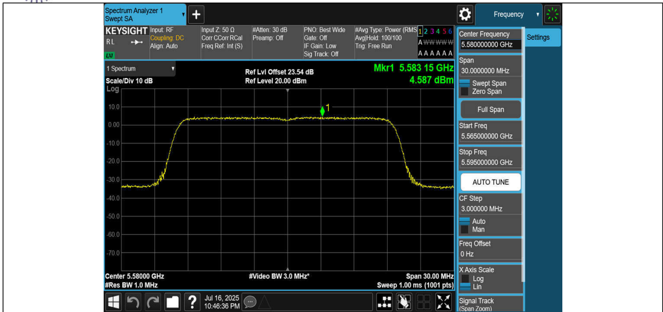
11BE20MIMO-Ant1-5580-PASS
