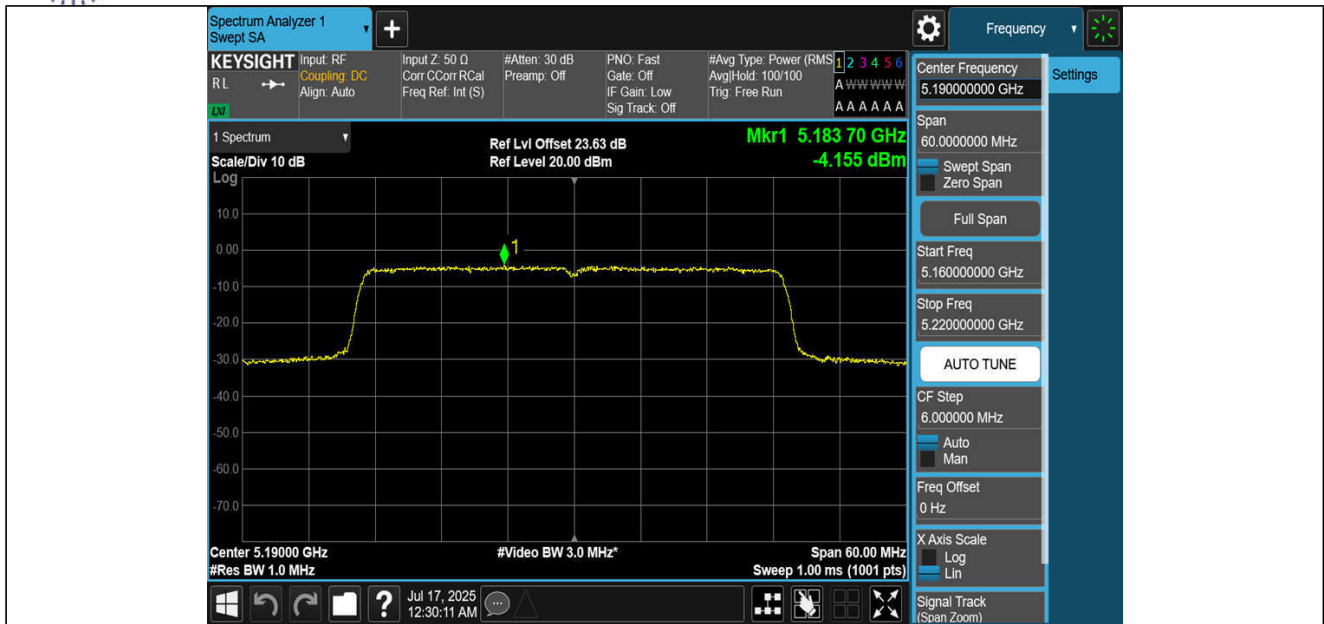
11BE40MIMO-Ant3-5190-PASS
