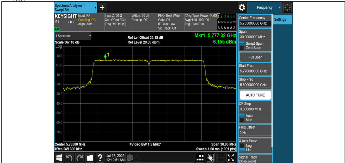
11BE20MIMO-Ant3-5785-PASS
