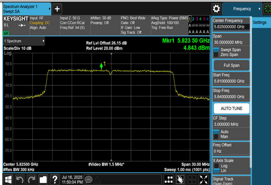
11BE20MIMO-Ant2-5825-PASS
