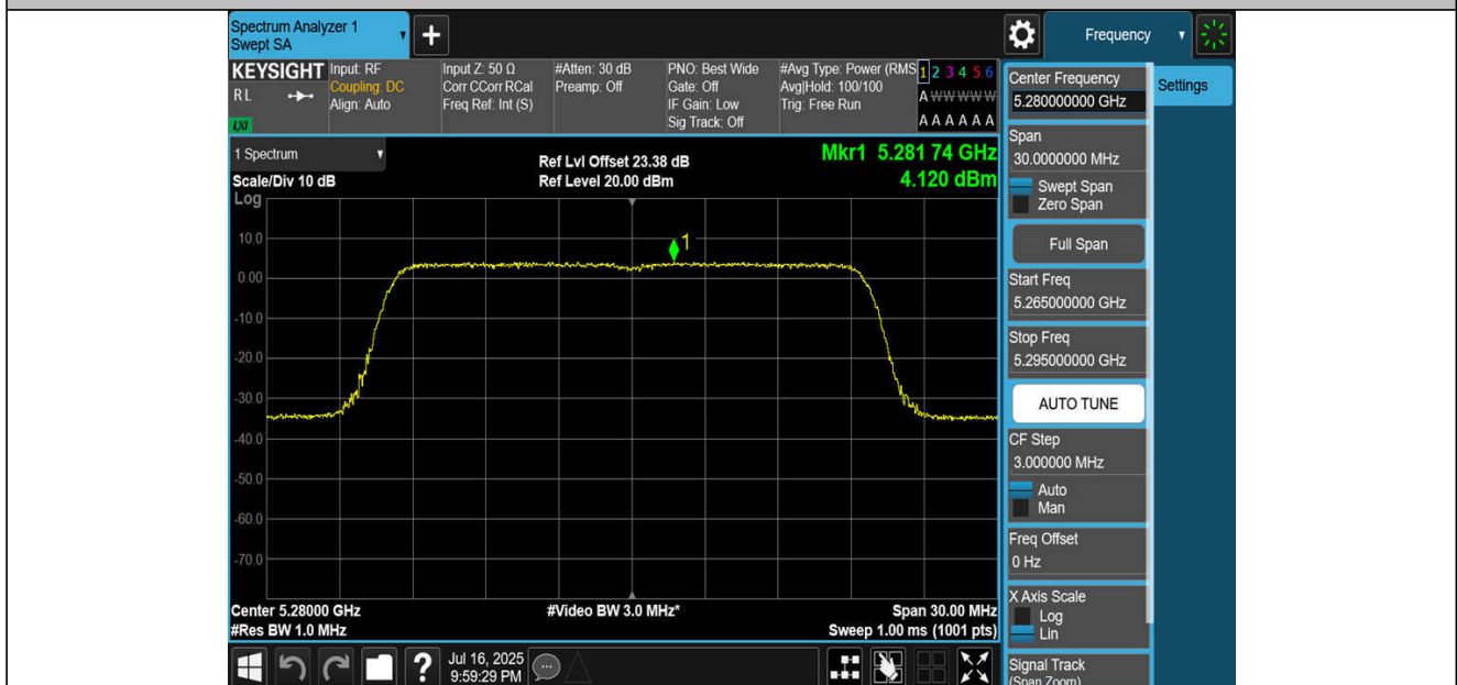
11BE20MIMO-Ant4-5280-PASS
