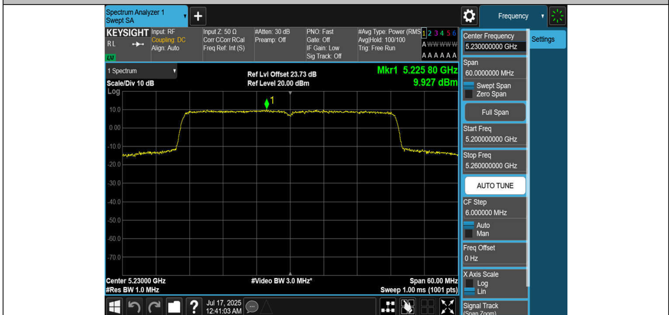
11BE40MIMO-Ant2-5230-PASS
