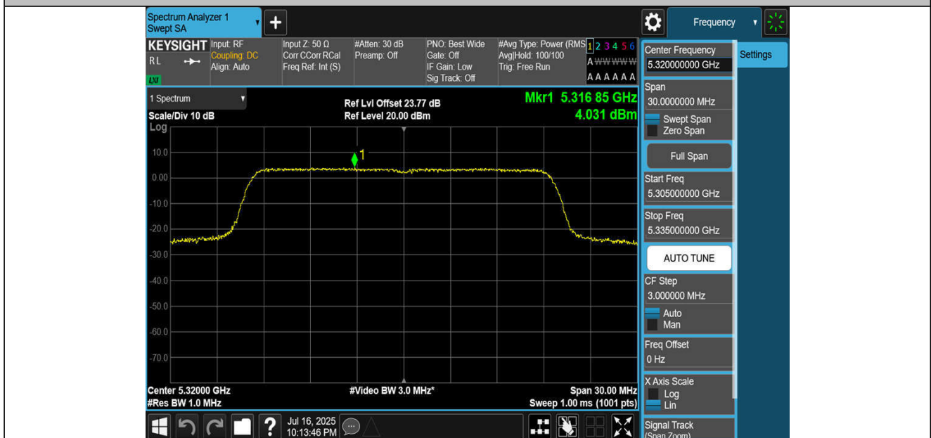
11BE20MIMO-Ant2-5320-PASS
