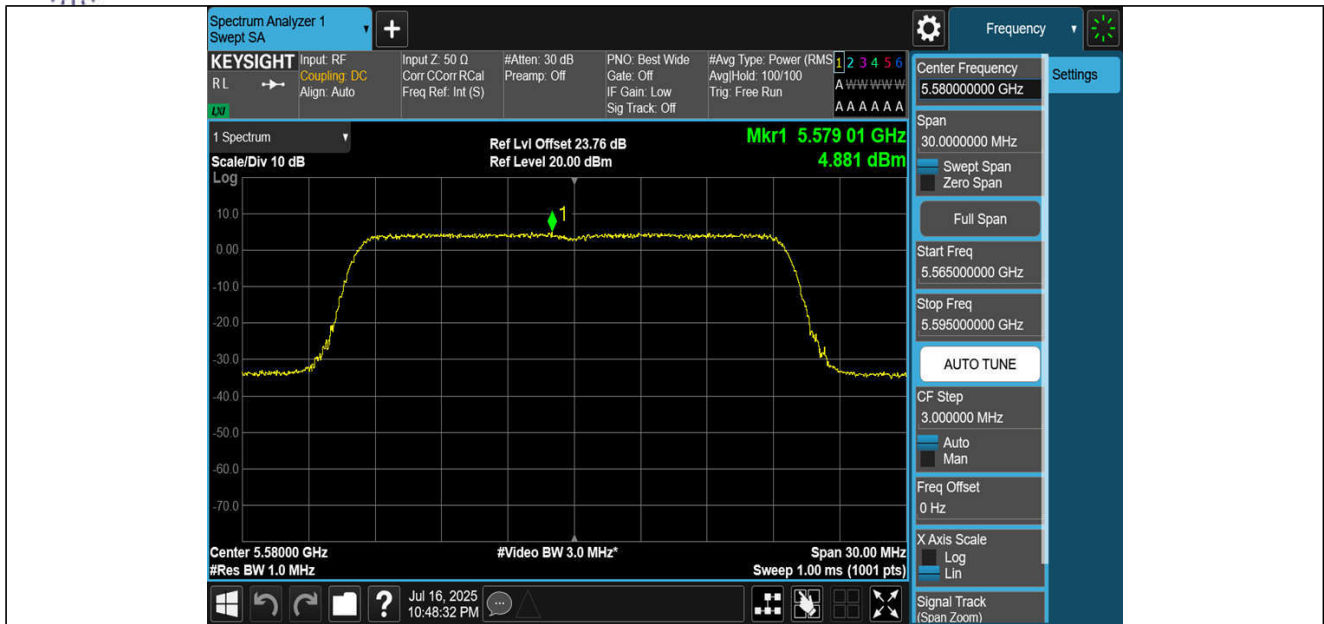
11BE20MIMO-Ant3-5580-PASS
