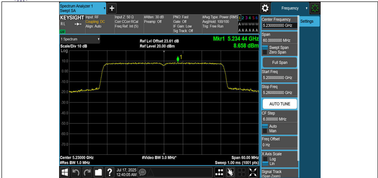
11BE40MIMO-Ant1-5230-PASS
