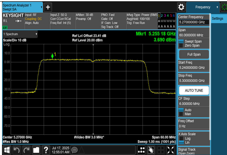
11BE40MIMO-Ant3-5270-PASS
