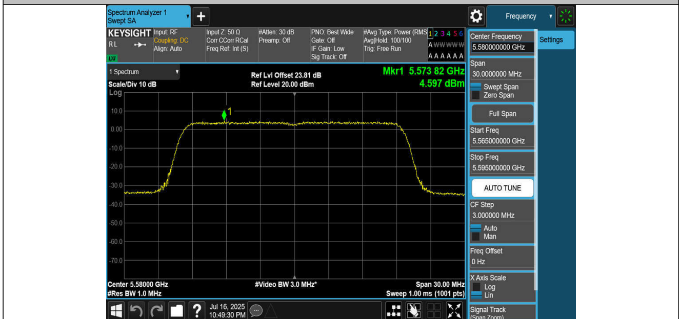
11BE20MIMO-Ant4-5580-PASS
