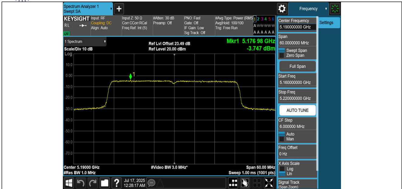
11BE40MIMO-Ant1-5190-PASS
