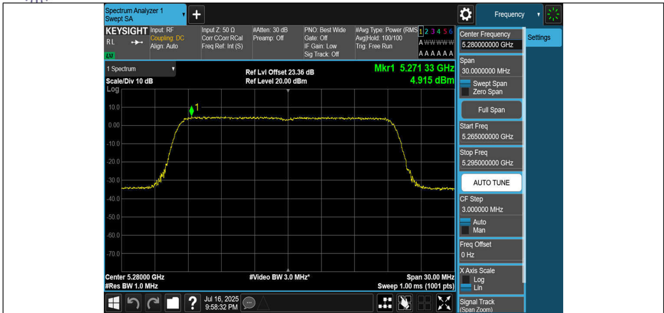
11BE20MIMO-Ant3-5280-PASS
