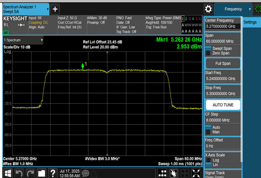
11BE40MIMO-Ant4-5270-PASS
