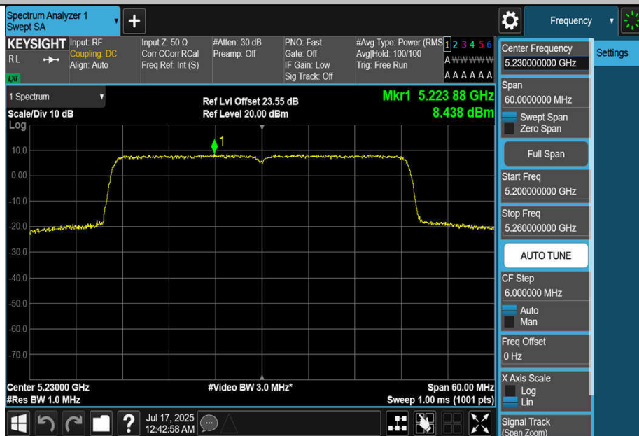
11BE40MIMO-Ant4-5230-PASS
