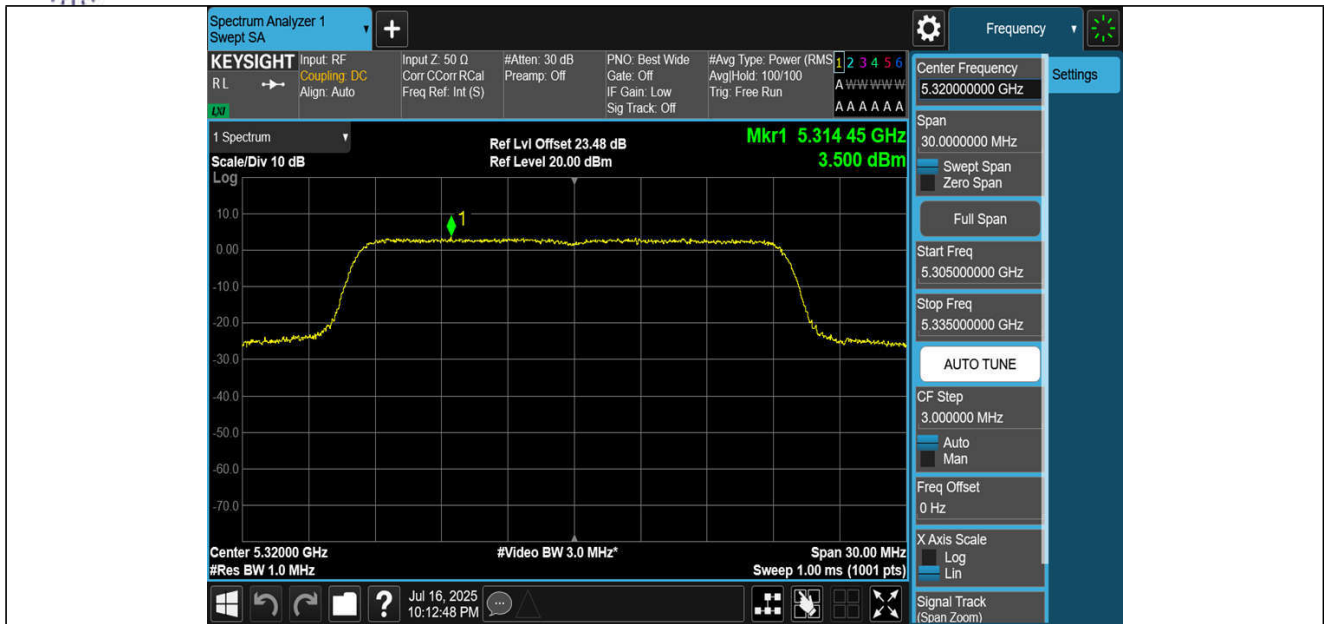
11BE20MIMO-Ant1-5320-PASS
