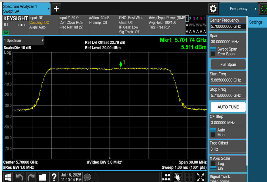
11BE20MIMO-Ant2-5700-PASS
