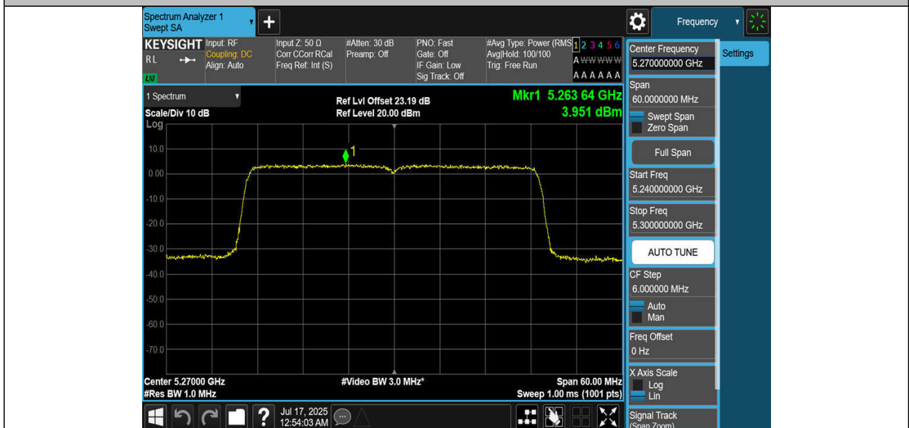
11BE40MIMO-Ant2-5270-PASS
