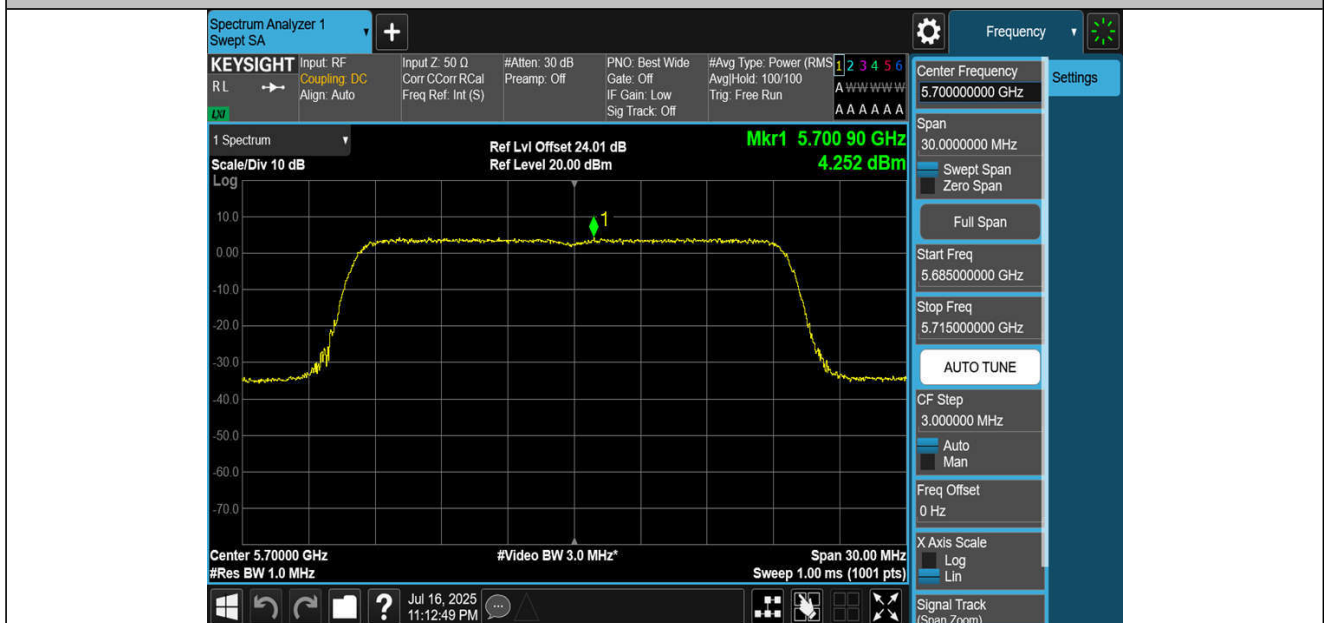
11BE20MIMO-Ant4-5700-PASS
