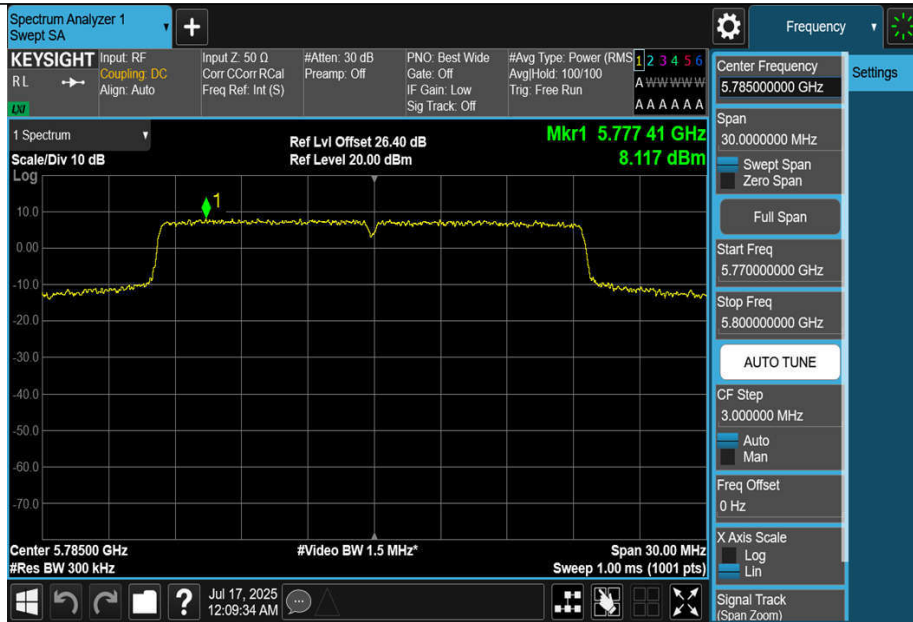
11BE20MIMO-Ant1-5785-PASS
