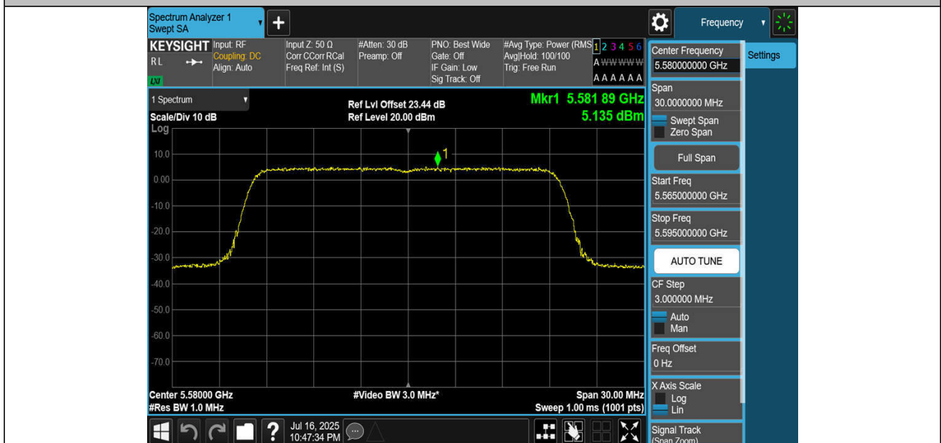
11BE20MIMO-Ant2-5580-PASS
