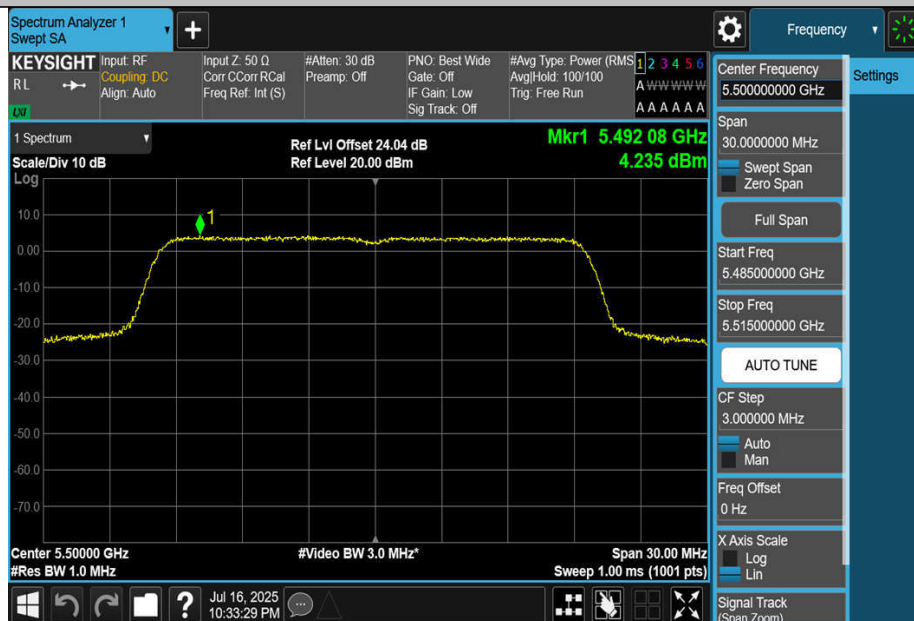
11BE20MIMO-Ant4-5500-PASS
