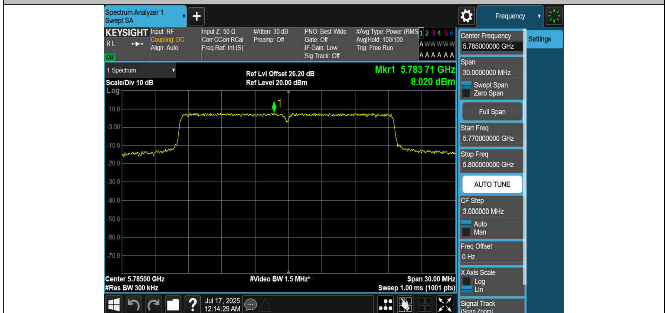
11BE20MIMO-Ant4-5785-PASS
