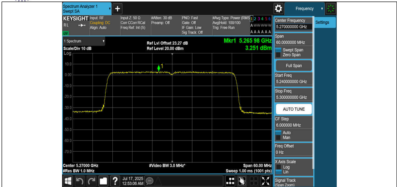
11BE40MIMO-Ant1-5270-PASS
