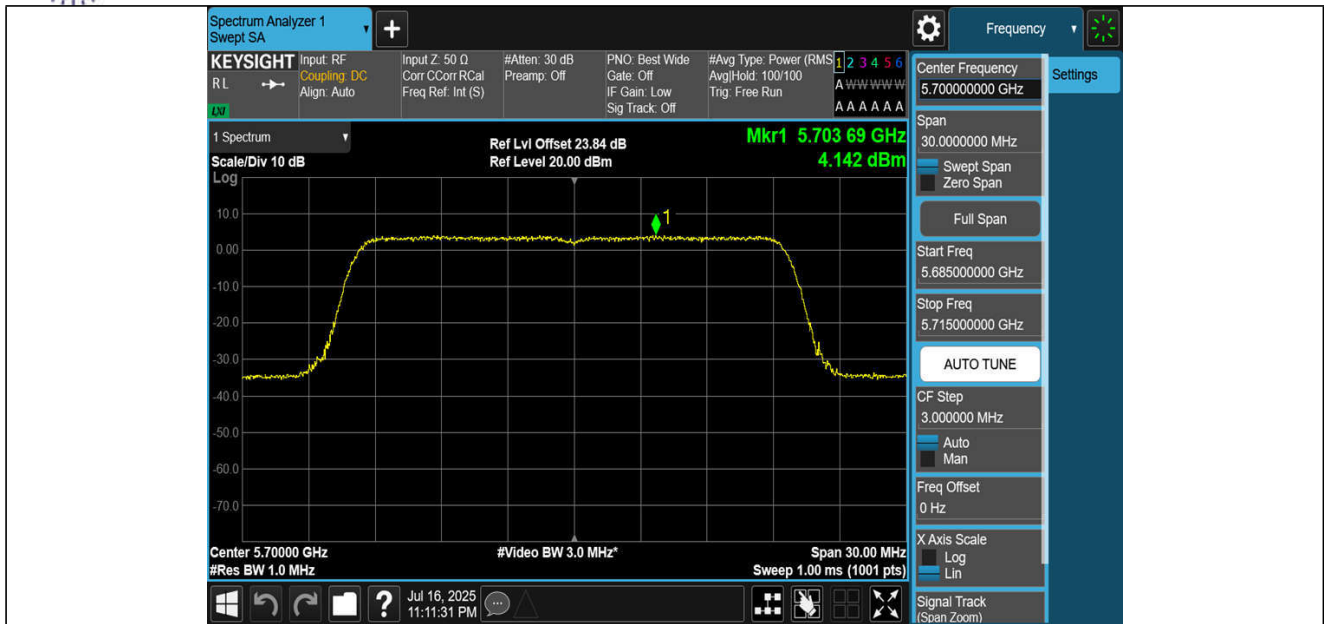
11BE20MIMO-Ant3-5700-PASS
