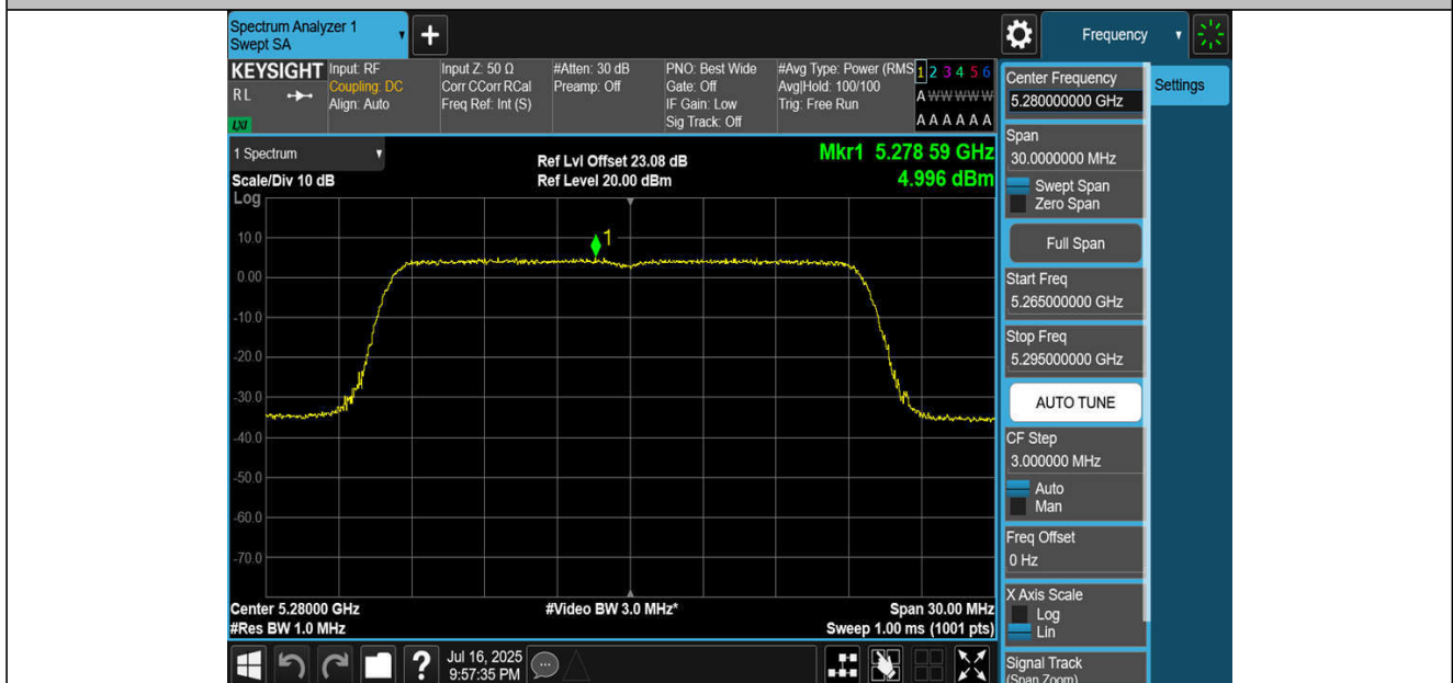
11BE20MIMO-Ant2-5280-PASS
