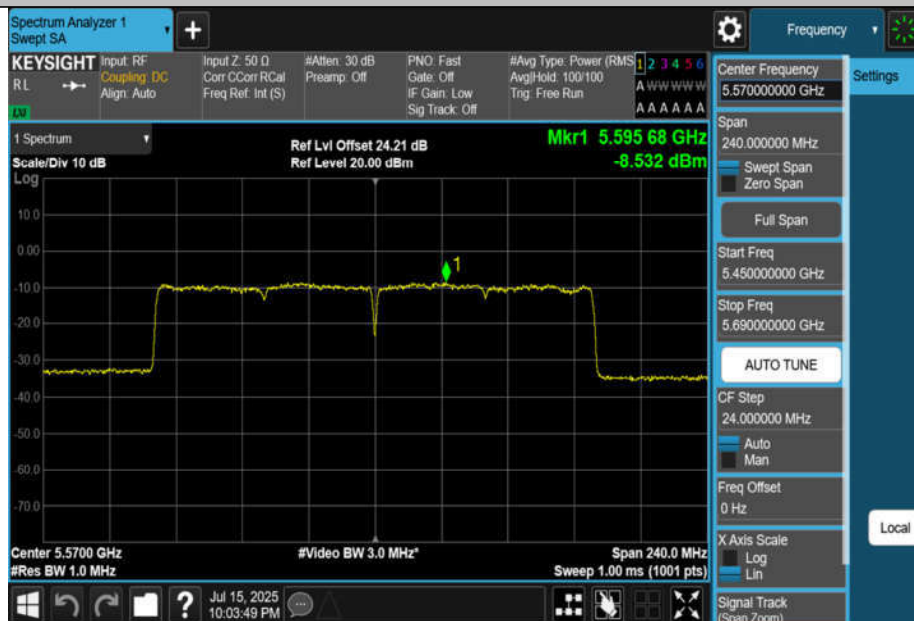
11AX160MIMO-Ant4-5570-PASS
