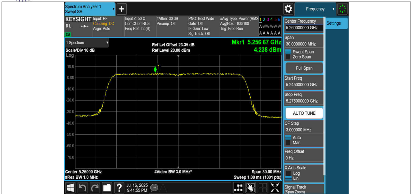
11BE20MIMO-Ant1-5260-PASS
