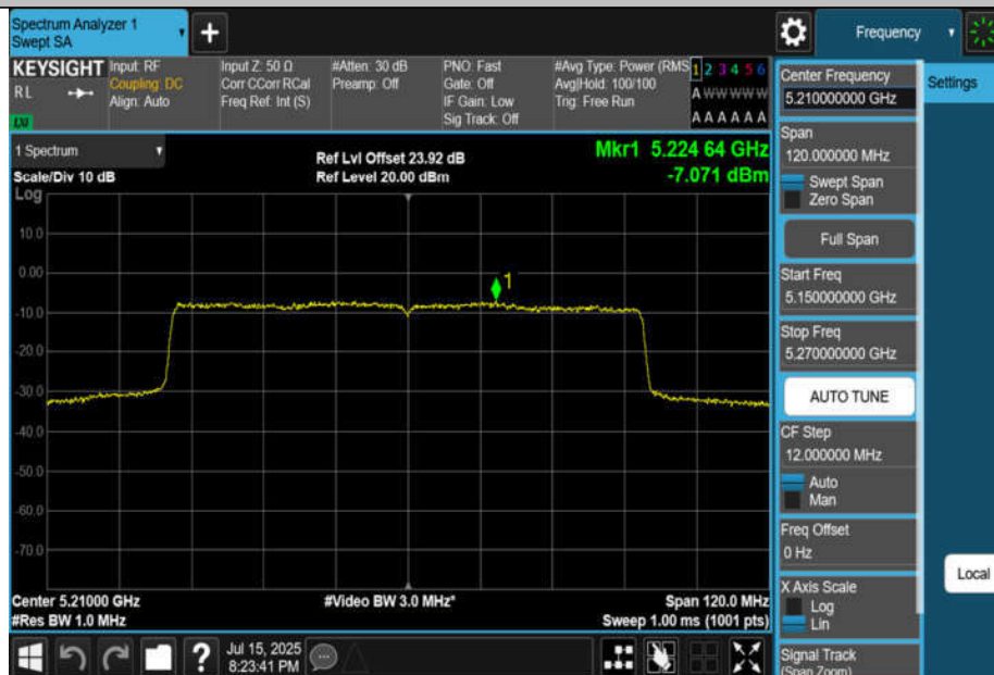
11AX80MIMO-Ant2-5210-PASS
