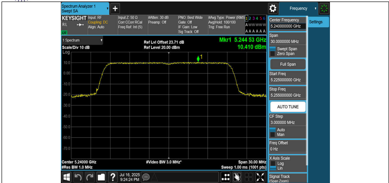
11BE20MIMO-Ant1-5240-PASS
