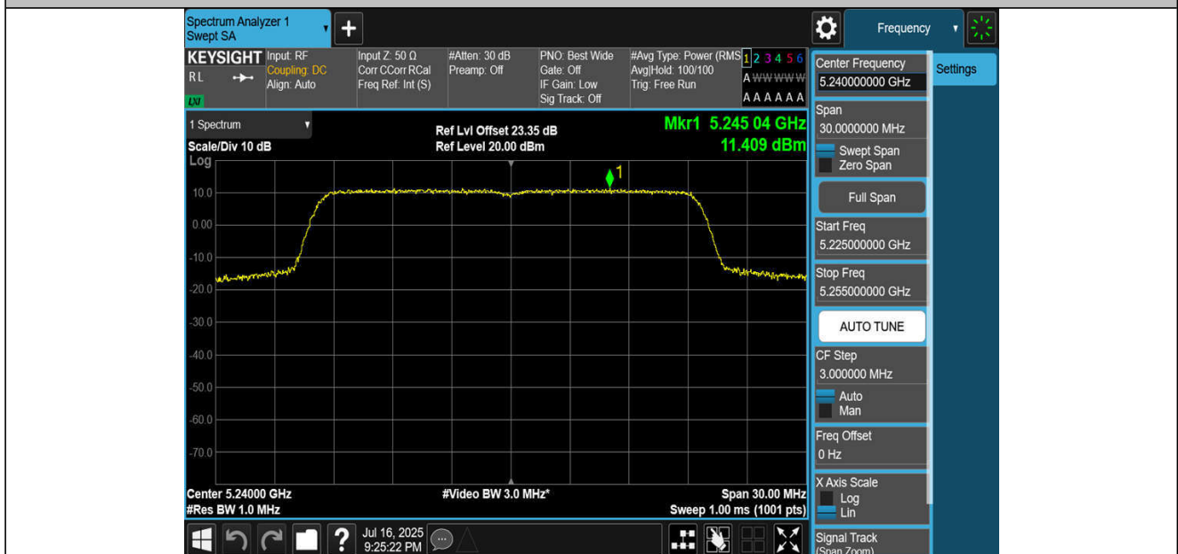
11BE20MIMO-Ant2-5240-PASS
