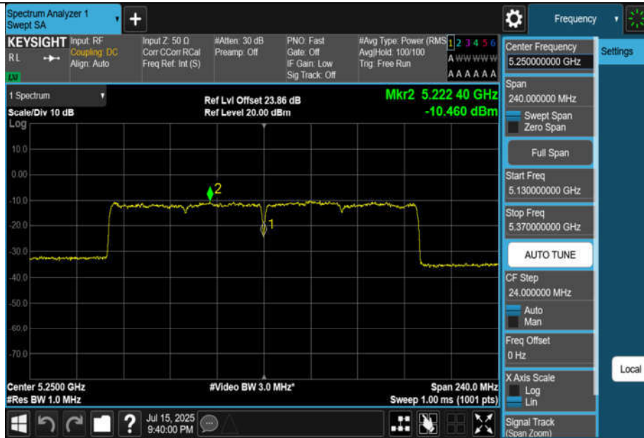
11AX160MIMO-Ant1-5250_UNII-1-PASS
