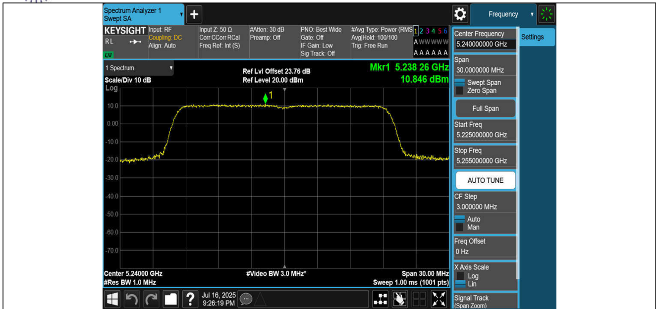
11BE20MIMO-Ant3-5240-PASS
