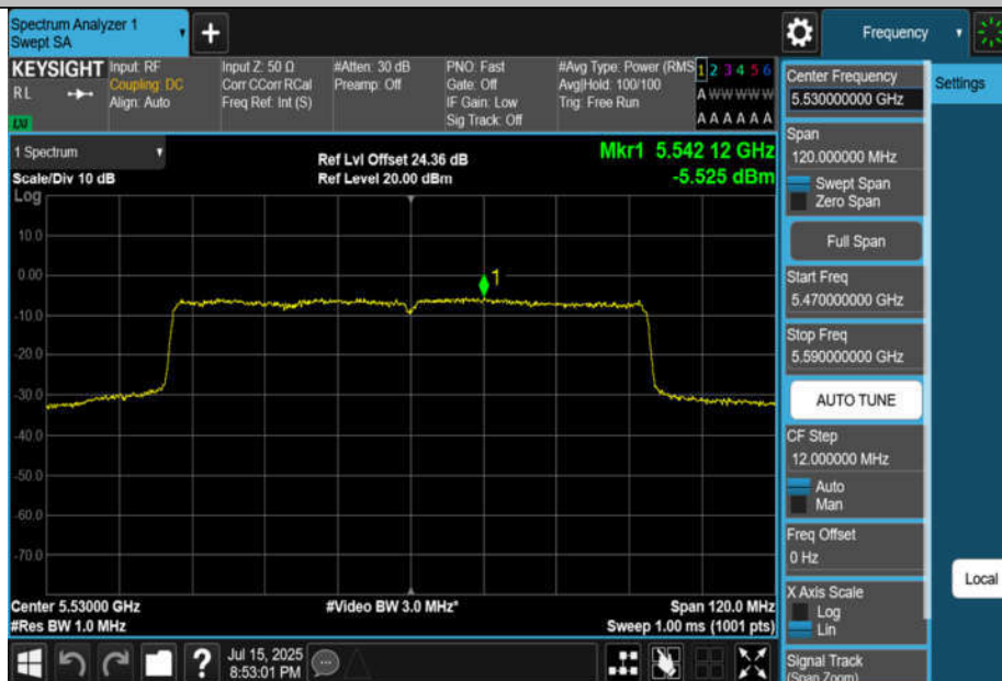
11AX80MIMO-Ant4-5530-PASS
