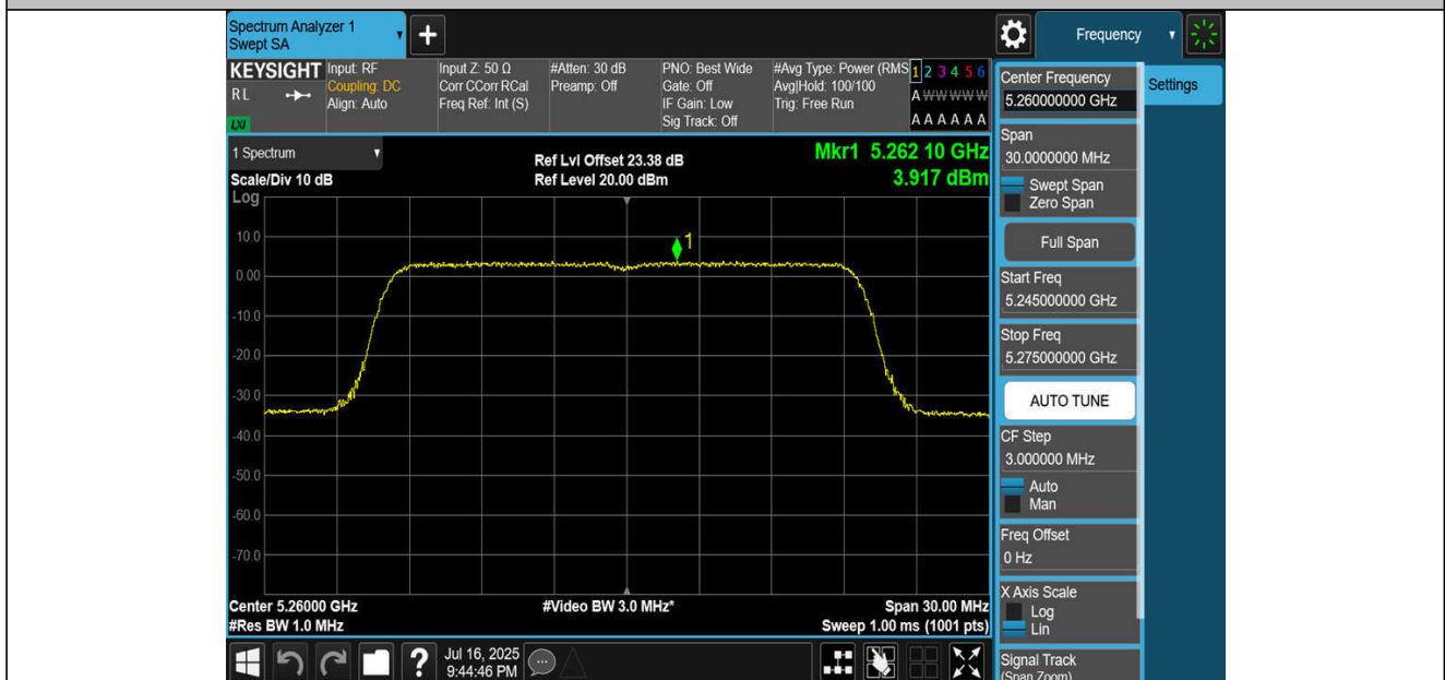
11BE20MIMO-Ant4-5260-PASS
