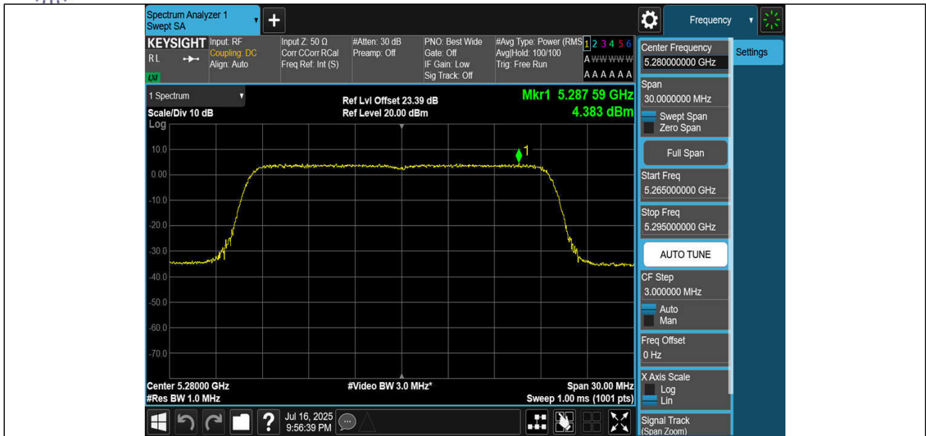
11BE20MIMO-Ant1-5280-PASS
