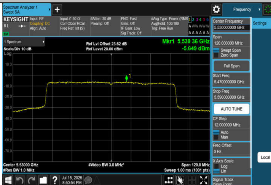
11AX80MIMO-Ant2-5530-PASS
