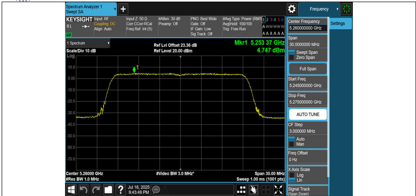
11BE20MIMO-Ant3-5260-PASS
