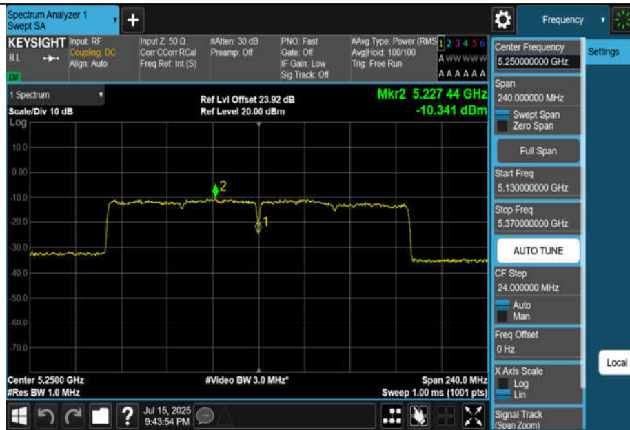
11AX160MIMO-Ant3-5250_UNII-1-PASS
