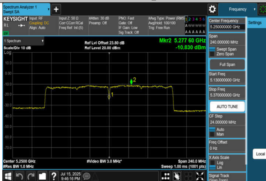
11AX160MIMO-Ant4-5250_UNII-2A-PASS
