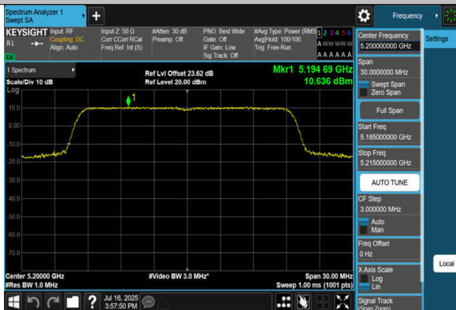
11BE20MIMO-Ant2-5200-PASS
