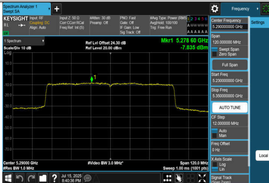
11AX80MIMO-Ant4-5290-PASS
