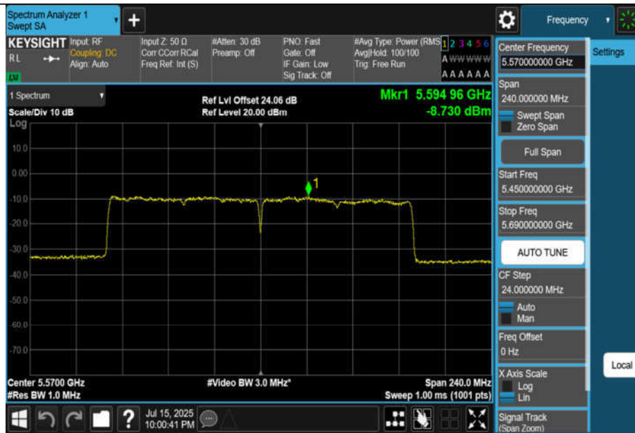
11AX160MIMO-Ant1-5570-PASS
