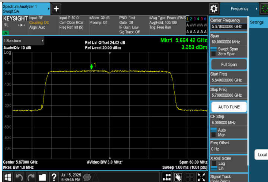
11AX40MIMO-Ant4-5670-PASS
