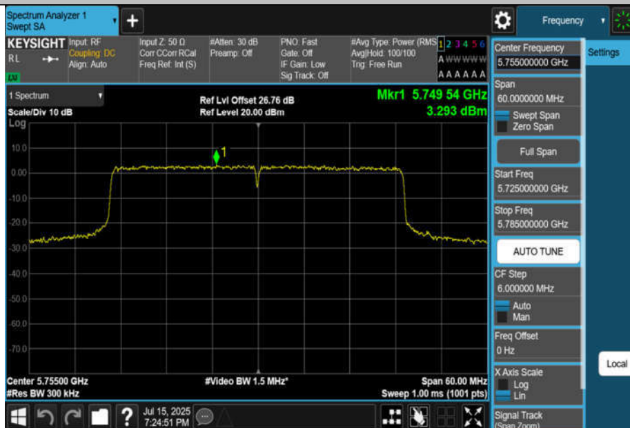
11AX40MIMO-Ant4-5755-PASS
