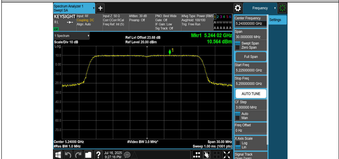
11BE20MIMO-Ant4-5240-PASS
