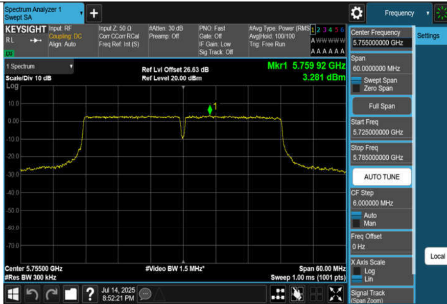
11AC40MIMO-Ant3-5755-PASS
