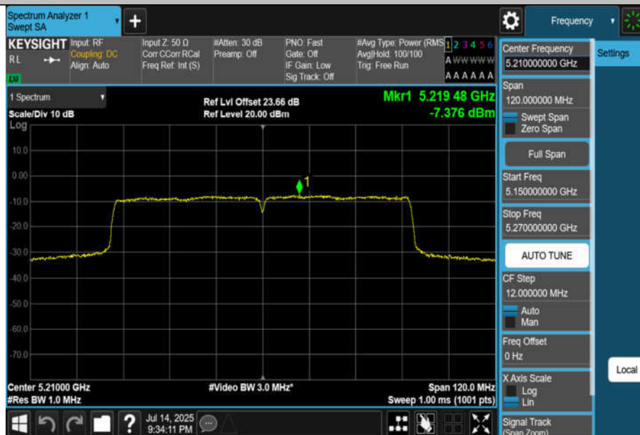
11AC80MIMO-Ant4-5210-PASS
