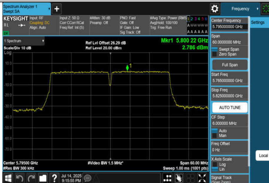
11AC40MIMO-Ant4-5795-PASS
