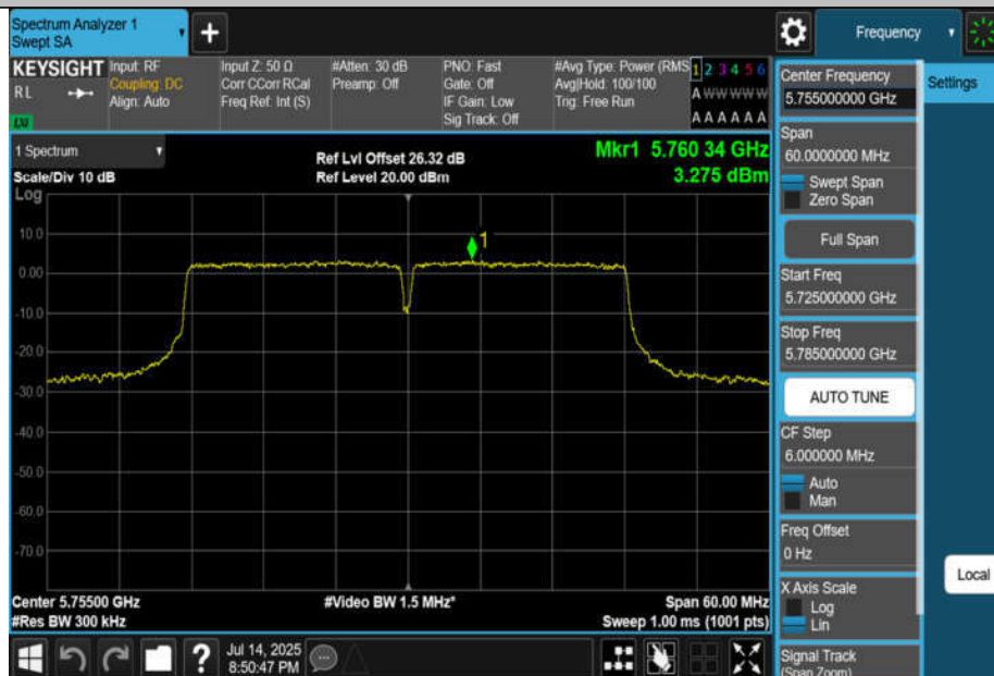
11AC40MIMO-Ant2-5755-PASS
