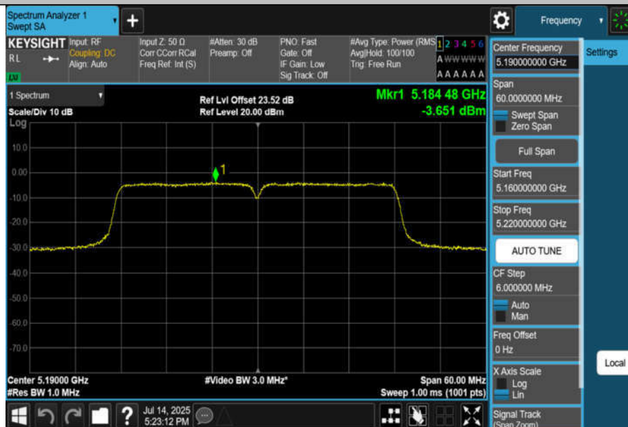
11AC40MIMO-Ant4-5190-PASS
