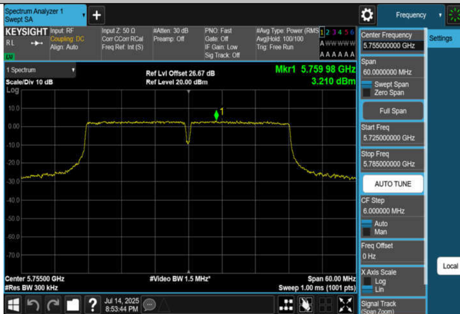
11AC40MIMO-Ant4-5755-PASS
