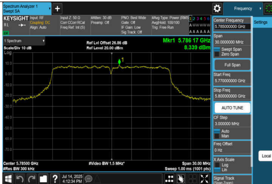
11AC20MIMO-Ant3-5785-PASS
