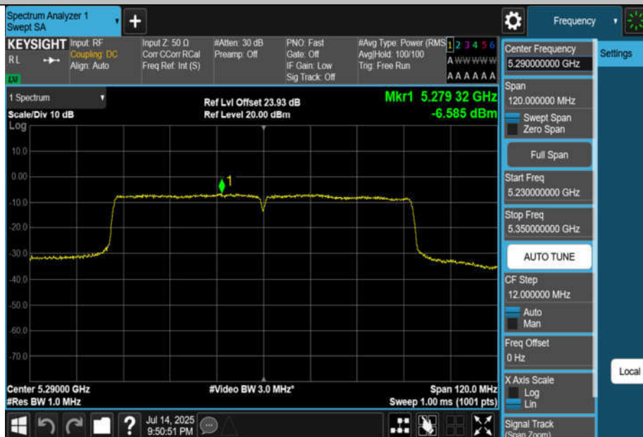
11AC80MIMO-Ant2-5290-PASS
