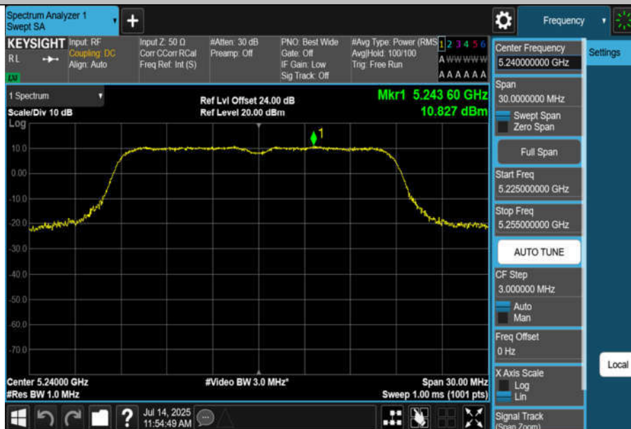
11AC20MIMO-Ant2-5240-PASS
