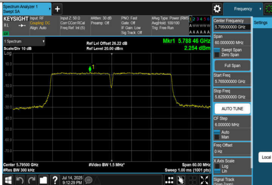
11AC40MIMO-Ant2-5795-PASS
