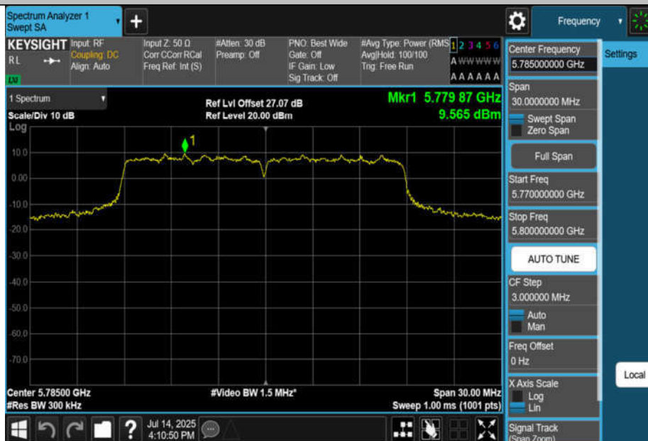
11AC20MIMO-Ant2-5785-PASS
