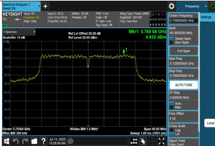
11N40MIMO-Ant3-5755-PASS
