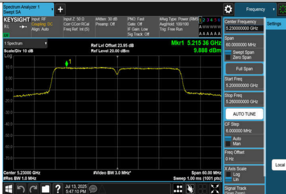
11N40MIMO-Ant2-5230-PASS
