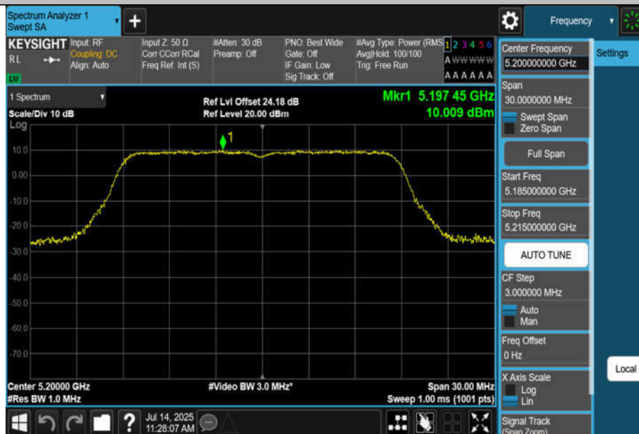
11AC20MIMO-Ant4-5200-PASS
