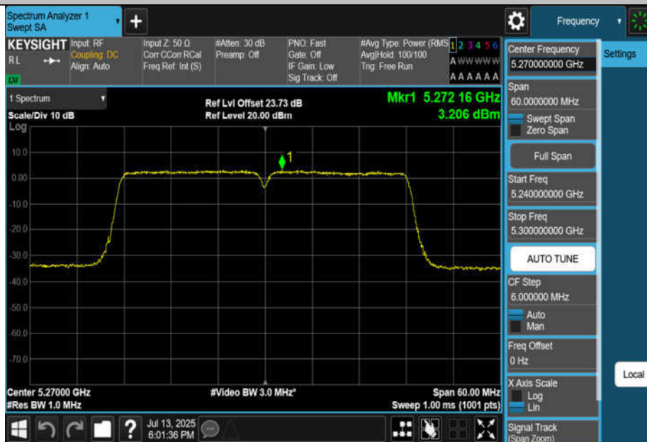
11N40MIMO-Ant4-5270-PASS
