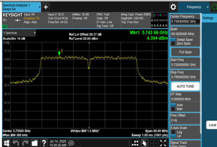
11N40MIMO-Ant4-5755-PASS
