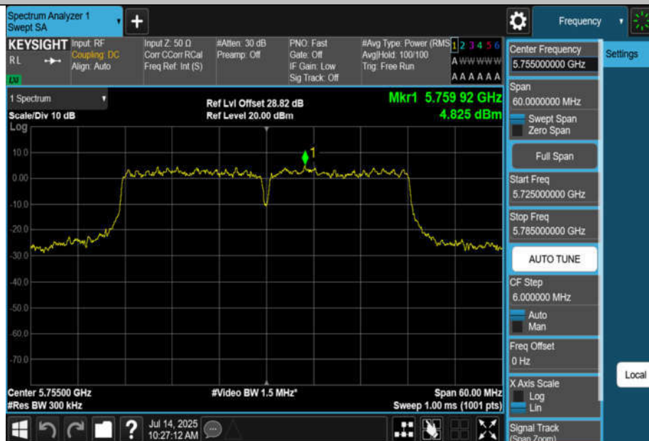
11N40MIMO-Ant2-5755-PASS
