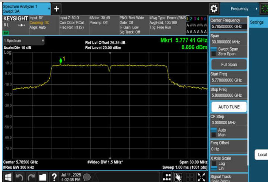
11N20MIMO-Ant4-5785-PASS
