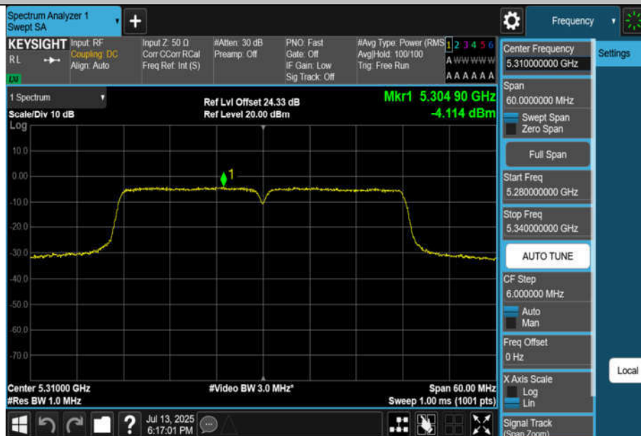
11N40MIMO-Ant4-5310-PASS
