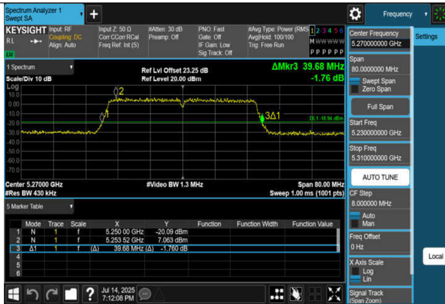
11AC40MIMO-Ant3-5270
