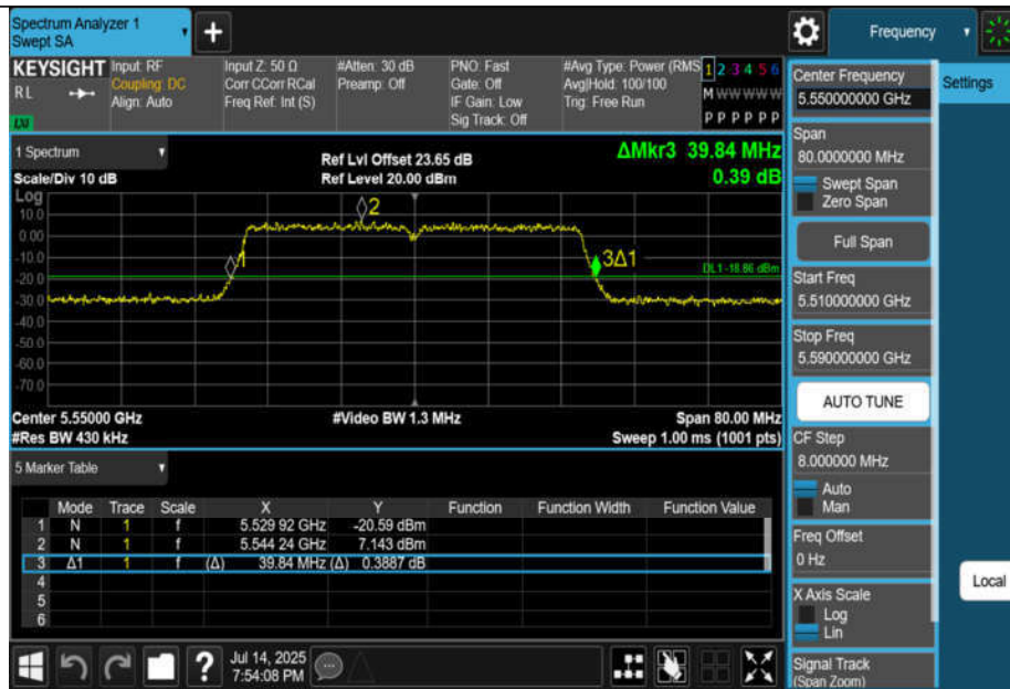
11AC40MIMO-Ant3-5550
