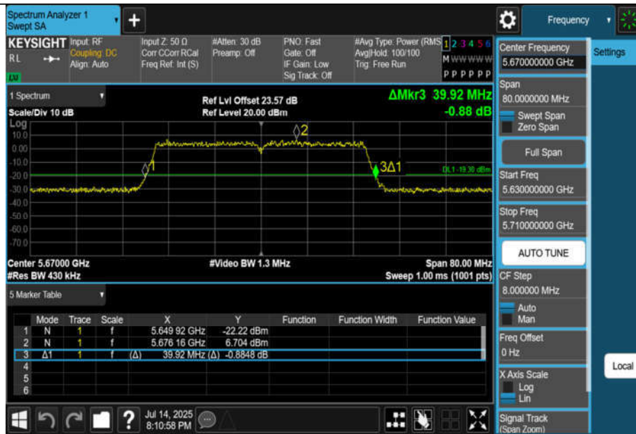
11AC40MIMO-Ant3-5670
