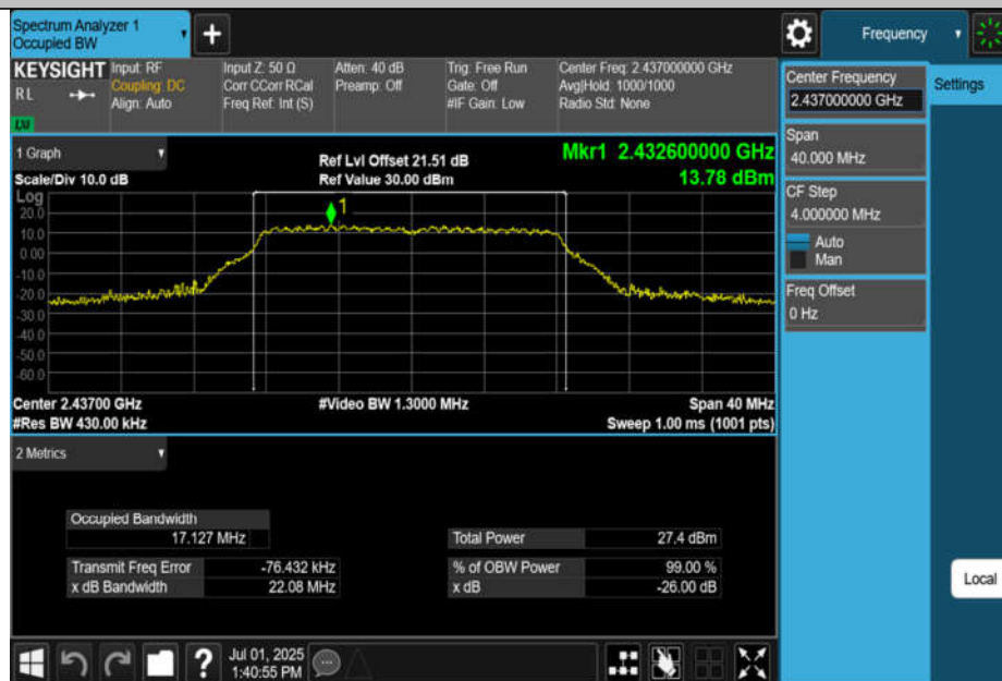
11G-CDD-Ant2-2437
