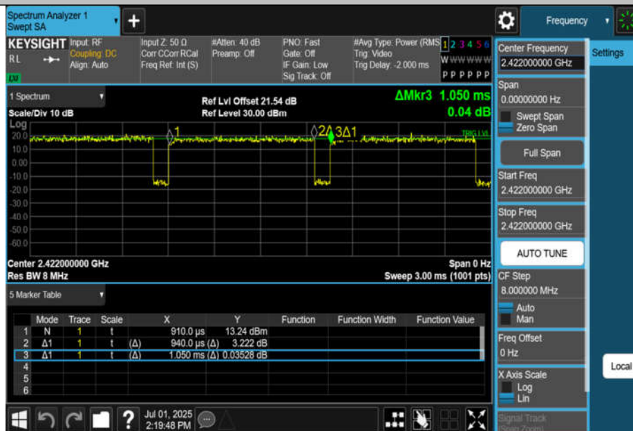
NTNV-11N40MIMO-Ant1-2422
