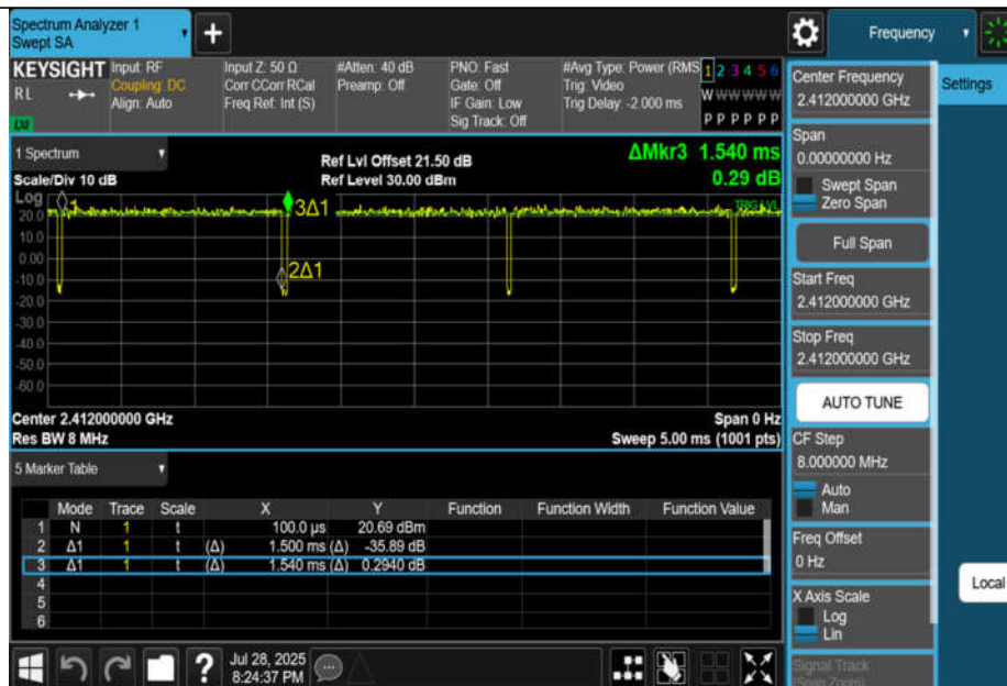
NTNV-11BE20MIMO-Ant1-2412
