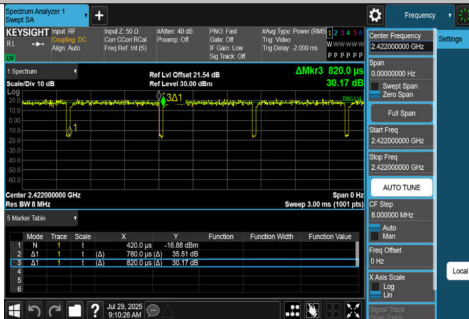
NTNV-11BE40MIMO-Ant1-2422
