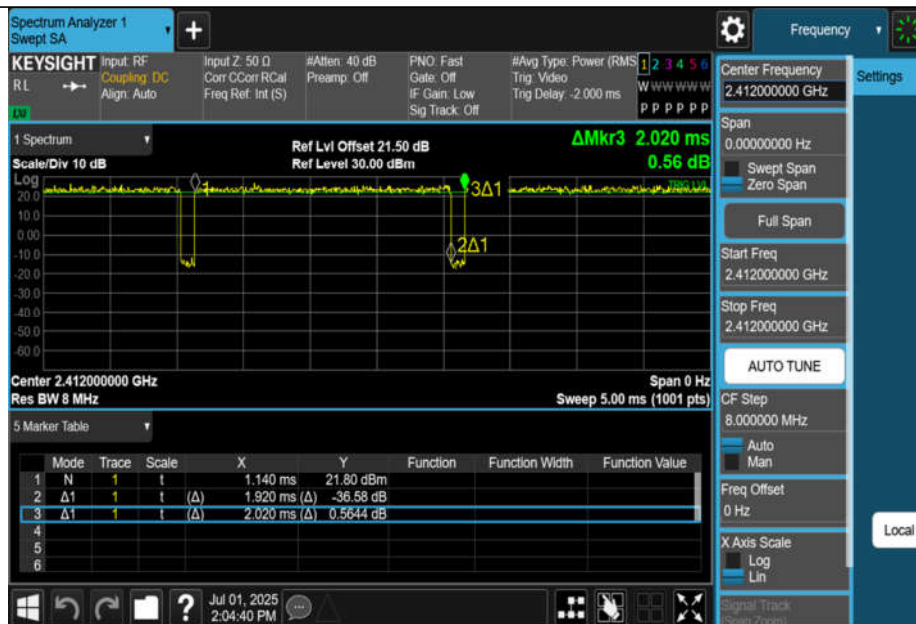
NTNV-11N20MIMO-Ant1-2412
