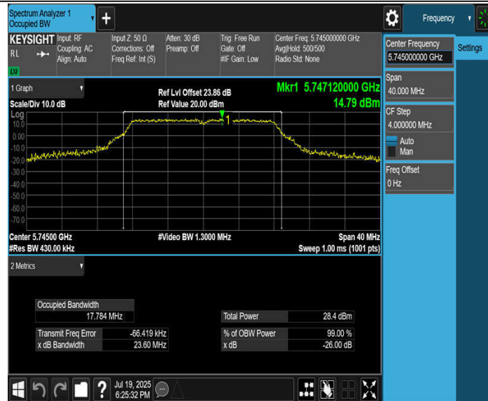
11A-CDD_Ant3_5745
