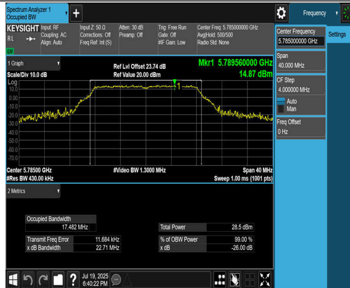
11A-CDD_Ant3_5785
