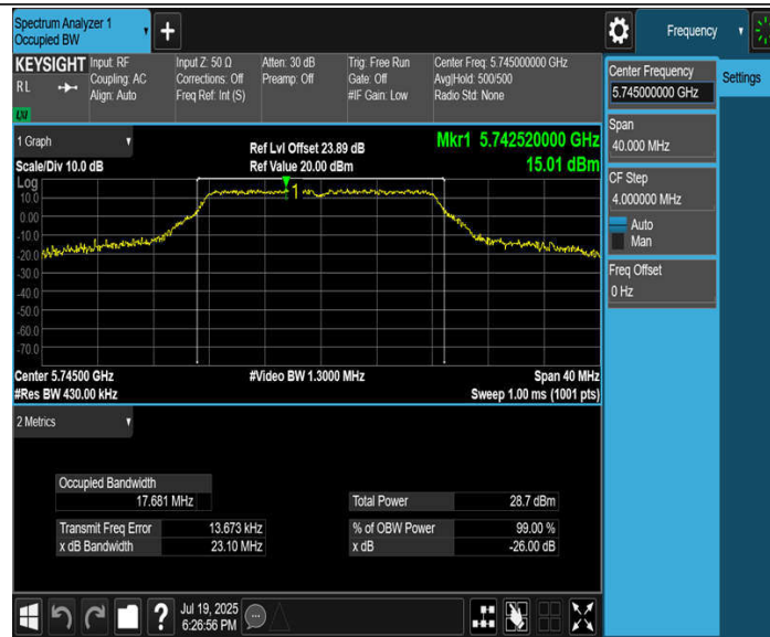
11A-CDD_Ant4_5745
