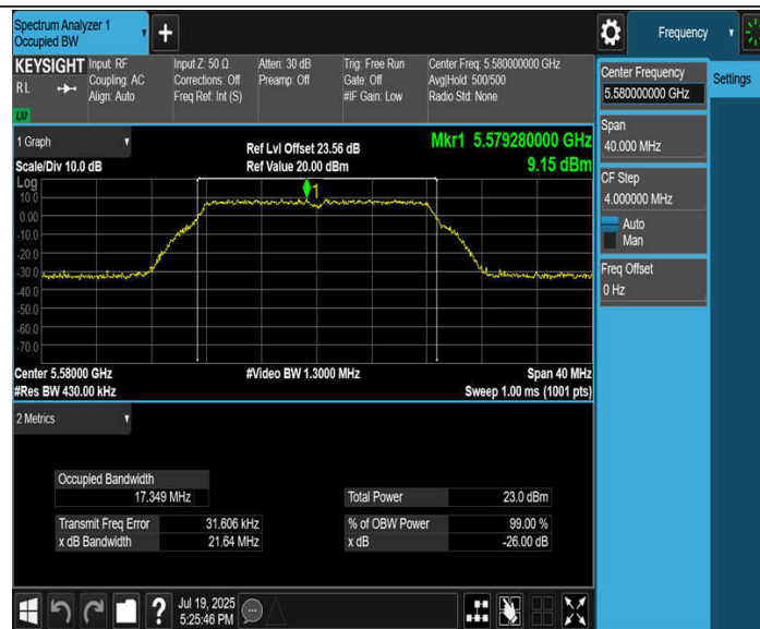
11A-CDD_Ant4_5580
