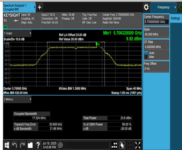
11A-CDD_Ant4_5700
