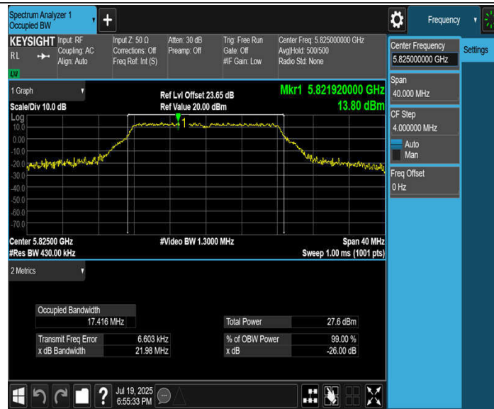
11A-CDD_Ant4_5825
