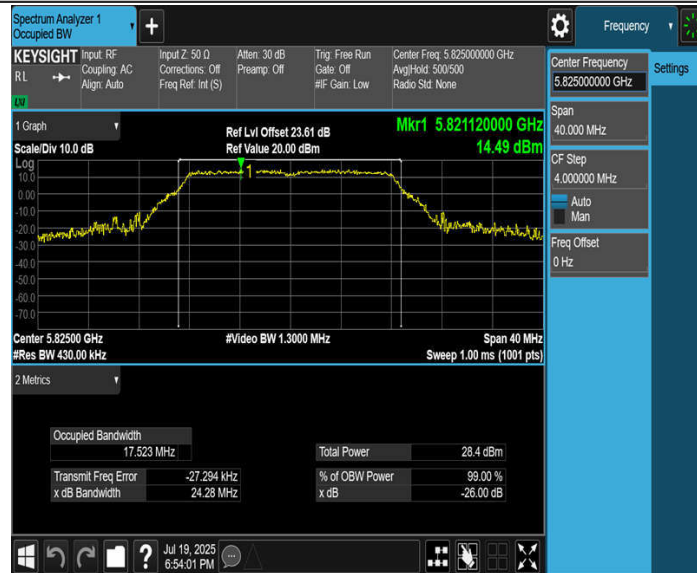
11A-CDD_Ant3_5825
