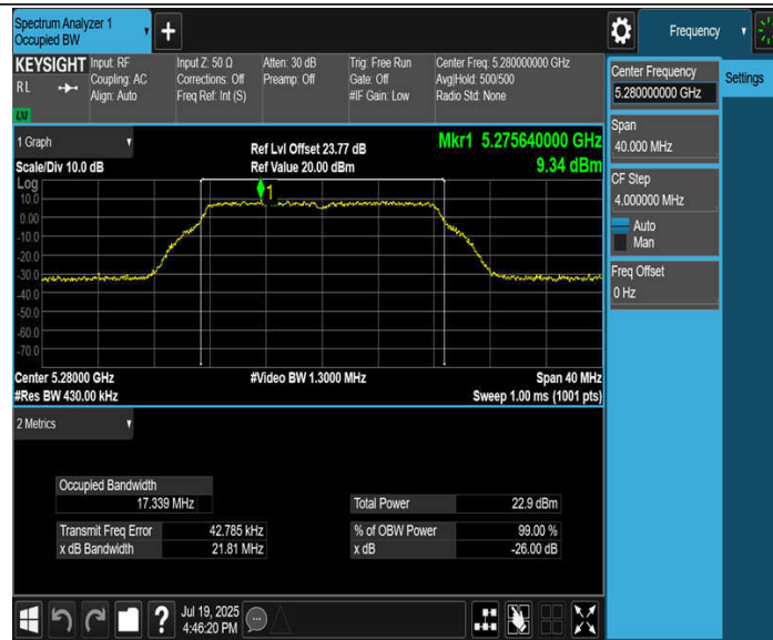
11A-CDD_Ant4_5280
