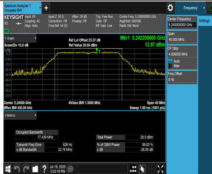
11A-CDD_Ant3_5240
