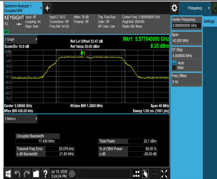
11A-CDD_Ant3_5580
