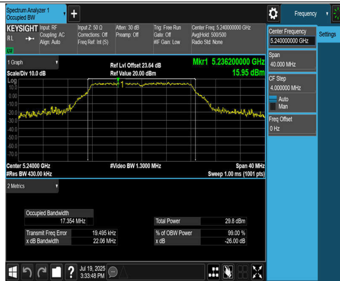
11A-CDD_Ant4_5240
