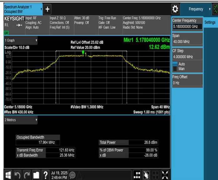
11A-CDD_Ant3_5180
