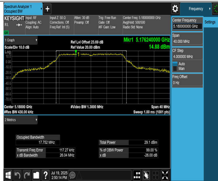
11A-CDD_Ant4_5180
