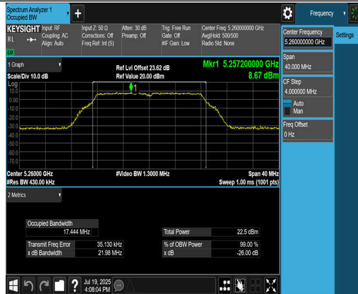
11A-CDD_Ant3_5260
