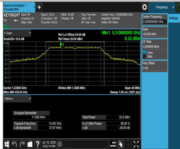
11A-CDD_Ant4_5320
