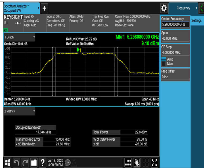
11A-CDD_Ant4_5260
