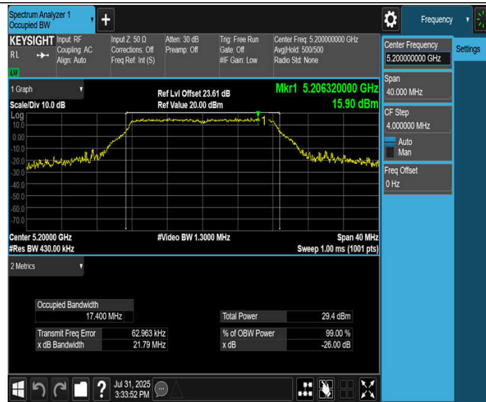
11A-CDD_Ant4_5200
