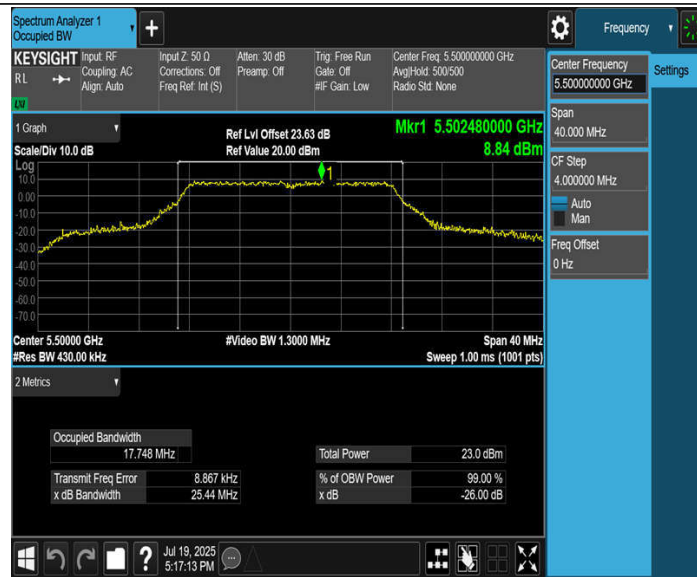
11A-CDD_Ant4_5500
