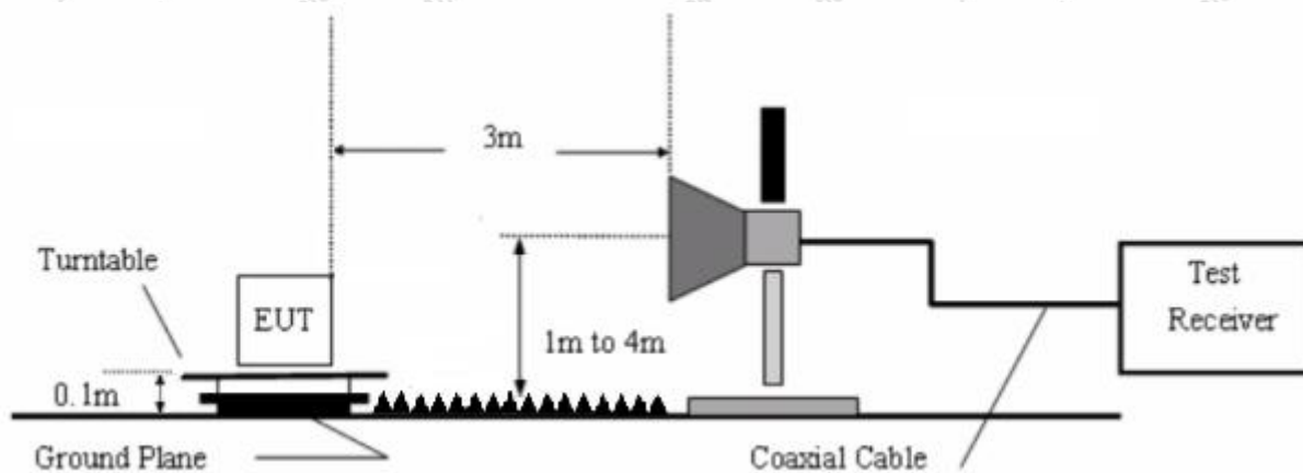
Figure 3. Above 1 GHz
