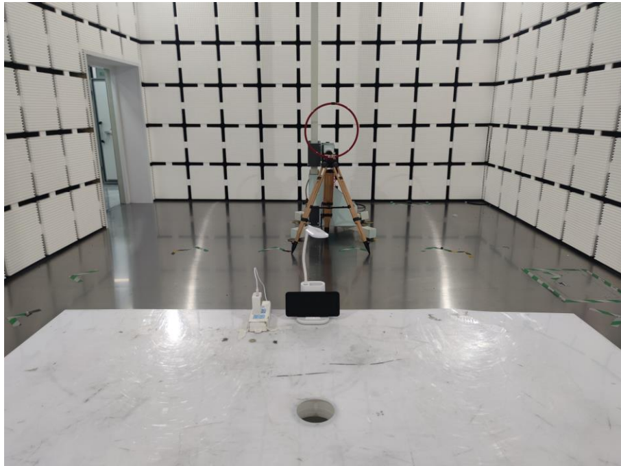
Radiation (9KHz-30MHz)
