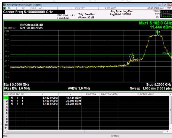
(802.11n20) Band Edge, Left Side
