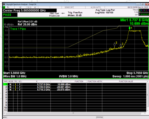
(802.11ac40) Band Edge, Left Side
