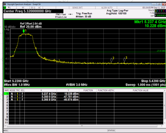
(802.11ac40) Band Edge, Right Side
