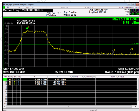
(802.11n40) Band Edge, Right Side
