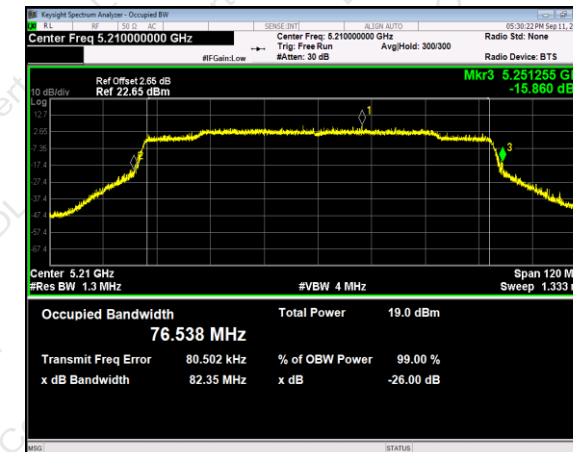
(802.11 ac80) 26dB Bandwidth plot on channel 42
