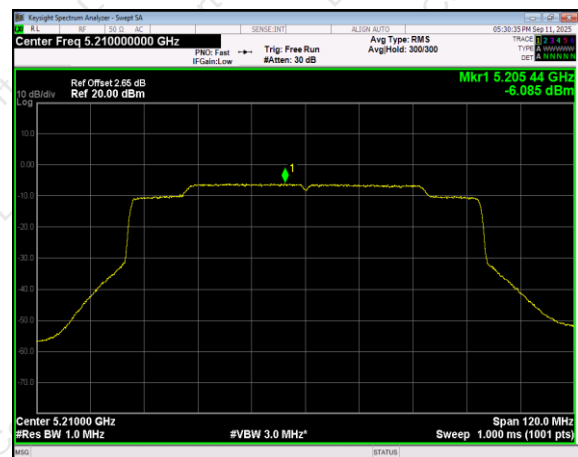
(802.11ac80) PSD plot on channel 42
