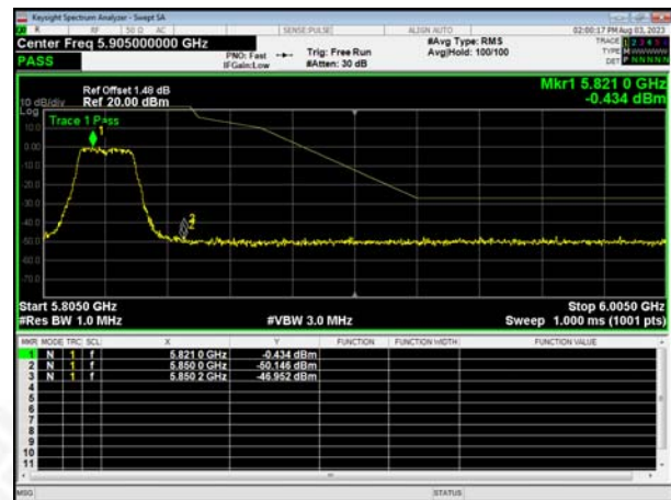
(802.11ac40) Highest channel
