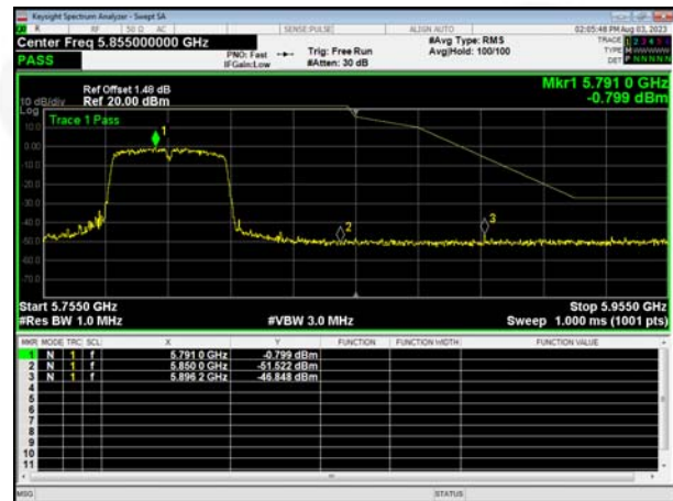
(802.11n40) Highest channel
