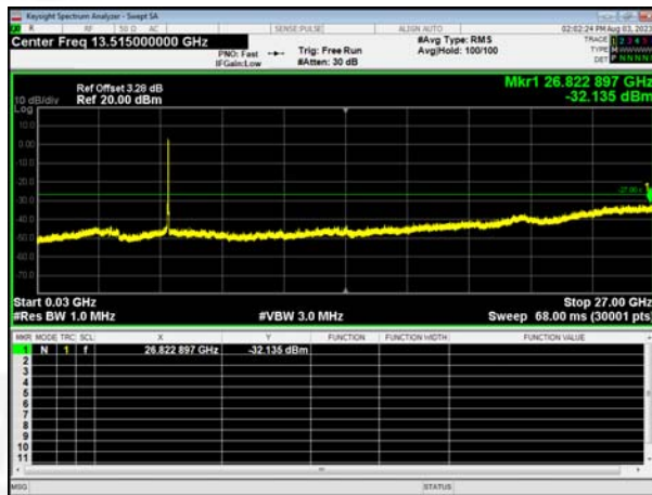
(802.11 n40) Tx. Spurious plot on channel 159
