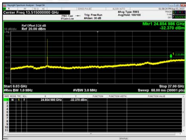
(802.11ac20) Tx. Spurious plot on channel 157
