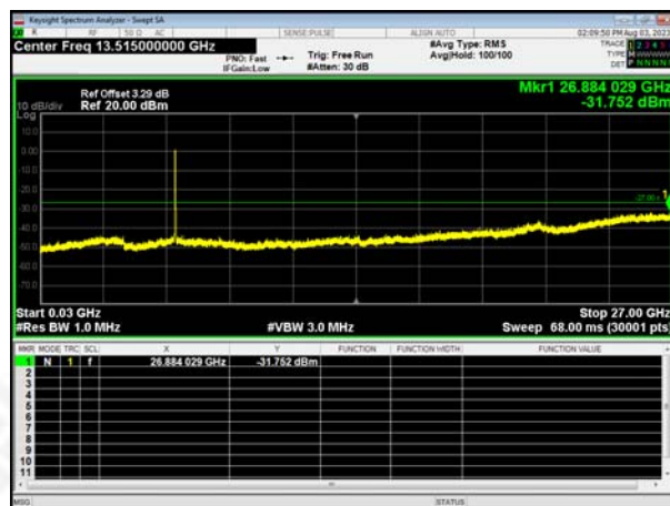
(802.11 ac40) Tx. Spurious plot on channel 159
