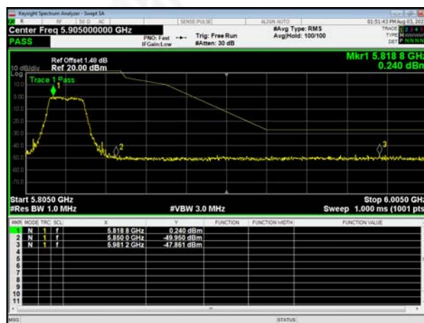
(802.11 n20) Highest channel
