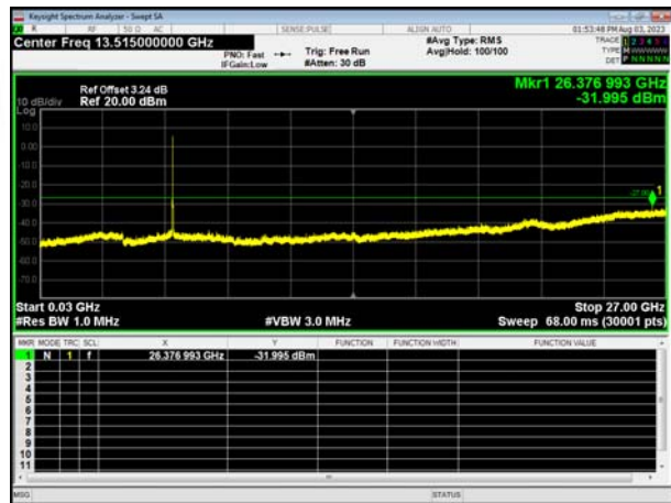
(802.11n20) Tx. Spurious plot on channel 157
