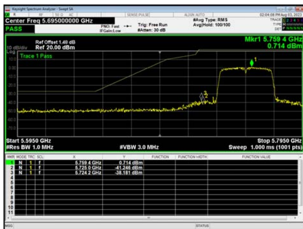
(802.11ac40) Lowest channel
