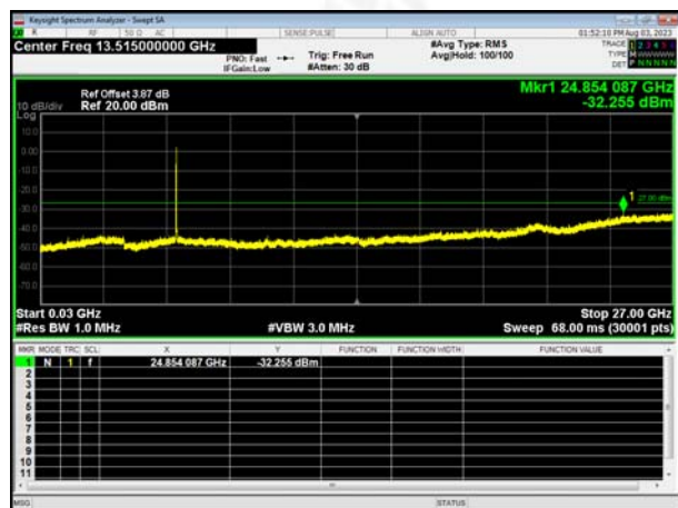
(802.11n20) Tx. Spurious plot on channel 165
