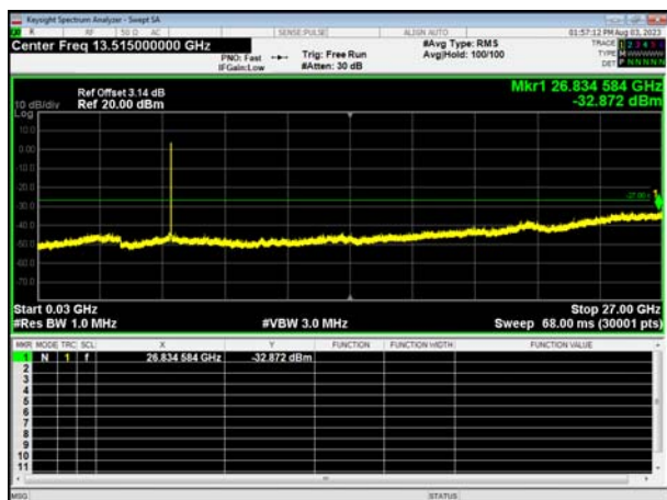
(802.11ac20) Tx. Spurious plot on channel 165
