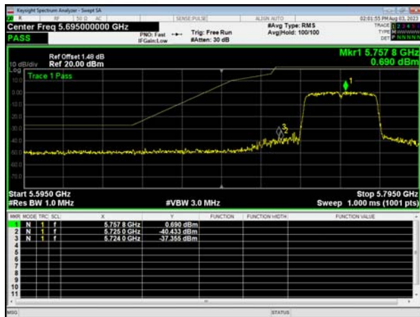
(802.11n40) Lowest channel
