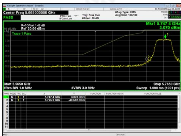
(802.11n20) Lowest channel
