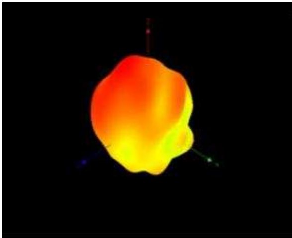
Frequency: 5800MHz Gain: 3.4dbi
