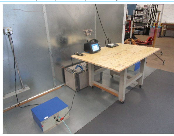
AC Mains Conducted Emissions
