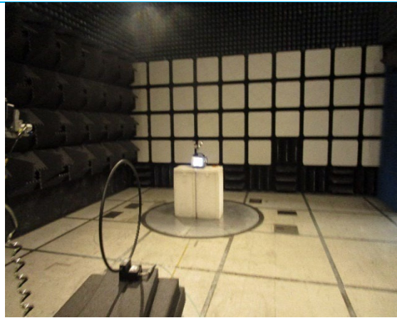
9 KHz-30 MHz – Perpendicular
