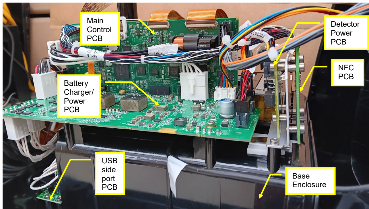
Figure 2 Front View - Base Enclosure with PCBs
