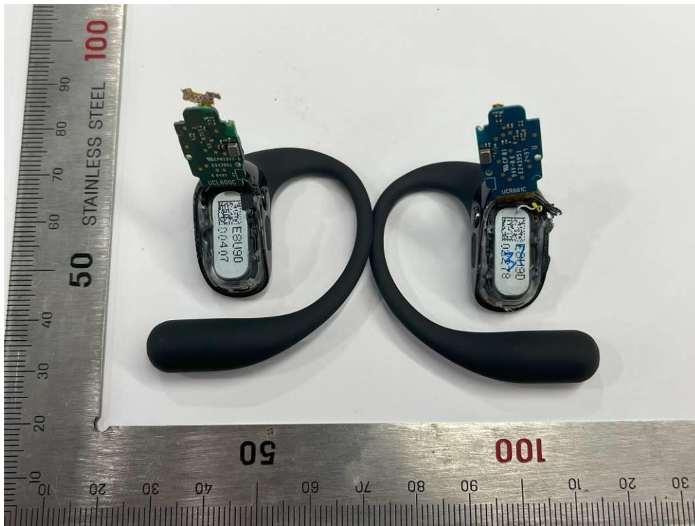
Fig. 2 Internal view 1 of earbuds
