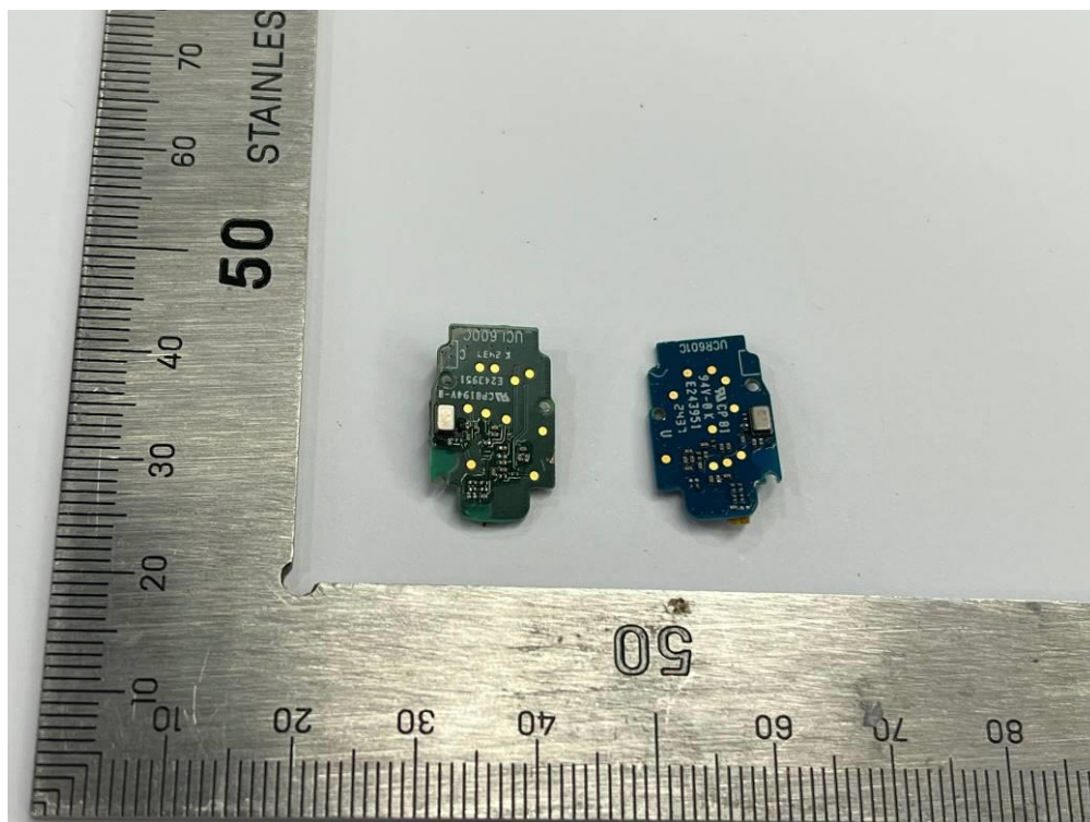
Fig. 4 PCB view 2 of earbuds
