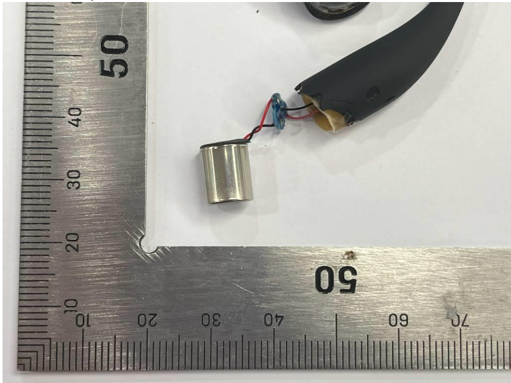
Fig. 7 Battery view 1 of earbuds
