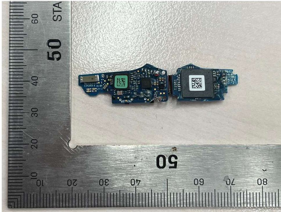
Fig. 1 PCB view 1
