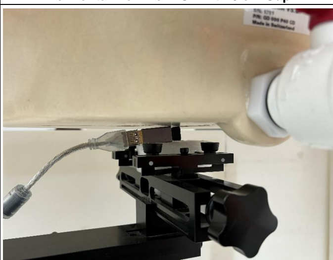
Vertical-Back of EUT with 0 cm Gap
