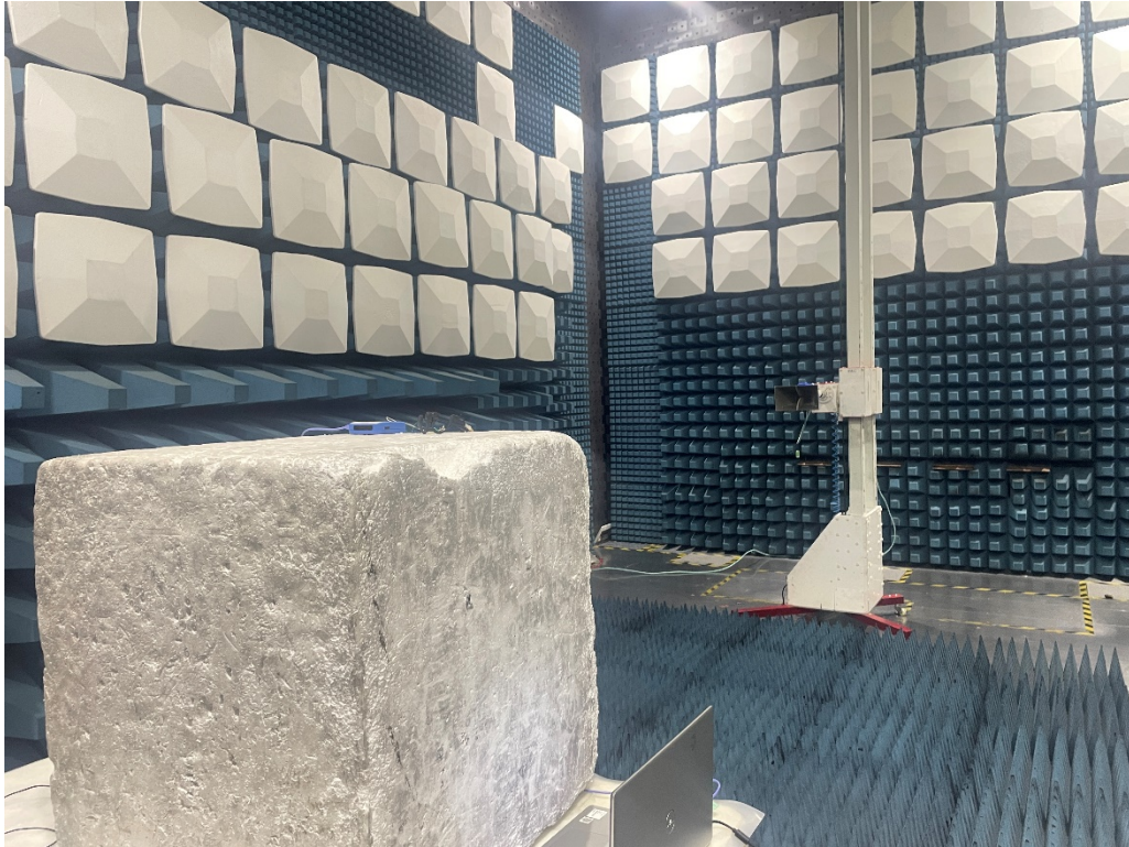
Photograph 3: Set-up for Radiated Spurious Emission, above 1GHz
