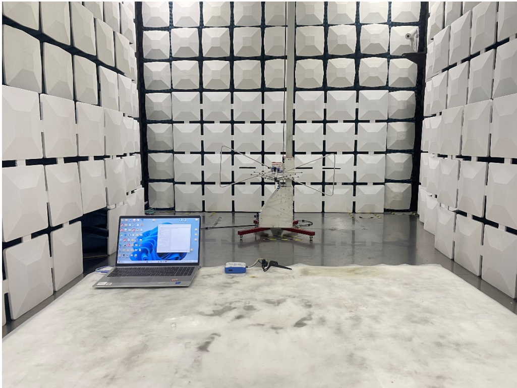
Photograph 2: Set-up for Radiated Spurious Emission, 30MHz - 1GHz
